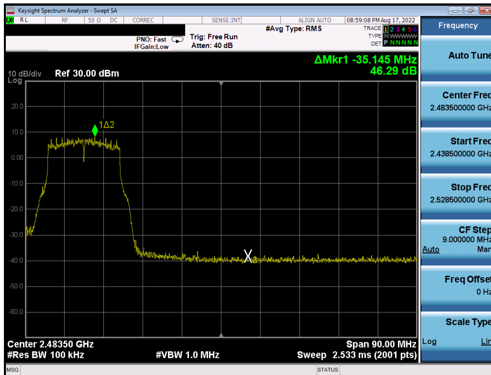
Plot 7-274. Band Edge Plot Antenna WF8 (802.11g - Ch.9) - 36Mbps
