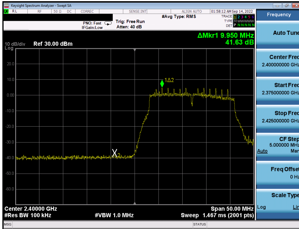
Plot 7-320. Band Edge Plot Antenna WF7 (802.11n (2.4GHz) - Ch. 1) - MCS2
