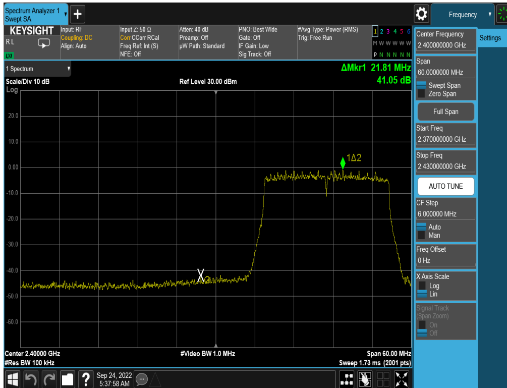
Plot 7-294. Band Edge Plot Antenna WF8 (802.11ax (SU - 2.4GHz) – Ch. 2) – MCS5
