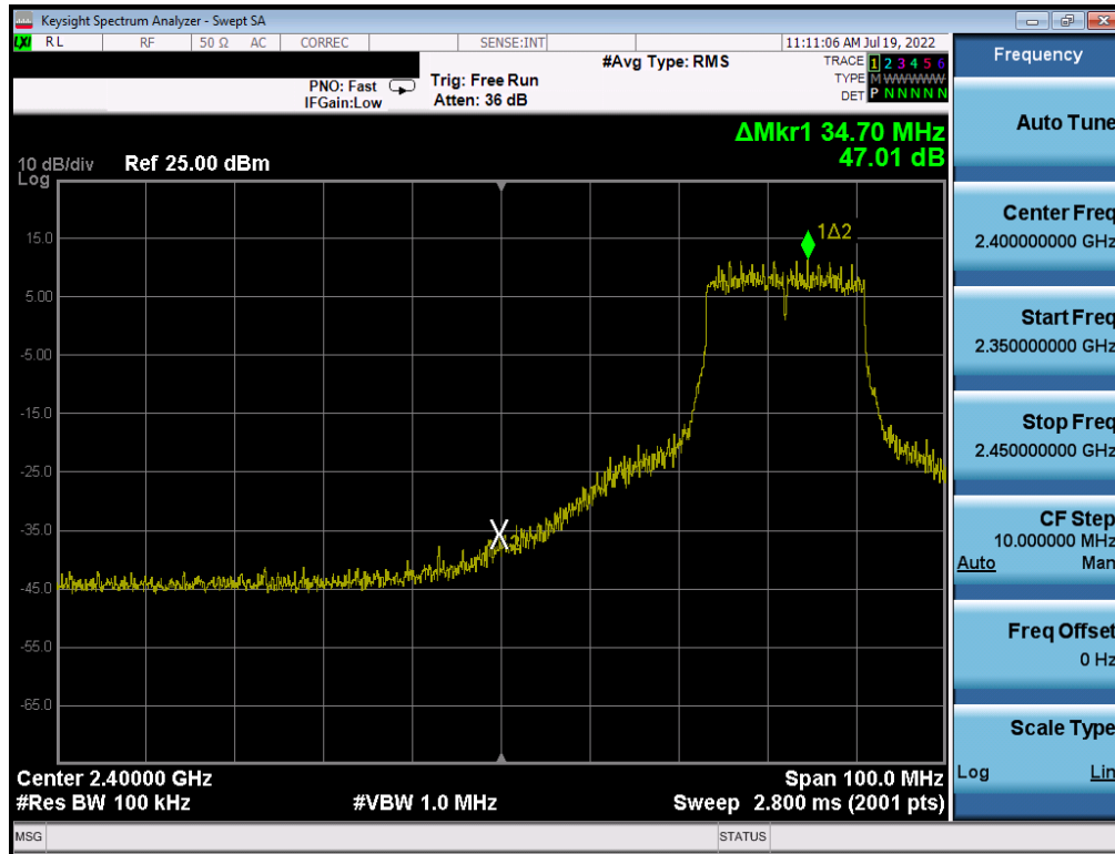
Plot 7-283. Band Edge Plot Antenna WF8 (802.11n (2.4GHz) - Ch. 5) - MCS5
