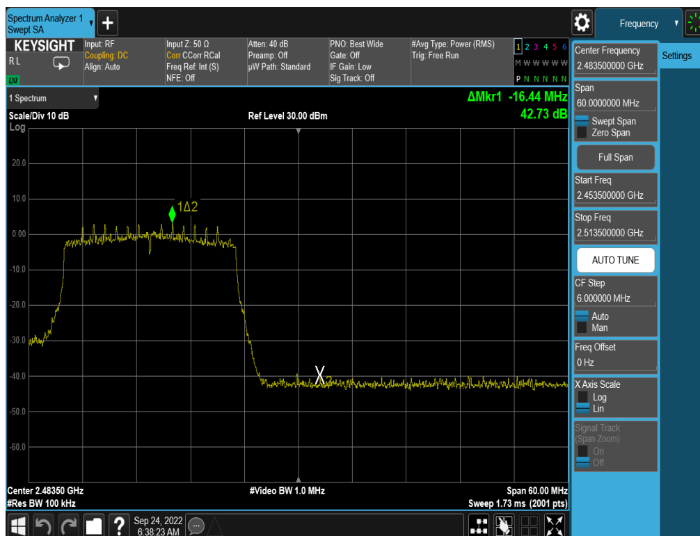
Plot 7- 346. Band Edge Plot Antenna WF7 (802.11ax (SU - 2.4GHz) – Ch. 12) – MCS2
