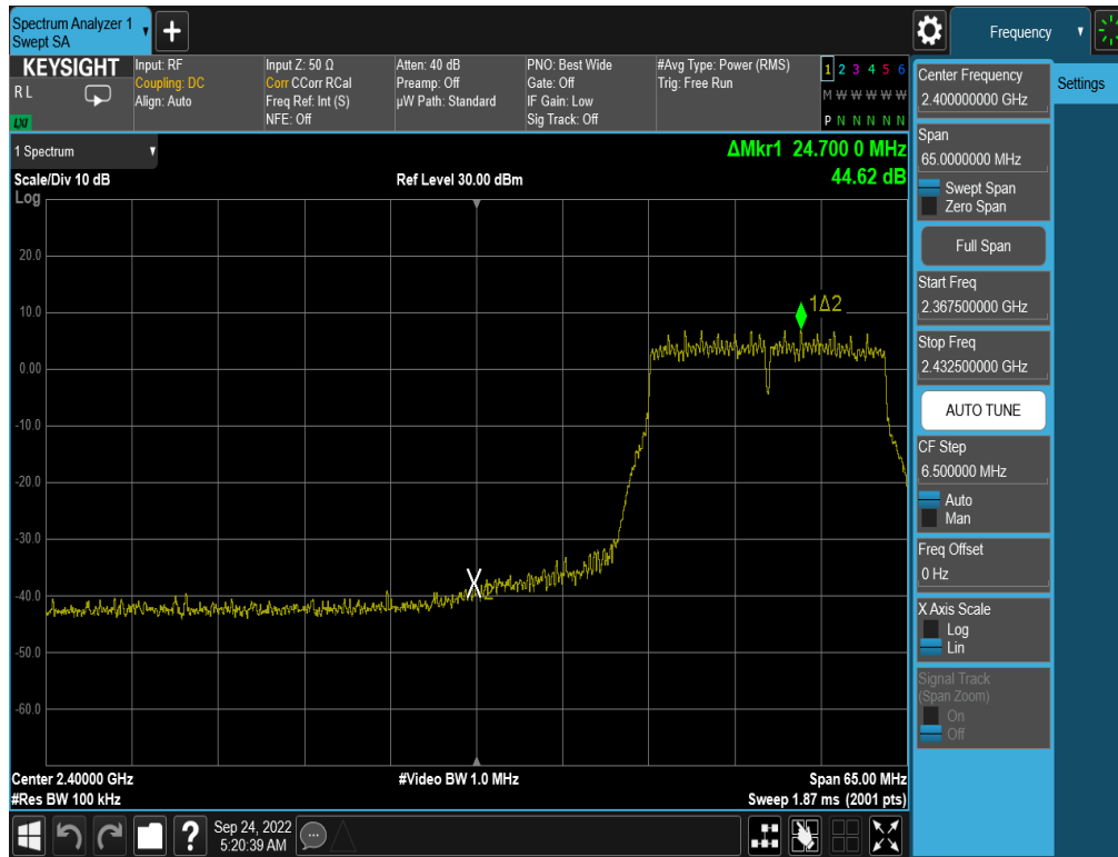
Plot 7-281. Band Edge Plot Antenna WF8 (802.11n (2.4GHz) – Ch. 3) – MCS5
