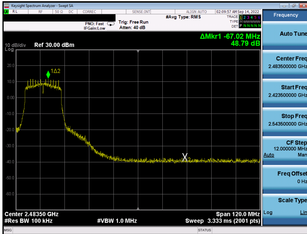
Plot 7-326 . Band Edge Plot Antenna WF7 (802.11n (2.4GHz) – Ch. 6 (high)) – MCS2
