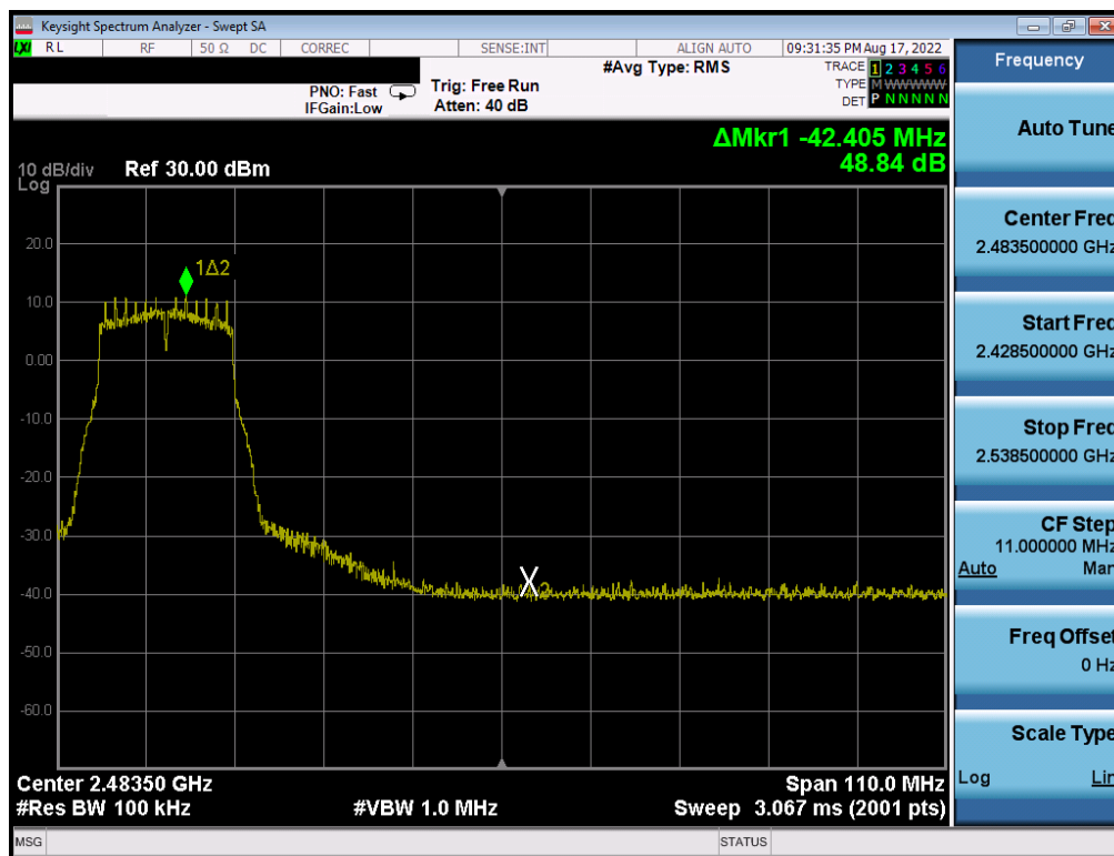
Plot 7-313 .Band Edge Plot Antenna WF7 (802.11g – Ch. 7) – 12Mbps
