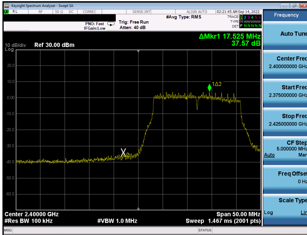
Plot 7-361 . Band Edge Plot Antenna WF7 (802.11n (2.4GHz) - Ch. 1) - MCS3
