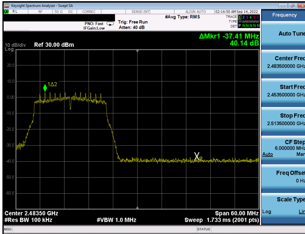
Plot 7-332 . Band Edge Plot Antenna WF7 (802.11n (2.4GHz) - Ch. 12) - MCS2
