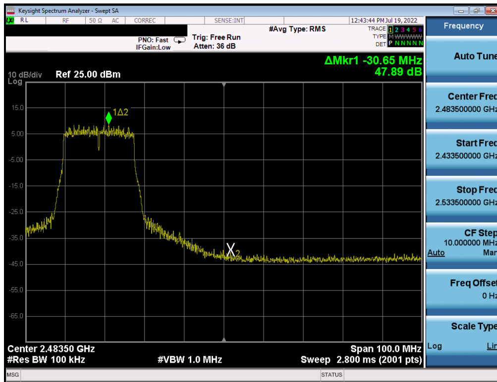
Plot 7-288. Band Edge Plot Antenna WF8 (802.11n (2.4GHz) - Ch. 9) - MCS5
