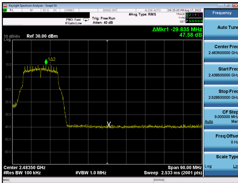
Plot 7-315. Band Edge Plot Antenna WF7 (802.11g - Ch. 9) - 12Mbps
