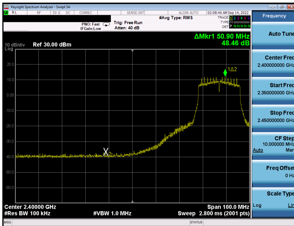
Plot 7-325. Band Edge Plot Antenna WF7 (802.11n (2.4GHz) - Ch. 6 (low)) - MCS2
