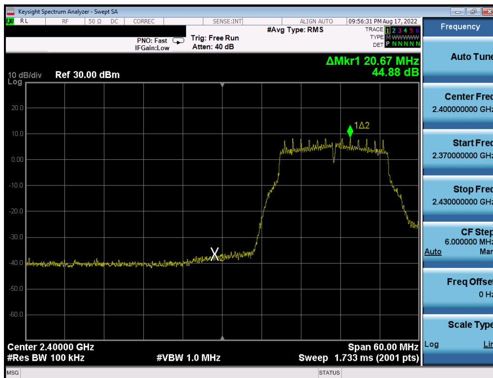
Plot 7- 348. Band Edge Plot Antenna WF7 (802.11g – Ch. 2) – 18Mbps
