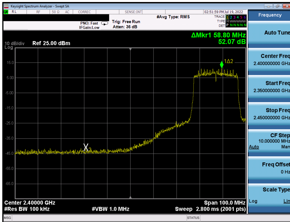
Plot 7- 339. Band Edge Plot Antenna WF7 (802.11ax (SU - 2.4GHz) – Ch. 6 (low)) – MCS2
