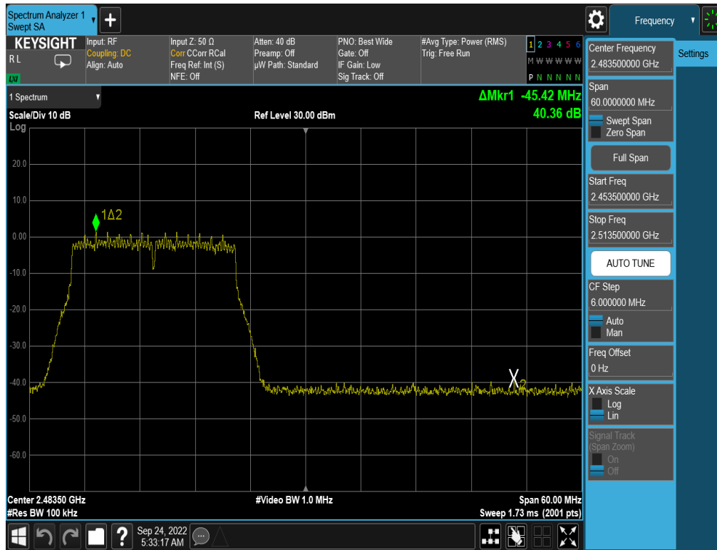
Plot 7-291. Band Edge Plot Antenna WF8 (802.11n (2.4GHz) – Ch. 12) – MCS5
