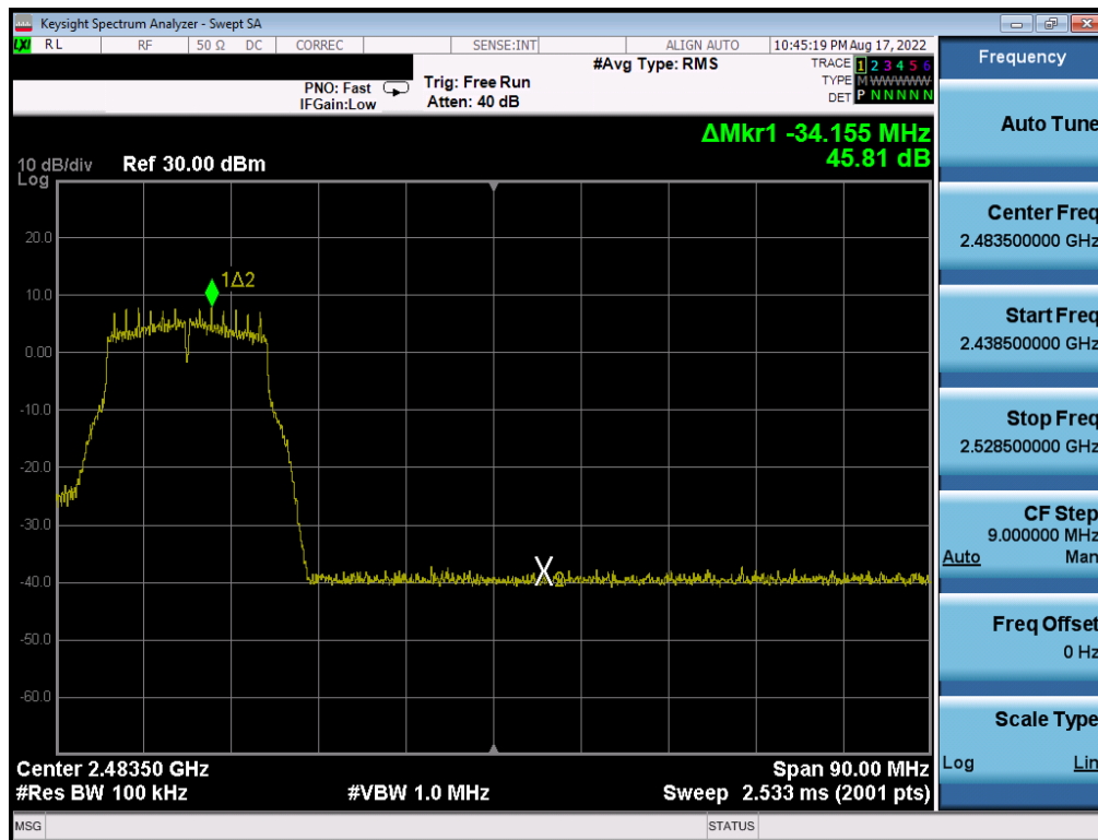
Plot 7-356 . Band Edge Plot Antenna WF7 (802.11g - Ch. 9) - 18Mbps
