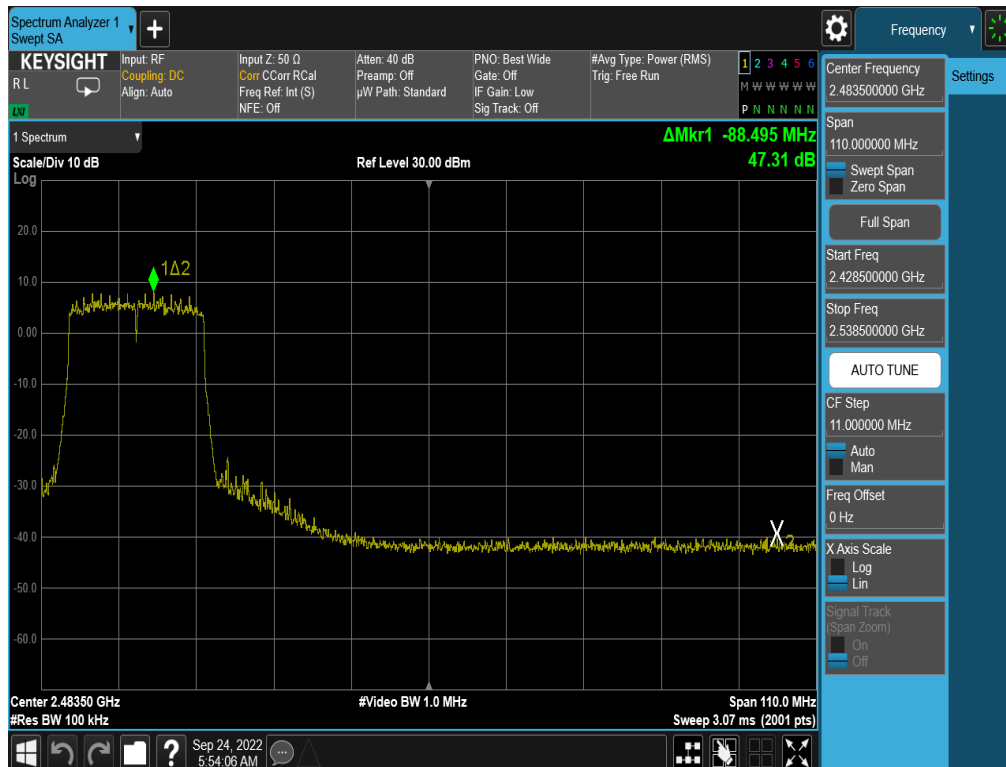
Plot 7-300. Band Edge Plot Antenna WF8 (802.11ax (SU - 2.4GHz) – Ch. 7) – MCS5
