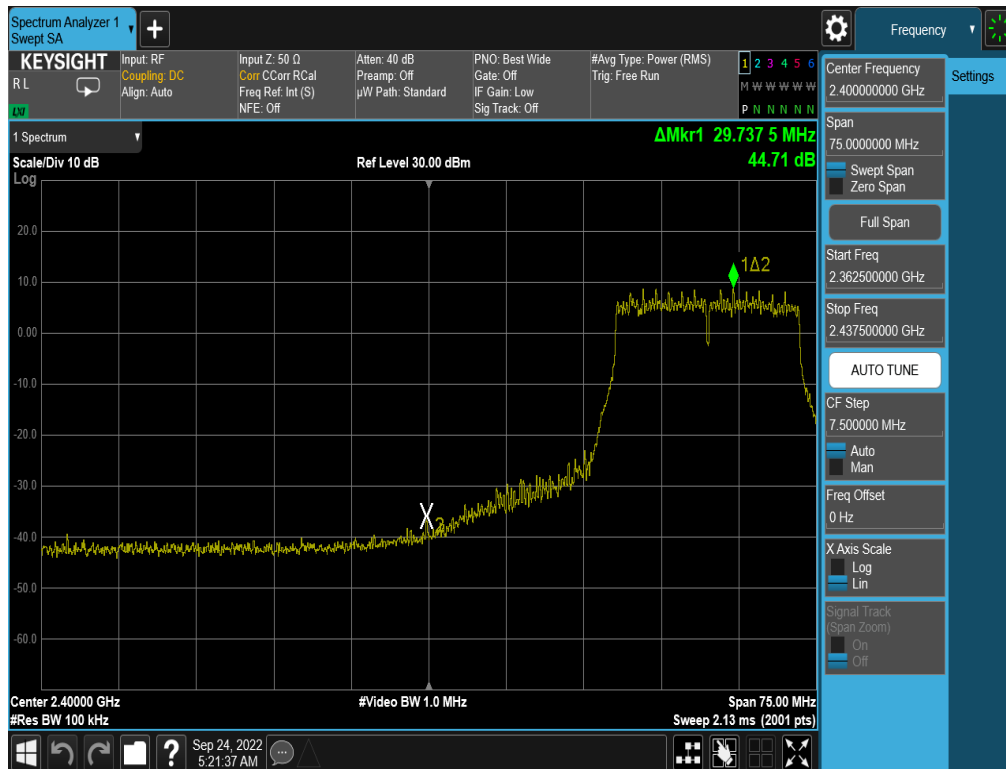
Plot 7-282. Band Edge Plot Antenna WF8 (802.11n (2.4GHz) – Ch. 4) – MCS5
