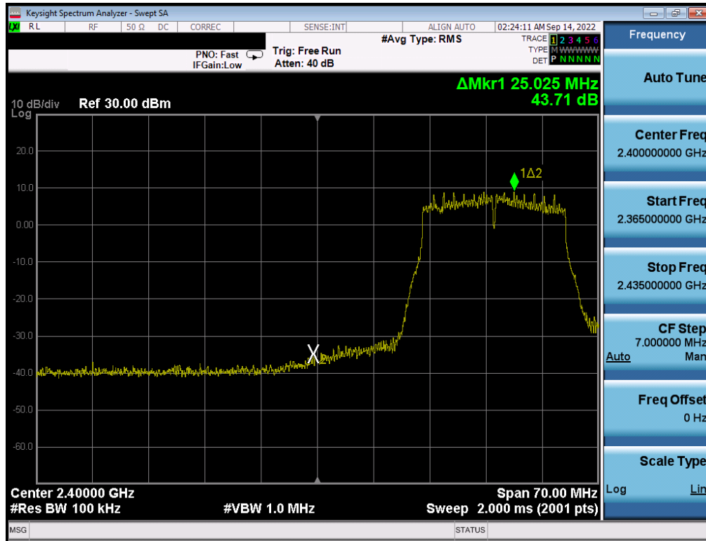
Plot 7-363 . Band Edge Plot Antenna WF7 (802.11n (2.4GHz) – Ch. 3) – MCS3
