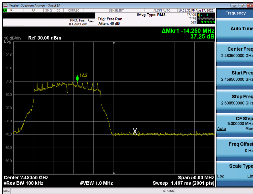
Plot 7-360 . Band Edge Plot Antenna WF7 (802.11g - Ch. 13) - 18Mbps
