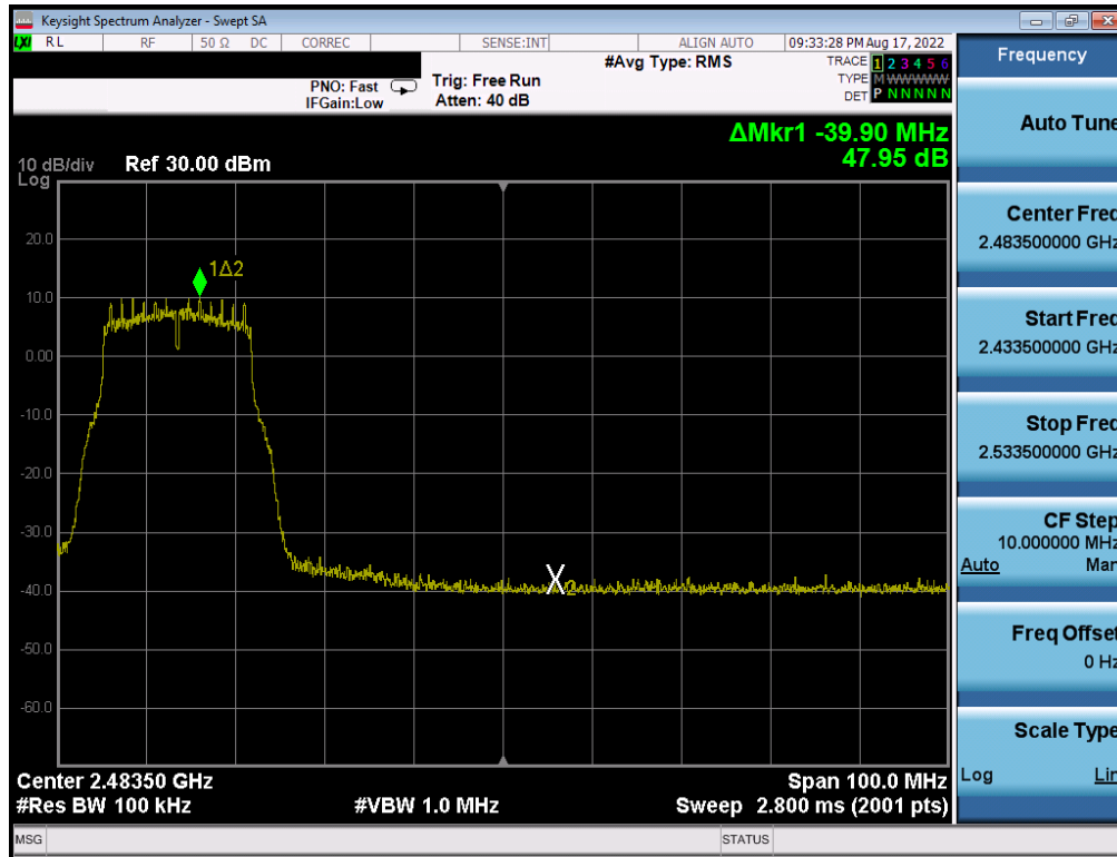
Plot 7-314. Band Edge Plot Antenna WF7 (802.11g - Ch. 8) - 12Mbps
