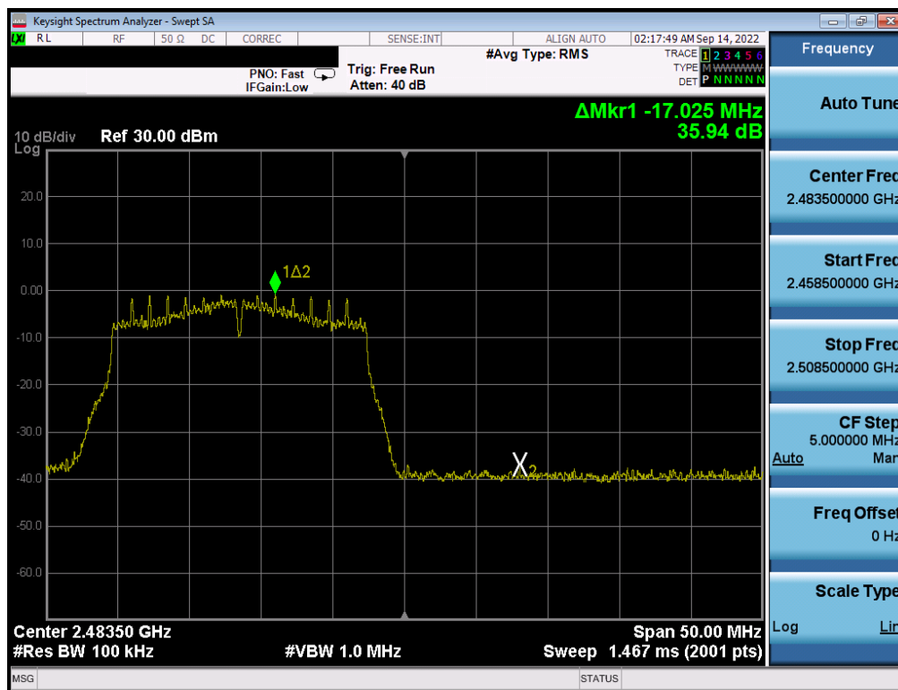
Plot 7-333 . Band Edge Plot Antenna WF7 (802.11n (2.4GHz) - Ch. 13) - MCS2
