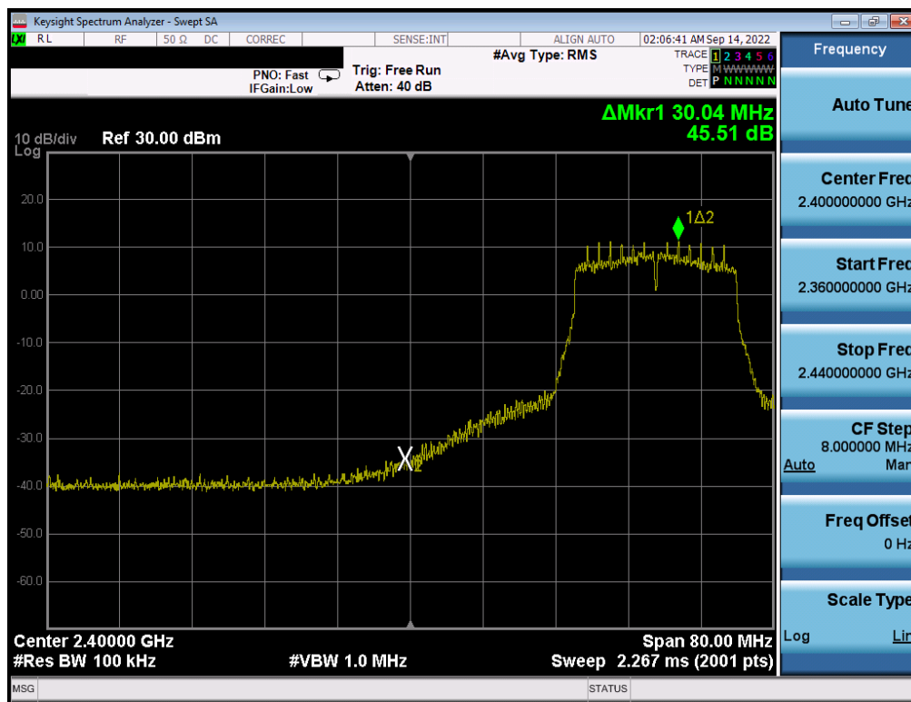
Plot 7-323. Band Edge Plot Antenna WF7 (802.11n (2.4GHz) - Ch. 4) - MCS2
