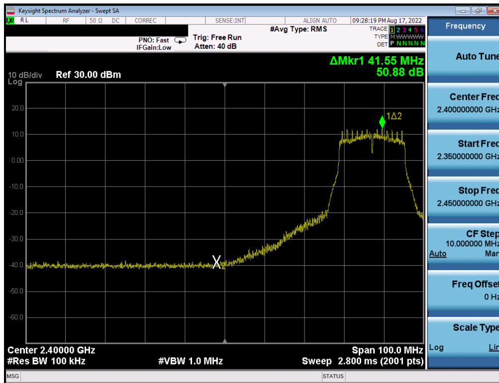
Plot 7-311. Band Edge Plot Antenna WF7 (802.11g – Ch. 6 (low)) – 12Mbps
