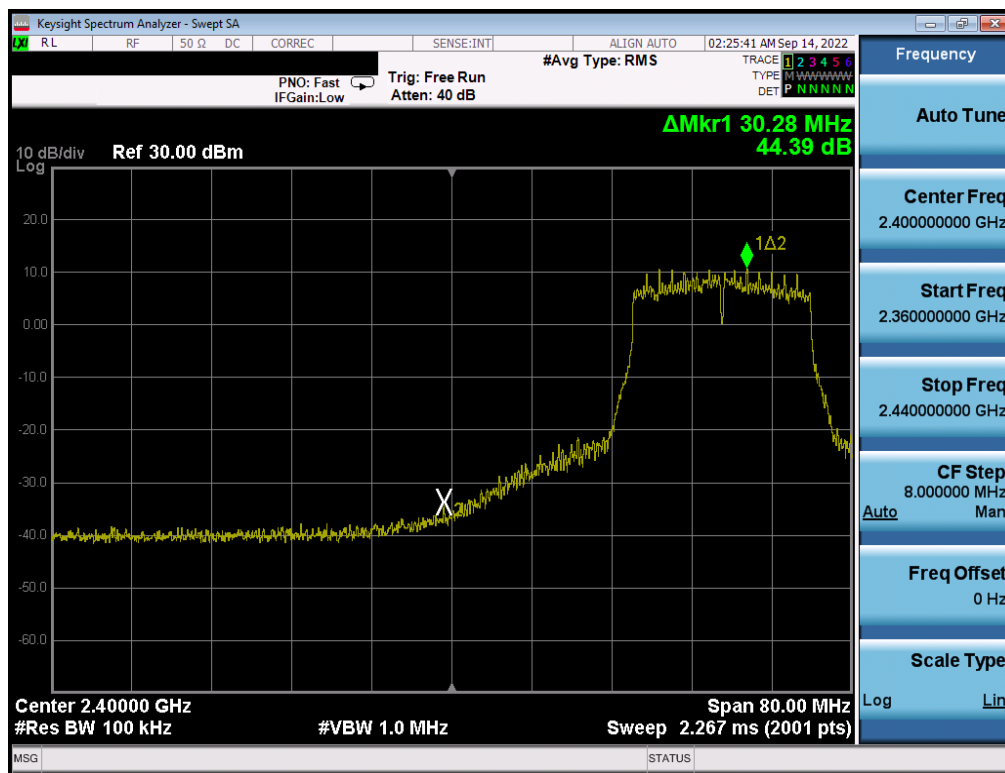
Plot 7- 364. Band Edge Plot Antenna WF7 (802.11n (2.4GHz) – Ch. 4) – MCS3
