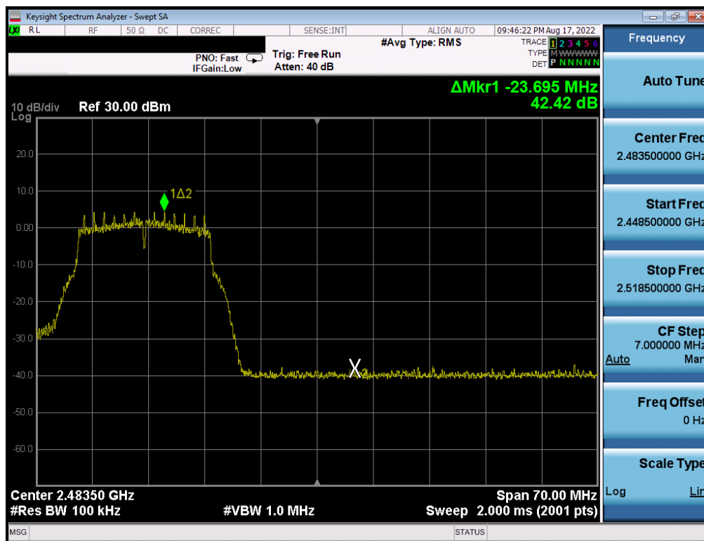
Plot 7-317. Band Edge Plot Antenna WF7 (802.11g - Ch. 11) - 12Mbps
