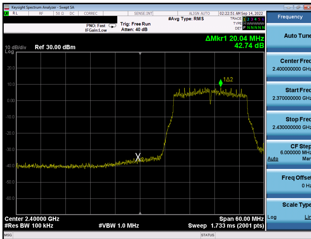
Plot 7-362 . Band Edge Plot Antenna WF7 (802.11n (2.4GHz) - Ch. 2) - MCS3
