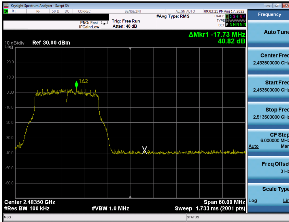
Plot 7-277. Band Edge Plot Antenna WF8 (802.11g - Ch. 12) - 36Mbps
