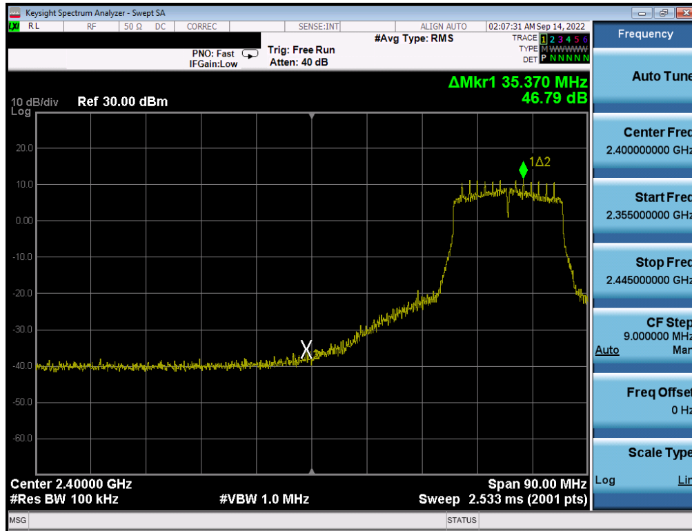
Plot 7-324. Band Edge Plot Antenna WF7 (802.11n (2.4GHz) - Ch. 5) - MCS2
