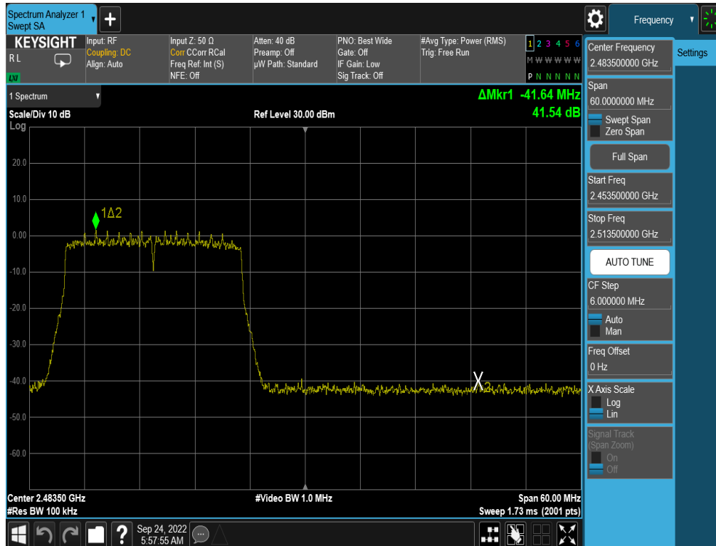
Plot 7-305. Band Edge Plot Antenna WF8 (802.11ax (SU - 2.4GHz) – Ch. 12) – MCS5
