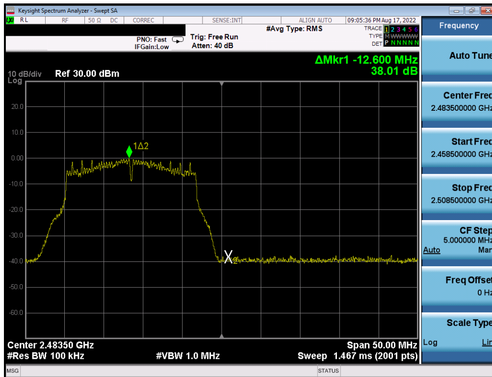
Plot 7-278. Band Edge Plot Antenna WF8 (802.11g - Ch. 13) - 36Mbps
