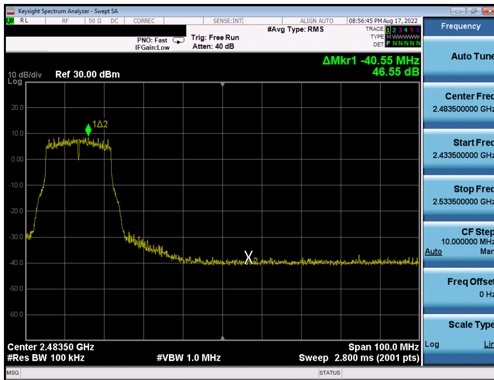
Plot 7-273. Band Edge Plot Antenna WF8 (802.11g - Ch. 8) - 36Mbps
