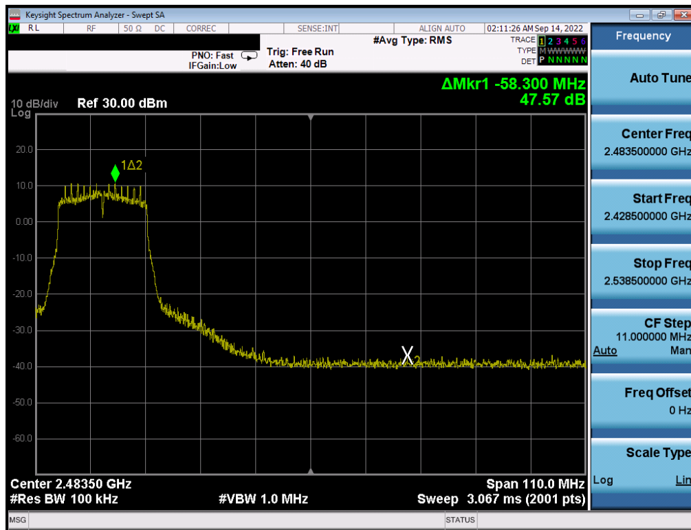
Plot 7- 327. Band Edge Plot Antenna WF7 (802.11n (2.4GHz) – Ch. 7) – MCS2
