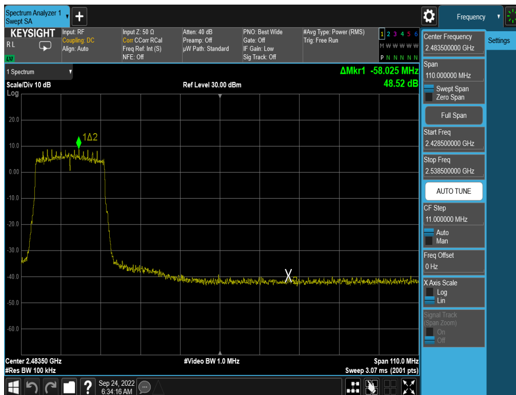
Plot 7-341 . Band Edge Plot Antenna WF7 (802.11ax (SU - 2.4GHz) – Ch. 7) – MCS2
