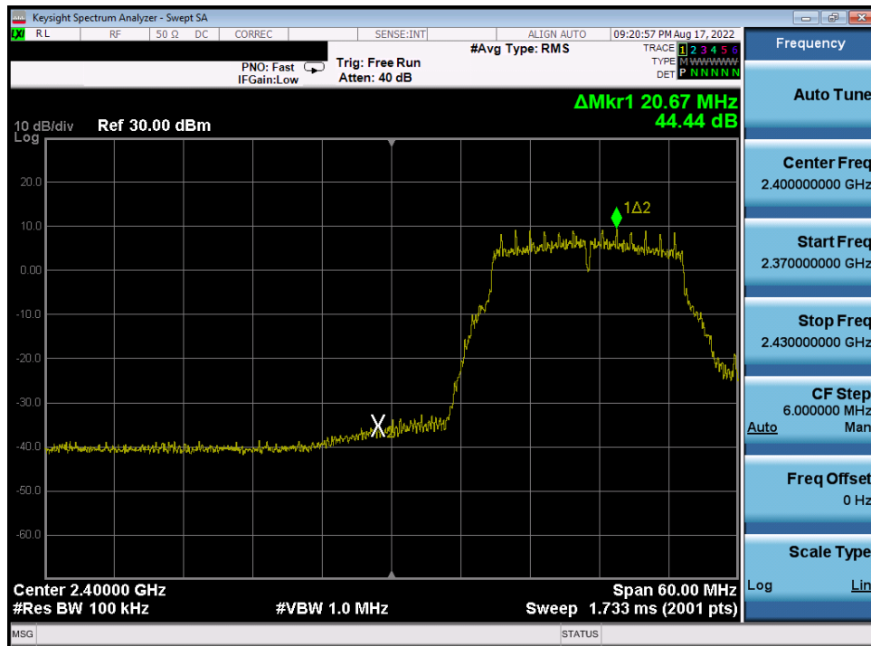
Plot 7-307. Band Edge Plot Antenna WF7 (802.11g – Ch. 2) – 12Mbps
