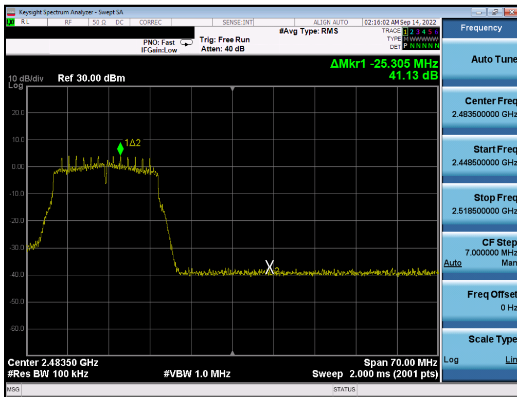
Plot 7-331 . Band Edge Plot Antenna WF7 (802.11n (2.4GHz) – Ch. 11) – MCS2
