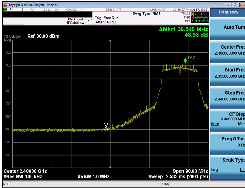
Plot 7-351 . Band Edge Plot Antenna WF7 (802.11g – Ch. 5) – 18Mbps
