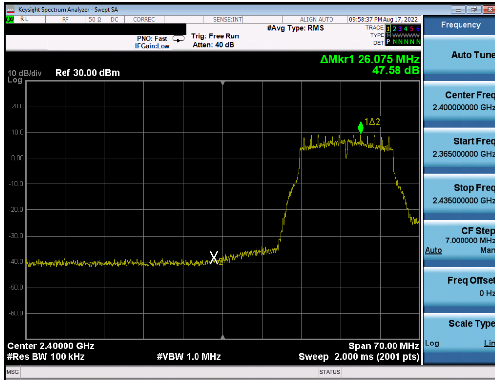
Plot 7-349 . Band Edge Plot Antenna WF7 (802.11g – Ch. 3) – 18Mbps
