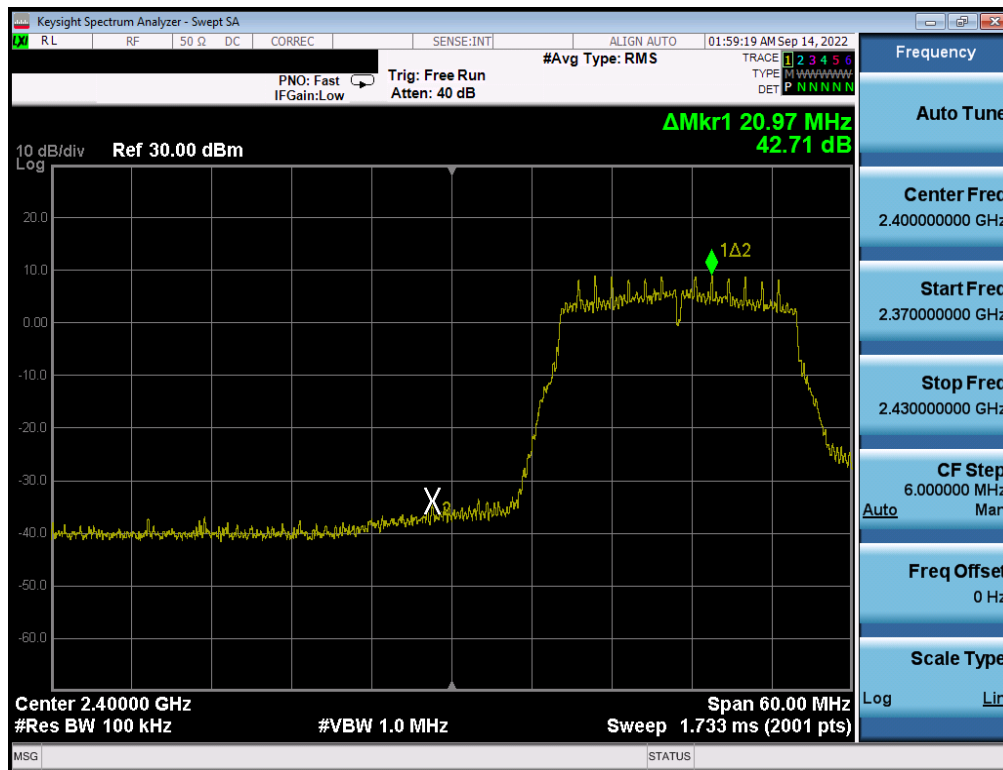
Plot 7-321. Band Edge Plot Antenna WF7 (802.11n (2.4GHz) - Ch. 2) - MCS2
