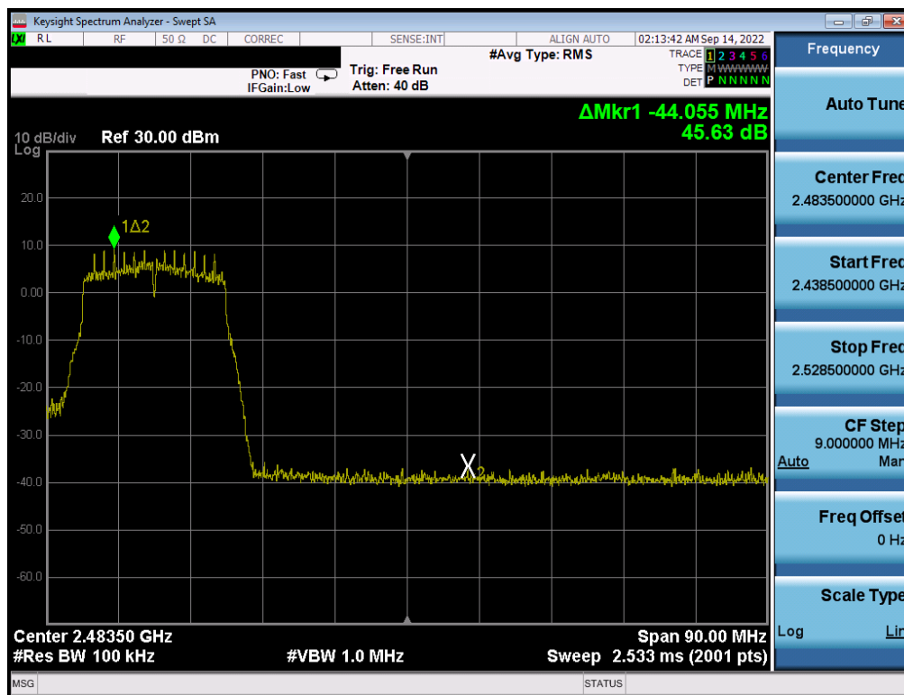
Plot 7-329 . Band Edge Plot Antenna WF7 (802.11n (2.4GHz) - Ch. 9) - MCS2
