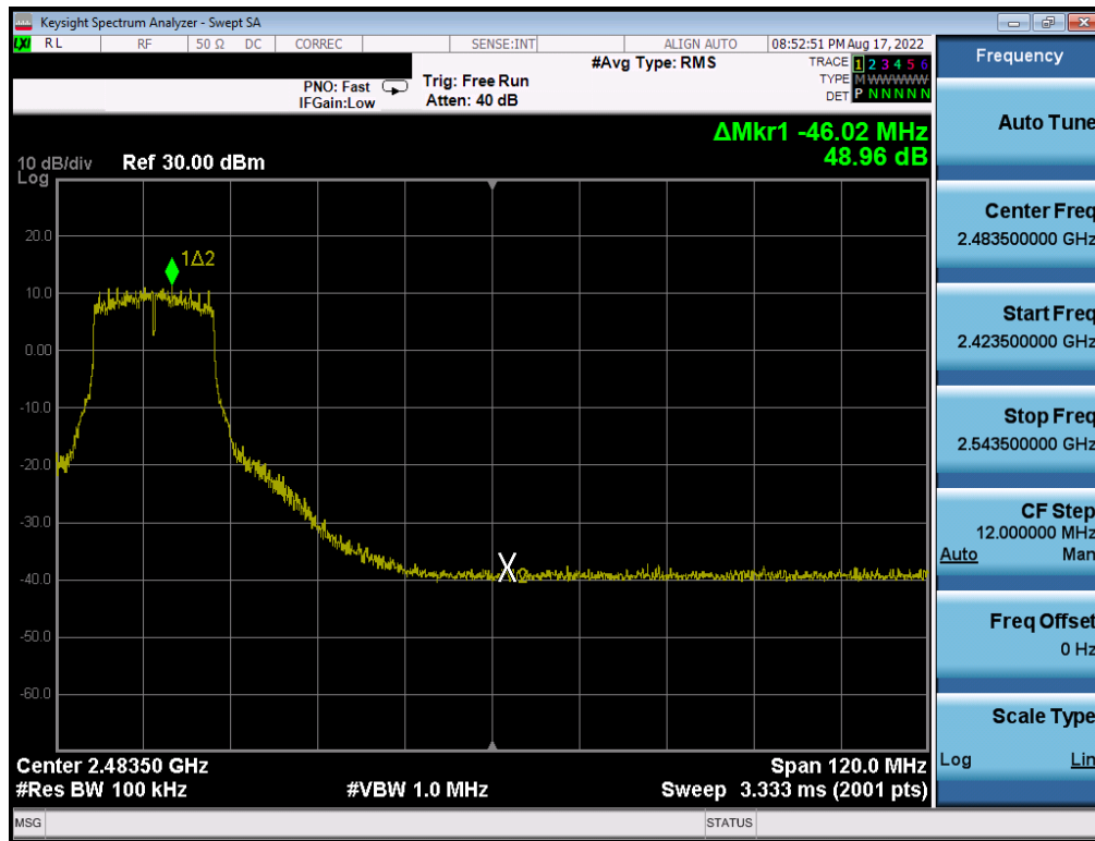
Plot 7-271. Band Edge Plot Antenna WF8 (802.11g – Ch. 6 (high)) – 36Mbps
