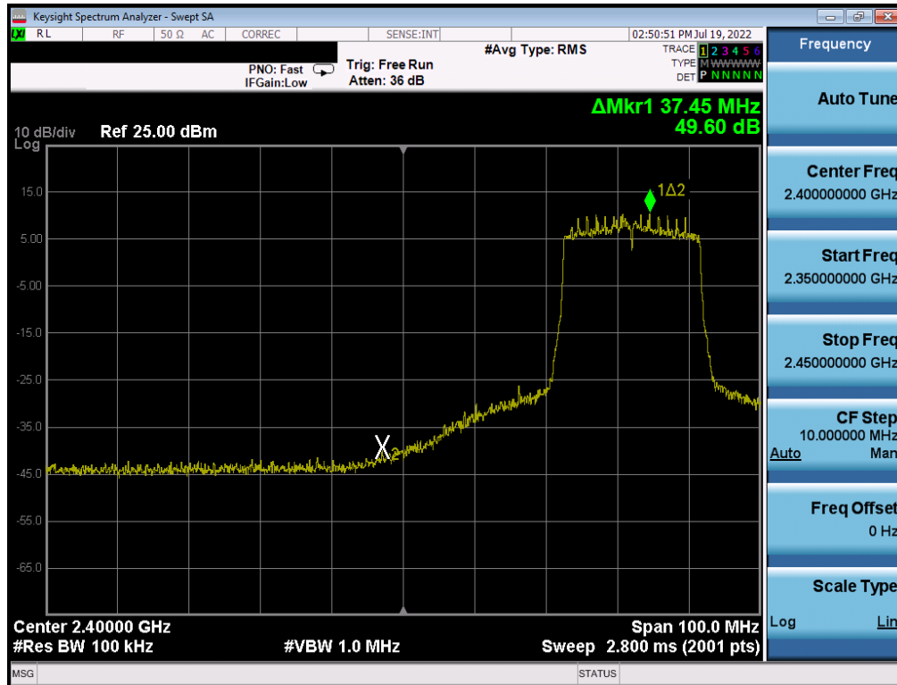
Plot 7-338 . Band Edge Plot Antenna WF7 (802.11ax (SU - 2.4GHz) – Ch. 5) – MCS2
