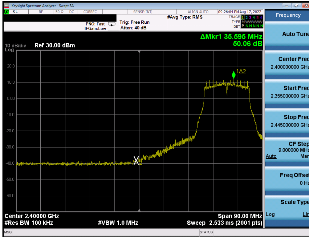
Plot 7-310. Band Edge Plot Antenna 2 WF7 (802.11g – Ch. 5) – 12Mbps
