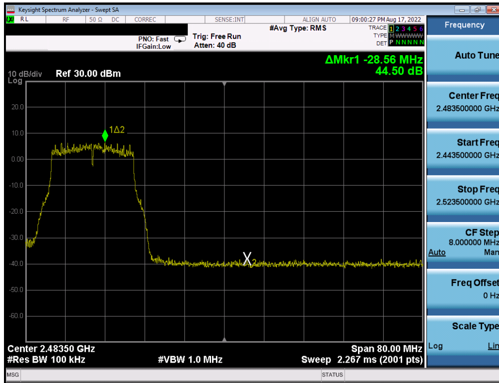
Plot 7-275. Band Edge Plot Antenna WF8 (802.11g - Ch. 10) - 36Mbps
