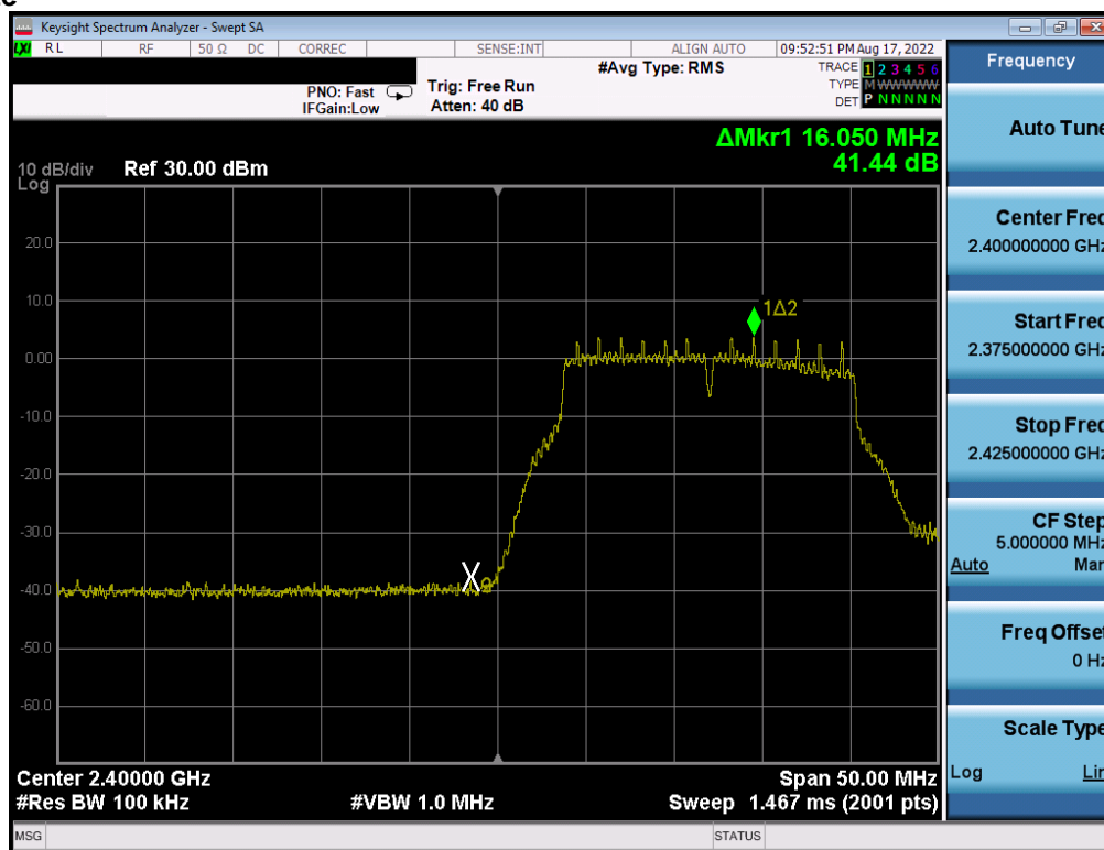
Plot 7-347 . Band Edge Plot Antenna WF7 (802.11g – Ch. 1) – 18Mbps
