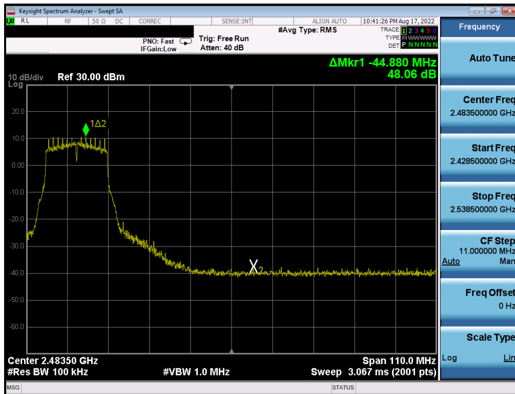
Plot 7-354 . Band Edge Plot Antenna WF7 (802.11g – Ch. 7) – 18Mbps
