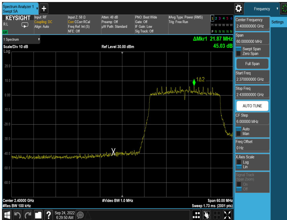
Plot 7-335 . Band Edge Plot Antenna WF7 (802.11ax (SU - 2.4GHz) – Ch. 2) – MCS2
