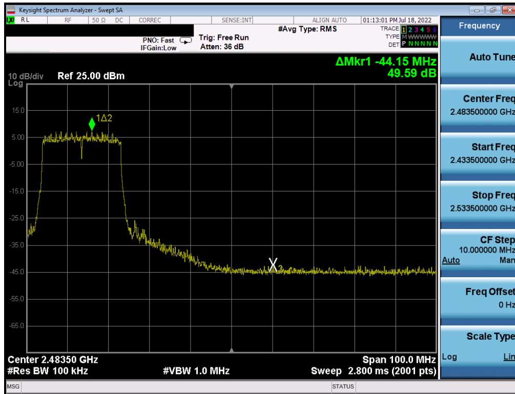
Plot 7-301. Band Edge Plot Antenna WF8 (802.11ax (SU - 2.4GHz) – Ch. 8) – MCS5
