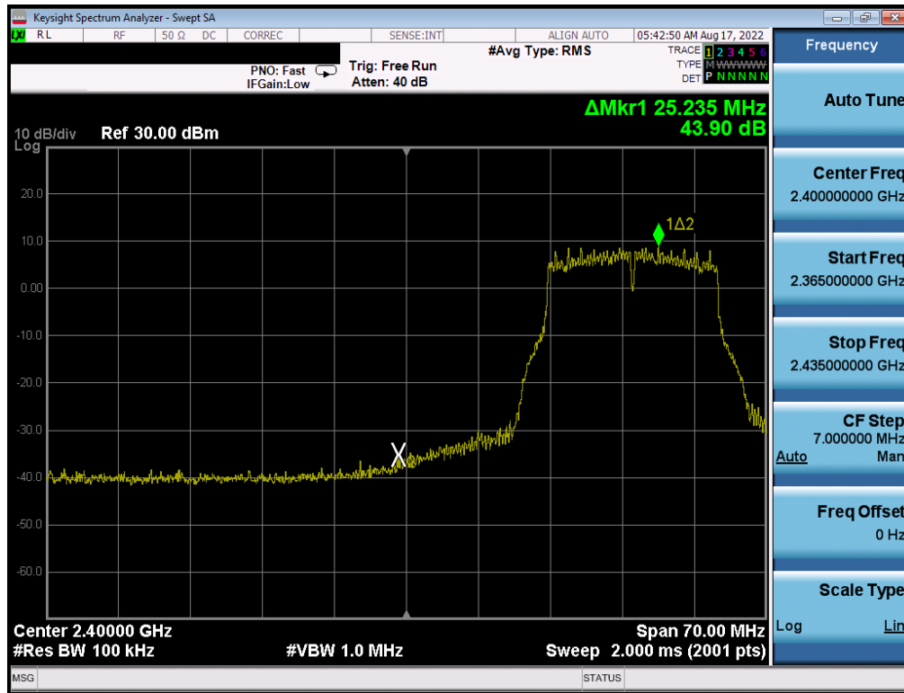
Plot 7-267. Band Edge Plot Antenna WF8 (802.11g – Ch. 3) – 36Mbps
