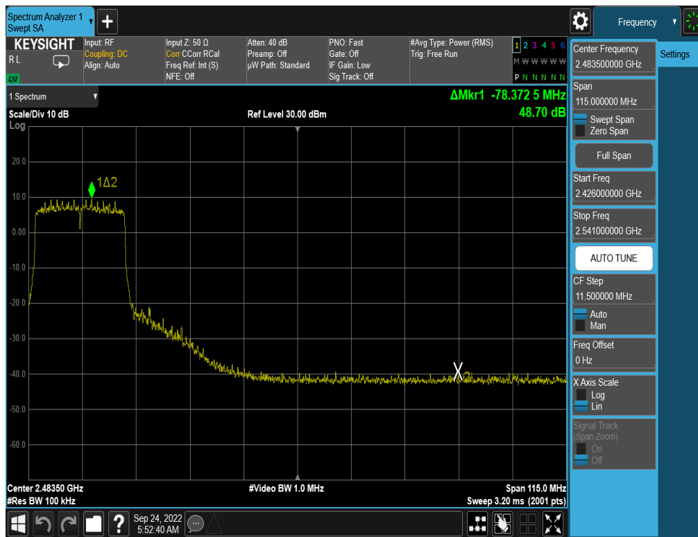
Plot 7-299. Band Edge Plot Antenna WF8 (802.11ax (SU - 2.4GHz) – Ch. 6 (high)) – MCS5
