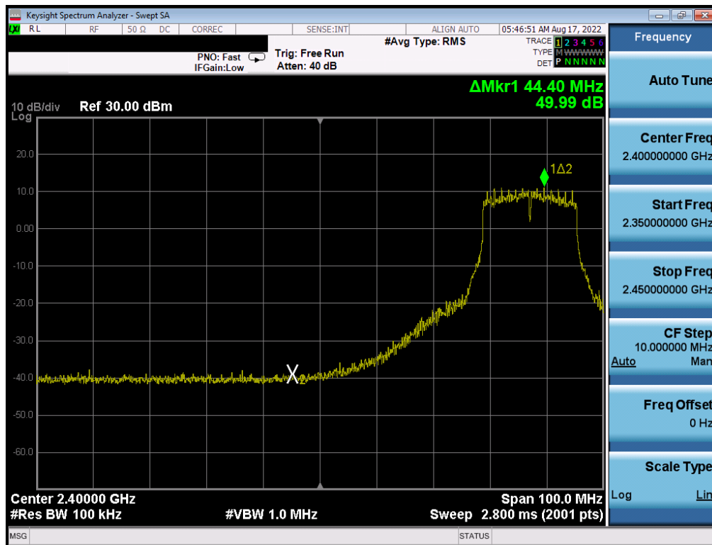
Plot 7-270. Band Edge Plot Antenna WF8 (802.11g – Ch. 6 (low)) – 36Mbps
