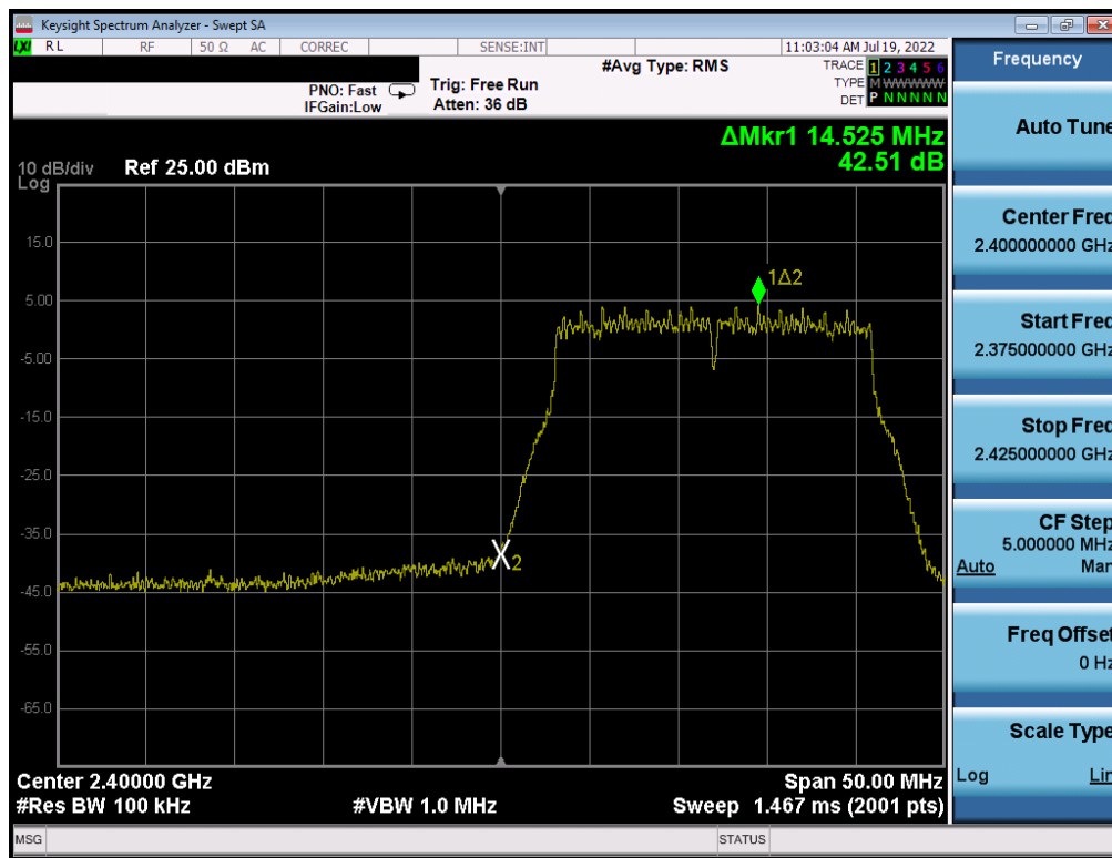
Plot 7-279. Band Edge Plot Antenna WF8 (802.11n (2.4GHz) – Ch. 1) – MCS5
