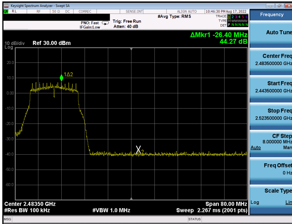
Plot 7- 357. Band Edge Plot Antenna WF7 (802.11g – Ch. 10) – 18Mbps
