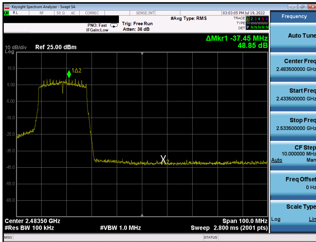
Plot 7-343 . Band Edge Plot Antenna WF7 (802.11ax (SU - 2.4GHz) – Ch. 9) – MCS2
