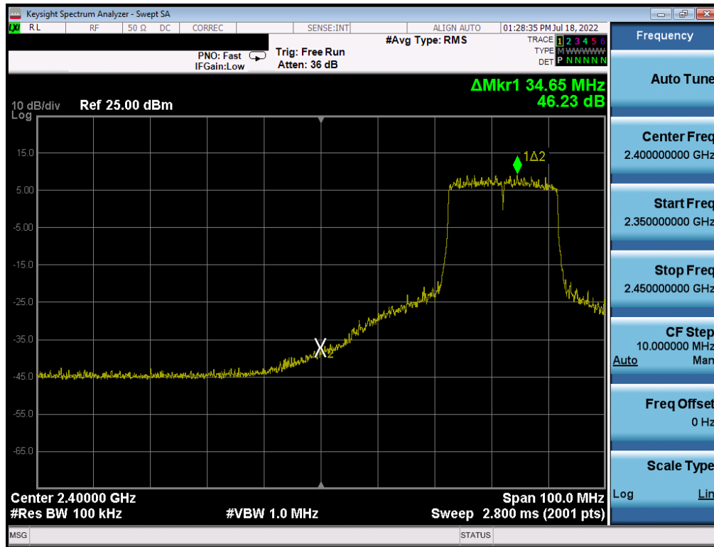
Plot 7-297. Band Edge Plot Antenna WF8 (802.11ax (SU - 2.4GHz) – Ch. 5) – MCS5
