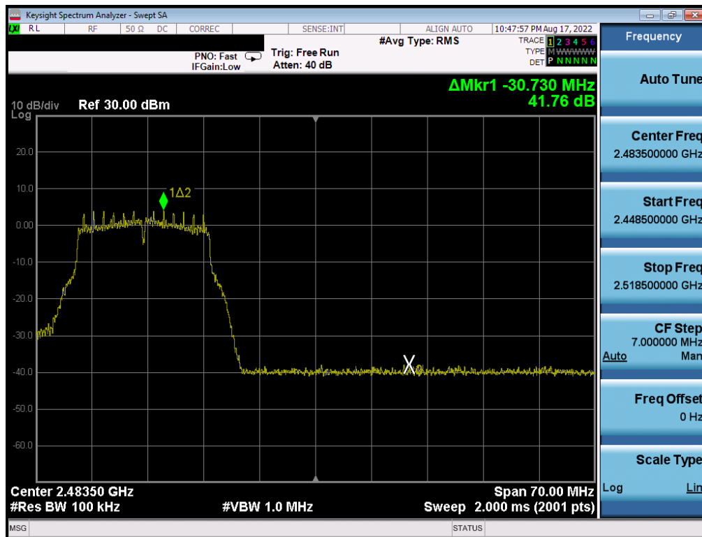
Plot 7- 358. Band Edge Plot Antenna WF7 (802.11g – Ch. 11) – 18Mbps
