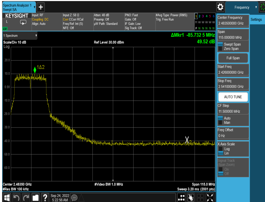
Plot 7-285. Band Edge Plot Antenna WF8 (802.11n (2.4GHz) – Ch. 6 (high)) – MCS5
