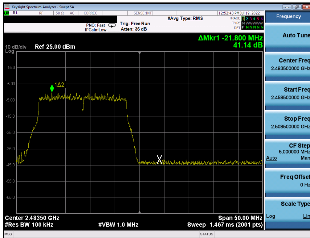
Plot 7-292. Band Edge Plot Antenna WF8 (802.11n (2.4GHz) – Ch. 13) – MCS5
