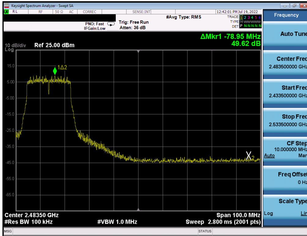
Plot 7-287. Band Edge Plot Antenna WF8 (802.11n (2.4GHz) - Ch. 8) - MCS5
