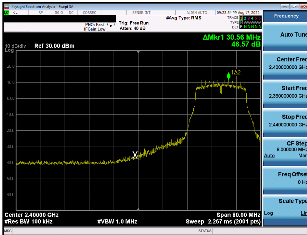
Plot 7-309. Band Edge Plot Antenna 2 WF7 (802.11g - Ch. 4) - 12Mbps
