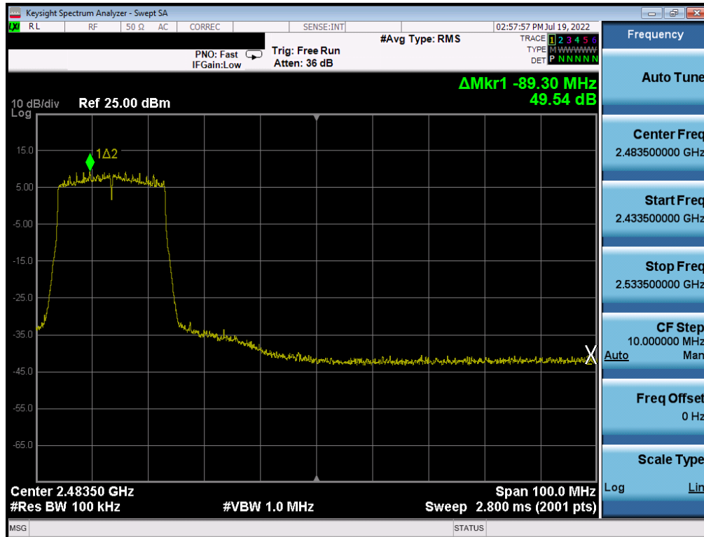
Plot 7-342 . Band Edge Plot Antenna WF7 (802.11ax (SU - 2.4GHz) – Ch. 8) – MCS2
