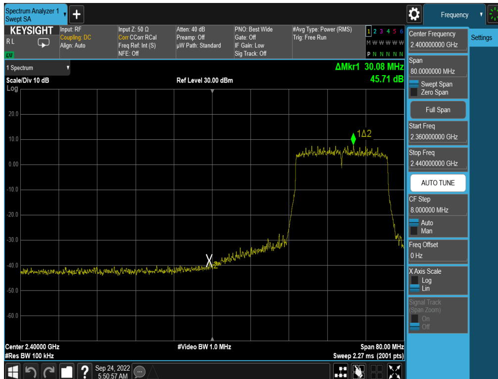
Plot 7-296. Band Edge Plot Antenna WF8 (802.11ax (SU - 2.4GHz) – Ch. 4) – MCS5
