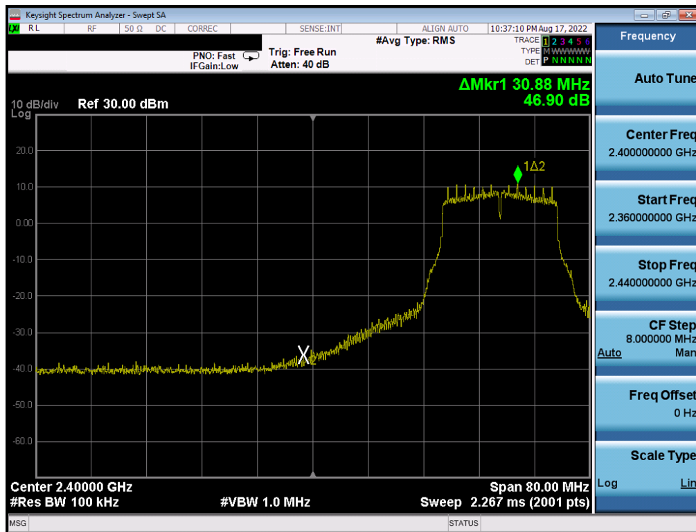
Plot 7-350 . Band Edge Plot Antenna WF7 (802.11g – Ch. 4) – 18Mbps
