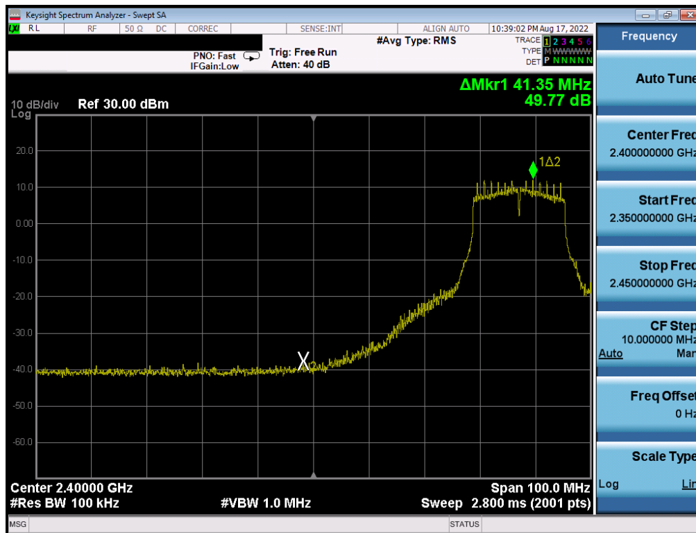
Plot 7-352 . Band Edge Plot Antenna WF7 (802.11g – Ch. 6 (low)) – 18Mbps
