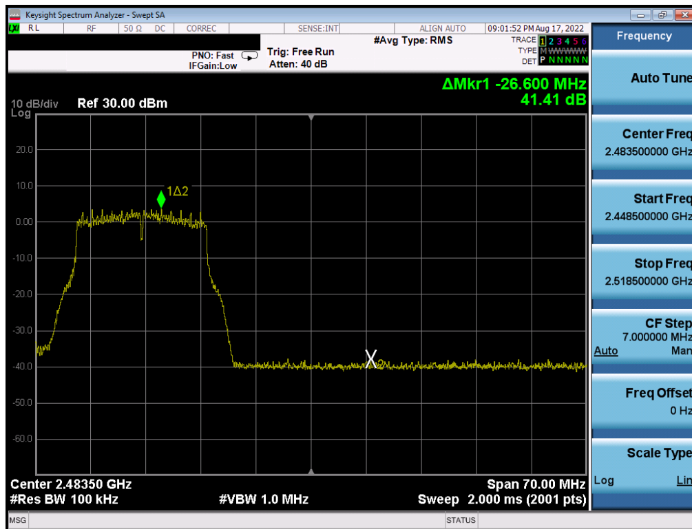
Plot 7-276. Band Edge Plot Antenna WF8 (802.11g - Ch. 11) - 36Mbps
