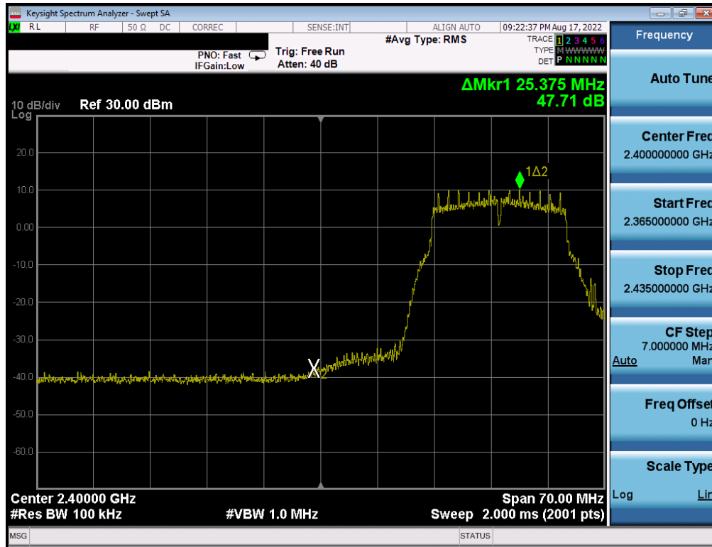
Plot 7-308. Band Edge Plot Antenna WF7 (802.11g - Ch. 3) - 12Mbps
