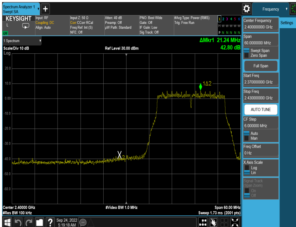
Plot 7-280. Band Edge Plot Antenna WF8 (802.11n (2.4GHz) – Ch. 2) – MCS5
