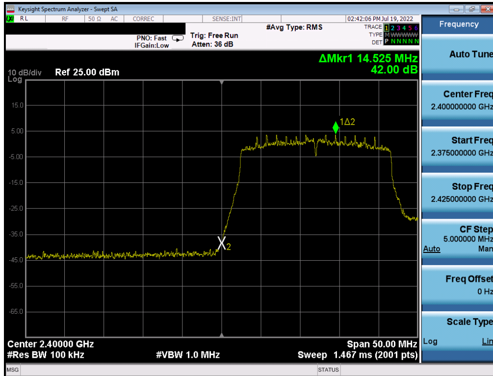
Plot 7-334 . Band Edge Plot Antenna WF7 (802.11ax (SU - 2.4GHz) – Ch. 1) – MCS2
