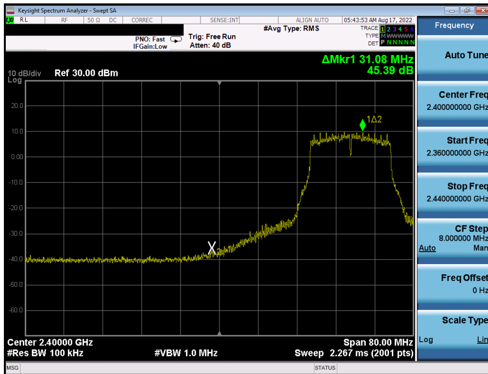
Plot 7-268. Band Edge Plot Antenna WF8 (802.11g – Ch. 4) – 36Mbps
