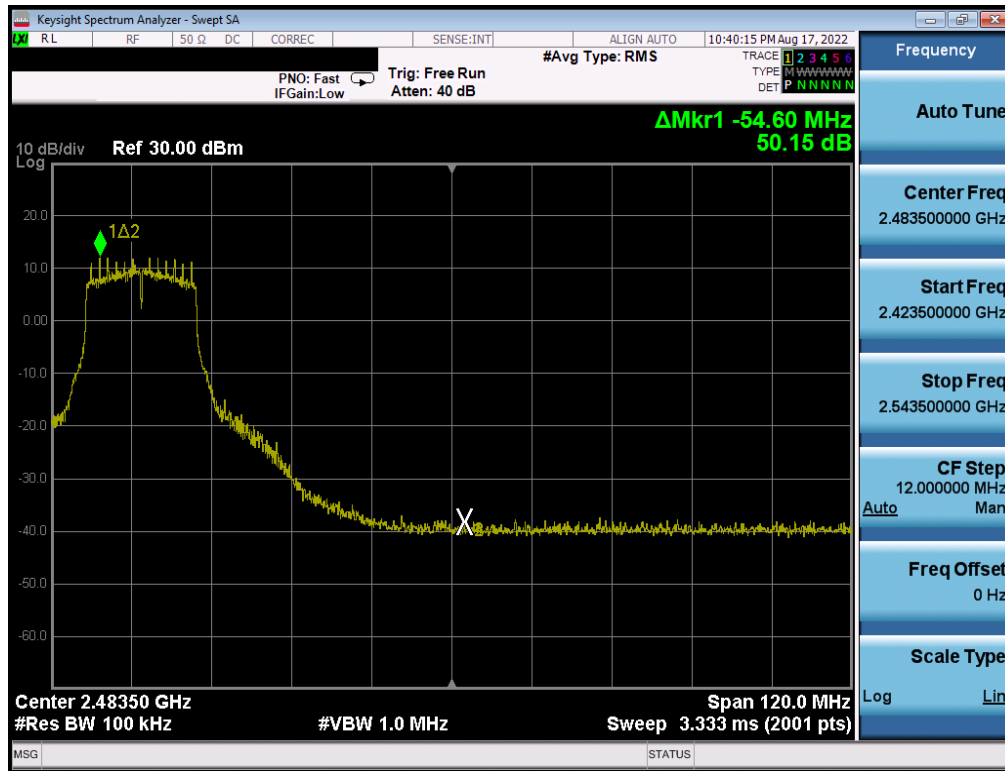
Plot 7-353 . Band Edge Plot Antenna WF7 (802.11g – Ch. 6 (high)) – 18Mbps
