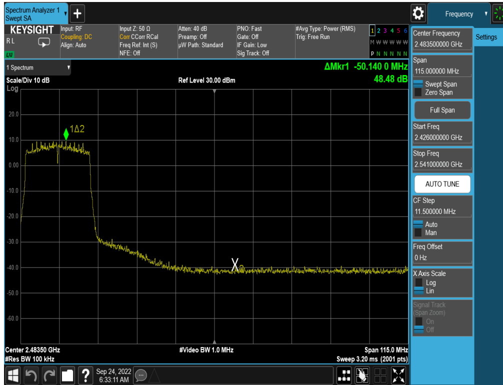
Plot 7-340 . Band Edge Plot Antenna WF7 (802.11ax (SU - 2.4GHz) – Ch. 6 (high) – MCS2
