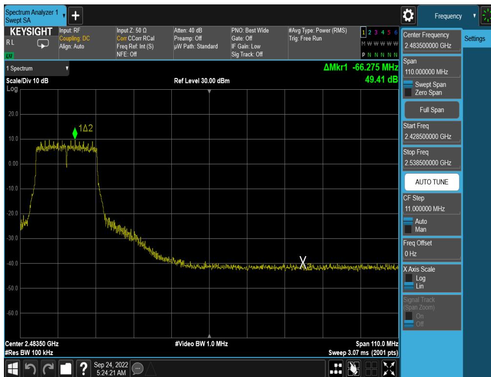
Plot 7-286. Band Edge Plot Antenna WF8 (802.11n (2.4GHz) – Ch. 7) – MCS5
