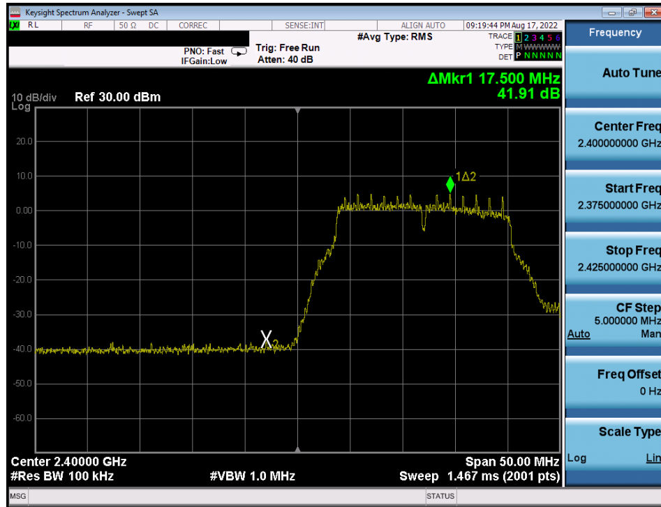
Plot 7-306. Band Edge Plot Antenna WF7 (802.11g – Ch. 1) – 12Mbps
