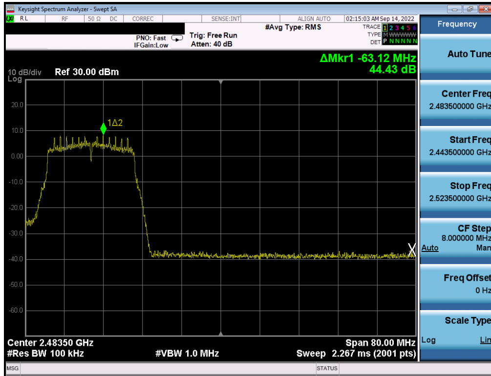
Plot 7-330 . Band Edge Plot Antenna WF7 (802.11n (2.4GHz) – Ch. 10) – MCS2
