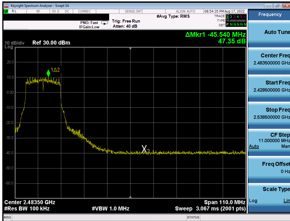
Plot 7-272. Band Edge Plot Antenna WF8 (802.11g – Ch. 7) – 36Mbps
