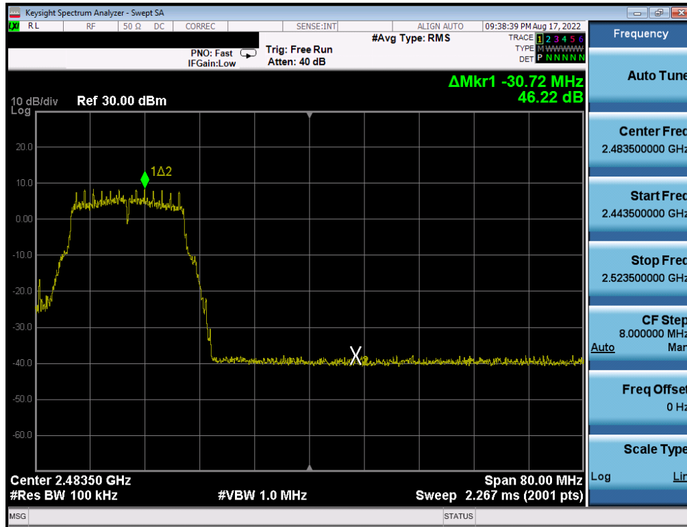
Plot 7-316. Band Edge Plot Antenna WF7 (802.11g - Ch. 10) - 12Mbps
