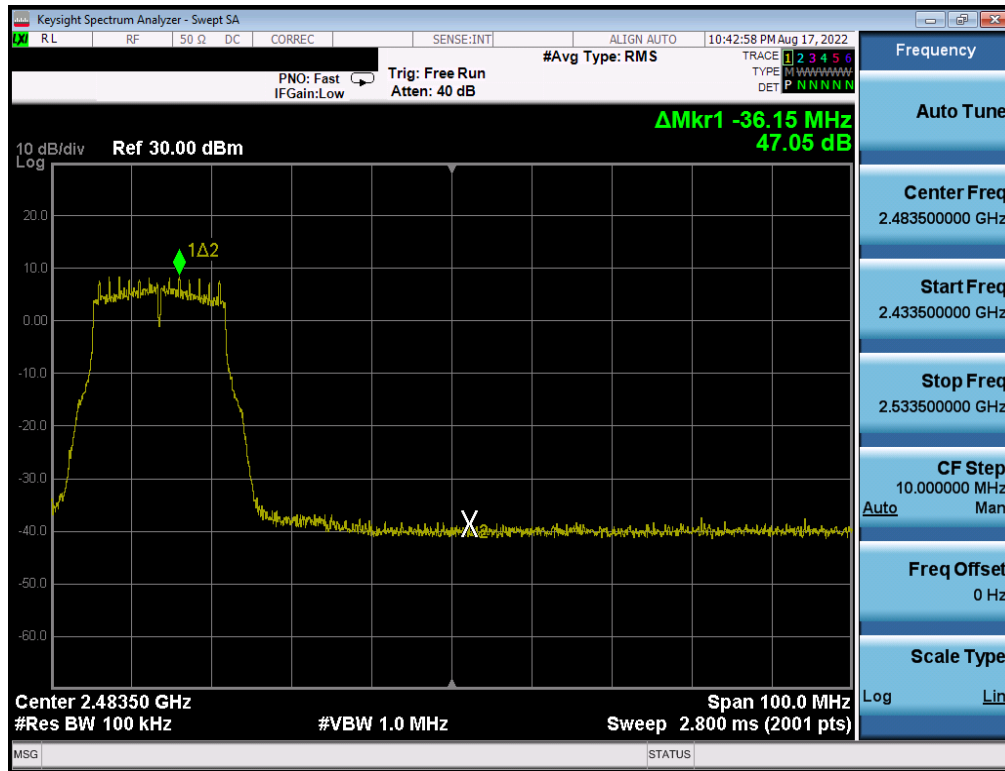
Plot 7-355 . Band Edge Plot Antenna WF7 (802.11g - Ch. 8) - 18Mbps
