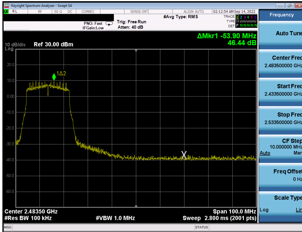
Plot 7-328 . Band Edge Plot Antenna WF7 (802.11n (2.4GHz) - Ch. 8) - MCS2
