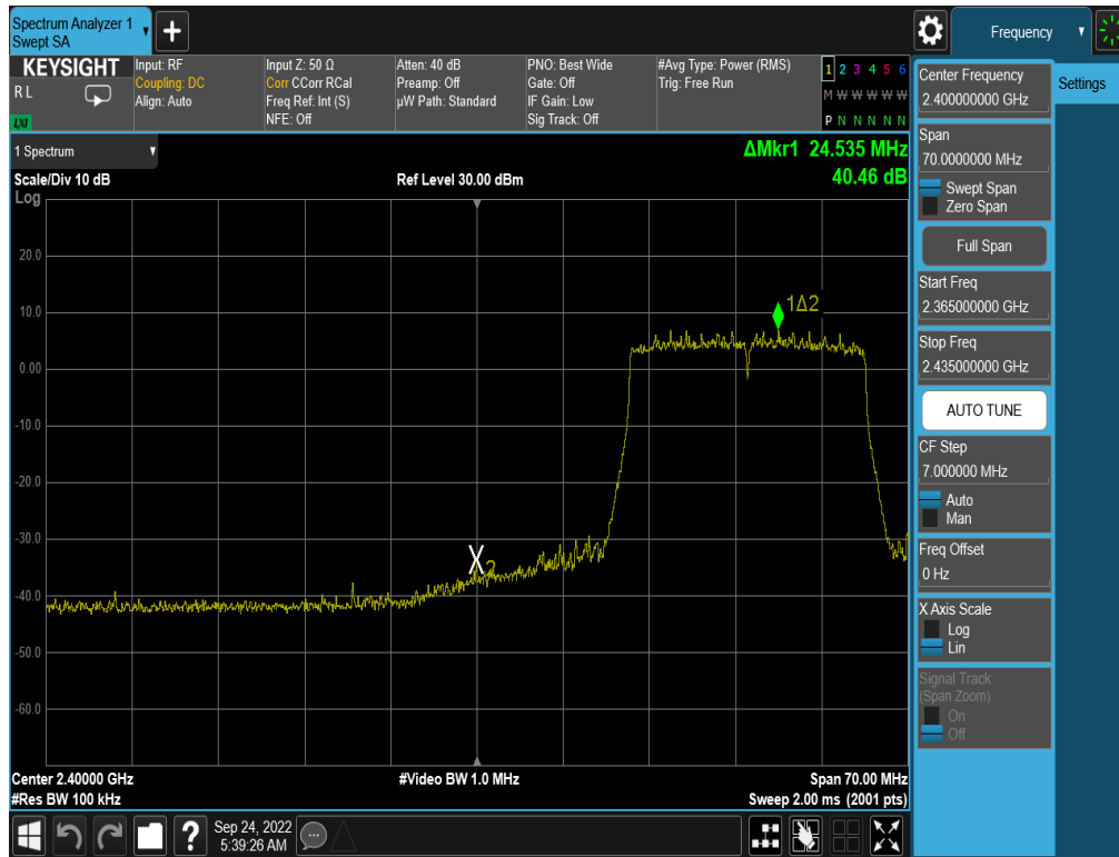
Plot 7-295. Band Edge Plot Antenna WF8 (802.11ax (SU - 2.4GHz) – Ch. 3) – MCS5
