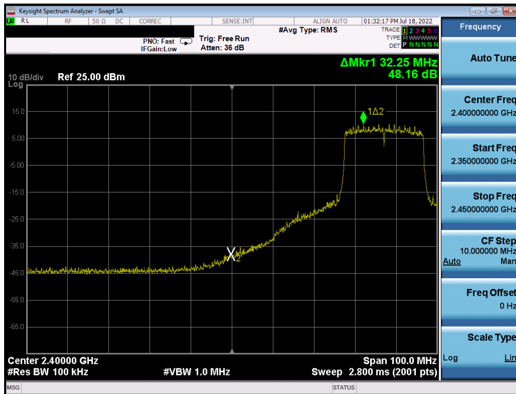
Plot 7-298. Band Edge Plot Antenna WF8 (802.11ax (SU - 2.4GHz) – Ch. 6 (low)) – MCS5
