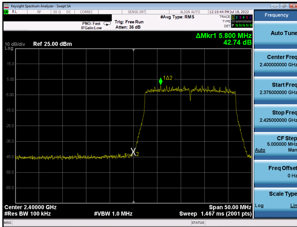
Plot 7-293. Band Edge Plot Antenna WF8 (802.11ax (SU - 2.4GHz) – Ch. 1) – MCS5
