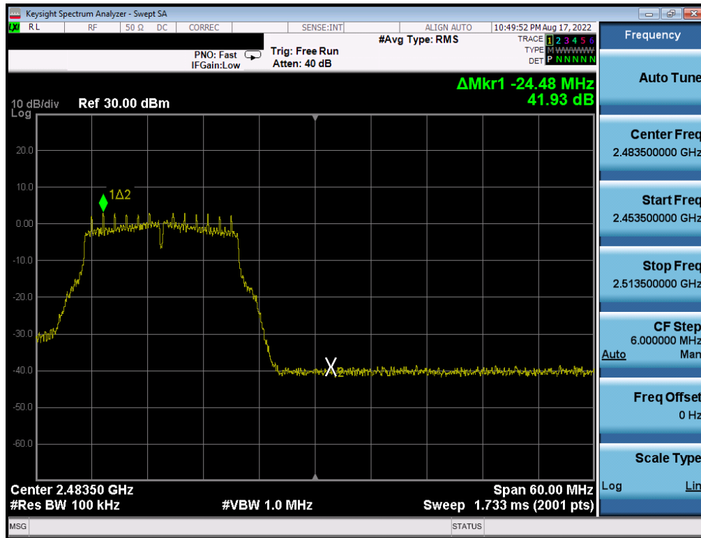
Plot 7- 359. Band Edge Plot Antenna WF7 (802.11g - Ch. 12) - 18Mbps
