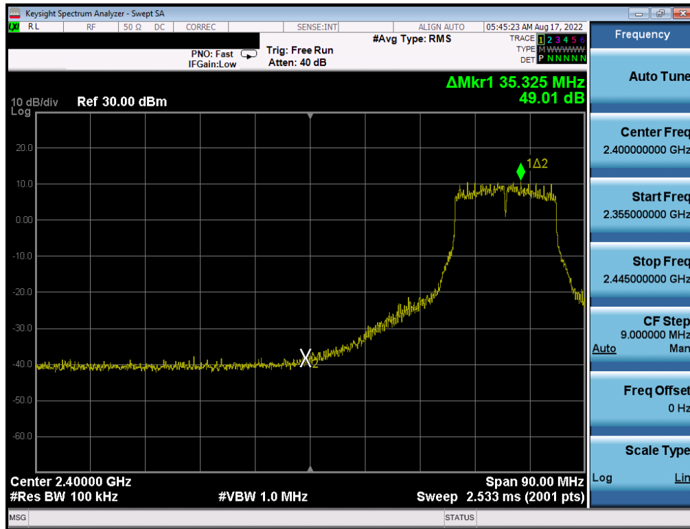
Plot 7-269. Band Edge Plot Antenna WF8 (802.11g – Ch. 5) – 36Mbps
