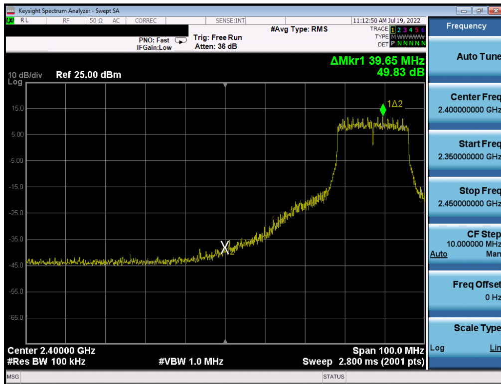
Plot 7-284. Band Edge Plot Antenna WF8 (802.11n (2.4GHz) - Ch. 6 (low)) - MCS5
