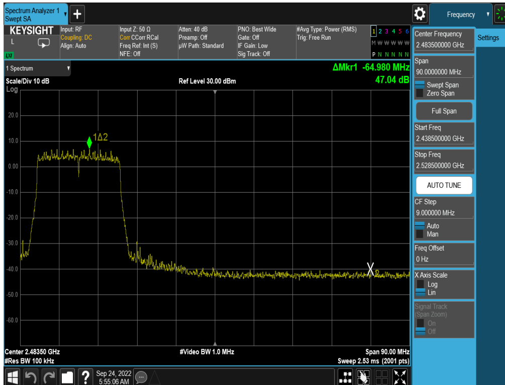
Plot 7-302. Band Edge Plot Antenna WF8 (802.11ax (SU - 2.4GHz) – Ch. 9) – MCS5
