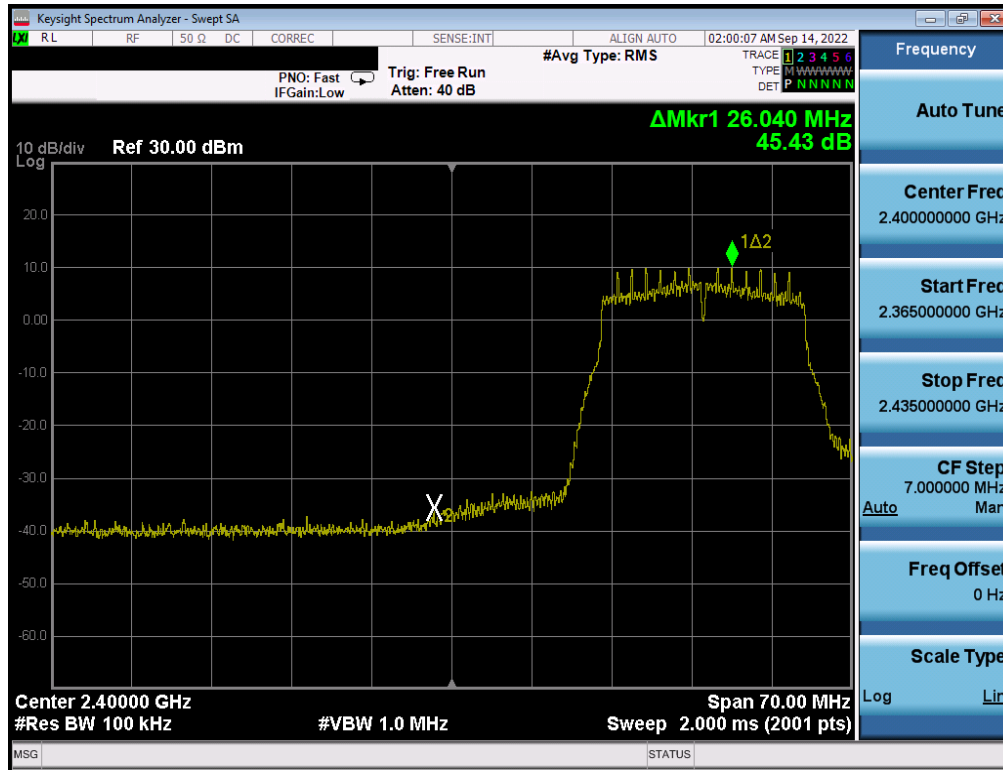
Plot 7-322. Band Edge Plot Antenna WF7 (802.11n (2.4GHz) - Ch. 3) - MCS2
