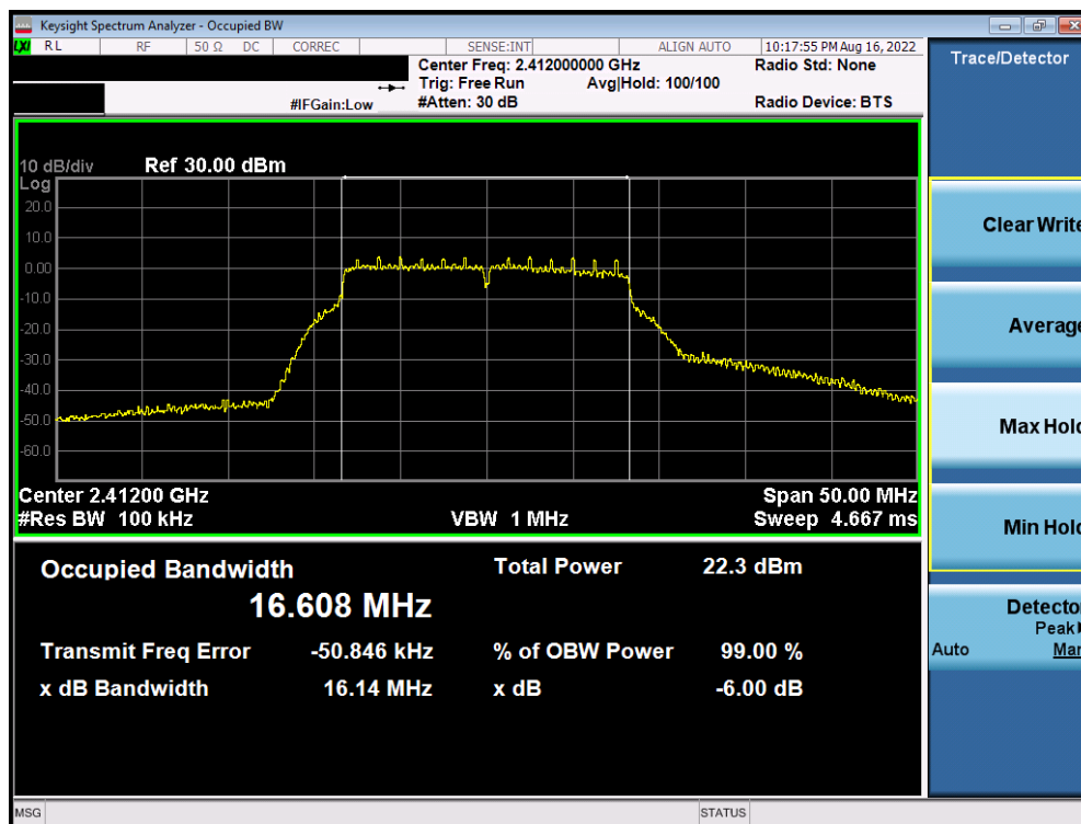
Plot 7-10. 6dB Bandwidth Plot Antenna WF8 (802.11g – Ch. 1) – 18Mbps
