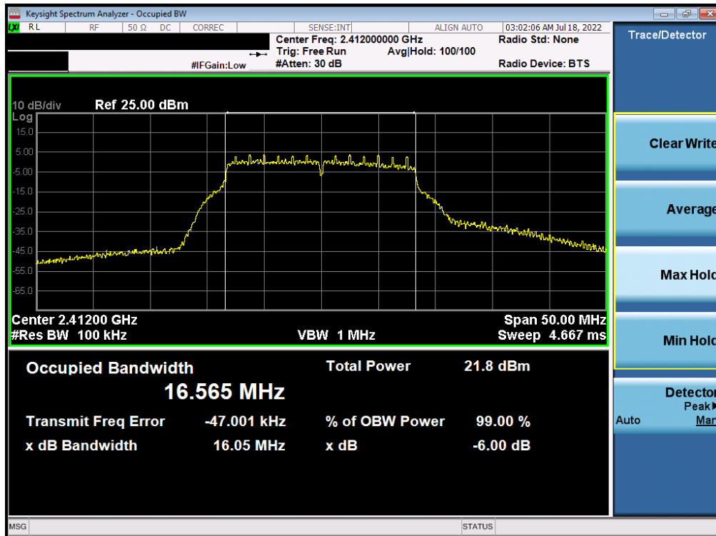
Plot 7-1. 6dB Bandwidth Plot Antenna WF8 (802.11g – Ch. 1) – 12Mbps
