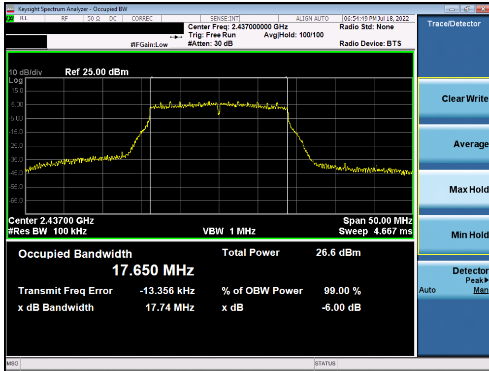
Plot 7-14. 6dB Bandwidth Plot Antenna WF8 (802.11n (2.4GHz) - Ch. 6) - MCS3
