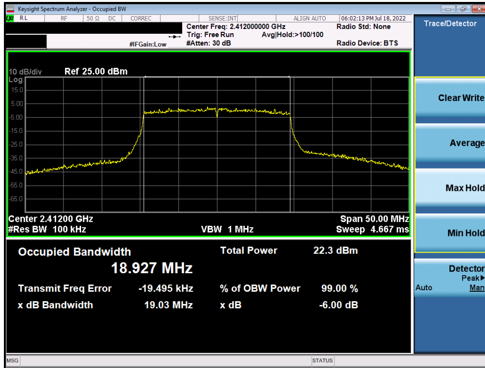
Plot 7-16. 6dB Bandwidth Plot Antenna WF8 (802. 11ax (SU - 2.4GHz) – Ch. 1) – MCS3
