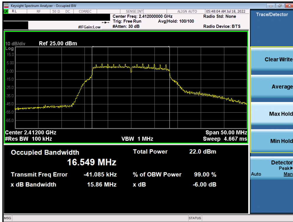
Plot 7-31. 6dB Bandwidth Plot Antenna WF7 (802.11g – Ch. 1) – 12Mbps
