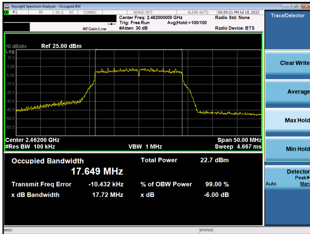
Plot 7-15. 6dB Bandwidth Plot Antenna WF8 (802.11n (2.4GHz) - Ch. 11) - MCS3
