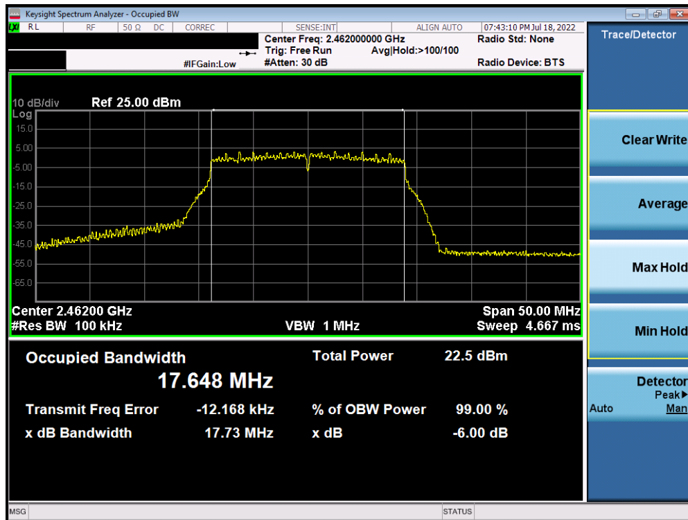
Plot 7-45. 6dB Bandwidth Plot Antenna WF7 (802.11n (2.4GHz) - Ch. 11) - MCS3
