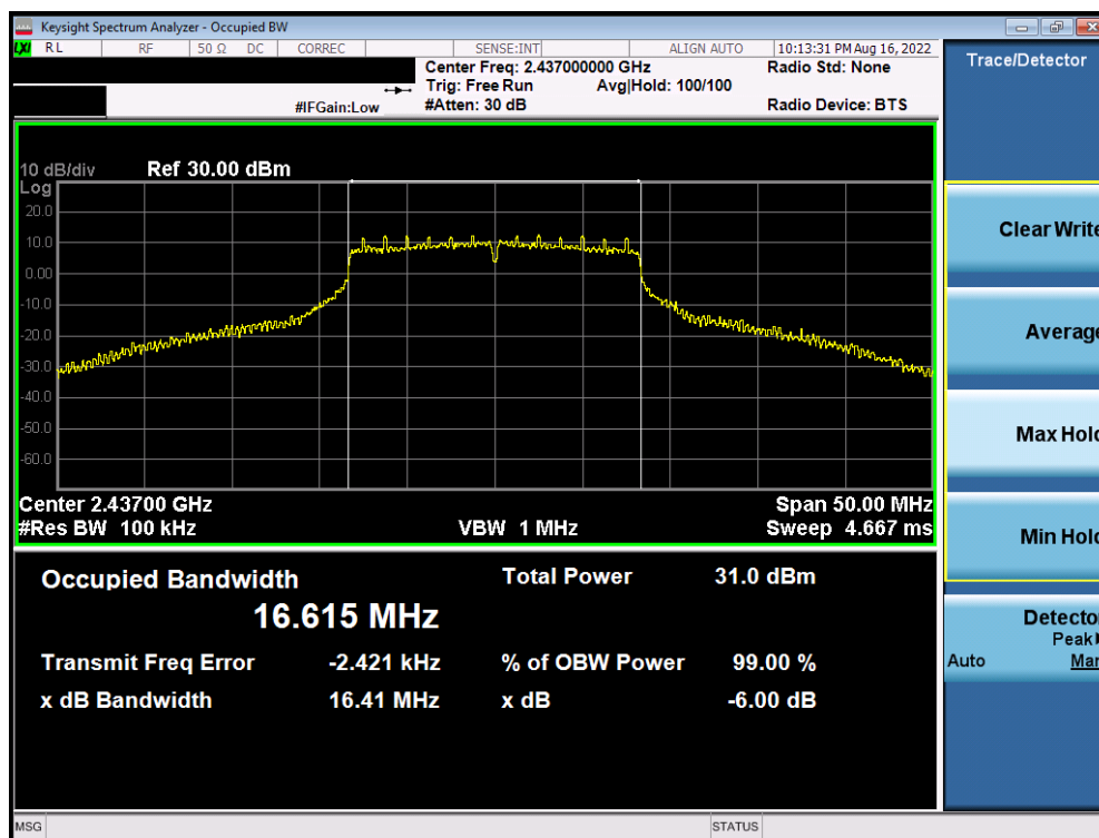
Plot 7-11. 6dB Bandwidth Plot Antenna WF8 (802.11g – Ch. 6) – 18Mbps
