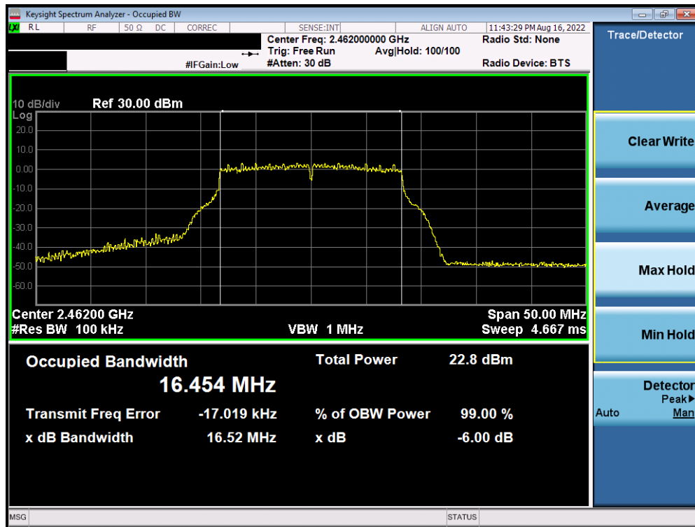
Plot 7-54. 6dB Bandwidth Plot Antenna WF7 (802.11g – Ch. 11) – 36Mbps
