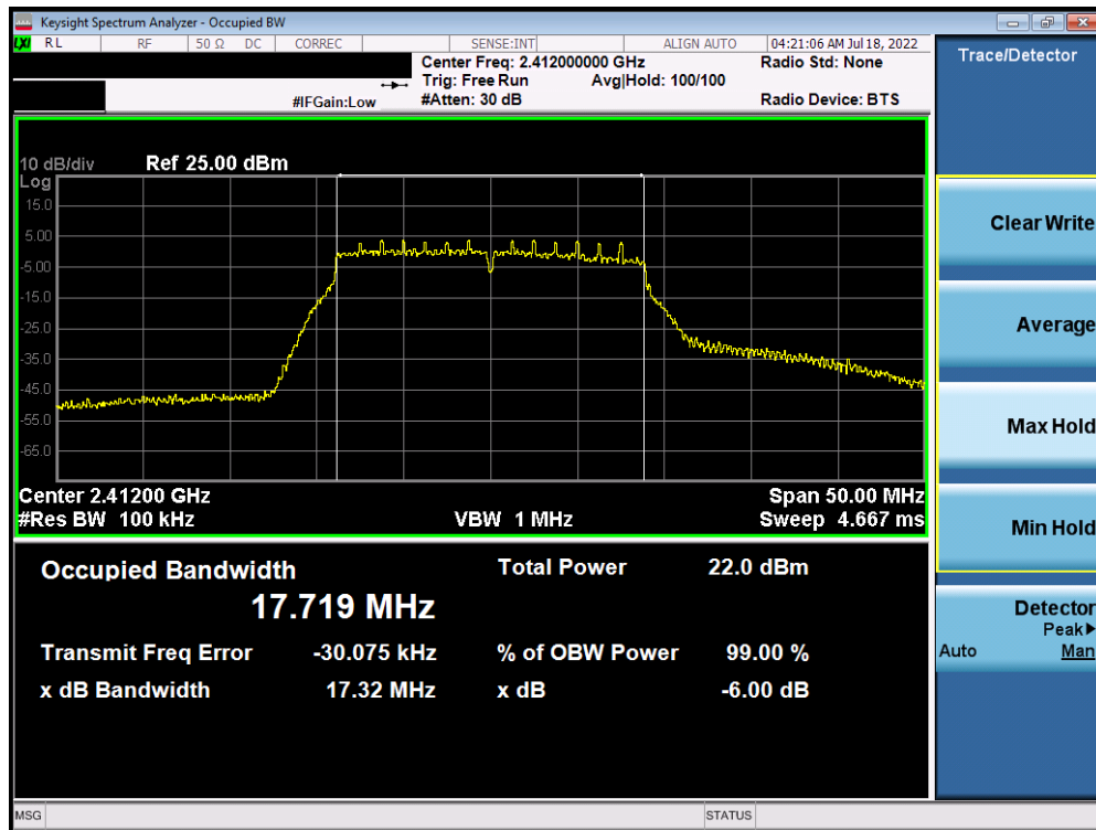
Plot 7-34. 6dB Bandwidth Plot Antenna WF7 (802.11n (2.4GHz) – Ch. 1) – MCS2
