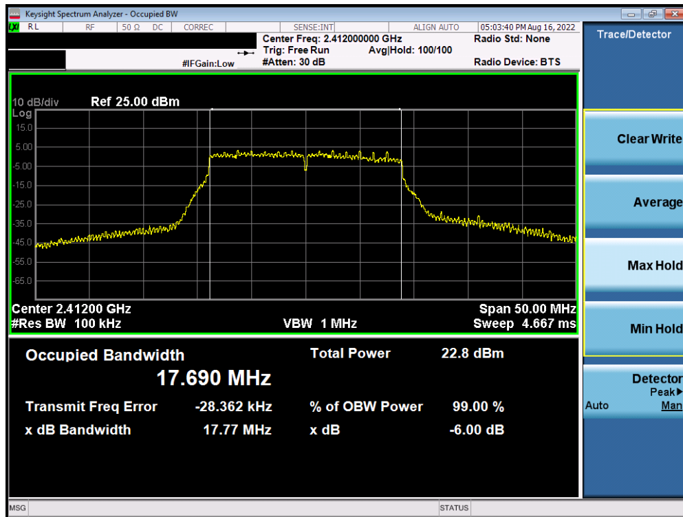
Plot 7-13. 6dB Bandwidth Plot Antenna WF8 (802.11n (2.4GHz) – Ch. 1) – MCS3
