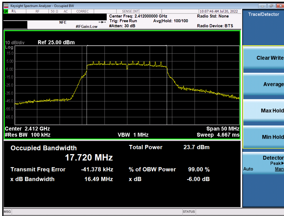
Plot 7-4. 6dB Bandwidth Plot Antenna WF8 (802.11n (2.4GHz) – Ch. 1) – MCS2
