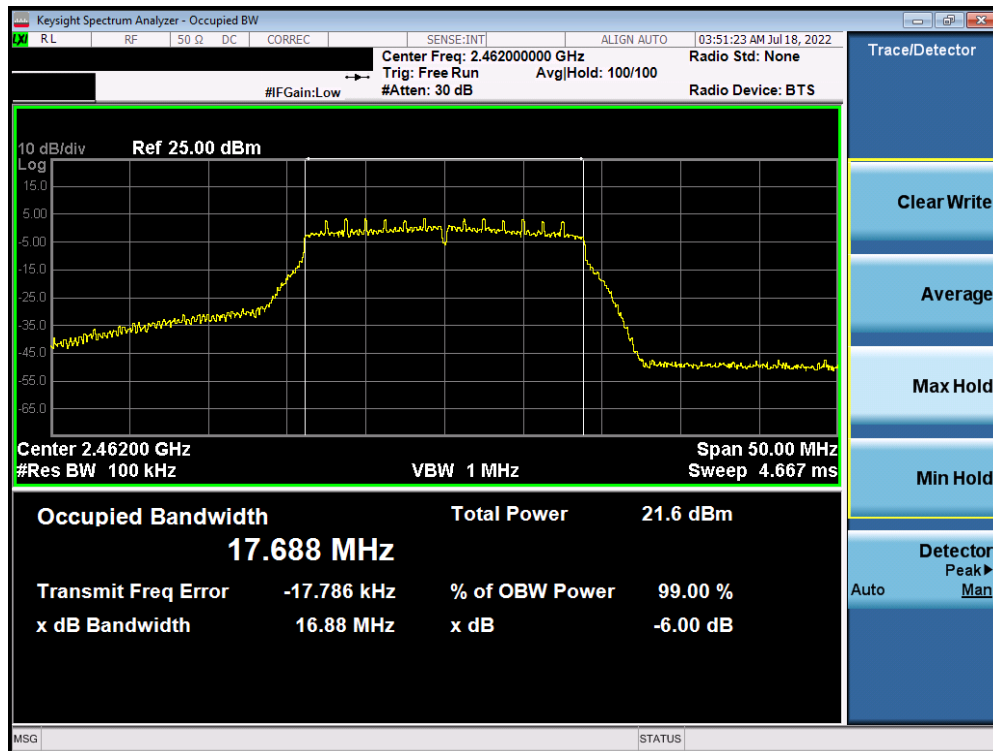
Plot 7-36. 6dB Bandwidth Plot Antenna WF7 (802.11n (2.4GHz) - Ch. 11) - MCS2
