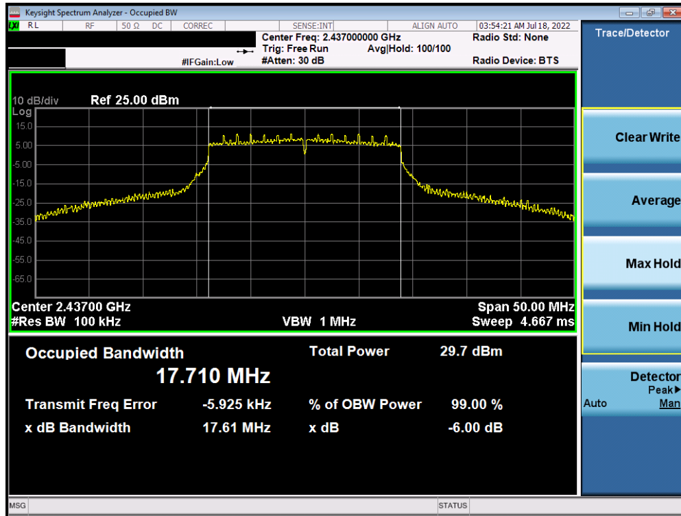
Plot 7-35. 6dB Bandwidth Plot Antenna WF7 (802.11n (2.4GHz) - Ch. 6) - MCS2
