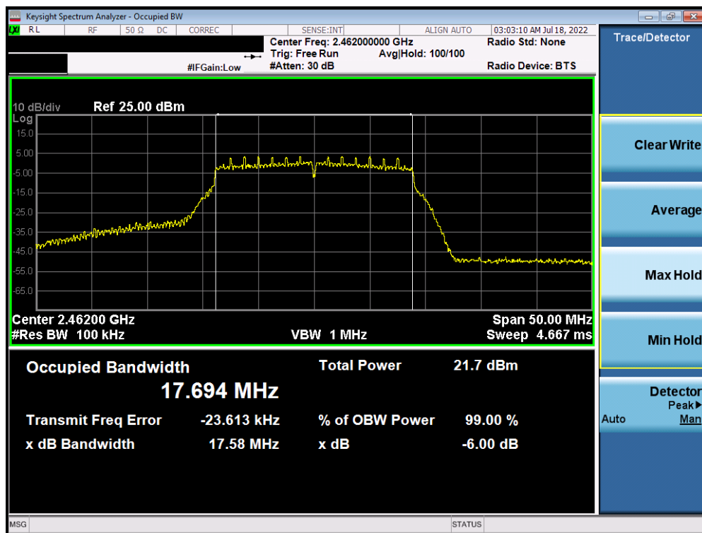
Plot 7-6. 6dB Bandwidth Plot Antenna WF8 (802.11n (2.4GHz) - Ch. 11) - MCS2
