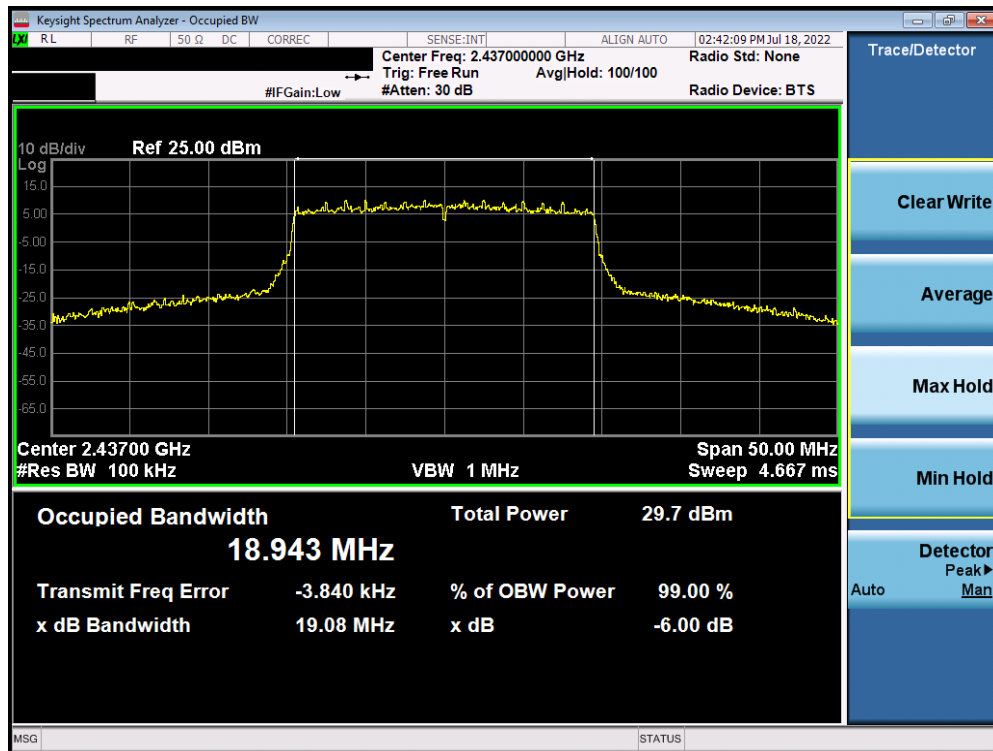
Plot 7-47. 6dB Bandwidth Plot Antenna WF7 (802. 11ax (SU - 2.4GHz) – Ch. 6) – MCS3
