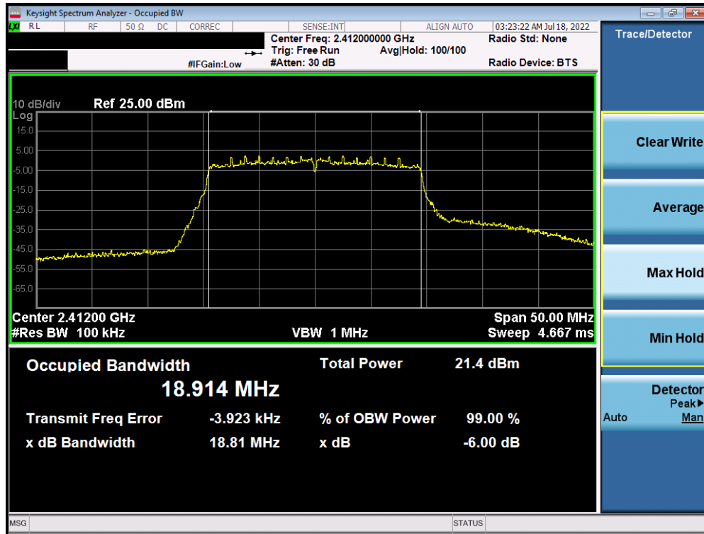
Plot 7-7. 6dB Bandwidth Plot Antenna WF8 (802.11ax (SU - 2.4GHz) – Ch. 1) – MCS2
