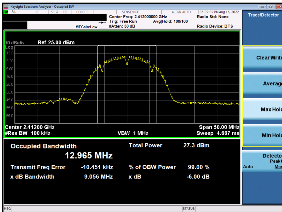
Plot 7-19. 6dB Bandwidth Plot Antenna WF8 (802.11b – Ch. 1) – 11Mbps
