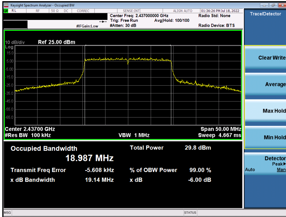
Plot 7-59. 6dB Bandwidth Plot Antenna WF7 (802.11ax (SU - 2.4GHz) – Ch. 6) – MCS5
