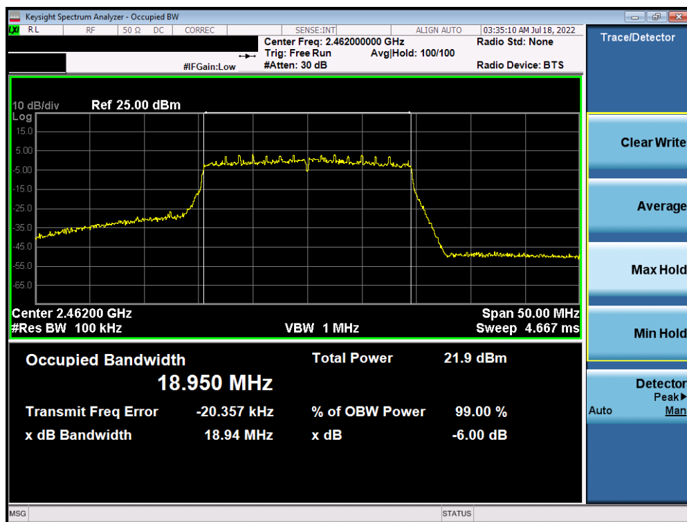
Plot 7-9. 6dB Bandwidth Plot Antenna WF8 (802. 11ax (SU - 2.4GHz) – Ch. 11) – MCS2
