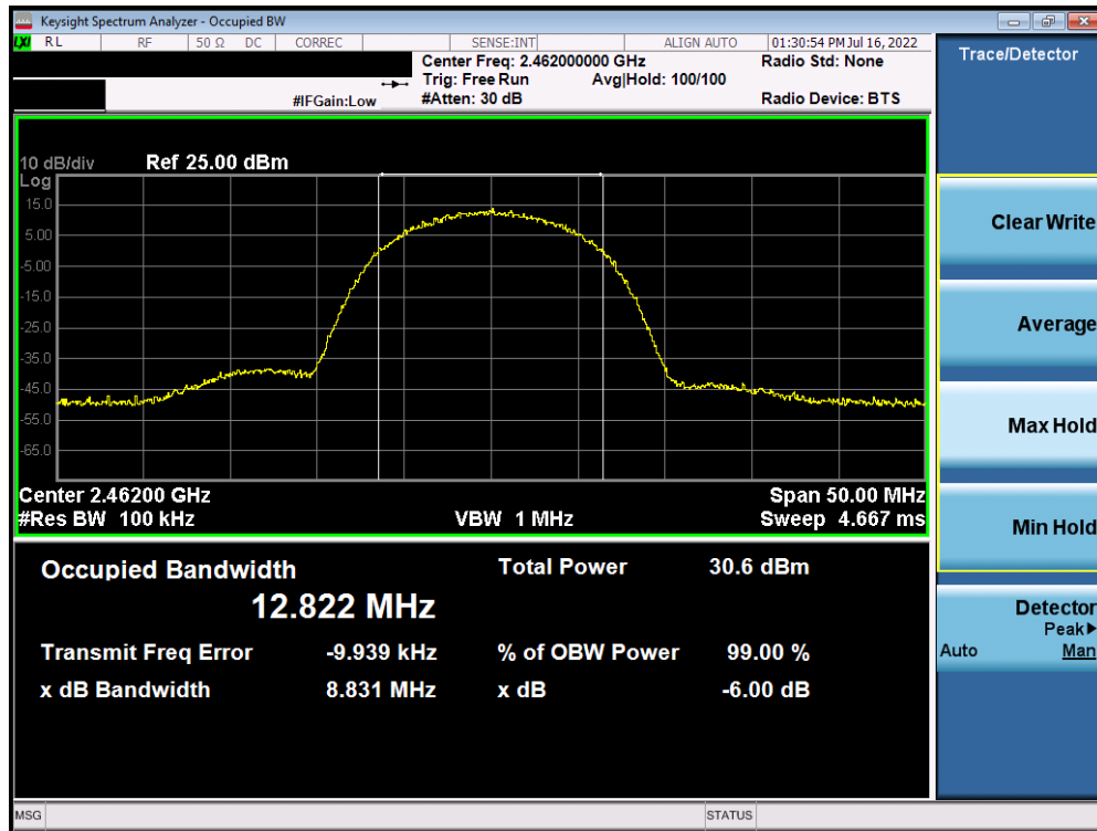
Plot 7-21. 6dB Bandwidth Plot Antenna WF8 (802.11b – Ch. 11) – 11Mbps
