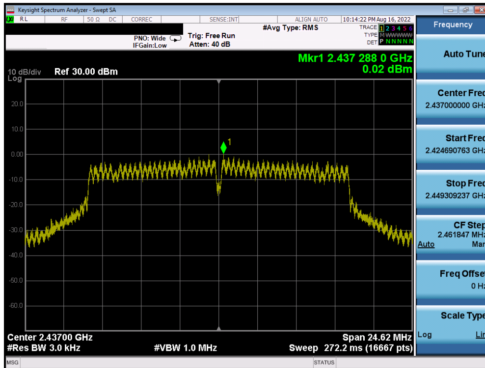
Plot 7-71. Power Spectral Density Plot Antenna WF8 (802.11g – Ch. 6) – 18Mbps
