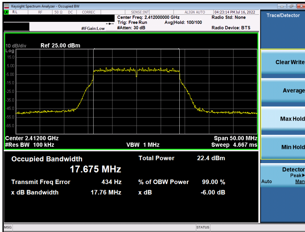
Plot 7-55. 6dB Bandwidth Plot Antenna WF7 (802.11n (2.4GHz) - Ch. 1) - MCS5
