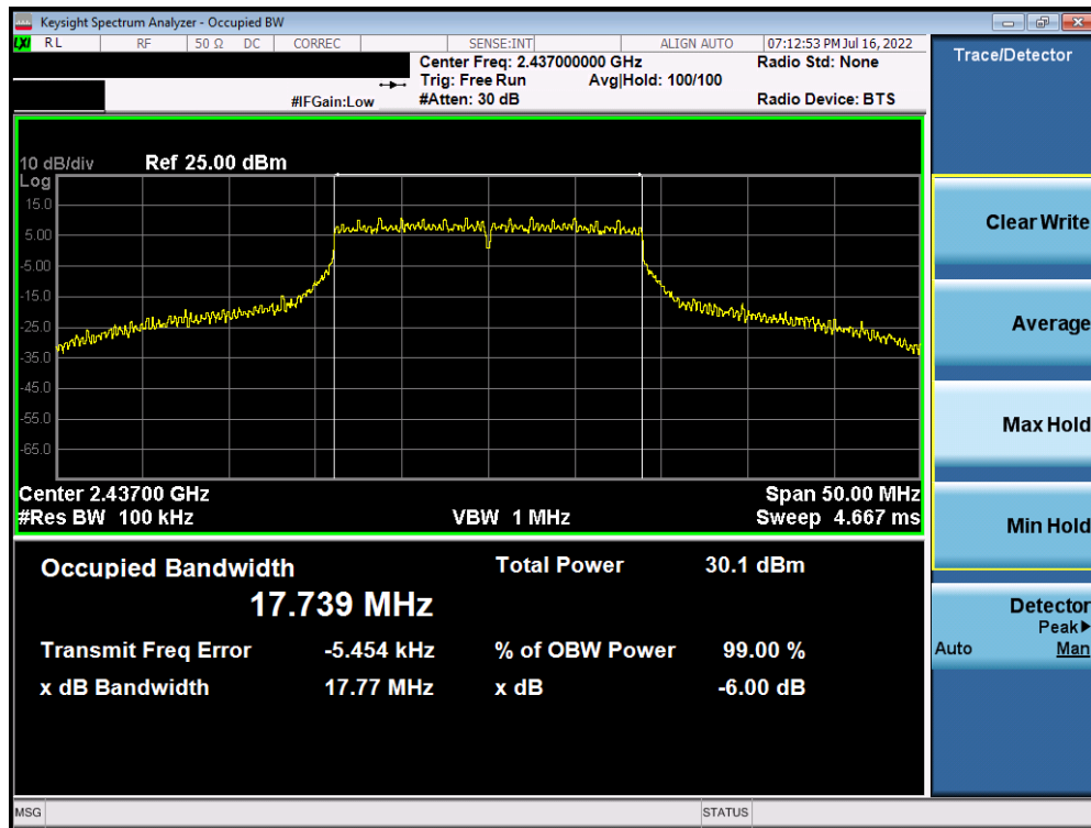
Plot 7-26. 6dB Bandwidth Plot Antenna WF8 (802.11n (2.4GHz) - Ch. 6) - MCS5
