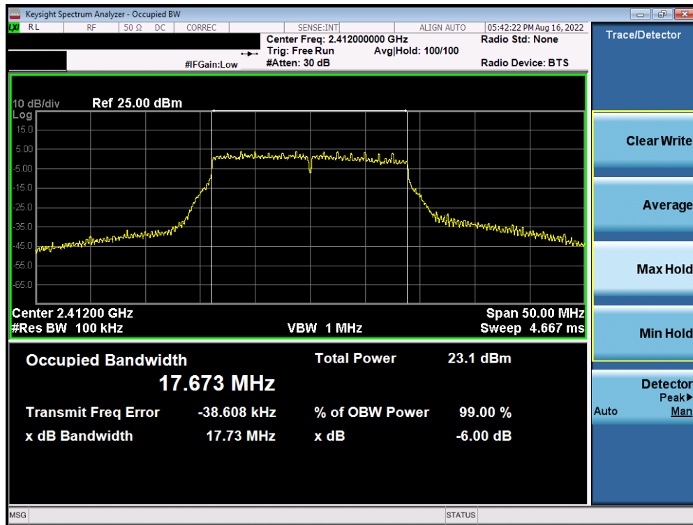
Plot 7-43. 6dB Bandwidth Plot Antenna WF7 (802.11n (2.4GHz) – Ch. 1) – MCS3
