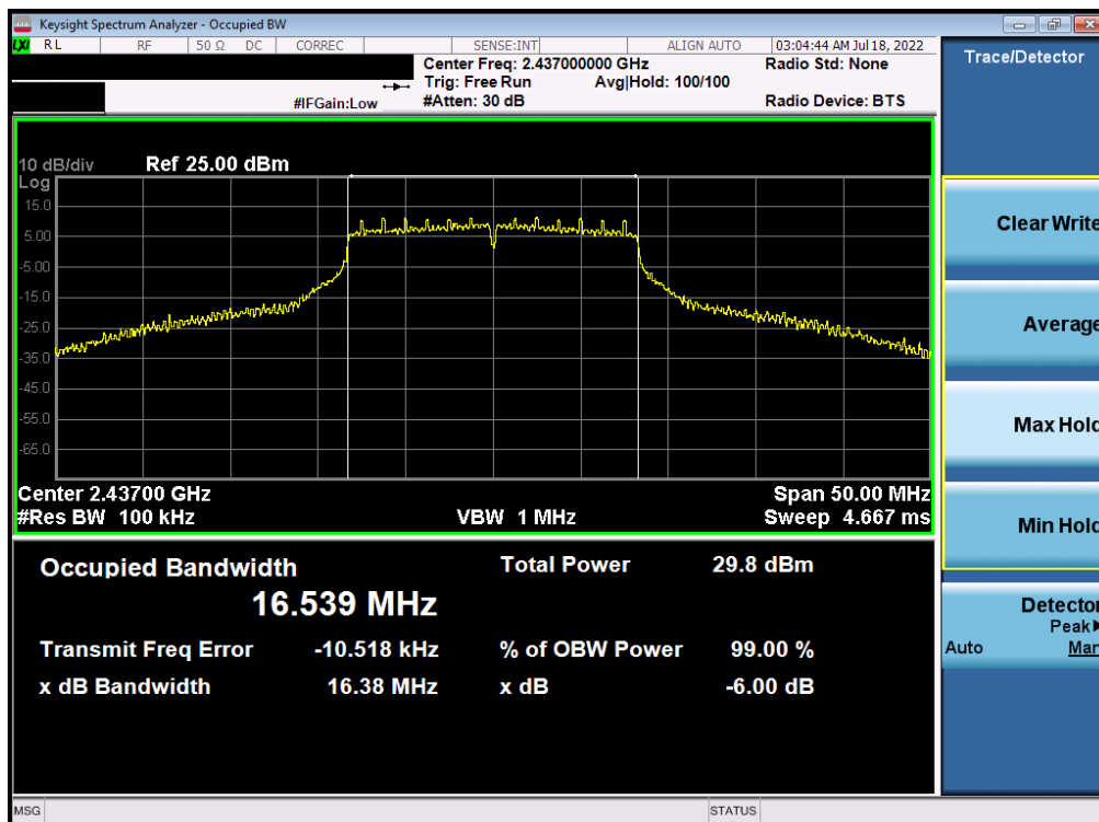
Plot 7-2. 6dB Bandwidth Plot Antenna WF8 (802.11g – Ch. 6) – 12Mbps
