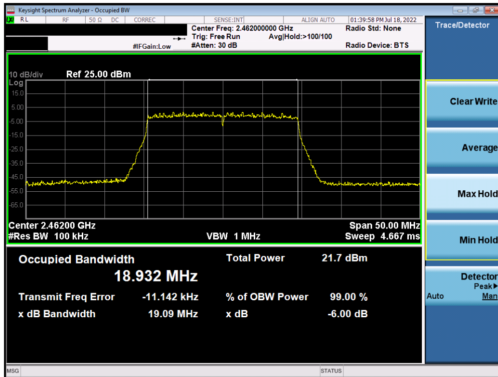
Plot 7-60. 6dB Bandwidth Plot Antenna WF7 (802.11ax (SU - 2.4GHz) – Ch. 11) – MCS5
