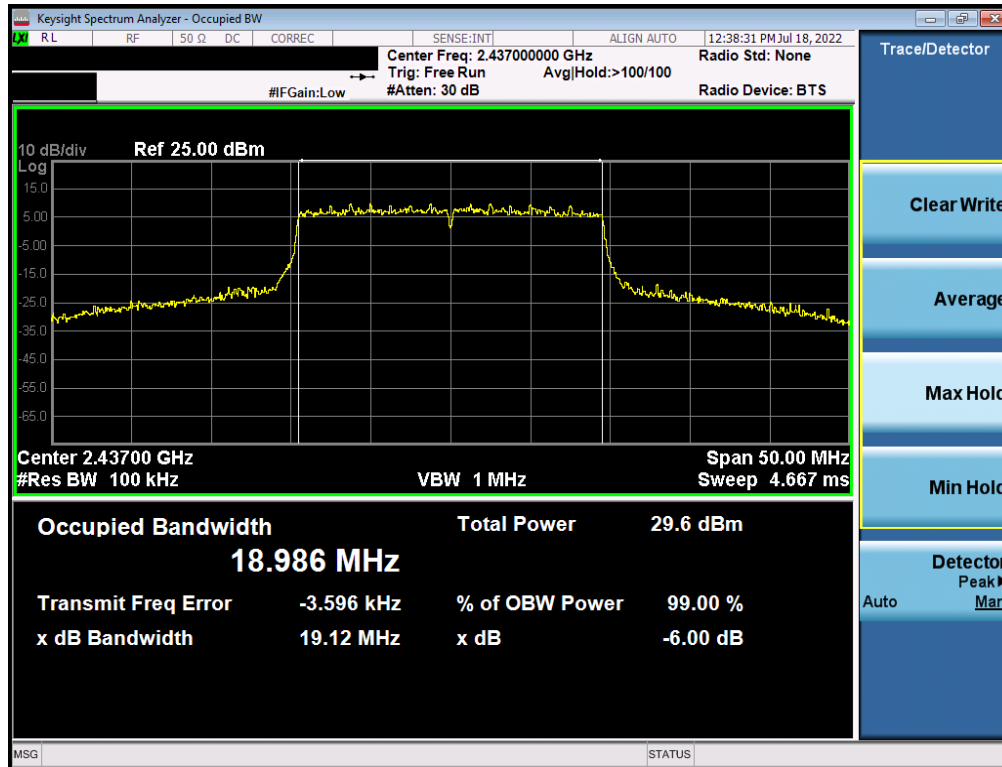
Plot 7-29. 6dB Bandwidth Plot Antenna WF8 (802.11ax (SU - 2.4GHz) - Ch. 6) - MCS5
