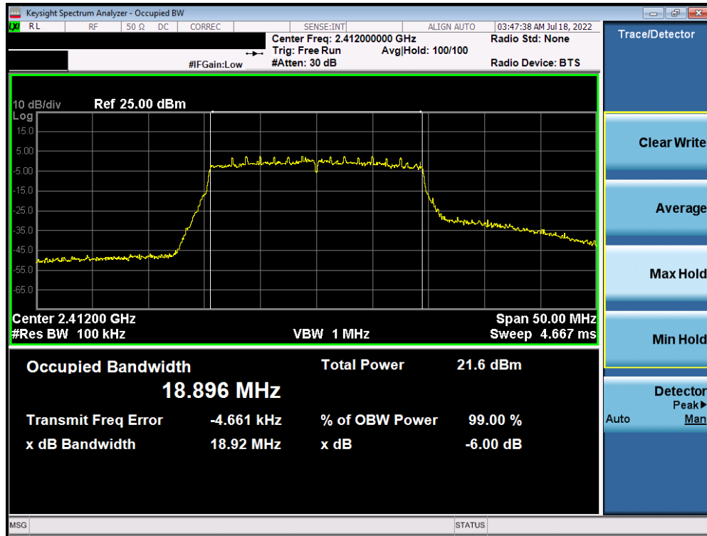
Plot 7-37. 6dB Bandwidth Plot Antenna WF7 (802.11ax (SU - 2.4GHz) – Ch. 1) – MCS2
