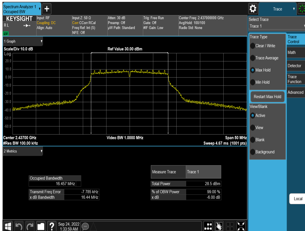
Plot 7-32. 6dB Bandwidth Plot Antenna WF7 (802.11g – Ch. 6) – 12Mbps
