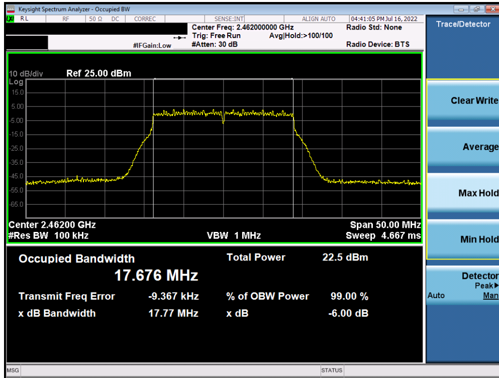
Plot 7-57. 6dB Bandwidth Plot Antenna WF7 (802.11n (2.4GHz) – Ch. 11) – MCS5
