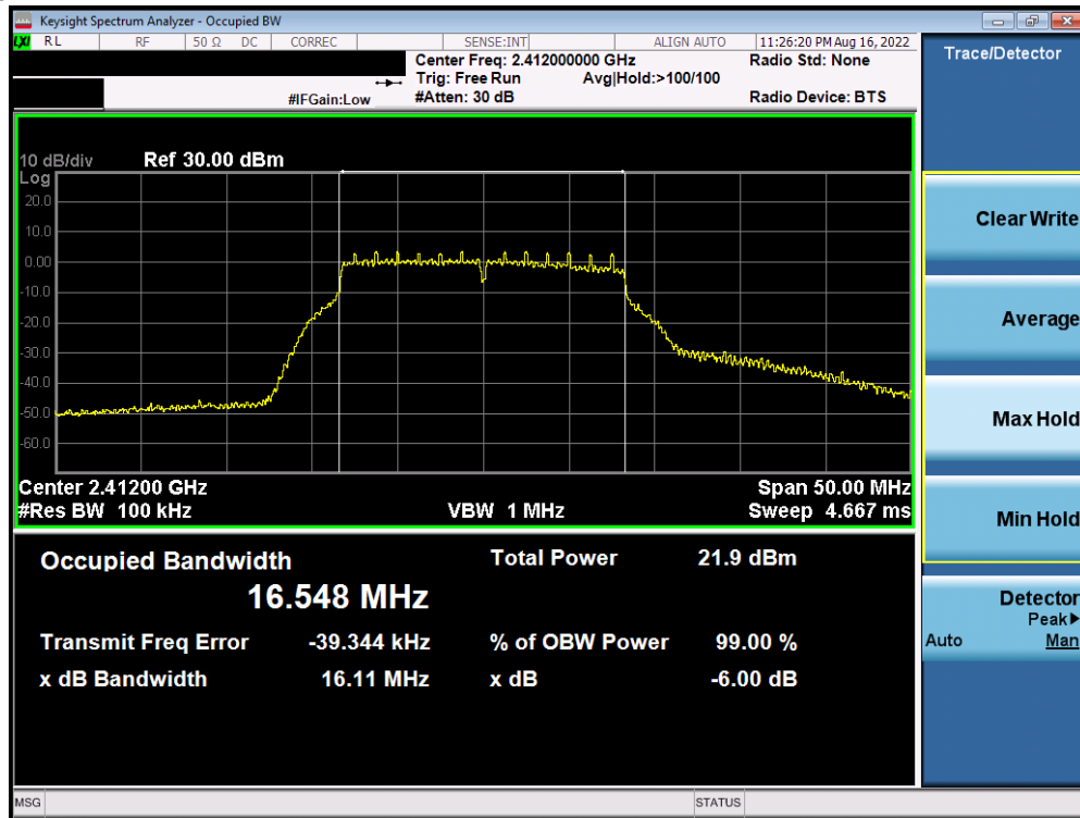
Plot 7-40. 6dB Bandwidth Plot Antenna WF7 (802.11g - Ch. 1) – 18Mbps
