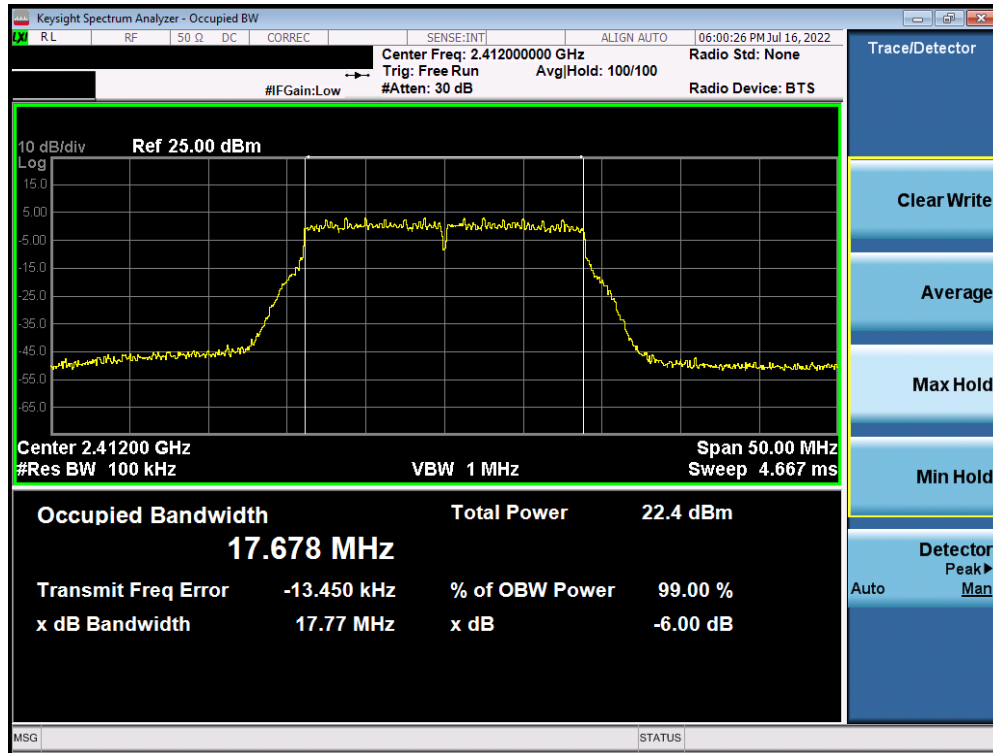
Plot 7-25. 6dB Bandwidth Plot Antenna WF8 (802.11n (2.4GHz) - Ch. 1) - MCS5
