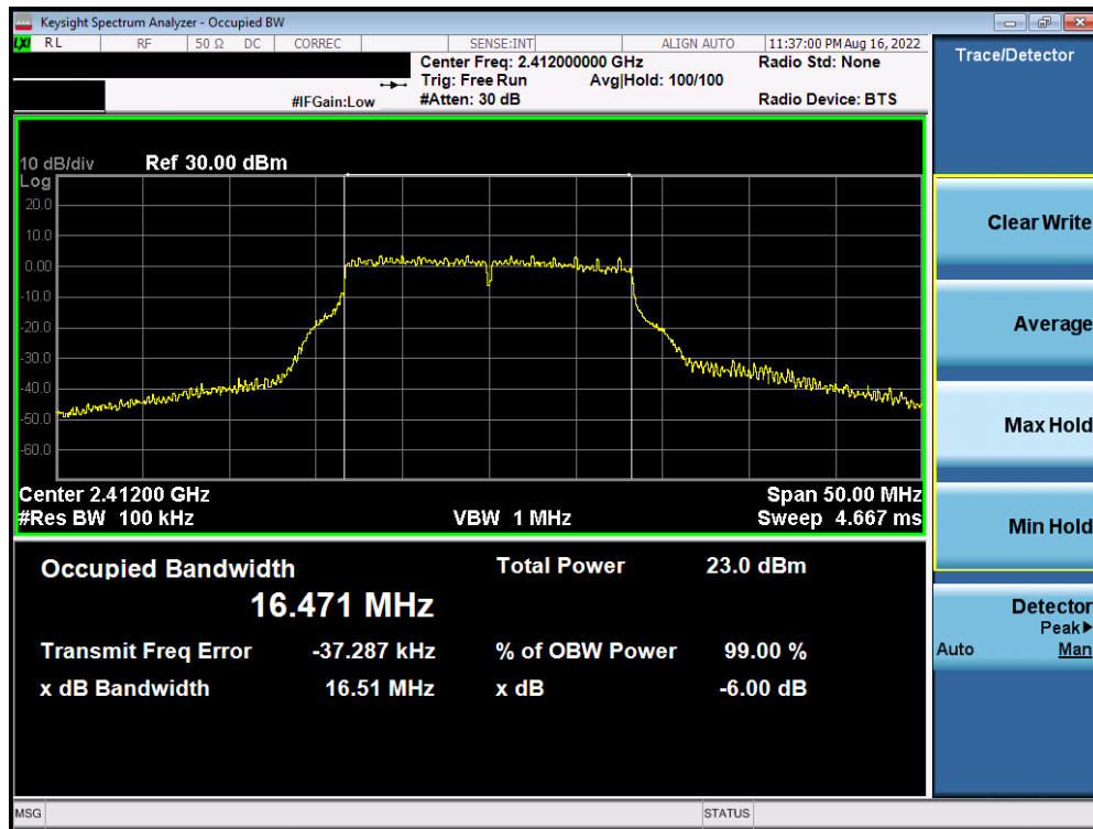
Plot 7-52. 6dB Bandwidth Plot Antenna WF7 (802.11g – Ch. 1) – 36Mbps
