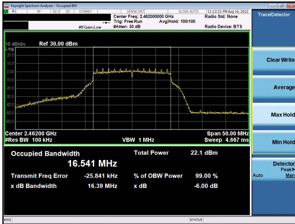
Plot 7-12. 6dB Bandwidth Plot Antenna WF8 (802.11g – Ch. 11) – 18Mbps
