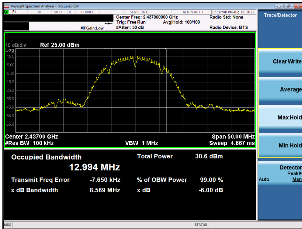
Plot 7-50. 6dB Bandwidth Plot Antenna WF7 (802.11b – Ch. 6) – 11Mbps
