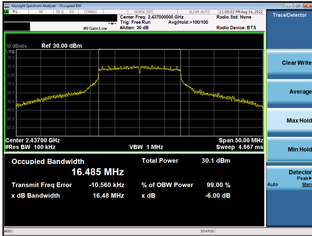
Plot 7-23. 6dB Bandwidth Plot Antenna WF8 (802.11g - Ch. 6) - 36Mbps
