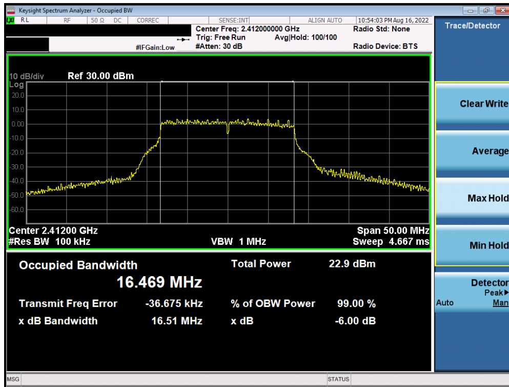
Plot 7-22. 6dB Bandwidth Plot Antenna WF8 (802.11g – Ch. 1) – 36Mbps
