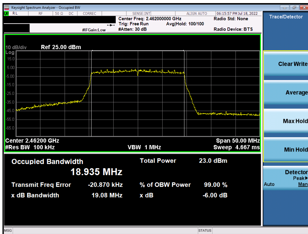
Plot 7-18. 6dB Bandwidth Plot Antenna WF8 (802. 11ax (SU - 2.4GHz) – Ch. 11) – MCS3
