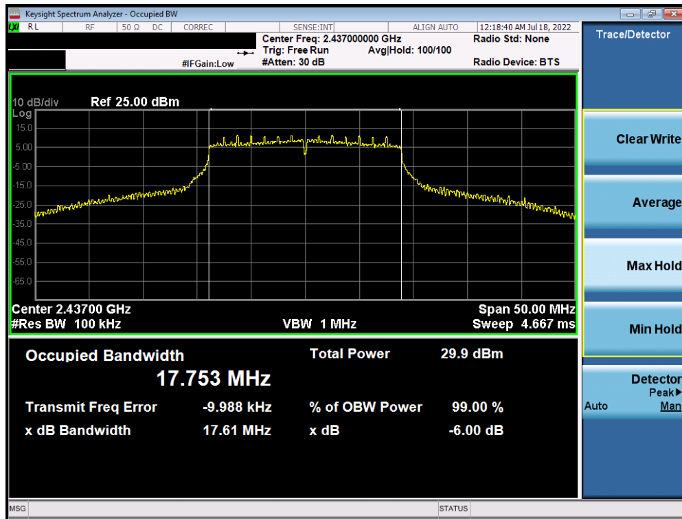
Plot 7-5. 6dB Bandwidth Plot Antenna WF8 (802.11n (2.4GHz) - Ch. 6) - MCS2
