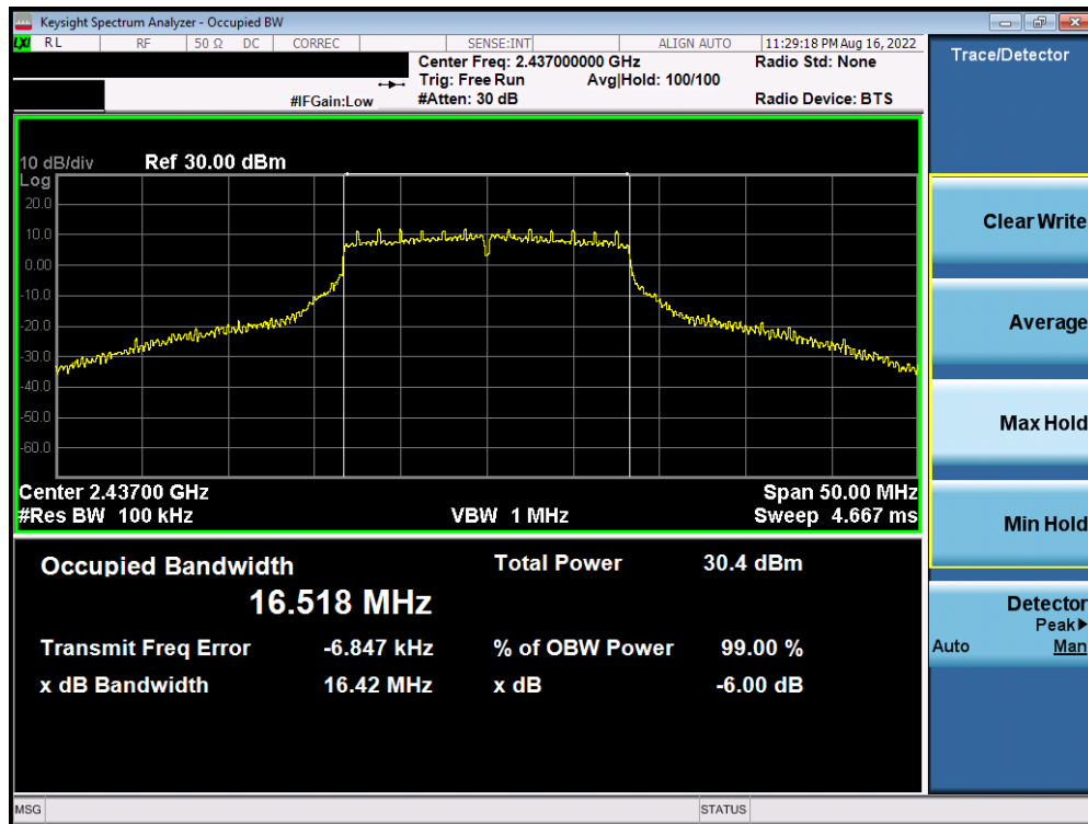
Plot 7-41. 6dB Bandwidth Plot Antenna WF7 (802.11g - Ch. 6) – 18Mbps
