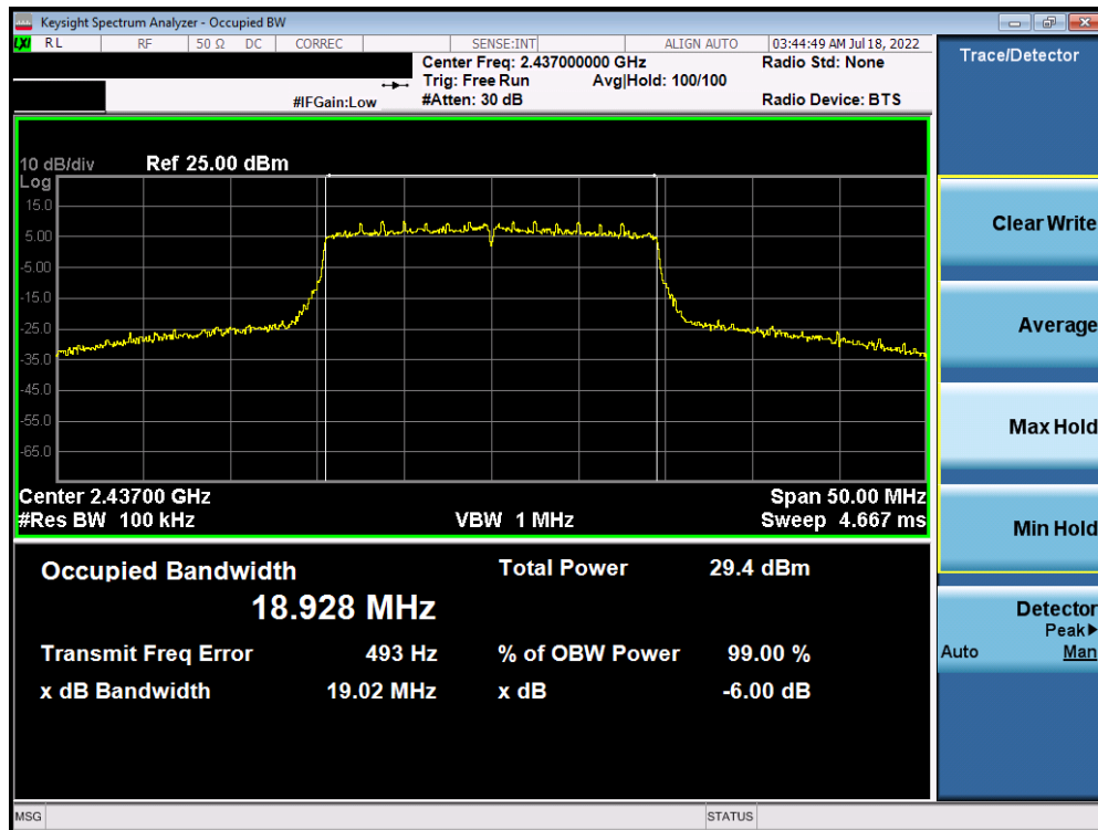
Plot 7-38. 6dB Bandwidth Plot Antenna WF7 (802.11ax (SU - 2.4GHz) – Ch. 6) – MCS2
