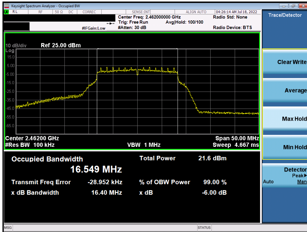
Plot 7-33. 6dB Bandwidth Plot Antenna WF7 (802.11g – Ch. 11) – 12Mbps
