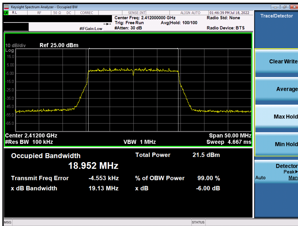
Plot 7-58. 6dB Bandwidth Plot Antenna WF7 (802.11ax (SU - 2.4GHz) – Ch. 1) – MCS5
