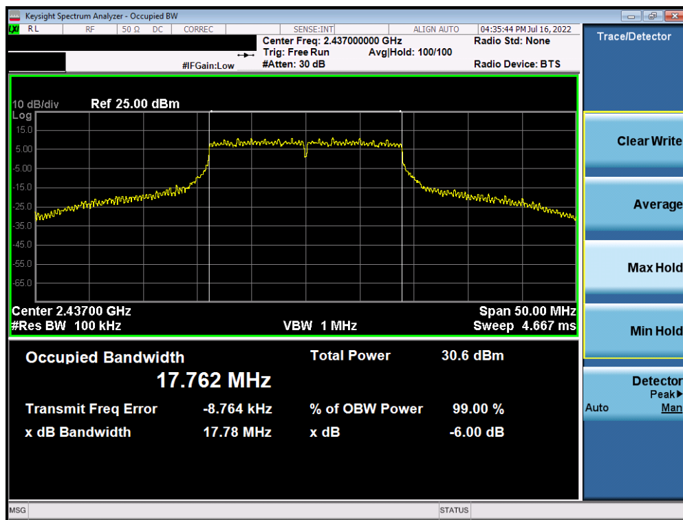
Plot 7-56. 6dB Bandwidth Plot Antenna WF7 (802.11n (2.4GHz) - Ch. 6) - MCS5
