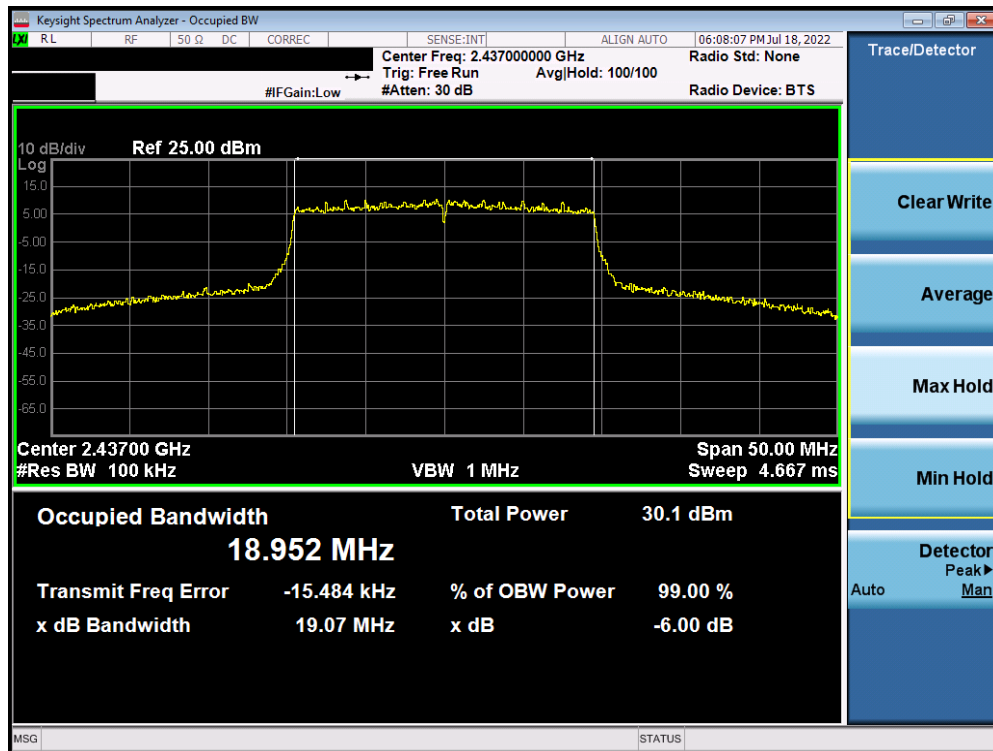
Plot 7-17. 6dB Bandwidth Plot Antenna WF8 (802. 11ax (SU - 2.4GHz) – Ch. 6) – MCS3
