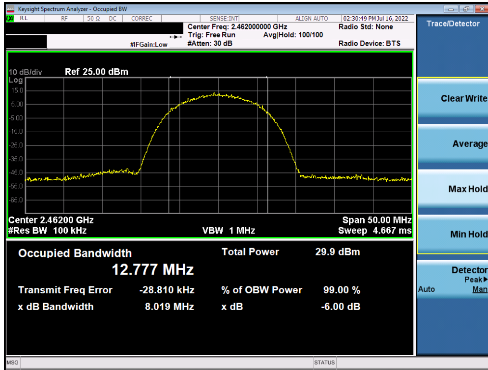
Plot 7-51. 6dB Bandwidth Plot Antenna WF7 (802.11b – Ch. 11) – 11Mbps
