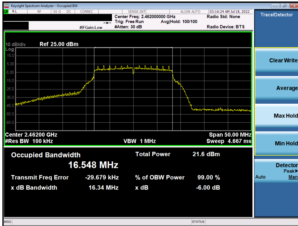
Plot 7-3. 6dB Bandwidth Plot Antenna WF8 (802.11g – Ch. 11) – 12Mbps
