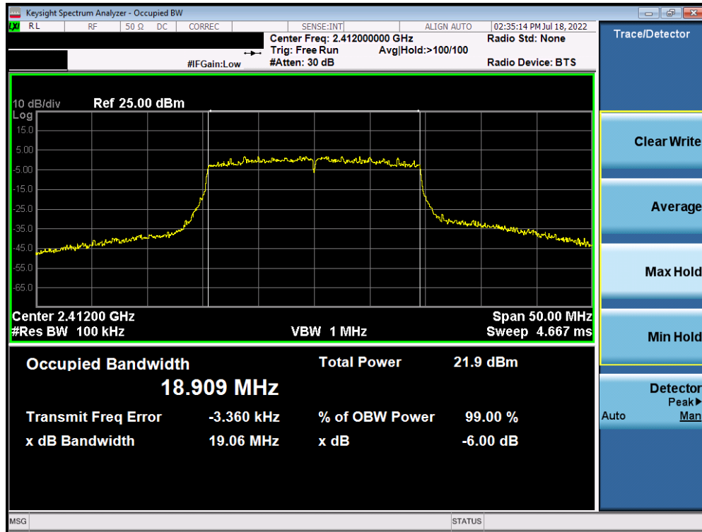
Plot 7-46. 6dB Bandwidth Plot Antenna WF7 (802. 11ax (SU - 2.4GHz) – Ch. 1) – MCS3
