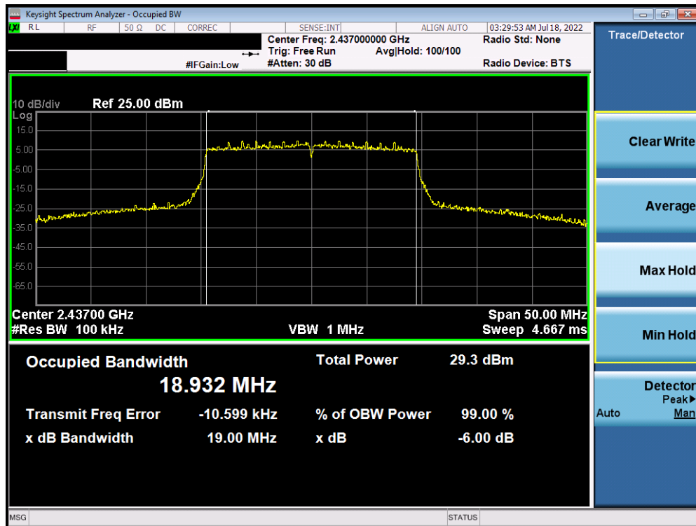
Plot 7-8. 6dB Bandwidth Plot Antenna WF8 (802.11ax (SU - 2.4GHz) – Ch. 6) – MCS2
