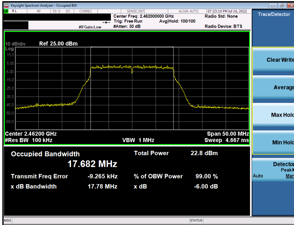
Plot 7-27. 6dB Bandwidth Plot Antenna WF8 (802.11n (2.4GHz) – Ch. 11) – MCS5
