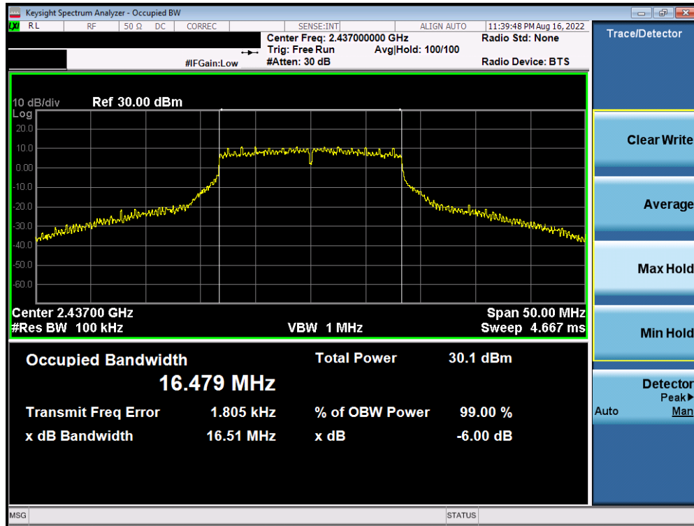
Plot 7-53. 6dB Bandwidth Plot Antenna WF7 (802.11g – Ch. 6) – 36Mbps
