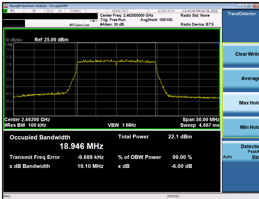
Plot 7-30. 6dB Bandwidth Plot Antenna WF8 (802.11ax (SU - 2.4GHz) - Ch. 11) - MCS5
