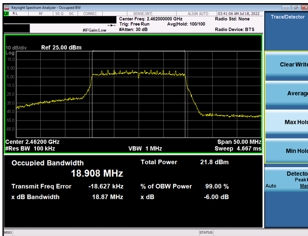
Plot 7-39. 6dB Bandwidth Plot Antenna WF7 (802.11ax (SU - 2.4GHz) - Ch. 11) - MCS2
