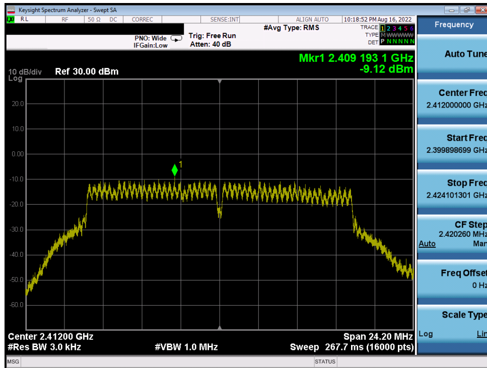
Plot 7-70. Power Spectral Density Plot Antenna WF8 (802.11g – Ch. 1) – 18Mbps
