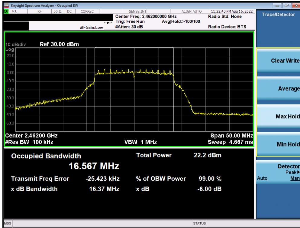
Plot 7-42. 6dB Bandwidth Plot Antenna WF7 (802.11g – Ch. 11) – 18Mbps
