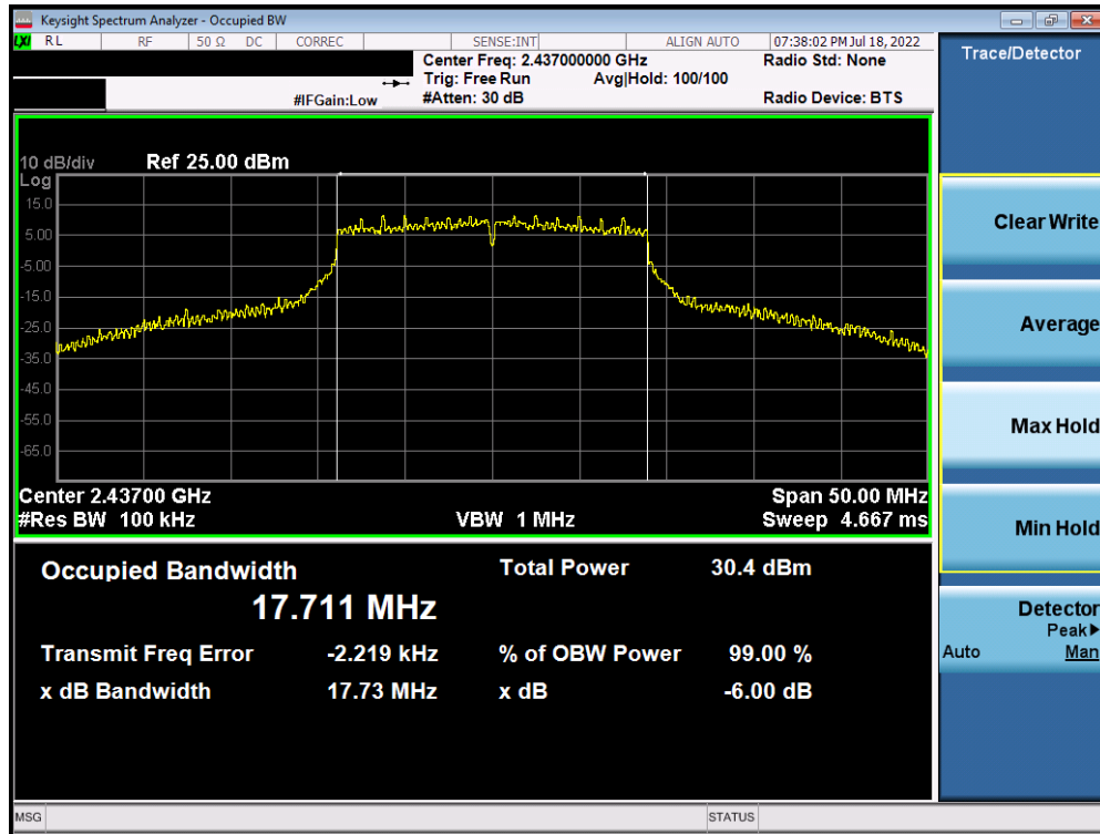
Plot 7-44. 6dB Bandwidth Plot Antenna WF7 (802.11n (2.4GHz) - Ch. 6) - MCS3
