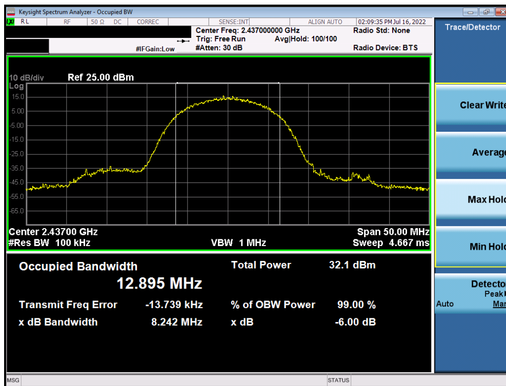
Plot 7-20. 6dB Bandwidth Plot Antenna WF8 (802.11b – Ch. 6) – 11Mbps
