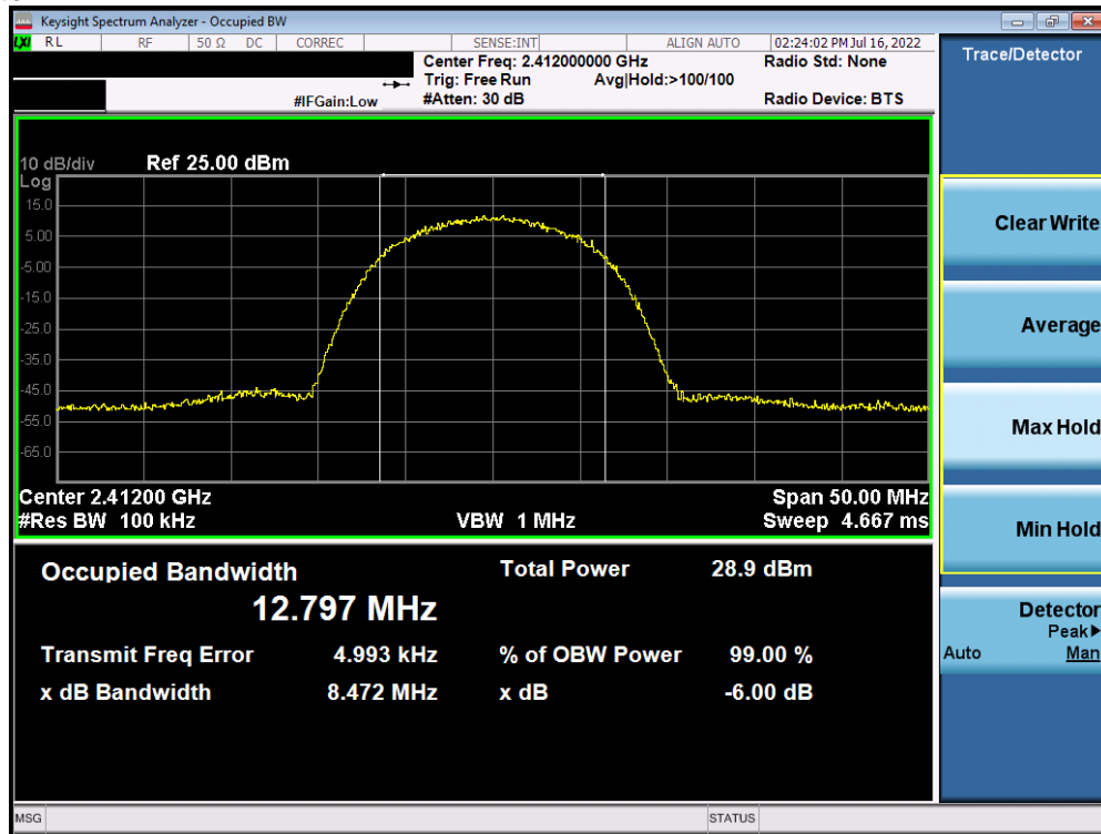
Plot 7-49. 6dB Bandwidth Plot Antenna WF7 (802.11b – Ch. 1) – 11Mbps
