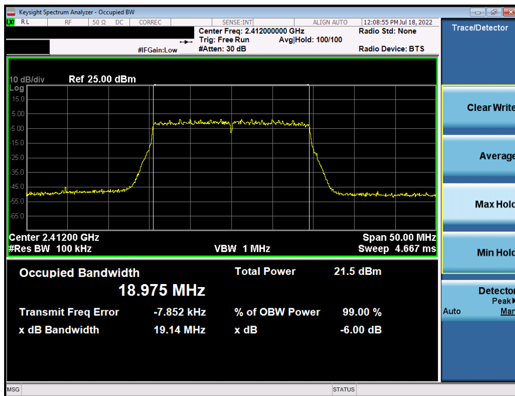
Plot 7-28. 6dB Bandwidth Plot Antenna WF8 (802.11ax (SU – 2.4GHz) – Ch. 1) – MCS5
