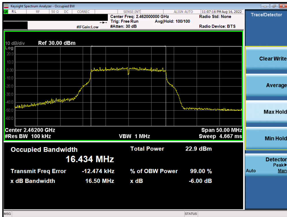
Plot 7-24. 6dB Bandwidth Plot Antenna WF8 (802.11g - Ch. 11) - 36Mbps
