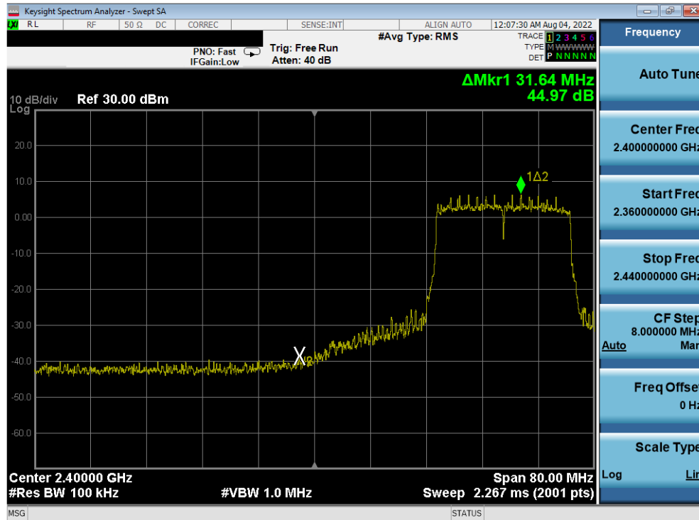
Plot 7-81. Band Edge Antenna WF8(802.11ax OFDMA – RU242 – Ch. 4)
