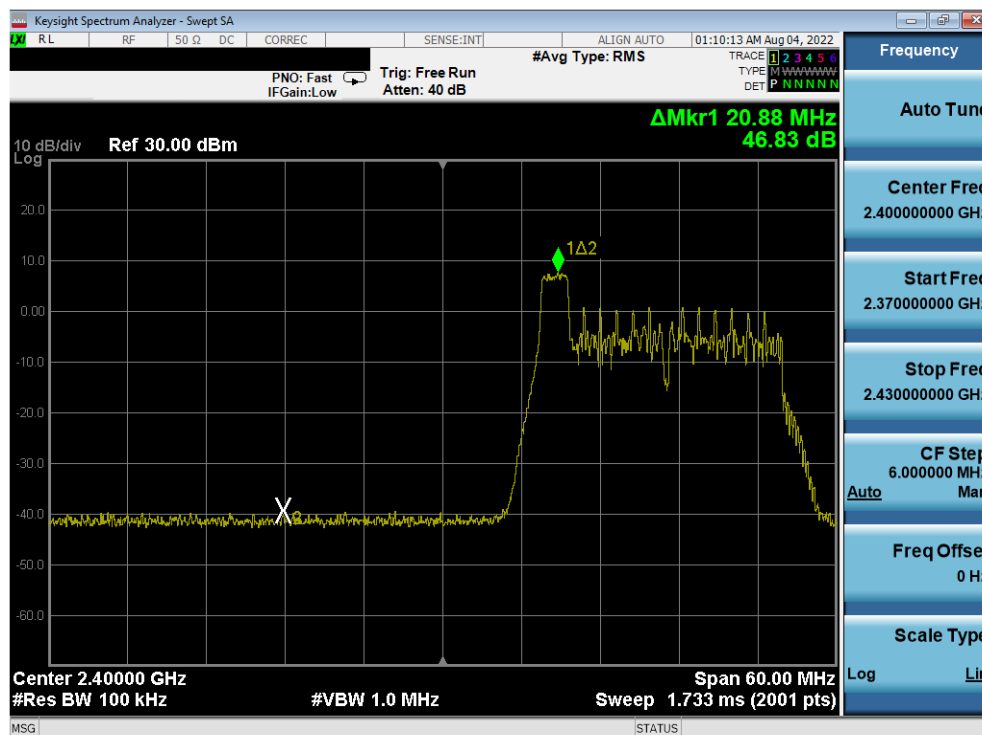
Plot 7-92. Band Edge Antenna WF7 (802.11ax OFDMA – RU26 Index 0 – Ch. 2)
