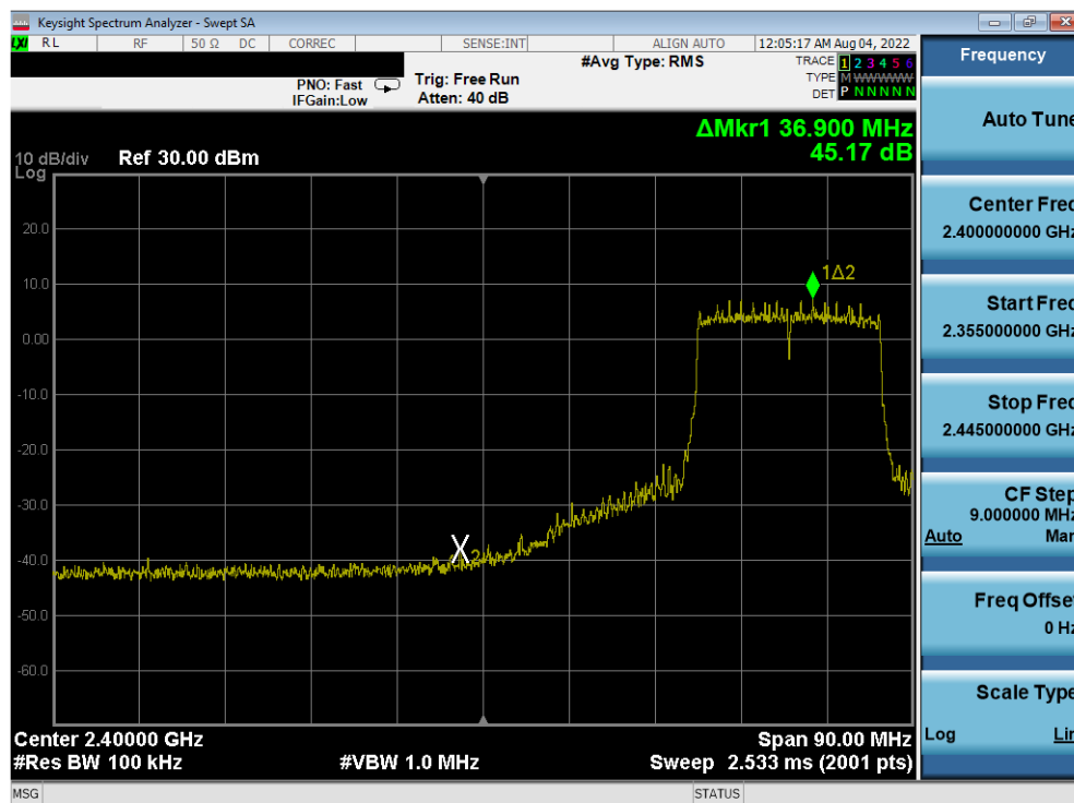
Plot 7-82. Band Edge Antenna WF8(802.11ax OFDMA – RU242 – Ch. 5)
