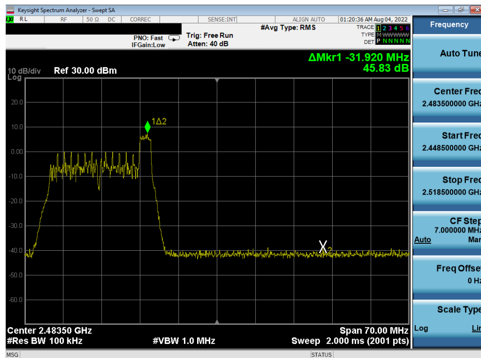
Plot 7-94. Band Edge Antenna WF7 (802.11ax OFDMA – RU26 Index 8 – Ch. 11)
