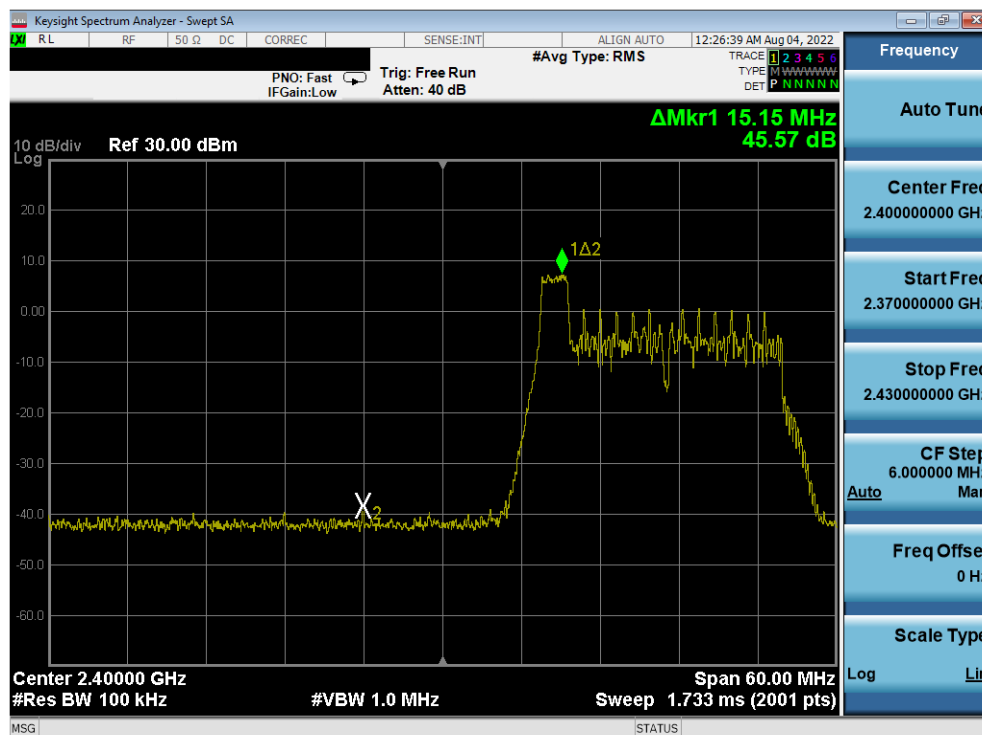
Plot 7-74. Band Edge Antenna WF8 (802.11ax OFDMA – RU26 Index 0 – Ch. 2)
