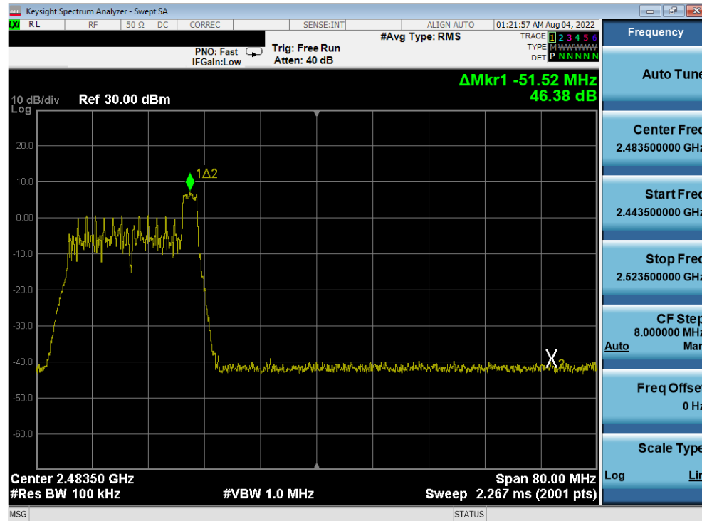
Plot 7-93. Band Edge Antenna WF7 (802.11ax OFDMA – RU26 Index 8 – Ch. 10)
