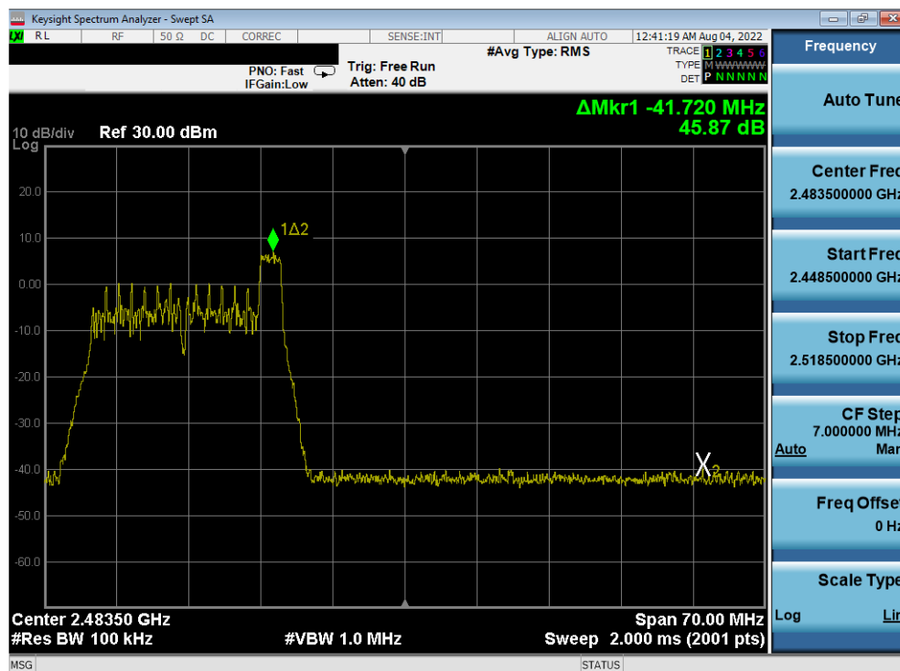
Plot 7-76. Band Edge Antenna WF8(802.11ax OFDMA – RU26 Index 8 – Ch. 11)
