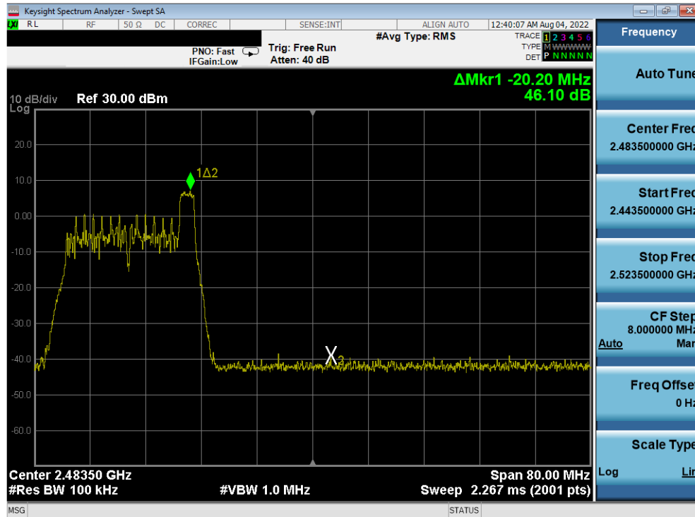
Plot 7-75. Band Edge Antenna WF8 (802.11ax OFDMA – RU26 Index 8 – Ch. 10)
