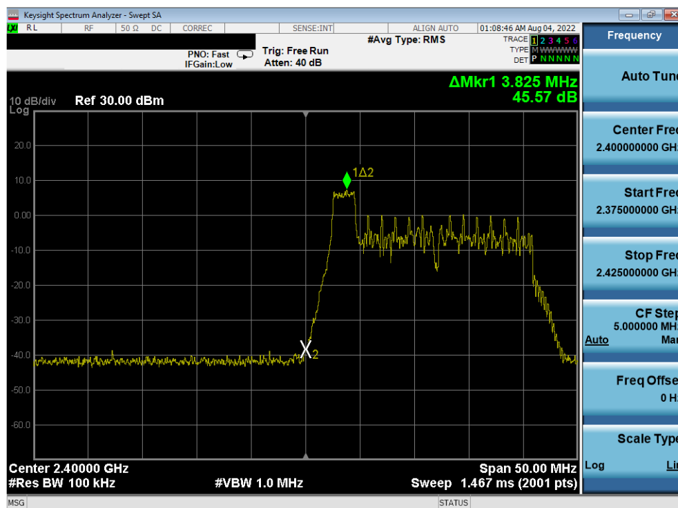
Plot 7-91. Band Edge Antenna WF7 (802.11ax OFDMA – RU26 Index 0 – Ch. 1)
