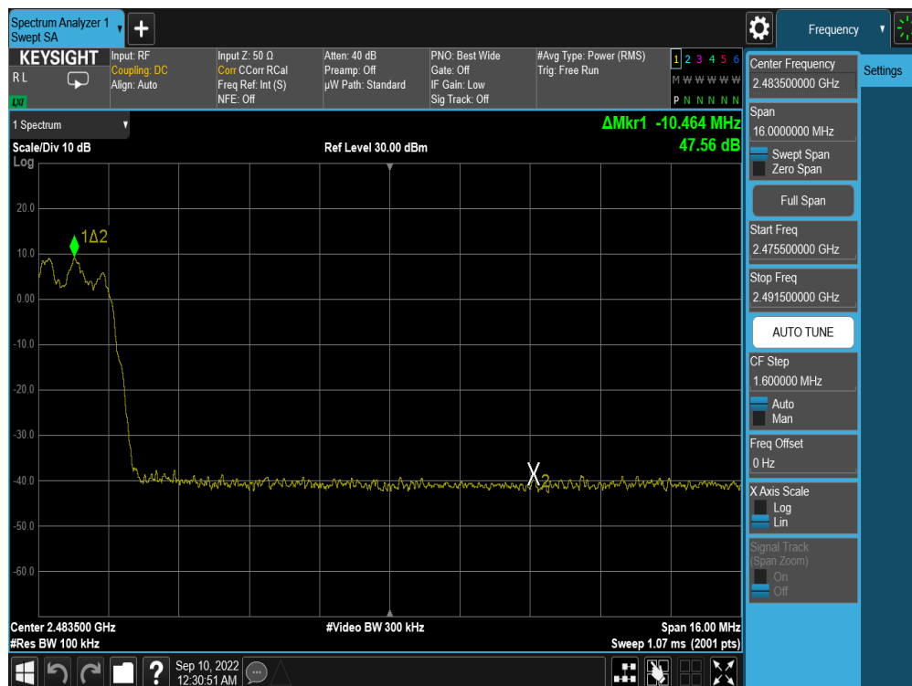
Plot 7-66. Band Edge Plot Antenna WF7 (Bluetooth (HDR4), ePA – Ch. 73)
