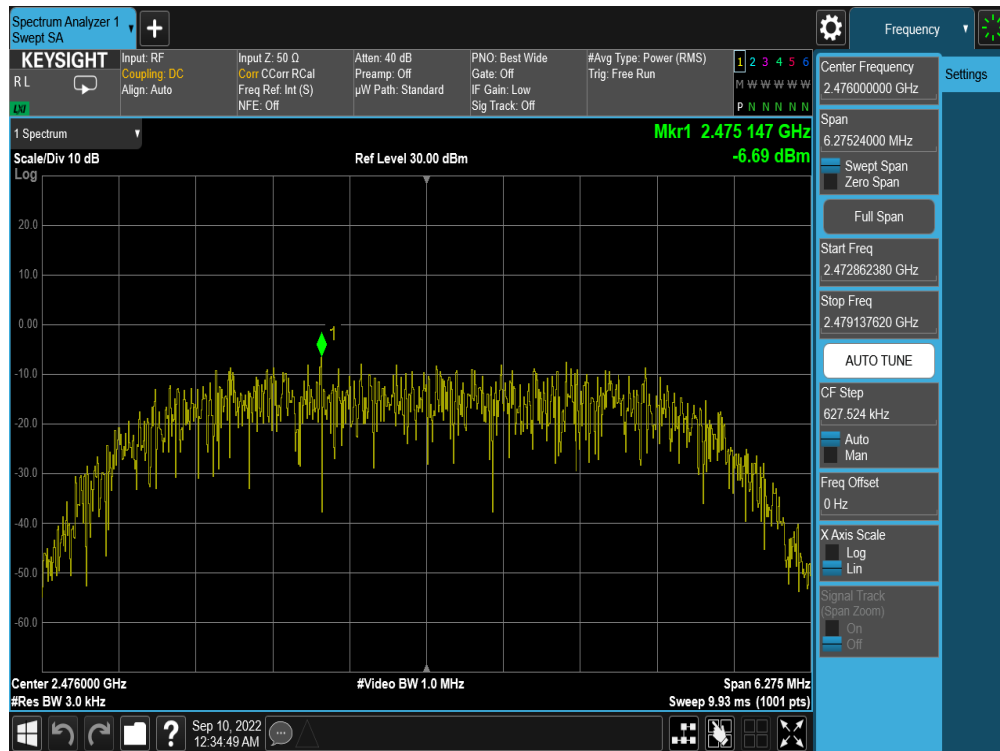
Plot 7-33. Power Spectral Density Plot Antenna WF7 (Bluetooth (HDR8), 8Mbps, ePA – Ch. 73)
