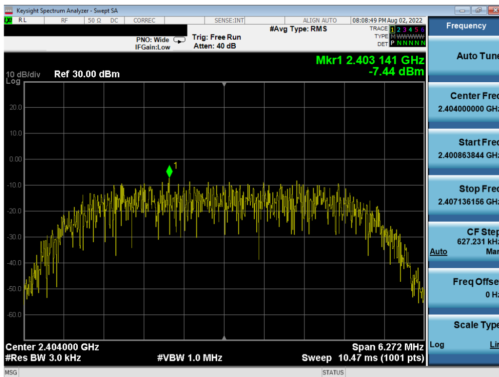
Plot 7-50. Power Spectral Density Plot TxBF Antenna WF7 (Bluetooth (HDR8), 8Mbps, ePA – Ch. 1)
