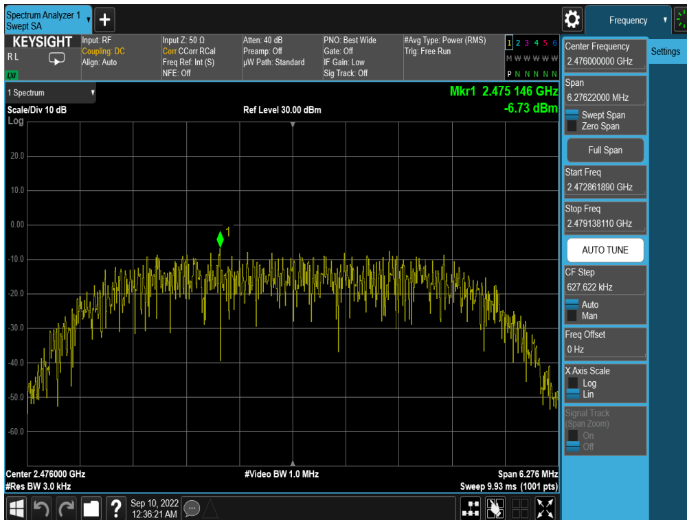
Plot 7-60. Power Spectral Density Plot TxBF Antenna WF7 (Bluetooth (HDR8), 8Mbps, iPA – Ch. 73)
