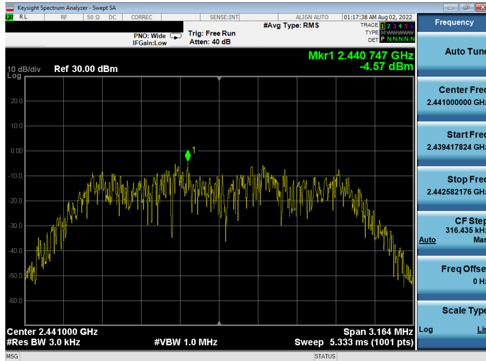
Plot 7-29. Power Spectral Density Plot Antenna WF7 (Bluetooth (HDR4), 4Mbps, iPA – Ch. 38)
