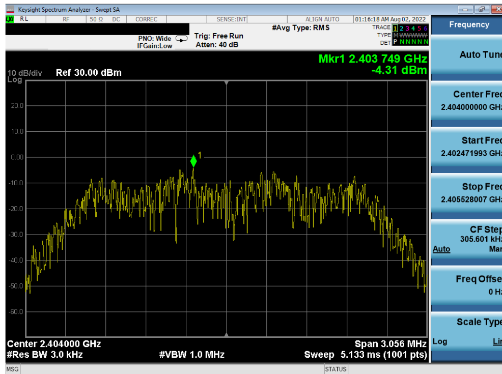
Plot 7-28. Power Spectral Density Plot Antenna WF7 (Bluetooth (HDR4), 4Mbps, iPA – Ch. 1)
