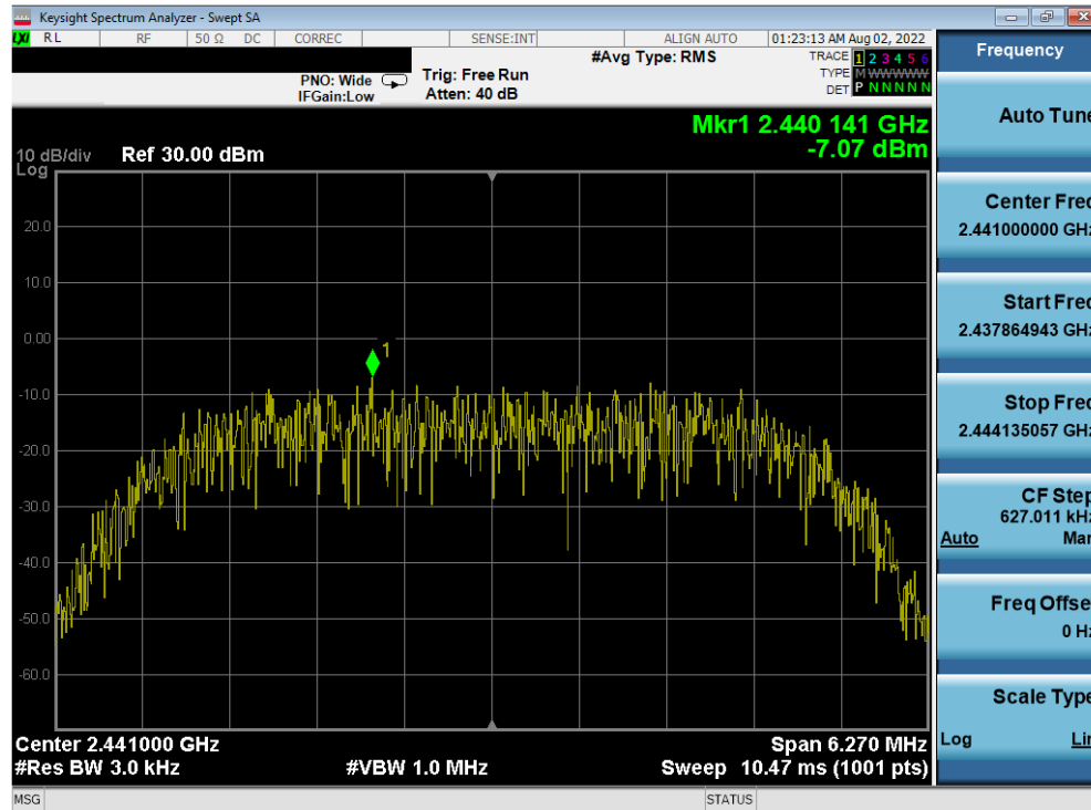
Plot 7-35. Power Spectral Density Plot Antenna WF7 (Bluetooth (HDR8), 8Mbps, iPA – Ch. 38)
