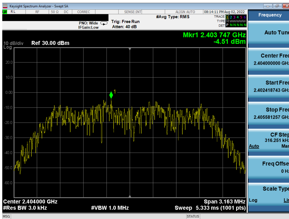
Plot 7-44. Power Spectral Density Plot TxBF Antenna WF7 (Bluetooth (HDR4), 4Mbps, iPA – Ch. 1)
