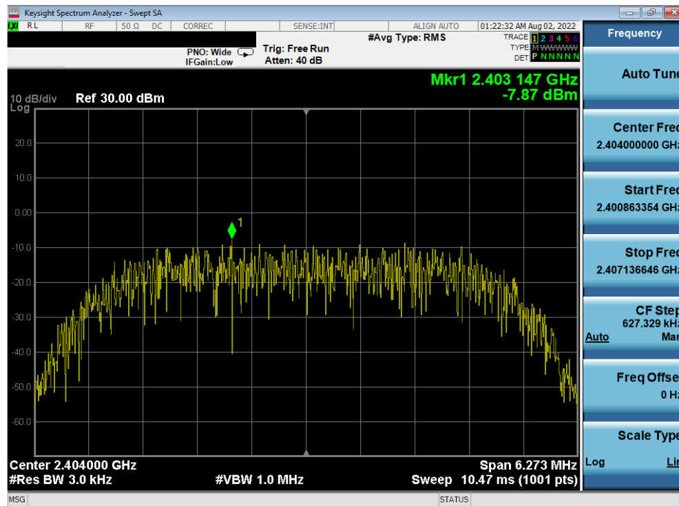
Plot 7-34. Power Spectral Density Plot Antenna WF7 (Bluetooth (HDR8), 8Mbps, iPA – Ch. 1)
