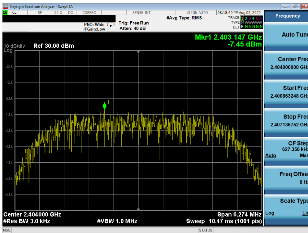
Plot 7-56. Power Spectral Density Plot TxBF Antenna WF7 (Bluetooth (HDR8), 8Mbps, iPA – Ch. 1)
