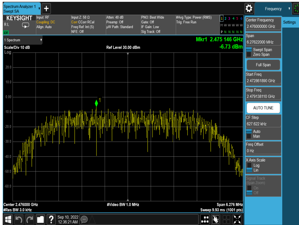
Plot 7-36. Power Spectral Density Plot Antenna WF7 (Bluetooth (HDR8), 8Mbps, iPA – Ch. 73)
