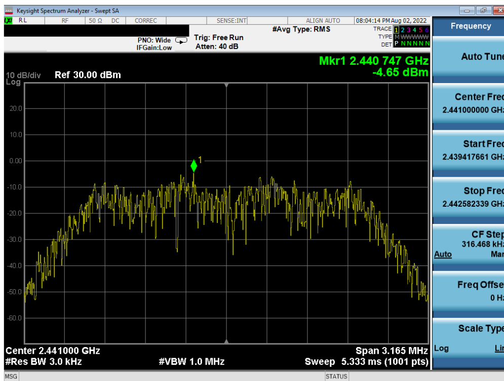
Plot 7-40. Power Spectral Density Plot TxBF Antenna WF7 (Bluetooth (HDR4), 4Mbps, ePA – Ch. 38)
