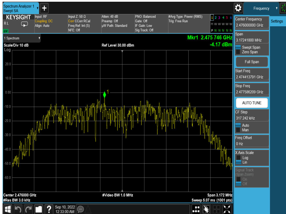
Plot 7-30. Power Spectral Density Plot Antenna WF7 (Bluetooth (HDR4), 4Mbps, iPA – Ch. 73)
