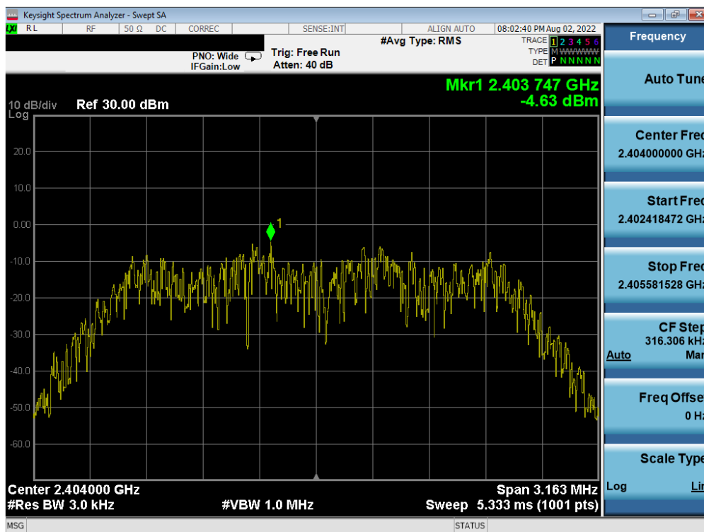
Plot 7-38. Power Spectral Density Plot TxBF Antenna WF7 (Bluetooth (HDR4), 4Mbps, ePA – Ch. 1)
