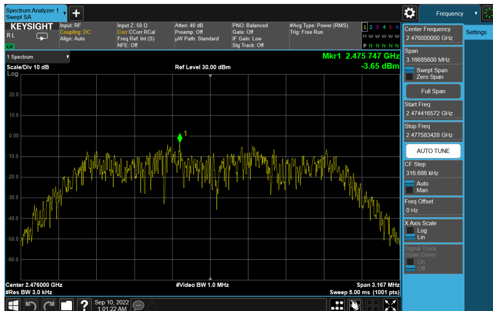
Plot 7-42. Power Spectral Density Plot TxBF Antenna WF7 (Bluetooth (HDR4), 4Mbps, ePA – Ch. 73)
