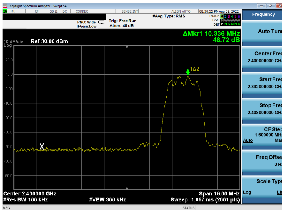
Plot 7-65. Band Edge Plot Antenna WF7 (Bluetooth (HDR4), ePA – Ch. 1)
