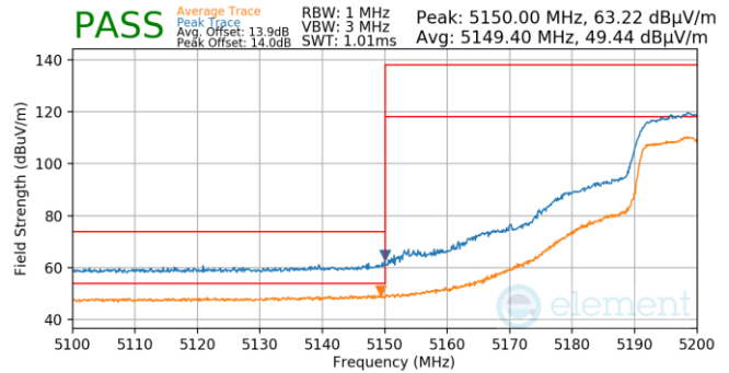
Plot 7-891. Antenna WF5B (Pk & Avg, Ch.40, 802.11n, MCS2)
