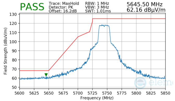
Plot 7-916. Antenna WF5B (Pk, Ch.149, 802.11n, MCS7)
