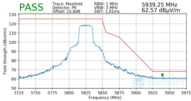
Plot 7-957. Antenna WF5B (Pk, Ch.165, 802.11ax(SU), MCS11)
