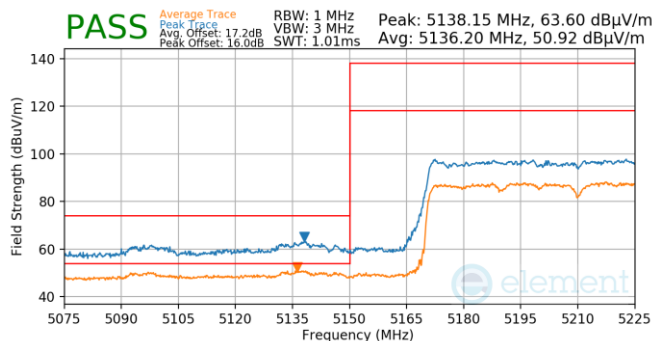
Plot 7-881. Antenna WF5T (Pk & Avg, Ch.50, 802. ax(SU), MCS9)
