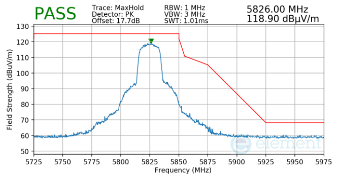
Plot 7-917. Antenna WF5B (Pk, Ch.165, 802.11n, MCS2)
