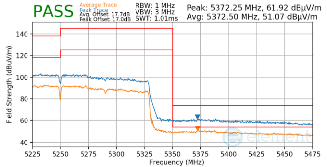
Plot 7-882. Antenna WF5T (Pk & Avg, Ch.50, 802.11 ax(SU), MCS2)
