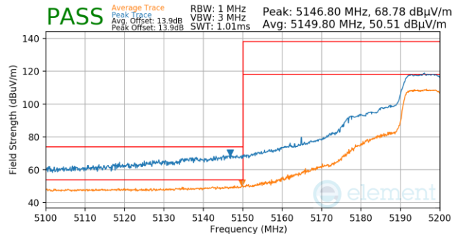
Plot 7-893. Antenna WF5B (Pk & Avg, Ch.40, 802.11n, MCS7)
