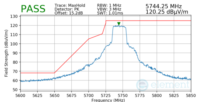
Plot 7-954. Antenna WF5B (Pk, Ch.149, 802.11ax(SU), MCS11)
