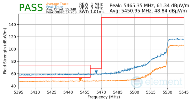
Plot 7-940. Antenna WF5B (Pk & Avg, Ch.108, 802.11ax(SU), MCS11)
