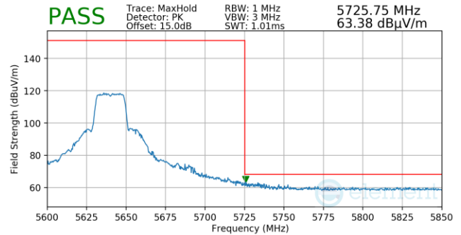
Plot 7-906. (FCC Only) Antenna WF5B (Pk, Ch.128, 802.11n, MCS7)
