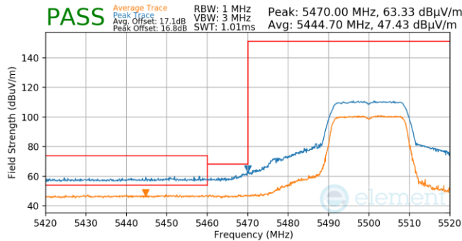
Plot 7-902. Antenna WF5B (Pk & Avg, Ch.100, 802.11n, MCS7)
