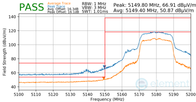
Plot 7-889. Antenna WF5B (Pk & Avg, Ch.36, 802.11n, MCS4)
