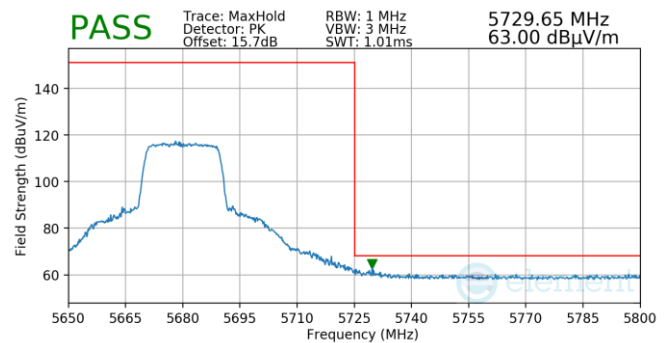
Plot 7-948. Antenna WF5B (Pk, Ch.136, 802.11ax(SU), MCS11)
