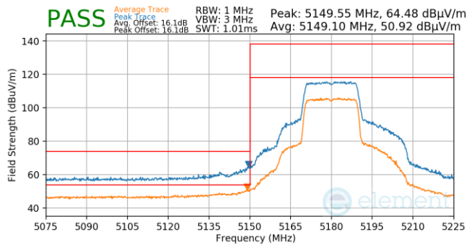
Plot 7-920. Antenna WF5B (Pk & Avg, Ch.36, 802.11ax(SU), MCS2)
