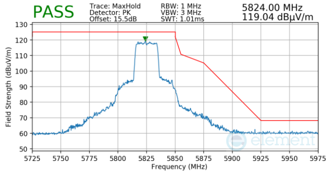
Plot 7-956. Antenna WF5B (Pk, Ch.165, 802.11ax(SU), MCS4)
