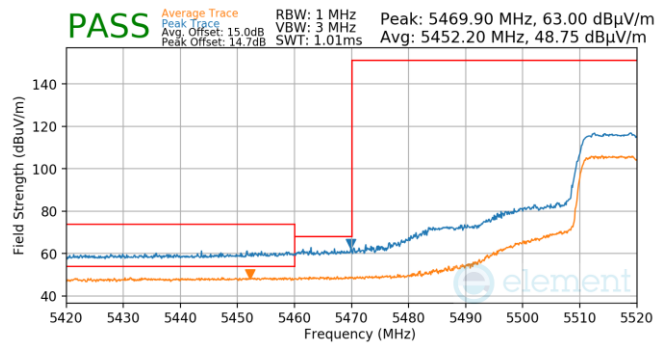
Plot 7-936. Antenna WF5B (Pk & Avg, Ch.104, 802.11ax(SU), MCS4)
