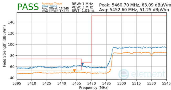
Plot 7-887. (FCC Only) Antenna WF5T (Pk & Avg, Ch.114, 802. ax(SU), MCS9)
