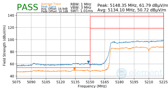
Plot 7-880. Antenna WF5T (Pk & Avg, Ch.50, 802. ax(SU), MCS4)
