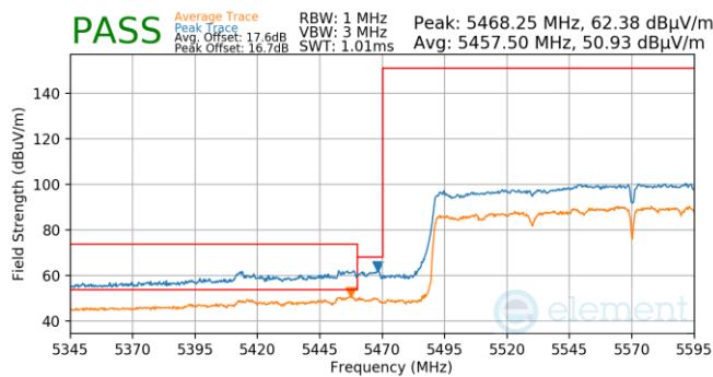
Plot 7-886. (FCC Only) Antenna WF5T (Pk & Avg, Ch.114, 802. ax(SU), MCS4)
