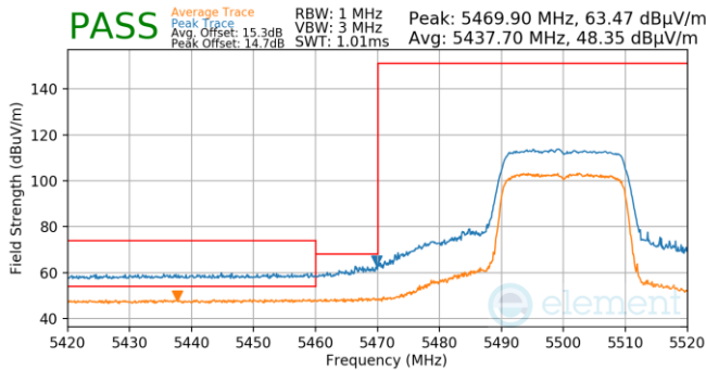
Plot 7-934. Antenna WF5B (Pk & Avg, Ch.100, 802.11ax(SU), MCS11)
