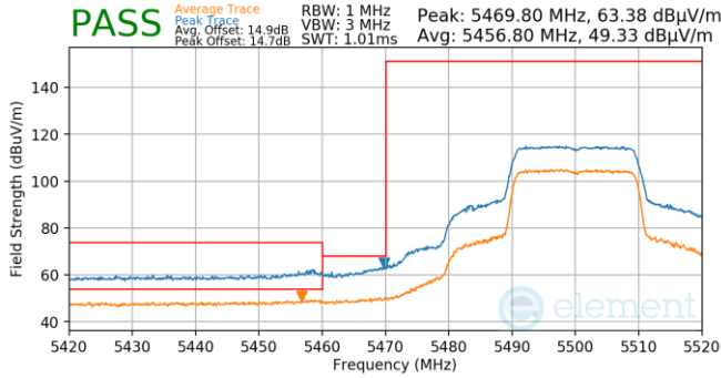
Plot 7-932. Antenna WF5B (Pk & Avg, Ch.100, 802.11ax(SU), MCS2)
