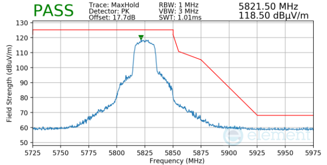
Plot 7-918. Antenna WF5B (Pk, Ch.165, 802.11n, MCS4)
