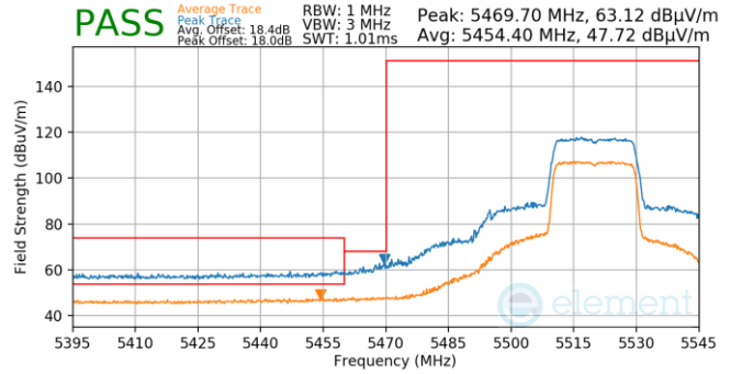
Plot 7-935. Antenna WF5B (Pk & Avg, Ch.104, 802.11ax(SU), MCS2)
