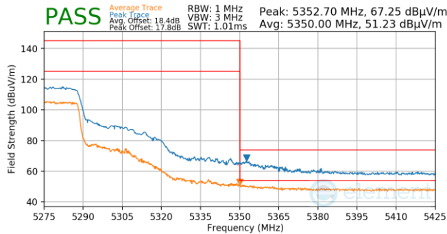
Plot 7-966. Antenna WF5B (Pk & Avg, Ch.54, 802.11n, MCS7)
