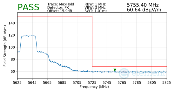
Plot 7-942. (FCC Only) Antenna WF5B (Pk, Ch.128, 802.11ax(SU), MCS11)
