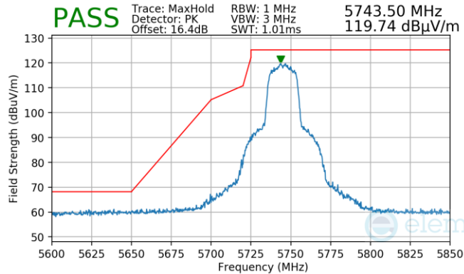
Plot 7-914. Antenna WF5B (Pk, Ch.149, 802.11n, MCS2)
