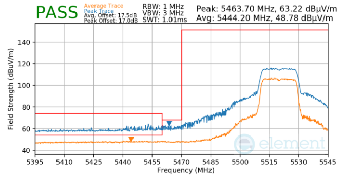
Plot 7-905. Antenna WF5B (Pk & Avg, Ch.104, 802.11n, MCS7)
