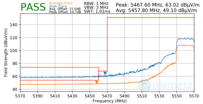
Plot 7-941. Antenna WF5B (Pk & Avg, Ch.112, 802.11ax(SU), MCS11)
