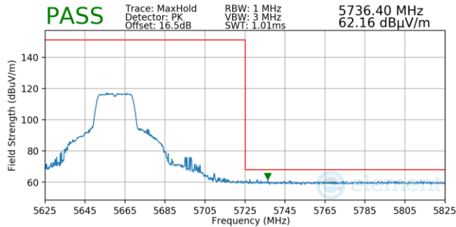
Plot 7-907. Antenna WF5B (Pk, Ch.132, 802.11n, MCS7)
