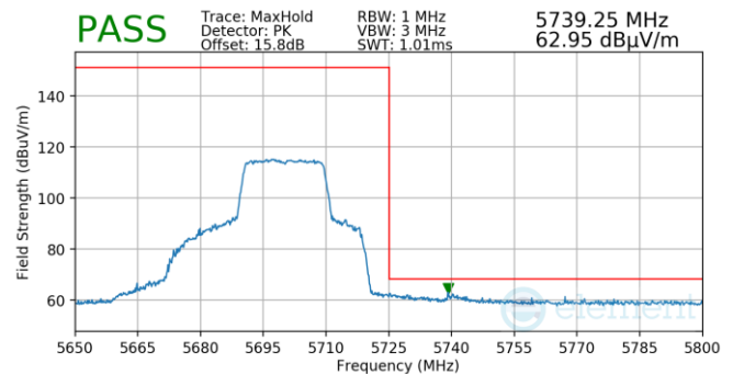
Plot 7-949. Antenna WF5B (Pk, Ch.140, 802.11ax(SU), MCS2)
