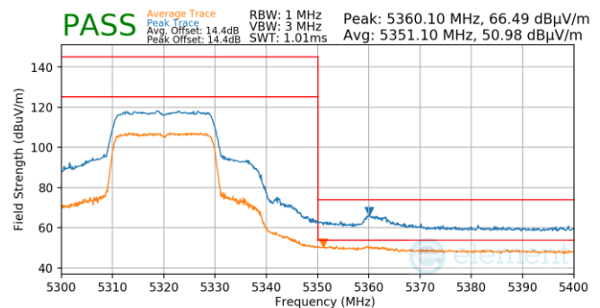
Plot 7-930. Antenna WF5B (Pk & Avg, Ch.64, 802.11ax(SU), MCS4)
