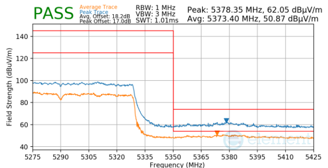
Plot 7-884. Antenna WF5T (Pk & Avg, Ch.50, 802. ax(SU), MCS9)
