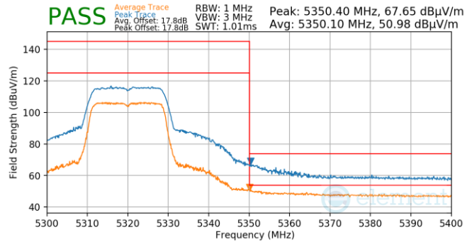
Plot 7-899. Antenna WF5B (Pk & Avg, Ch.64, 802.11n, MCS7)
