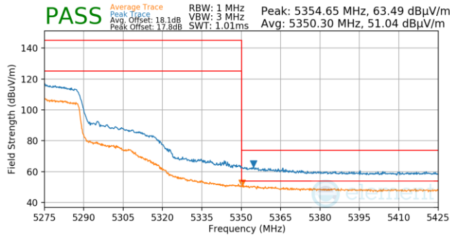
Plot 7-964. Antenna WF5B (Pk & Avg, Ch.54, 802.11n, MCS2)
