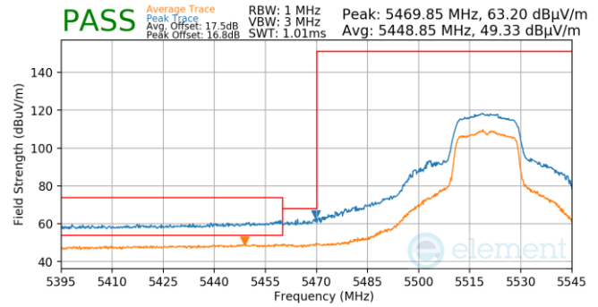
Plot 7-904. Antenna WF5B (Pk & Avg, Ch.104, 802.11n, MCS4)
