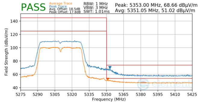
Plot 7-969. Antenna WF5B (Pk & Avg, Ch.62, 802.11n, MCS7)
