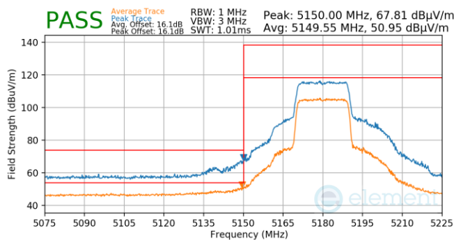
Plot 7-921. Antenna WF5B (Pk & Avg, Ch.36, 802.11ax(SU), MCS4)
