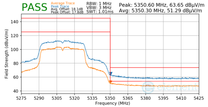
Plot 7-967. Antenna WF5B (Pk & Avg, Ch.62, 802.11n, MCS2)
