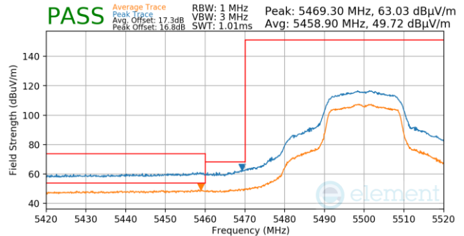
Plot 7-900. Antenna WF5B (Pk & Avg, Ch.100, 802.11n, MCS2)
