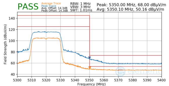
Plot 7-931. Antenna WF5B (Pk & Avg, Ch.64, 802.11ax(SU), MCS11)
