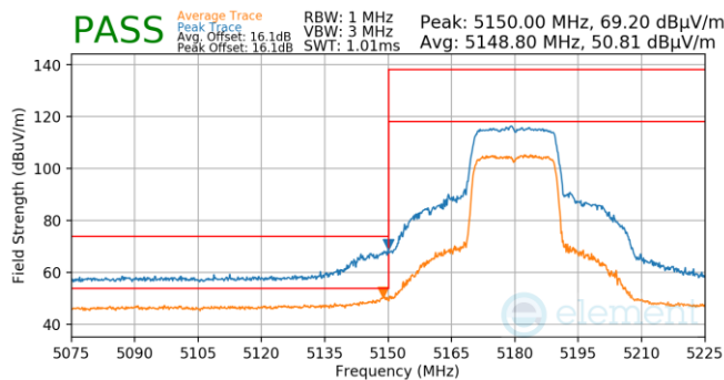
Plot 7-922. Antenna WF5B (Pk & Avg, Ch.36, 802.11ax(SU), MCS11)
