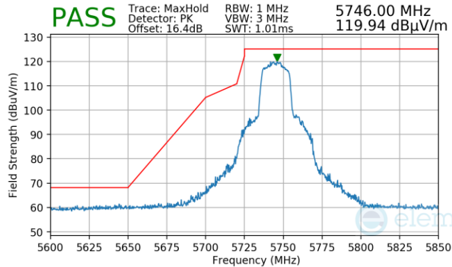
Plot 7-915. Antenna WF5B (Pk, Ch.149, 802.11n, MCS4)
