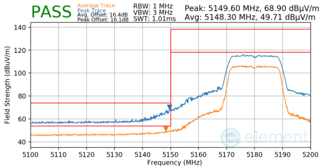
Plot 7-890. Antenna WF5B (Pk & Avg, Ch.36, 802.11n, MCS7)
