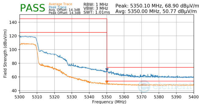
Plot 7-928. Antenna WF5B (Pk & Avg, Ch.60, 802.11ax(SU), MCS11)
