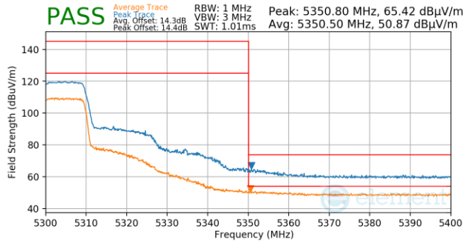
Plot 7-926. Antenna WF5B (Pk & Avg, Ch.60, 802.11ax(SU), MCS2)
