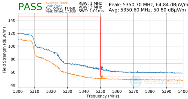
Plot 7-895. Antenna WF5B (Pk & Avg, Ch.60, 802.11n, MCS4)
