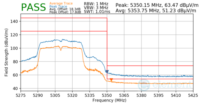
Plot 7-968. Antenna WF5B (Pk & Avg, Ch.62, 802.11n, MCS4)
