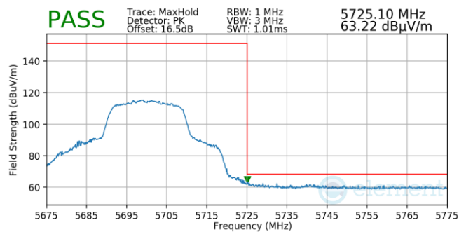
Plot 7-912. Antenna WF5B (Pk, Ch.140, 802.11n, MCS4)
