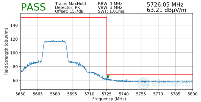
Plot 7-947. Antenna WF5B (Pk, Ch.136, 802.11ax(SU), MCS4)
