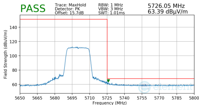
Plot 7-951. Antenna WF5B (Pk, Ch.140, 802.11ax(SU), MCS11)
