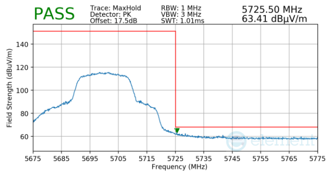
Plot 7-911. Antenna WF5B (Pk, Ch.140, 802.11n, MCS2)
