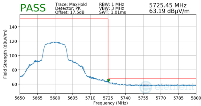
Plot 7-909. Antenna WF5B (Pk, Ch.136, 802.11n, MCS4)
