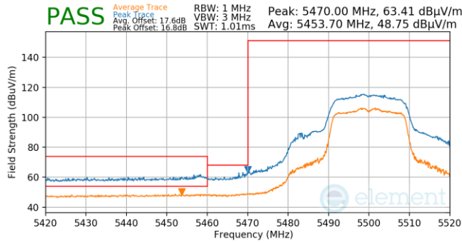
Plot 7-901. Antenna WF5B (Pk & Avg, Ch.100, 802.11n, MCS4)
