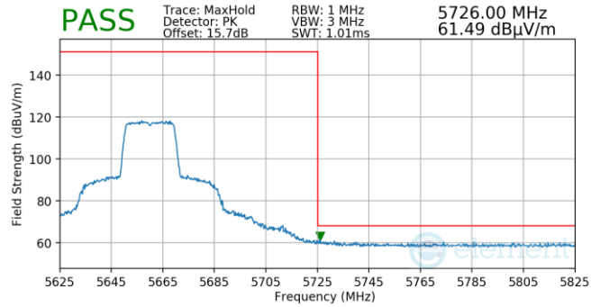
Plot 7-943. Antenna WF5B (Pk, Ch.132, 802.11ax(SU), MCS2)
