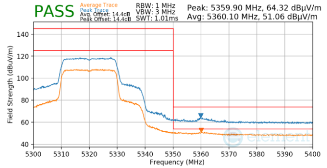
Plot 7-929. Antenna WF5B (Pk & Avg, Ch.64, 802.11ax(SU), MCS2)
