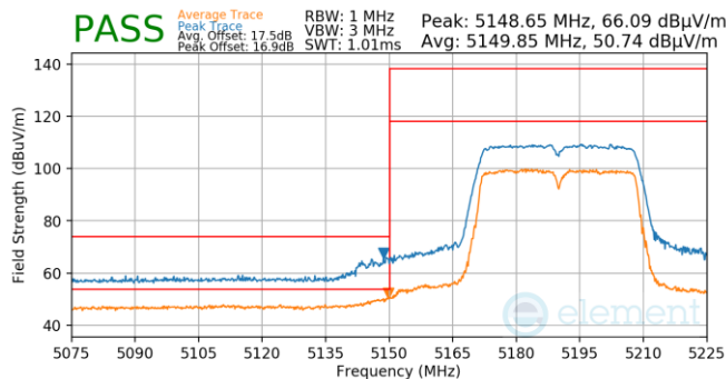
Plot 7-960. Antenna WF5B (Pk & Avg, Ch.38, 802.11n, MCS7)
