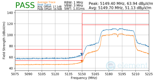
Plot 7-958. Antenna WF5B (Pk & Avg, Ch.38, 802.11n, MCS2)
