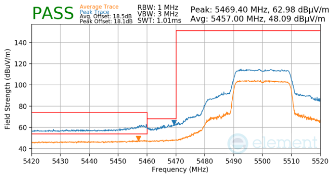
Plot 7-933. Antenna WF5B (Pk & Avg, Ch.100, 802.11ax(SU), MCS4)
