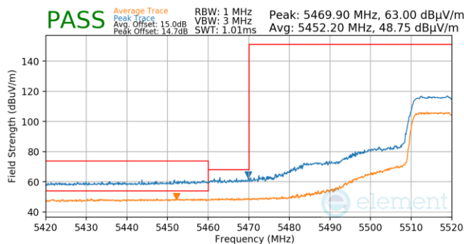
Plot 7-939. Antenna WF5B (Pk & Avg, Ch.108, 802.11ax(SU), MCS4)
