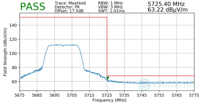
Plot 7-913. Antenna WF5B (Pk, Ch.140, 802.11n, MCS7)
