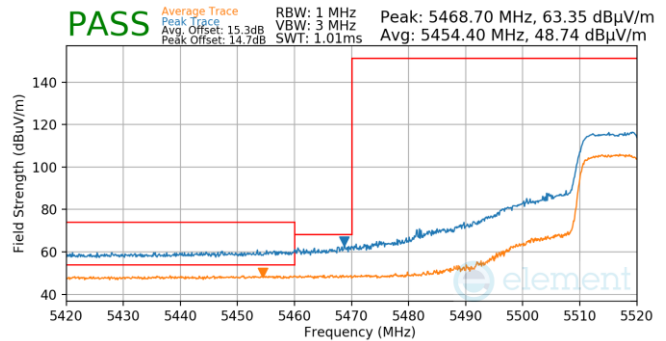
Plot 7-937. Antenna WF5B (Pk & Avg, Ch.104, 802.11ax(SU), MCS11)
