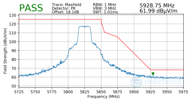
Plot 7-919. Antenna WF5B (Pk, Ch.165, 802.11n, MCS7)
