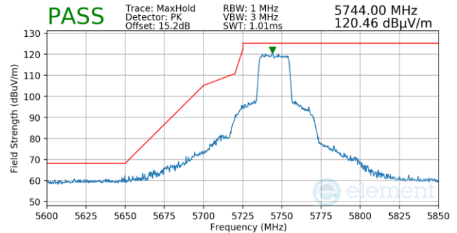
Plot 7-953. Antenna WF5B (Pk, Ch.149, 802.11ax(SU), MCS4)
