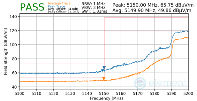
Plot 7-892. Antenna WF5B (Pk & Avg, Ch.40, 802.11n, MCS4)
