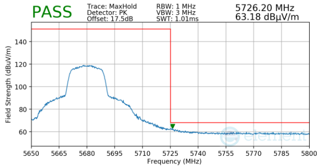
Plot 7-908. Antenna WF5B (Pk, Ch.136, 802.11n, MCS2)
