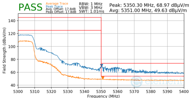
Plot 7-896. Antenna WF5B (Pk & Avg, Ch.60, 802.11n, MCS7)
