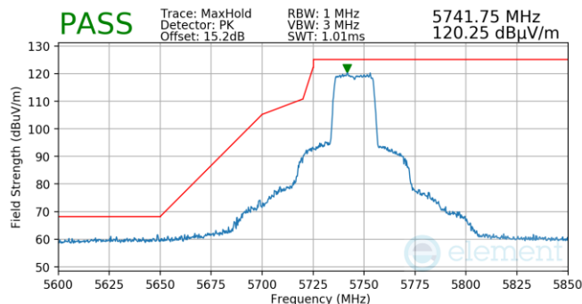
Plot 7-952. Antenna WF5B (Pk, Ch.149, 802.11ax(SU), MCS2)
