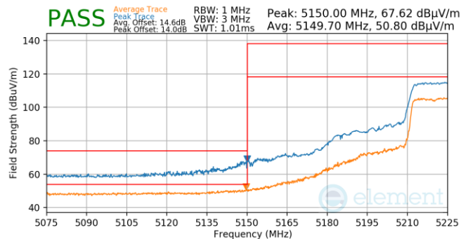
Plot 7-963. Antenna WF5B (Pk & Avg, Ch.46, 802.11n, MCS7)
