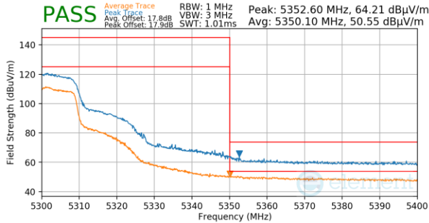
Plot 7-894. Antenna WF5B (Pk & Avg, Ch.60, 802.11n, MCS2)
