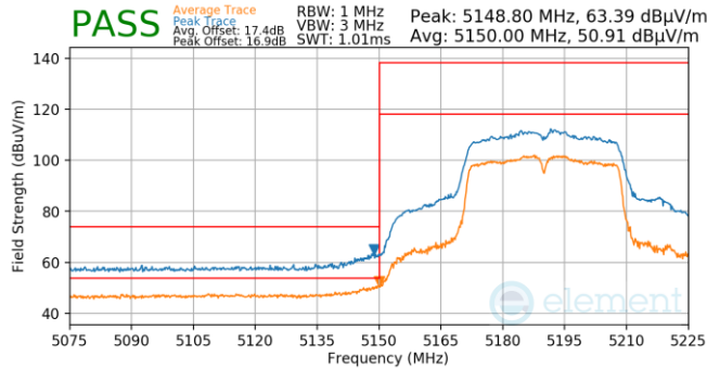
Plot 7-959. Antenna WF5B (Pk & Avg, Ch.38, 802.11n, MCS4)
