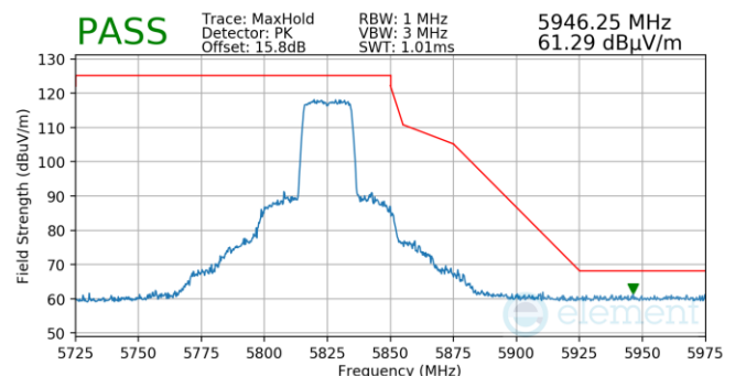
Plot 7-955. Antenna WF5B (Pk, Ch.165, 802.11ax(SU), MCS2)
