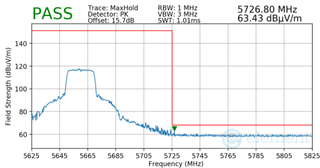
Plot 7-945. Antenna WF5B (Pk, Ch.132, 802.11ax(SU), MCS11)
