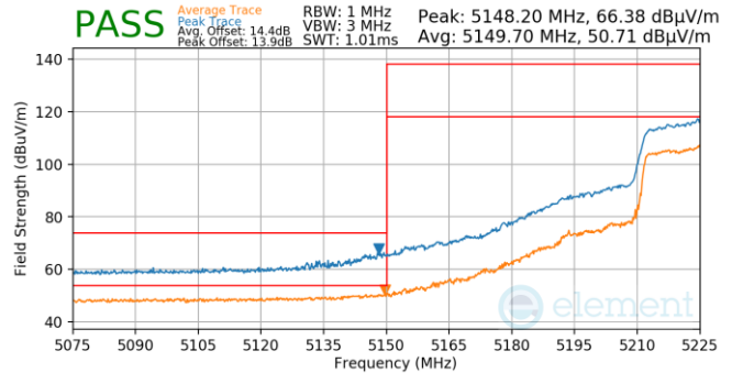
Plot 7-962. Antenna WF5B (Pk & Avg, Ch.46, 802.11n, MCS4)
