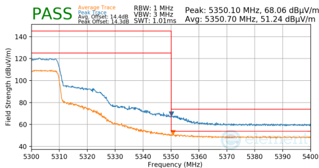
Plot 7-927. Antenna WF5B (Pk & Avg, Ch.60, 802.11ax(SU), MCS4)
