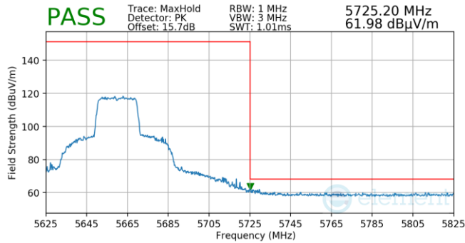
Plot 7-944. Antenna WF5B (Pk, Ch.132, 802.11ax(SU), MCS4)
