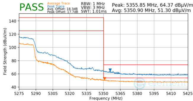
Plot 7-965. Antenna WF5B (Pk & Avg, Ch.54, 802.11n, MCS4)
