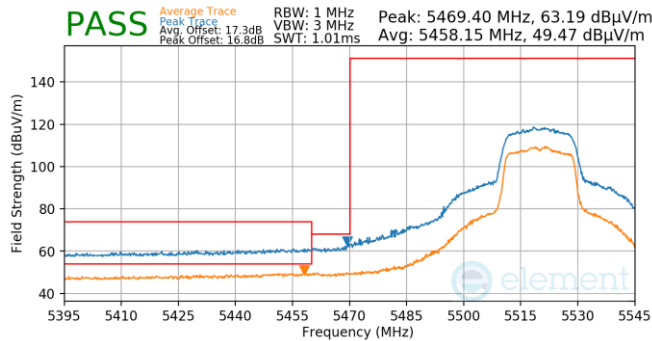
Plot 7-903. Antenna WF5B (Pk & Avg, Ch.104, 802.11n, MCS2)
