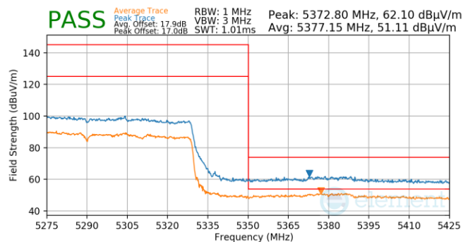
Plot 7-883. Antenna WF5T (Pk & Avg, Ch.50, 802. ax(SU), MCS4)
