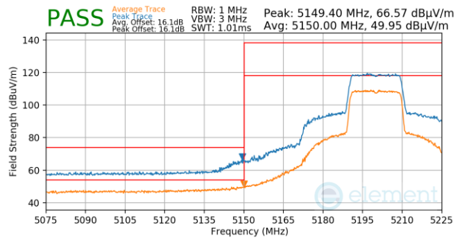
Plot 7-923. Antenna WF5B (Pk & Avg, Ch.40, 802.11ax(SU), MCS2)
