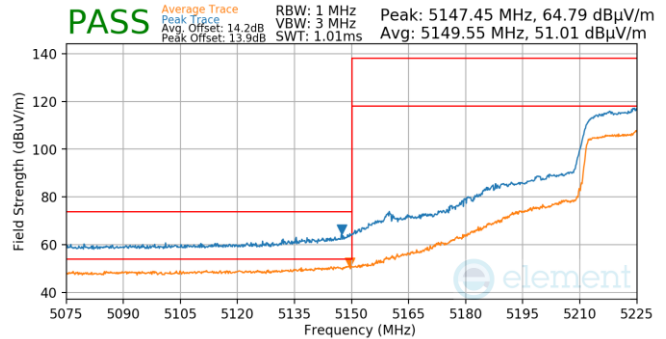
Plot 7-961. Antenna WF5B (Pk & Avg, Ch.46, 802.11n, MCS2)
