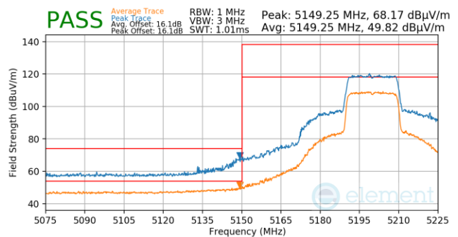
Plot 7-924. Antenna WF5B (Pk & Avg, Ch.40, 802.11ax(SU), MCS4)
