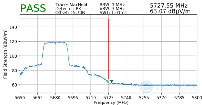
Plot 7-946. Antenna WF5B (Pk, Ch.136, 802.11ax(SU), MCS2)
