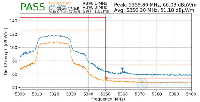
Plot 7-898. Antenna WF5B (Pk & Avg, Ch.64, 802.11n, MCS4)
