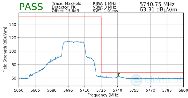
Plot 7-950. Antenna WF5B (Pk, Ch.140, 802.11ax(SU), MCS4)
