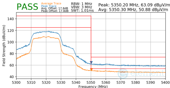
Plot 7-897. Antenna WF5B (Pk & Avg, Ch.64, 802.11n, MCS2)
