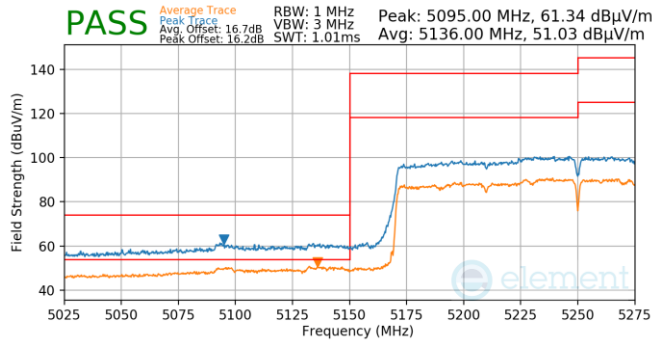
Plot 7-879. Antenna WF5T (Pk & Avg, Ch.50, 802.11ax(SU), MCS2)
