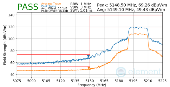
Plot 7-925. Antenna WF5B (Pk & Avg, Ch.40, 802.11ax(SU), MCS11)
