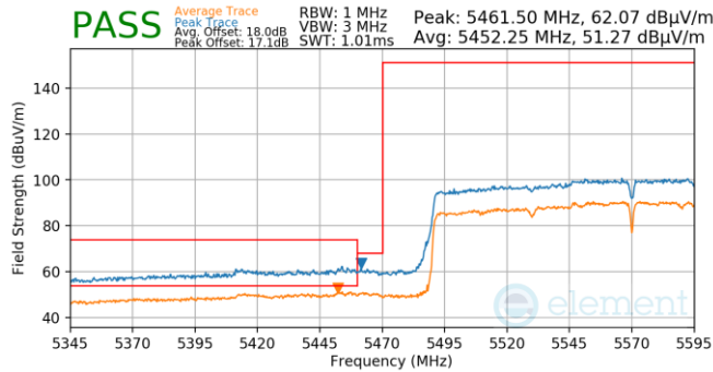
Plot 7-885. (FCC Only) Antenna WF5T (Pk & Avg, Ch.114, 802. ax(SU), MCS2)
