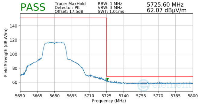
Plot 7-910. Antenna WF5B (Pk, Ch.136, 802.11n, MCS7)
