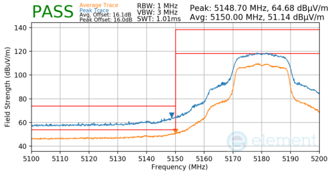
Plot 7-888. Antenna WF5B (Pk & Avg, Ch.36, 802.11n, MCS2)
