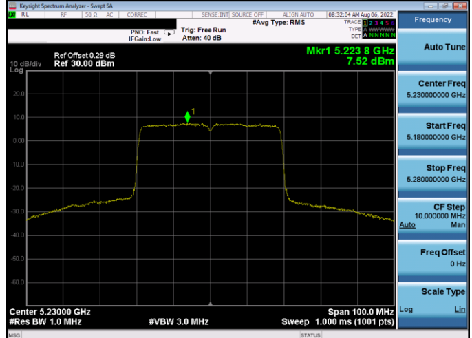
Plot 7-172. PSD Antenna WF5T (40MHz BW 802.11ax(SU) – Ch. 46, MCS2)
