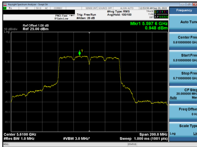
Plot 7-187. PSD Antenna WF5T (80MHz BW 802.11ac – Ch. 122, MCS2)
