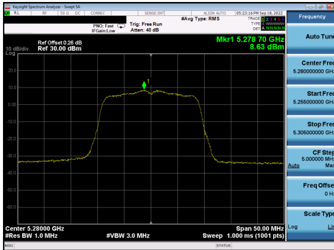
Plot 7-199. PSD Antenna WF5T (20MHz BW 802.11n – Ch. 56, MCS4)
