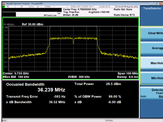
Plot 7-165. 6dB BW & 99% OBW Antenna WF5B (40MHz BW 802.11n - Ch. 151, MCS7)
