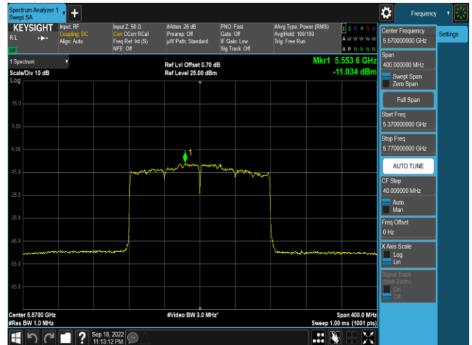
Plot 7-190. PSD Antenna WF5T (160MHz BW 802.11ax(SU) – Ch. 114, MCS2)
