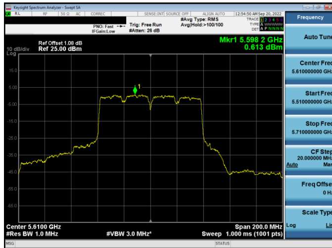
Plot 7-209. PSD Antenna WF5T (80MHz BW 802.11ac – Ch. 122, MCS4)
