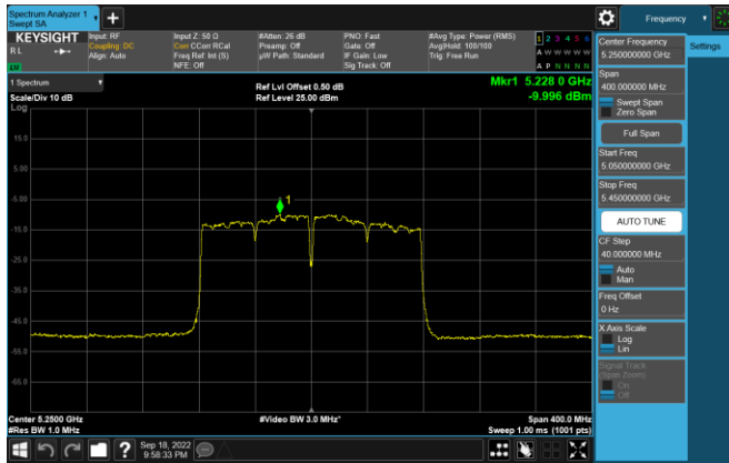
Plot 7-175. PSD Antenna WF5T (160MHz BW 802.11ac - Ch. 50, MCS2)
