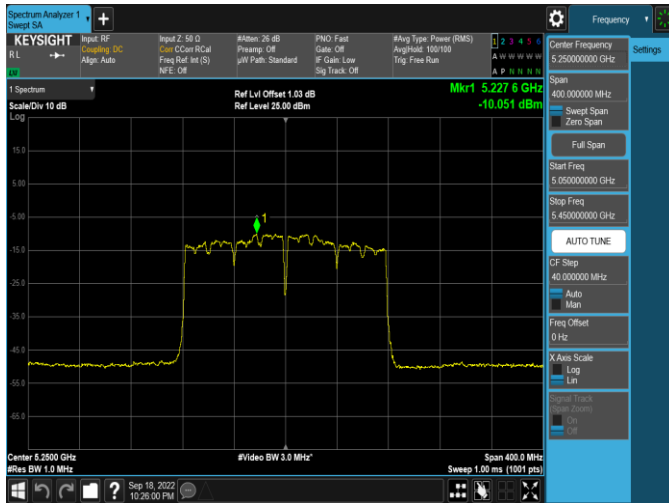
Plot 7-197. PSD Antenna WF5T (160MHz BW 802.11ac – Ch. 50, MCS4)
