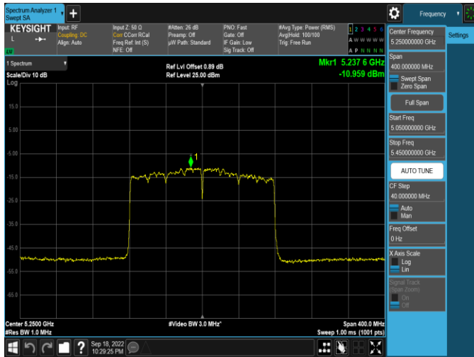
Plot 7-198. PSD Antenna WF5T (160MHz BW 802.11ax(SU) – Ch. 50, MCS4)
