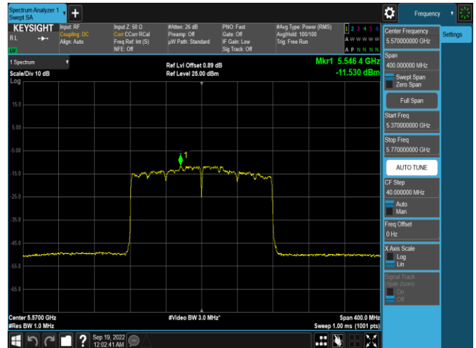
Plot 7-212. PSD Antenna WF5T (160MHz BW 802.11ax(SU) – Ch. 114, MCS4)
