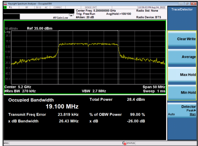
Plot 7-40. 26dB BW & 99% OBW Antenna 3a (20MHz BW 11ax– RU242 – Ch.40)
