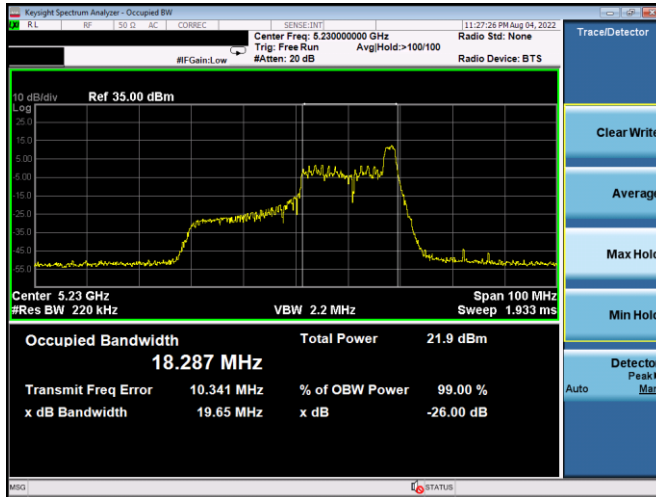
Plot 7-43. 26dB BW & 99% OBW Antenna 3a (40MHz BW 11ax Index 17 – RU26 – Ch.46)
