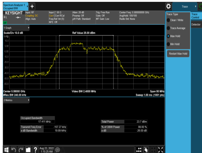
Plot 7-26. 26dB BW & 99% OBW Antenna 3c (20MHz BW 11ax Index 38 – RU52 – Ch.116)
