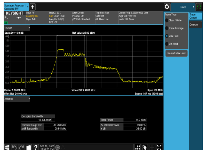
Plot 7-29. 26dB BW & 99% OBW Antenna 3c (40MHz BW 11ax Index 37 – RU52 – Ch.110)
