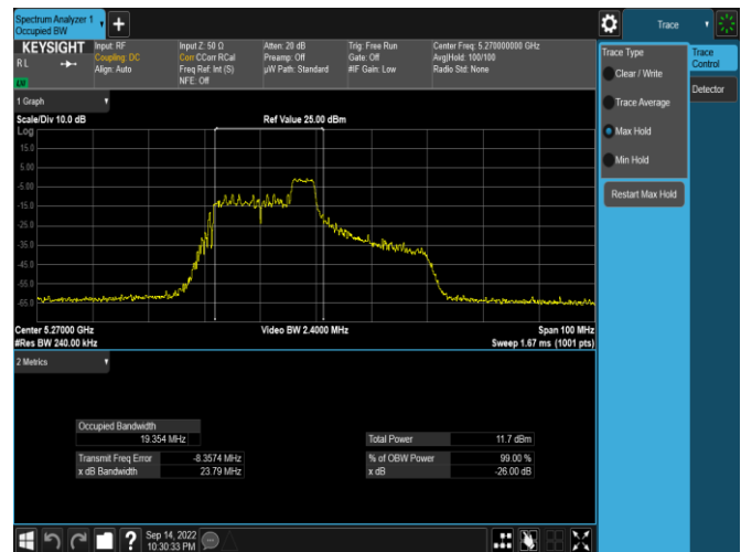
Plot 7-18. 26dB BW & 99% OBW Antenna 3c (40MHz BW 11ax Index 40 – RU52 – Ch.54)
