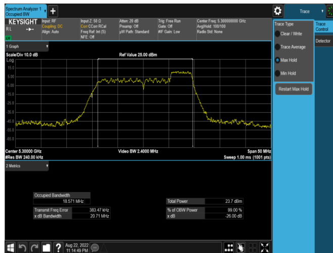
Plot 7-15. 26dB BW & 99% OBW Antenna 3c (20MHz BW 11ax Index 40 – RU52 – Ch.60)
