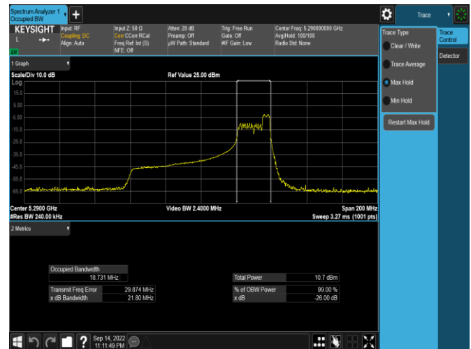
Plot 7-23. 26dB BW & 99% OBW Antenna 3c (80MHz BW 11ax Index 52 – RU52 – Ch.58)
