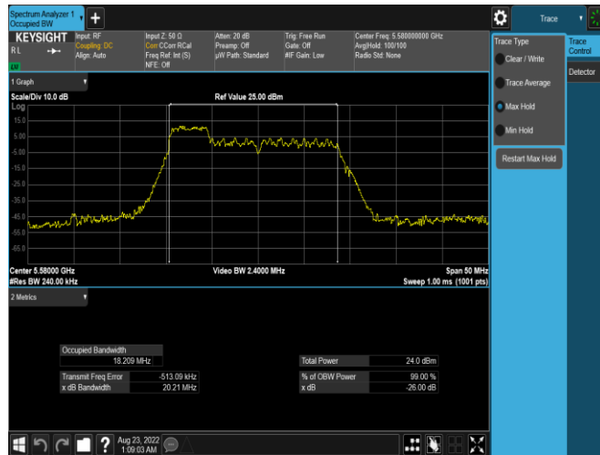
Plot 7-25. 26dB BW & 99% OBW Antenna 3c (20MHz BW 11ax Index 37 – RU52 – Ch.116)
