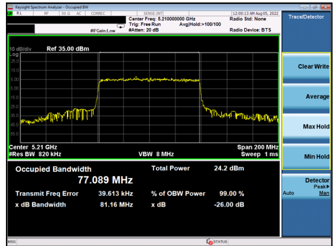
Plot 7-48. 26dB BW & 99% OBW Antenna 3a (80MHz BW 11ax – RU996 – Ch.42)
