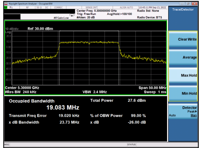
Plot 7-52: 26dB BW & 99% OBW Antenna 3a (20MHz BW 11ax – RU242 – Ch.60)
