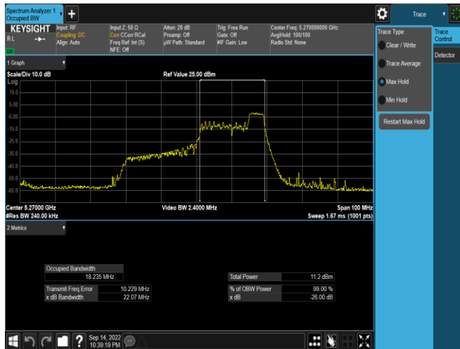
Plot 7-19. 26dB BW & 99% OBW Antenna 3c (40MHz BW 11ax Index 44 – RU52 – Ch.54)
