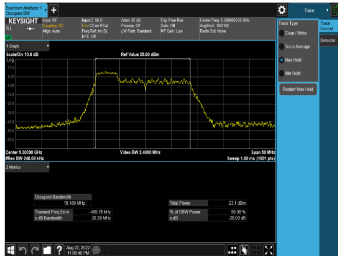
Plot 7-13. 26dB BW & 99% OBW Antenna 3c (20MHz BW 11ax Index 37 – RU52 – Ch.60)
