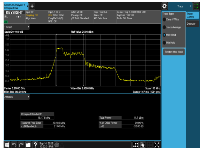
Plot 7-17. 26dB BW & 99% OBW Antenna 3c (40MHz BW 11ax Index 37 – RU52 – Ch.54)
