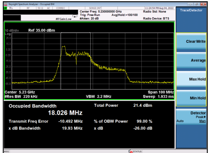
Plot 7-41. 26dB BW & 99% OBW Antenna 3a (40MHz BW 11ax Index 0 – RU26 – Ch.46)
