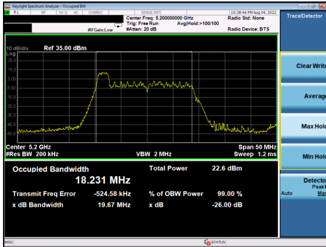
Plot 7-37. 26dB BW & 99% OBW Antenna 3a (20MHz BW 11ax Index 0 – RU26 – Ch.40)
