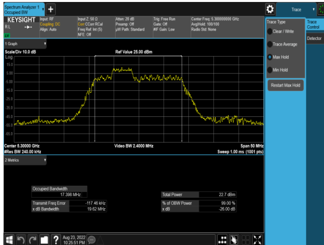
Plot 7-50: 26dB BW & 99% OBW Antenna 3a (20MHz BW 11ax Index 38 – RU52 – Ch.60)
