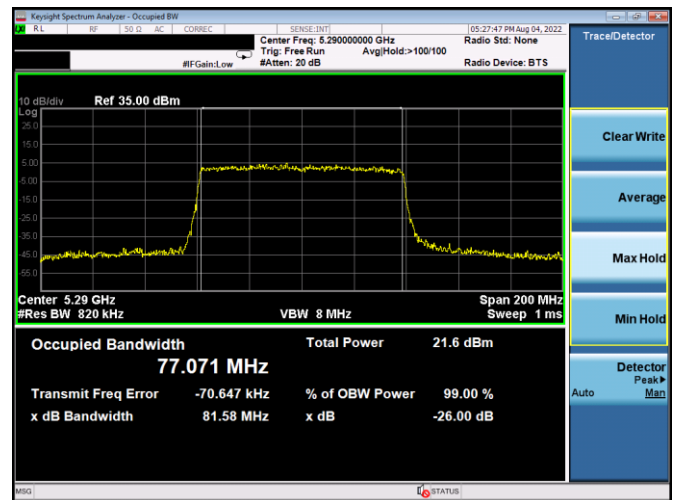
Plot 7-24. 26dB BW & 99% OBW Antenna 3c (80MHz BW 11ax – RU996 – Ch.58)
