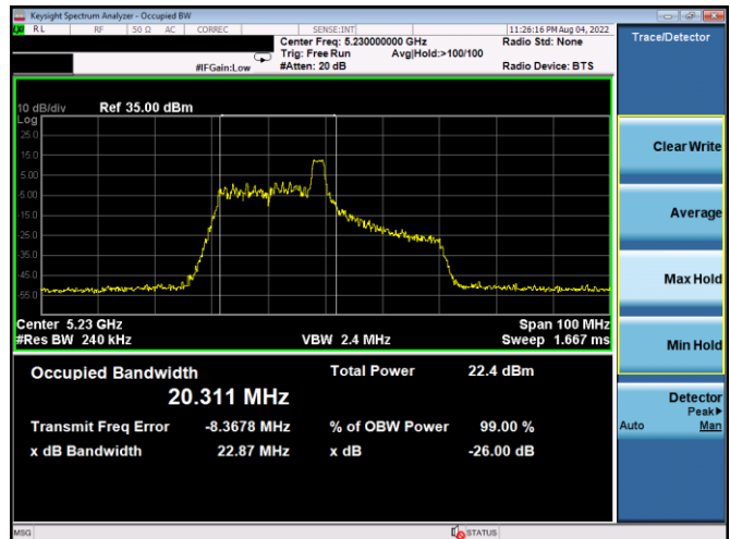
Plot 7-42. 26dB BW & 99% OBW Antenna 3a (40MHz BW 11ax Index 8 – RU26 – Ch.46)
