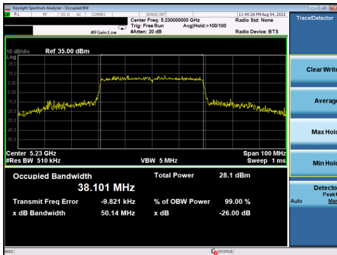
Plot 7-44. 26dB BW & 99% OBW Antenna 3a (40MHz BW 11ax – RU484 – Ch.46)
