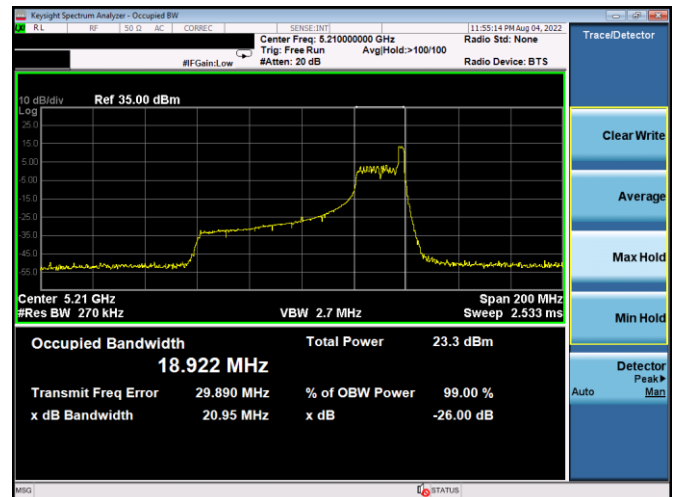
Plot 7-47. 26dB BW & 99% OBW Antenna 3a (80MHz BW 11ax Index 36 – RU26 – Ch.42)
