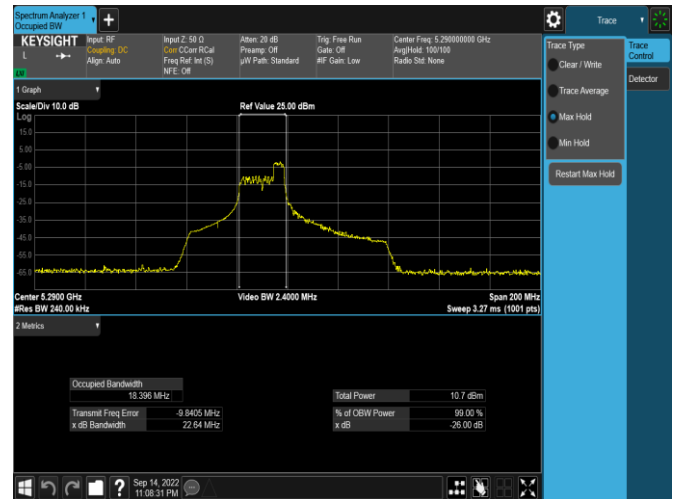
Plot 7-22. 26dB BW & 99% OBW Antenna 3c (80MHz BW 11ax Index 44 – RU52 – Ch.58)
