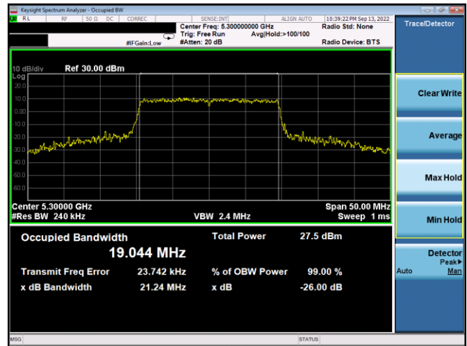
Plot 7-16. 26dB BW & 99% OBW Antenna 3c (20MHz BW 11ax – RU242 – Ch.60)
