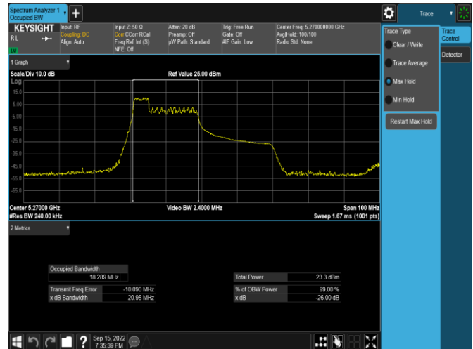
Plot 7-53: 26dB BW & 99% OBW Antenna 3a (40MHz BW 11ax Index 37 – RU52 – Ch.54)
