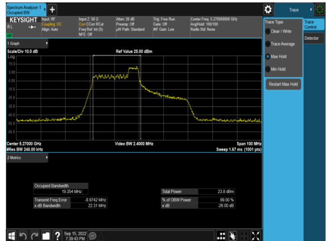
Plot 7-54: 26dB BW & 99% OBW Antenna 3a (40MHz BW 11ax Index 40 – RU52 – Ch.54)
