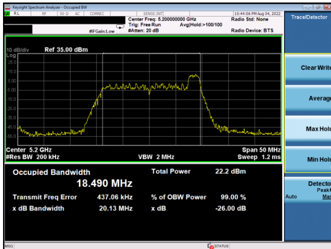
Plot 7-39. 26dB BW & 99% OBW Antenna 3a (20MHz BW 11ax Index 8– RU26 – Ch.40)
