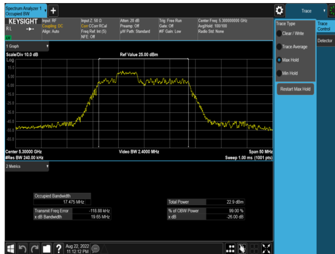
Plot 7-14. 26dB BW & 99% OBW Antenna 3c (20MHz BW 11ax Index 38 – RU52 – Ch.60)
