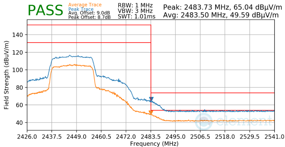
Plot 7-630. Radiated Restricted Upper Band Edge Measurement Antenna 1a
