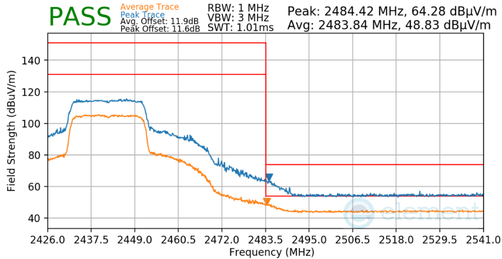
Plot 7-628. Radiated Restricted Upper Band Edge Measurement Antenna 1a
