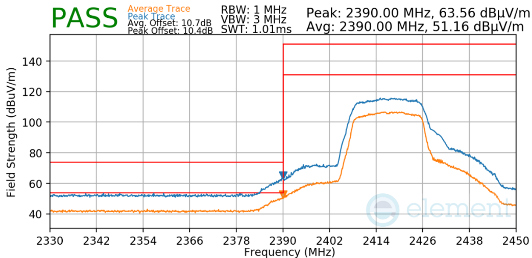
Plot 7-647. Radiated Restricted Lower Band Edge Measurement CDD
