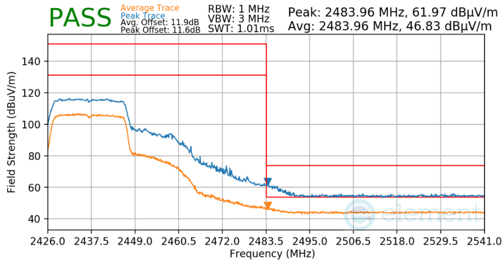
Plot 7-625. Radiated Restricted Upper Band Edge Measurement Antenna 1a
