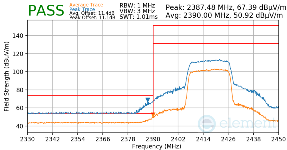
Plot 7-610. Radiated Restricted Lower Band Edge Measurement Antenna 1a
