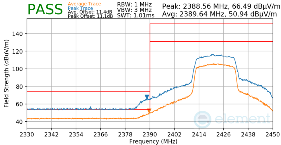
Plot 7-612. Radiated Restricted Lower Band Edge Measurement Antenna 1a
