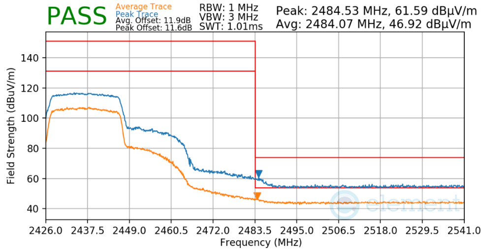
Plot 7-624. Radiated Restricted Upper Band Edge Measurement Antenna 1a
