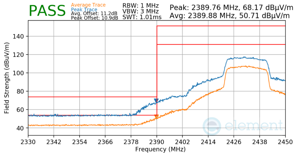
Plot 7-618. Radiated Restricted Lower Band Edge Measurement Antenna 1a
