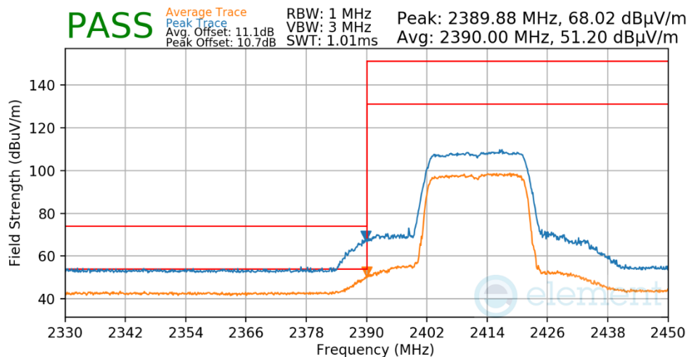
Plot 7-607. Radiated Restricted Lower Band Edge Measurement Antenna 1a
