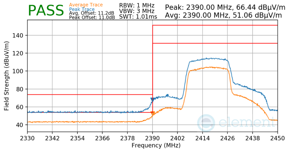
Plot 7-608. Radiated Restricted Lower Band Edge Measurement Antenna 1a
