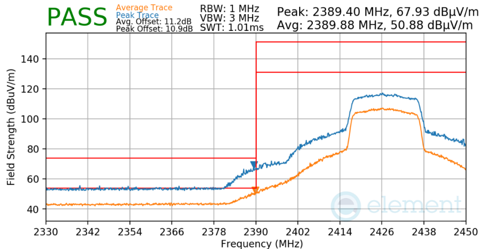
Plot 7-615. Radiated Restricted Lower Band Edge Measurement Antenna 1a
