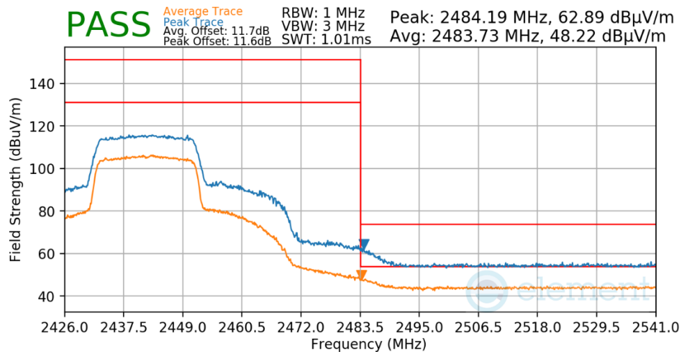
Plot 7-626. Radiated Restricted Upper Band Edge Measurement Antenna 1a
