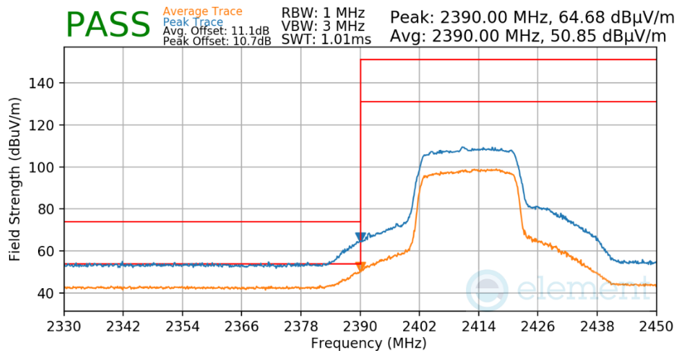
Plot 7-606. Radiated Restricted Lower Band Edge Measurement Antenna 1a
