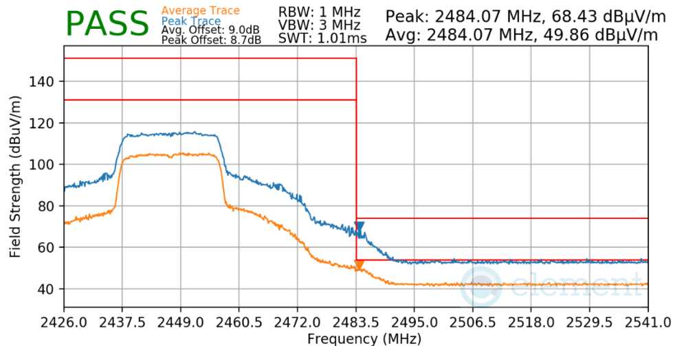
Plot 7-631. Radiated Restricted Upper Band Edge Measurement Antenna 1a
