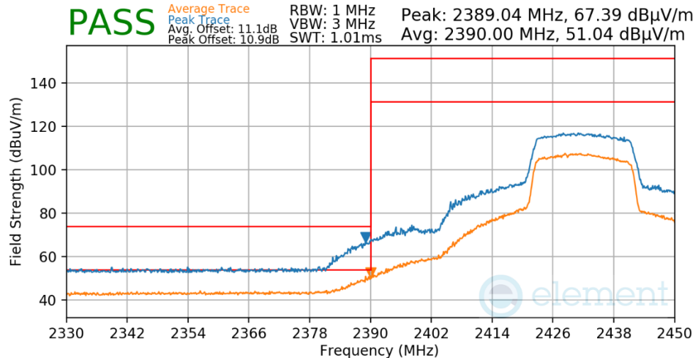
Plot 7-617. Radiated Restricted Lower Band Edge Measurement Antenna 1a
