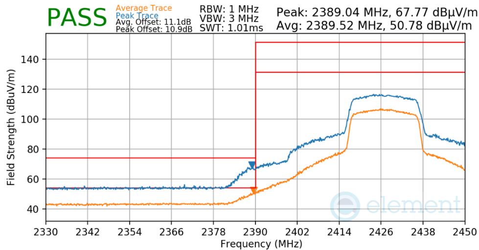
Plot 7-614. Radiated Restricted Lower Band Edge Measurement Antenna 1a
