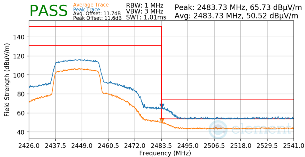
Plot 7-629. Radiated Restricted Upper Band Edge Measurement Antenna 1a
