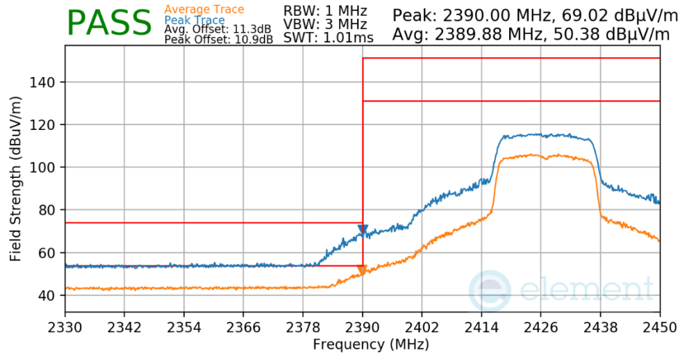
Plot 7-616. Radiated Restricted Lower Band Edge Measurement Antenna 1a
