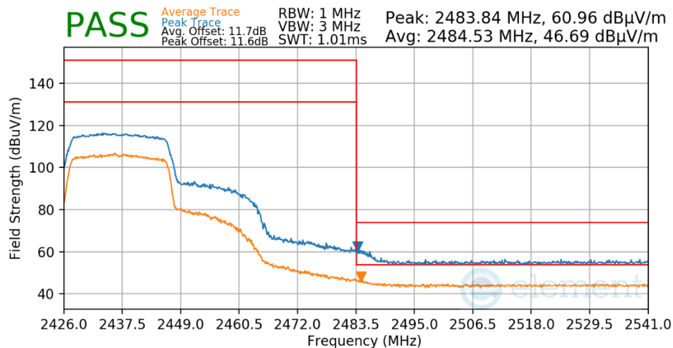
Plot 7-623. Radiated Restricted Upper Band Edge Measurement Antenna 1a
