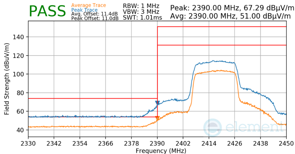
Plot 7-609. Radiated Restricted Lower Band Edge Measurement Antenna 1a
