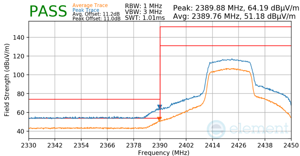
Plot 7-611. Radiated Restricted Lower Band Edge Measurement Antenna 1a
