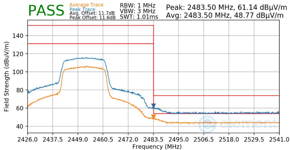
Plot 7-632. Radiated Restricted Upper Band Edge Measurement Antenna 1a
