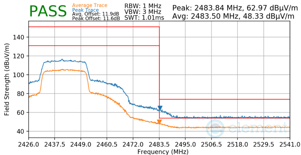
Plot 7-627. Radiated Restricted Upper Band Edge Measurement Antenna 1a
