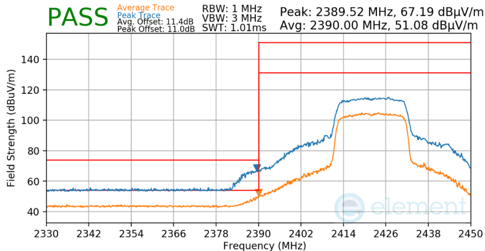
Plot 7-613. Radiated Restricted Lower Band Edge Measurement Antenna 1a
