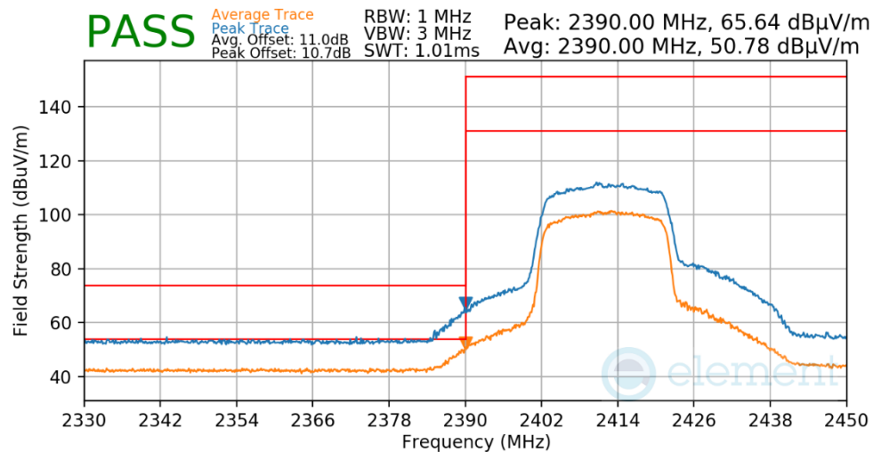
Plot 7-518. Radiated Restricted Lower Band Edge Measurement Antenna 3a
