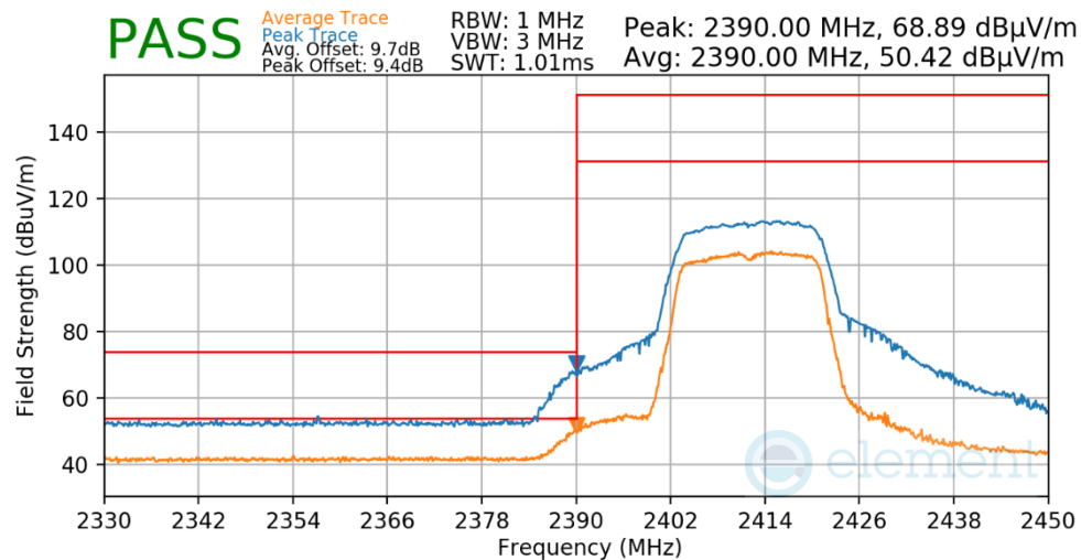
Plot 7-478. Radiated Restricted Lower Band Edge Measurement Antenna 3a
