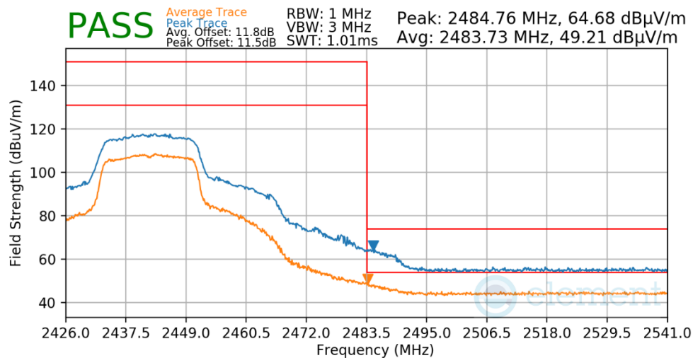
Plot 7-497. Radiated Restricted Upper Band Edge Measurement Antenna 3a
