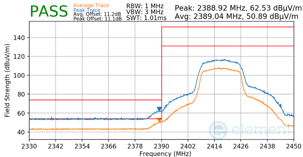
Plot 7-479. Radiated Restricted Lower Band Edge Measurement Antenna 3a
