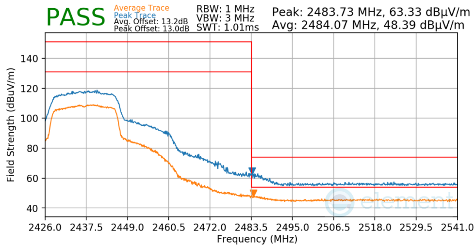
Plot 7-494. Radiated Restricted Upper Band Edge Measurement Antenna 3a
