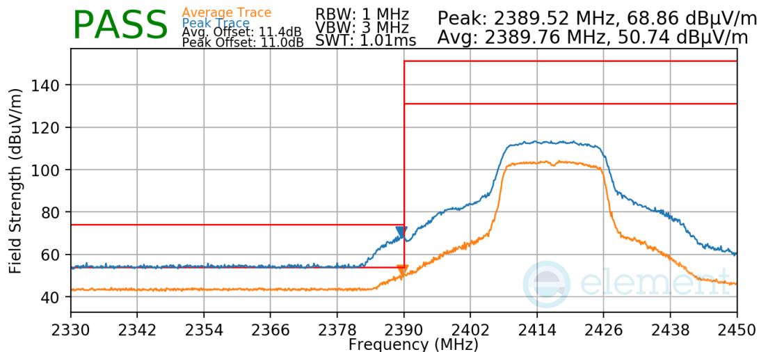
Plot 7-481. Radiated Restricted Lower Band Edge Measurement Antenna 3a
