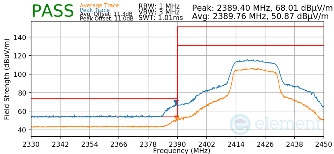
Plot 7-483. Radiated Restricted Lower Band Edge Measurement Antenna 3a
