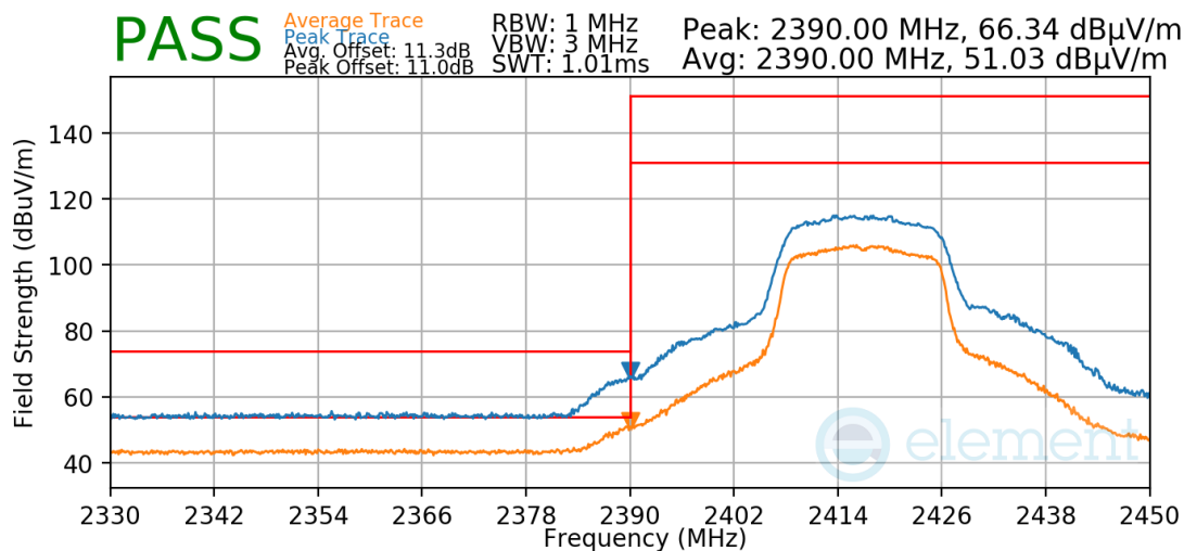
Plot 7-480. Radiated Restricted Lower Band Edge Measurement Antenna 3a
