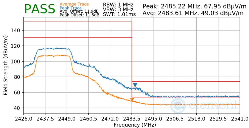
Plot 7-498. Radiated Restricted Upper Band Edge Measurement Antenna 3a
