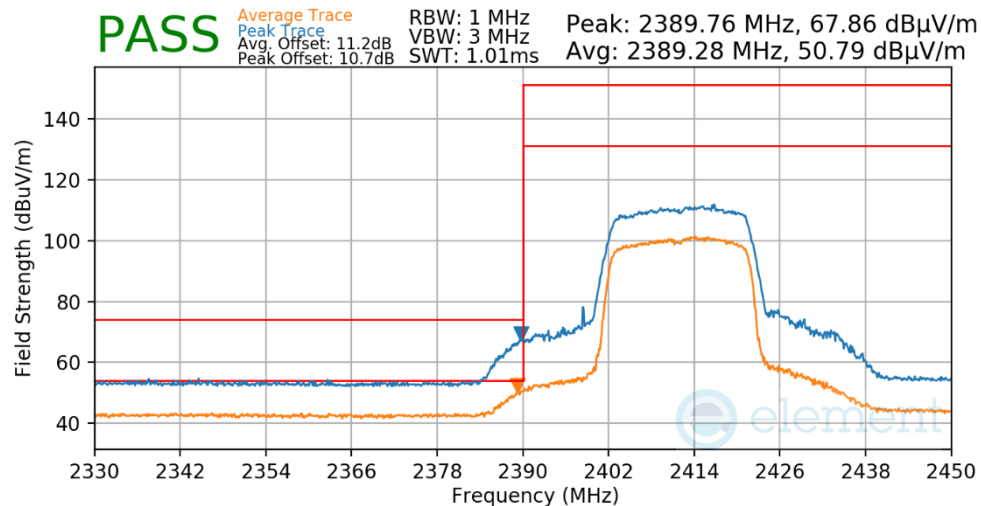
Plot 7-519. Radiated Restricted Lower Band Edge Measurement Antenna 3a
