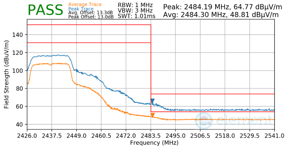
Plot 7-495. Radiated Restricted Upper Band Edge Measurement Antenna 3a
