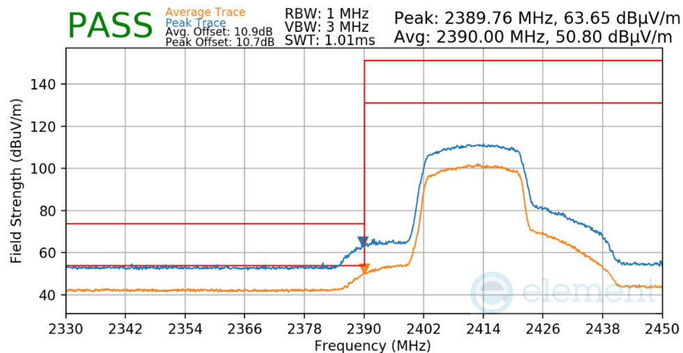
Plot 7-517. Radiated Restricted Lower Band Edge Measurement Antenna 3a
