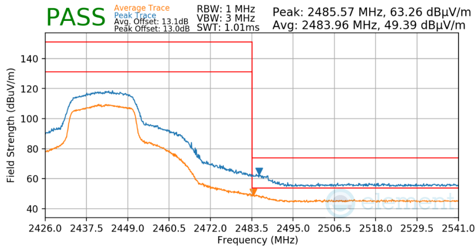
Plot 7-496. Radiated Restricted Upper Band Edge Measurement Antenna 3a
