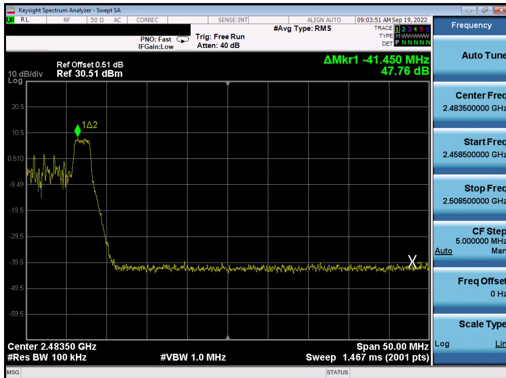
Plot 7-91. Band Edge Antenna 1a (802.11ax OFDMA – RU26 Index 8 – Ch. 10)
