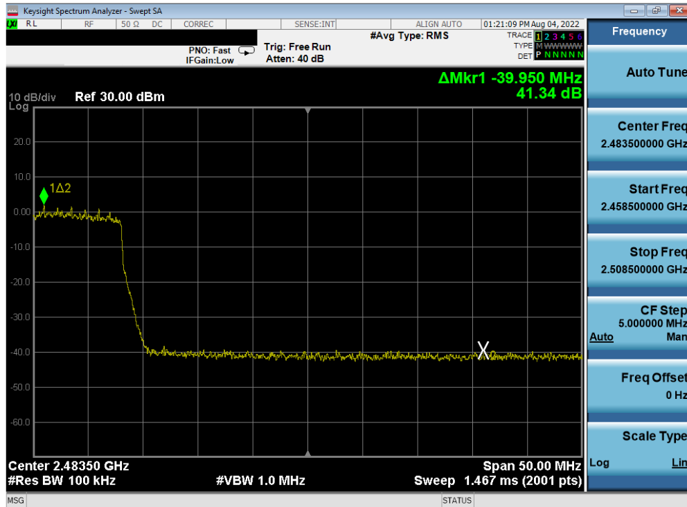
Plot 7-87. Band Edge Antenna 3a (802.11ax OFDMA – RU242 – Ch. 10)
