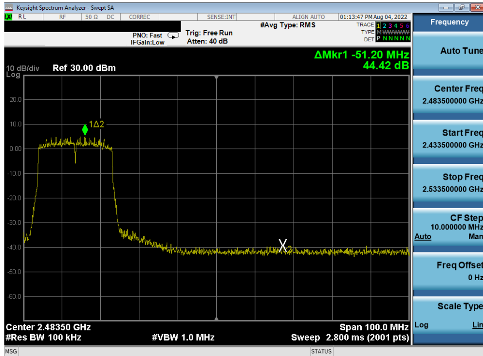
Plot 7-85. Band Edge Antenna 3a (802.11ax OFDMA – RU242 – Ch. 8)
