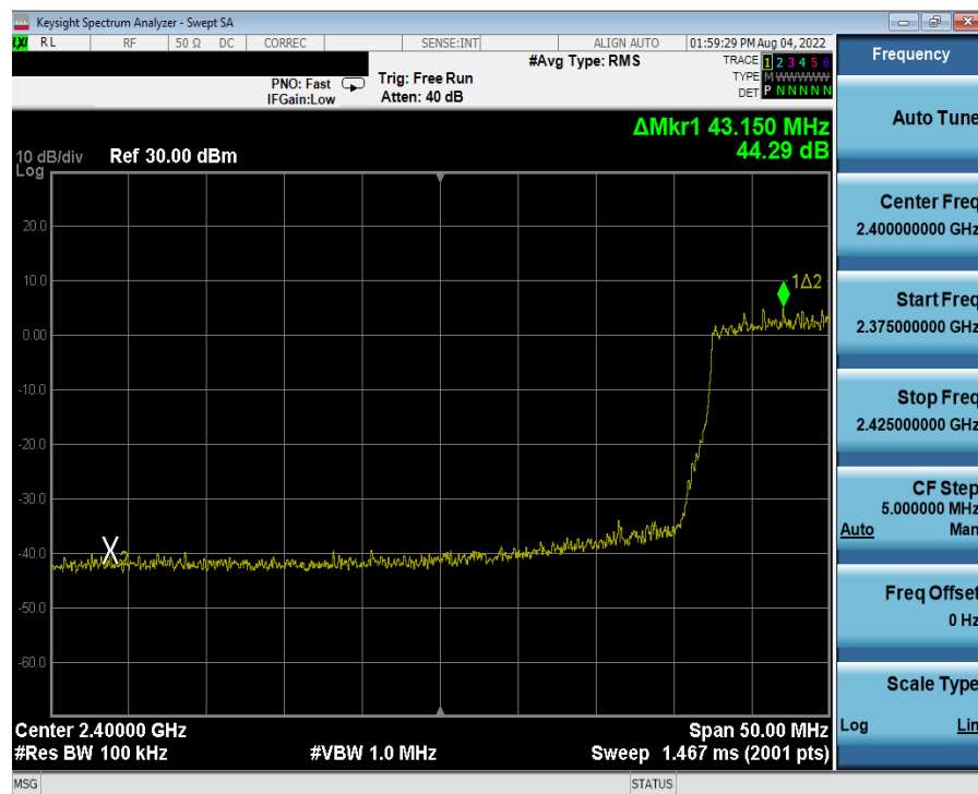
Plot 7-97. Band Edge Antenna 1a (802.11ax OFDMA – RU242 – Ch. 4)
