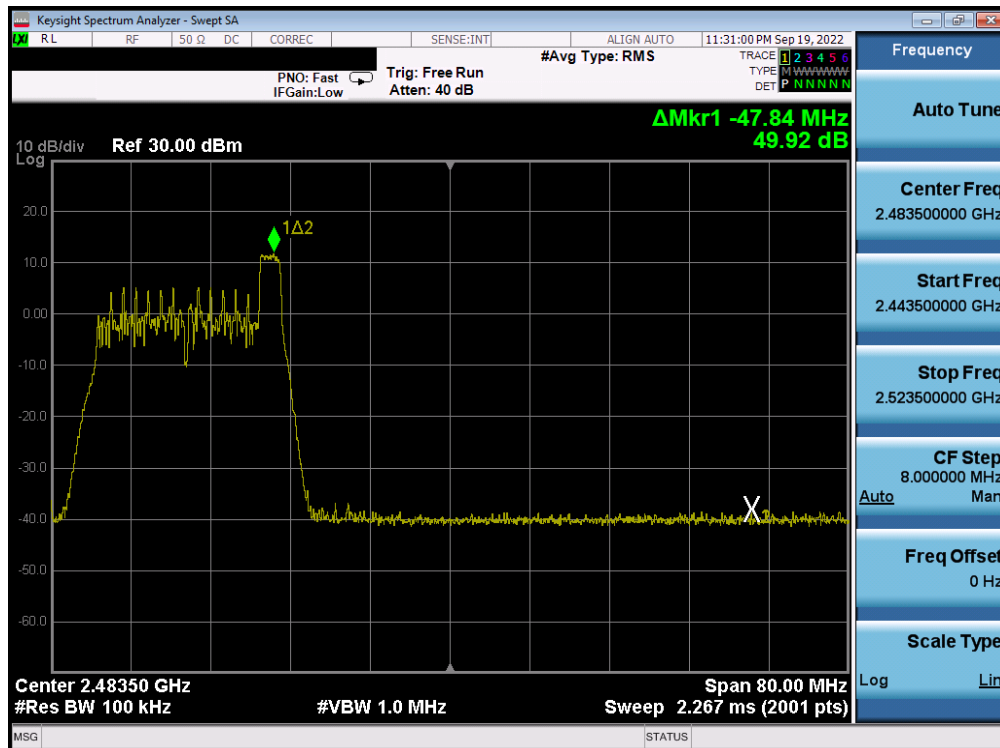
Plot 7-74. Band Edge Antenna 3a (802.11ax OFDMA – RU26 Index 8 – Ch. 10)
