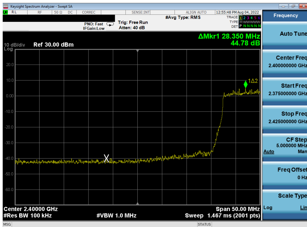
Plot 7-80. Band Edge Antenna 3a (802.11ax OFDMA – RU242 – Ch. 4)
