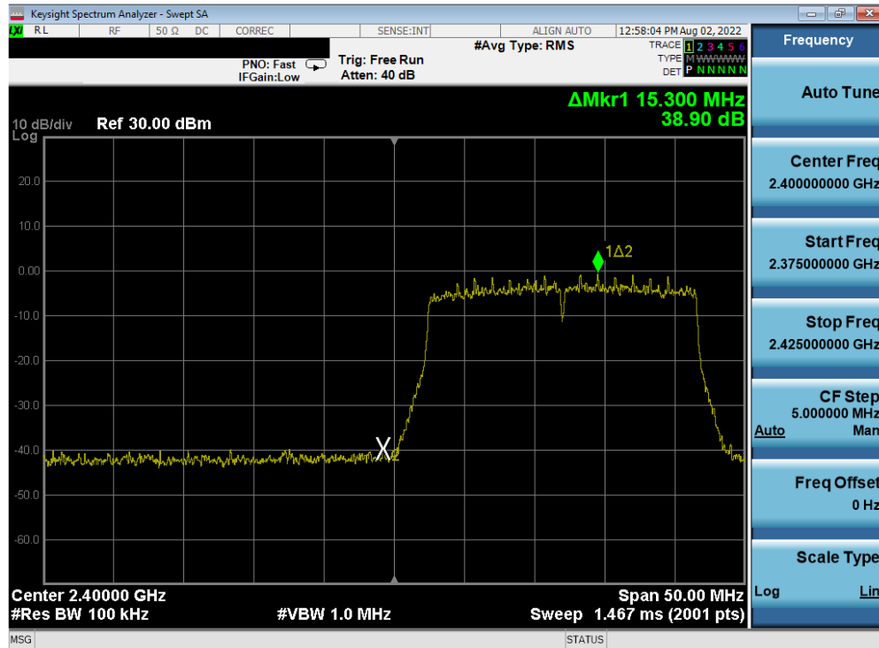
Plot 7-94. Band Edge Antenna 1a (802.11ax OFDMA – RU242 – Ch. 1)
