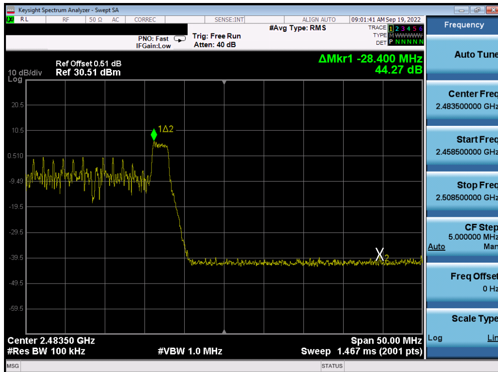
Plot 7-93. Band Edge Antenna 1a (802.11ax OFDMA – RU26 Index 8 – Ch. 12)
