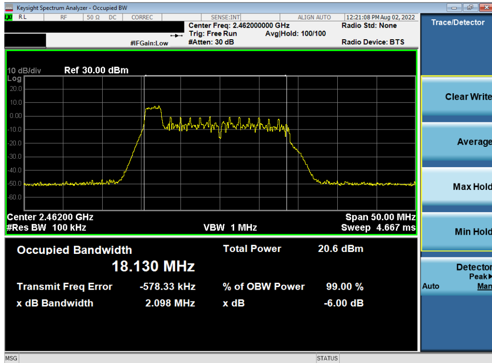
Plot 7-19. 6dB BW & 99% OBW Plot Antenna 1a (802.11ax OFDMA – RU26 Index 0 – Ch. 11)
