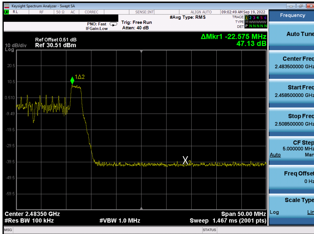
Plot 7-92. Band Edge Antenna 1a (802.11ax OFDMA – RU26 Index 8 – Ch. 11)
