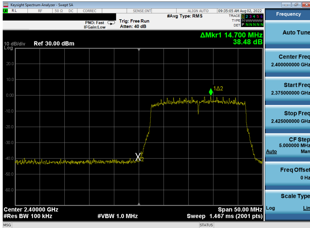
Plot 7-77. Band Edge Antenna 3a (802.11ax OFDMA – RU242 – Ch. 1)
