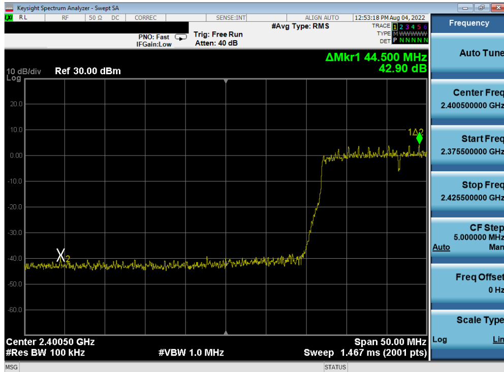
Plot 7-79. Band Edge Antenna 3a (802.11ax OFDMA – RU242 – Ch. 3)
