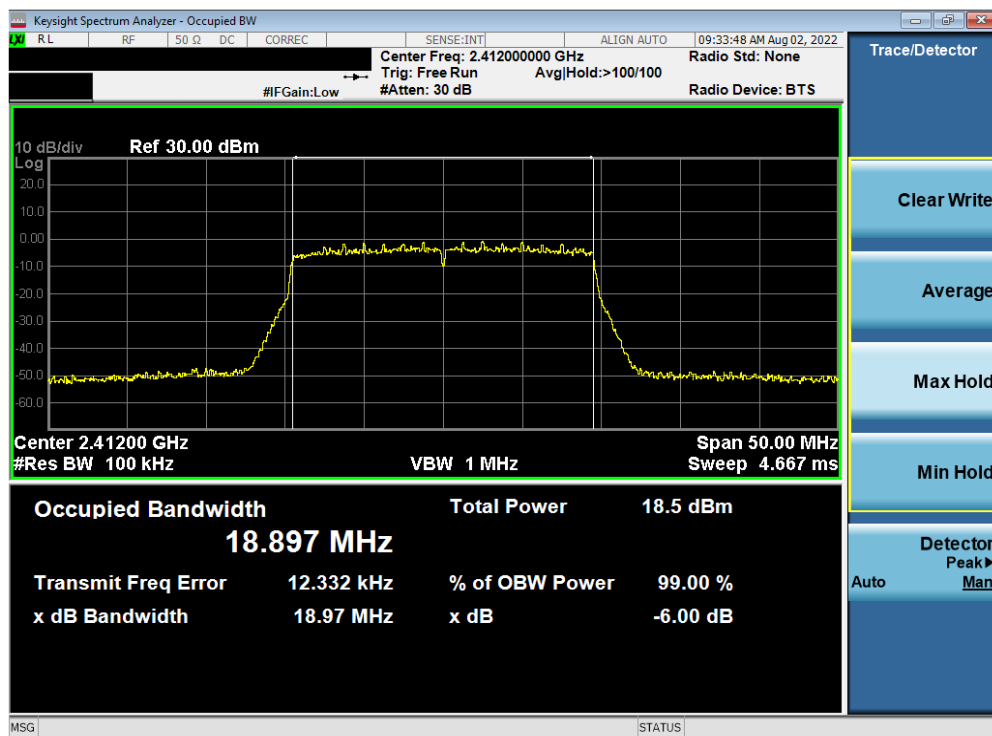
Plot 7-10. 6dB BW & 99% OBW Plot Antenna 3a (802.11ax OFDMA – RU242 – Ch. 1)
