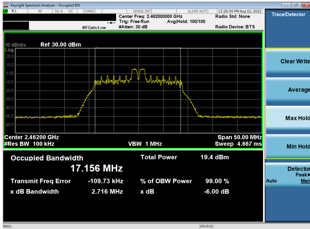
Plot 7-20. 6dB BW & 99% OBW Plot Antenna 1a (802.11ax OFDMA – RU26 Index 4 – Ch. 11)
