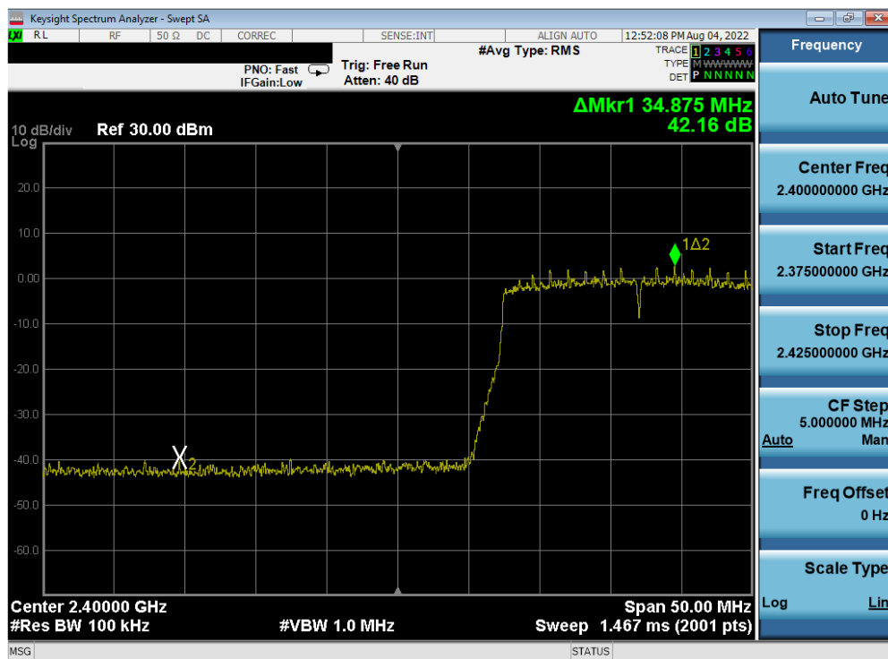
Plot 7-78. Band Edge Antenna 3a (802.11ax OFDMA – RU242 – Ch. 2)
