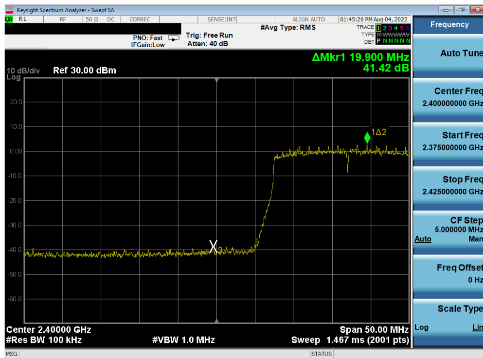
Plot 7-95. Band Edge Antenna 1a (802.11ax OFDMA – RU242 – Ch. 2)
