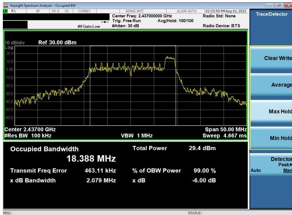
Plot 7-18. 6dB BW & 99% OBW Plot Antenna 1a (802.11ax OFDMA – RU26 Index 8 – Ch. 6)
