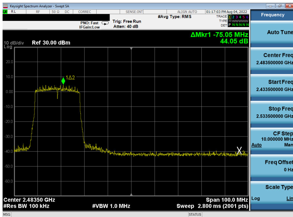
Plot 7-86. Band Edge Antenna 3a (802.11ax OFDMA – RU242 – Ch. 9)
