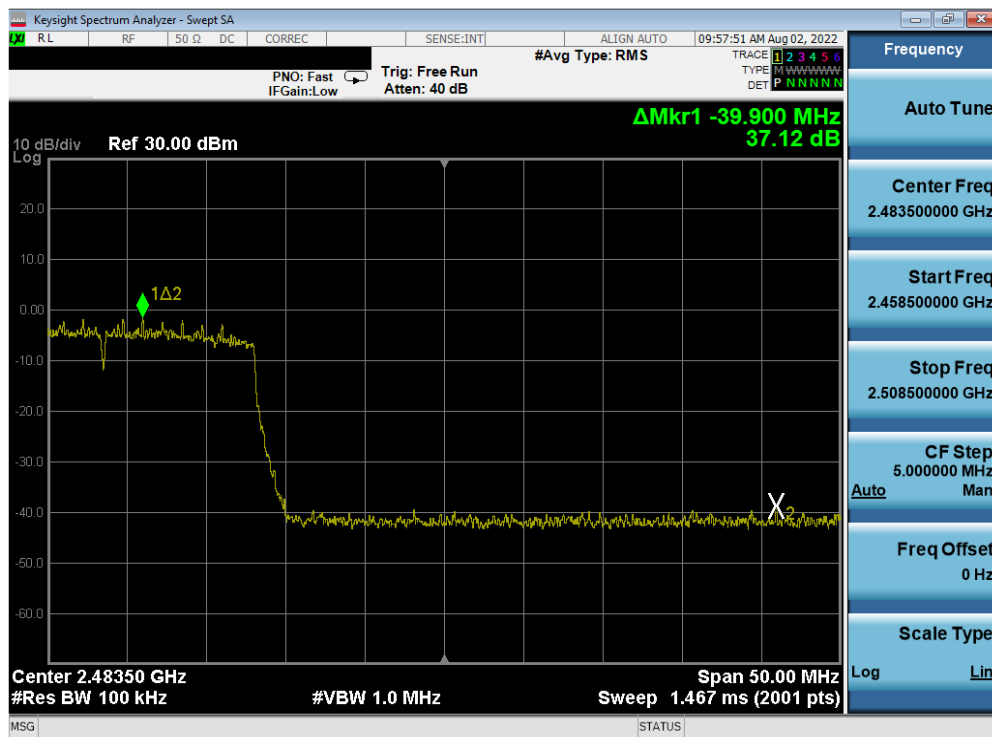
Plot 7-88. Band Edge Antenna 3a (802.11ax OFDMA – RU242 – Ch. 11)
