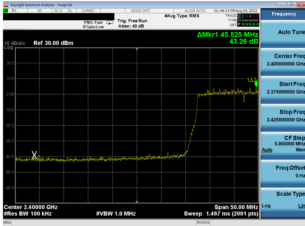
Plot 7-96. Band Edge Antenna 1a (802.11ax OFDMA – RU242 – Ch. 3)
