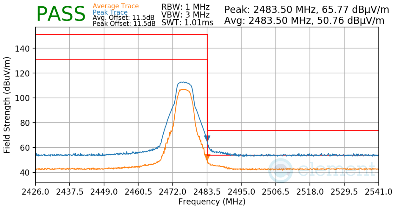
Plot 7-95. Radiated Restricted Upper Band Edge Measurement Antenna 3a
