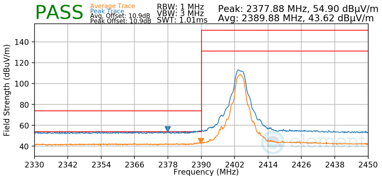
Plot 7-100. Radiated Restricted Lower Band Edge Measurement TxBF
