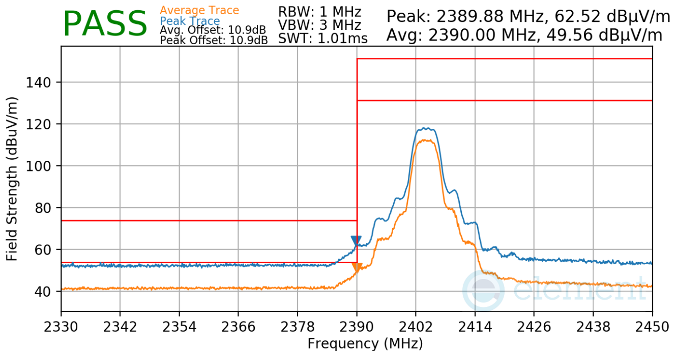
Plot 7-97. Radiated Restricted Lower Band Edge Measurement Antenna 1a
