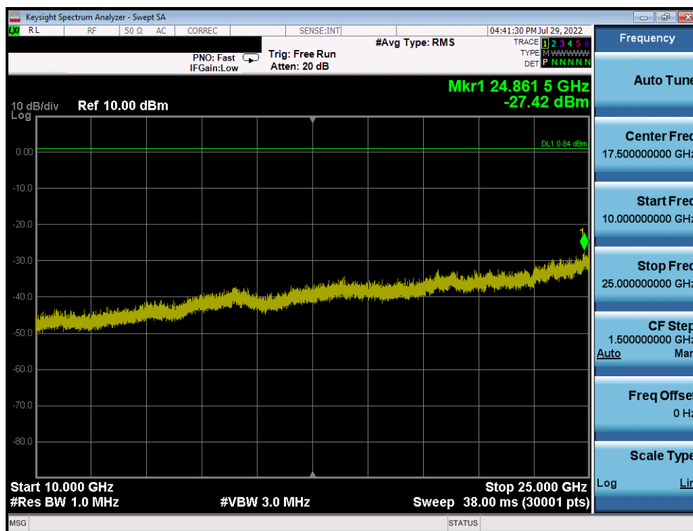
Plot 7-76. Conducted Spurious Plot Antenna 1a (Bluetooth (HDR4), 4 Mbps, ePA – Ch. 1)
