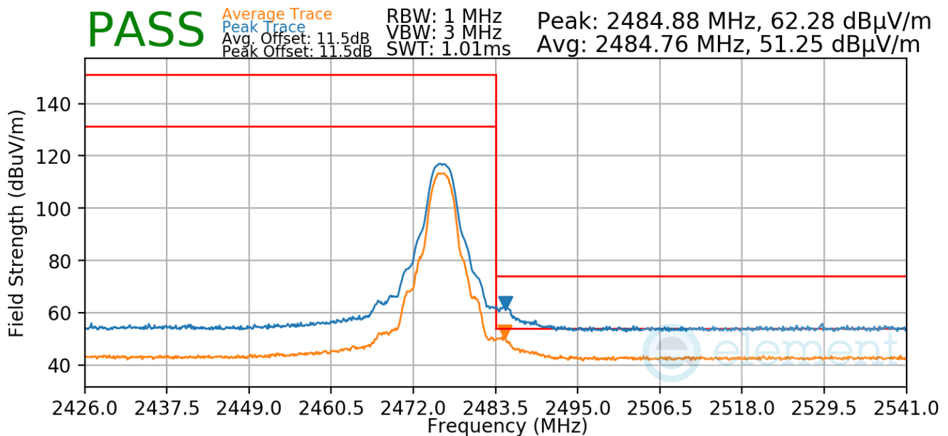
Plot 7-102. Radiated Restricted Upper Band Edge Measurement TxBF
