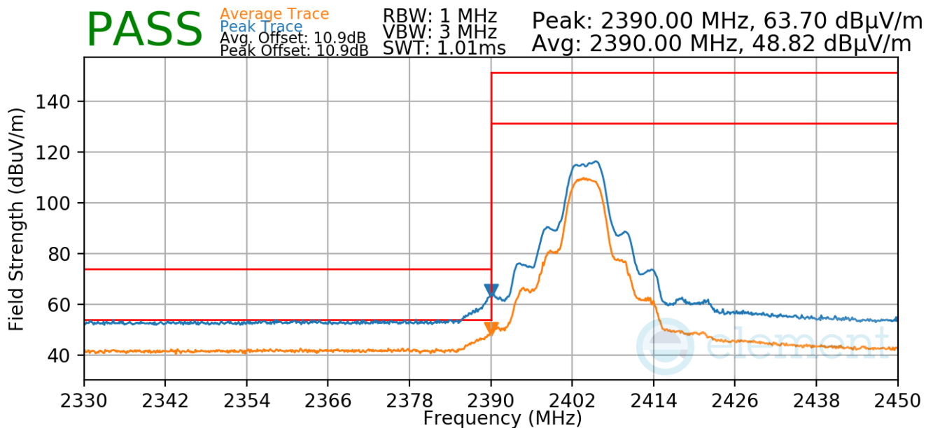
Plot 7-101. Radiated Restricted Lower Band Edge Measurement TxBF
