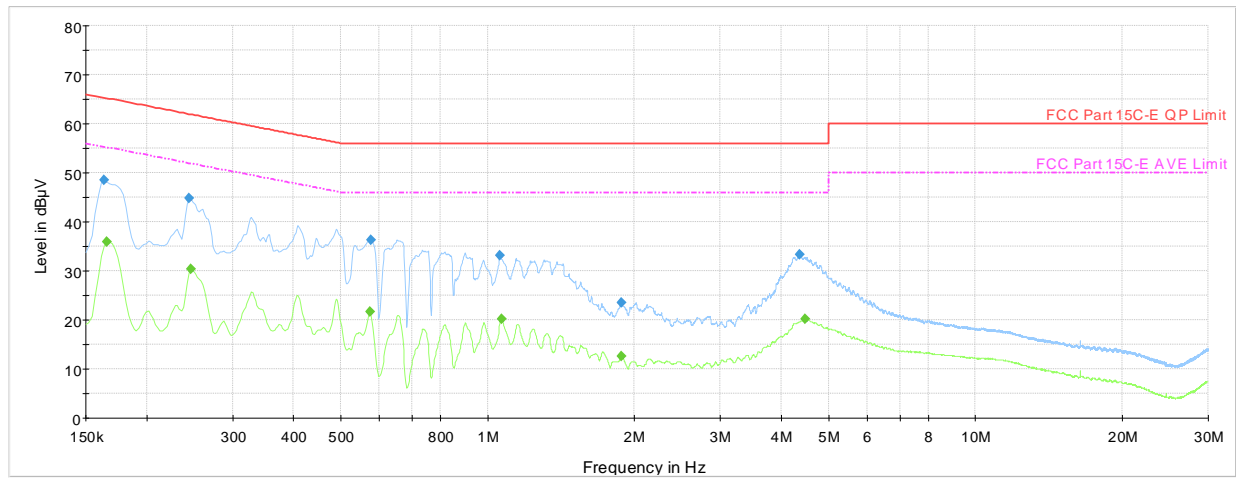
Plot 7-106. AC Line Conducted Plot with Bluetooth HDR (N, 4Mbps ePA - Ch.38 with AC/DC Adapter)
