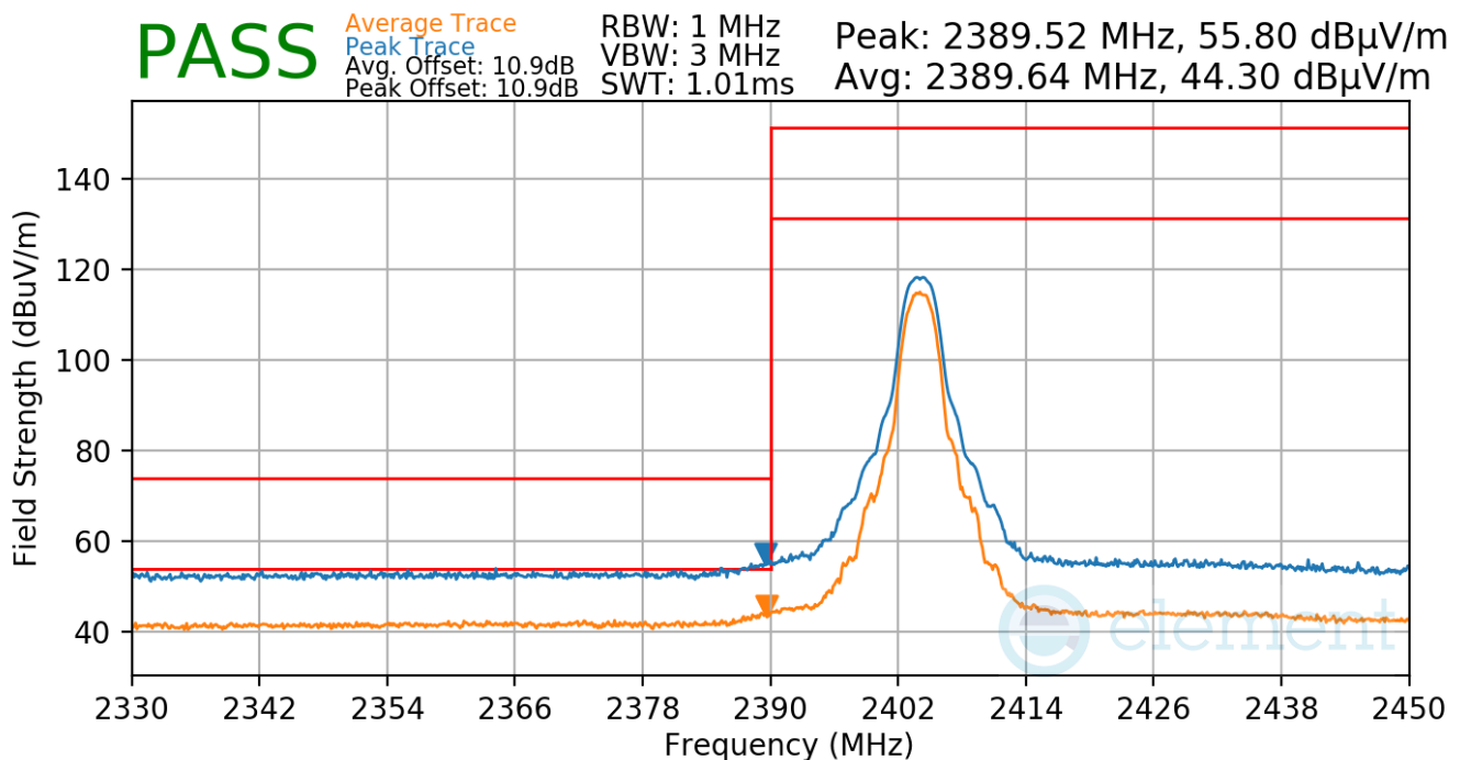
Plot 7-96. Radiated Restricted Lower Band Edge Measurement Antenna 1a
