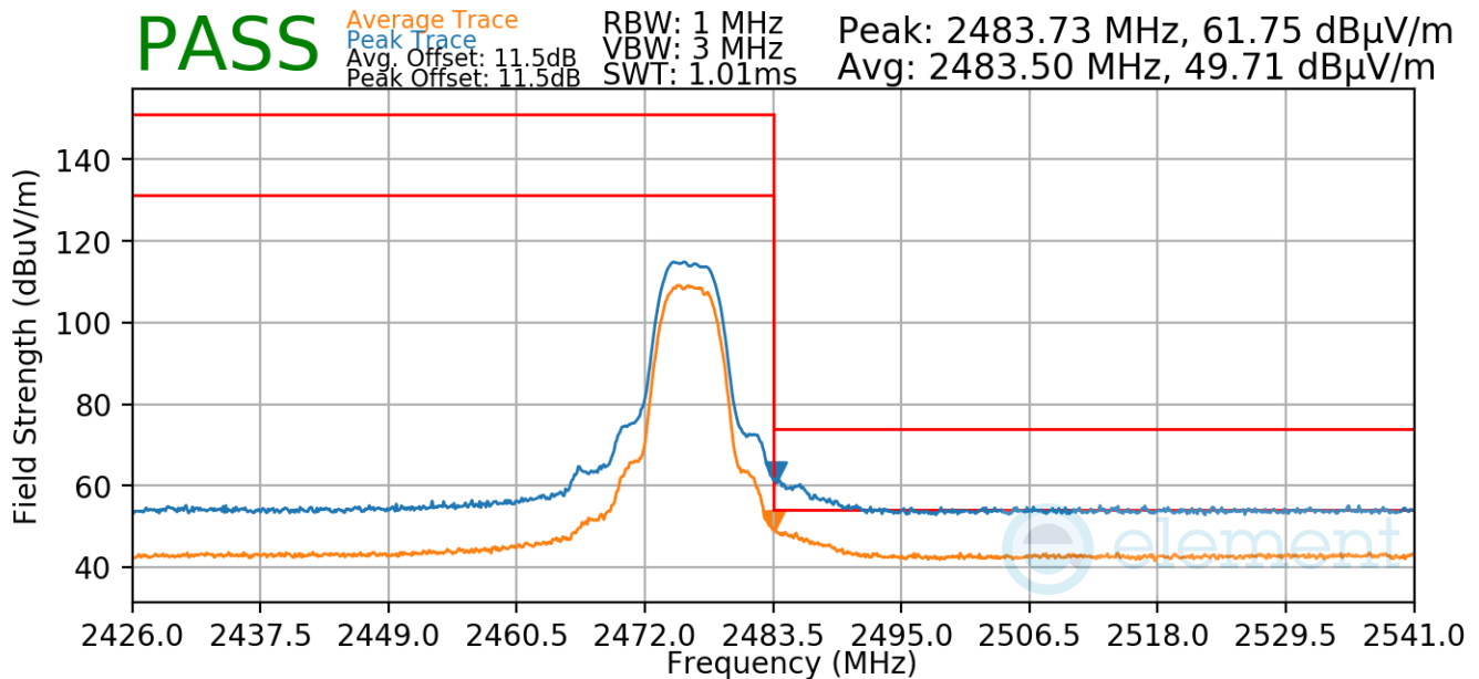
Plot 7-103. Radiated Restricted Upper Band Edge Measurement TxBF
