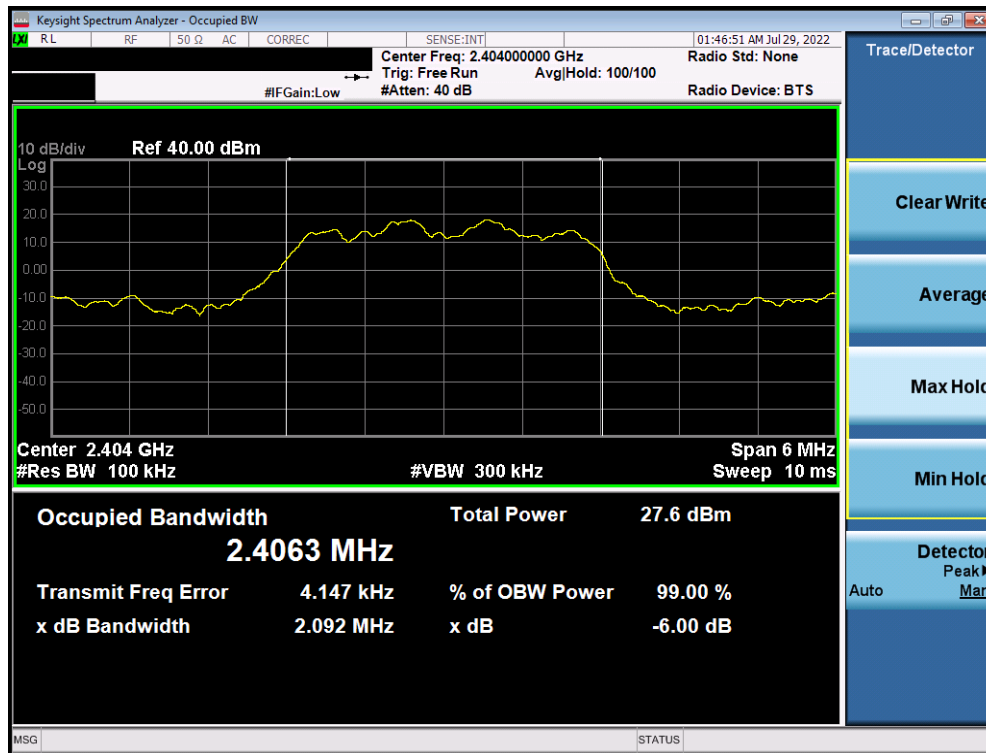
Plot 7-1. 6dB BW & 99% OBW Plot Antenna 3a (Bluetooth (HDR4), 4Mbps, ePA – Ch. 1)
