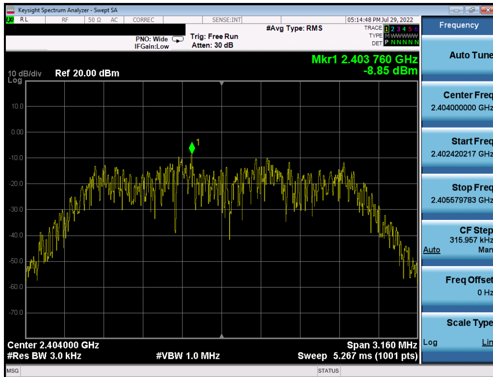
Plot 7-44. Power Spectral Density Plot Tx BF Antenna 1a (Bluetooth (HDR4), 4Mbps, iPA – Ch. 1)
