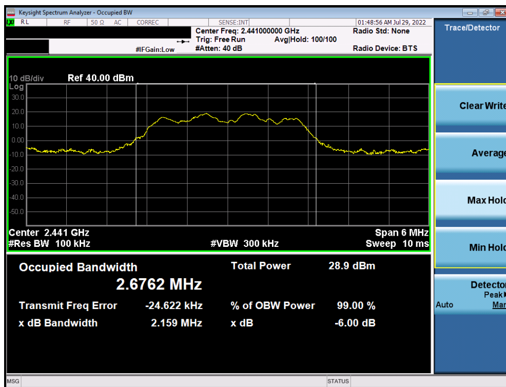
Plot 7-2. 6dB BW & 99% OBW Plot Antenna 3a (Bluetooth (HDR4), 4Mbps, ePA – Ch. 38)
