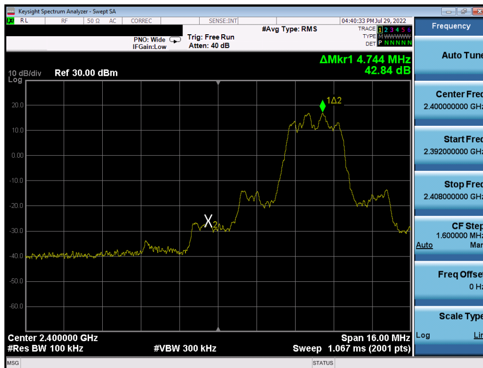
Plot 7-65. Band Edge Plot Antenna 1a (Bluetooth (HDR4), ePA – Ch. 1)
