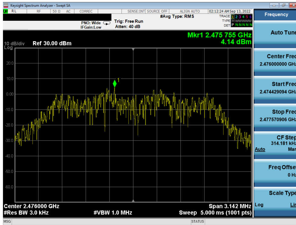
Plot 7-53. Power Spectral Density Plot TxBF Antenna 3a (Bluetooth (HDR8), 8Mbps, ePA – Ch. 73)
