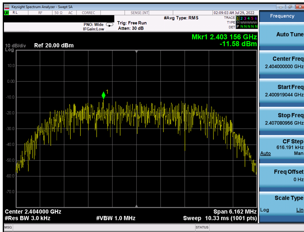
Plot 7-55. Power Spectral Density Plot Tx BF Antenna 3a (Bluetooth (HDR8), 8Mbps, iPA – Ch. 1)
