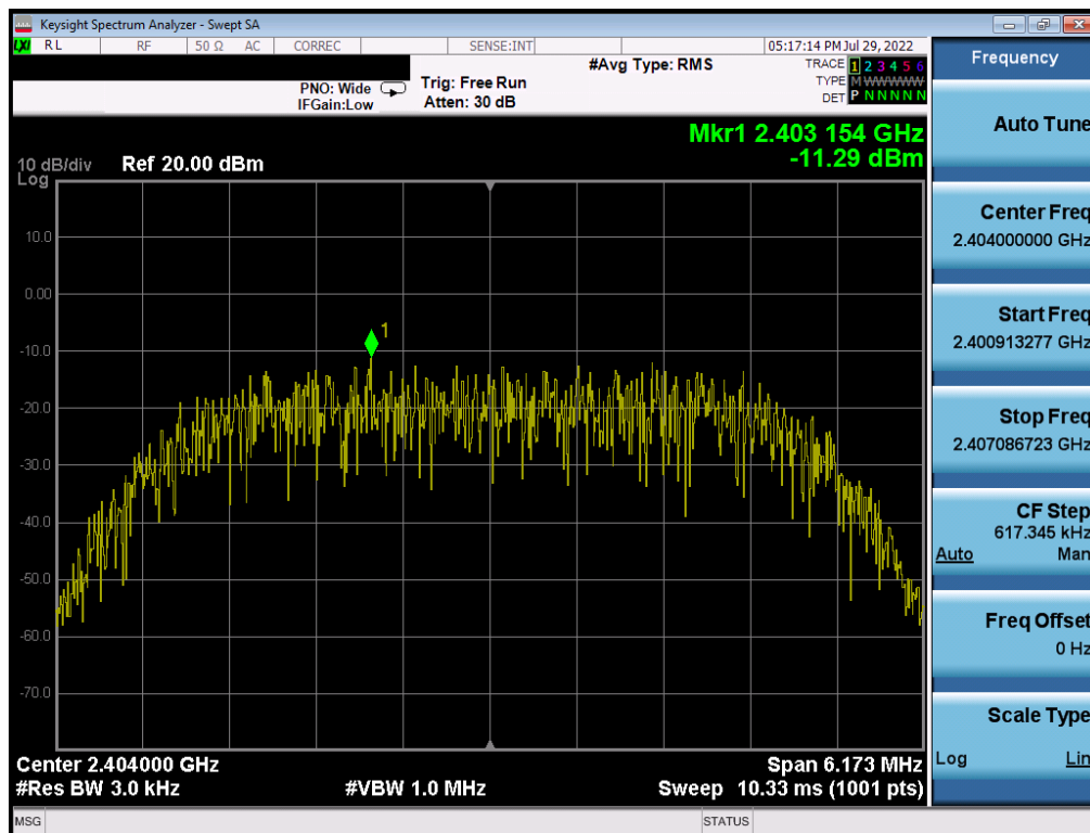
Plot 7-56. Power Spectral Density Plot Tx BF Antenna 1a (Bluetooth (HDR8), 8Mbps, iPA – Ch. 1)
