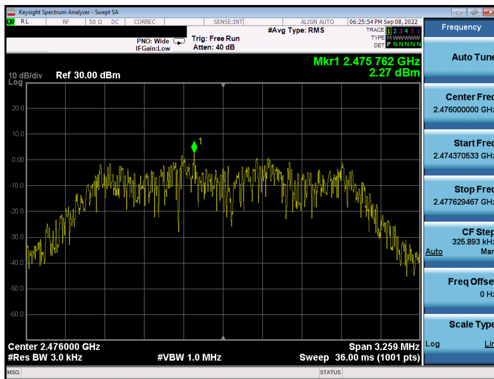
Plot 7-15. Power Spectral Density Plot Antenna 3a (Bluetooth (HDR4), 4Mbps, ePA – Ch. 73)
