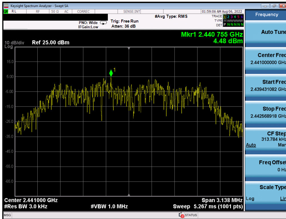
Plot 7-39. Power Spectral Density Plot TxBF Antenna 3a (Bluetooth (HDR4), 4Mbps, ePA – Ch. 38)
