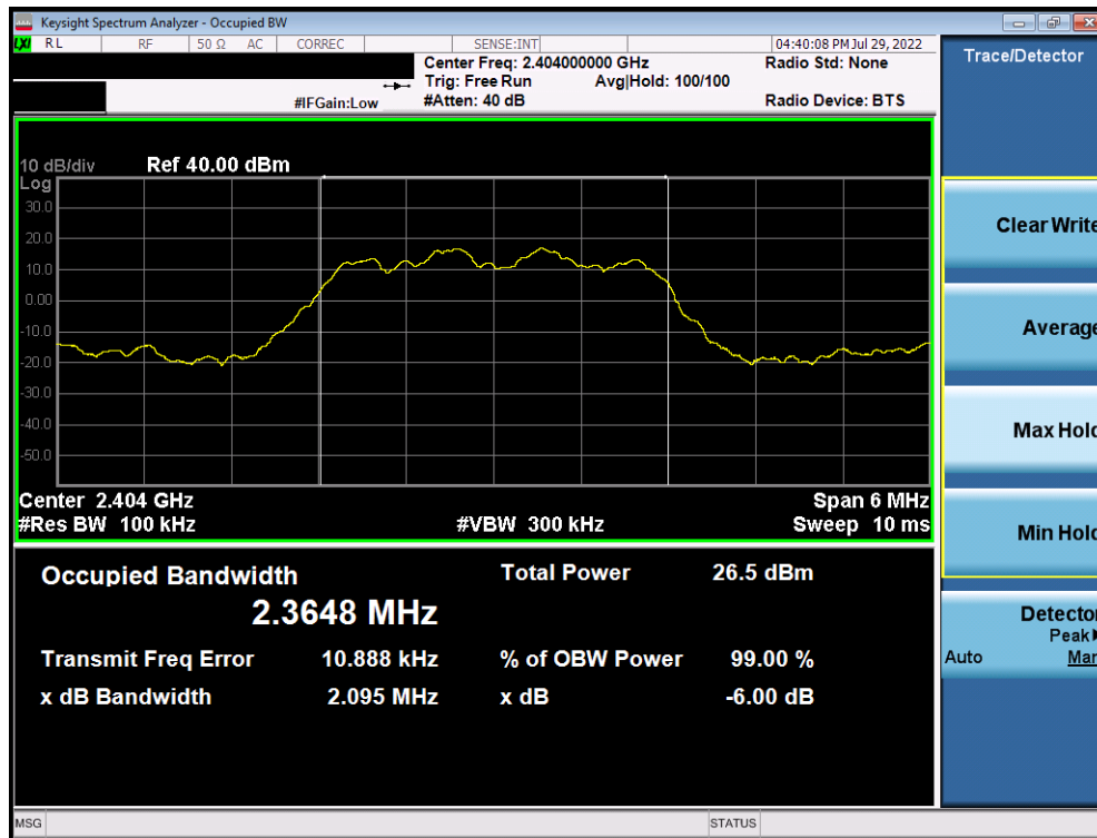
Plot 7-7. 6dB BW & 99% OBW Plot Antenna 1a (Bluetooth (HDR4), 4Mbps, ePA – Ch. 1)
