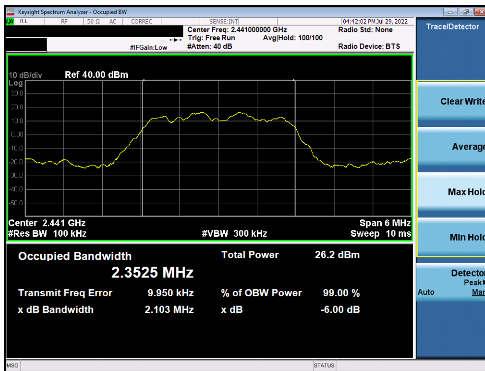
Plot 7-8. 6dB BW & 99% OBW Plot Antenna 1a (Bluetooth (HDR4), 4Mbps, ePA – Ch. 38)
