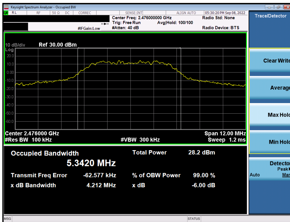
Plot 7-6. 6dB BW & 99% OBW Plot Antenna 3a (Bluetooth (HDR8), 8Mbps, ePA – Ch. 73)
