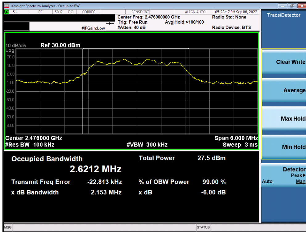
Plot 7-3. 6dB BW & 99% OBW Plot Antenna 3a (Bluetooth (HDR4), 4Mbps, ePA – Ch. 73)
