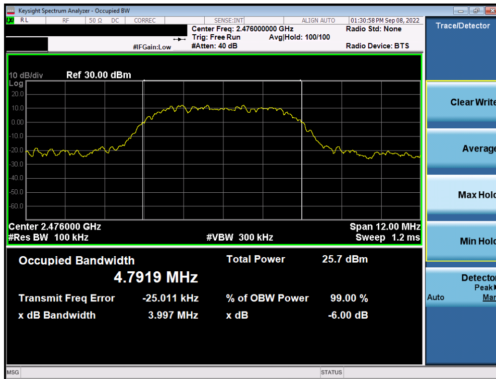
Plot 7-12. 6dB BW & 99% OBW Plot Antenna 1a (Bluetooth (HDR8), 8Mbps, ePA – Ch. 73)
