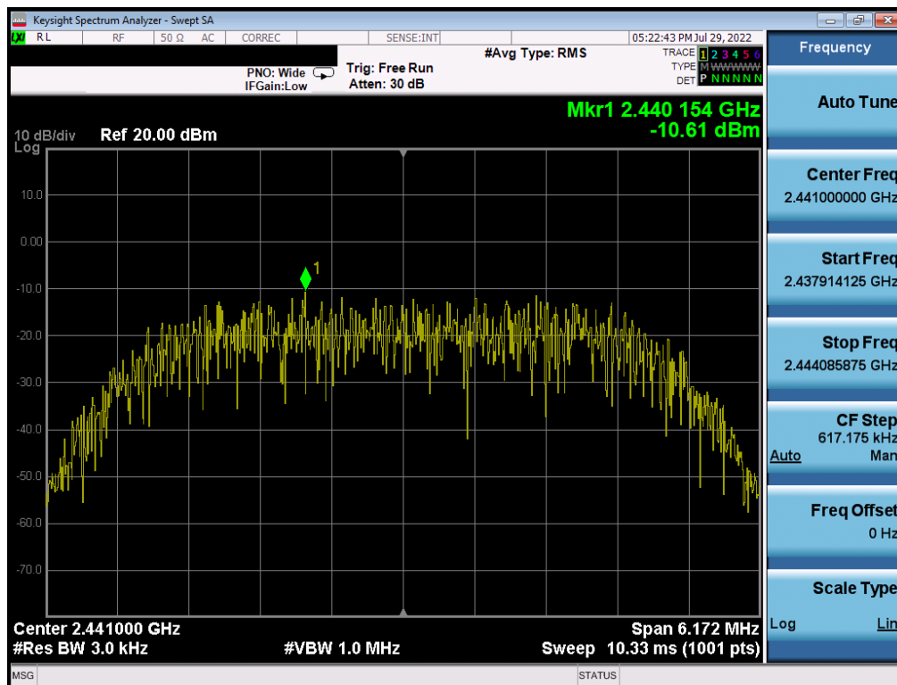
Plot 7-58. Power Spectral Density Plot TxBF Antenna 1a (Bluetooth (HDR8), 8Mbps, iPA – Ch. 38)
