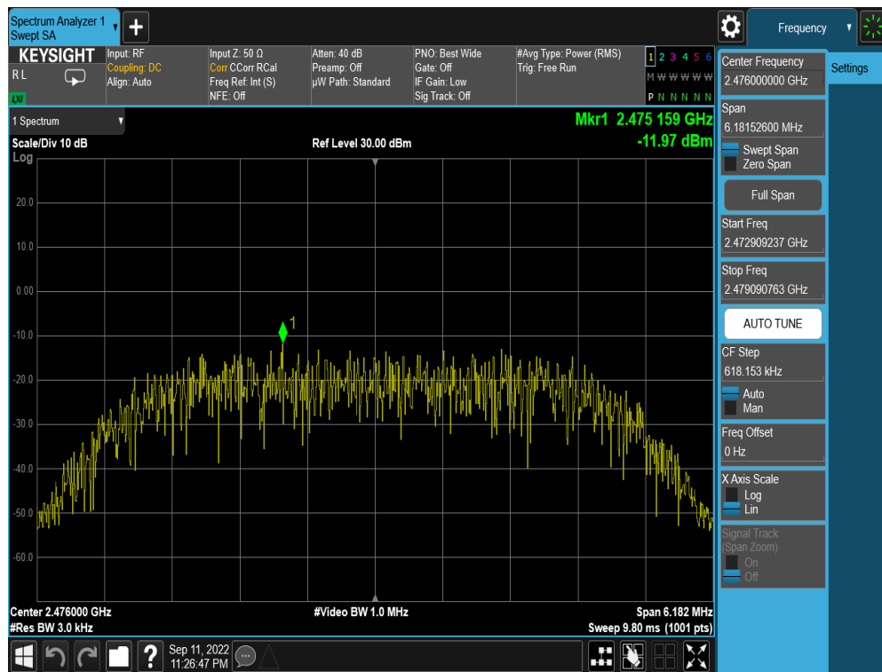
Plot 7-59. Power Spectral Density Plot TxBF Antenna 3a (Bluetooth (HDR8), 8Mbps, iPA – Ch. 73)
