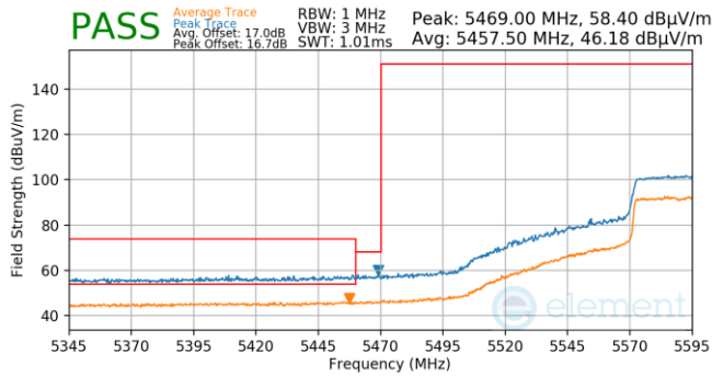
Plot 7-1497. (FCC Only) Antenna 1b (Pk & Avg, Ch.122, 802.11ac, MCS0)
