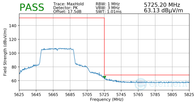
Plot 7-1480. Antenna 1b (Pk, Ch.134, 802.11ax(SU), MCS4)
