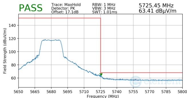
Plot 7-1548. CDD Primary (Pk, Ch.136, 802.11n, MCS13)
