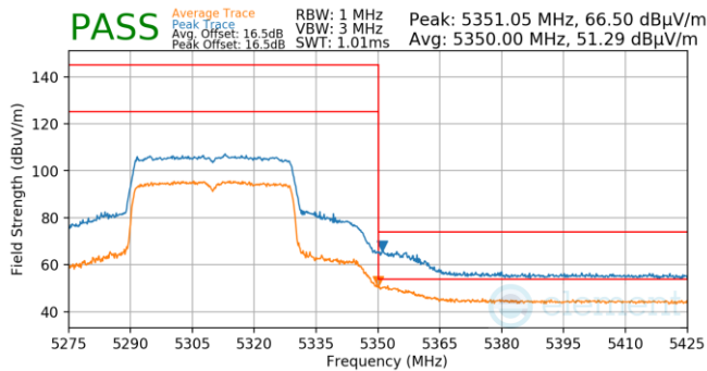
Plot 7-1465. Antenna 1b (Pk & Avg, Ch.62, 802.11ax(SU), MCS4)
