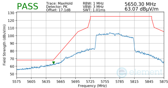
Plot 7-1505. Antenna 1b (Pk, Ch.155, 802.11ac, MCS7)
