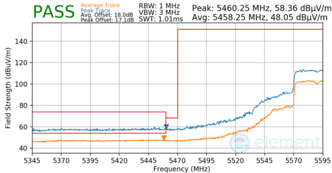
Plot 7-1474. (FCC Only) Antenna 1b (Pk & Avg, Ch.118, 802.11ax(SU), MCS11)
