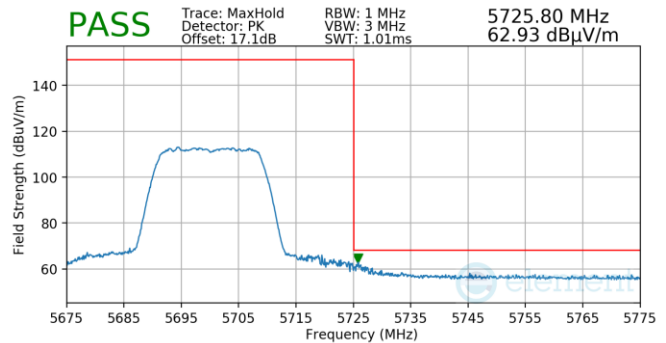
Plot 7-1551. CDD Primary (Pk, Ch.140, 802.11n, MCS13)
