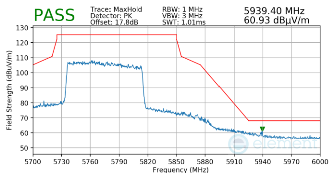
Plot 7-1527. Antenna 1b (Pk, Ch.155, 802.11ax(SU), MCS0)
