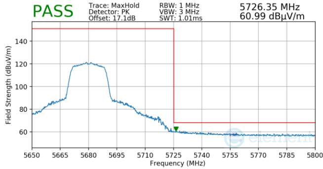
Plot 7-1546. CDD Primary (Pk, Ch.136, 802.11n, MCS6)
