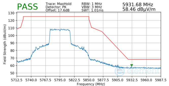
Plot 7-1486. Antenna 1b (Pk, Ch.159, 802.11ax(SU), MCS4)
