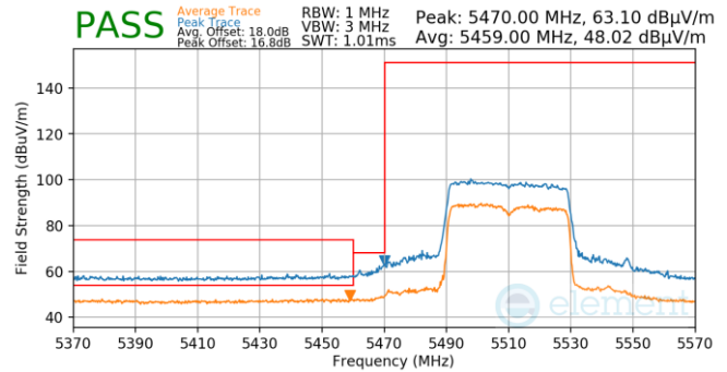
Plot 7-1469. Antenna 1b (Pk & Avg, Ch.102, 802.11ax(SU), MCS11)
