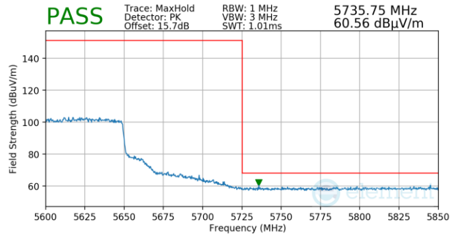
Plot 7-1521. (FCC Only) Antenna 1b (Pk, Ch.122, 802.11ax(SU), MCS0)
