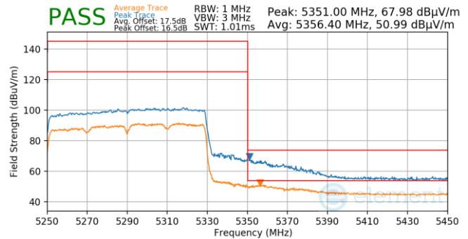
Plot 7-1514. Antenna 1b (Pk & Avg, Ch.58, 802.11ax(SU), MCS11)
