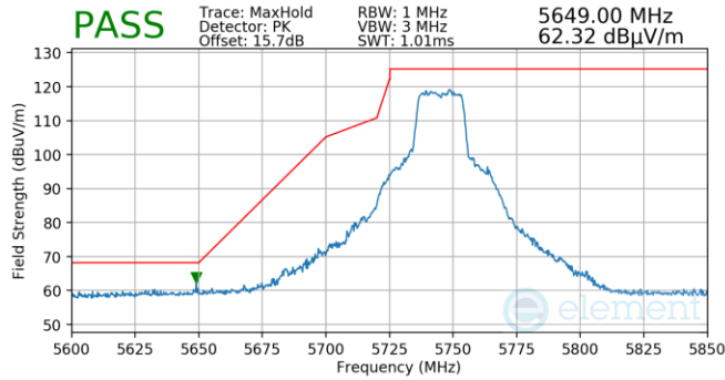
Plot 7-1554. CDD Primary (Pk, Ch.149, 802.11n, MCS13)
