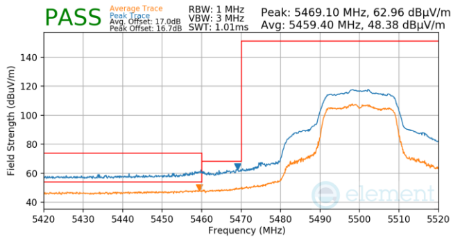
Plot 7-1540. CDD Primary (Pk & Avg, Ch.100, 802.11n, MCS11)
