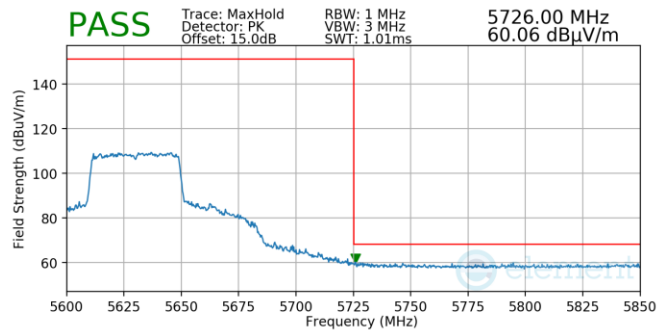
Plot 7-1477. (FCC Only) Antenna 1b (Pk, Ch.126, 802.11ax(SU), MCS4)
