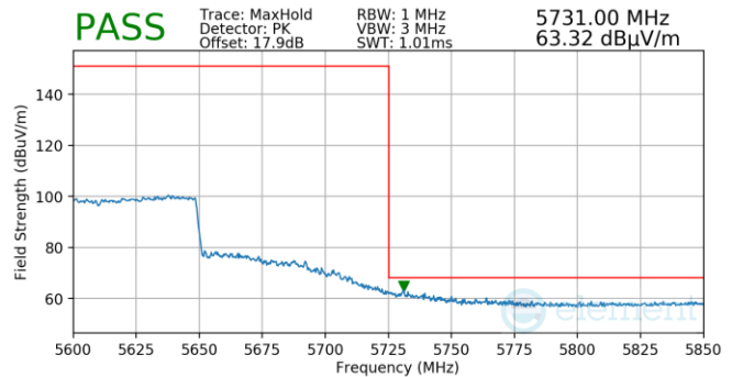
Plot 7-1523. (FCC Only) Antenna 1b (Pk, Ch.122, 802.11ax(SU), MCS11)
