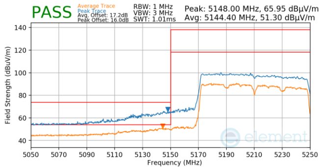
Plot 7-1490. Antenna 1b (Pk & Avg, Ch.42, 802.11ac, MCS7)
