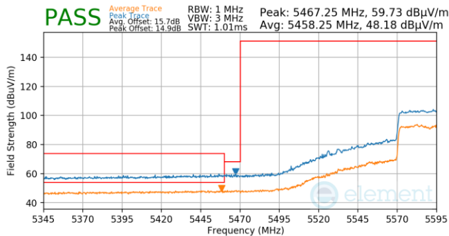
Plot 7-1519. (FCC Only) Antenna 1b (Pk & Avg, Ch.122, 802.11ax(SU), MCS4)
