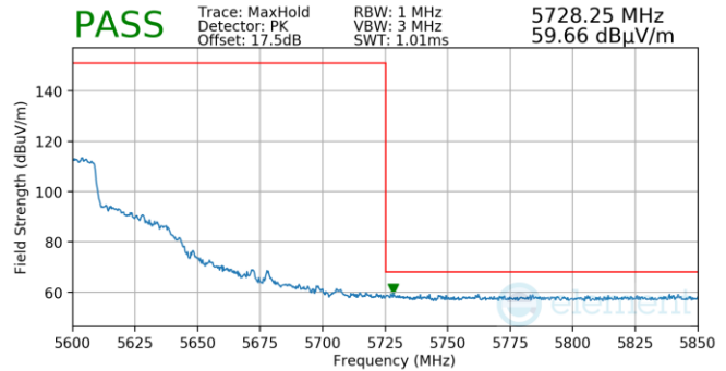
Plot 7-1475. (FCC Only) Antenna 1b (Pk, Ch.118, 802.11ax(SU), MCS11)
