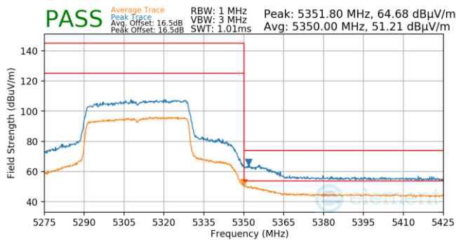
Plot 7-1464. Antenna 1b (Pk & Avg, Ch.62, 802.11ax(SU), MCS0)
