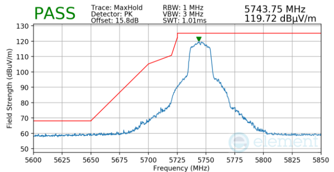
Plot 7-1553. CDD Primary (Pk, Ch.149, 802.11n, MCS11)
