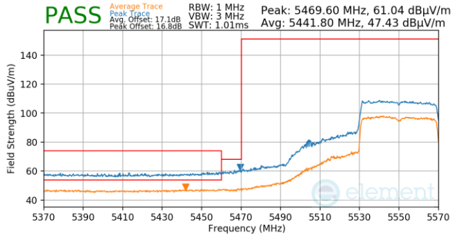
Plot 7-1471. Antenna 1b (Pk & Avg, Ch.110, 802.11ax(SU), MCS4)
