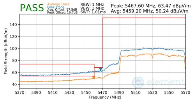
Plot 7-1495. Antenna 1b (Pk & Avg, Ch.106, 802.11ac, MCS4)
