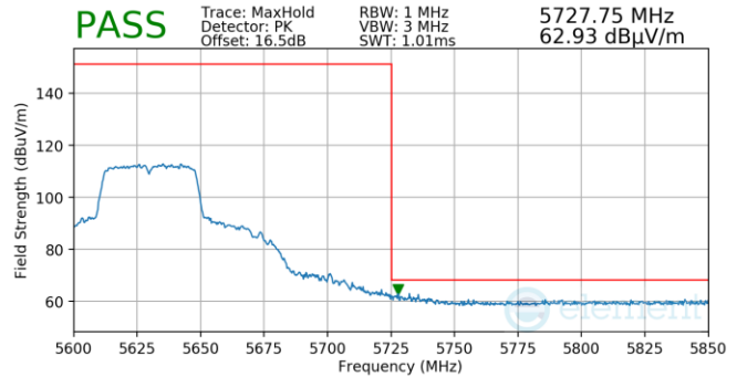
Plot 7-1270. (FCC Only) Antenna 3a (Pk, Ch.126, 802.11n, MCS7)
