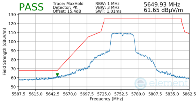
Plot 7-1276. Antenna 3a (Pk, Ch.151, 802.11n, MCS7)
