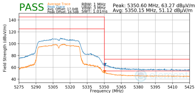
Plot 7-1260. Antenna 3a (Pk & Avg, Ch.62, 802.11n, MCS4)
