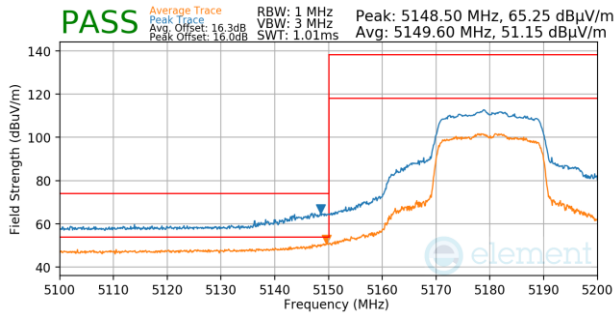
Plot 7-1215. Antenna 3a (Pk & Avg, Ch.36, 802.11ax(SU), MCS4)
