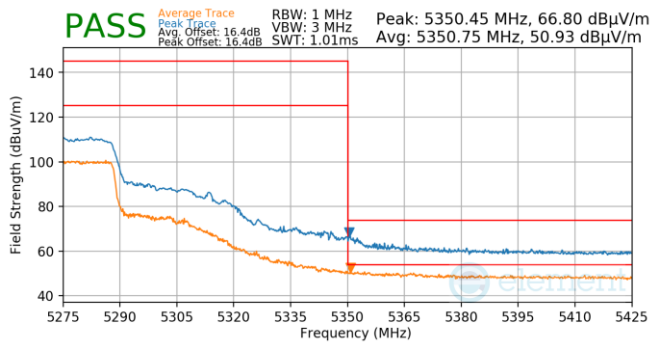
Plot 7-1258. Antenna 3a (Pk & Avg, Ch.54, 802.11n, MCS7)
