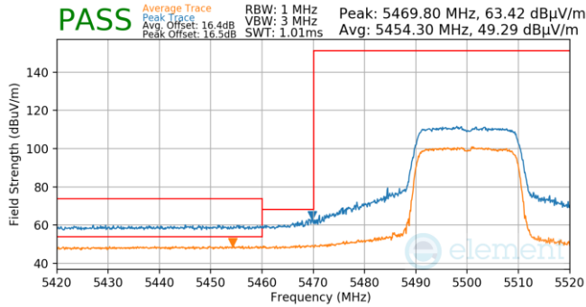
Plot 7-1228. Antenna 3a (Pk & Avg, Ch.100, 802.11ax(SU), MCS11)
