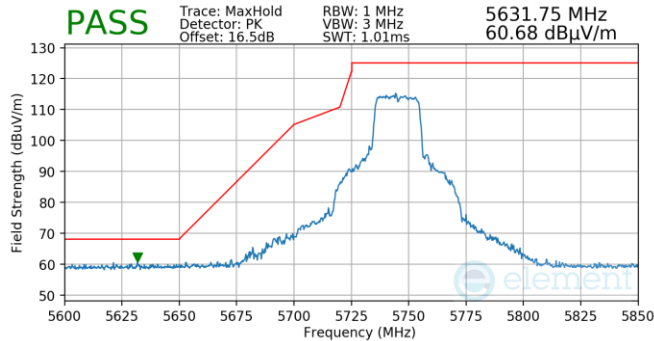
Plot 7-1246. Antenna 3a (Pk, Ch.149, 802.11ax(SU), MCS11)
