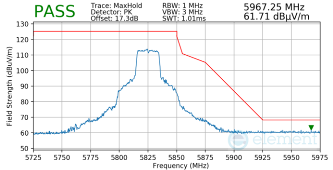
Plot 7-1249. Antenna 3a (Pk, Ch.165, 802.11ax(SU), MCS11)
