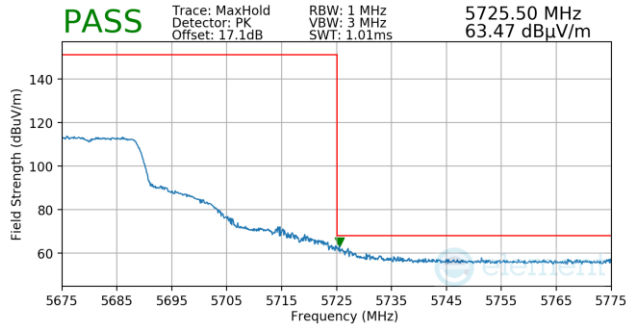
Plot 7-1204. Antenna 3a (Pk, Ch.136, 802.11n, MCS7)
