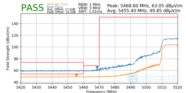
Plot 7-1231. Antenna 3a (Pk & Avg, Ch.104, 802.11ax(SU), MCS11)
