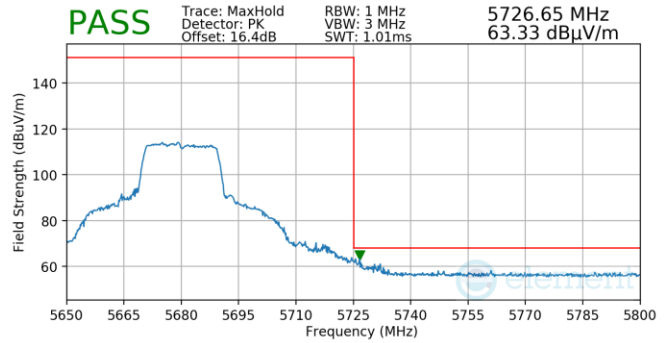
Plot 7-1240. Antenna 3a (Pk, Ch.136, 802.11ax(SU), MCS11)
