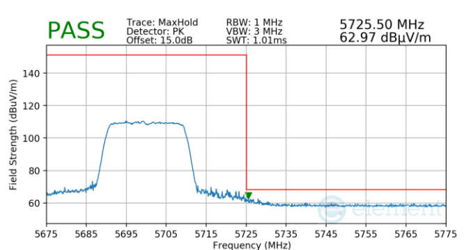
Plot 7-1243. Antenna 3a (Pk, Ch.140, 802.11ax(SU), MCS11)
