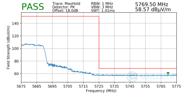
Plot 7-1238. Antenna 3a (Pk, Ch.136, 802.11ax(SU), MCS0)
