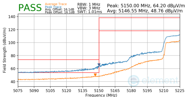
Plot 7-1253. Antenna 3a (Pk & Avg, Ch.46, 802.11n, MCS0)
