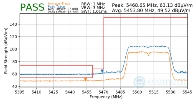
Plot 7-1264. Antenna 3a (Pk & Avg, Ch.102, 802.11n, MCS7)
