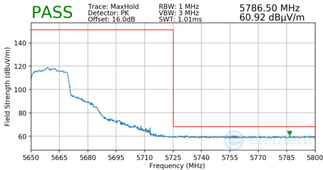
Plot 7-1237. Antenna 3a (Pk, Ch.132, 802.11ax(SU), MCS11)
