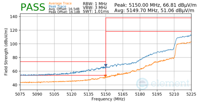
Plot 7-1254. Antenna 3a (Pk & Avg, Ch.46, 802.11n, MCS4)
