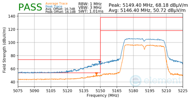
Plot 7-1252. Antenna 3a (Pk & Avg, Ch.38, 802.11n, MCS7)
