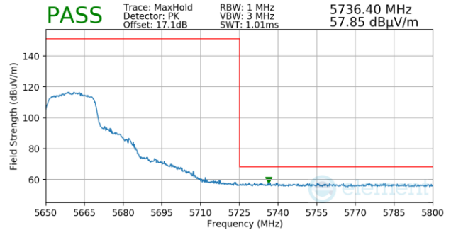
Plot 7-1200. Antenna 3a (Pk, Ch.132, 802.11n, MCS4)
