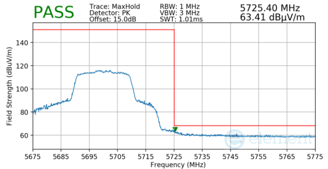
Plot 7-1241. Antenna 3a (Pk, Ch.140, 802.11ax(SU), MCS0)
