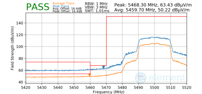
Plot 7-1226. Antenna 3a (Pk & Avg, Ch.100, 802.11ax(SU), MCS0)
