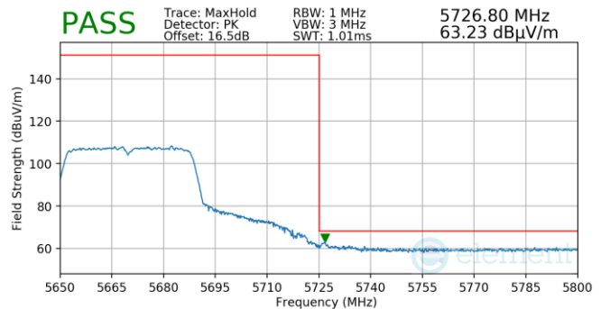
Plot 7-1273. Antenna 3a (Pk, Ch.134, 802.11n, MCS7)
