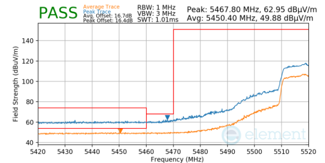
Plot 7-1230. Antenna 3a (Pk & Avg, Ch.104, 802.11ax(SU), MCS4)
