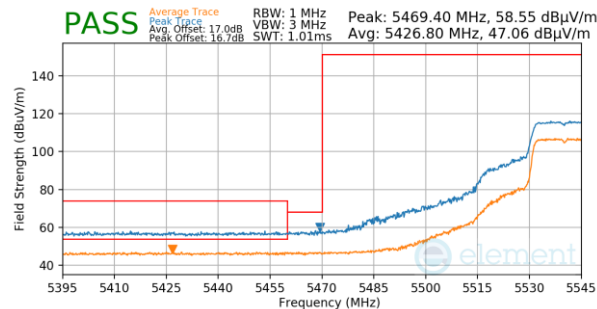
Plot 7-1198. Antenna 3a (Pk & Avg, Ch.108, 802.11n, MCS7)
