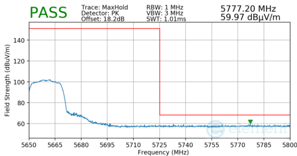
Plot 7-1199. Antenna 3a (Pk, Ch.132, 802.11n, MCS0)
