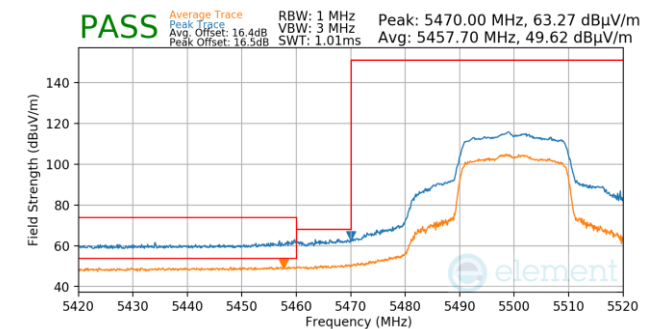
Plot 7-1227. Antenna 3a (Pk & Avg, Ch.100, 802.11ax(SU), MCS4)
