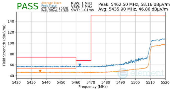
Plot 7-1229. Antenna 3a (Pk & Avg, Ch.104, 802.11ax(SU), MCS0)
