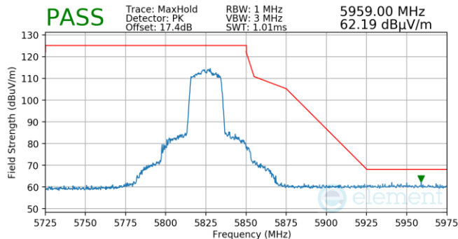
Plot 7-1247. Antenna 3a (Pk, Ch.165, 802.11ax(SU), MCS0)
