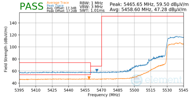
Plot 7-1232. Antenna 3a (Pk & Avg, Ch.108, 802.11ax(SU), MCS0)
