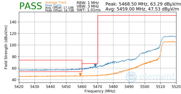
Plot 7-1196. Antenna 3a (Pk & Avg, Ch.104, 802.11n, MCS7)
