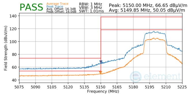
Plot 7-1218. Antenna 3a (Pk & Avg, Ch.40, 802.11ax(SU), MCS4)
