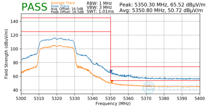
Plot 7-1224. Antenna 3a (Pk & Avg, Ch.64, 802.11ax(SU), MCS4)
