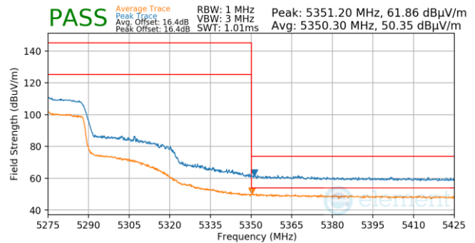
Plot 7-1256. Antenna 3a (Pk & Avg, Ch.54, 802.11n, MCS0)
