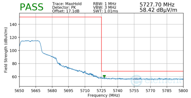
Plot 7-1201. Antenna 3a (Pk, Ch.132, 802.11n, MCS7)
