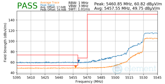
Plot 7-1234. Antenna 3a (Pk & Avg, Ch.108, 802.11ax(SU), MCS11)
