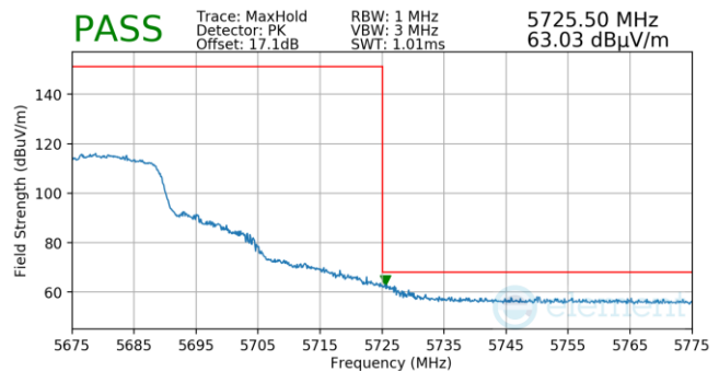
Plot 7-1203. Antenna 3a (Pk, Ch.136, 802.11n, MCS4)
