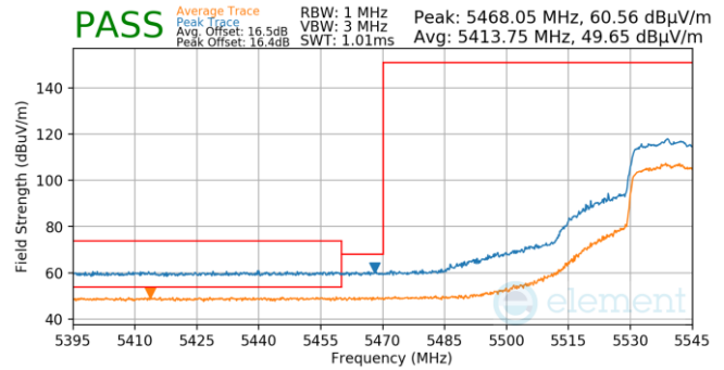
Plot 7-1233. Antenna 3a (Pk & Avg, Ch.108, 802.11ax(SU), MCS4)
