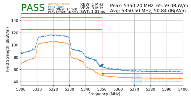
Plot 7-1223. Antenna 3a (Pk & Avg, Ch.64, 802.11ax(SU), MCS0)
