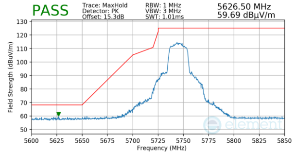
Plot 7-1209. Antenna 3a (Pk, Ch.149, 802.11n, MCS4)
