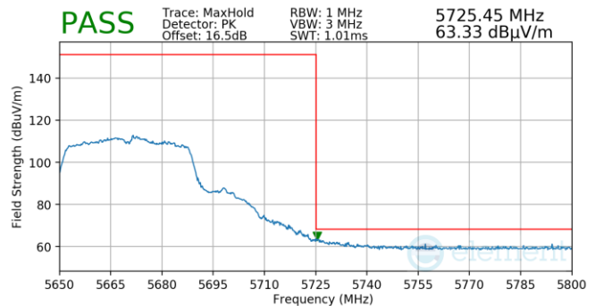
Plot 7-1272. Antenna 3a (Pk, Ch.134, 802.11n, MCS4)
