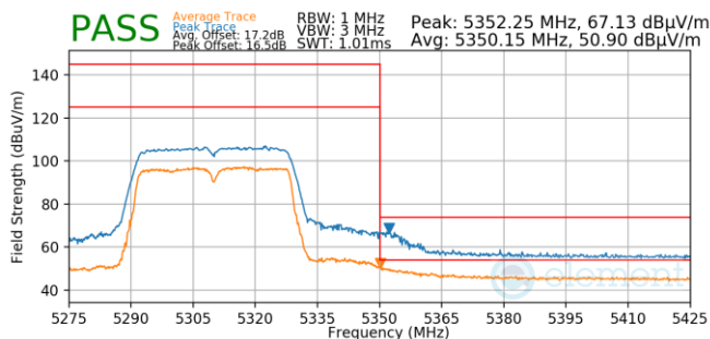
Plot 7-1261. Antenna 3a (Pk & Avg, Ch.62, 802.11n, MCS7)
