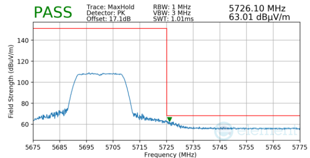
Plot 7-1207. Antenna 3a (Pk, Ch.140, 802.11n, MCS7)
