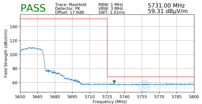
Plot 7-1235. Antenna 3a (Pk, Ch.132, 802.11ax(SU), MCS0)
