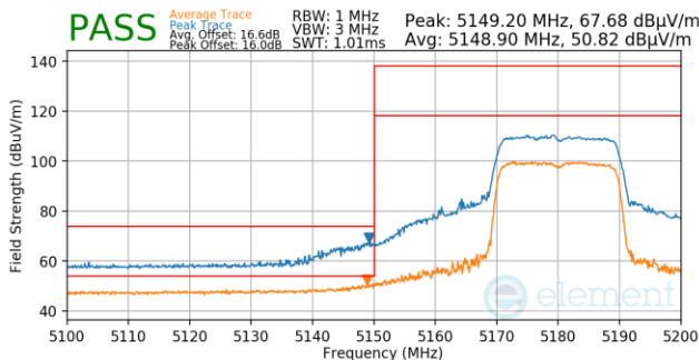
Plot 7-1216. Antenna 3a (Pk & Avg, Ch.36, 802.11ax(SU), MCS11)
