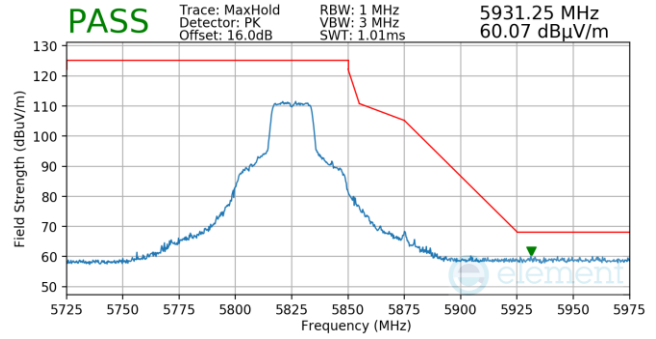
Plot 7-1213. Antenna 3a (Pk, Ch.165, 802.11n, MCS7)
