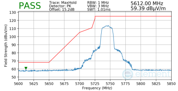
Plot 7-1208. Antenna 3a (Pk, Ch.149, 802.11n, MCS0)
