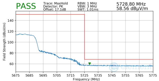
Plot 7-1202. Antenna 3a (Pk, Ch.136, 802.11n, MCS0)
