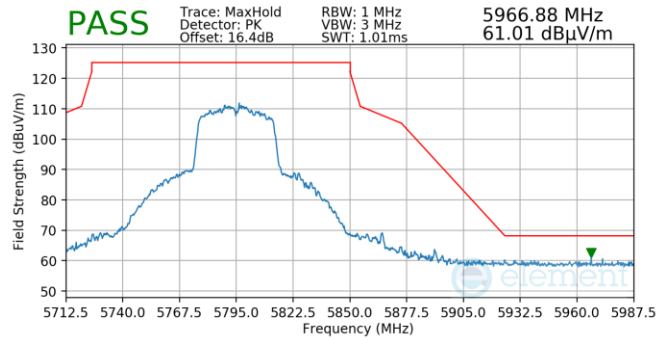
Plot 7-1278. Antenna 3a (Pk, Ch.159, 802.11n, MCS4)
