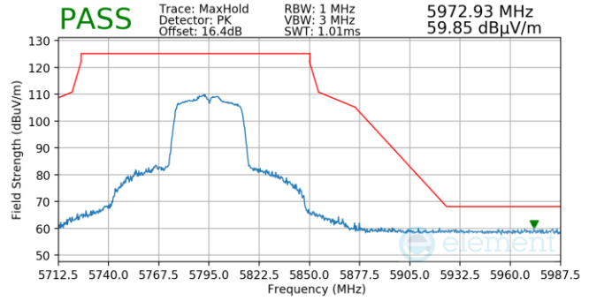
Plot 7-1277. Antenna 3a (Pk, Ch.159, 802.11n, MCS0)
