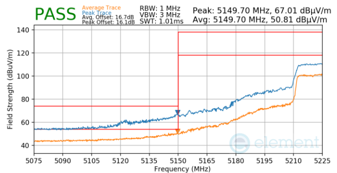
Plot 7-1255. Antenna 3a (Pk & Avg, Ch.46, 802.11n, MCS7)
