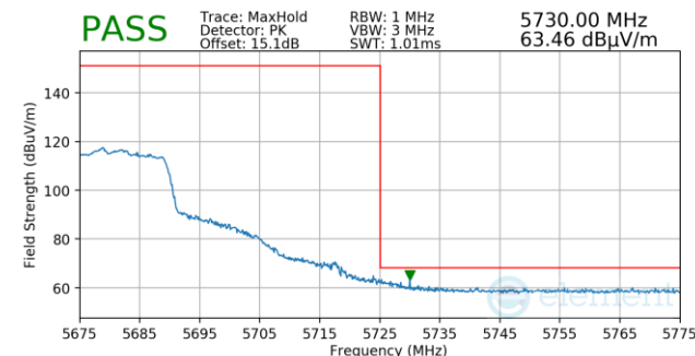
Plot 7-1239. Antenna 3a (Pk, Ch.136, 802.11ax(SU), MCS4)
