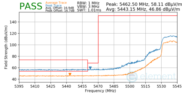
Plot 7-1197. Antenna 3a (Pk & Avg, Ch.108, 802.11n, MCS4)
