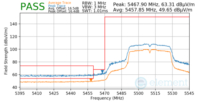
Plot 7-1262. Antenna 3a (Pk & Avg, Ch.102, 802.11n, MCS0)
