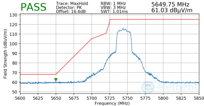
Plot 7-1245. Antenna 3a (Pk, Ch.149, 802.11ax(SU), MCS4)
