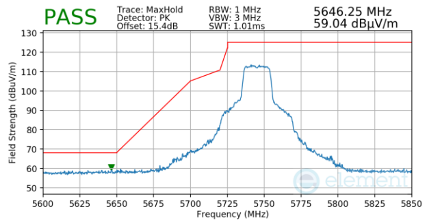
Plot 7-1210. Antenna 3a (Pk, Ch.149, 802.11n, MCS7)
