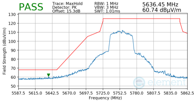
Plot 7-1275. Antenna 3a (Pk, Ch.151, 802.11n, MCS4)
