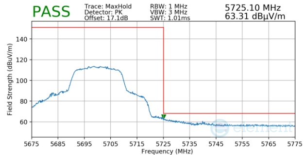
Plot 7-1206. Antenna 3a (Pk, Ch.140, 802.11n, MCS4)
