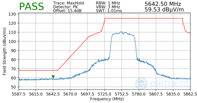
Plot 7-1274. Antenna 3a (Pk, Ch.151, 802.11n, MCS0)
