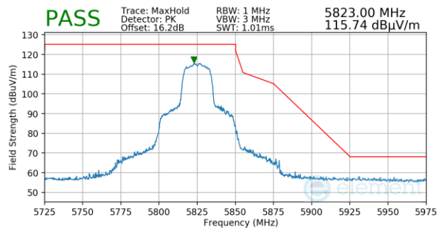
Plot 7-1211. Antenna 3a (Pk, Ch.165, 802.11n, MCS0)
