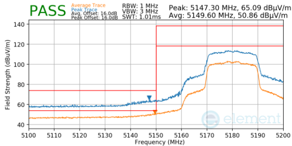
Plot 7-1214. Antenna 3a (Pk & Avg, Ch.36, 802.11ax(SU), MCS0)
