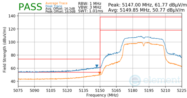
Plot 7-1250. Antenna 3a (Pk & Avg, Ch.38, 802.11n, MCS0)
