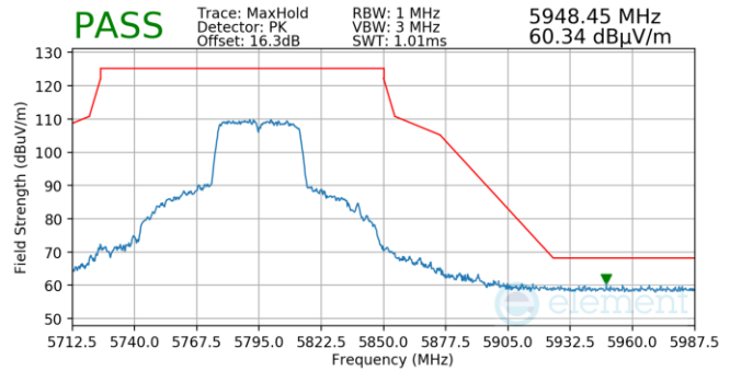
Plot 7-1279. Antenna 3a (Pk, Ch.159, 802.11n, MCS7)
