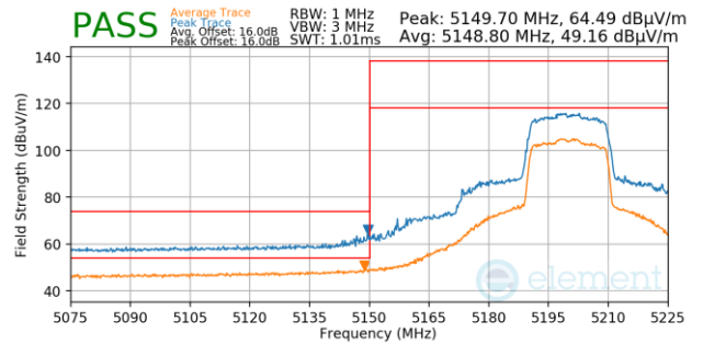
Plot 7-1217. Antenna 3a (Pk & Avg, Ch.40, 802.11ax(SU), MCS0)
