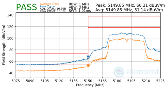
Plot 7-1251. Antenna 3a (Pk & Avg, Ch.38, 802.11n, MCS4)
