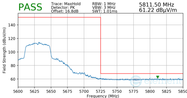
Plot 7-1269. (FCC Only) Antenna 3a (Pk, Ch.126, 802.11n, MCS4)
