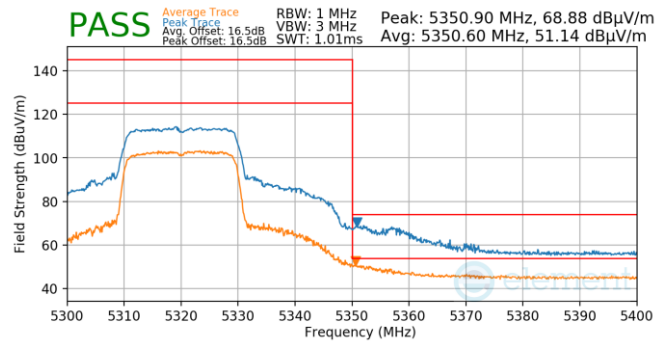
Plot 7-1225. Antenna 3a (Pk & Avg, Ch.64, 802.11ax(SU), MCS11)
