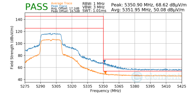
Plot 7-1222. Antenna 3a (Pk & Avg, Ch.60, 802.11ax(SU), MCS11)
