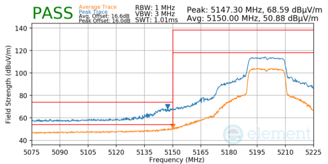
Plot 7-1219. Antenna 3a (Pk & Avg, Ch.40, 802.11ax(SU), MCS11)
