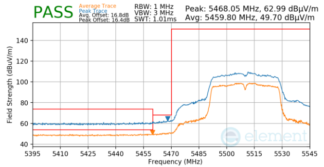
Plot 7-1263. Antenna 3a (Pk & Avg, Ch.102, 802.11n, MCS4)
