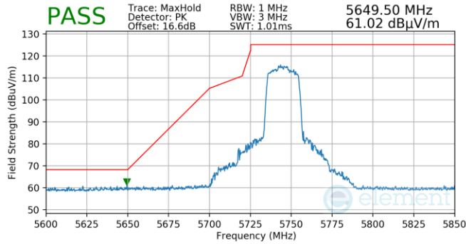
Plot 7-1244. Antenna 3a (Pk, Ch.149, 802.11ax(SU), MCS0)
