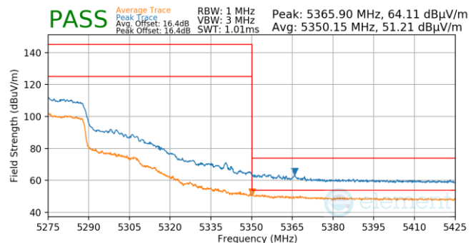
Plot 7-1257. Antenna 3a (Pk & Avg, Ch.54, 802.11n, MCS4)
