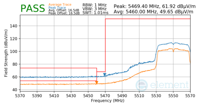
Plot 7-1265. Antenna 3a (Pk & Avg, Ch.110, 802.11n, MCS0)
