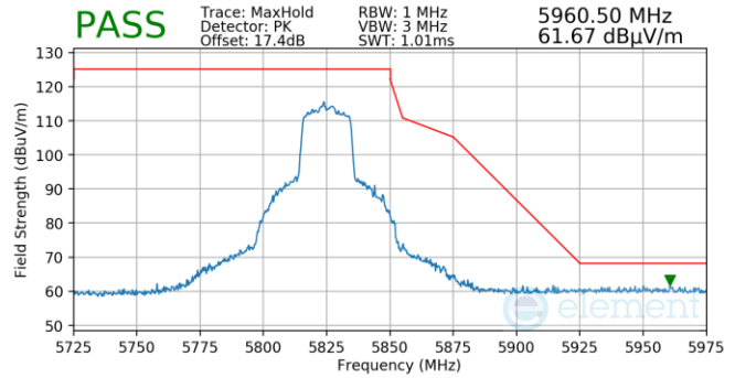
Plot 7-1248. Antenna 3a (Pk, Ch.165, 802.11ax(SU), MCS4)
