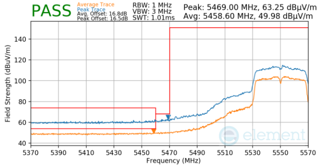
Plot 7-1266. Antenna 3a (Pk & Avg, Ch.110, 802.11n, MCS4)
