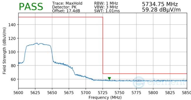
Plot 7-1268. (FCC Only) Antenna 3a (Pk, Ch.126, 802.11n, MCS0)
