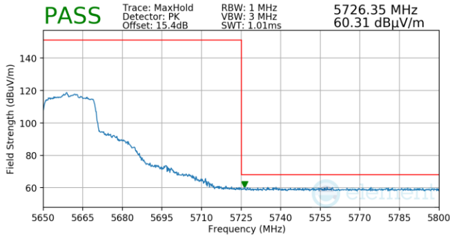
Plot 7-1236. Antenna 3a (Pk, Ch.132, 802.11ax(SU), MCS4)
