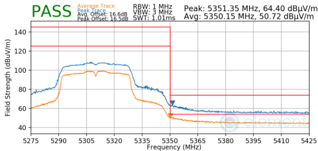
Plot 7-1259. Antenna 3a (Pk & Avg, Ch.62, 802.11n, MCS0)
