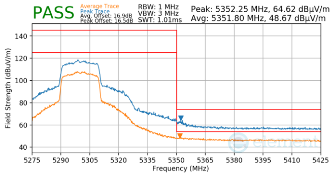
Plot 7-1221. Antenna 3a (Pk & Avg, Ch.60, 802.11ax(SU), MCS4)
