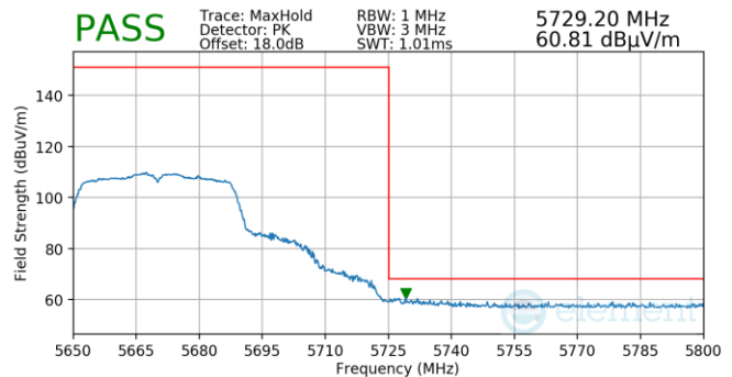
Plot 7-1271. Antenna 3a (Pk, Ch.134, 802.11n, MCS0)
