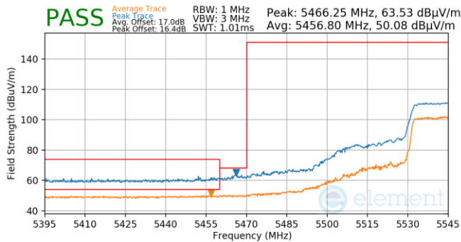
Plot 7-1267. Antenna 3a (Pk & Avg, Ch.110, 802.11n, MCS7)
