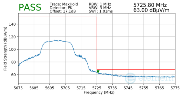
Plot 7-1205. Antenna 3a (Pk, Ch.140, 802.11n, MCS0)
