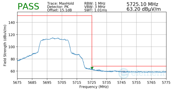
Plot 7-1242. Antenna 3a (Pk, Ch.140, 802.11ax(SU), MCS4)
