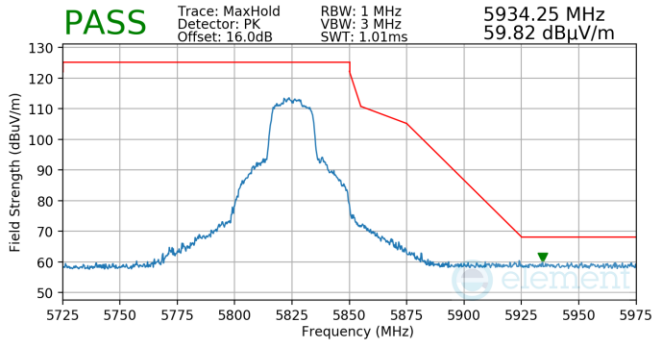
Plot 7-1212. Antenna 3a (Pk, Ch.165, 802.11n, MCS4)
