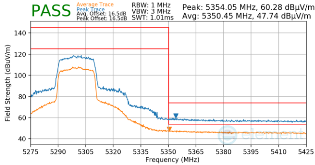
Plot 7-1220. Antenna 3a (Pk & Avg, Ch.60, 802.11ax(SU), MCS0)
