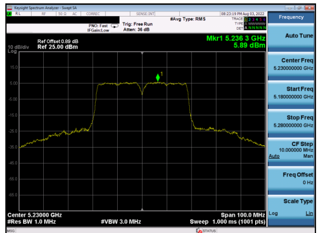
Plot 7-744. PSD CDD Antenna 1b (40MHz BW 802.11n – Ch. 46, MCS15)
