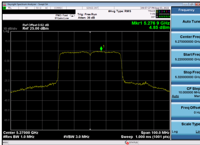
Plot 7-722. PSD CDD Antenna 1b (40MHz BW 802.11ax(SU) – Ch. 54, MCS4)
