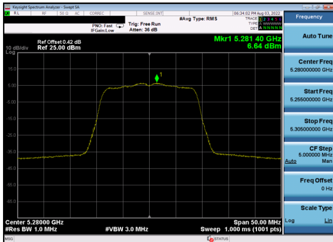
Plot 7-716. PSD CDD Antenna 1b (20MHz BW 802.11n – Ch. 56, MCS12)
