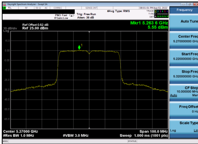
Plot 7-721. PSD CDD Antenna 3c (40MHz BW 802.11ax(SU) – Ch. 54, MCS4)
