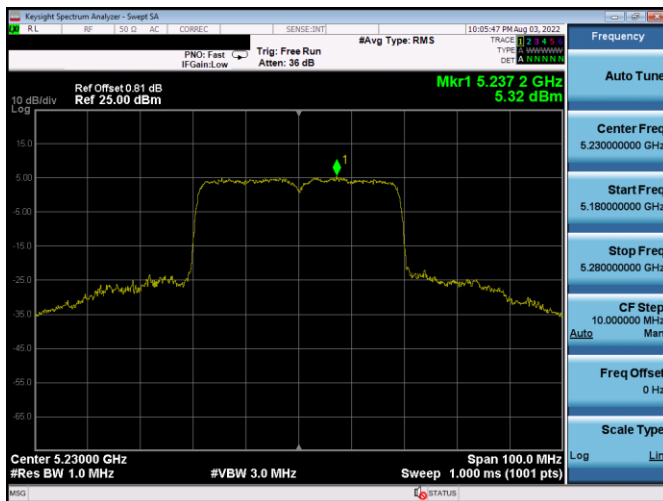
Plot 7-746. PSD CDD Antenna 1b (40MHz BW 802.11ax(SU) – Ch. 46, MCS11)
