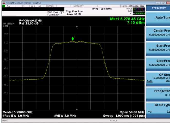
Plot 7-715. PSD CDD Antenna 3c (20MHz BW 802.11n – Ch. 56, MCS12)
