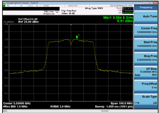
Plot 7-731. PSD CDD Antenna 3c (40MHz BW 802.11n – Ch. 110, MCS12)
