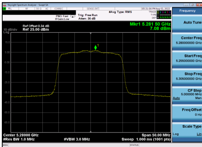
Plot 7-717. PSD CDD Antenna 3c (20MHz BW 802.11ax(SU) – Ch. 56, MCS4)
