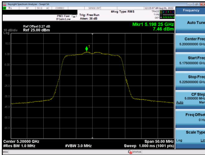
Plot 7-703. PSD CDD Antenna 3c (20MHz BW 802.11n – Ch. 40, MCS12)
