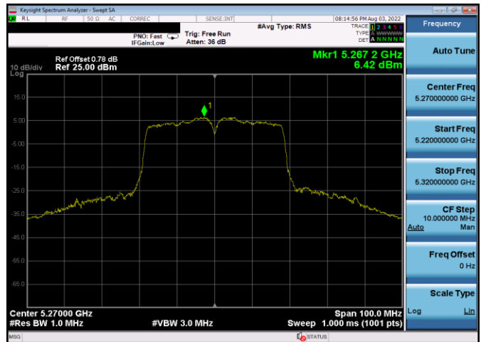
Plot 7-720. PSD CDD Antenna 1b (40MHz BW 802.11n – Ch. 54, MCS12)
