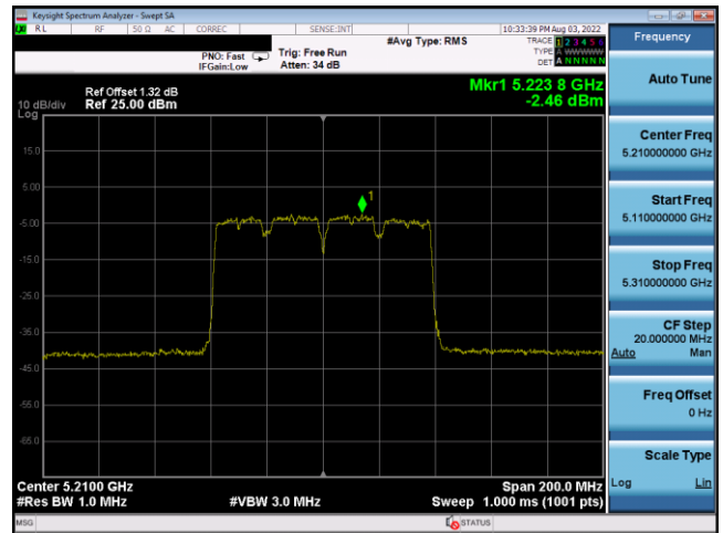
Plot 7-748. PSD CDD Antenna 1b (80MHz BW 802.11ac – Ch. 42, MCS9)
