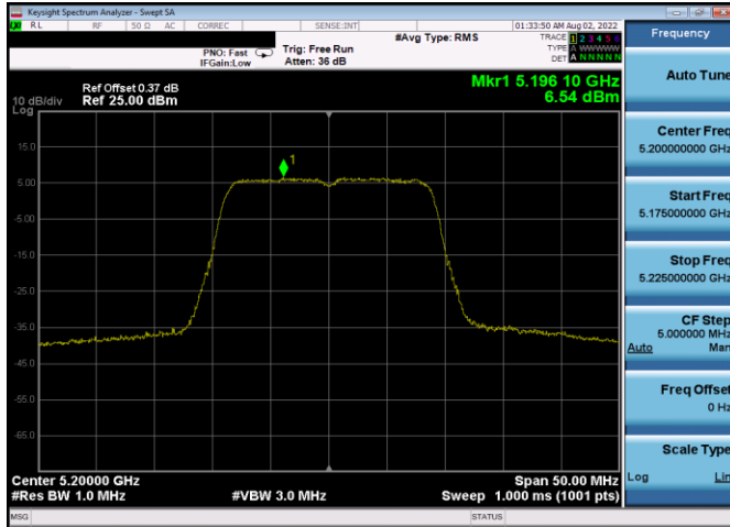
Plot 7-739. PSD CDD Antenna 3c (20MHz BW 802.11n – Ch. 40, MCS15)
