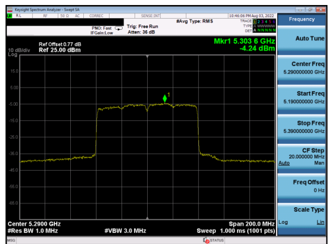
Plot 7-726. PSD CDD Antenna 1b (80MHz BW 802.11ax(SU) – Ch. 58, MCS4)
