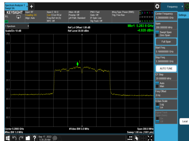
Plot 7-723. PSD CDD Antenna 3c (80MHz BW 802.11ac – Ch. 58, MCS4)
