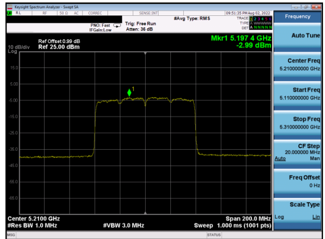
Plot 7-749. PSD CDD Antenna 3c (80MHz BW 802.11ax(SU) – Ch. 42, MCS11)
