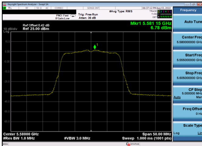
Plot 7-728. PSD CDD Antenna 1b (20MHz BW 802.11n – Ch. 116, MCS12)
