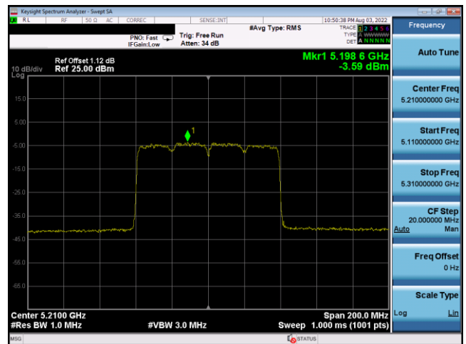
Plot 7-750. PSD CDD Antenna 1b (80MHz BW 802.11ax(SU) – Ch. 42, MCS11)
