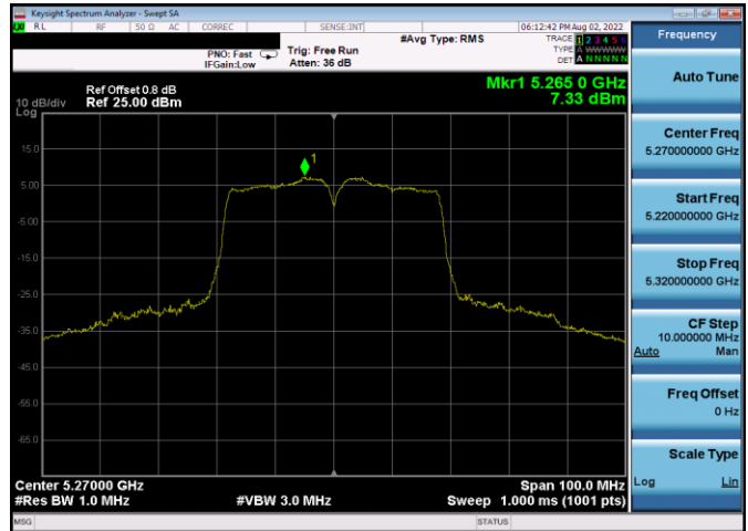
Plot 7-719. PSD CDD Antenna 3c (40MHz BW 802.11n – Ch. 54, MCS12)
