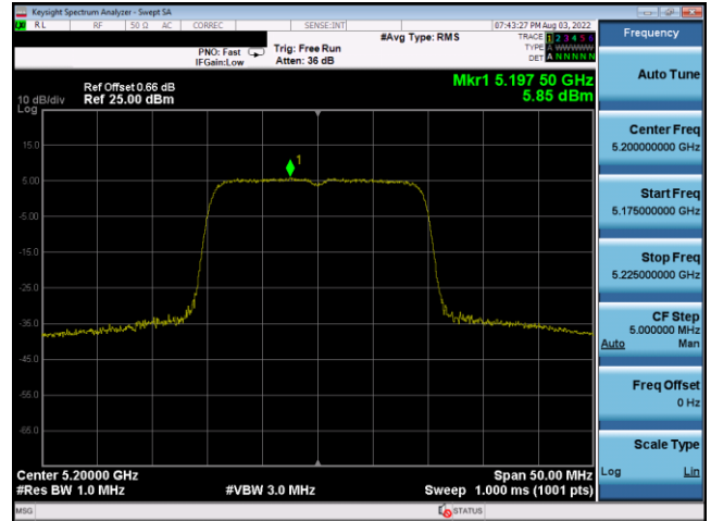
Plot 7-742. PSD CDD Antenna 1b (20MHz BW 802.11ax(SU) – Ch. 40, MCS11)
