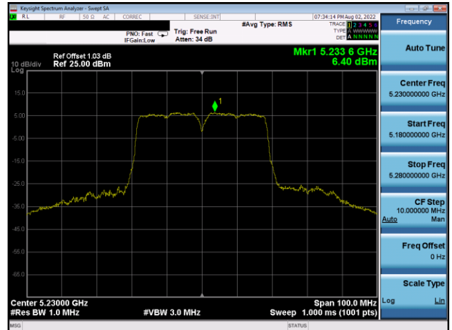
Plot 7-743. PSD CDD Antenna 3c (40MHz BW 802.11n – Ch. 46, MCS15)
