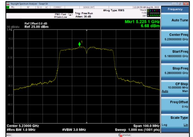
Plot 7-707. PSD CDD Antenna 3c (40MHz BW 802.11n – Ch. 46, MCS12)
