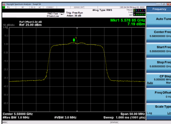
Plot 7-729. PSD CDD Antenna 3c (20MHz BW 802.11ax(SU) – Ch. 116, MCS4)
