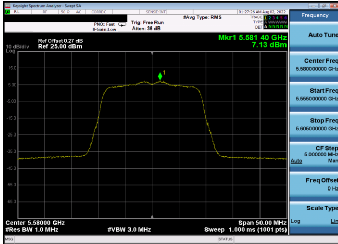
Plot 7-727. PSD CDD Antenna 3c (20MHz BW 802.11n – Ch. 116, MCS12)
