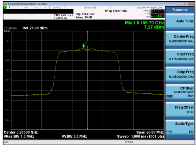
Plot 7-706. PSD CDD Antenna 1b (20MHz BW 802.11ax(SU) – Ch. 40, MCS4)
