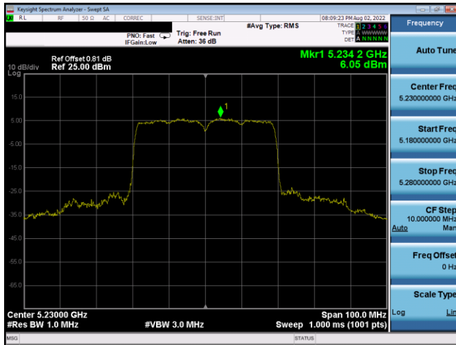
Plot 7-745. PSD CDD Antenna 3c (40MHz BW 802.11ax(SU) – Ch. 46, MCS11)
