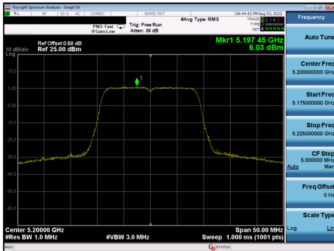
Plot 7-740. PSD CDD Antenna 1b (20MHz BW 802.11n – Ch. 40, MCS15)
