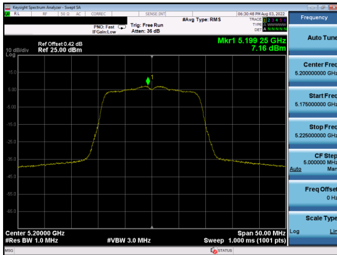
Plot 7-704. PSD CDD Antenna 1b (20MHz BW 802.11n – Ch. 40, MCS12)
