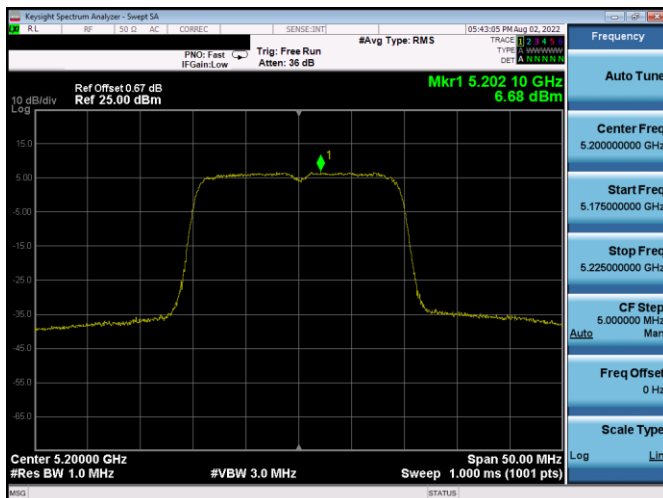
Plot 7-741. PSD CDD Antenna 3c (20MHz BW 802.11ax(SU) – Ch. 40, MCS11)
