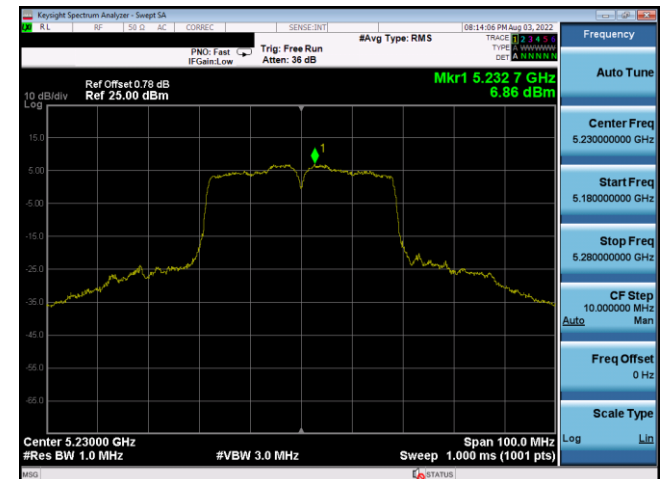
Plot 7-708. PSD CDD Antenna 1b (40MHz BW 802.11n – Ch. 46, MCS12)
