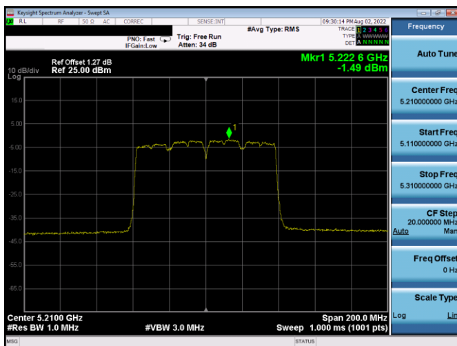
Plot 7-747. PSD CDD Antenna 3c (80MHz BW 802.11ac – Ch. 42, MCS9)
