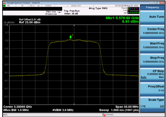
Plot 7-730. PSD CDD Antenna 1b (20MHz BW 802.11ax(SU) – Ch. 116, MCS4)
