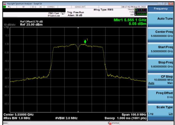
Plot 7-732. PSD CDD Antenna 1b (40MHz BW 802.11n – Ch. 110, MCS12)
