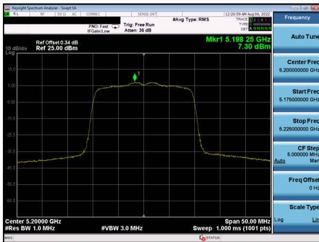
Plot 7-705. PSD CDD Antenna 3c (20MHz BW 802.11ax(SU) – Ch. 40, MCS4)
