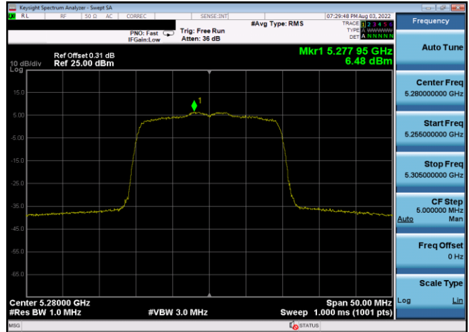
Plot 7-718. PSD CDD Antenna 1b (20MHz BW 802.11ax(SU) – Ch. 56, MCS4)
