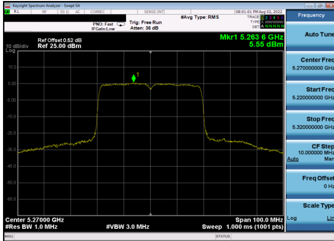
Plot 7-541. PSD CDD Antenna 3c (40MHz BW 802.11ax(SU) – Ch. 54, MCS4)
