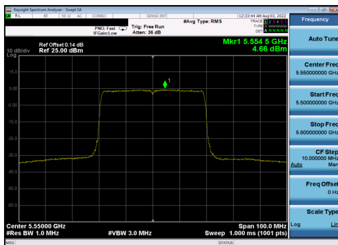
Plot 7-518. PSD CDD Antenna 3a (40MHz BW 802.11ax(SU) – Ch. 110, MCS0)
