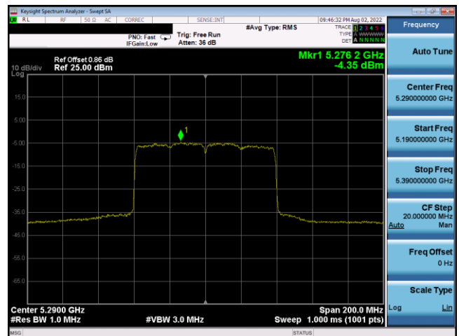
Plot 7-545. PSD CDD Antenna 3c (80MHz BW 802.11ax(SU) – Ch. 58, MCS4)
