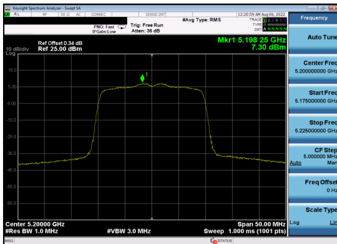
Plot 7-525. PSD CDD Antenna 3c (20MHz BW 802.11ax(SU) – Ch. 40, MCS4)
