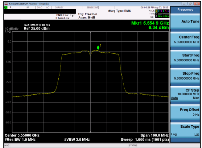
Plot 7-515. PSD CDD Antenna 3c (40MHz BW 802.11n – Ch. 110, MCS8)
