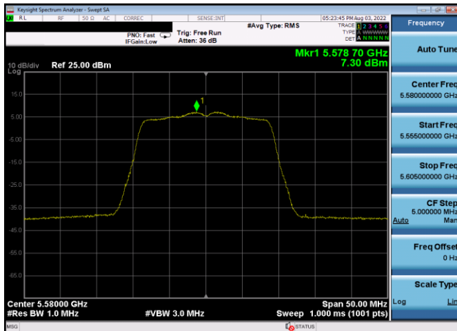
Plot 7-512. PSD CDD Antenna 3a (20MHz BW 802.11n – Ch. 116, MCS8)
