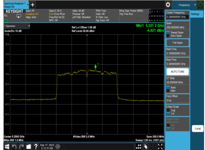
Plot 7-544. PSD CDD Antenna 3a (80MHz BW 802.11ac – Ch. 58, MCS4)
