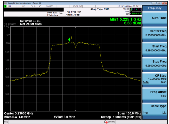
Plot 7-527. PSD CDD Antenna 3c (40MHz BW 802.11n – Ch. 46, MCS12)
