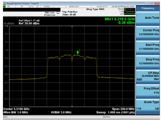
Plot 7-532. PSD CDD Antenna 3a (80MHz BW 802.11ac – Ch. 42, MCS4)
