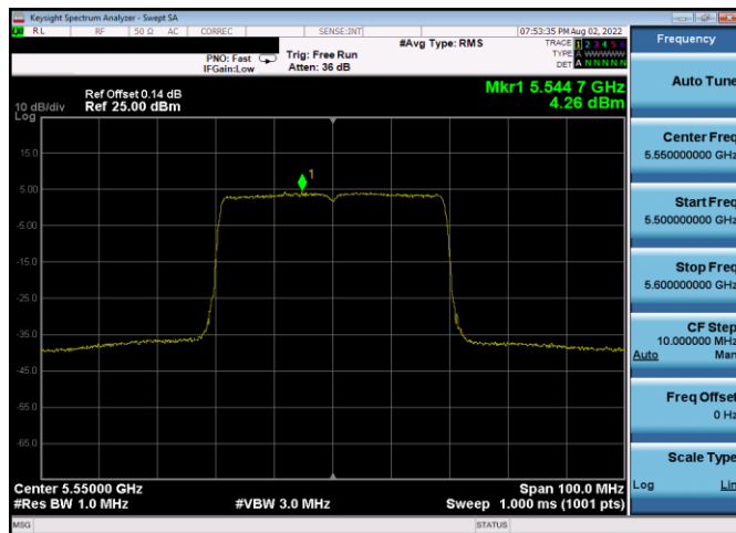
Plot 7-517. PSD CDD Antenna 3c (40MHz BW 802.11ax(SU) – Ch. 110, MCS0)
