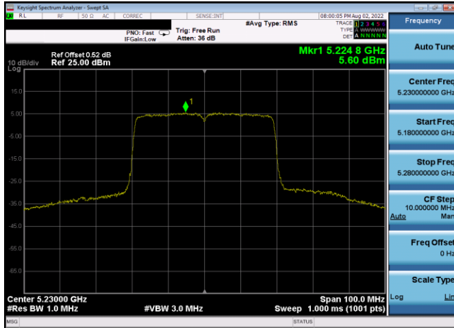
Plot 7-529. PSD CDD Antenna 3c (40MHz BW 802.11ax(SU) – Ch. 46, MCS4)
