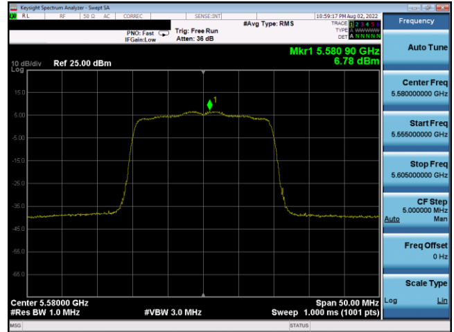
Plot 7-514. PSD CDD Antenna 3a (20MHz BW 802.11ax(SU) – Ch. 116, MCS0)
