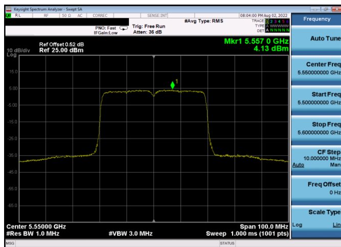
Plot 7-553. PSD CDD Antenna 3c (40MHz BW 802.11ax(SU) – Ch. 110, MCS4)
