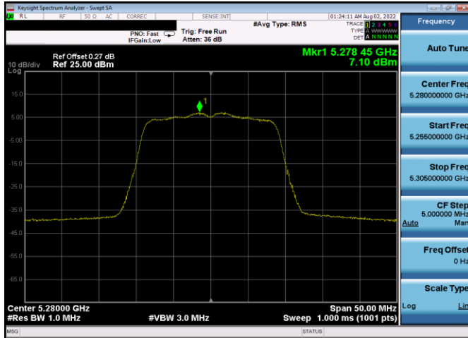
Plot 7-535. PSD CDD Antenna 3c (20MHz BW 802.11n – Ch. 56, MCS12)
