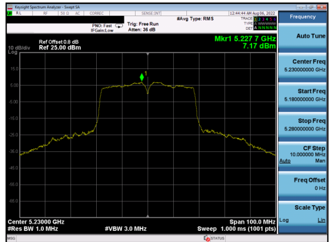
Plot 7-528. PSD CDD Antenna 3a (40MHz BW 802.11n – Ch. 46, MCS12)
