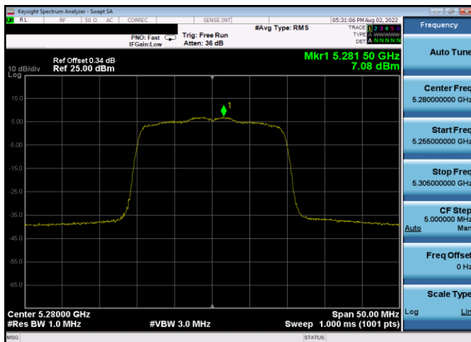
Plot 7-537. PSD CDD Antenna 3c (20MHz BW 802.11ax(SU) – Ch. 56, MCS4)
