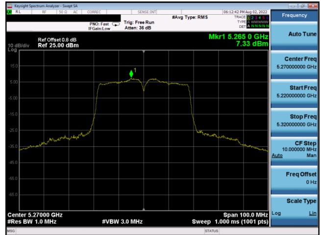
Plot 7-539. PSD CDD Antenna 3c (40MHz BW 802.11n – Ch. 54, MCS12)
