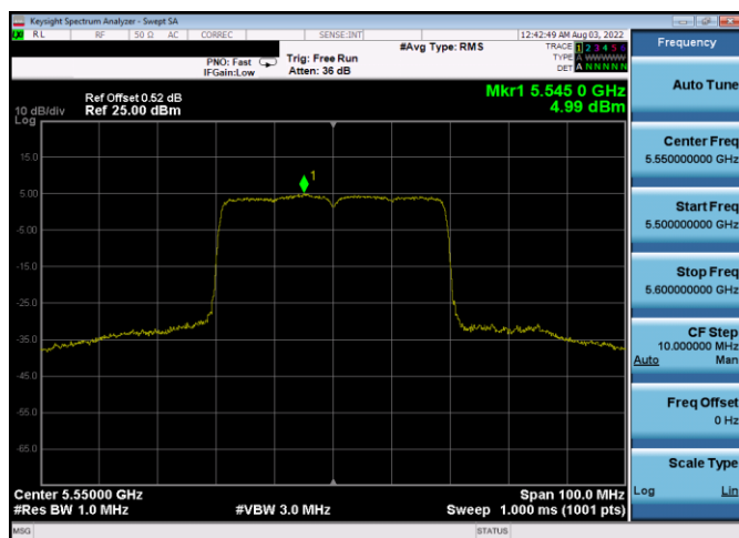
Plot 7-554. PSD CDD Antenna 3a (40MHz BW 802.11ax(SU) – Ch. 110, MCS4)
