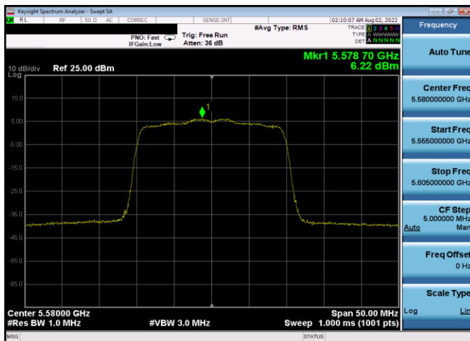
Plot 7-513. PSD CDD Antenna 3c (20MHz BW 802.11ax(SU) – Ch. 116, MCS0)
