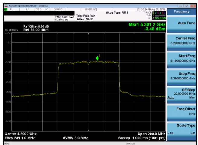
Plot 7-546. PSD CDD Antenna 3a (80MHz BW 802.11ax(SU) – Ch. 58, MCS4)
