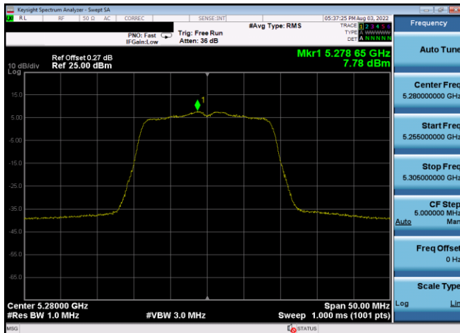
Plot 7-536. PSD CDD Antenna 3a (20MHz BW 802.11n – Ch. 56, MCS12)
