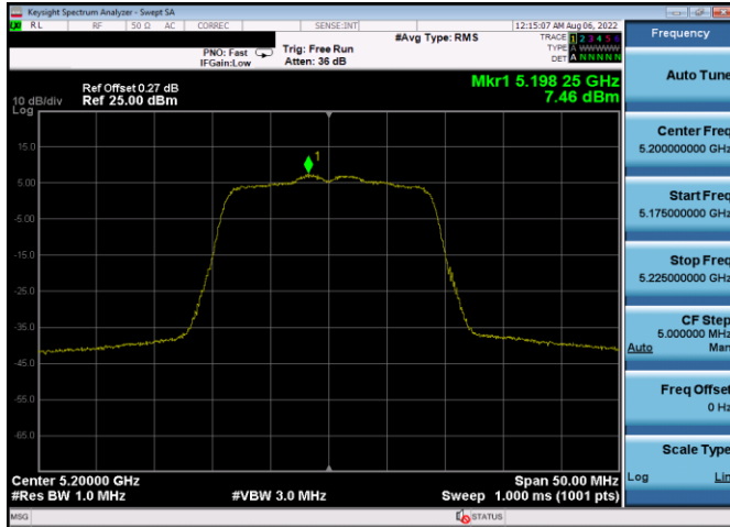
Plot 7-523. PSD CDD Antenna 3c (20MHz BW 802.11n – Ch. 40, MCS12)
