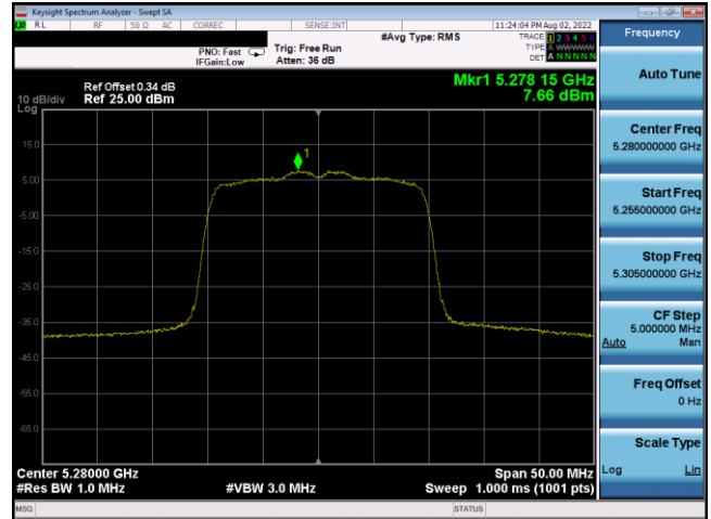
Plot 7-538. PSD CDD Antenna 3a (20MHz BW 802.11ax(SU) – Ch. 56, MCS4)
