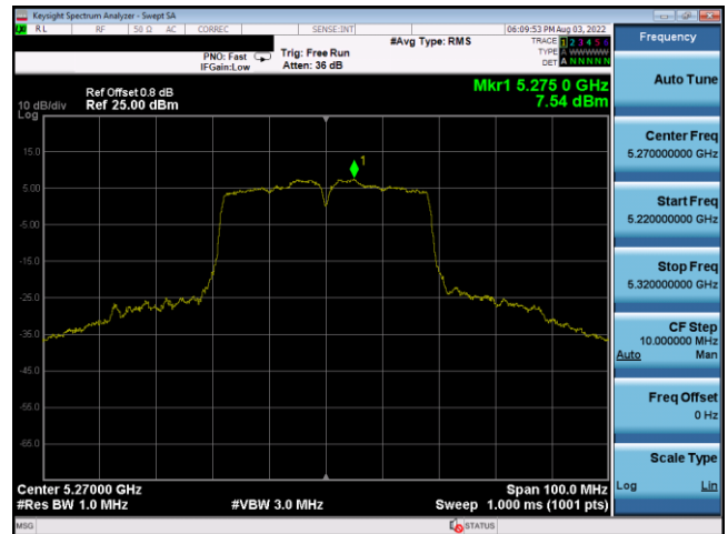
Plot 7-540. PSD CDD Antenna 3a (40MHz BW 802.11n – Ch. 54, MCS12)
