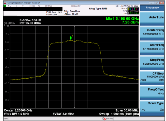
Plot 7-526. PSD CDD Antenna 3a (20MHz BW 802.11ax(SU) – Ch. 40, MCS4)
