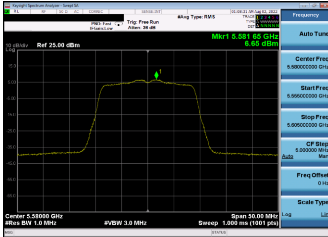
Plot 7-511. PSD CDD Antenna 3c (20MHz BW 802.11n – Ch. 116, MCS8)
