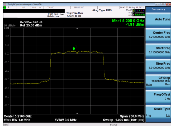
Plot 7-533. PSD CDD Antenna 3c (80MHz BW 802.11ax(SU) – Ch. 42, MCS4)
