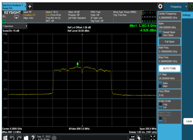
Plot 7-543. PSD CDD Antenna 3c (80MHz BW 802.11ac – Ch. 58, MCS4)
