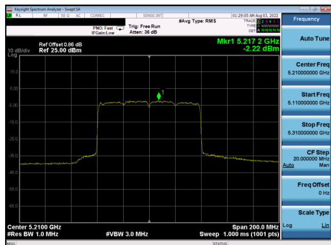
Plot 7-534. PSD CDD Antenna 3a (80MHz BW 802.11ax(SU) – Ch. 42, MCS4)
