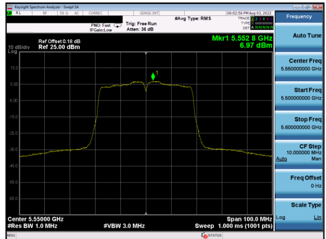
Plot 7-516. PSD CDD Antenna 3a (40MHz BW 802.11n – Ch. 110, MCS8)
