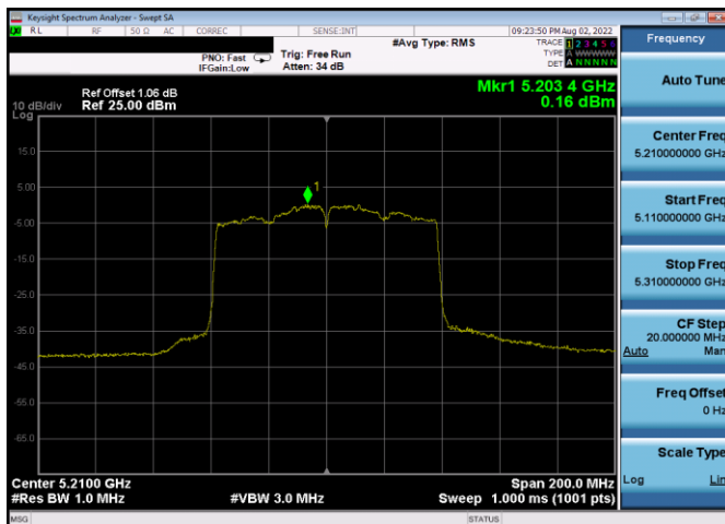
Plot 7-531. PSD CDD Antenna 3c (80MHz BW 802.11ac – Ch. 42, MCS4)
