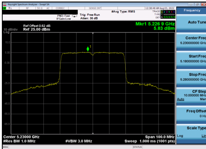
Plot 7-530. PSD CDD Antenna 3a (40MHz BW 802.11ax(SU) – Ch. 46, MCS4)
