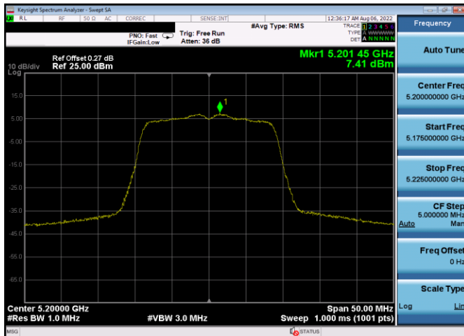
Plot 7-524. PSD CDD Antenna 3a (20MHz BW 802.11n – Ch. 40, MCS12)
