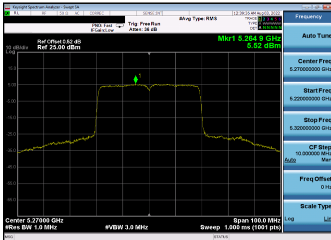
Plot 7-542. PSD CDD Antenna 3a (40MHz BW 802.11ax(SU) – Ch. 54, MCS4)
