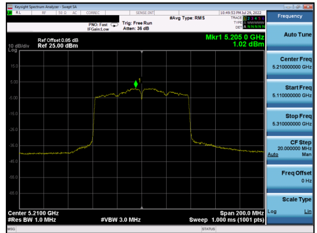
Plot 7-239. PSD Antenna 3c (80MHz BW 802.11ac – Ch. 42, MCS4)
