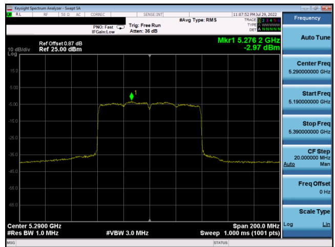
Plot 7-246. PSD Antenna 3c (80MHz BW 802.11ax(SU) – Ch. 58, MCS4)
