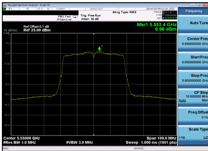
Plot 7-231. PSD Antenna 3c (40MHz BW 802.11n – Ch. 110, MCS0)
