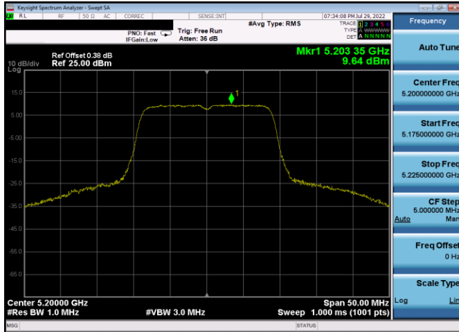
Plot 7-253. PSD Antenna 3c (20MHz BW 802.11n – Ch. 40, MCS7)
