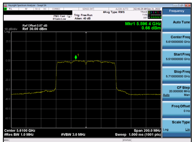
Plot 7-252. PSD Antenna 3c (80MHz BW 802.11ax(SU) – Ch. 122, MCS4)
