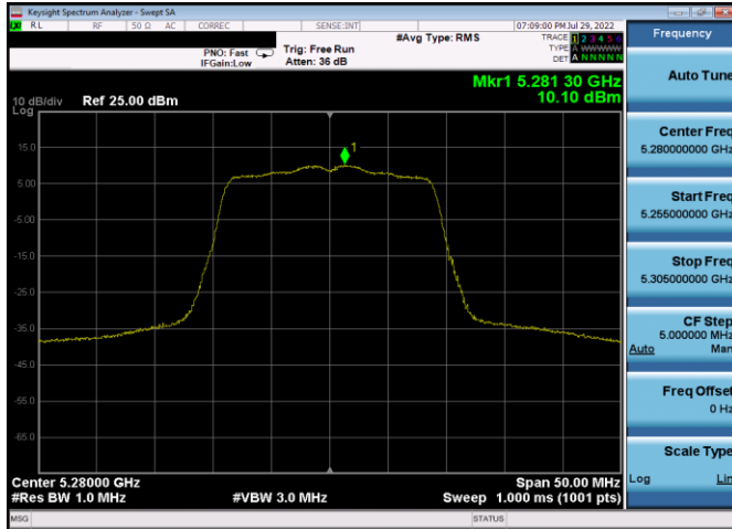
Plot 7-223. PSD Antenna 3c (20MHz BW 802.11n – Ch. 56, MCS0)
