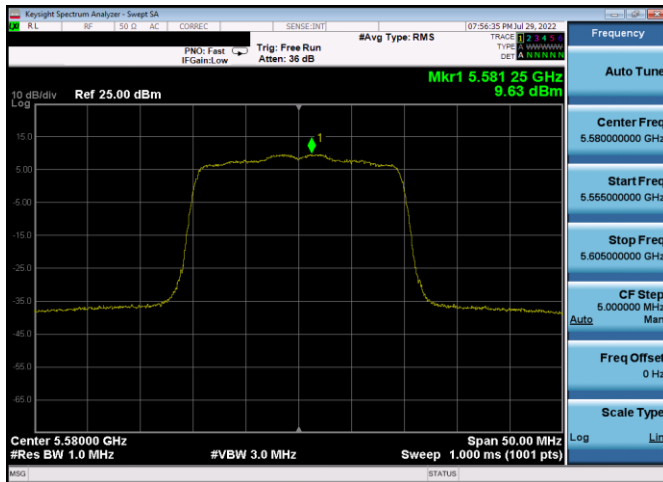
Plot 7-230. PSD Antenna 3c (20MHz BW 802.11ax(SU) – Ch. 116, MCS0)
