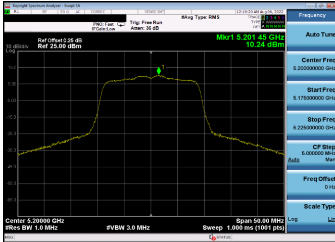
Plot 7-235. PSD Antenna 3c (20MHz BW 802.11n – Ch. 40, MCS4)
