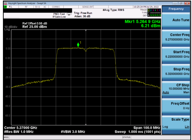
Plot 7-244. PSD Antenna 3c (40MHz BW 802.11ax(SU) – Ch. 54, MCS4)
