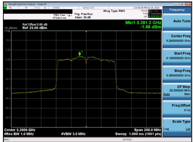
Plot 7-245. PSD Antenna 3c (80MHz BW 802.11ac – Ch. 58, MCS4)
