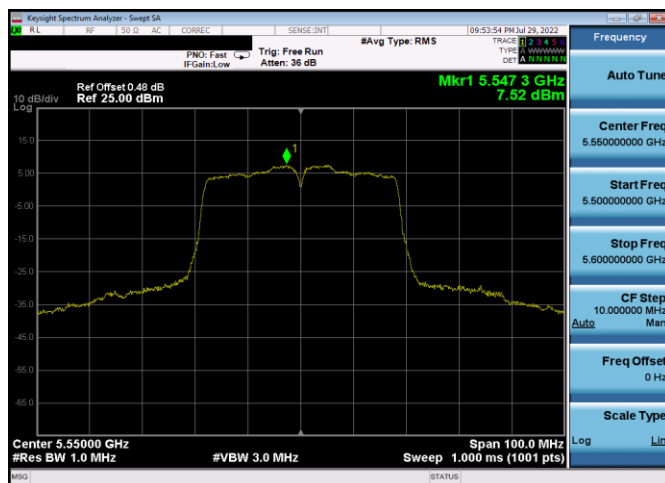
Plot 7-249. PSD Antenna 3c (40MHz BW 802.11n – Ch. 110, MCS4)
