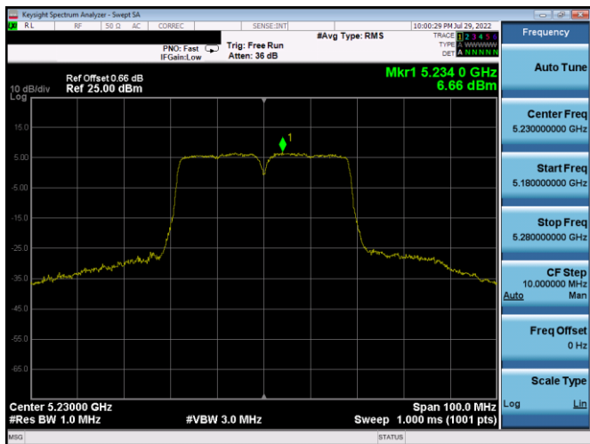
Plot 7-255. PSD Antenna 3c (40MHz BW 802.11n – Ch. 46, MCS7)
