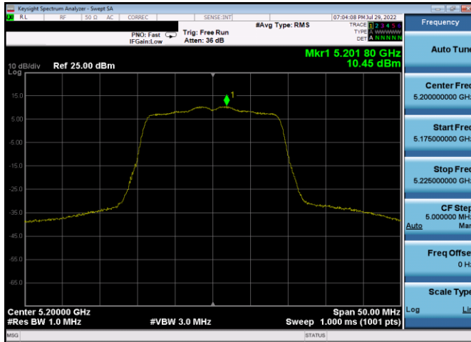
Plot 7-217. PSD Antenna 3c (20MHz BW 802.11n – Ch. 40, MCS0)
