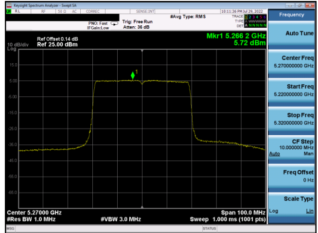
Plot 7-226. PSD Antenna 3c (40MHz BW 802.11ax(SU) – Ch. 54, MCS0)
