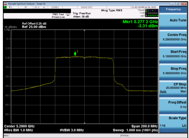
Plot 7-228. PSD Antenna 3c (80MHz BW 802.11ax(SU) – Ch. 58, MCS0)
