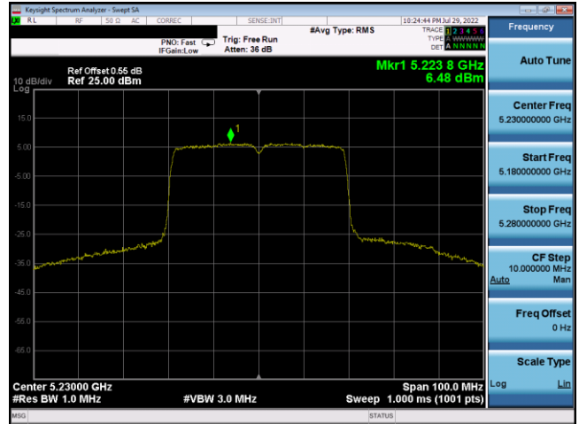
Plot 7-238. PSD Antenna 3c (40MHz BW 802.11ax(SU) – Ch. 46, MCS4)
