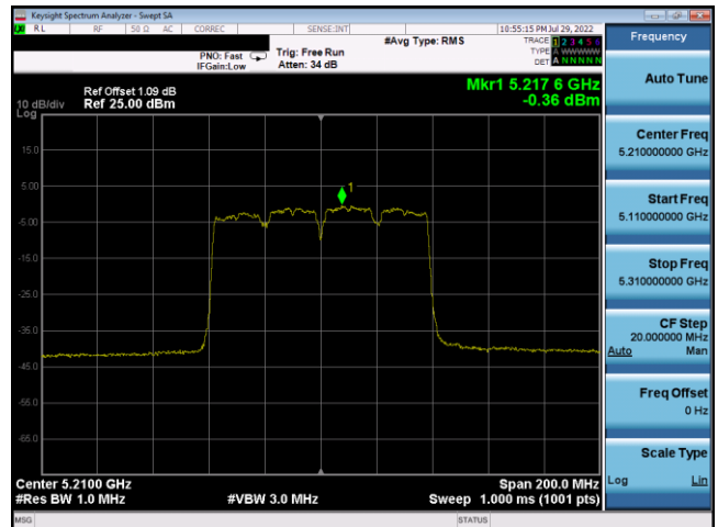
Plot 7-257. PSD Antenna 3c (80MHz BW 802.11ac – Ch. 42, MCS9)
