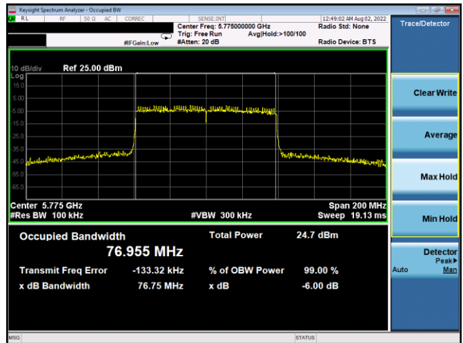
Plot 7-216. 6dB BW & 99% OBW Antenna 1b (80MHz BW 802.11ax(SU) – Ch. 155, MCS11)
