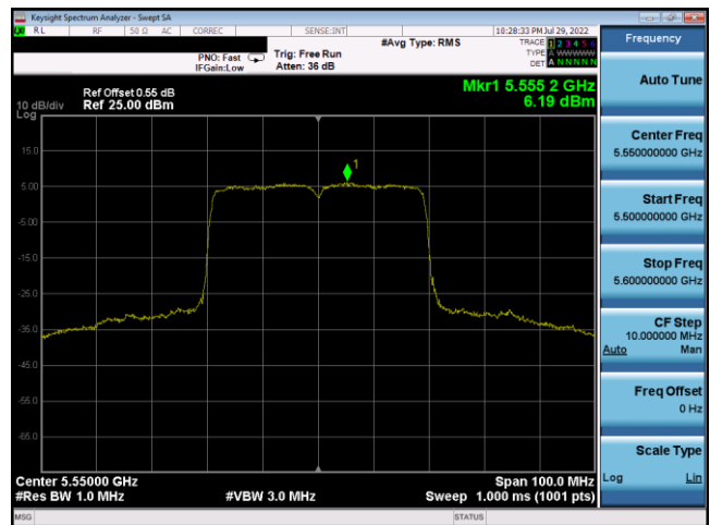
Plot 7-250. PSD Antenna 3c (40MHz BW 802.11ax(SU) – Ch. 110, MCS4)
