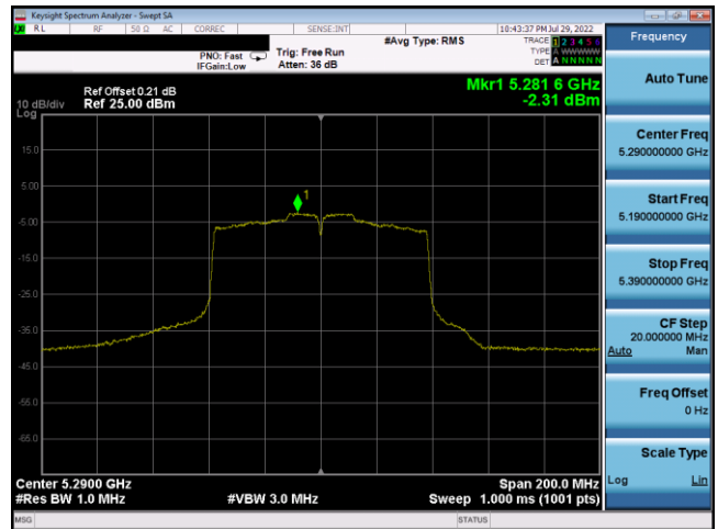
Plot 7-227. PSD Antenna 3c (80MHz BW 802.11ac – Ch. 58, MCS0)
