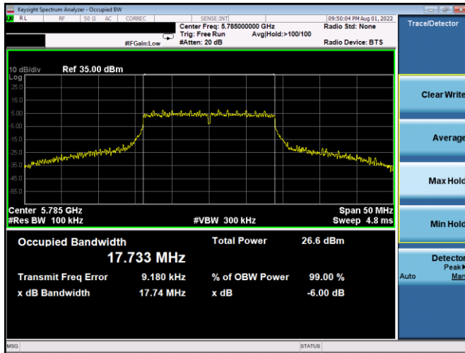
Plot 7-211. 6dB BW & 99% OBW Antenna 1b (20MHz BW 802.11n – Ch. 157, MCS7)
