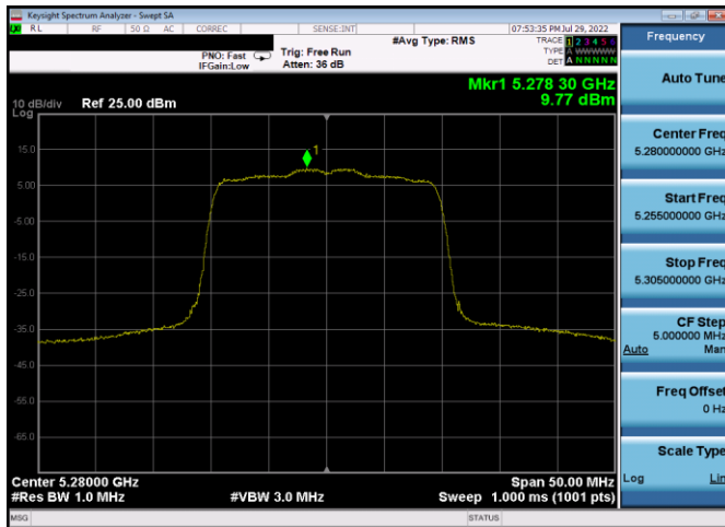
Plot 7-224. PSD Antenna 3c (20MHz BW 802.11ax(SU) – Ch. 56, MCS0)
