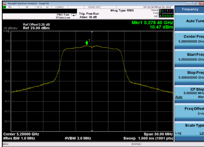
Plot 7-241. PSD Antenna 3c (20MHz BW 802.11n – Ch. 56, MCS4)
