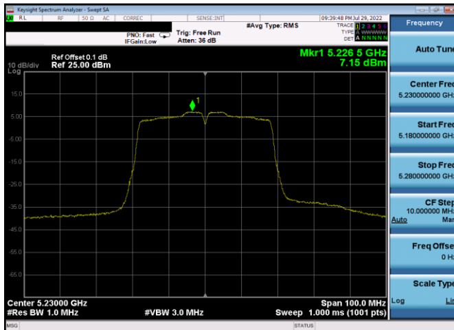
Plot 7-219. PSD Antenna 3c (40MHz BW 802.11n – Ch. 46, MCS0)
