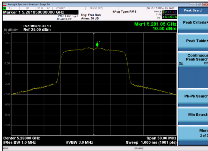
Plot 7-242. PSD Antenna 3c (20MHz BW 802.11ax(SU) – Ch. 56, MCS4)
