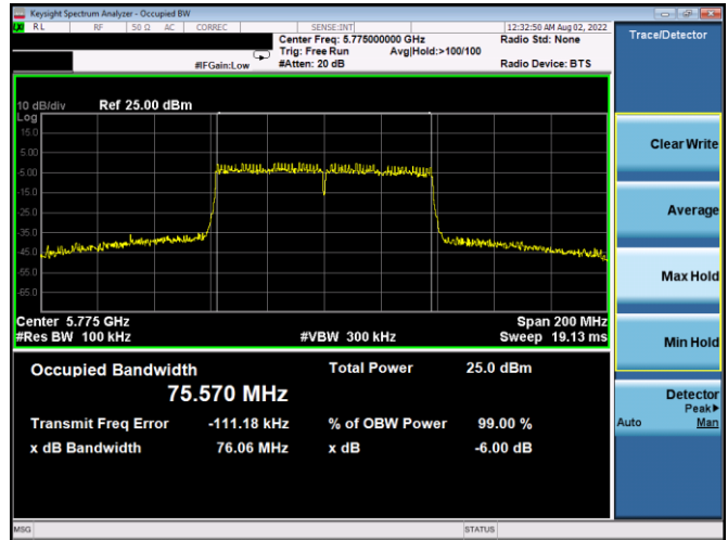
Plot 7-215. 6dB BW & 99% OBW Antenna 1b (80MHz BW 802.11ac – Ch. 155, MCS9)
