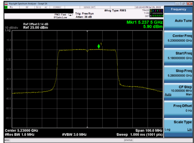
Plot 7-220. PSD Antenna 3c (40MHz BW 802.11ax(SU) – Ch. 46, MCS0)
