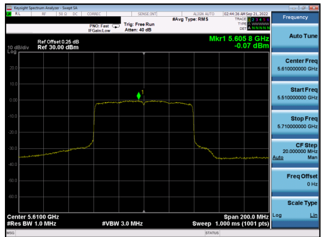
Plot 7-234. PSD Antenna 3c (80MHz BW 802.11ax(SU) – Ch. 122, MCS0)
