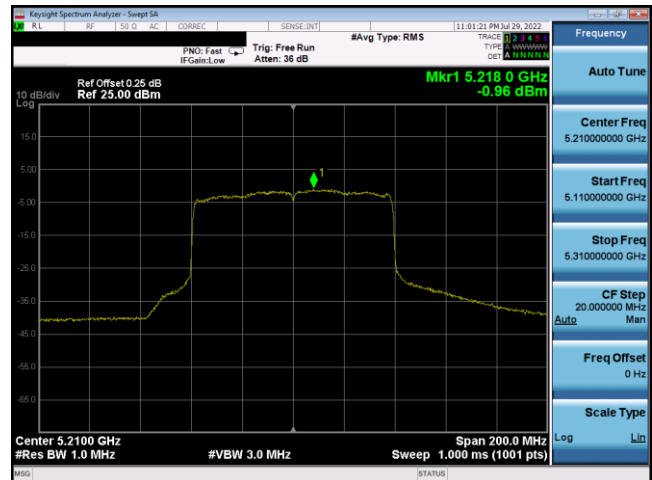
Plot 7-222. PSD Antenna 3c (80MHz BW 802.11ax(SU) – Ch. 42, MCS0)
