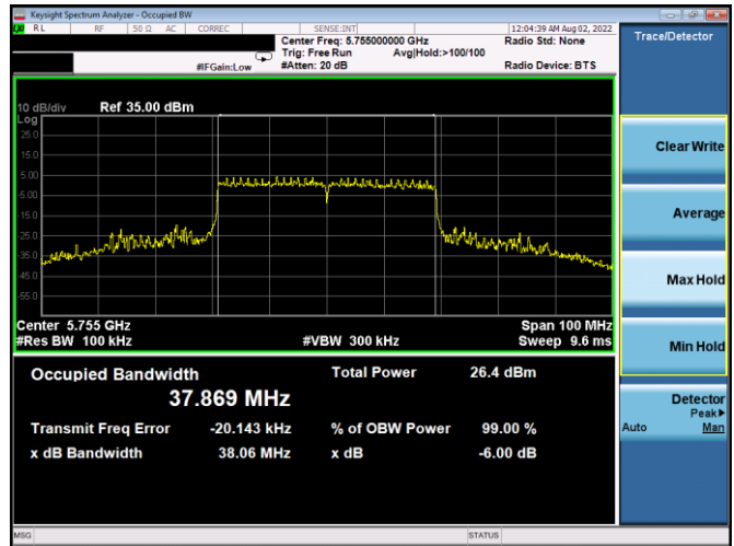
Plot 7-214. 6dB BW & 99% OBW Antenna 1b (40MHz BW 802.11ax(SU) – Ch. 151, MCS11)
