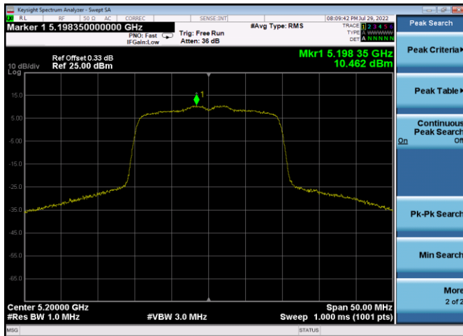
Plot 7-236. PSD Antenna 3c (20MHz BW 802.11ax(SU) – Ch. 40, MCS4)
