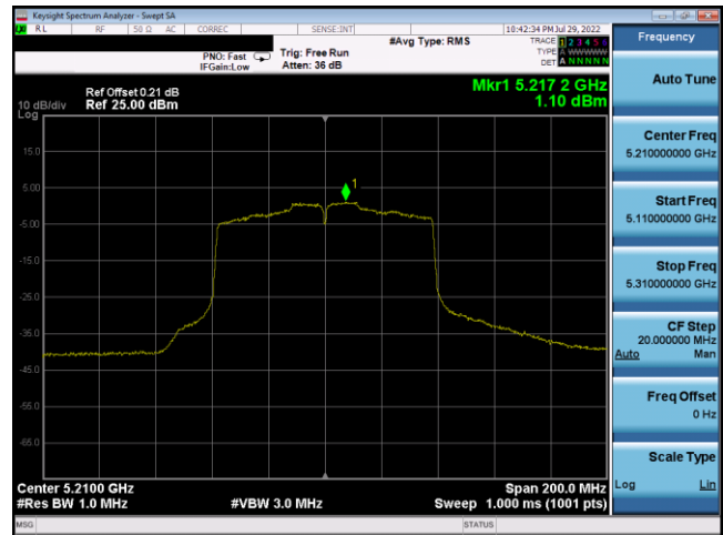
Plot 7-221. PSD Antenna 3c (80MHz BW 802.11ac – Ch. 42, MCS0)
