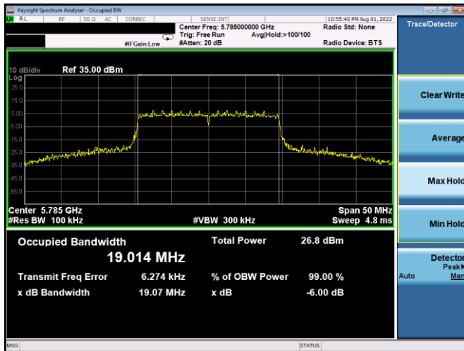
Plot 7-212. 6dB BW & 99% OBW Antenna 1b (20MHz BW 802.11ax(SU) – Ch. 157, MCS11)
