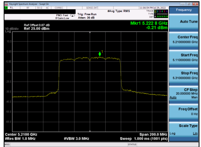
Plot 7-240. PSD Antenna 3c (80MHz BW 802.11ax(SU) – Ch. 42, MCS4)
