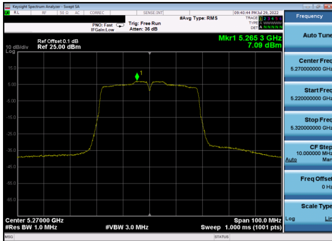
Plot 7-225. PSD Antenna 3c (40MHz BW 802.11n – Ch. 54, MCS0)
