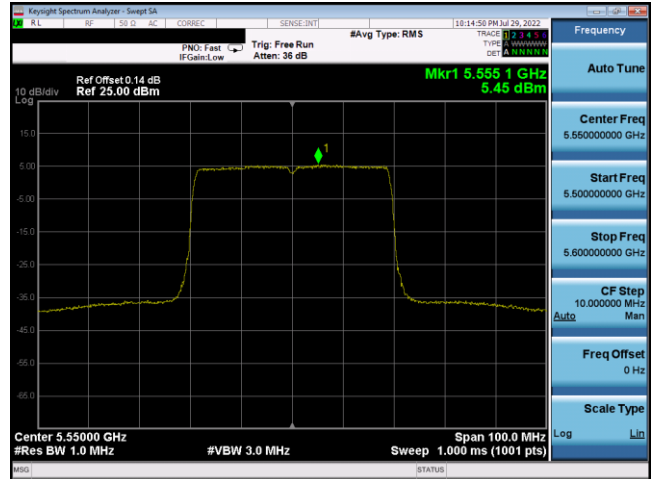
Plot 7-232. PSD Antenna 3c (40MHz BW 802.11ax(SU) – Ch. 110, MCS0)
