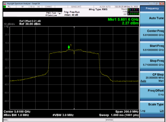
Plot 7-233. PSD Antenna 3c (80MHz BW 802.11ac – Ch. 122, MCS0)
