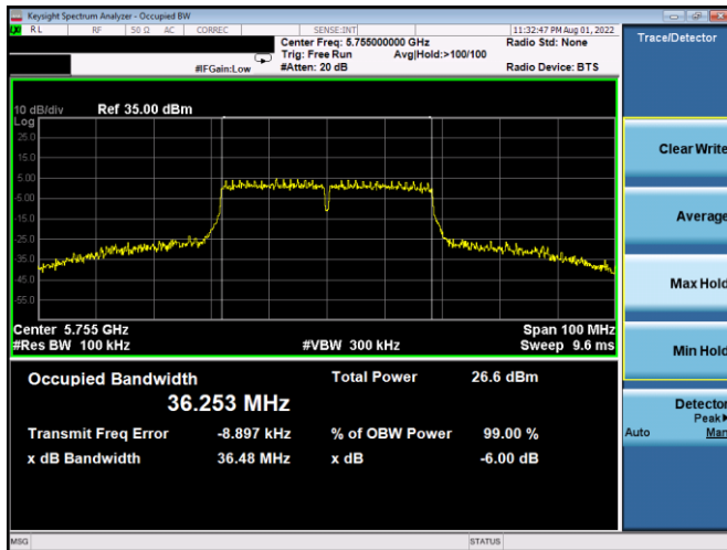
Plot 7-213. 6dB BW & 99% OBW Antenna 1b (40MHz BW 802.11n – Ch. 151, MCS7)
