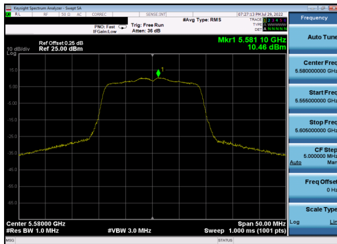
Plot 7-247. PSD Antenna 3c (20MHz BW 802.11n – Ch. 116, MCS4)
