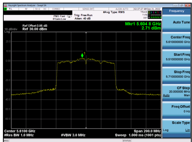
Plot 7-251. PSD Antenna 3c (80MHz BW 802.11ac – Ch. 122, MCS4)
