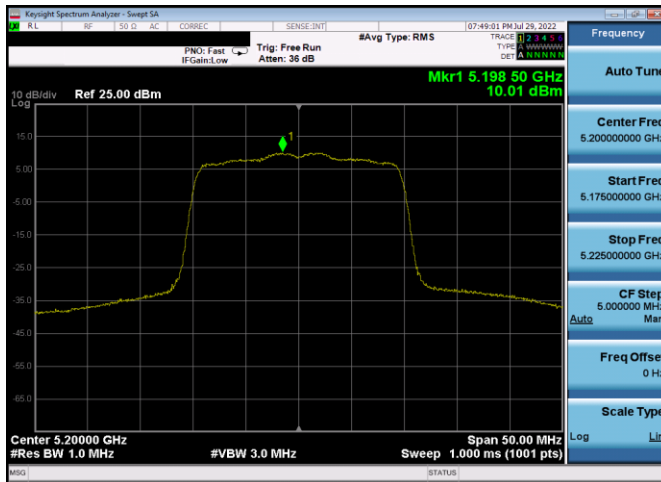
Plot 7-218. PSD Antenna 3c (20MHz BW 802.11ax(SU) – Ch. 40, MCS0)
