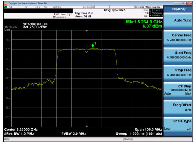
Plot 7-256. PSD Antenna 3c (40MHz BW 802.11ax(SU) – Ch. 46, MCS11)
