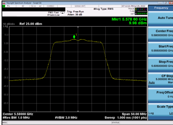
Plot 7-229. PSD Antenna 3c (20MHz BW 802.11n – Ch. 116, MCS0)
