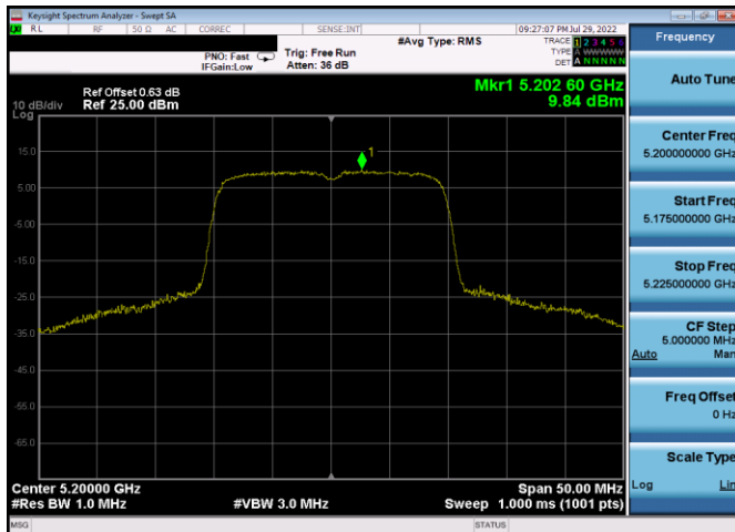
Plot 7-254. PSD Antenna 3c (20MHz BW 802.11ax(SU) – Ch. 40, MCS11)
