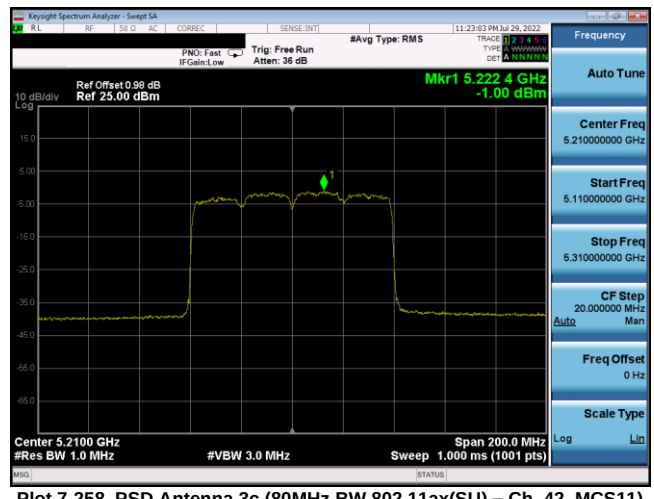
Plot 7-258. PSD Antenna 3c (80MHz BW 802.11ax(SU) – Ch. 42, MCS11)
