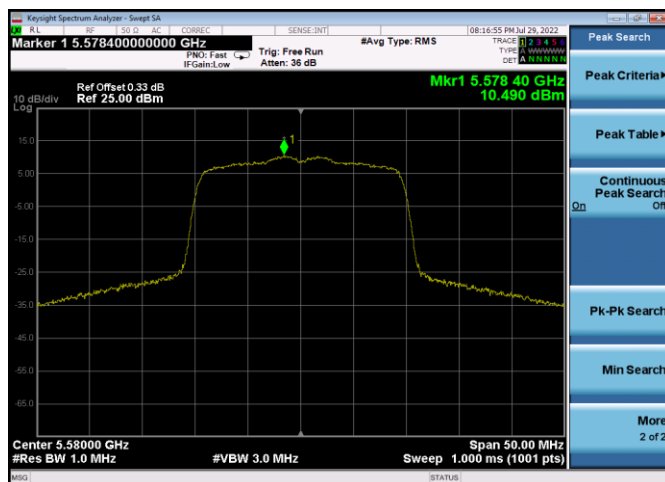
Plot 7-248. PSD Antenna 3c (20MHz BW 802.11ax(SU) – Ch. 116, MCS4)
