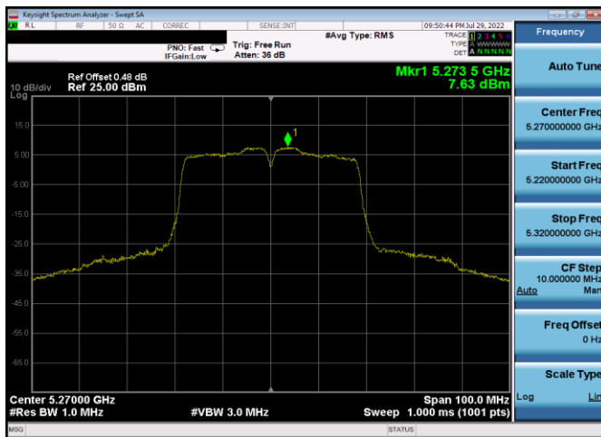
Plot 7-243. PSD Antenna 3c (40MHz BW 802.11n – Ch. 54, MCS4)
