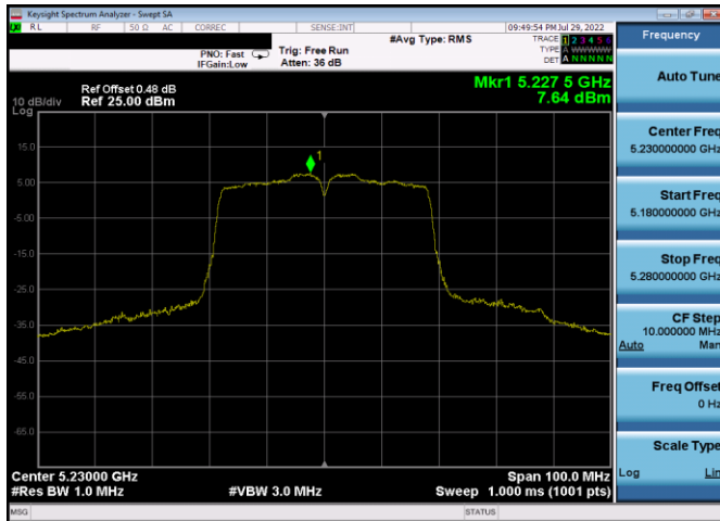
Plot 7-237. PSD Antenna 3c (40MHz BW 802.11n – Ch. 46, MCS4)
