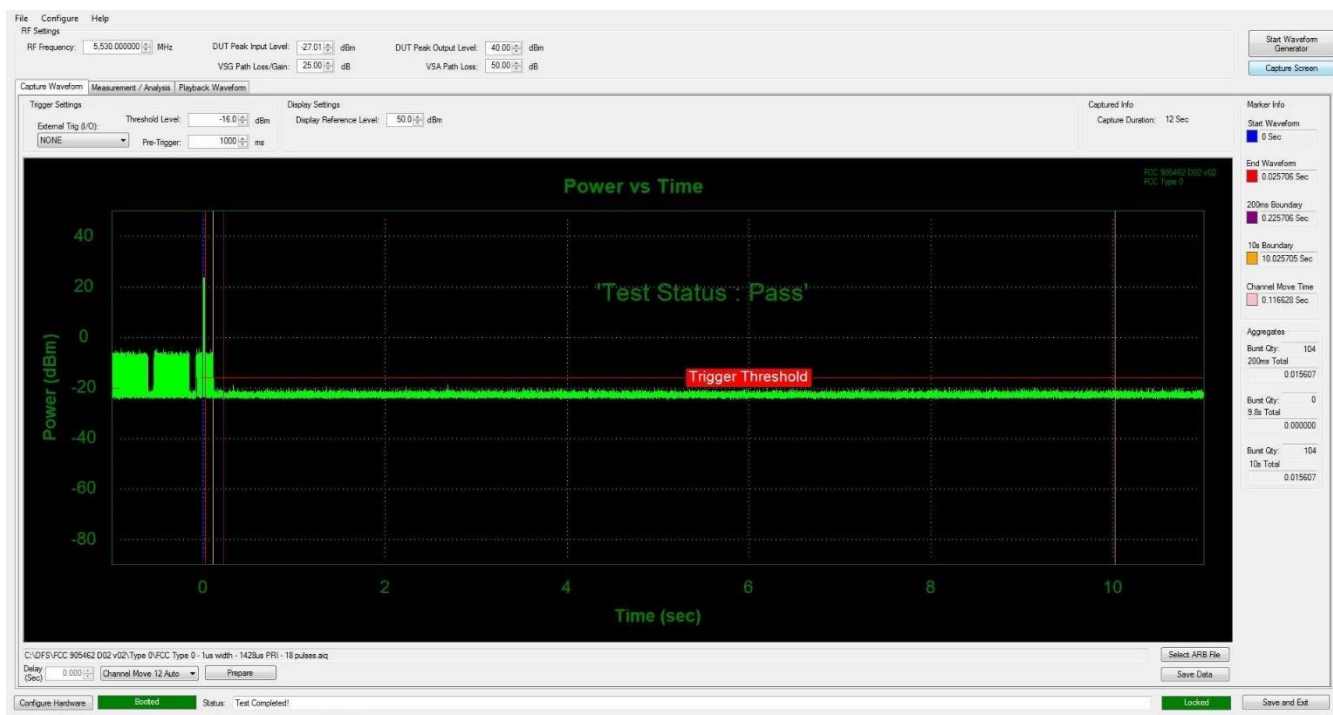
Figure 9-12. 5530MHz - Channel Move/ Closing Transmission Time - Mode 4 (80 MHz)
