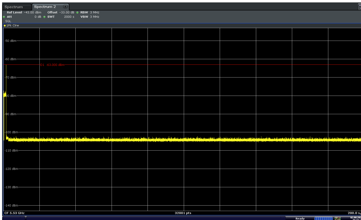
Figure 9-13. 5530MHz - Non-Occupancy Period (30 Minutes) - Mode 1 (80MHz)
