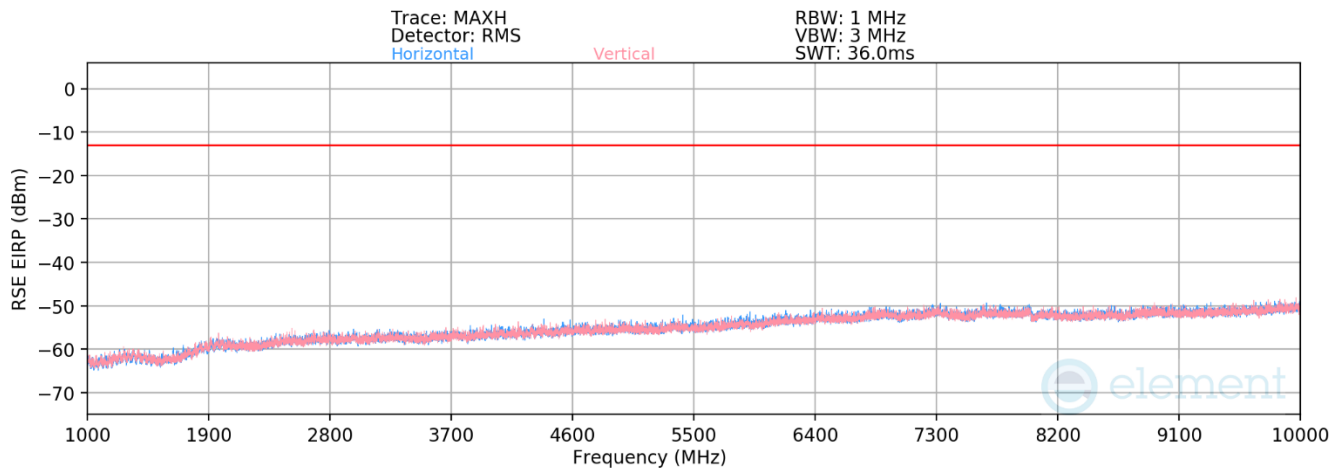
Plot 7-59. Antenna 4 Radiated Spurious Plot above 1GHz (LTE Band 26)
