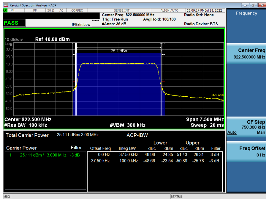
Plot 7-46. Channel Edge Plot (LTE Band 26 - 3MHz QPSK - High Channel)
