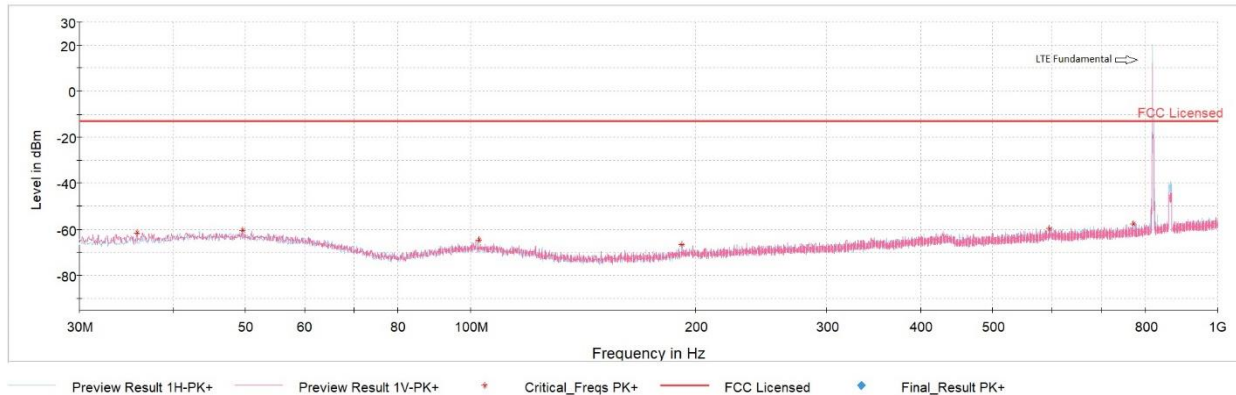
Plot 7-58. Antenna 4 Radiated Spurious Plot below 1GHz (LTE Band 26)
