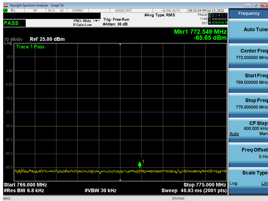
Plot 7-55. Lower Emission Mask Plot (LTE Band 14, 10MHz QPSK - RB Size 50)
