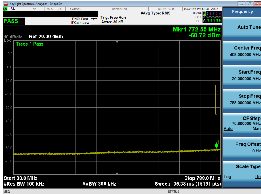
Plot 7-40. Conducted Spurious Plot (LTE Band 14 - 5MHz QPSK - RB Size 1, RB Offset 0 - High Channel)
