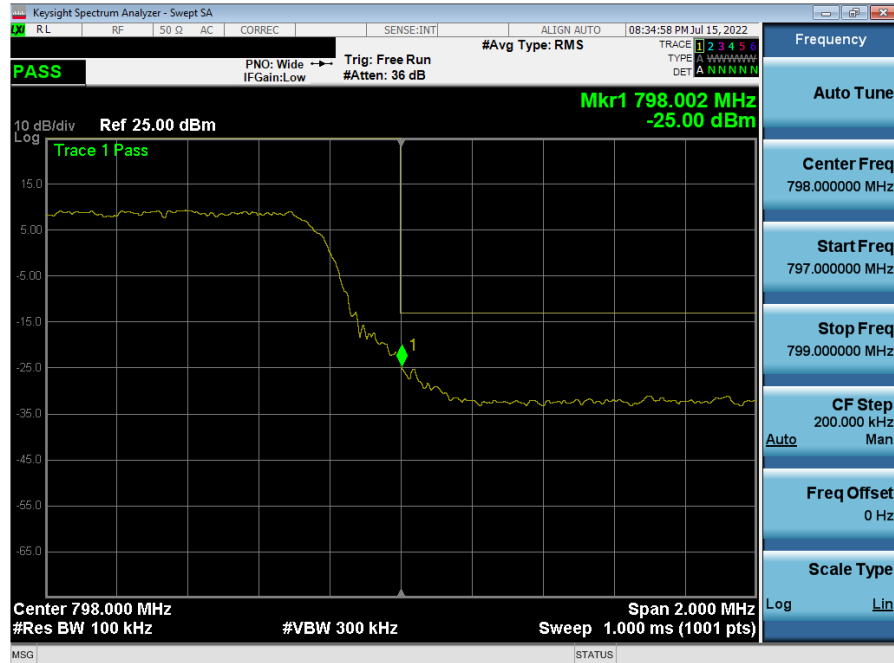
Plot 7-52. Upper Band Edge Plot (LTE Band 14, 5MHz QPSK - RB Size 25)
