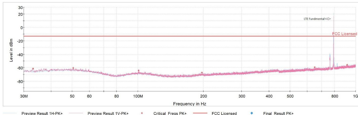
Plot 7-60. Antenna 4 Radiated Spurious Plot below 1GHz (LTE Band 14)
