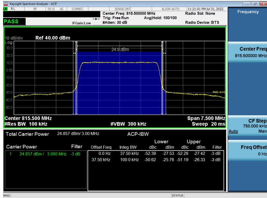
Plot 7-45. Channel Edge Plot (LTE Band 26 - 3MHz QPSK - Low Channel)
