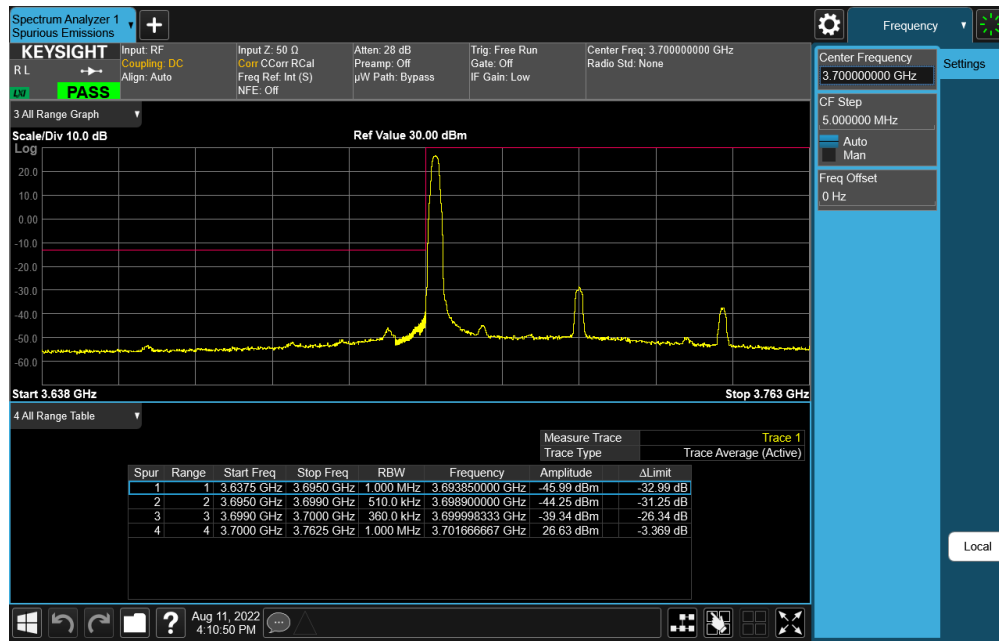
Plot 7-133. Lower ACP Plot (NR Band n77 - 50MHz DFT-s-OFDM \pi/2 BPSK - 1RB)
