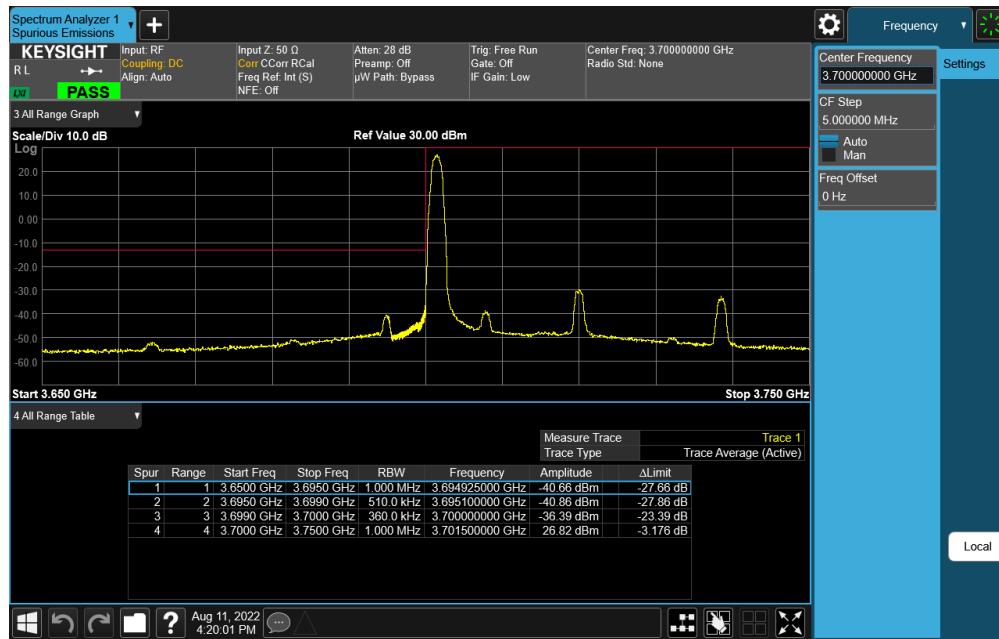
Plot 7-131. Lower ACP Plot (NR Band n77 - 40MHz DFT-s-OFDM QPSK – 1RB)
