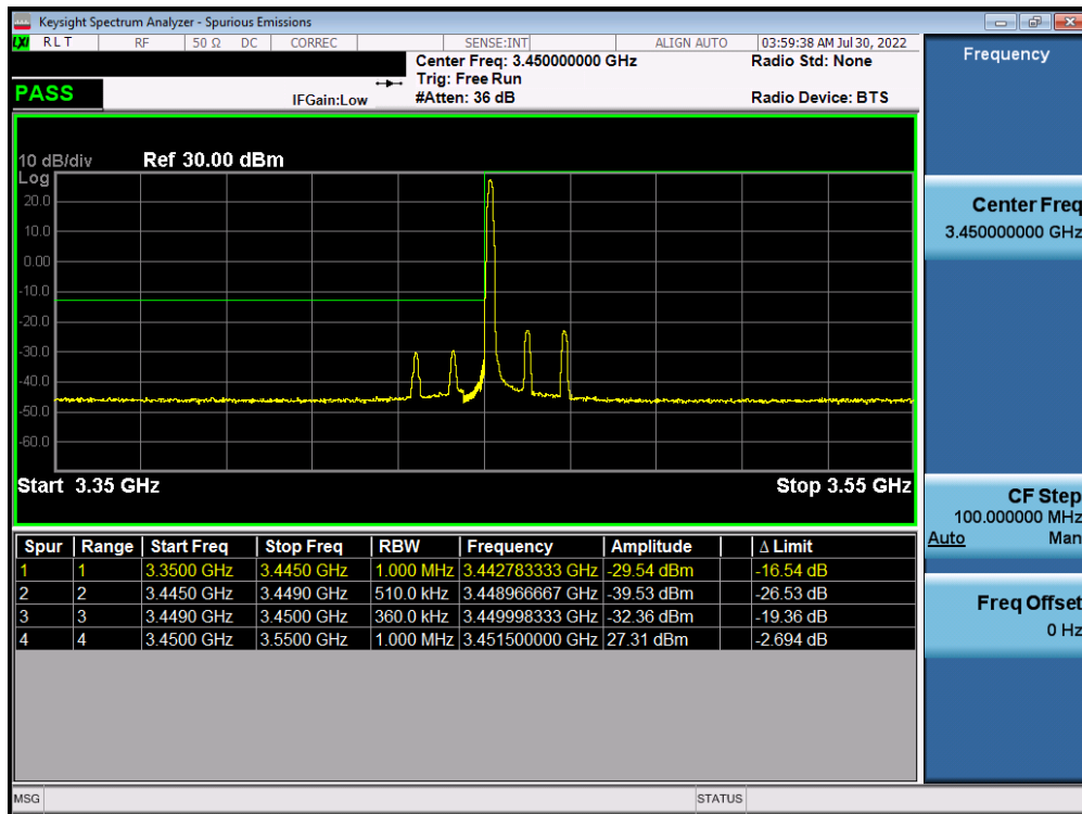
Plot 7-109. Lower ACP Plot (NR Band n77 - 20MHz DFT-s-OFDM \pi/2 BPSK – 1RB)
