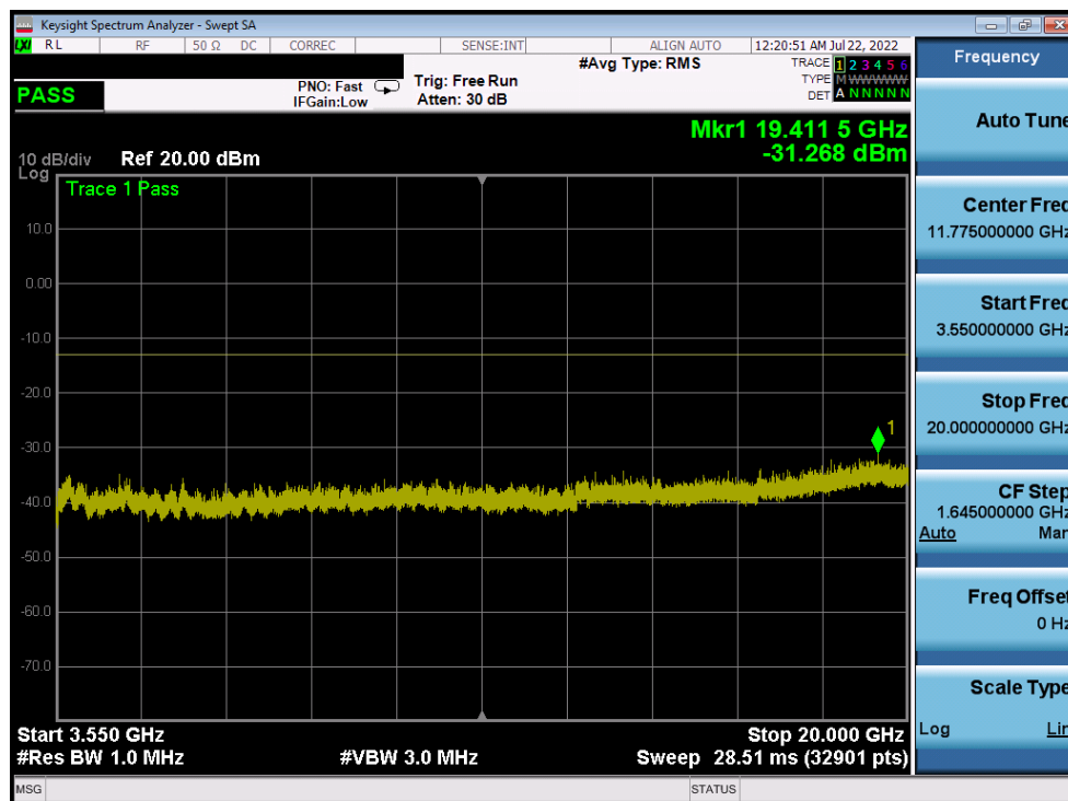
Plot 7-98. Conducted Spurious Plot (NR Band n77 DoD Band - 90MHz DFT-s-OFDM QPSK - RB Size 1, RB Offset 0 - High Channel)
