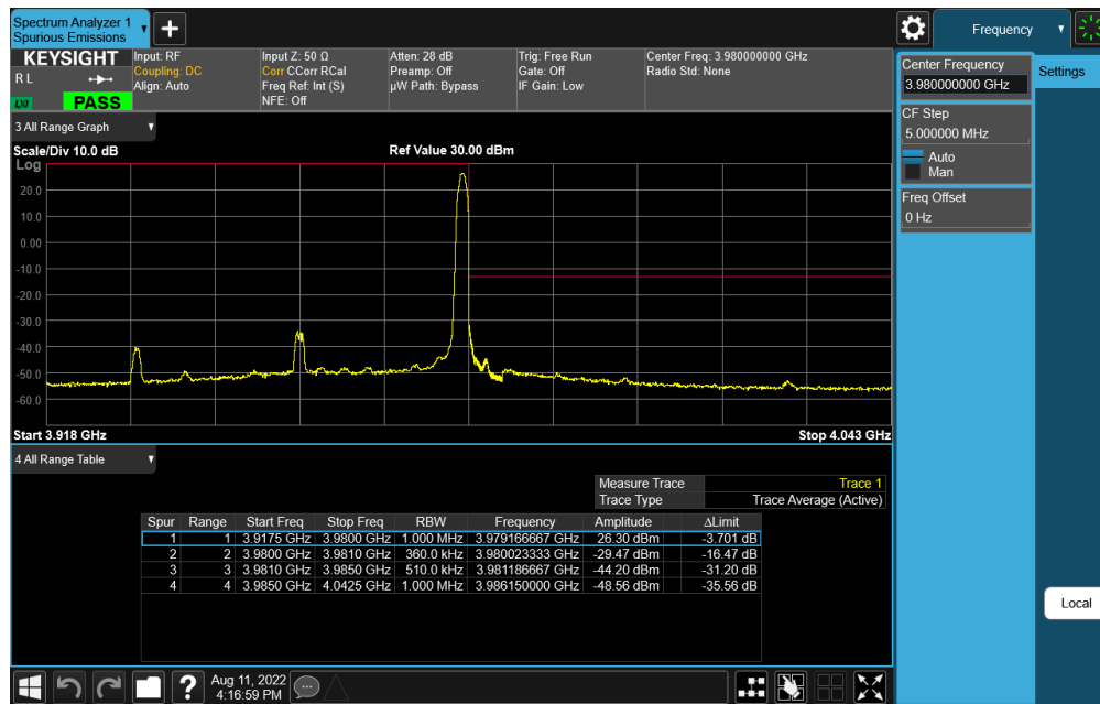
Plot 7-134. Upper ACP Plot (NR Band n77 - 50MHz DFT-s-OFDM \pi/2 BPSK - 1RB)
