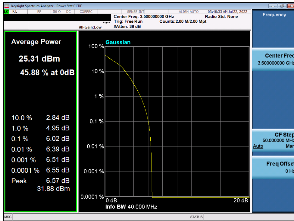
Plot 7-157. PAR Plot (NR Band n77 - 40MHz DFT-s-OFDM 16-QAM - Full RB)
