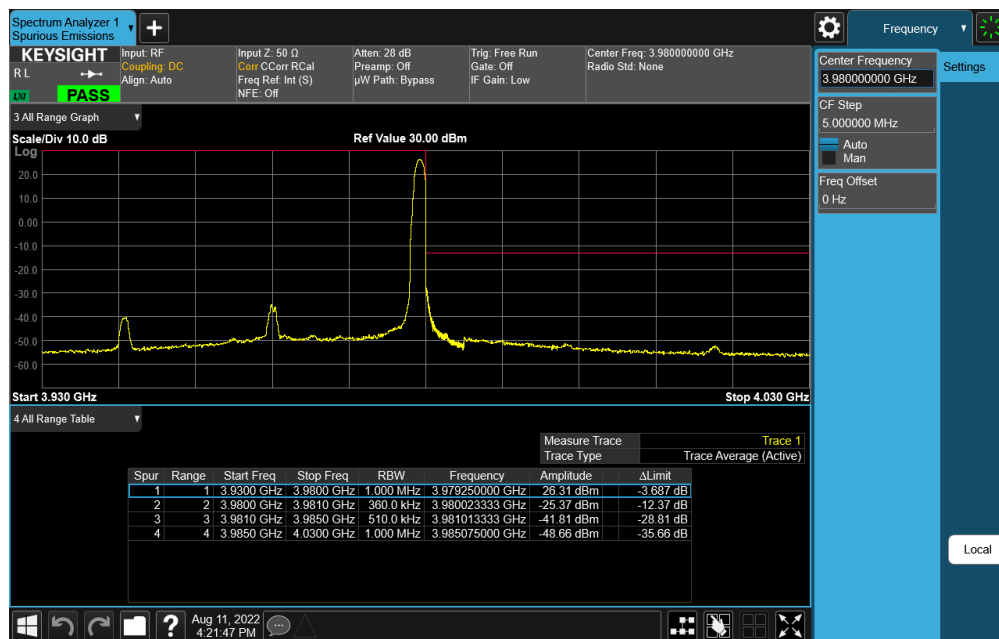
Plot 7-132. Upper ACP Plot (NR Band n77 - 40MHz DFT-s-OFDM \pi/2 BPSK – 1RB)
