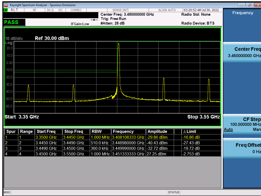
Plot 7-123. Lower ACP Plot (NR Band n77 - 90MHz DFT-s-OFDM \pi/2 BPSK - 1RB)
