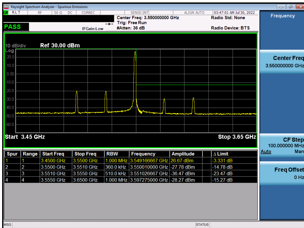
Plot 7-116. Upper ACP Plot (NR Band n77 - 50MHz DFT-s-OFDM \pi/2 BPSK - 1RB)
