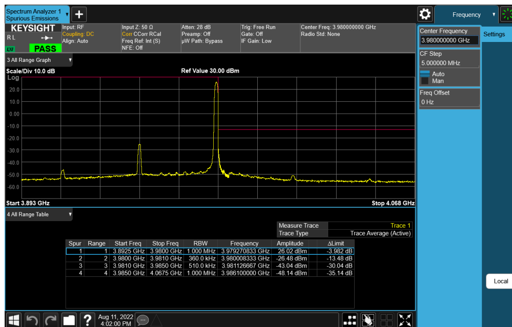
Plot 7-138. Upper ACP Plot (NR Band n77 - 70MHz DFT-s-OFDM \pi/2 BPSK – 1RB)
