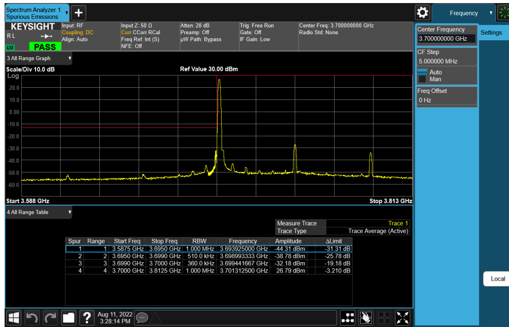
Plot 7-141. Lower ACP Plot (NR Band n77 - 90MHz DFT-s-OFDM \pi/2 BPSK - 1RB)
