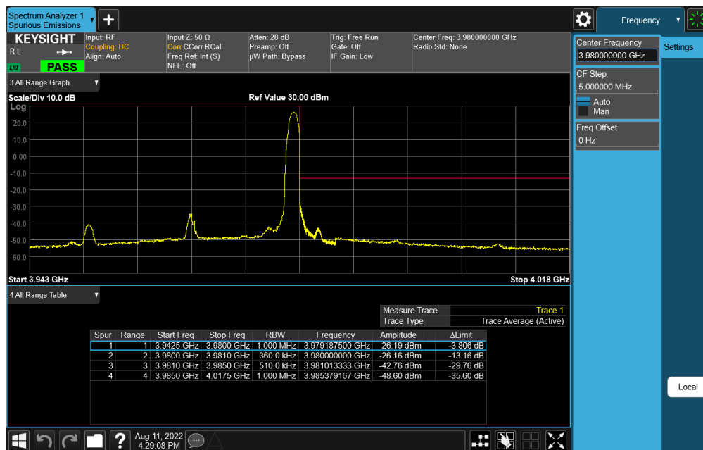
Plot 7-130. Upper ACP Plot (NR Band n77 - 30MHz DFT-s-OFDM \pi/2 BPSK – 1RB)
