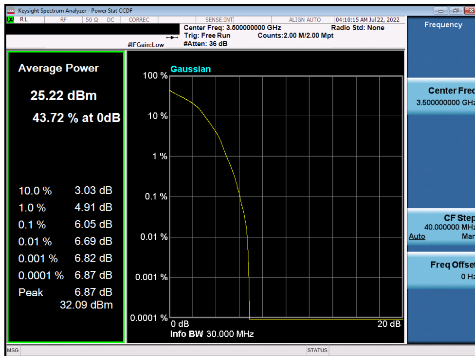
Plot 7-152. PAR Plot (NR Band n77 - 30MHz DFT-s-OFDM 16-QAM - Full RB)
