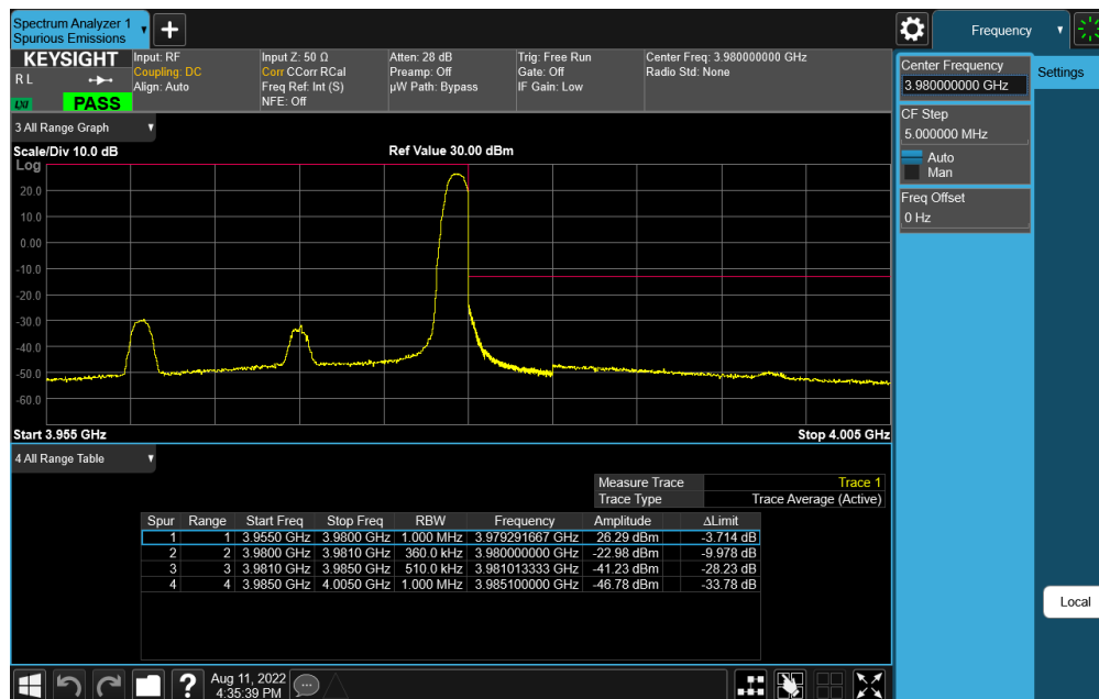
Plot 7-128. Upper ACP Plot (NR Band n77 - 20MHz DFT-s-OFDM \pi/2 BPSK – 1RB)
