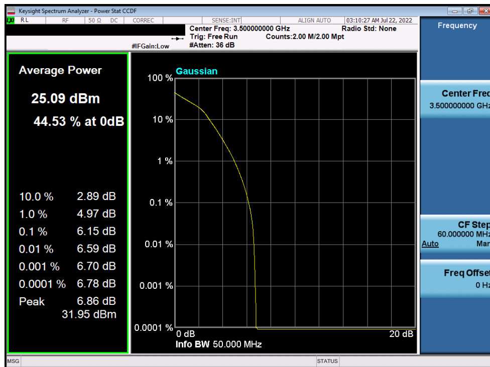
Plot 7-162. PAR Plot (NR Band n77 - 50MHz DFT-s-OFDM 16-QAM - Full RB)
