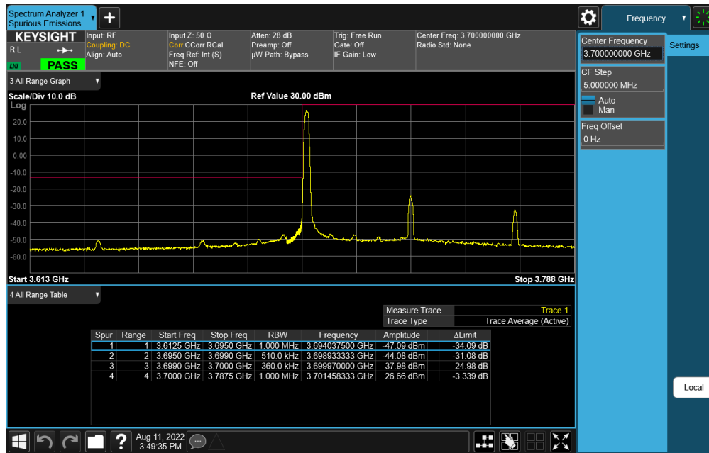
Plot 7-137. Lower ACP Plot (NR Band n77 - 70MHz DFT-s-OFDM QPSK – 1RB)
