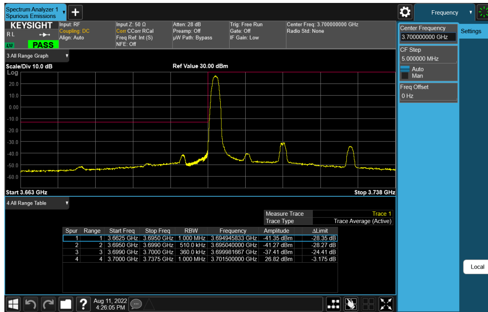
Plot 7-129. Lower ACP Plot (NR Band n77 - 30MHz DFT-s-OFDM QPSK – 1RB)
