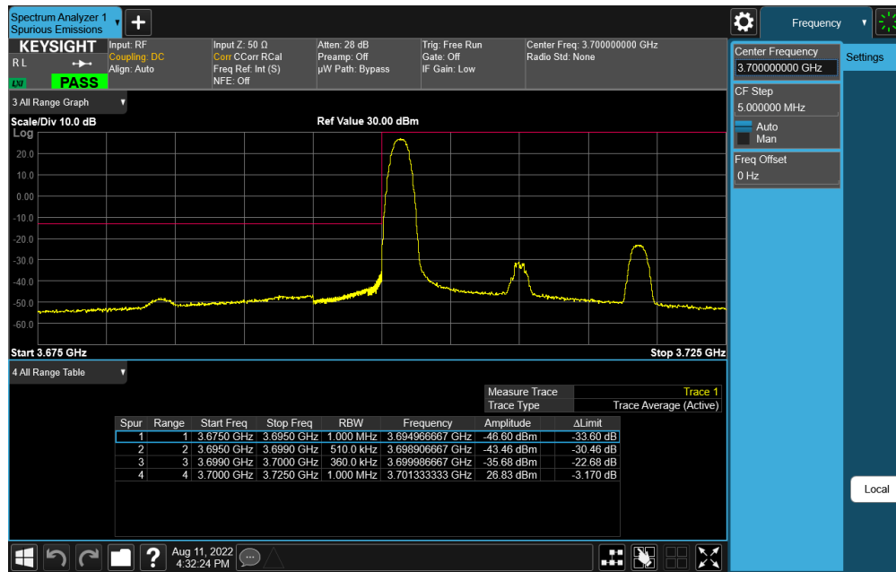
Plot 7-127. Lower ACP Plot (NR Band n77 - 20MHz DFT-s-OFDM \pi/2 BPSK – 1RB)
