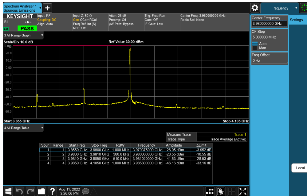
Plot 7-144. Upper ACP Plot (NR Band n77 - 100MHz DFT-s-OFDM \pi/2 BPSK – 1RB)
