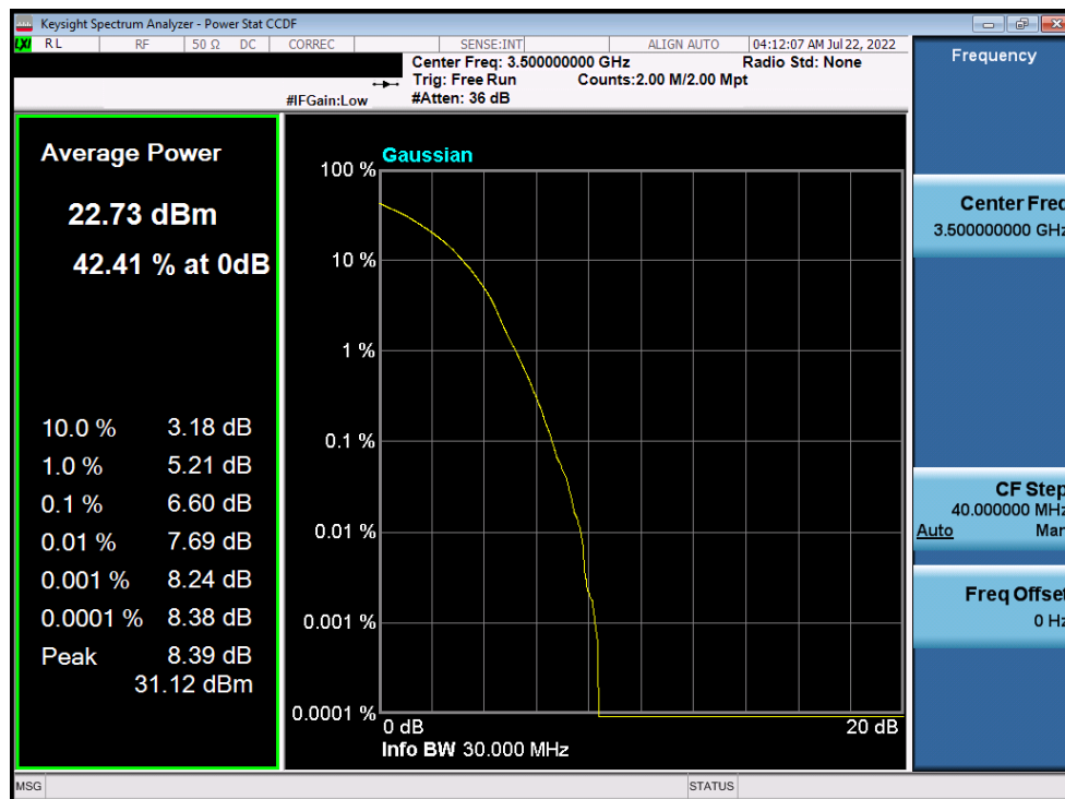
Plot 7-154. PAR Plot (NR Band n77 - 30MHz DFT-s-OFDM 256-QAM - Full RB)
