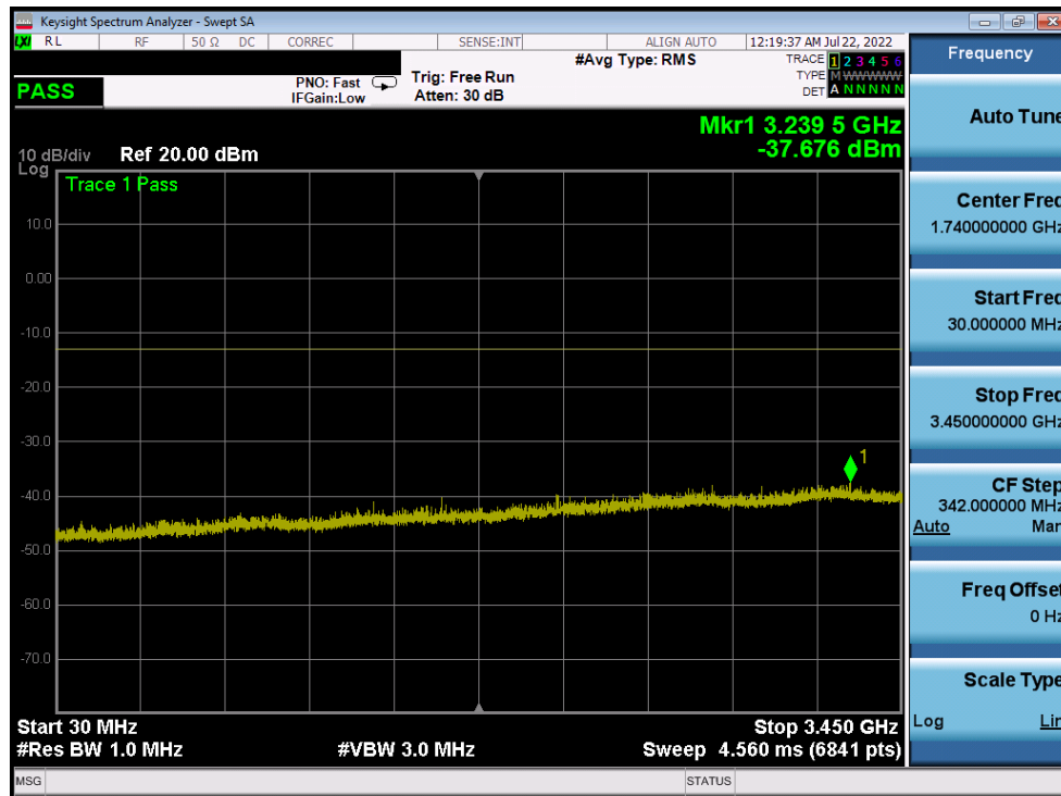
Plot 7-97. Conducted Spurious Plot (NR Band n77 DoD Band - 90MHz DFT-s-OFDM QPSK - RB Size 1, RB Offset 0 - High Channel)
