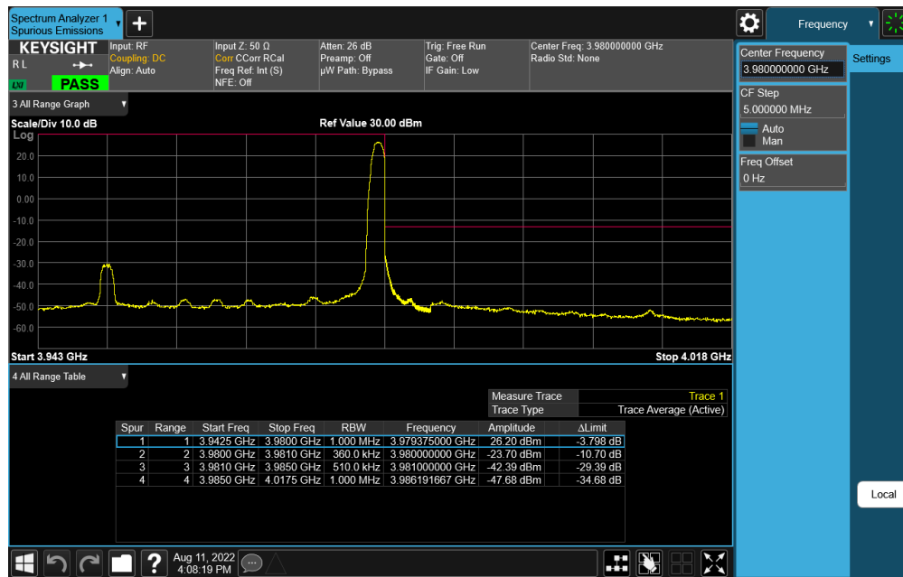
Plot 7-136. Upper ACP Plot (NR Band n77 - 60MHz DFT-s-OFDM \pi/2 BPSK - 1RB)
