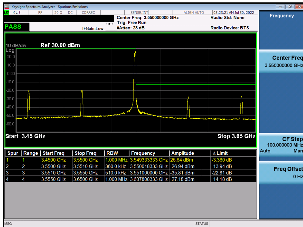
Plot 7-124. Upper ACP Plot (NR Band n77 - 90MHz DFT-s-OFDM \pi/2 BPSK - 1RB)
