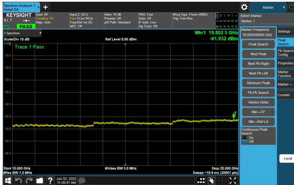
Plot 7-72. Conducted Spurious Plot (NR Band n25 - 40.0MHz - RB Size 1, RB Offset 0 - Low Channel)
