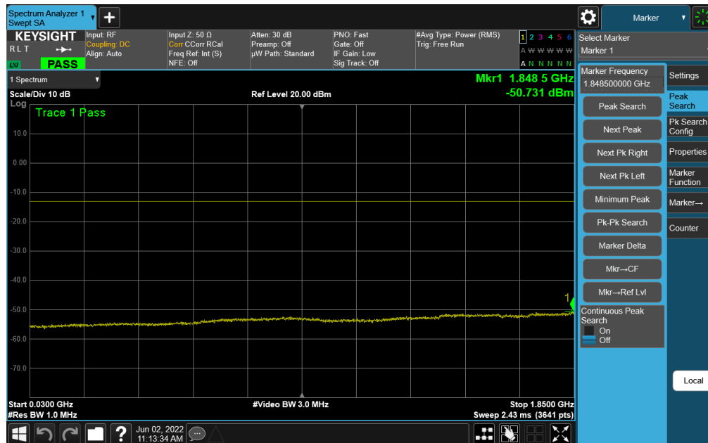
Plot 7-76. Conducted Spurious Plot (NR Band n25 - 40.0MHz - RB Size 1, RB Offset 0 - High Channel)
