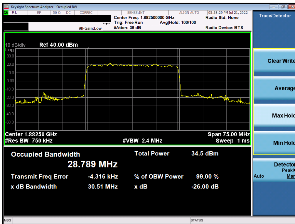
Plot 7-50. Occupied Bandwidth Plot (NR Band n25 - 30.0MHz DFT-s-OFDM \pi/2 BPSK - Full RB)
