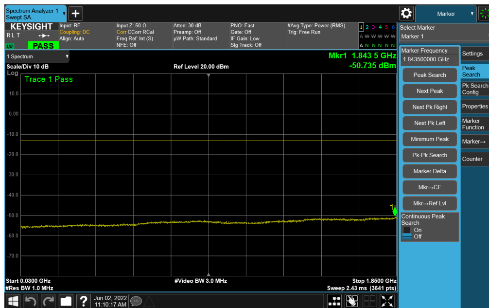
Plot 7-73. Conducted Spurious Plot (NR Band n25 - 40.0MHz - RB Size 1, RB Offset 0 - Mid Channel)
