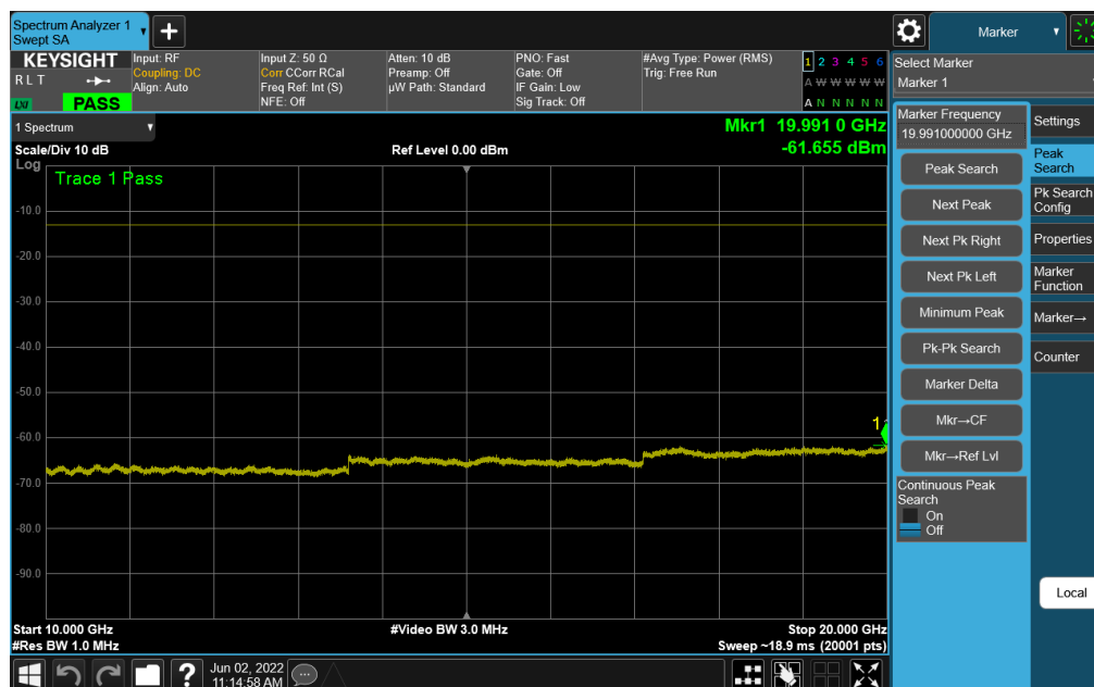
Plot 7-78. Conducted Spurious Plot (NR Band n25 - 40.0MHz - RB Size 1, RB Offset 0 - High Channel)
