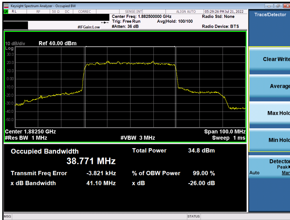
Plot 7-55. Occupied Bandwidth Plot (NR Band n25 - 40.0MHz DFT-s-OFDM \pi/2 BPSK - Full RB)
