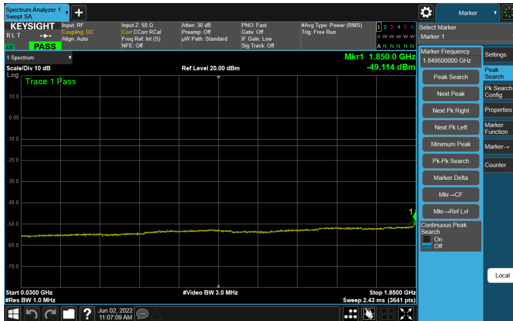
Plot 7-70. Conducted Spurious Plot (NR Band n25 - 40.0MHz - RB Size 1, RB Offset 0 - Low Channel)
