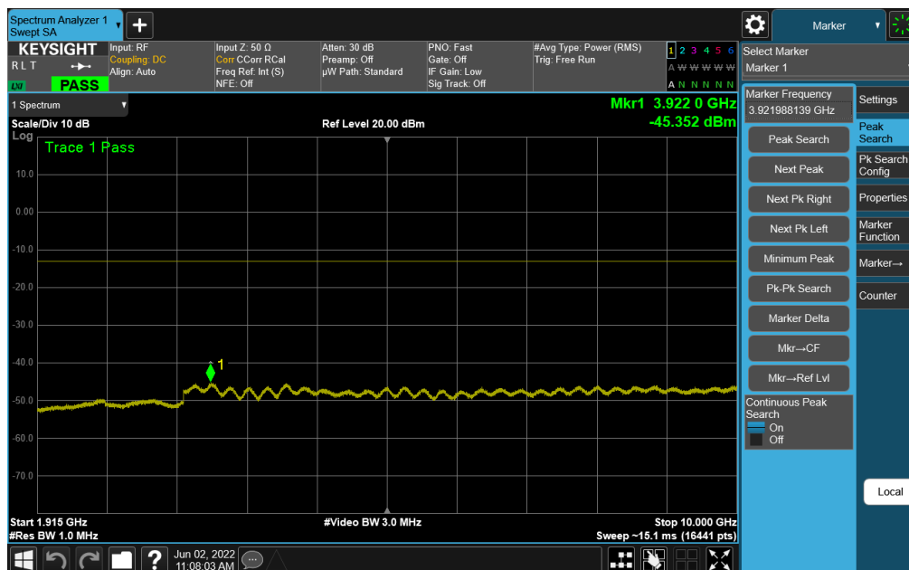
Plot 7-71. Conducted Spurious Plot (NR Band n25 - 40.0MHz - RB Size 1, RB Offset 0 - Low Channel)
