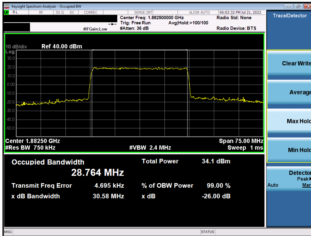
Plot 7-52. Occupied Bandwidth Plot (NR Band n25 - 30.0MHz CP-OFDM 16QAM - Full RB)
