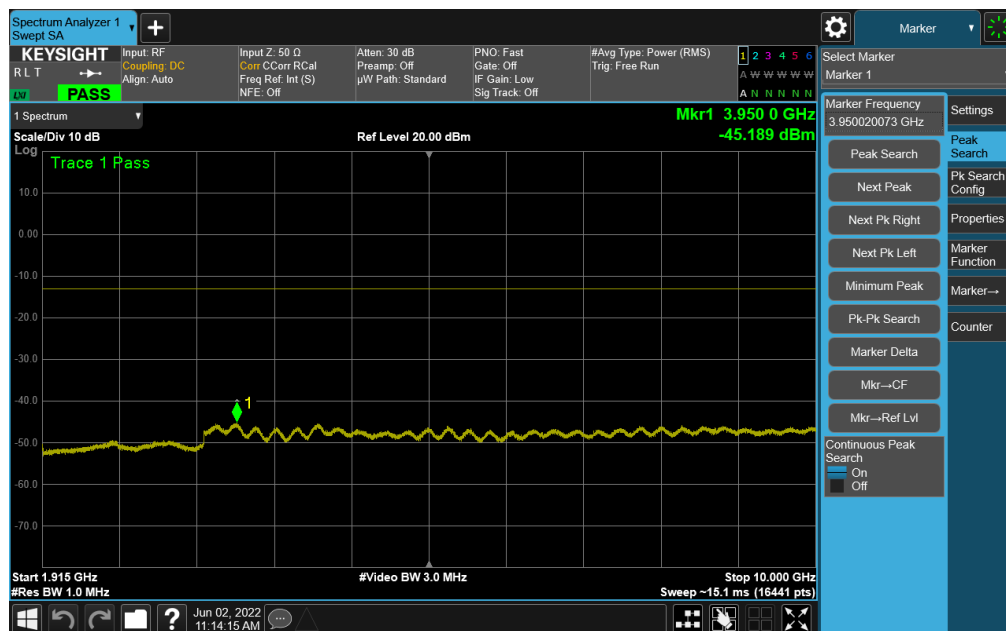
Plot 7-77. Conducted Spurious Plot (NR Band n25 - 40.0MHz - RB Size 1, RB Offset 0 - High Channel)
