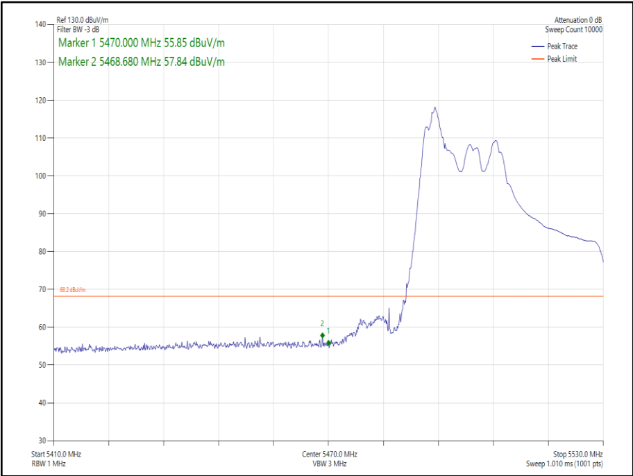
Figure 218 - 802. 11ax HE40 SDM, Cores 0-1, 26-0 - 5510 MHz Band Edge Frequency 5470 MHz
