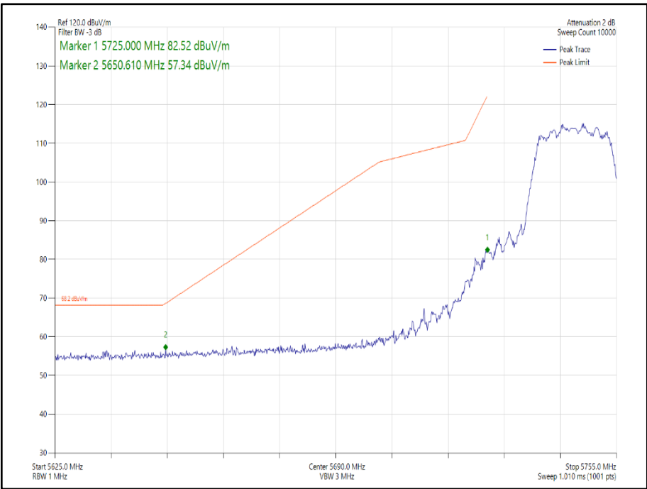
Figure 189 - 802.11n HT20 CDD, Cores 0-1 - 5745 MHz Band Edge Frequency 5725 MHz
