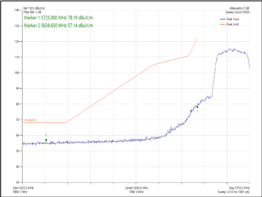
Figure 190 - 802.11n HT20 SDM, Cores 0-1 - 5745 MHz Band Edge Frequency 5725 MHz
