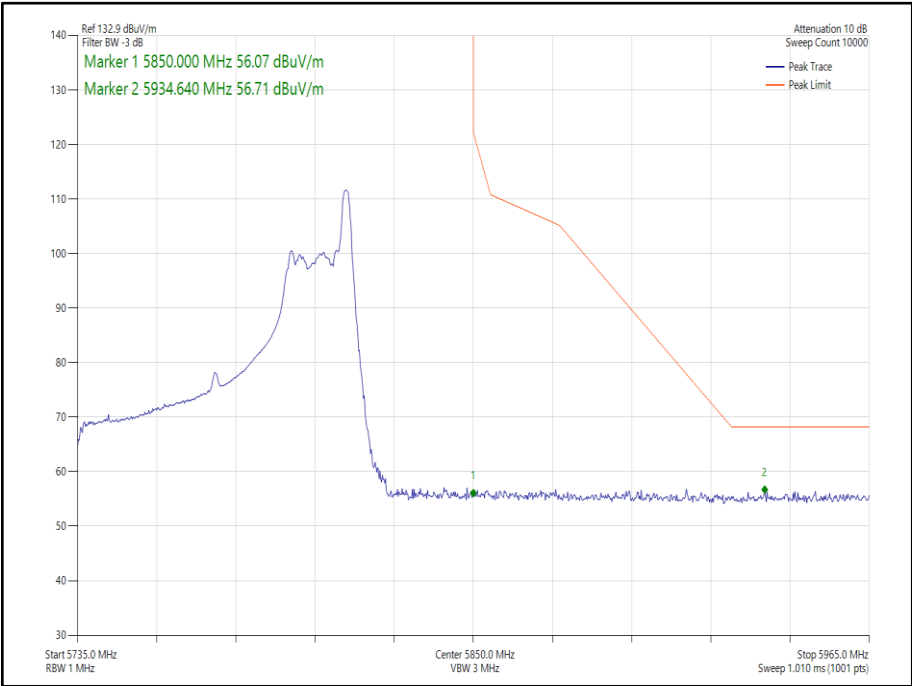
Figure 248 - 802.11ax HE80 Core 1 26-36 - 5775 MHz Band Edge Frequency 5850 MHz
