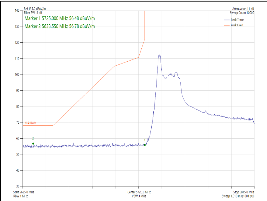
Figure 245 - 802.11ax HE80 Core 1 26-0 - 5775 MHz Band Edge Frequency 5725 MHz
