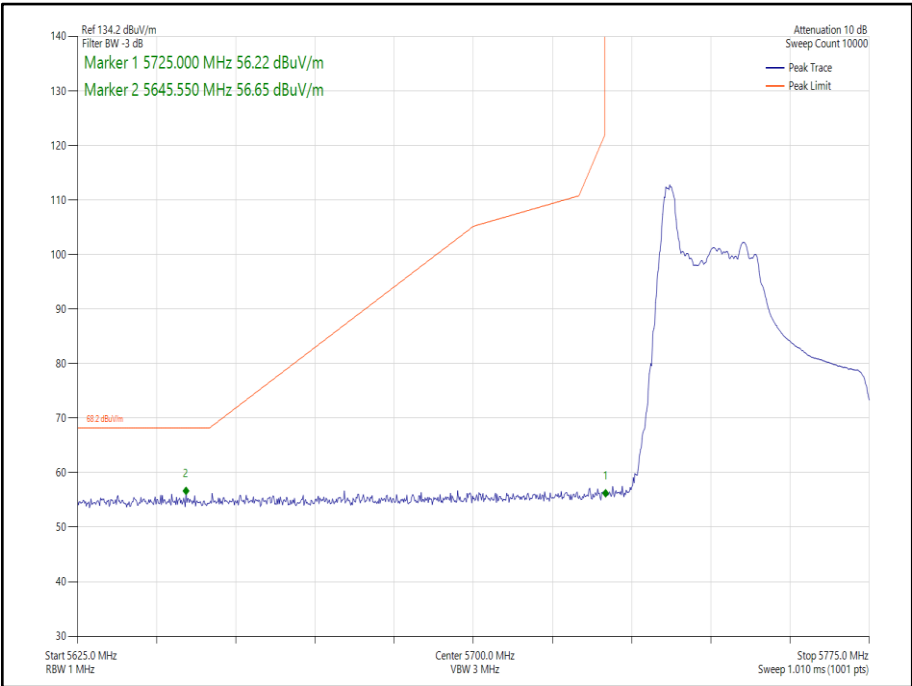
Figure 209 - 802.11ax HE40, Core 1, 26-0 - 5755 MHz Band Edge Frequency 5725 MHz
