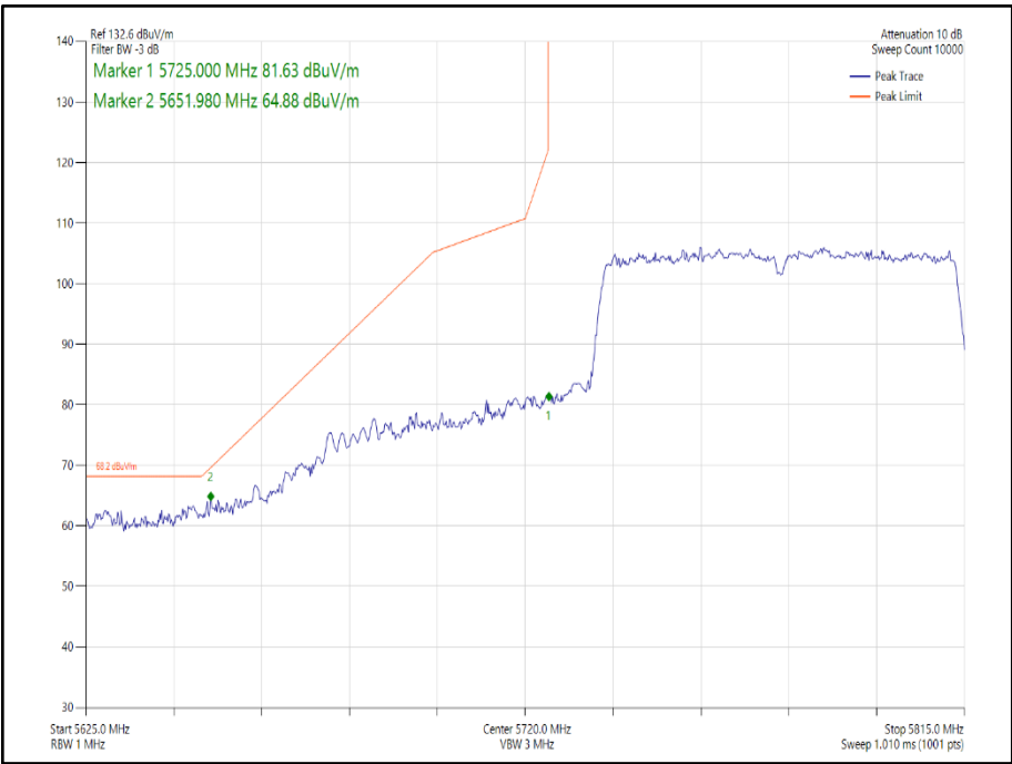
Figure 243 - 802.11ac VHT80 Core 1 - 5775 MHz Band Edge Frequency 5725 MHz
