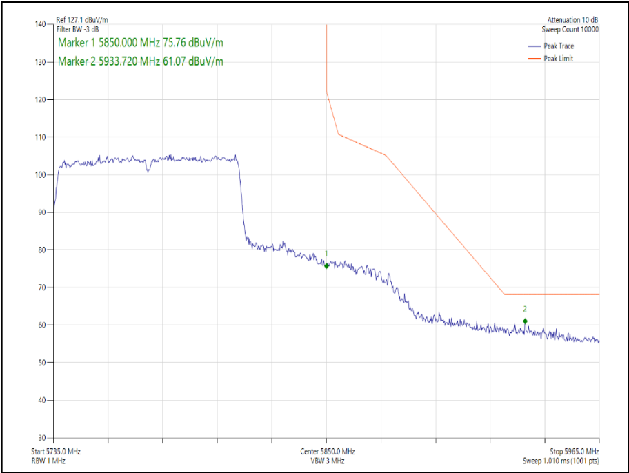
Figure 246 - 802.11ac VHT80 Core 1 - 5775 MHz Band Edge Frequency 5850 MHz
