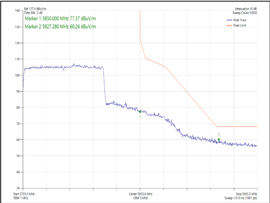
Figure 247 - 802.11ax HE80 Core 1 SU - 5775 MHz Band Edge Frequency 5850 MHz
