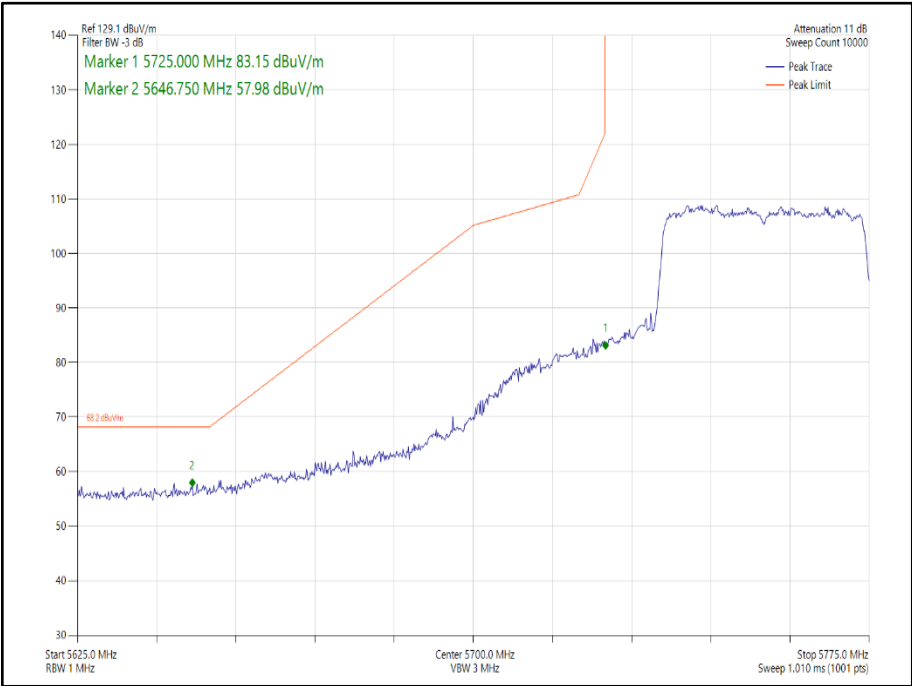
Figure 208 - 802.11ax HE40, Core 1, SU - 5755 MHz Band Edge Frequency 5725 MHz
