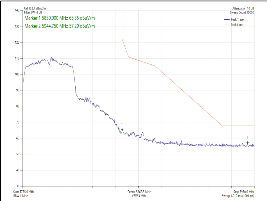
Figure 210 - 802.11n HT40, Core 1 - 5795 MHz Band Edge Frequency 5850 MHz
