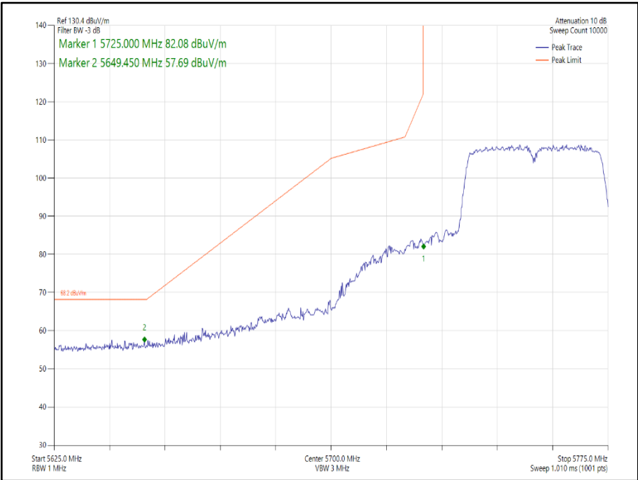
Figure 207 - 802.11n HT40, Core 1 - 5755 MHz Band Edge Frequency 5725 MHz
