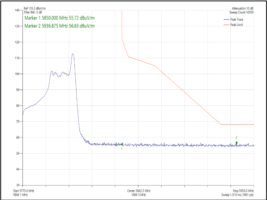
Figure 212 - 802.11ax HE40, Core 1, 26-17 - 5795 MHz Band Edge Frequency 5850 MHz
