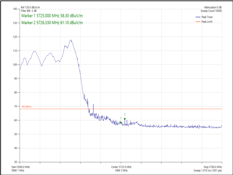
Figure 188 - 802.11ax HE20 SDM, Cores 0-1, 52-40 - 5700 MHz Band Edge Frequency 5725 MHz
