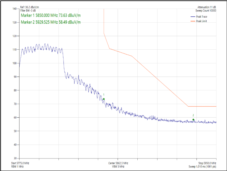
Figure 233 - 802.11ax HE40 CDD, Cores 0-1, SU - 5795 MHz Band Edge Frequency 5850 MHz
