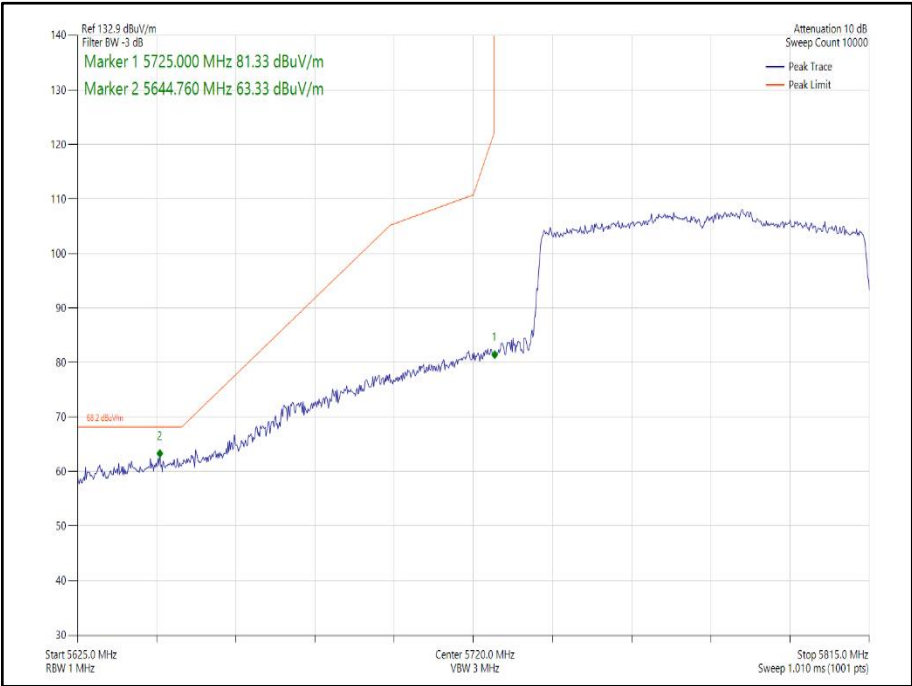
Figure 244 - 802.11ax HE80 Core 1 SU - 5775 MHz Band Edge Frequency 5725 MHz
