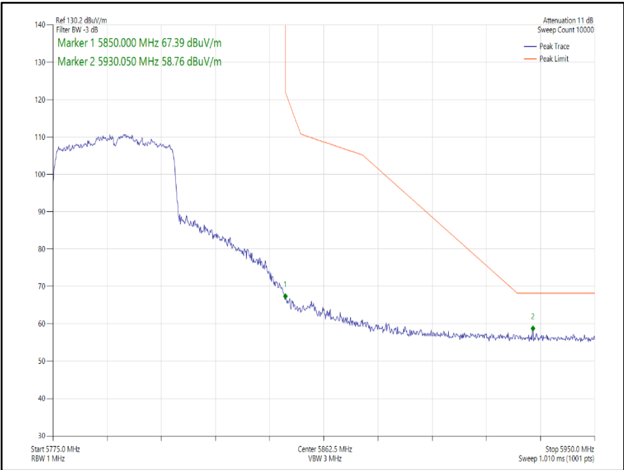
Figure 211 - 802.11ax HE40, Core 1, SU - 5795 MHz Band Edge Frequency 5850 MHz
