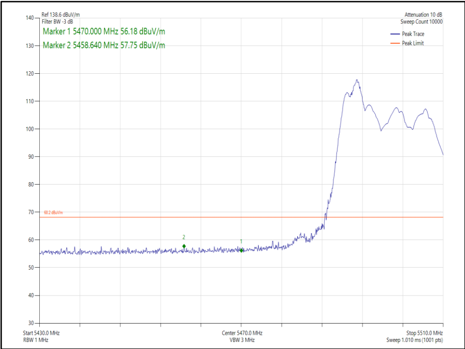
Figure 182 - 802.11ax HE20 SDM, Cores 0-1 52-37 - 5500 MHz Band Edge Frequency 5470 MHz
