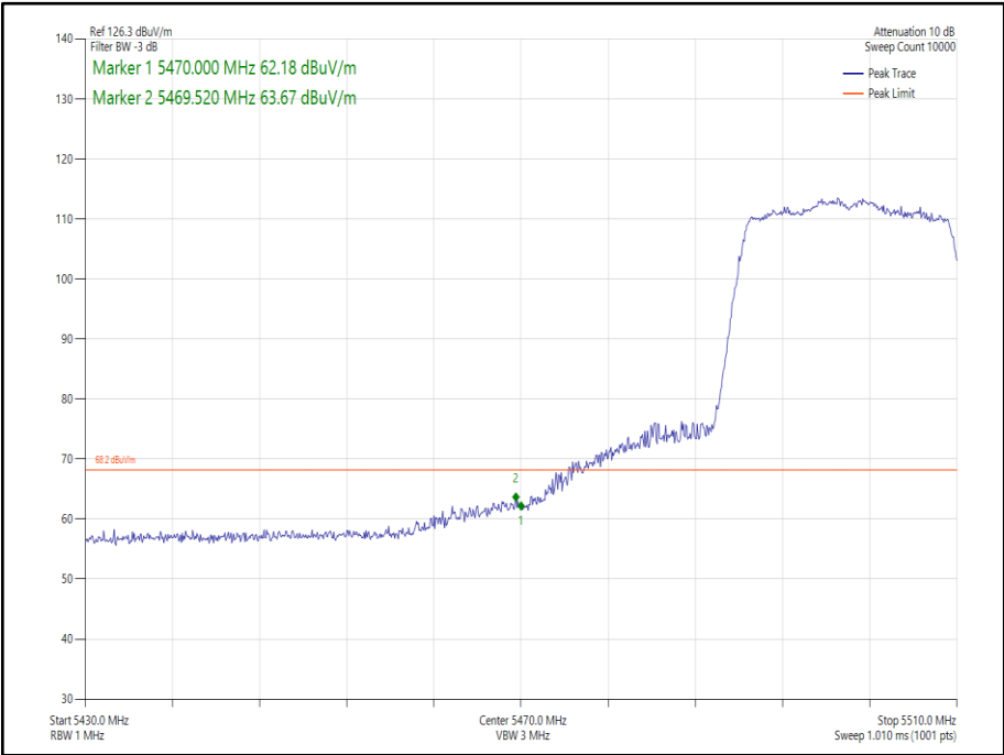
Figure 163- 802.11ax HE20, Core 1, SU - 5500 MHz Band Edge Frequency 5470 MHz
