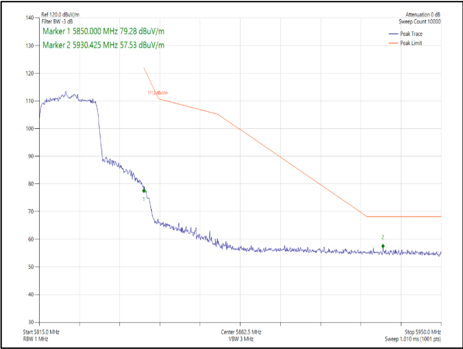
Figure 175- 802.11ax HE20, Core 1, SU - 5825 MHz Band Edge Frequency 5850 MHz
