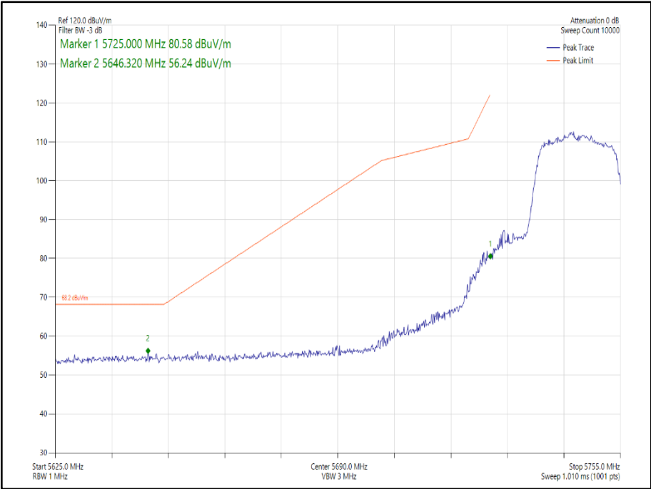
Figure 170 - 802.11n HT20, Core 1 - 5745 MHz Band Edge Frequency 5725 MHz
