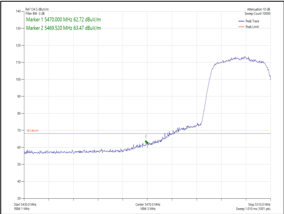
Figure 162 - 802.11n HT20, Core 1 - 5500 MHz Band Edge Frequency 5470 MHz
