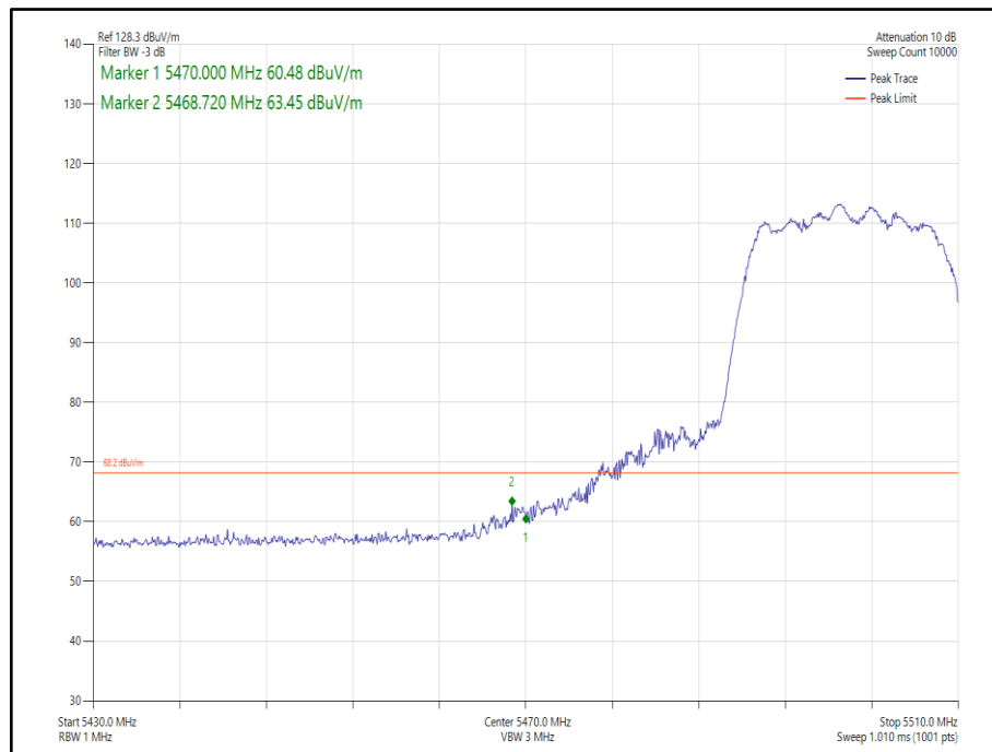
Figure 177 - 802.11n HT20 CDD, Cores 0-1 - 5500 MHz Band Edge Frequency 5470 MHz
