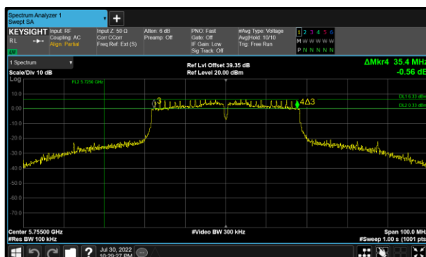
Figure 139 - 802.11n HT40 Minimum 6 dB EBW
