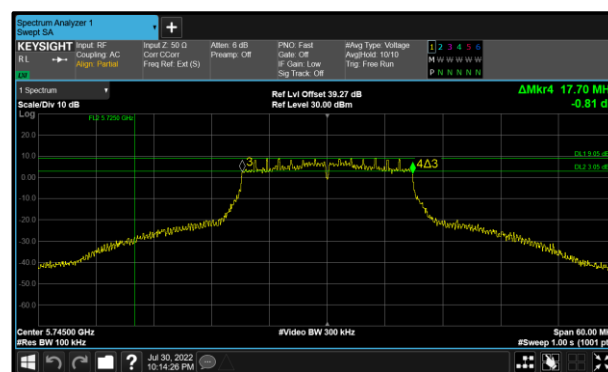
Figure 138 - 802.11n HT20 Maximum 6 dB EBW
