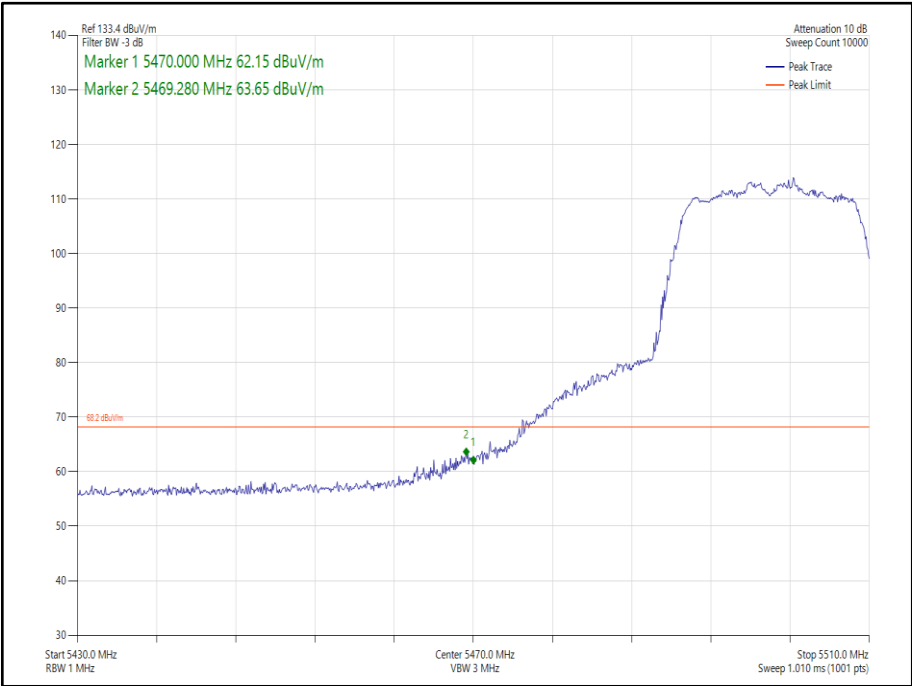
Figure 178 - 802.11n HT20 SDM, Cores 0-1 - 5500 MHz Band Edge Frequency 5470 MHz
