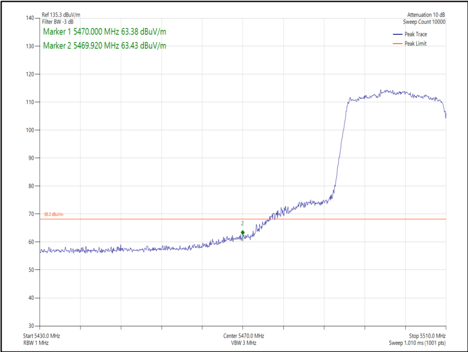
Figure 181 - - 802.11ax HE20 SDM, Cores 0-1 SU - 5500 MHz Band Edge Frequency 5470 MHz
