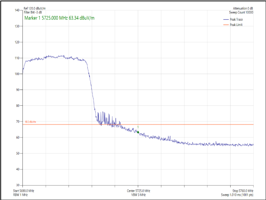
Figure 167- 802.11ax HE20, Core 1, SU - 5700 MHz Band Edge Frequency 5725 MHz
