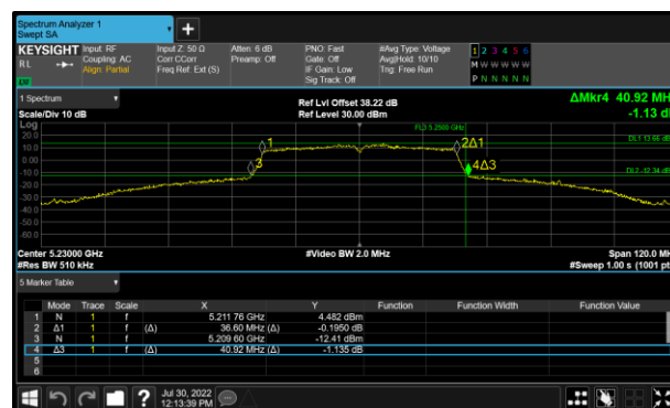
Figure 152 - 802.11n HT40 Maximum 99% OBW
