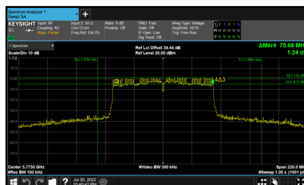
Figure 142 - 802.11ac VHT80 Maximum 6 dB EBW
