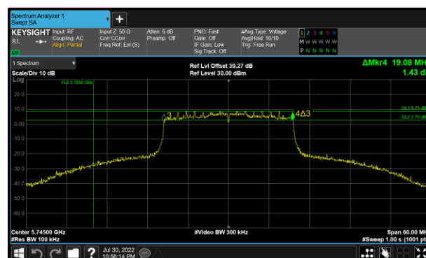
Figure 144 - 802.11ax HE20 SU Maximum 6 dB EBW
