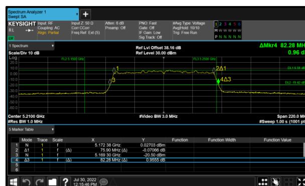
Figure 154 - 802.11ac VHT80 Maximum 99% OBW
