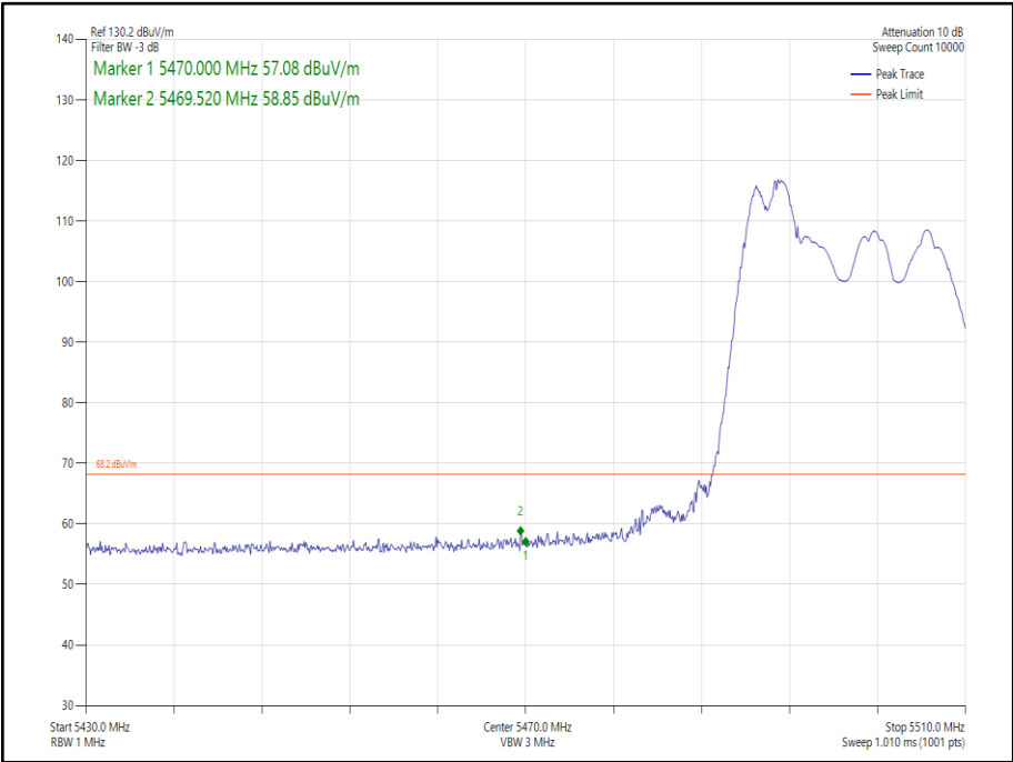
Figure 180 - 802.11ax HE20 CDD, Cores 0-1 52-37 - 5500 MHz Band Edge Frequency 5470 MHz
