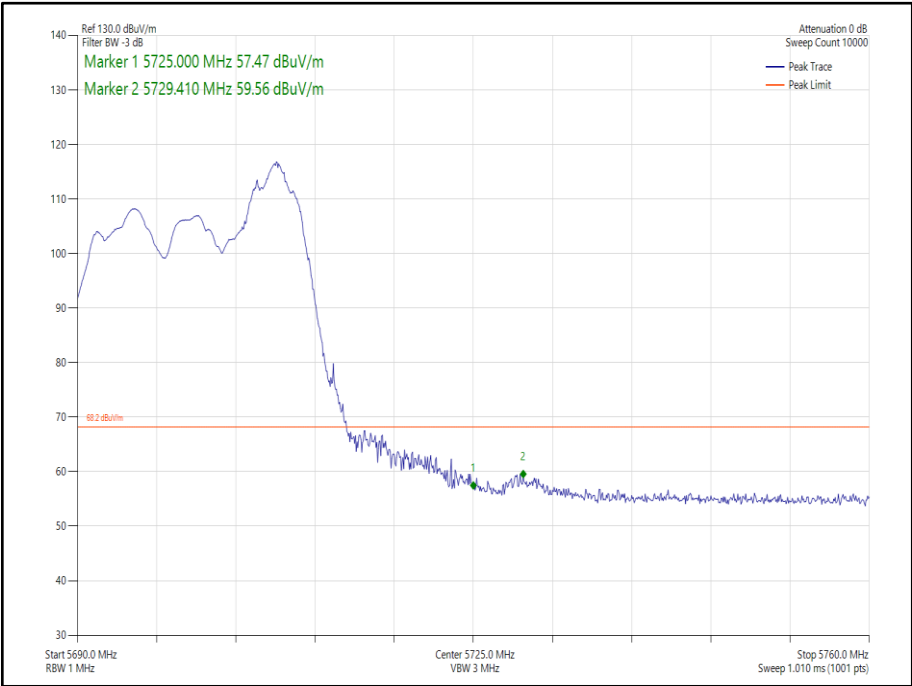
Figure 186 - 802.11ax HE20 CDD, Cores 0-1, 52-40 - 5700 MHz Band Edge Frequency 5725 MHz
