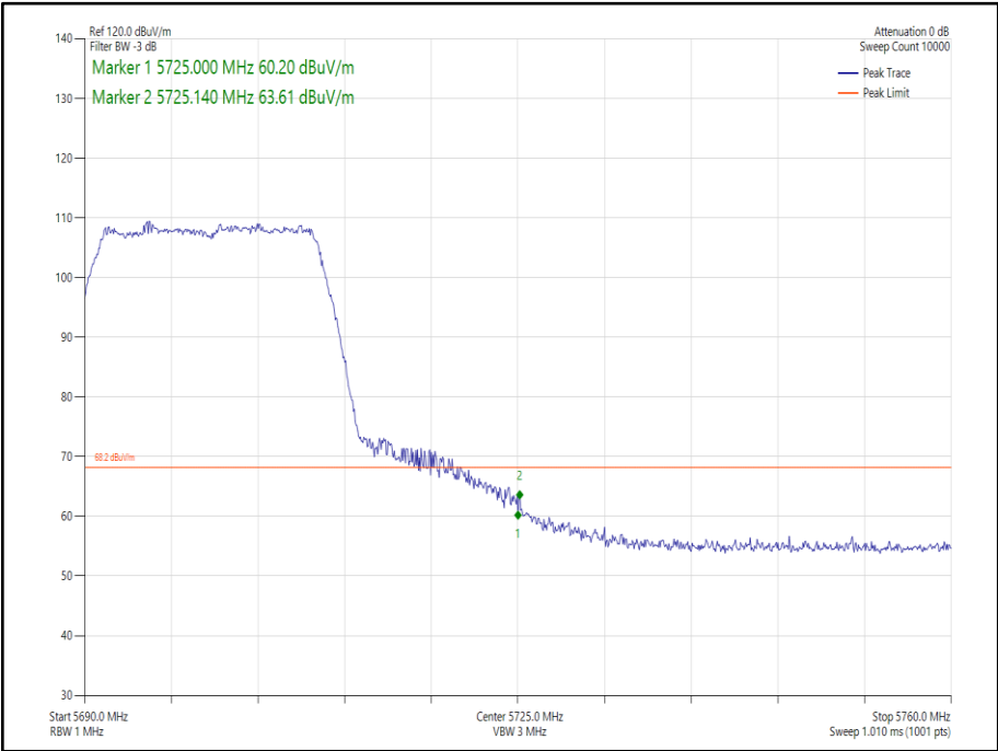
Figure 184 - 802.11n HT20 SDM, Cores 0-1 - 5700 MHz Band Edge Frequency 5725 MHz
