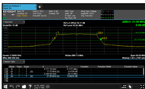
Figure 149 - 802.11n HT20 Minimum 99% OBW
