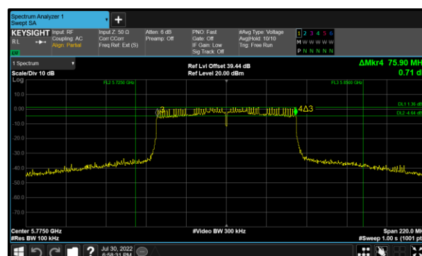
Figure 118 - 802.11ac VHT80 Maximum 6 dB EBW
