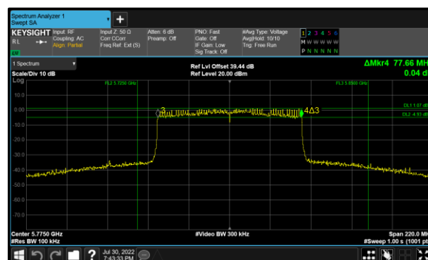
Figure 124 - 802.11ax HE80 SU Maximum 6 dB EBW
