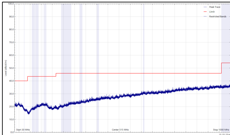
Figure 152 - 2441 MHz (CH39), DH5, ePA, Core 0 + Core 1, 30 MHz to 1 GHz, Vertical (Peak)
