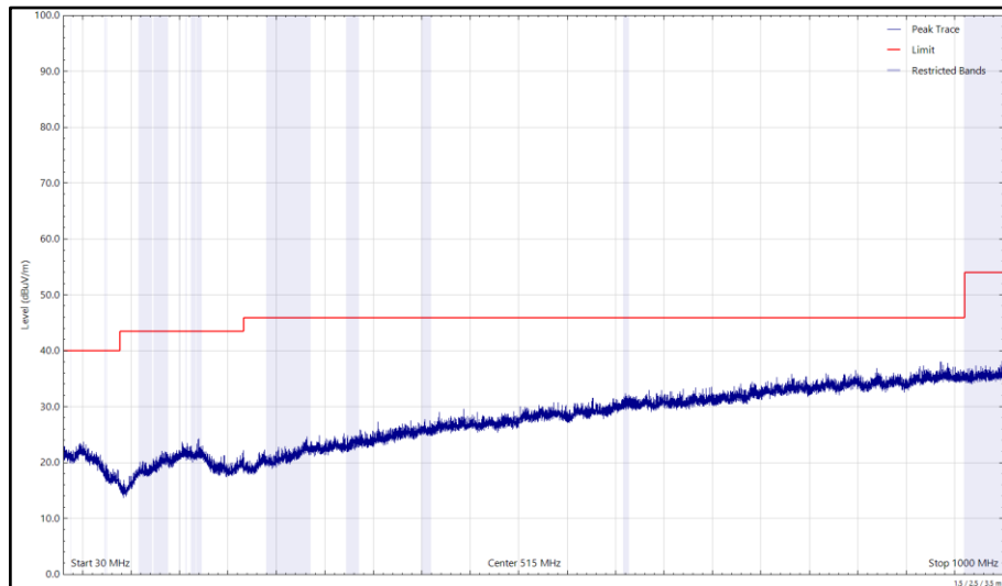
Figure 142 - 2441 MHz (CH39), DH5, iPA, Core 0 + Core 1, 30 MHz to 1 GHz, Horizontal (Peak)
