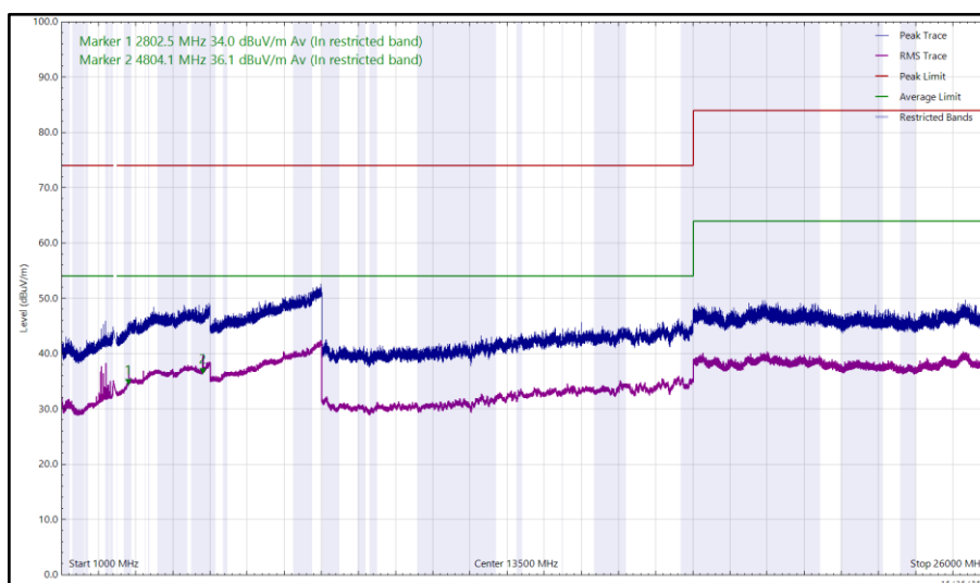
Figure 141 - 2402 MHz (CH0), DH5, iPA, Core 0 + Core 1, 1 GHz to 26 GHz, Vertical
