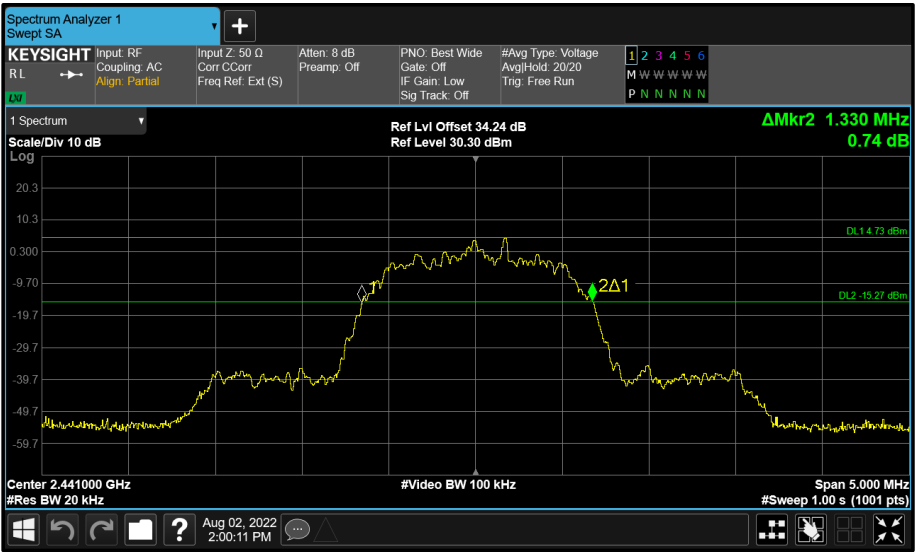
Figure 129 - BT Core 0 (A) 2441 MHz (CH39) 20 dB Bandwidth
