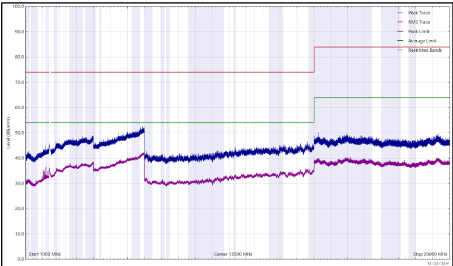
Figure 156 - 2402 MHz (CH0), DH5, iPA, Core 2, 1 GHz to 26 GHz, Horizontal
