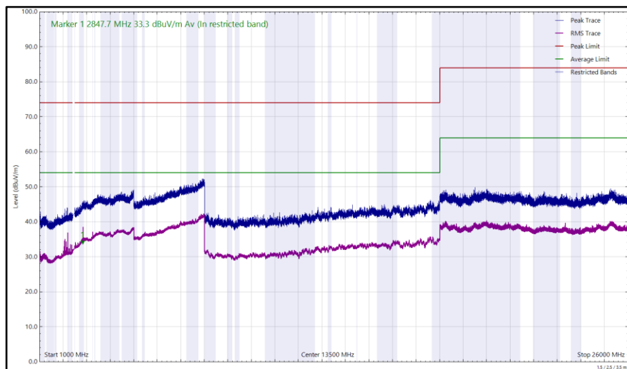
Figure 143 - 2441 MHz (CH39), DH5, iPA, Core 0 + Core 1, 1 GHz to 26 GHz, Horizontal
