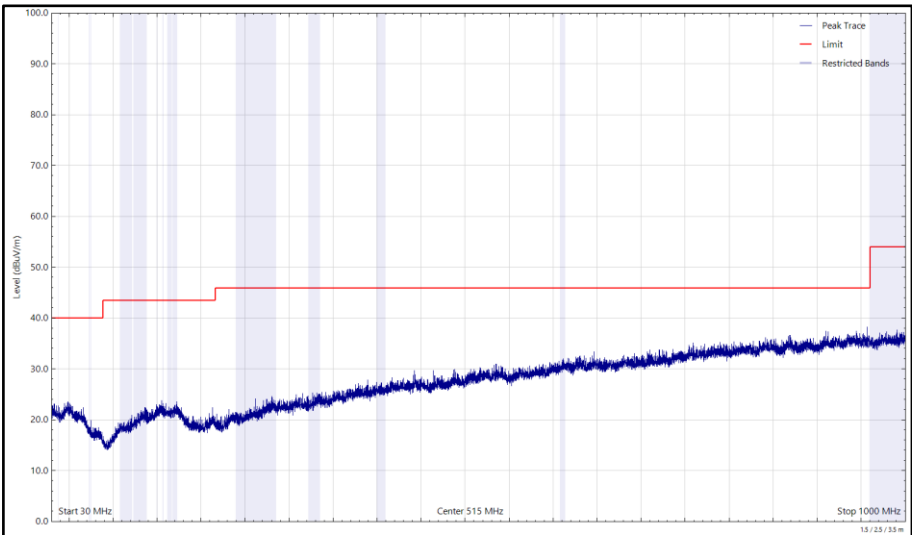
Figure 150 - 2441 MHz (CH39), DH5, ePA, Core 0 + Core 1, 30 MHz to 1 GHz, Horizontal (Peak)
