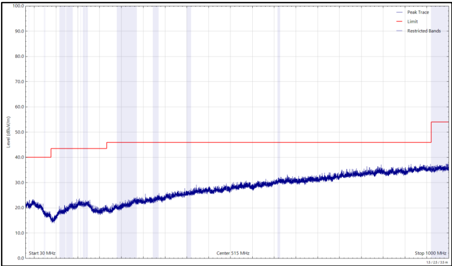
Figure 144 - 2441 MHz (CH39), DH5, iPA, Core 0 + Core 1, 30 MHz to 1 GHz, Vertical (Peak)
