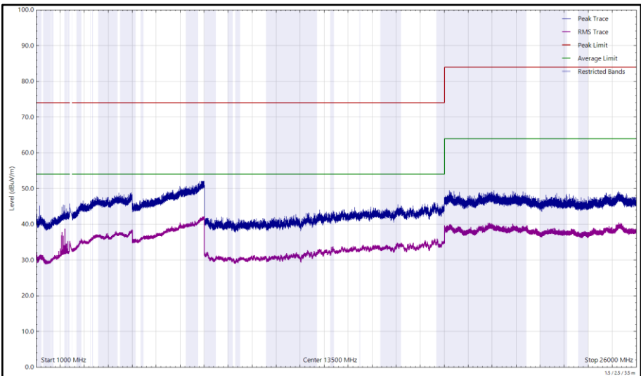
Figure 157 - 2402 MHz (CH0), DH5, iPA, Core 2, 1 GHz to 26 GHz, Vertical
