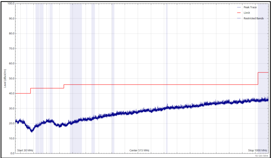
Figure 160 - 2441 MHz (CH39), DH5, iPA, Core 2, 30 MHz to 1 GHz, Vertical (Peak)
