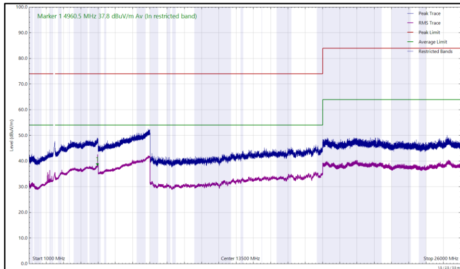
Figure 146 - 2480 MHz (CH78), DH5, iPA, Core 0 + Core 1, 1 GHz to 26 GHz, Horizontal
