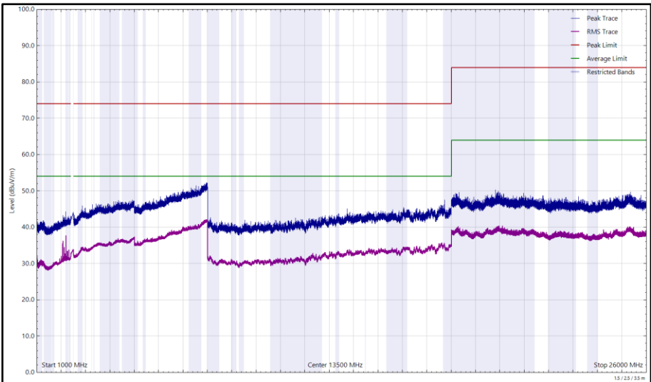
Figure 154 - 2480 MHz (CH78), DH5, ePA, Core 0 + Core 1, 1 GHz to 26 GHz, Horizontal
