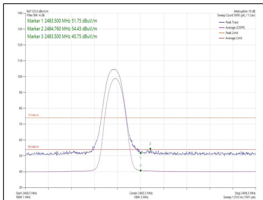
Figure 11 - Static - \pi/4 DQPSK/2DH5 - 2480 MHz - Band Edge Frequency 2483.5 MHz
