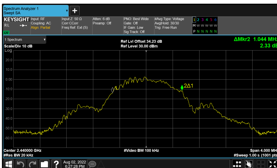
Figure 91 - BT Core 1 (B) 2440 MHz (CH17) 99% Bandwidth
