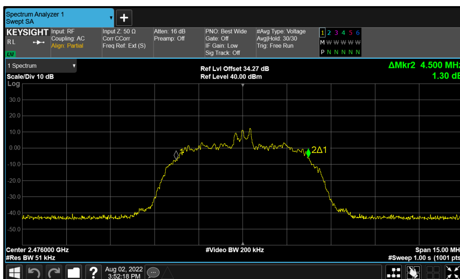
Figure 133 - BT Core 0 (A) 2476 MHz (CH74) 99% Bandwidth
