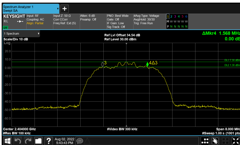
Figure 78 - BT Core 2 (C) 2404 MHz (CH2) 6 dB Bandwidth
