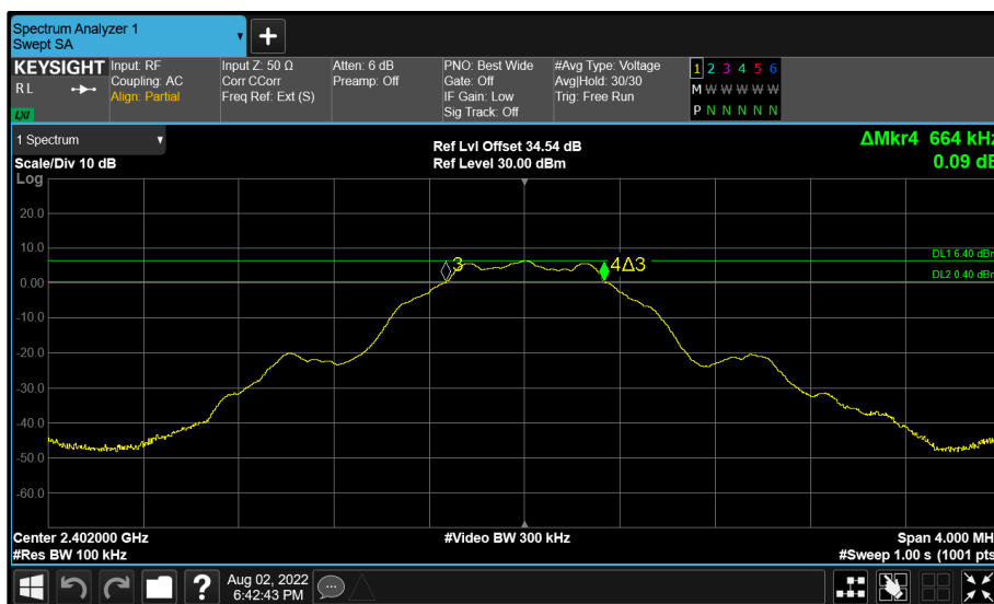
Figure 102 - BT Core 2 (C) 2402 MHz (CH37) 6 dB Bandwidth
