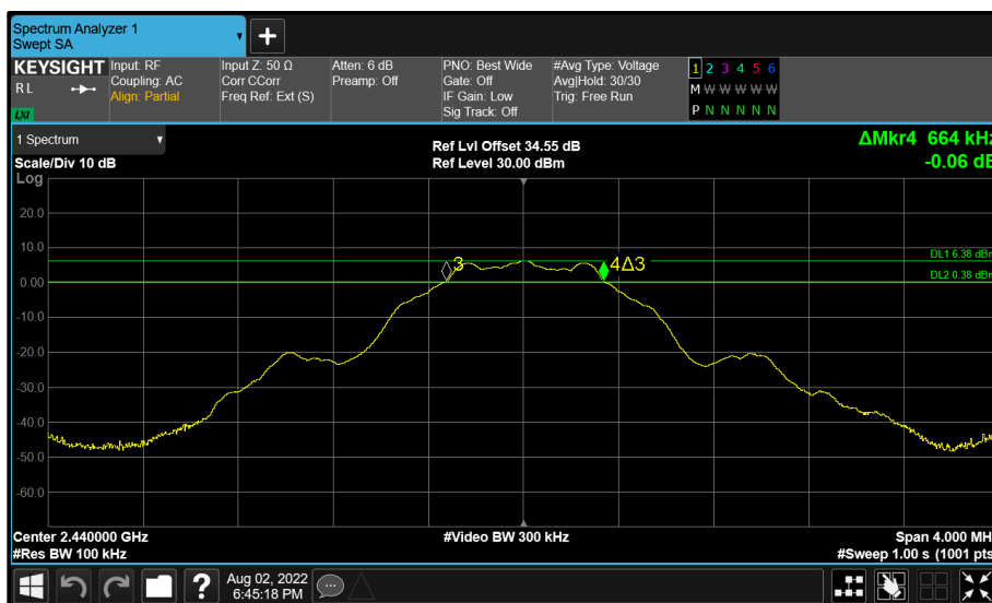
Figure 104 - BT Core 2 (C) 2440 MHz (CH17) 6 dB Bandwidth
