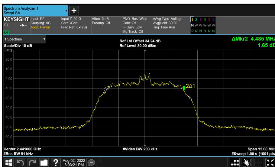
Figure 153 - BT Core 0 (A) 2441 MHz (CH39) 99% Bandwidth
