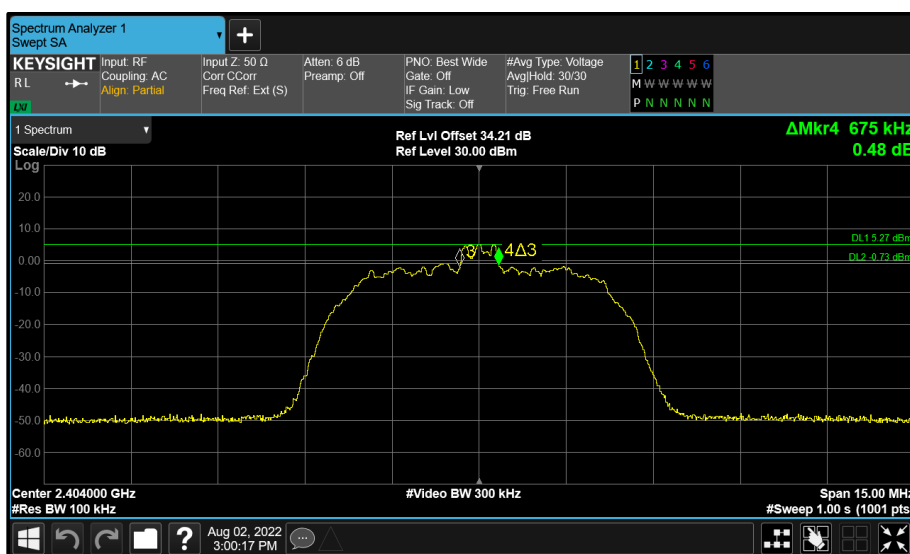
Figure 152 - BT Core 1 (B) 2404 MHz (CH2) 6 dB Bandwidth
