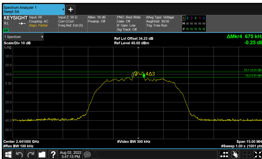
Figure 132 - BT Core 1 (B) 2441 MHz (CH39) 6 dB Bandwidth
