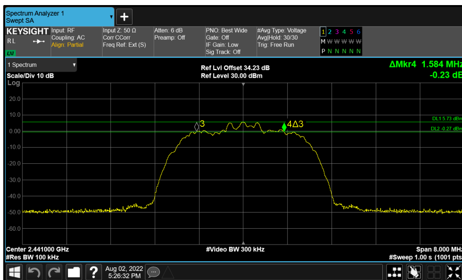
Figure 68 - BT Core 1 (B) 2441 MHz (CH39) 6 dB Bandwidth
