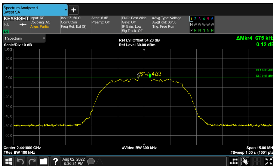
Figure 74 - BT Core 1 (B) 2441 MHz (CH39) 6 dB Bandwidth
