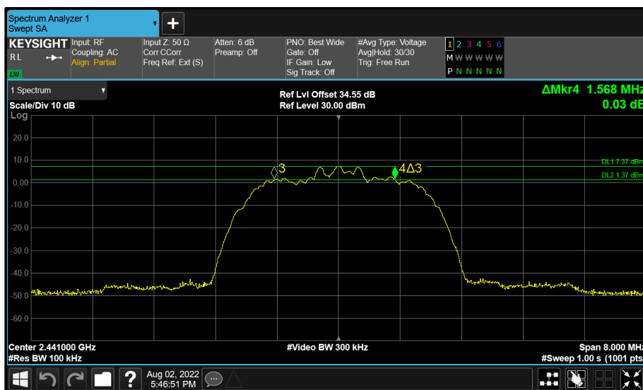
Figure 80 - BT Core 2 (C) 2441 MHz (CH39) 6 dB Bandwidth
