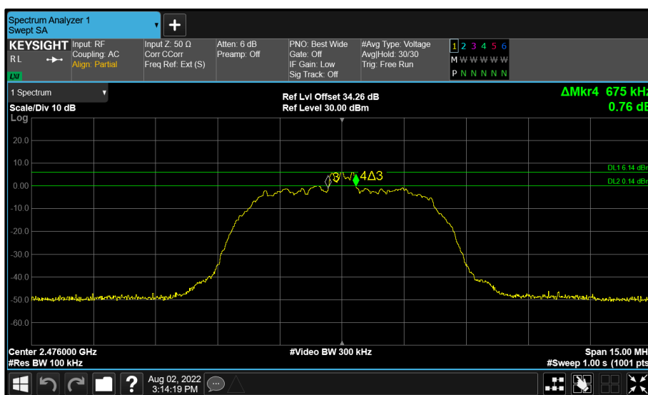
Figure 160 - BT Core 1 (B) 2476 MHz (CH74) 6 dB Bandwidth
