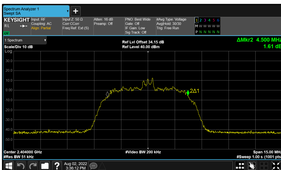
Figure 125 - BT Core 0 (A) 2404 MHz (CH2) 99% Bandwidth
