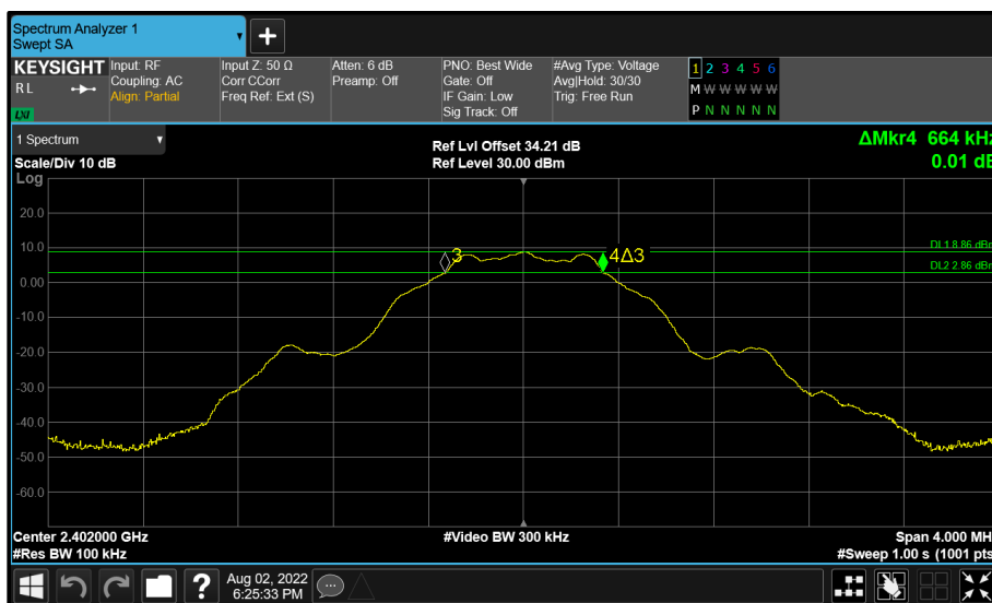
Figure 90 - BT Core 1 (B) 2402 MHz (CH37) 6 dB Bandwidth
