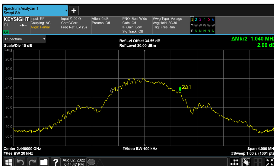
Figure 103 - BT Core 2 (C) 2440 MHz (CH17) 99% Bandwidth
