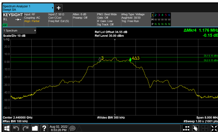
Figure 110 - BT Core 2 (C) 2440 MHz (CH17) 6 dB Bandwidth
