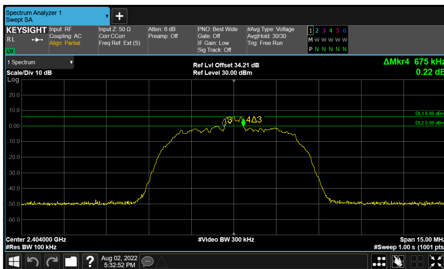
Figure 72 - BT Core 1 (B) 2404 MHz (CH2) 6 dB Bandwidth
