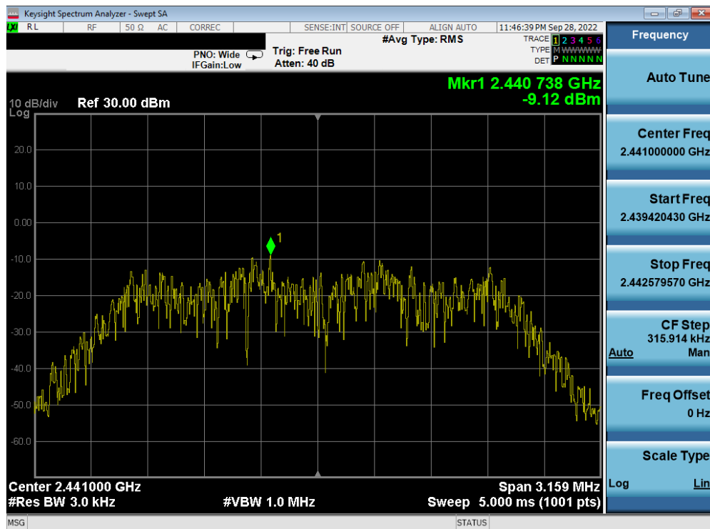
Plot 7-46. Power Spectral Density Plot Antenna WF7b (Bluetooth (HDR4), 4Mbps, iPA – Ch. 38)
