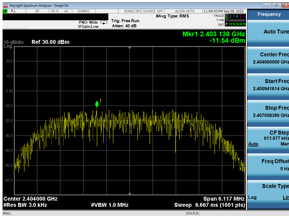
Plot 7-56. Power Spectral Density Plot Antenna WF7b (Bluetooth (HDR8), 8Mbps, iPA – Ch. 1)
