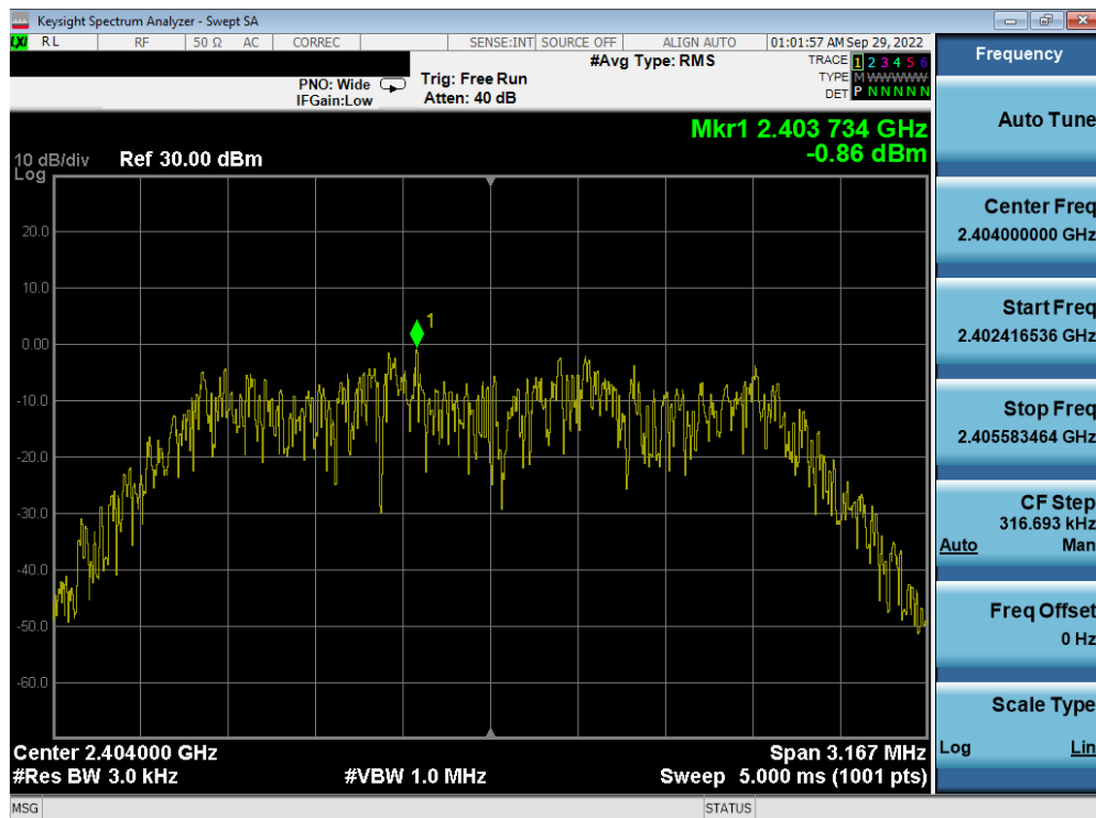
Plot 7-38. Power Spectral Density Plot Antenna WF7b (Bluetooth (HDR4), 4Mbps, ePA – Ch. 1)
