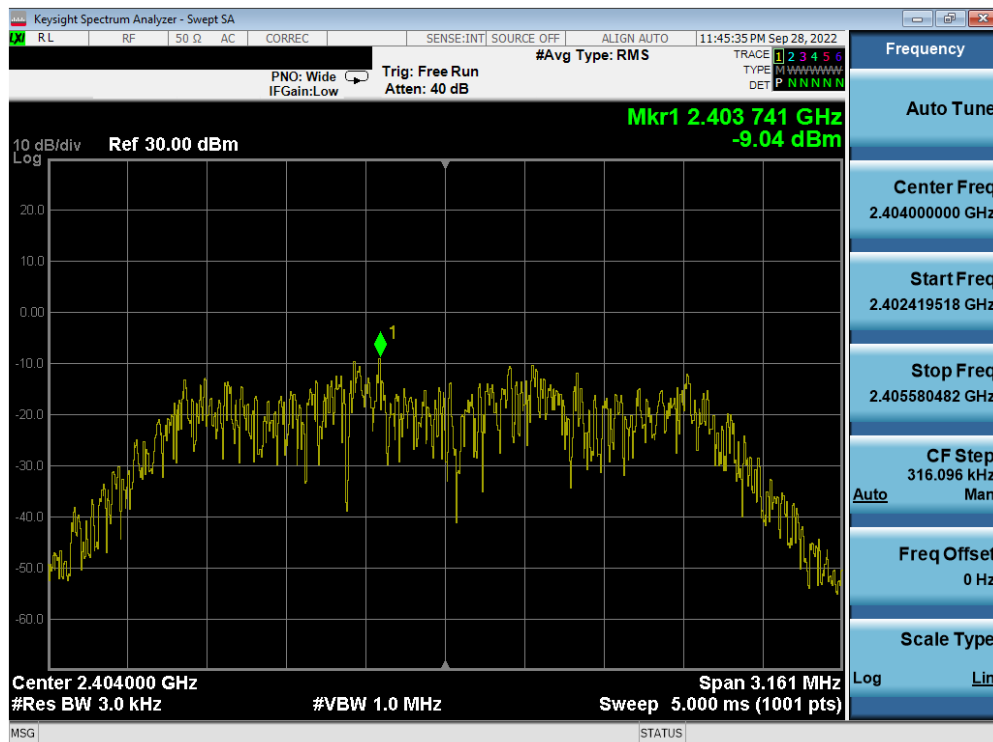
Plot 7-44. Power Spectral Density Plot Antenna WF7b (Bluetooth (HDR4), 4Mbps, iPA – Ch. 1)
