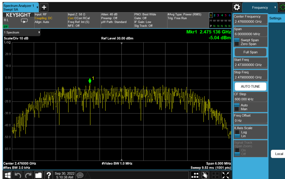
Plot 7-54. Power Spectral Density Plot Antenna WF7b (Bluetooth (HDR8), 8Mbps, ePA – Ch. 73)
