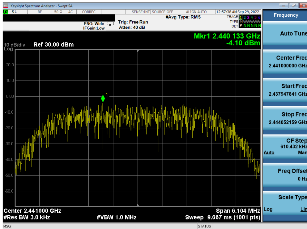
Plot 7-52. Power Spectral Density Plot Antenna WF7b (Bluetooth (HDR8), 8Mbps, ePA – Ch. 38)
