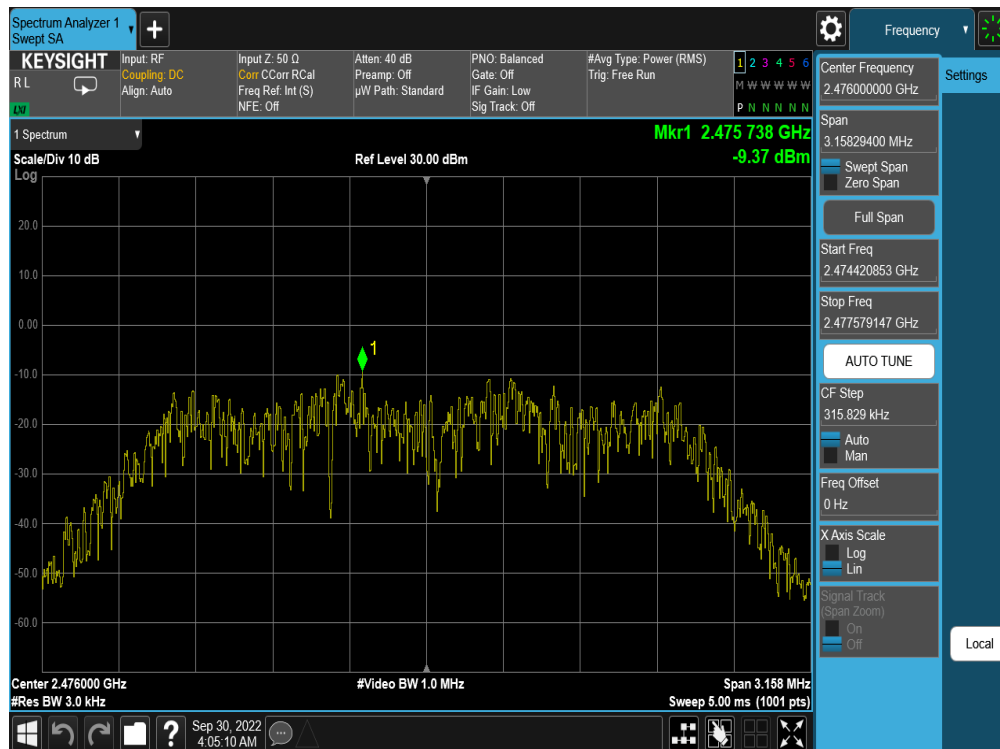
Plot 7-48. Power Spectral Density Plot Antenna WF7b (Bluetooth (HDR4), 4Mbps, iPA – Ch. 73)
