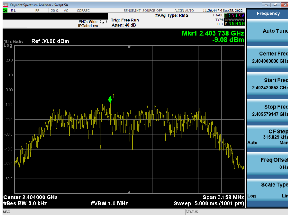
Plot 7-43. Power Spectral Density Plot Antenna WF8 (Bluetooth (HDR4), 4Mbps, iPA – Ch. 1)
