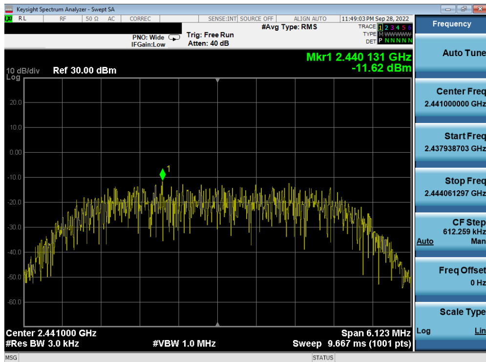
Plot 7-58. Power Spectral Density Plot Antenna WF7b (Bluetooth (HDR8), 8Mbps, iPA – Ch. 38)
