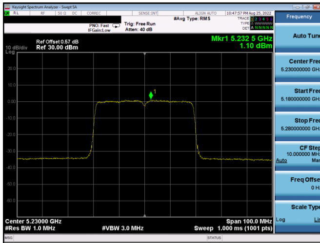
Plot 7-327. ISED PSD SDM Antenna WF8 (40MHz BW 11ax - RU484 - Ch.46)
