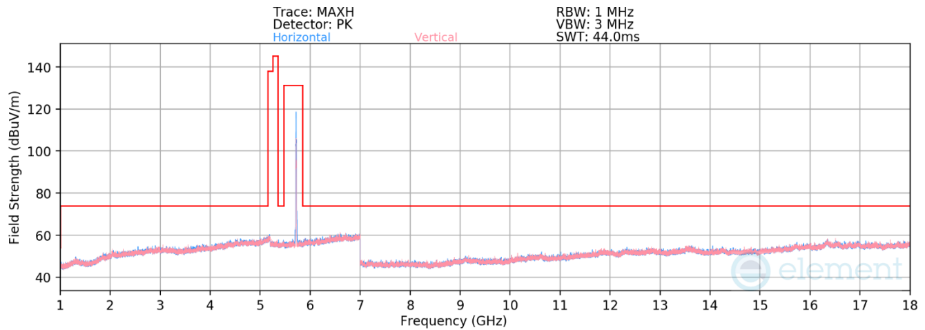
Plot 7-345. RSE above 1GHz Antenna WF8 (11ax – Ch.144 – RU52)
