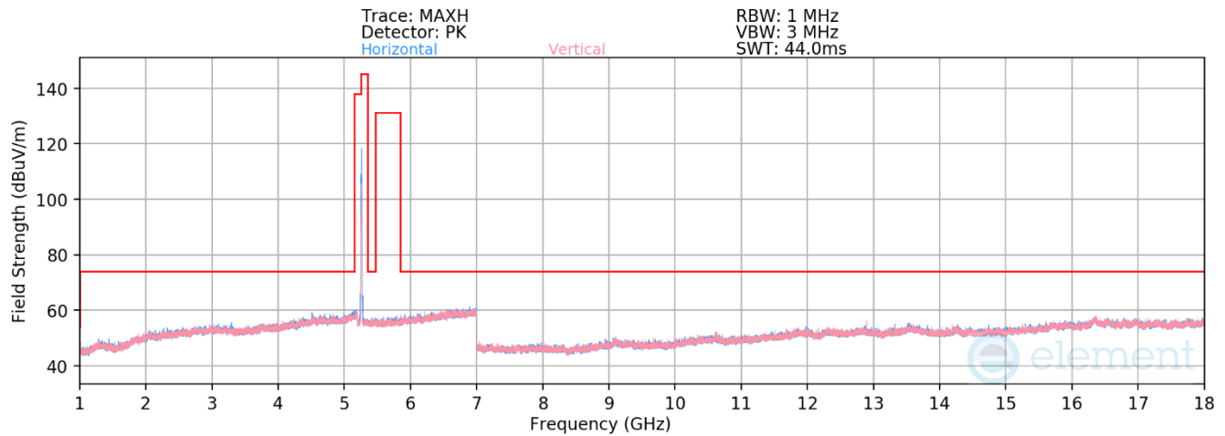
Plot 7-364. RSE above 1GHz Antenna WF7a (11ax – Ch.52 – RU52)
