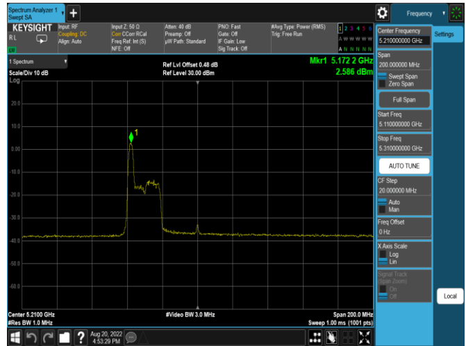
Plot 7-330. ISED PSD SDM Antenna WF7a (80MHz BW 11ax Index 0 - RU26 - Ch.42)
