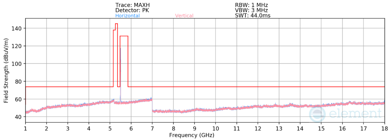
Plot 7-343. RSE above 1GHz Antenna WF8 (11ax – Ch.100 – RU52)
