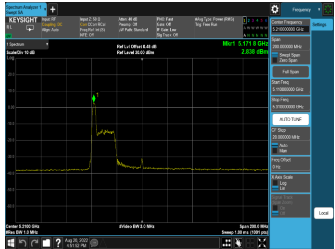
Plot 7-329. ISED PSD SDM Antenna WF8 (80MHz BW 11ax Index 0 - RU26 - Ch.42)
