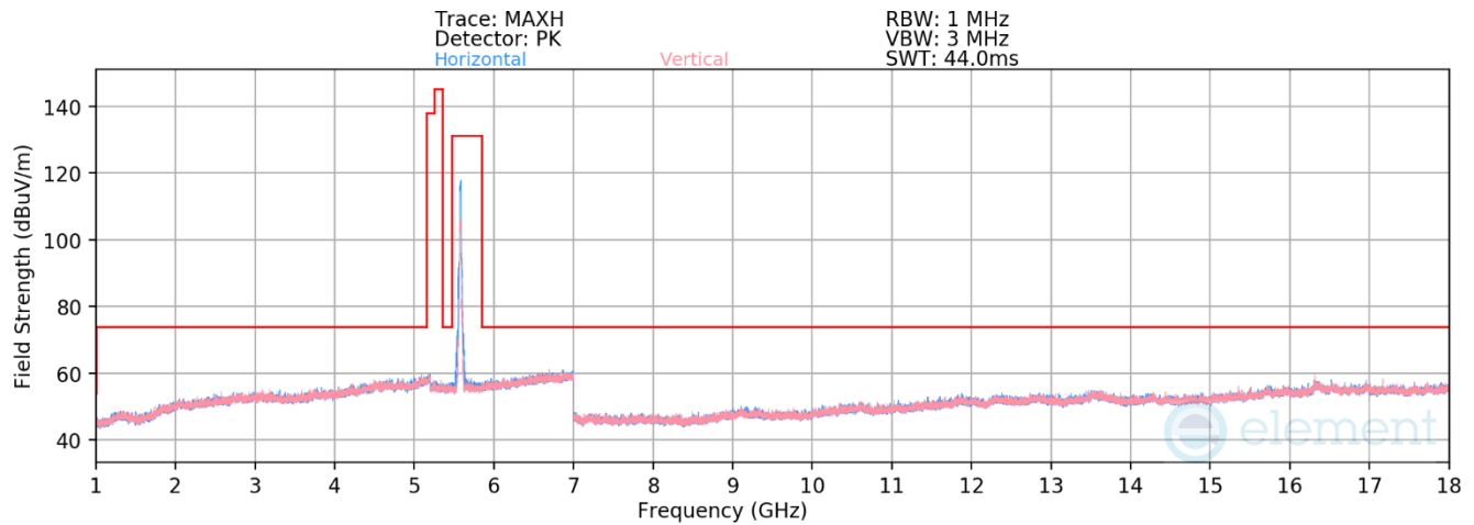
Plot 7-356. RSE above 1GHz Antenna WF8 (11ax – Ch.116 – RU242)
