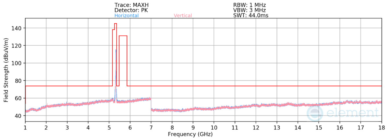
Plot 7-354. RSE above 1GHz Antenna WF8 (11ax – Ch.64 – RU242)
