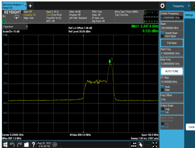
Plot 7-326. ISED PSD SDM Antenna WF7a (40MHz BW 11ax Index 17 - RU26 - Ch.46)
