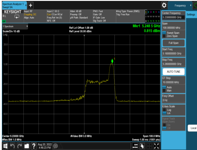
Plot 7-325. ISED PSD SDM Antenna WF8 (40MHz BW 11ax Index 17 - RU26 - Ch.46)
