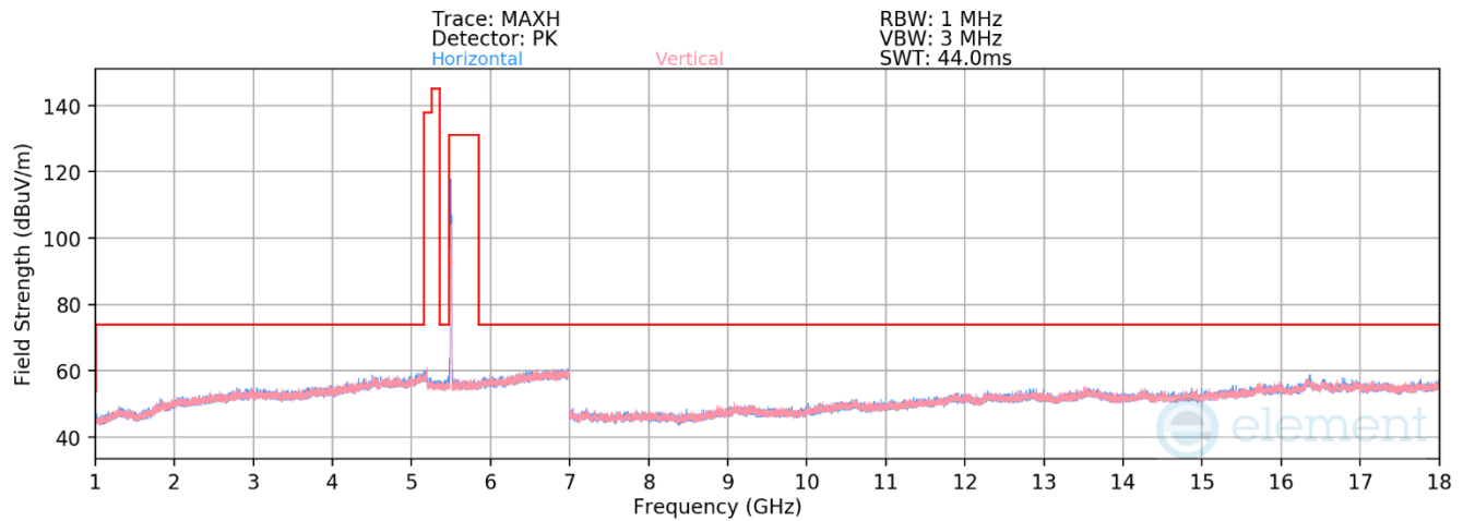
Plot 7-367. RSE above 1GHz Antenna WF7a (11ax – Ch.100 – RU52)
