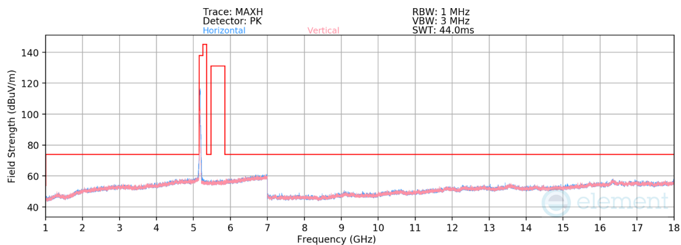
Plot 7-349. RSE above 1GHz Antenna WF8 (11ax – Ch.36 – RU242)
