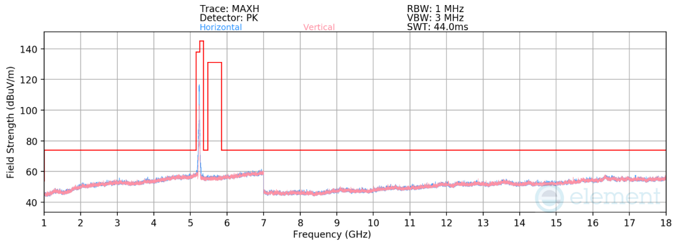
Plot 7-351. RSE above 1GHz Antenna WF8 (11ax – Ch.48 – RU242)
