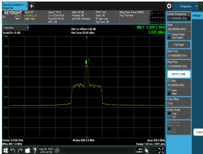
Plot 7-332. ISED PSD SDM Antenna WF7a (80MHz BW 11ax Index 18 – RU26 – Ch.42)
