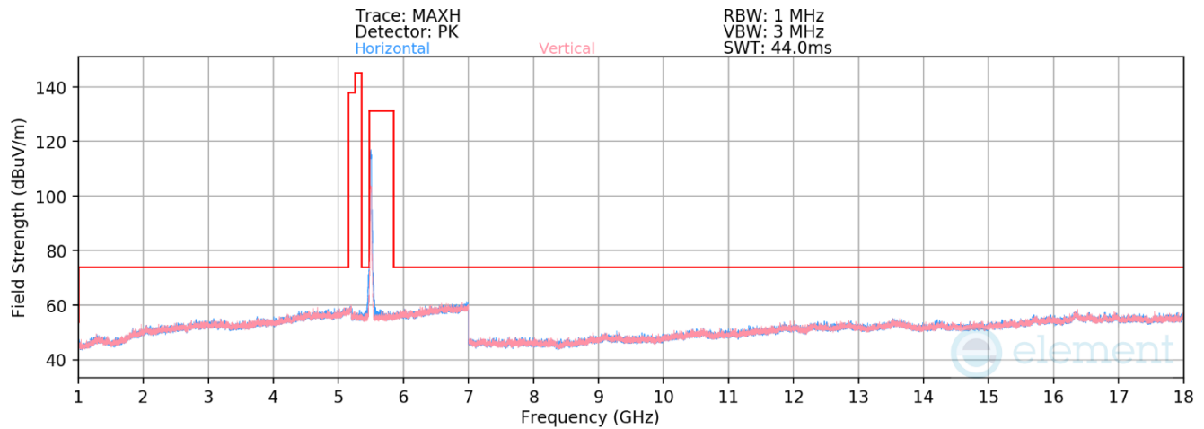
Plot 7-355. RSE above 1GHz Antenna WF8 (11ax – Ch.100 – RU242)
