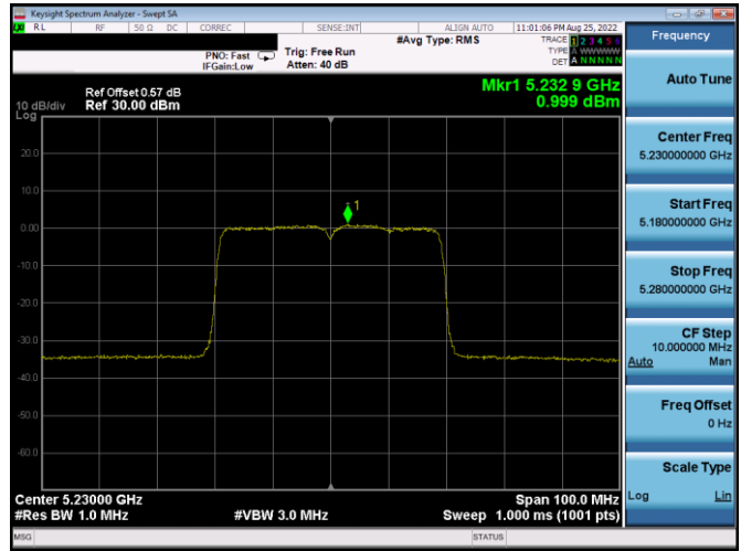
Plot 7-328. ISED PSD SDM Antenna WF7a (40MHz BW 11ax - RU484 - Ch.46)
