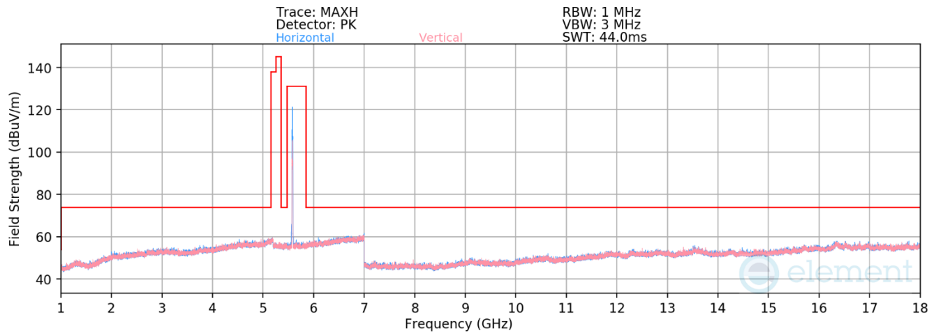
Plot 7-344. RSE above 1GHz Antenna WF8 (11ax – Ch.116 – RU52)
