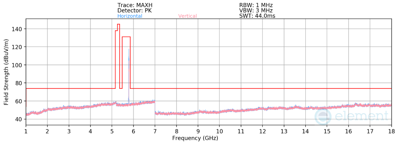
Plot 7-347. RSE above 1GHz Antenna WF8 (11ax – Ch.157 – RU26)
