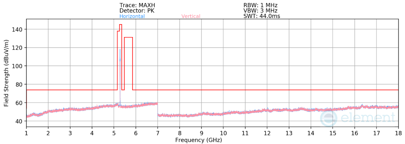
Plot 7-365. RSE above 1GHz Antenna WF7a (11ax – Ch.56 – RU52)
