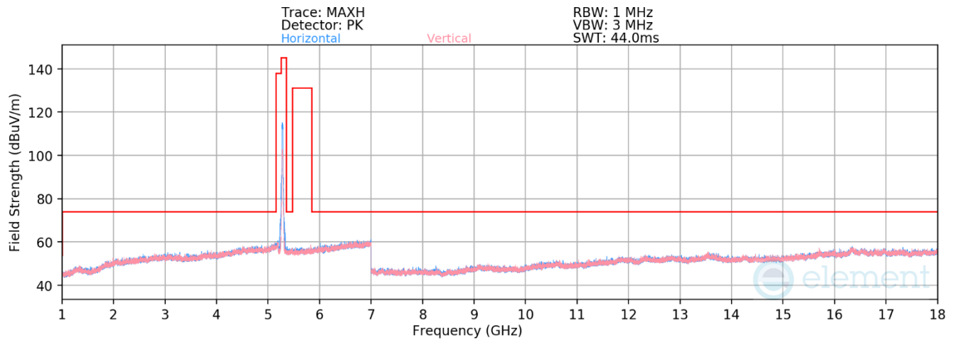
Plot 7-353. RSE above 1GHz Antenna WF8 (11ax - Ch.56 - RU242)
