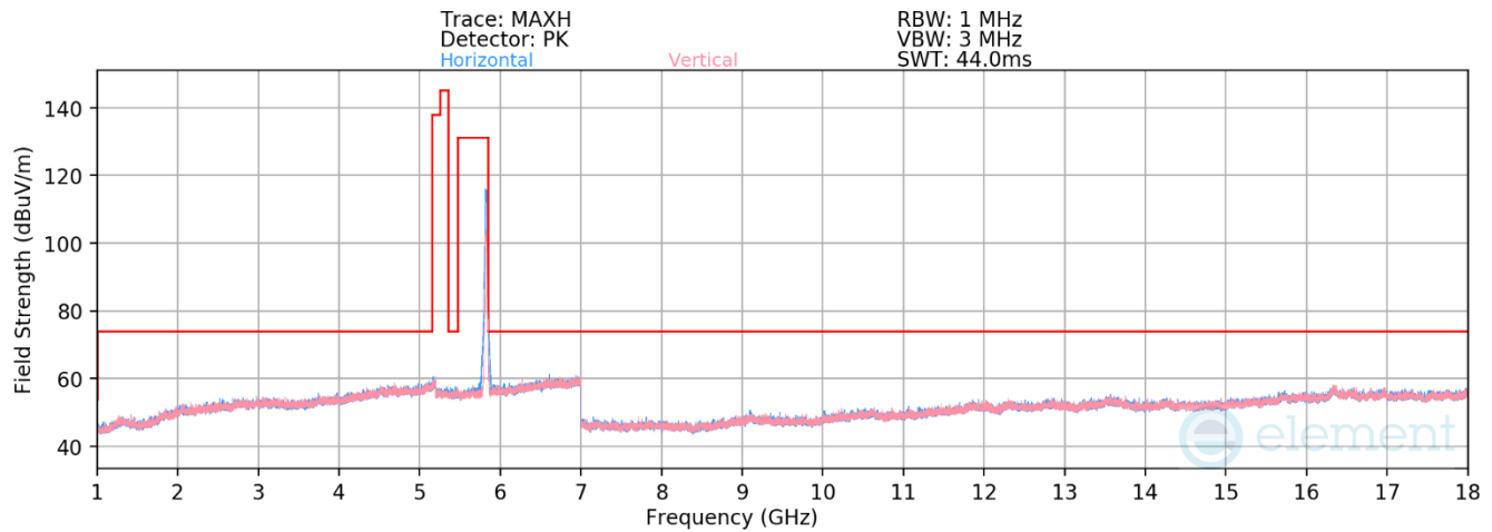
Plot 7-360. RSE above 1GHz Antenna WF8 (11ax – Ch.165 – RU242)
