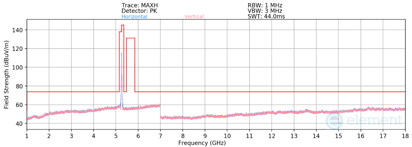
Plot 7-352. RSE above 1GHz Antenna WF8 (11ax – Ch.52 – RU242)
