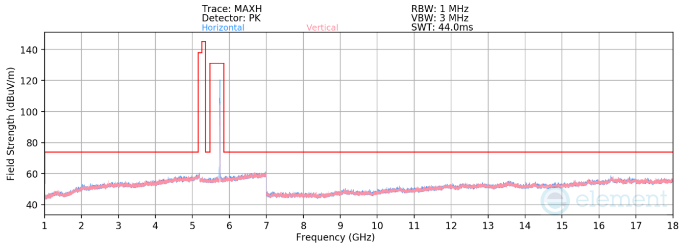
Plot 7-346. RSE above 1GHz Antenna WF8 (11ax – Ch.149 – RU26)
