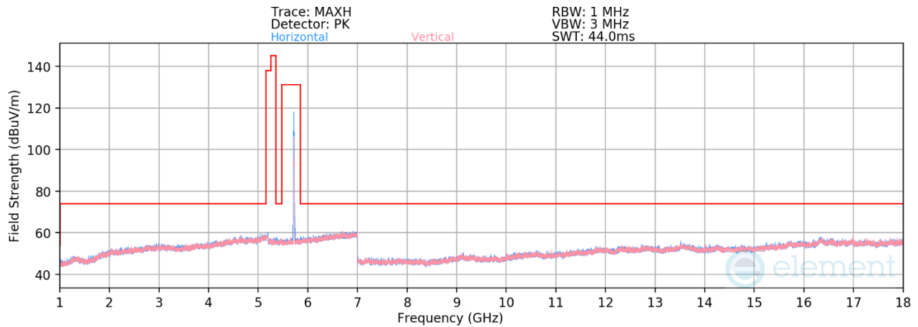
Plot 7-369. RSE above 1GHz Antenna WF7a (11ax – Ch.144 – RU52)
