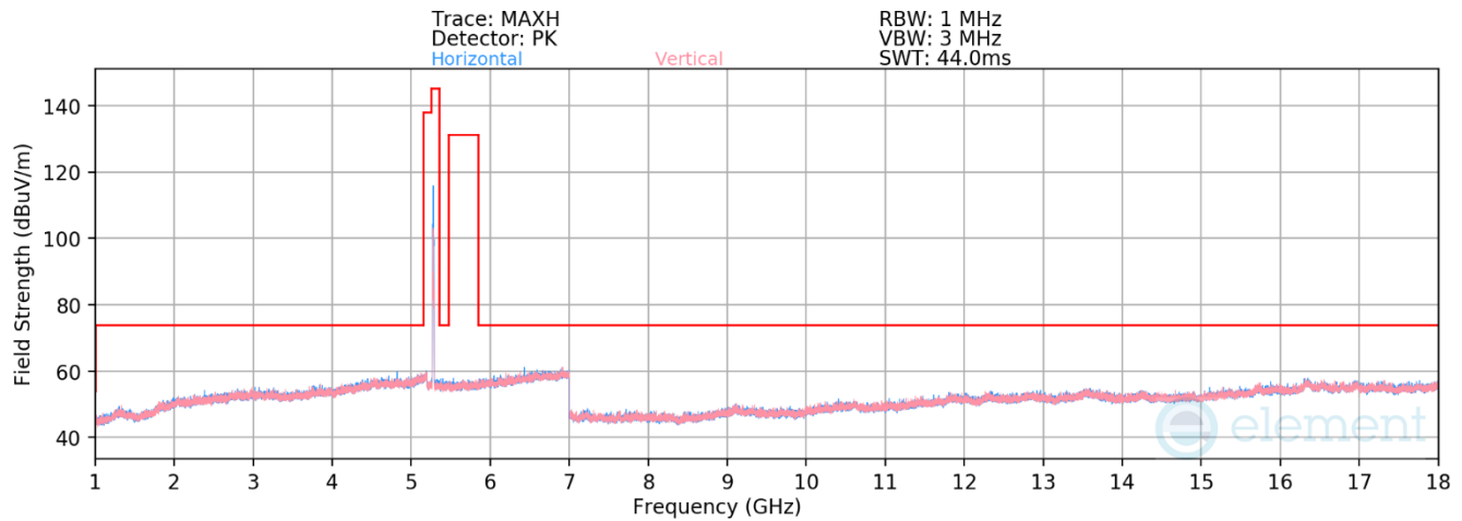
Plot 7-341. RSE above 1GHz Antenna WF8 (11ax – Ch.56 – RU52)
