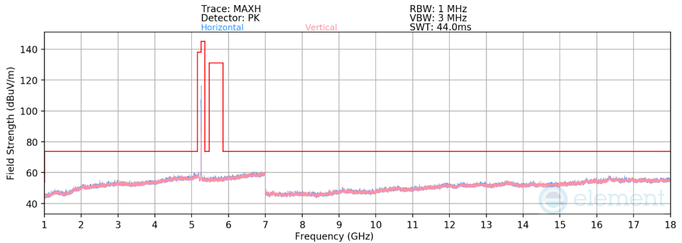
Plot 7-340. RSE above 1GHz Antenna WF8 (11ax – Ch.52 – RU52)
