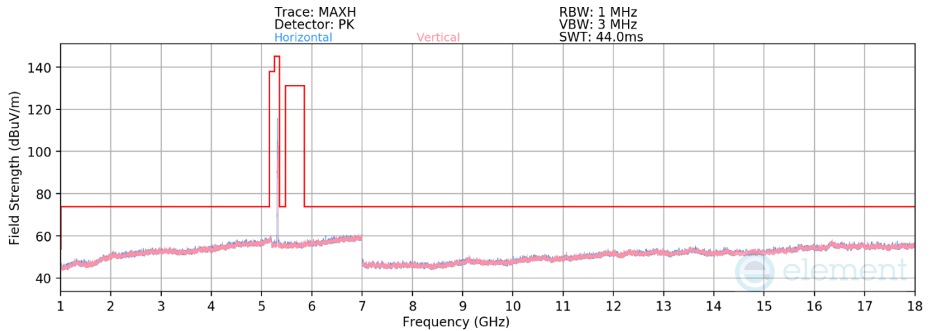
Plot 7-342. RSE above 1GHz Antenna WF8 (11ax – Ch.64 – RU52)
