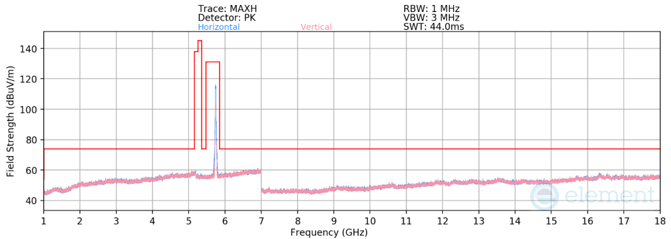
Plot 7-358. RSE above 1GHz Antenna WF8 (11ax – Ch.149 – RU242)
