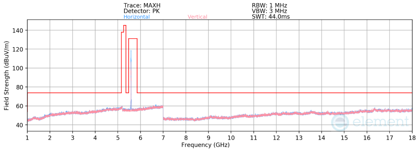
Plot 7-368. RSE above 1GHz Antenna WF7a (11ax – Ch.116 – RU52)
