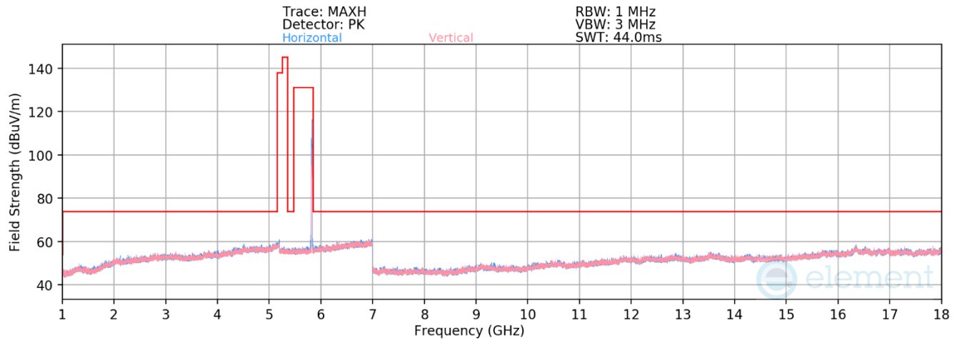
Plot 7-348. RSE above 1GHz Antenna WF8 (11ax – Ch.165 – RU26)
