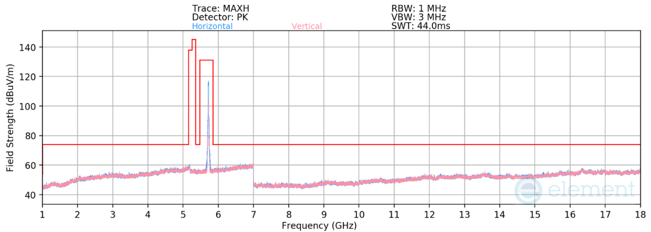
Plot 7-357. RSE above 1GHz Antenna WF8 (11ax – Ch.144 – RU242)
