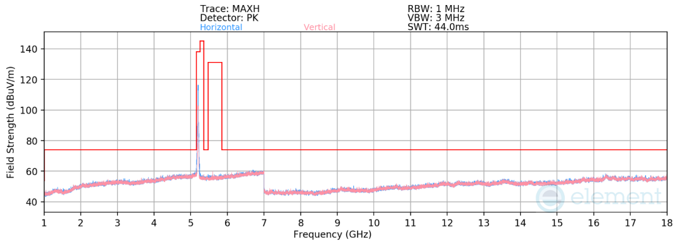
Plot 7-350. RSE above 1GHz Antenna WF8 (11ax – Ch.40 – RU242)
