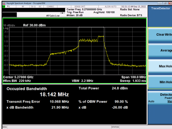
Plot 7-19. 26dB BW & 99% OBW Antenna WF8 (40MHz BW 11ax Index 44 - RU52 - Ch.54)
