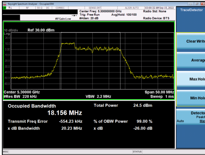
Plot 7-49. 26dB BW & 99% OBW Antenna WF7a (20MHz BW 11ax Index 37 – RU52 – Ch.60)
