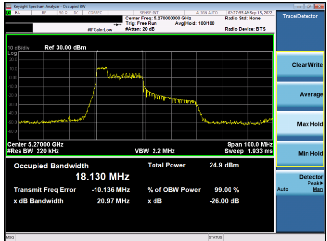
Plot 7-17. 26dB BW & 99% OBW Antenna WF8 (40MHz BW 11ax Index 37 – RU52 – Ch.54)
