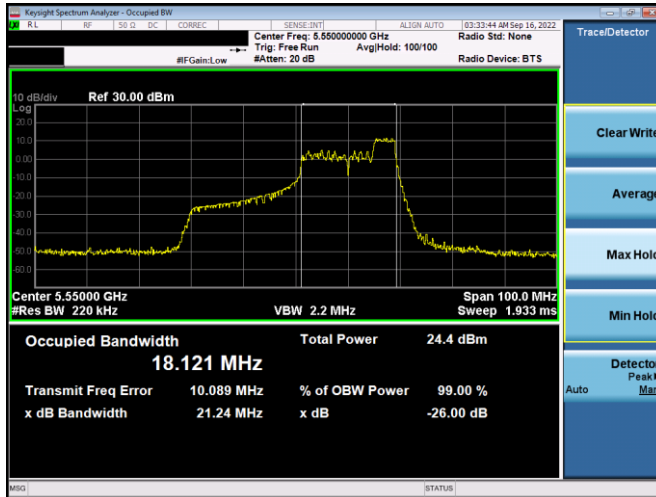
Plot 7-31. 26dB BW & 99% OBW Antenna WF8 (40MHz BW 11ax Index 44 – RU52 – Ch.110)
