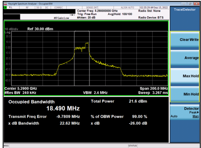
Plot 7-22. 26dB BW & 99% OBW Antenna WF8 (80MHz BW 11ax Index 44 - RU52 - Ch.58)
