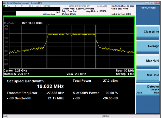
Plot 7-16. 26dB BW & 99% OBW Antenna WF8 (20MHz BW 11ax- RU242 – Ch.56)
