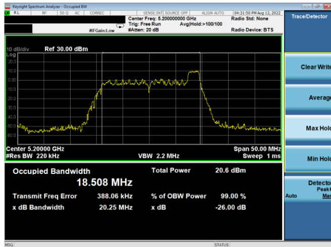
Plot 7-39. 26dB BW & 99% OBW Antenna WF7a (20MHz BW 11ax Index 8 – RU26 – Ch.40)
