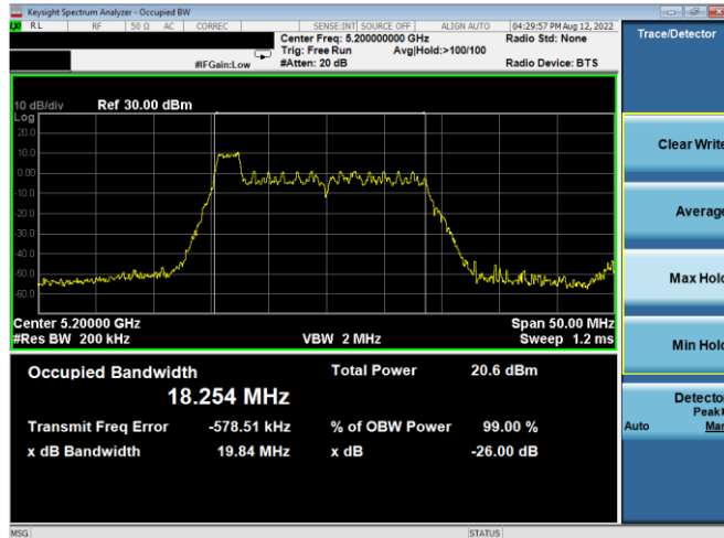
Plot 7-37. 26dB BW & 99% OBW Antenna WF7a (20MHz BW 11ax Index 0 – RU26 – Ch.40)
