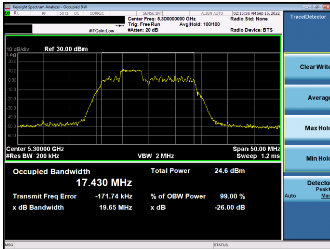
Plot 7-14. 26dB BW & 99% OBW Antenna WF8 (20MHz BW 11ax Index 38 – RU52 – Ch.60)
