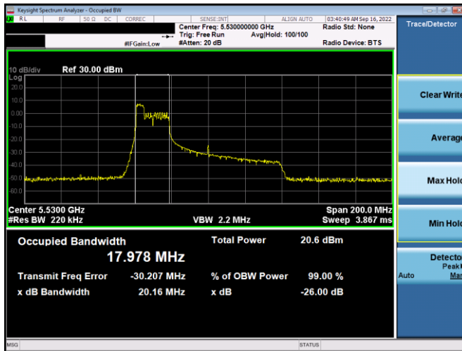
Plot 7-33. 26dB BW & 99% OBW Antenna WF8 (80MHz BW 11ax Index 37 – RU52 – Ch.106)
