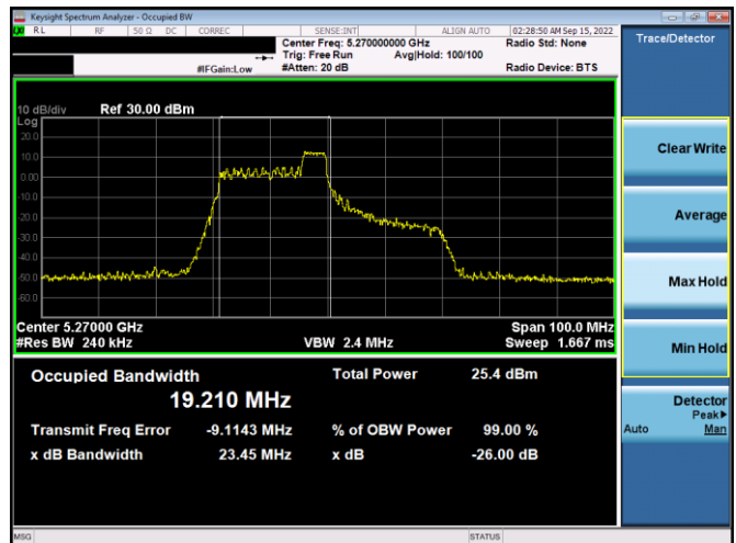
Plot 7-18. 26dB BW & 99% OBW Antenna WF8 (40MHz BW 11ax Index 40 – RU52 – Ch.54)
