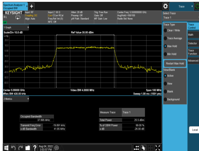
Plot 7-32. 26dB BW & 99% OBW Antenna WF8 (40MHz BW 11ax – RU484 – Ch.110)
