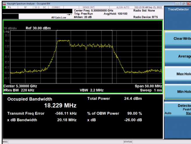
Plot 7-13. 26dB BW & 99% OBW Antenna WF8 (20MHz BW 11ax Index 37 – RU52 – Ch.60)
