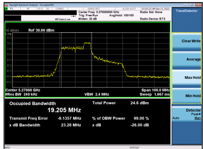
Plot 7-54. 26dB BW & 99% OBW Antenna WF7a (40MHz BW 11ax Index 40 – RU52 – Ch.54)
