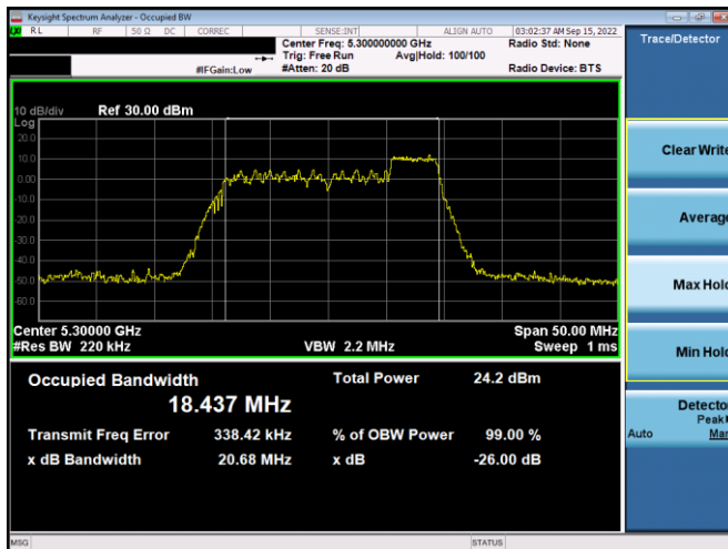
Plot 7-51. 26dB BW & 99% OBW Antenna WF7a (20MHz BW 11ax Index 40 – RU52 – Ch.60)
