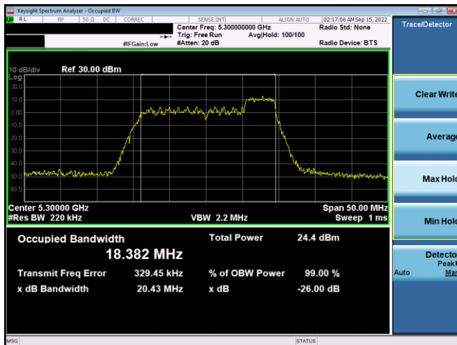
Plot 7-15. 26dB BW & 99% OBW Antenna WF8 (20MHz BW 11ax Index 40 – RU52 – Ch.60)
