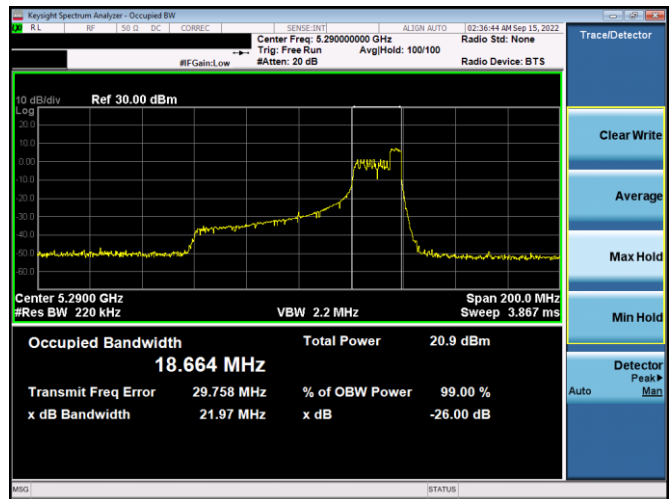
Plot 7-23. 26dB BW & 99% OBW Antenna WF8 (80MHz BW 11ax Index 52 - RU52 - Ch.58)
