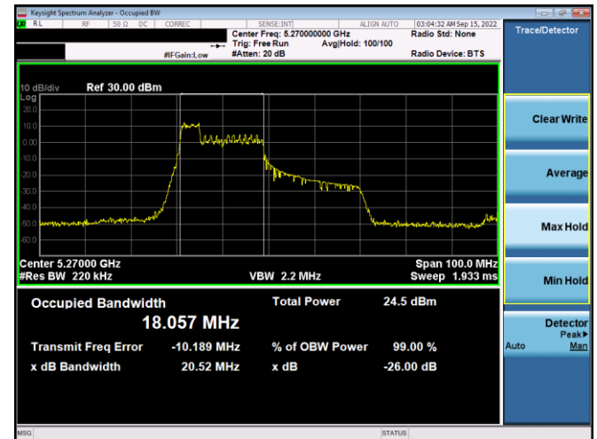
Plot 7-53. 26dB BW & 99% OBW Antenna WF7a (40MHz BW 11ax Index 37 – RU52 – Ch.54)
