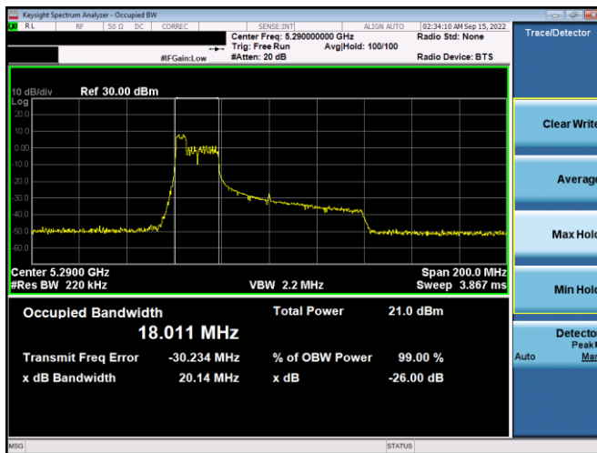
Plot 7-21. 26dB BW & 99% OBW Antenna WF8 (80MHz BW 11ax Index 37 - RU52 - Ch.58)
