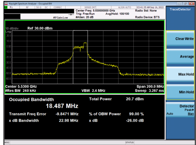
Plot 7-34. 26dB BW & 99% OBW Antenna WF8 (80MHz BW 11ax Index 44 – RU52 – Ch.106)
