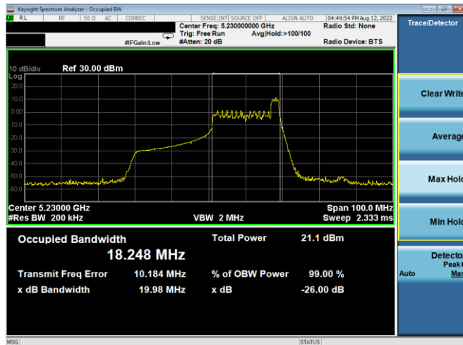
Plot 7-43. 26dB BW & 99% OBW Antenna WF7a (40MHz BW 11ax Index 17 – RU26 – Ch.46)
