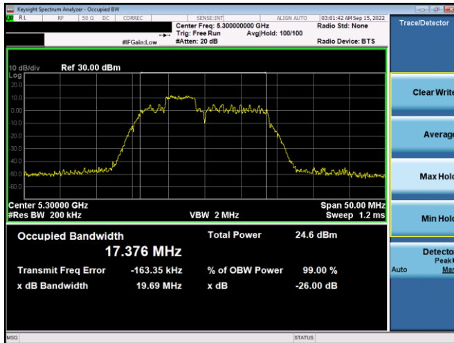
Plot 7-50. 26dB BW & 99% OBW Antenna WF7a (20MHz BW 11ax Index 38 – RU52 – Ch.60)
