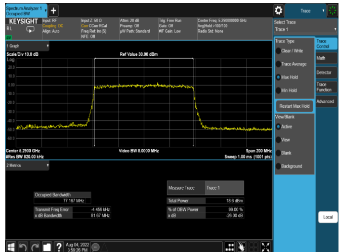
Plot 7-24. 26dB BW & 99% OBW Antenna WF8 (80MHz BW 11ax - RU996 - Ch.58)
