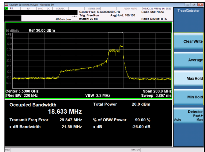
Plot 7-35. 26dB BW & 99% OBW Antenna WF8 (80MHz BW 11ax Index 52 – RU52 – Ch.106)
