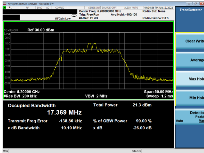
Plot 7-38. 26dB BW & 99% OBW Antenna WF7a (20MHz BW 11ax Index 4 – RU26 – Ch.40)
