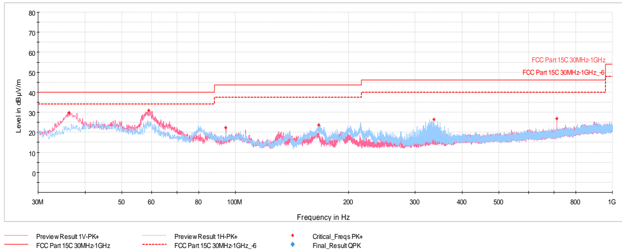
Plot 7-705. Radiated Spurious Emissions below 1GHz CDD 11ax - SU Ch.6, with AC/DC Adapter
