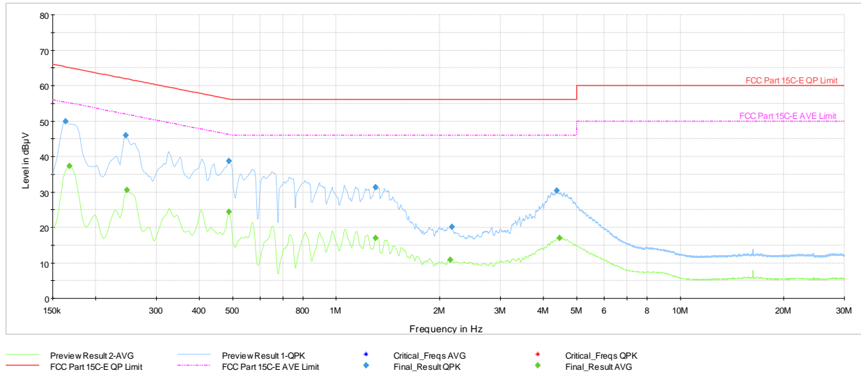
Plot 7-709. AC Line Conducted Plot with CDD 11ax - SU Ch.6 (N, with AC/DC Adapter)
