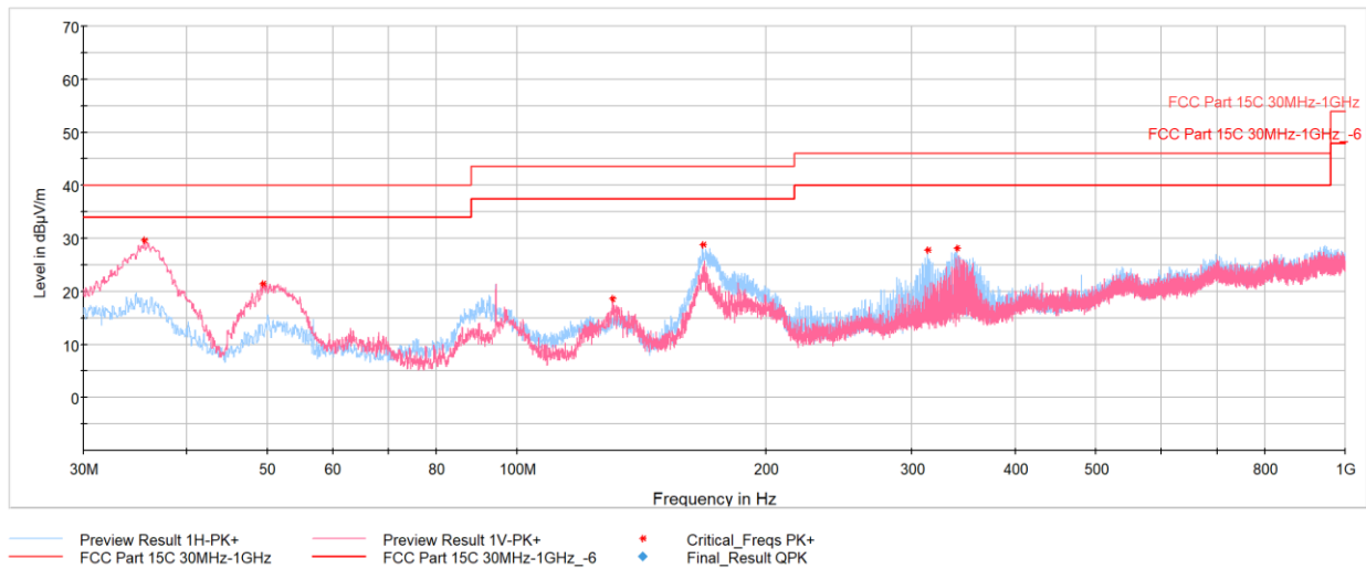
Plot 7-704. Radiated Spurious Emissions below 1GHz CDD 11n Ch.6, with AC/DC Adapter
