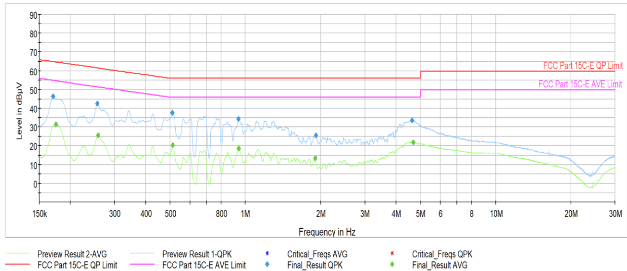
Plot 7-707. AC Line Conducted Plot with CDD 11n Ch.6 (N, with AC/DC Adapter)
