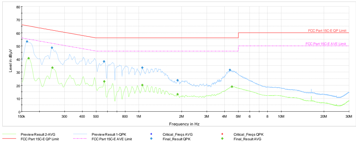
Plot 7-708. AC Line Conducted Plot with CDD 11ax - SU Ch.6 (L1, with AC/DC Adapter)
