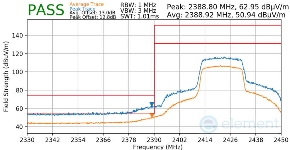
Plot 7-595. Radiated Restricted Lower Band Edge Measurement Antenna WF7b
