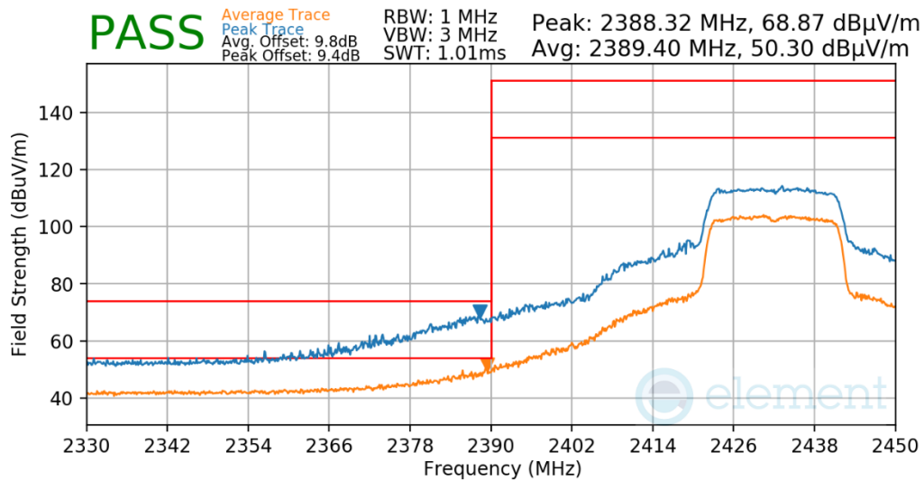
Plot 7-603. Radiated Restricted Lower Band Edge Measurement Antenna WF7b
