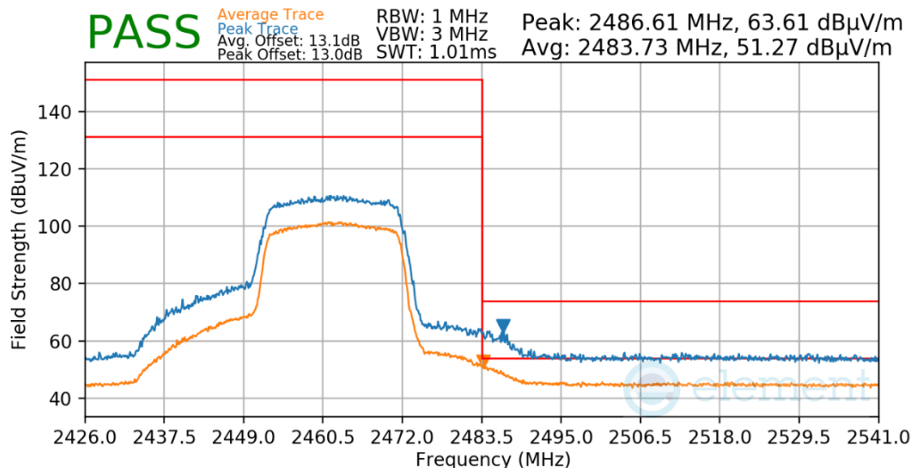
Plot 7-621. Radiated Restricted Upper Band Edge Measurement Antenna WF7b
