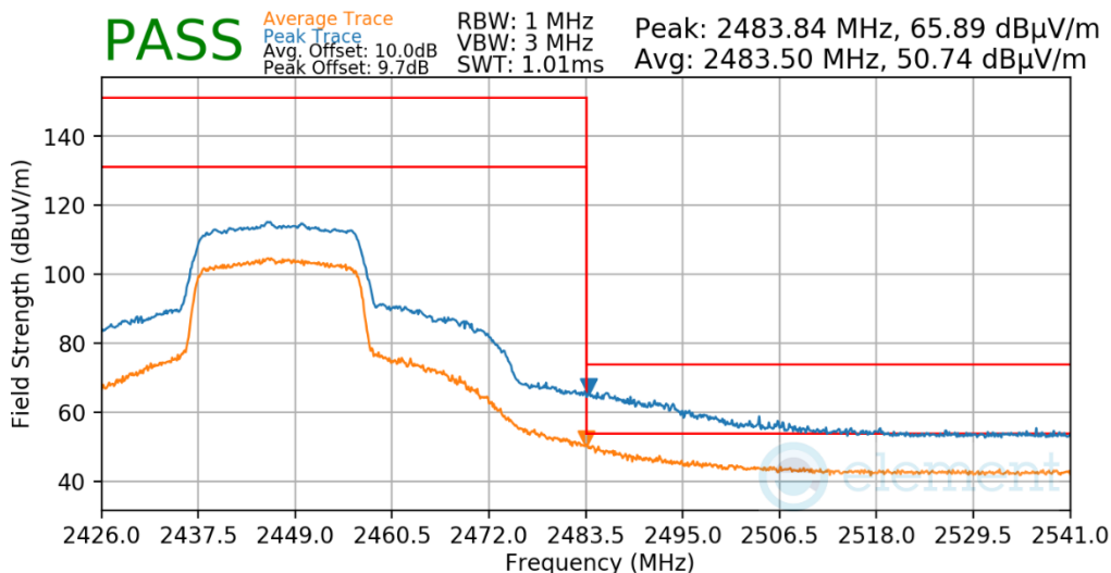
Plot 7-613. Radiated Restricted Upper Band Edge Measurement Antenna WF7b
