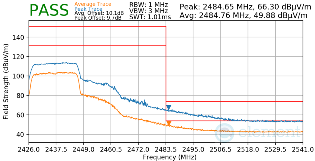
Plot 7-608. Radiated Restricted Upper Band Edge Measurement Antenna WF7b
