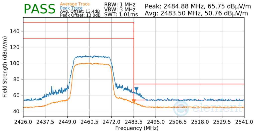
Plot 7-623. Radiated Restricted Upper Band Edge Measurement Antenna WF7b
