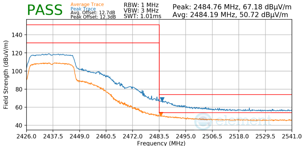
Plot 7-607. Radiated Restricted Upper Band Edge Measurement Antenna WF7b
