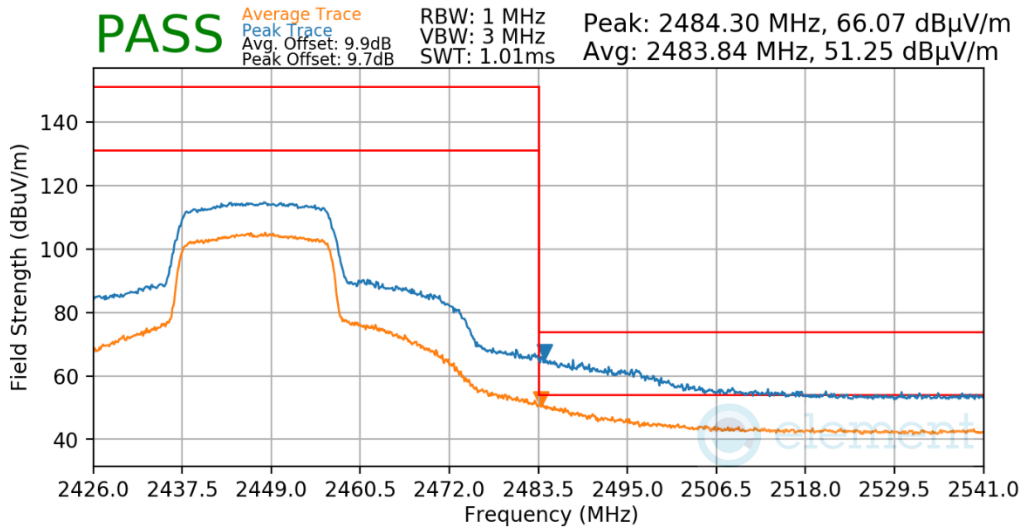
Plot 7-612. Radiated Restricted Upper Band Edge Measurement Antenna WF7b
