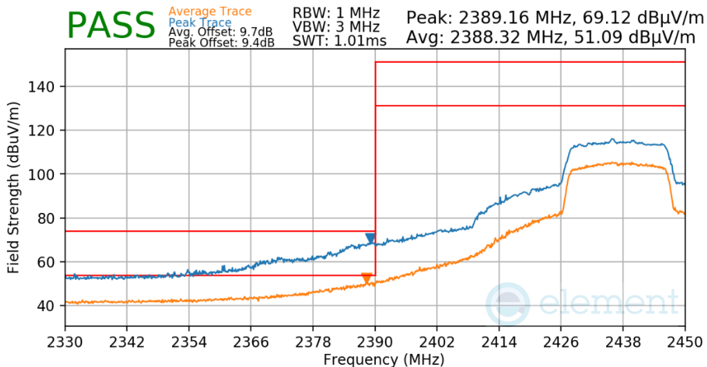
Plot 7-605. Radiated Restricted Lower Band Edge Measurement Antenna WF7b
