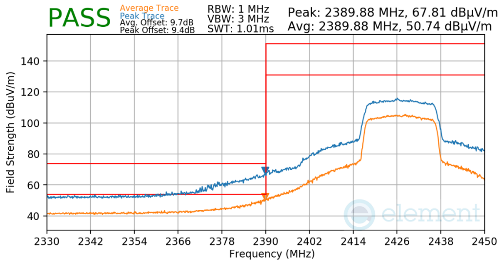
Plot 7-599. Radiated Restricted Lower Band Edge Measurement Antenna WF7b
