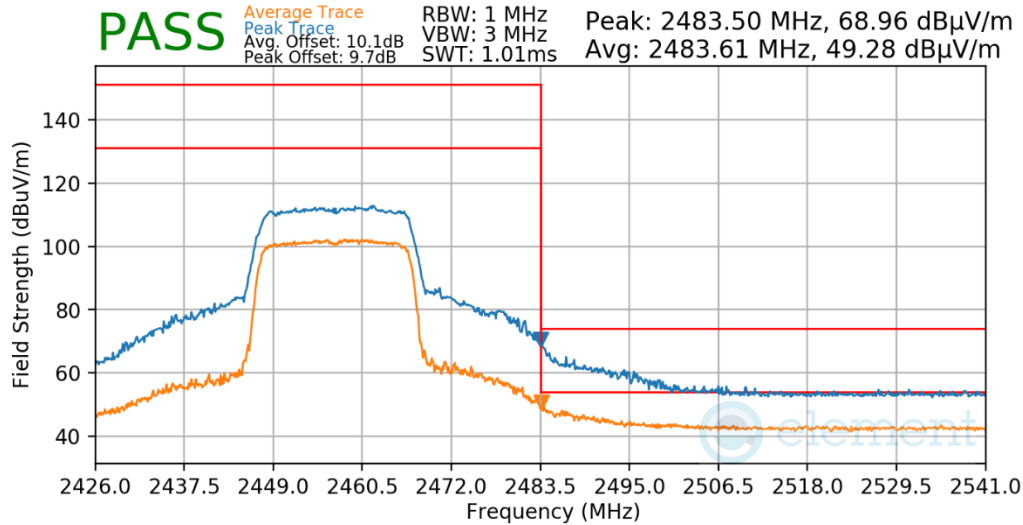
Plot 7-620. Radiated Restricted Upper Band Edge Measurement Antenna WF7b
