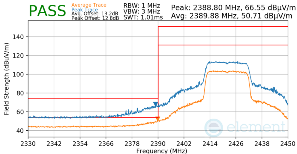
Plot 7-597. Radiated Restricted Lower Band Edge Measurement Antenna WF7b
