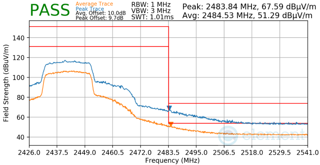
Plot 7-610. Radiated Restricted Upper Band Edge Measurement Antenna WF7b
