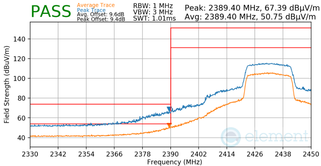
Plot 7-601. Radiated Restricted Lower Band Edge Measurement Antenna WF7b
