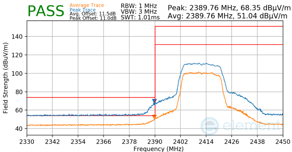
Plot 7-628. Radiated Restricted Lower Band Edge Measurement CDD
