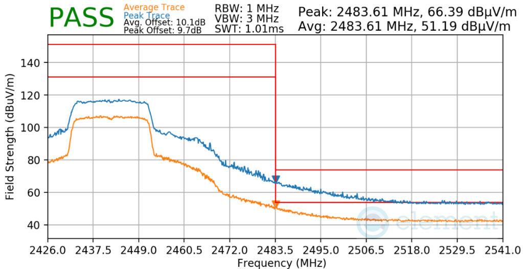
Plot 7-611. Radiated Restricted Upper Band Edge Measurement Antenna WF7b
