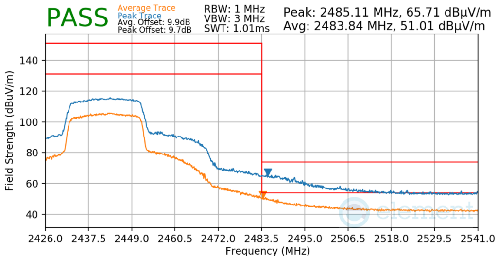
Plot 7-609. Radiated Restricted Upper Band Edge Measurement Antenna WF7b
