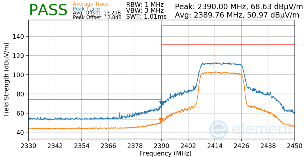
Plot 7-594. Radiated Restricted Lower Band Edge Measurement Antenna WF7b
