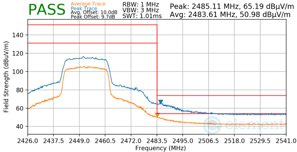
Plot 7-616. Radiated Restricted Upper Band Edge Measurement Antenna WF7b
