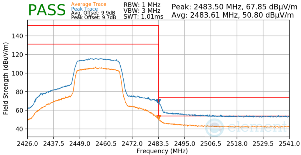
Plot 7-618. Radiated Restricted Upper Band Edge Measurement Antenna WF7b
