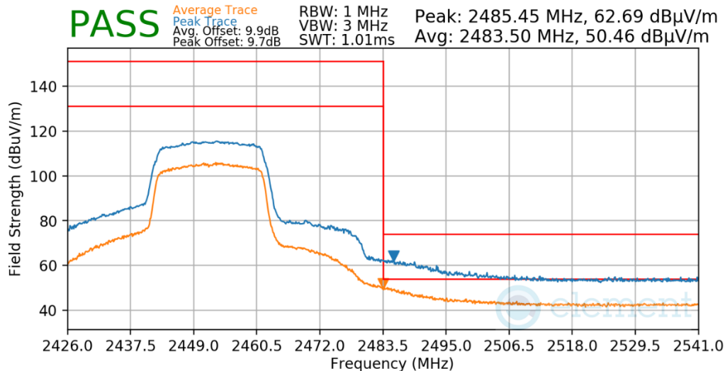
Plot 7-615. Radiated Restricted Upper Band Edge Measurement Antenna WF7b
