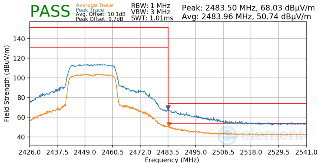
Plot 7-617. Radiated Restricted Upper Band Edge Measurement Antenna WF7b
