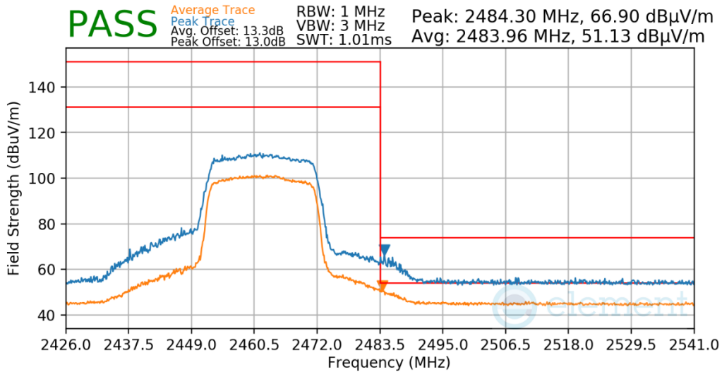
Plot 7-622. Radiated Restricted Upper Band Edge Measurement Antenna WF7b
