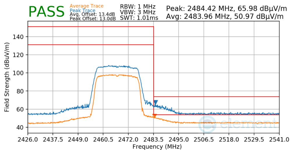
Plot 7-626. Radiated Restricted Upper Band Edge Measurement Antenna WF7b
