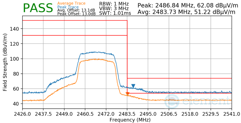
Plot 7-624. Radiated Restricted Upper Band Edge Measurement Antenna WF7b
