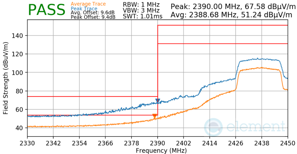
Plot 7-604. Radiated Restricted Lower Band Edge Measurement Antenna WF7b
