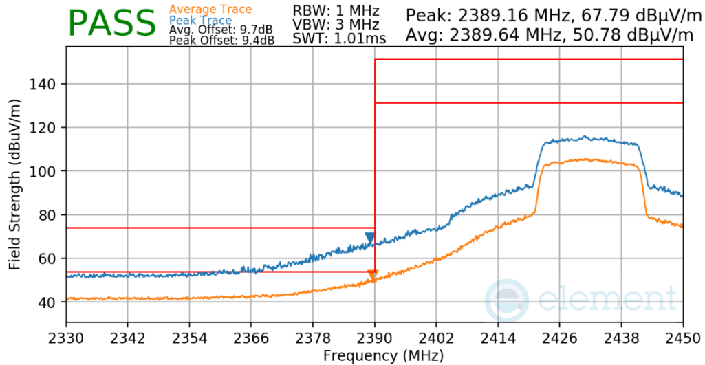
Plot 7-602. Radiated Restricted Lower Band Edge Measurement Antenna WF7b
