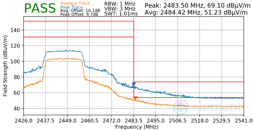
Plot 7-614. Radiated Restricted Upper Band Edge Measurement Antenna WF7b
