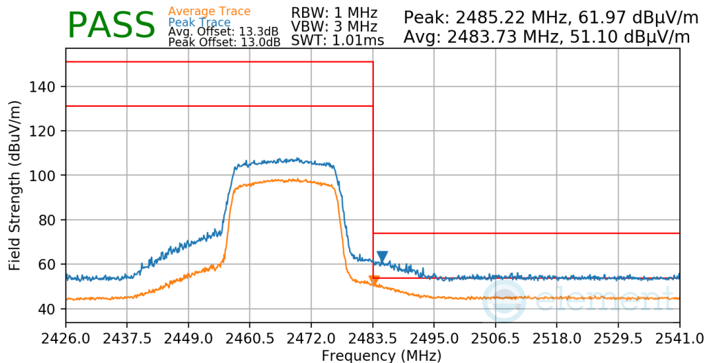
Plot 7-625. Radiated Restricted Upper Band Edge Measurement Antenna WF7b
