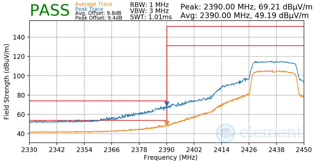
Plot 7-606. Radiated Restricted Lower Band Edge Measurement Antenna WF7b
