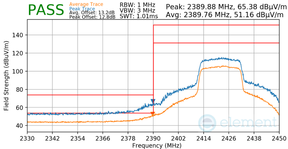
Plot 7-596. Radiated Restricted Lower Band Edge Measurement Antenna WF7b
