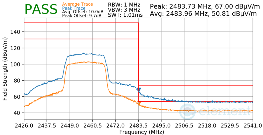
Plot 7-619. Radiated Restricted Upper Band Edge Measurement Antenna WF7b
