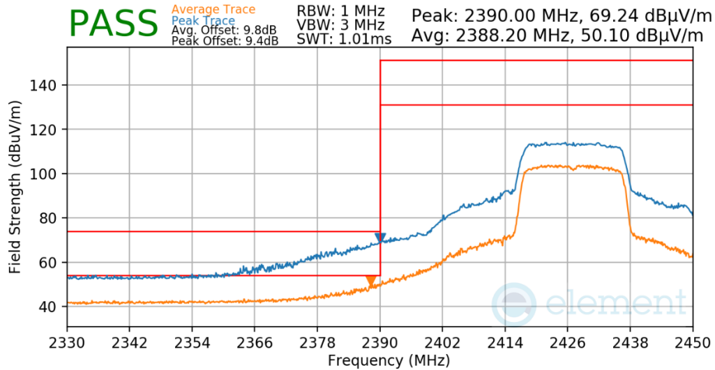
Plot 7-600. Radiated Restricted Lower Band Edge Measurement Antenna WF7b
