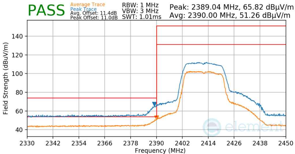
Plot 7-627. Radiated Restricted Lower Band Edge Measurement CDD
