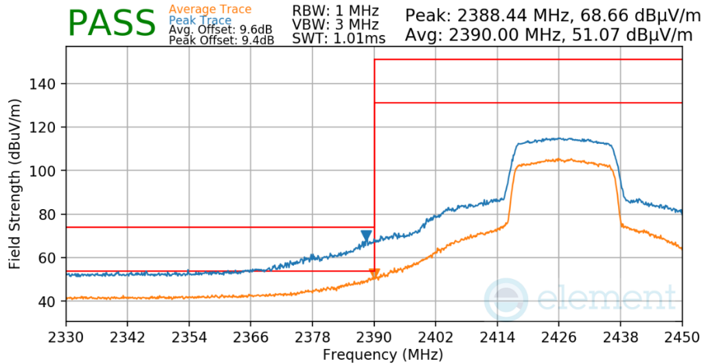
Plot 7-598. Radiated Restricted Lower Band Edge Measurement Antenna WF7b
