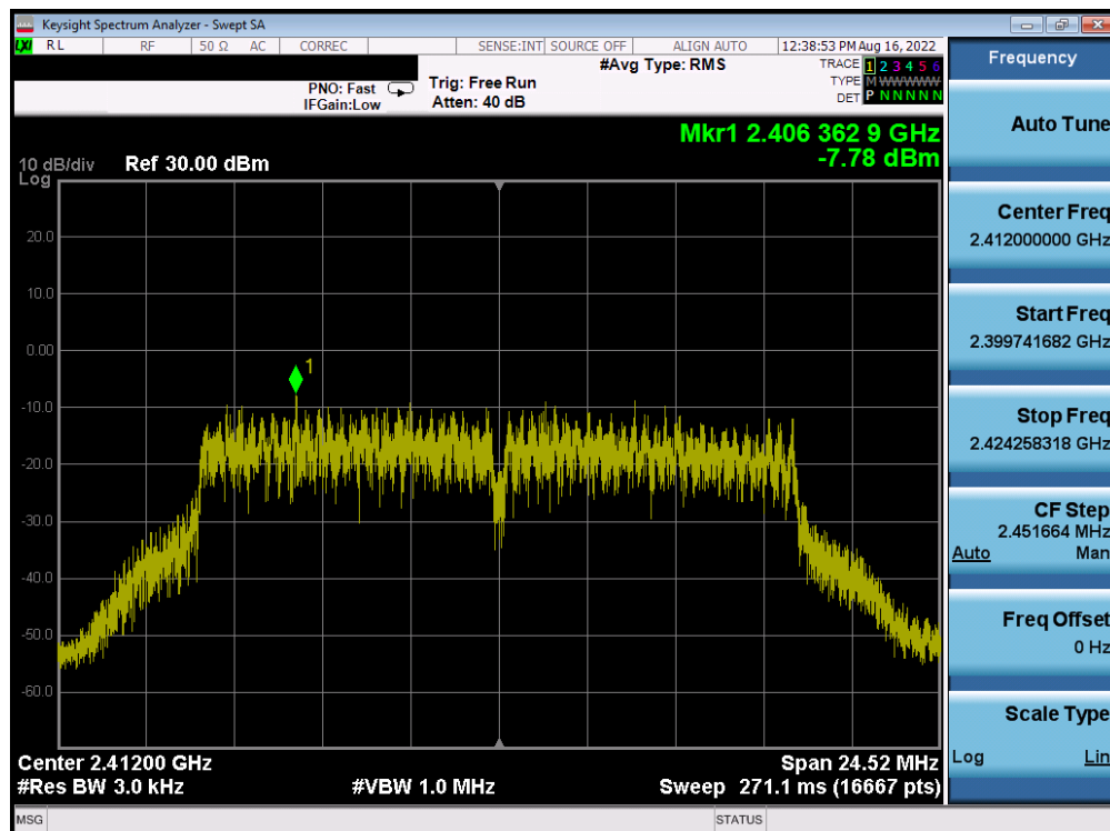
Plot 7-82. Power Spectral Density Plot Antenna WF8 (802.11g – Ch. 1) – 36Mbps
