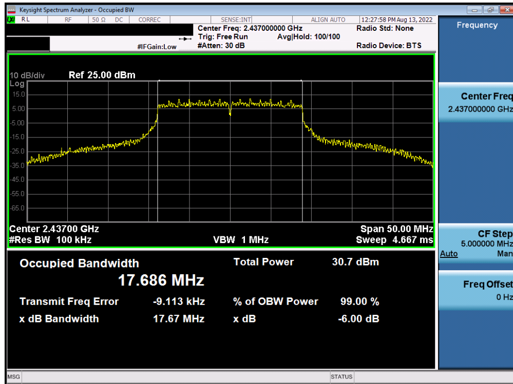
Plot 7-56. 6dB BW and 99% OBW Plot Antenna WF7b (802.11n (2.4GHz) – Ch. 6) – MCS5
