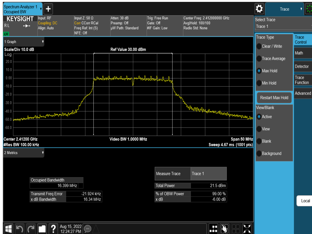
Plot 7-22. 6dB BW and 99% OBW Plot Antenna WF8 (802.11g – Ch. 1) – 36Mbps
