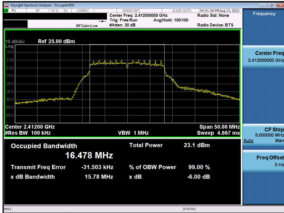
Plot 7-31. 6dB BW and 99% OBW Plot Antenna WF7b (802.11g – Ch. 1) – 12Mbps
