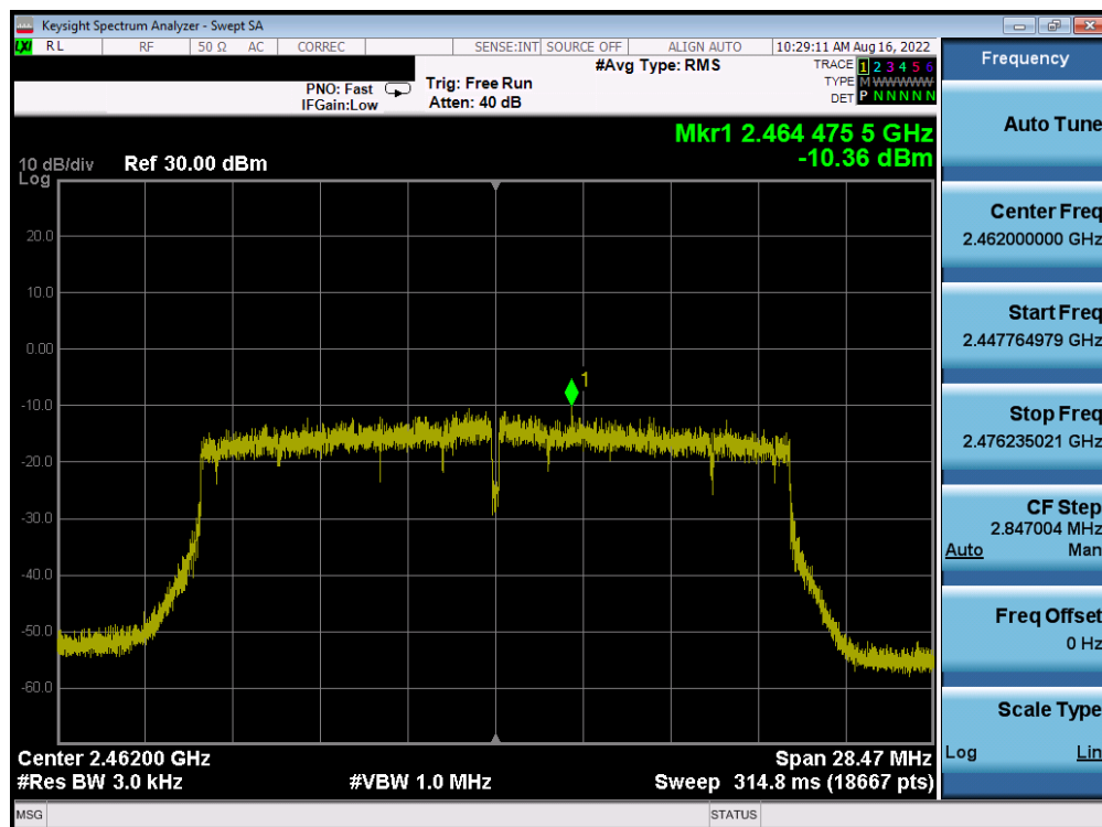
Plot 7-78. Power Spectral Density Plot Antenna WF8 (802.11ax (SU - 2.4GHz) – Ch. 11) – MCS4
