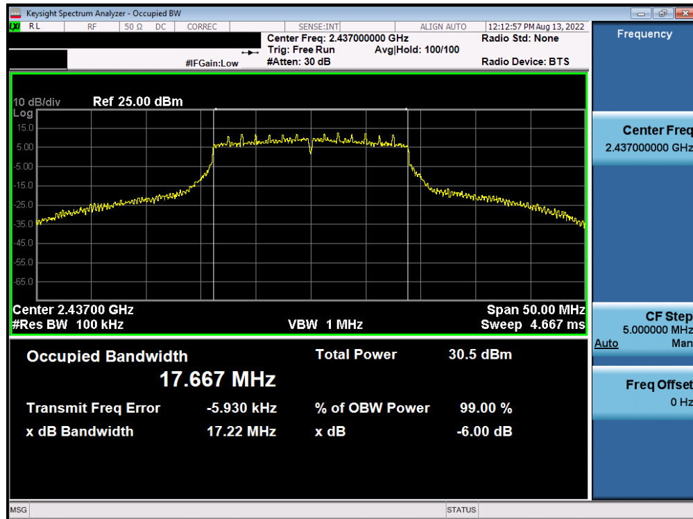
Plot 7-35. 6dB BW and 99% OBW Plot Antenna WF7b (802.11n (2.4GHz) – Ch. 6) – MCS2
