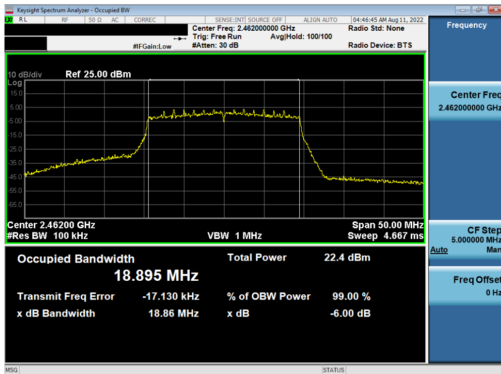
Plot 7-39. 6dB BW and 99% OBW Plot Antenna WF7b (802.11ax (SU - 2.4GHz) – Ch. 11) – MCS2
