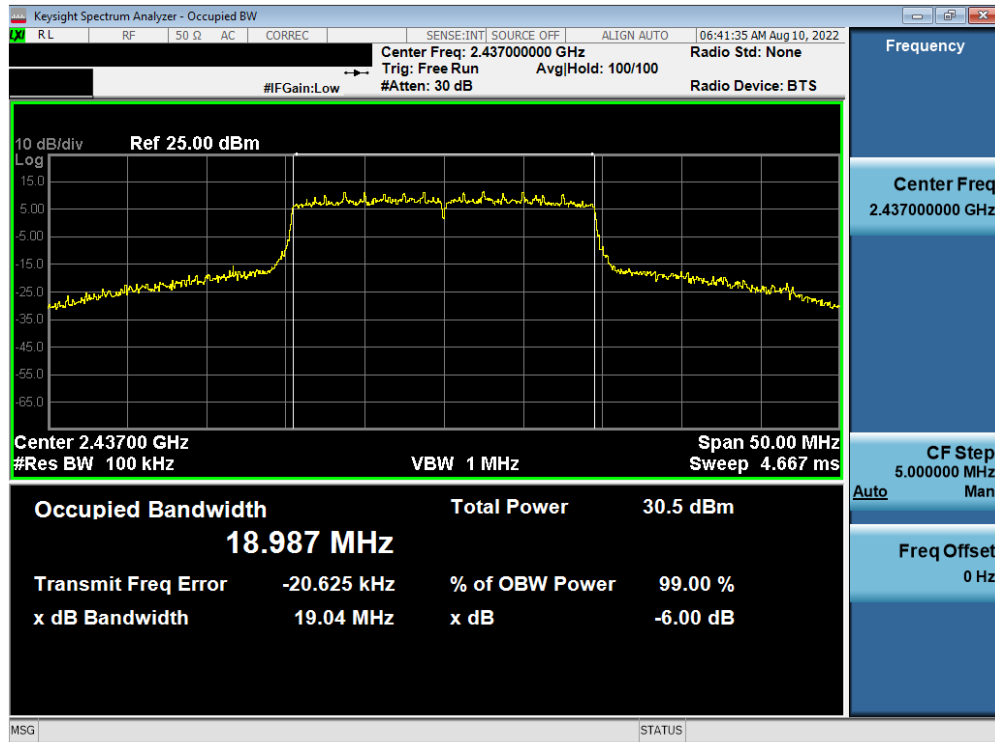
Plot 7-29. 6dB BW and 99% OBW Plot Antenna WF8 (802.11ax (SU - 2.4GHz) – Ch. 6) – MCS5
