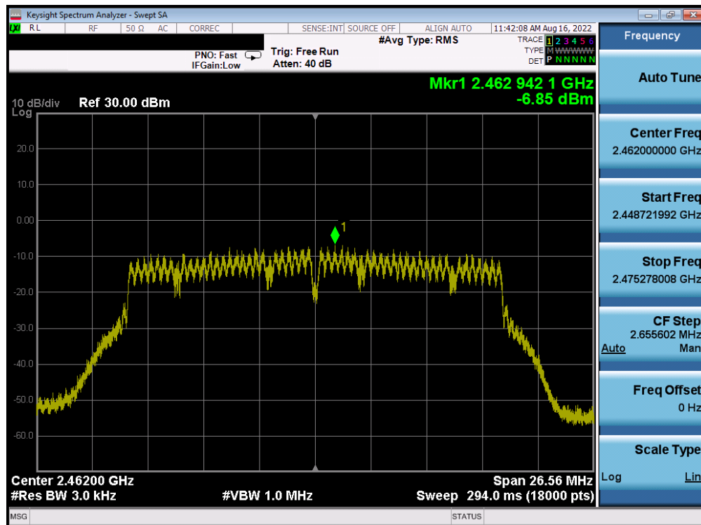
Plot 7-75. Power Spectral Density Plot Antenna WF8 (802.11n (2.4GHz) – Ch. 11) – MCS4
