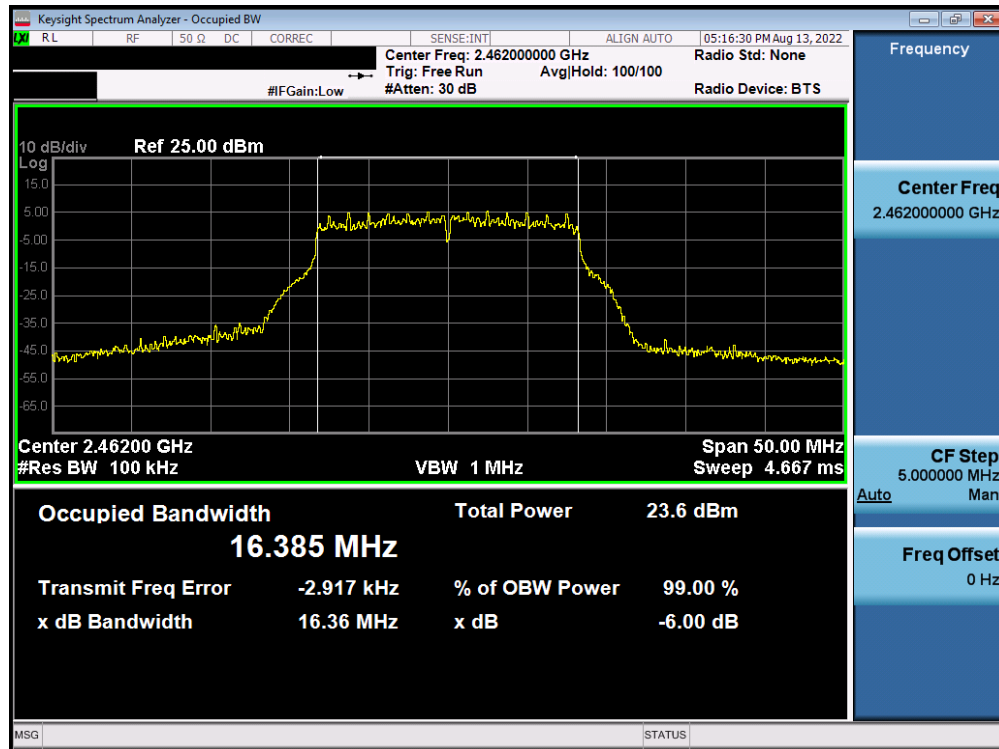
Plot 7-54. 6dB BW and 99% OBW Plot Antenna WF7b (802.11g – Ch. 11) – 36Mbps
