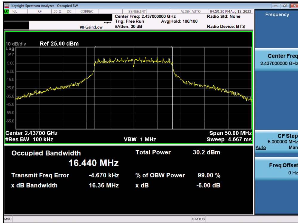
Plot 7-53. 6dB BW and 99% OBW Plot Antenna WF7b (802.11g – Ch. 6) – 36Mbps
