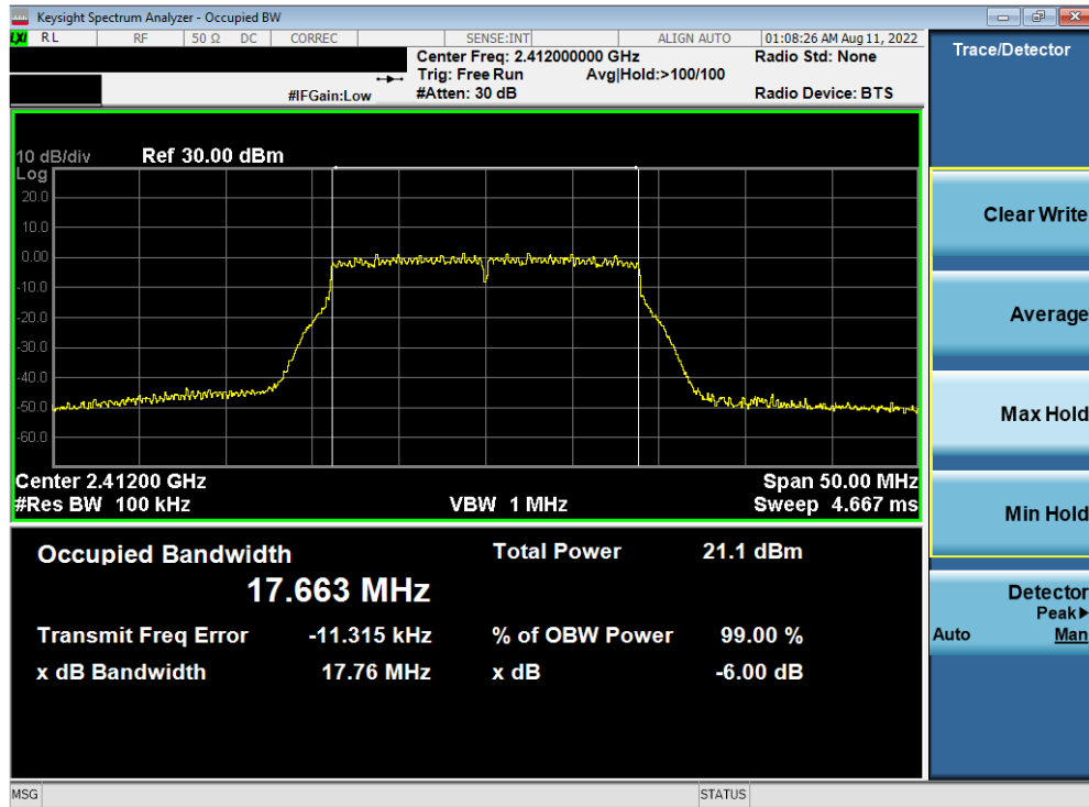
Plot 7-25. 6dB BW and 99% OBW Plot Antenna WF8 (802.11n (2.4GHz) – Ch. 1) – MCS5
