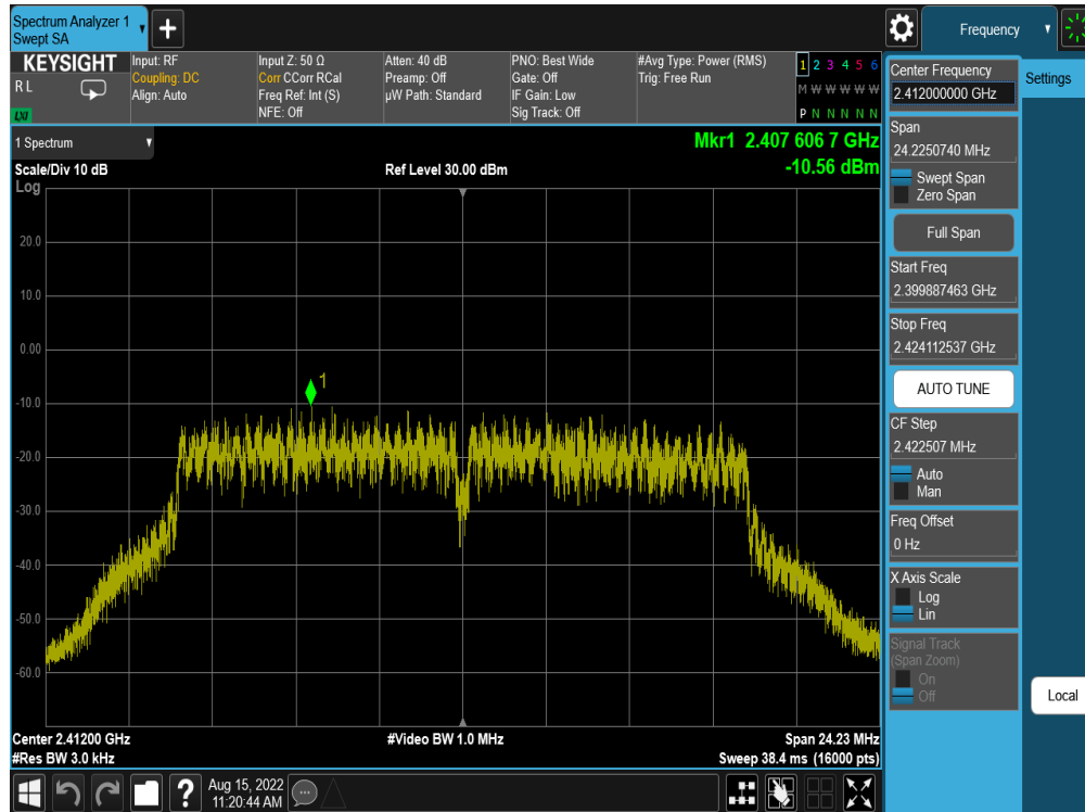
Plot 7-70. Power Spectral Density Plot Antenna WF8 (802.11g – Ch. 1) – 24Mbps
