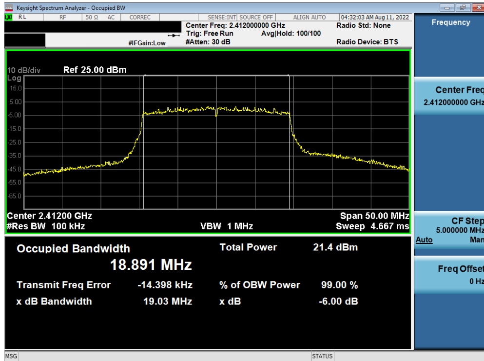
Plot 7-46. 6dB BW and 99% OBW Plot Antenna WF7b (802.11ax (SU - 2.4GHz) – Ch. 1) – MCS4
