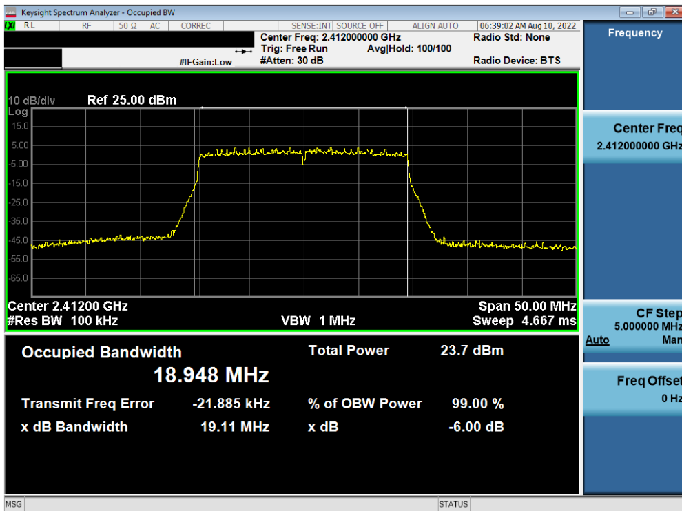
Plot 7-28. 6dB BW and 99% OBW Plot Antenna WF8 (802.11ax (SU - 2.4GHz) – Ch. 1) – MCS5
