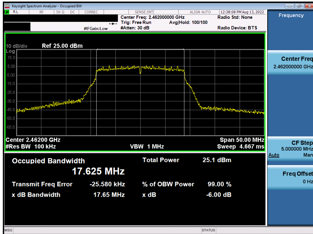
Plot 7-45. 6dB BW and 99% OBW Plot Antenna WF7b (802.11n (2.4GHz) – Ch. 11) – MCS4
