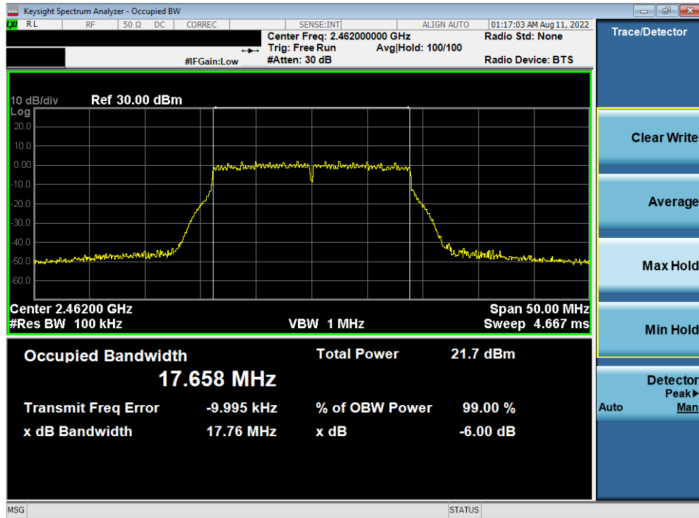
Plot 7-27. 6dB BW and 99% OBW Plot Antenna WF8 (802.11n (2.4GHz) – Ch. 11) – MCS5
