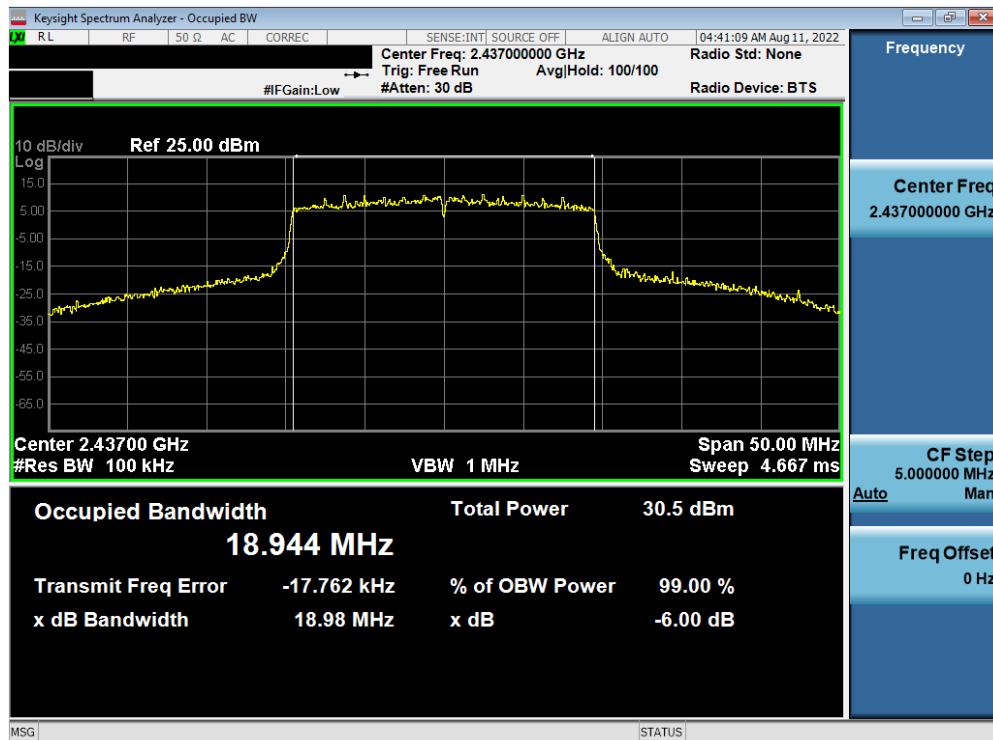
Plot 7-47. 6dB BW and 99% OBW Plot Antenna WF7b (802.11ax (SU - 2.4GHz) – Ch. 6) – MCS4
