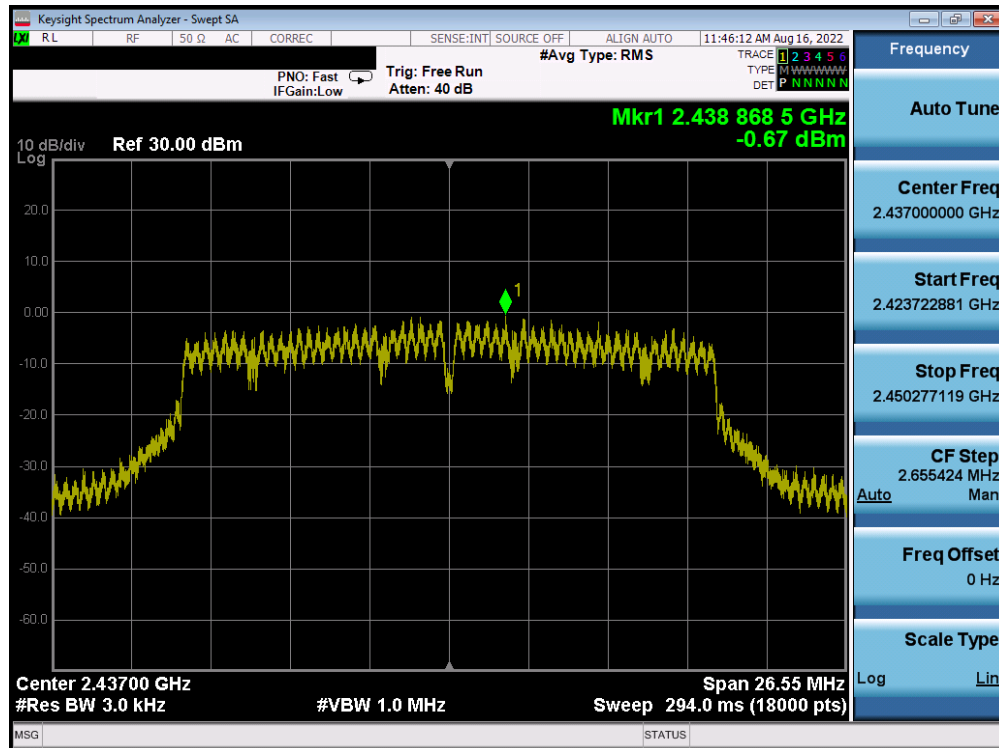
Plot 7-74. Power Spectral Density Plot Antenna WF8 (802.11n (2.4GHz) – Ch. 6) – MCS4
