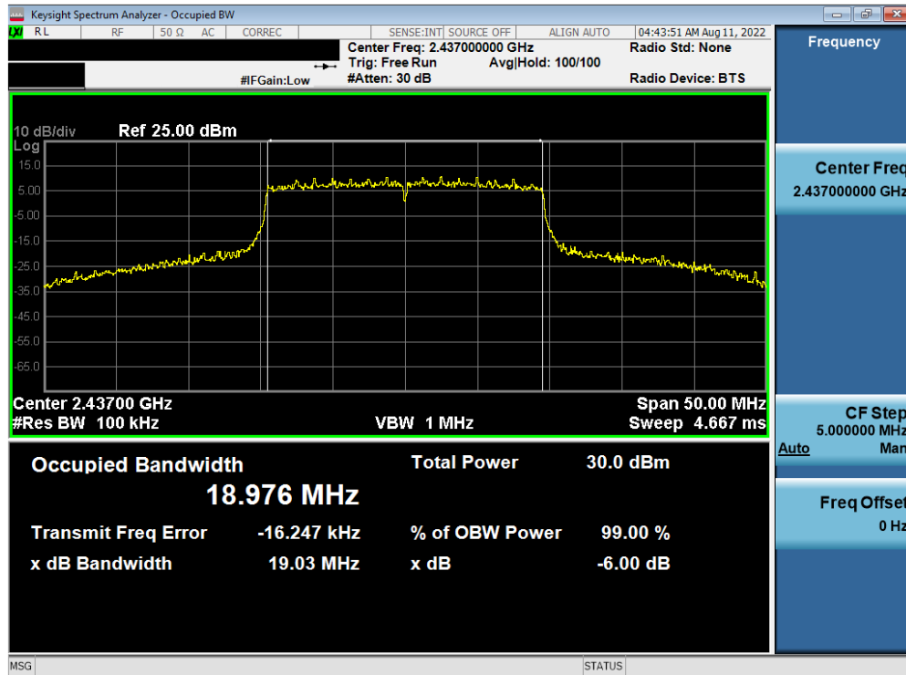
Plot 7-59. 6dB BW and 99% OBW Plot Antenna WF7b (802.11ax (SU - 2.4GHz) – Ch. 6) – MCS5
