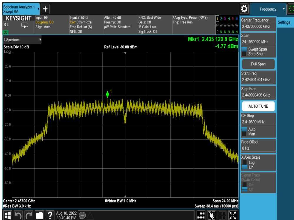
Plot 7-62. Power Spectral Density Plot Antenna WF8 (802.11g - Ch. 6) - 12Mbps
