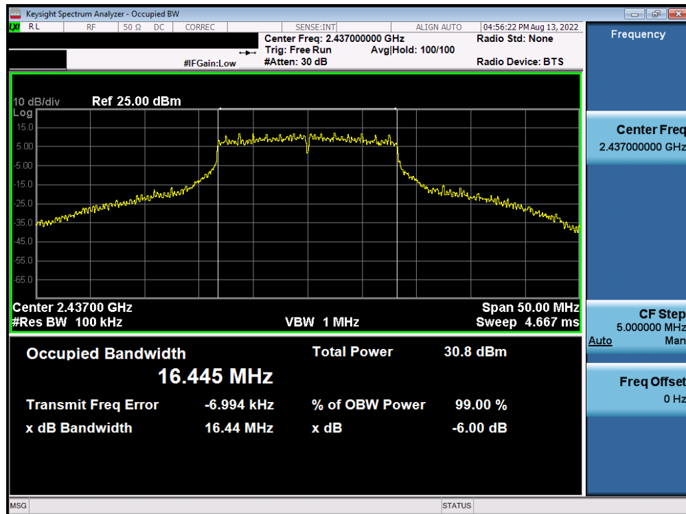
Plot 7-41. 6dB BW and 99% OBW Plot Antenna WF7b (802.11g – Ch. 6) – 24Mbps
