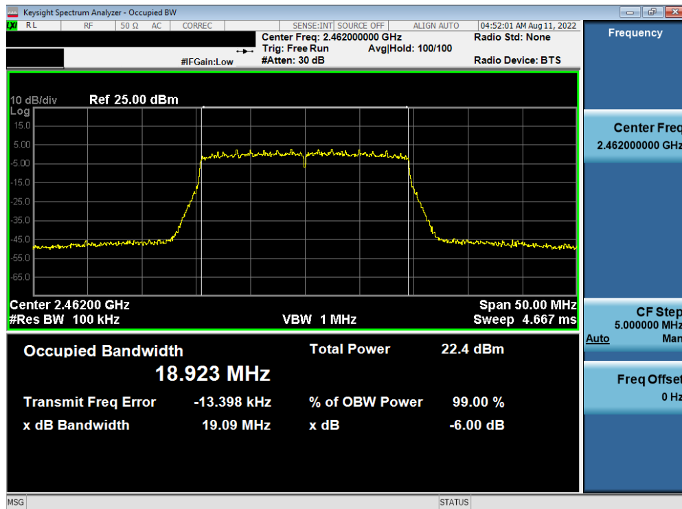
Plot 7-60. 6dB BW and 99% OBW Plot Antenna WF7b (802.11ax (SU - 2.4GHz) – Ch. 11) – MCS5
