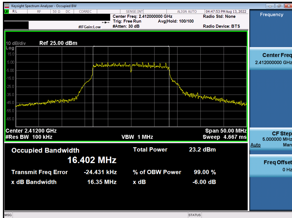
Plot 7-52. 6dB BW and 99% OBW Plot Antenna WF7b (802.11g – Ch. 1) – 36Mbps
