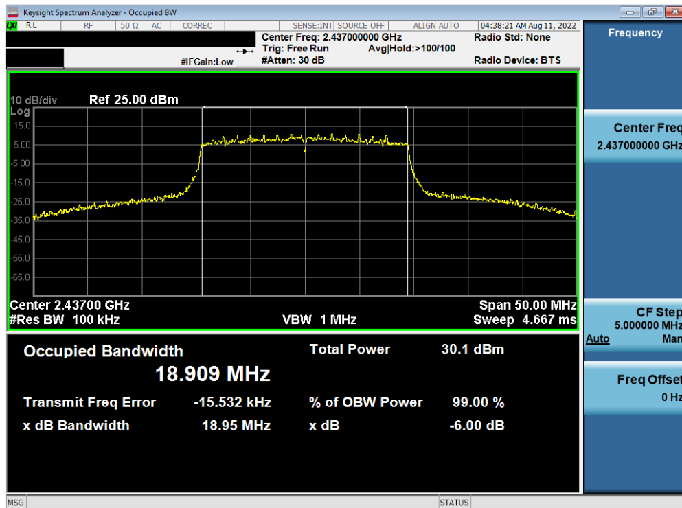
Plot 7-38. 6dB BW and 99% OBW Plot Antenna WF7b (802.11ax (SU - 2.4GHz) – Ch. 6) – MCS2
