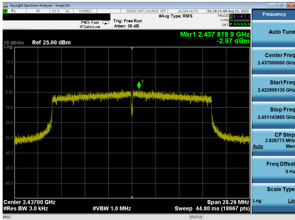
Plot 7-68. Power Spectral Density Plot Antenna WF8 (802.11ax (SU - 2.4GHz) – Ch. 6) – MCS2
