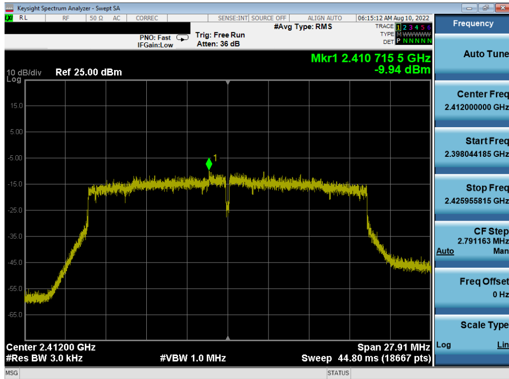
Plot 7-67. Power Spectral Density Plot Antenna WF8 (802.11ax (SU - 2.4GHz) – Ch. 1) – MCS2
