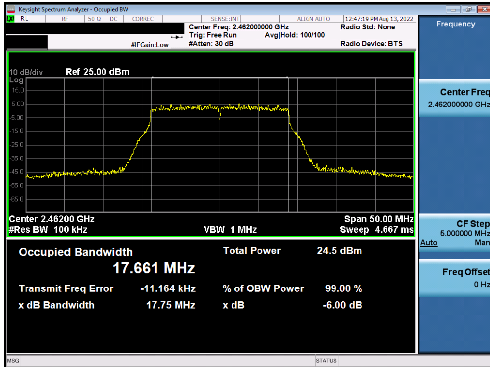
Plot 7-57. 6dB BW and 99% OBW Plot Antenna WF7b (802.11n (2.4GHz) – Ch. 11) – MCS5
