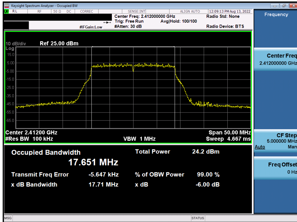
Plot 7-55. 6dB BW and 99% OBW Plot Antenna WF7b (802.11n (2.4GHz) – Ch. 1) – MCS5
