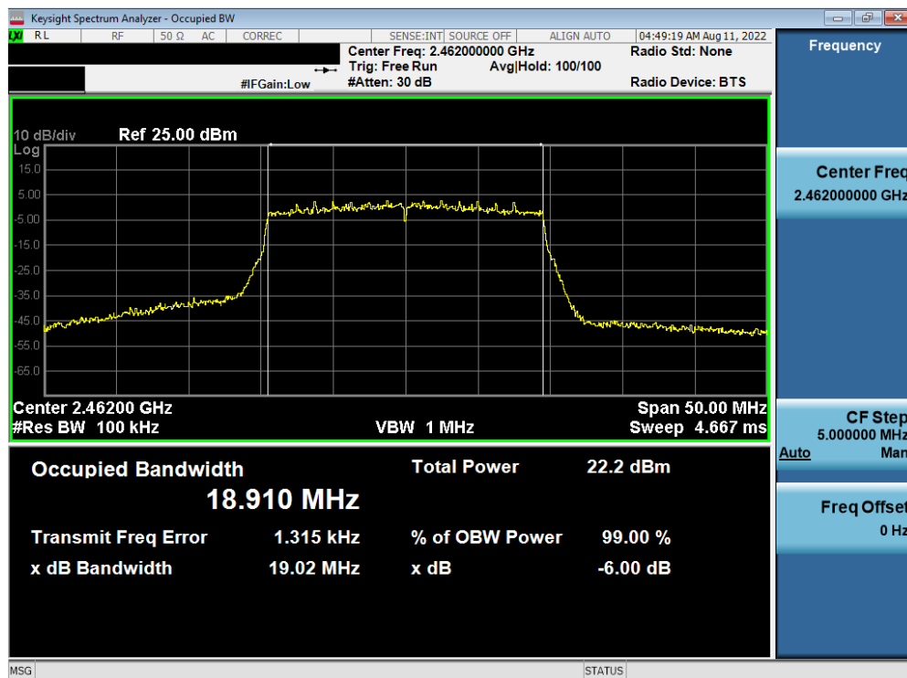
Plot 7-48. 6dB BW and 99% OBW Plot Antenna WF7b (802.11ax (SU - 2.4GHz) – Ch. 11) – MCS4
