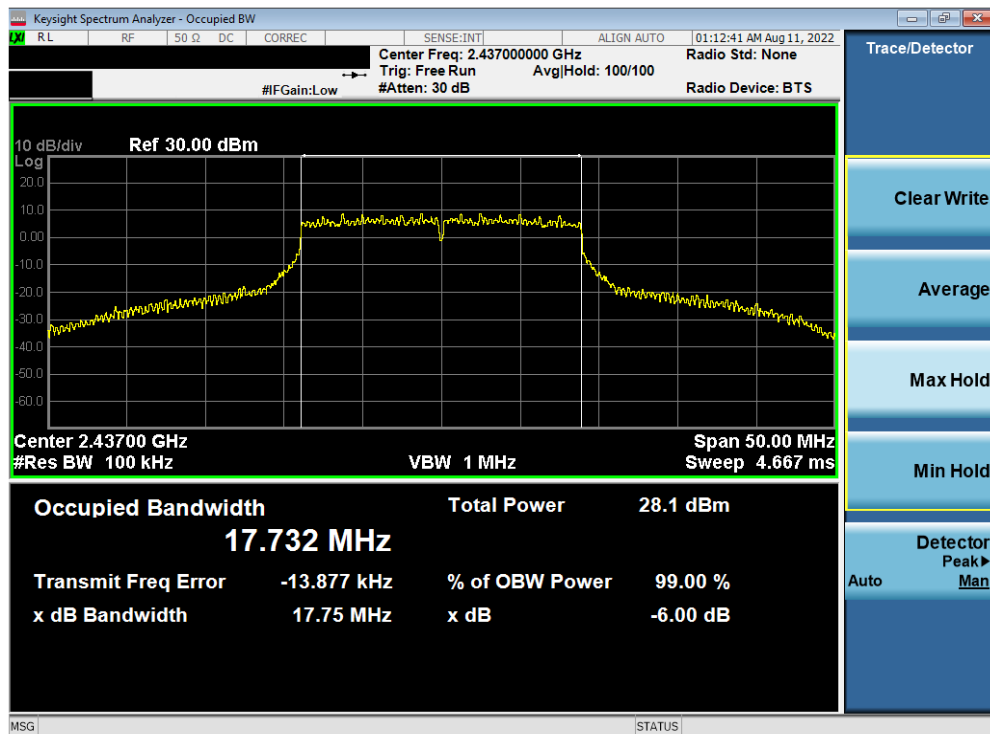
Plot 7-26. 6dB BW and 99% OBW Plot Antenna WF8 (802.11n (2.4GHz) – Ch. 6) – MCS5
