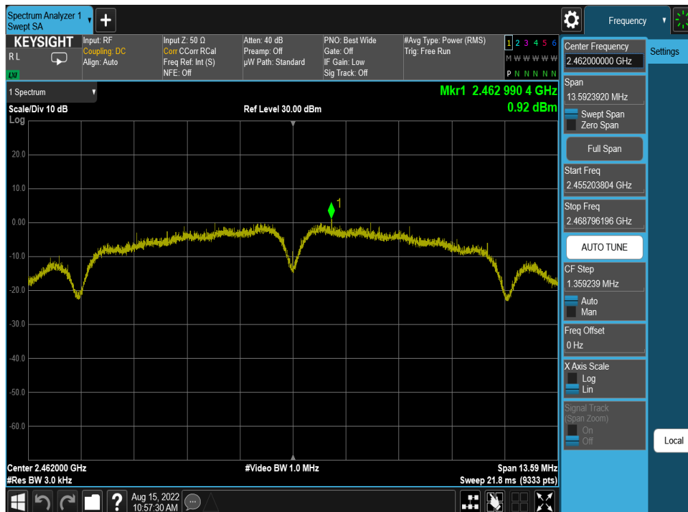
Plot 7-81. Power Spectral Density Plot Antenna WF8 (802.11b – Ch. 11) – 11Mbps
