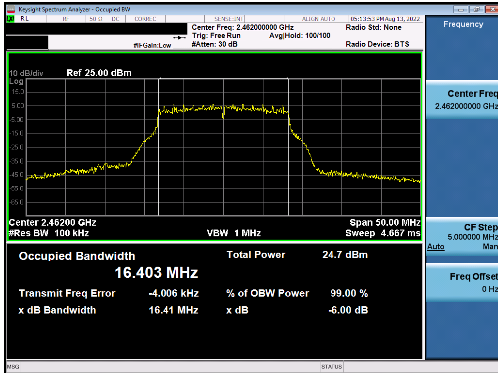
Plot 7-42. 6dB BW and 99% OBW Plot Antenna WF7b (802.11g – Ch. 11) – 24Mbps
