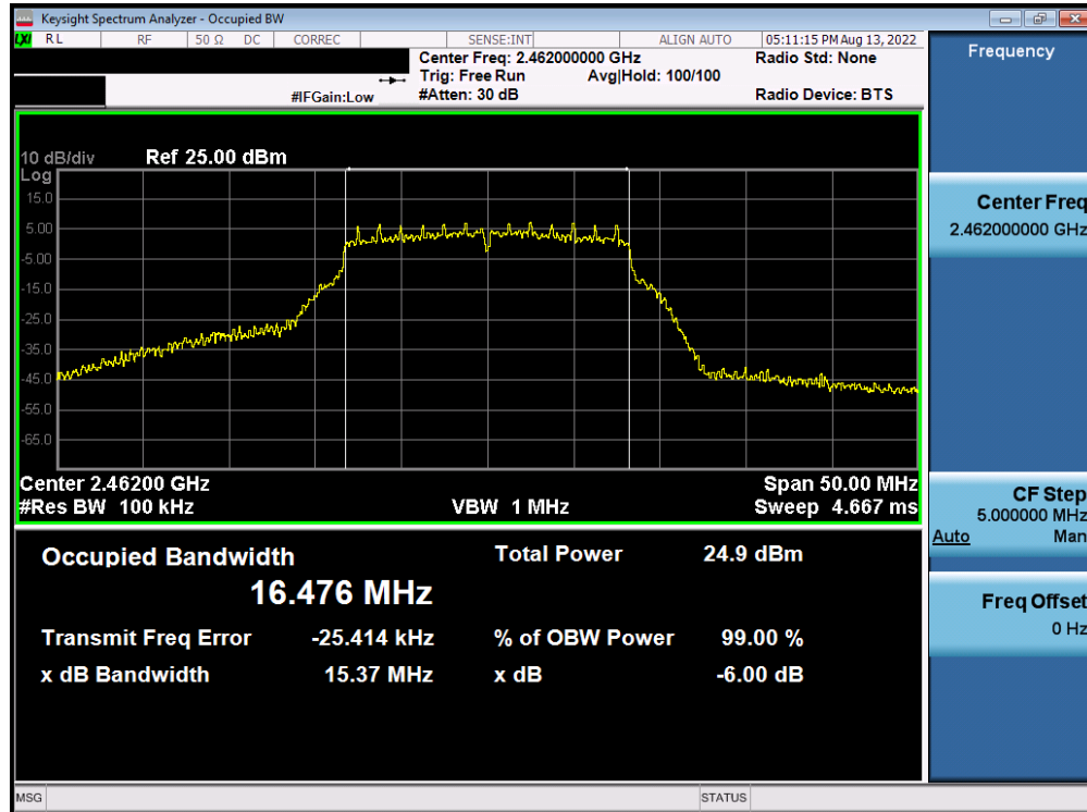
Plot 7-33. 6dB BW and 99% OBW Plot Antenna WF7b (802.11g – Ch. 11) – 12Mbps
