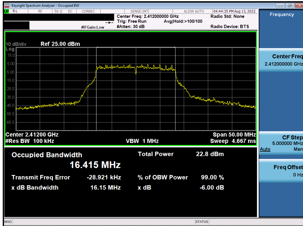
Plot 7-40. 6dB BW and 99% OBW Plot Antenna WF7b (802.11g – Ch. 1) – 24Mbps
