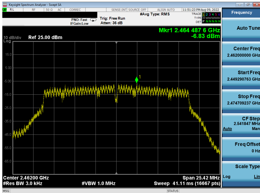
Plot 7-66. Power Spectral Density Plot Antenna WF8 (802.11n (2.4GHz) – Ch. 11) – MCS2
