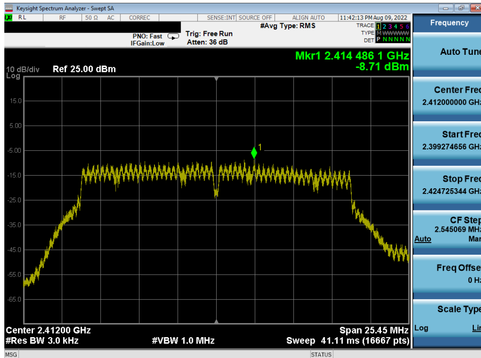
Plot 7-64. Power Spectral Density Plot Antenna WF8 (802.11n (2.4GHz) – Ch. 1) – MCS2
