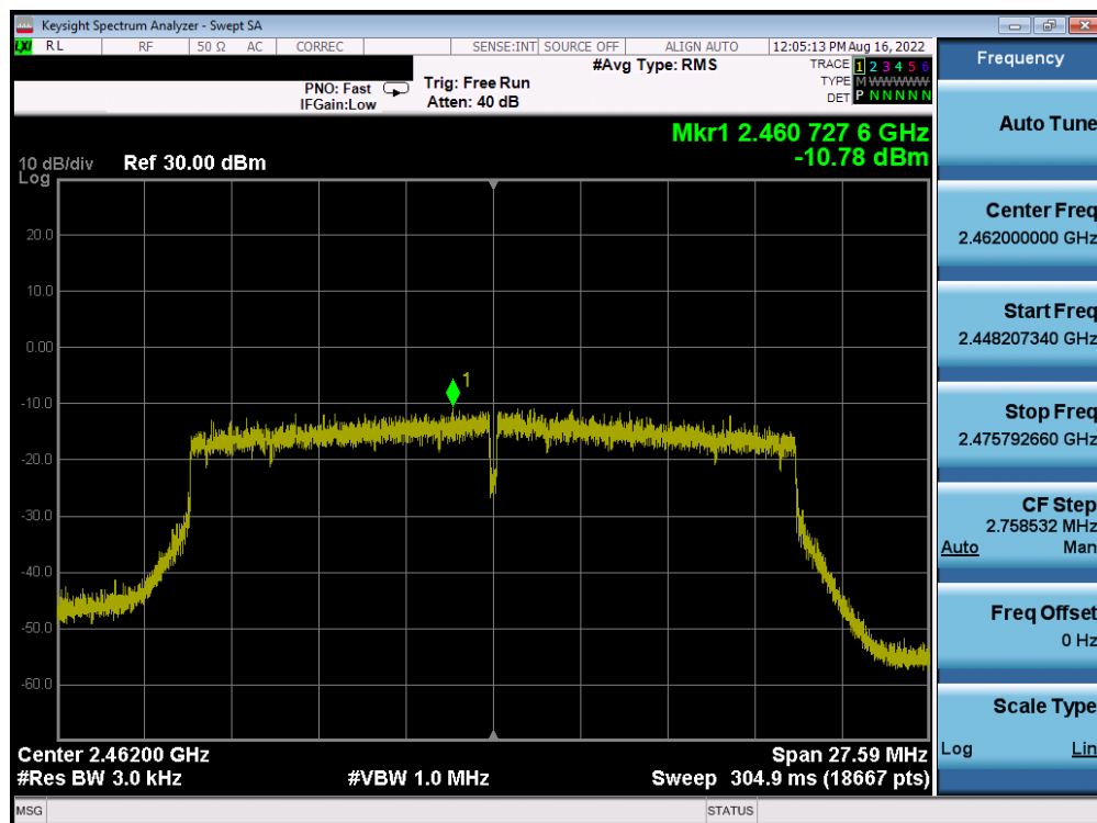
Plot 7-69. Power Spectral Density Plot Antenna WF8 (802.11ax (SU - 2.4GHz) – Ch. 11) – MCS2
