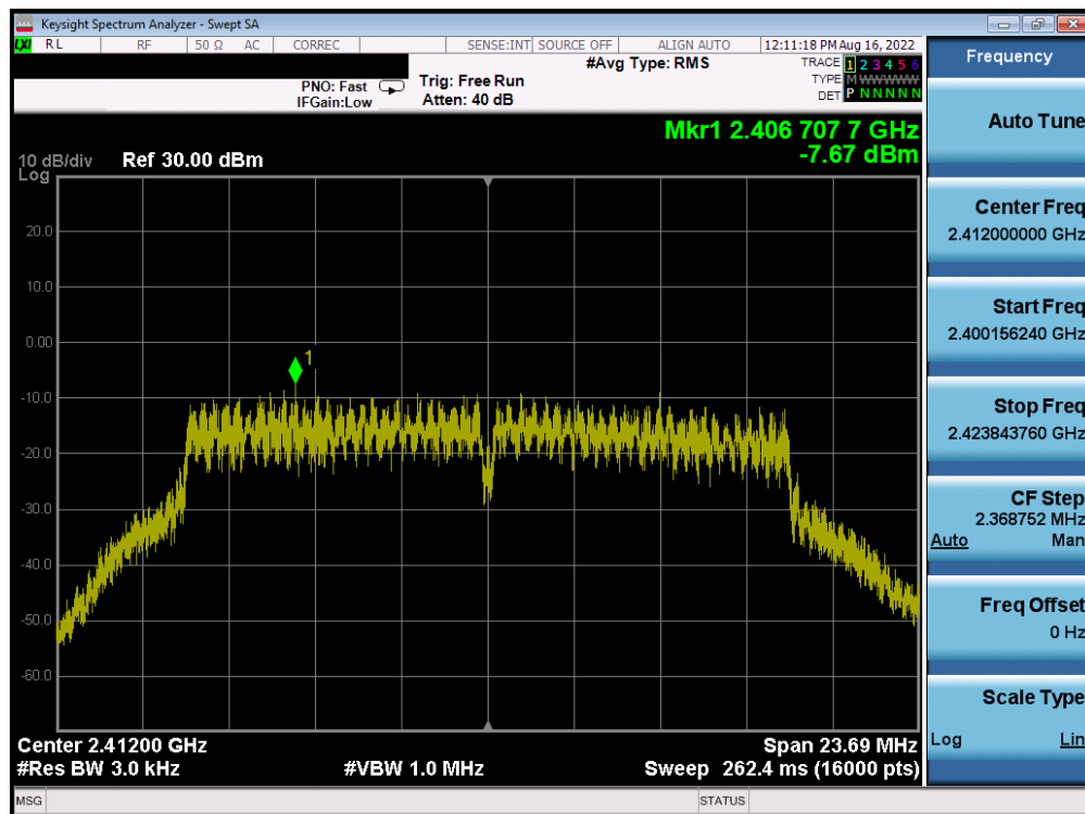
Plot 7-61. Power Spectral Density Plot Antenna WF8 (802.11g - Ch. 1) - 12Mbps
