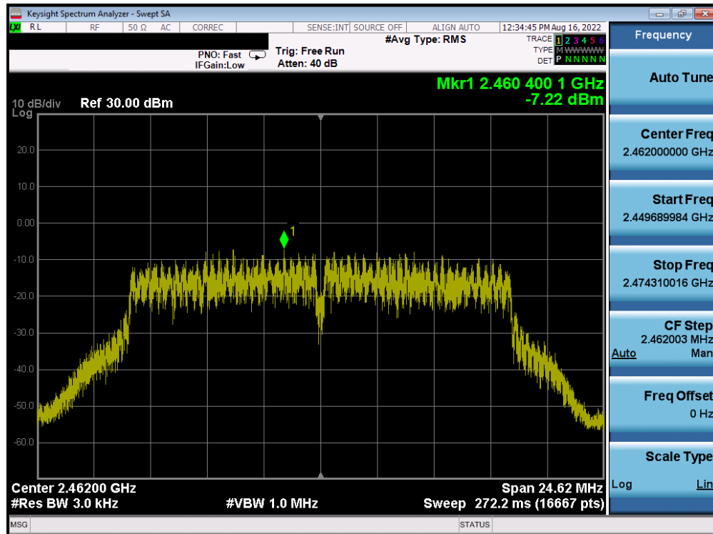
Plot 7-72. Power Spectral Density Plot Antenna WF8 (802.11g – Ch. 11) – 24Mbps
