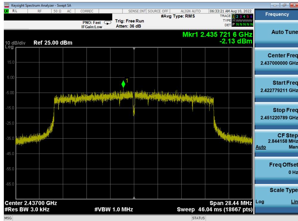
Plot 7-77. Power Spectral Density Plot Antenna WF8 (802.11ax (SU - 2.4GHz) – Ch. 6) – MCS4
