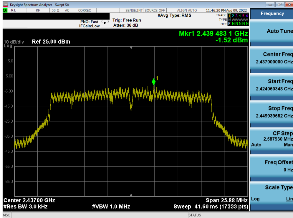
Plot 7-65. Power Spectral Density Plot Antenna WF8 (802.11n (2.4GHz) – Ch. 6) – MCS2
