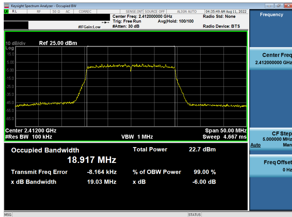
Plot 7-58. 6dB BW and 99% OBW Plot Antenna WF7b (802.11ax (SU - 2.4GHz) – Ch. 1) – MCS5
