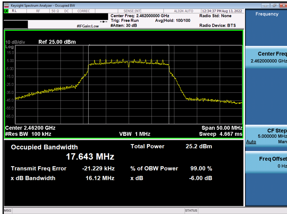
Plot 7-36. 6dB BW and 99% OBW Plot Antenna WF7b (802.11n (2.4GHz) – Ch. 11) – MCS2
