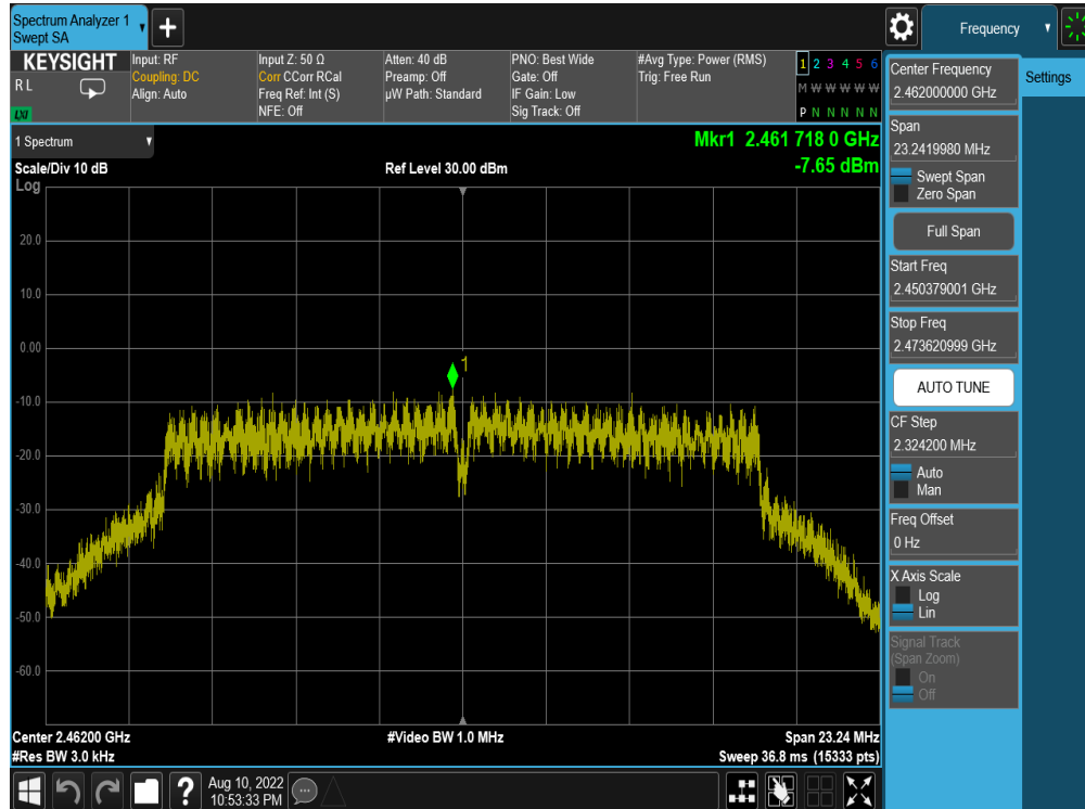
Plot 7-63. Power Spectral Density Plot Antenna WF8 (802.11g – Ch. 11) – 12Mbps
