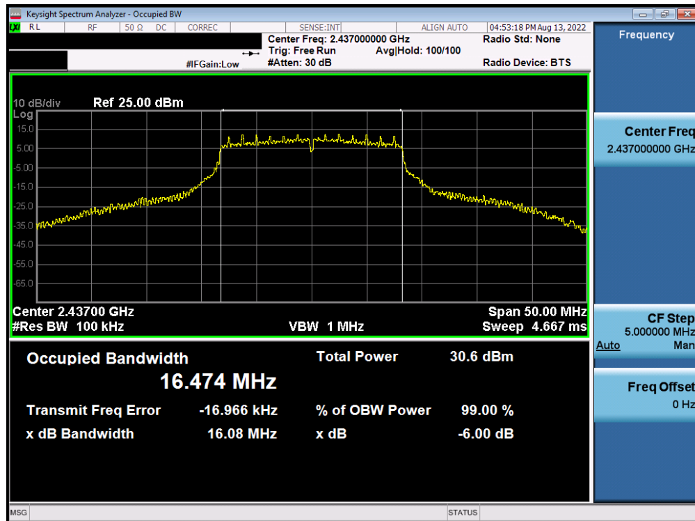
Plot 7-32. 6dB BW and 99% OBW Plot Antenna WF7b (802.11g – Ch. 6) – 12Mbps
