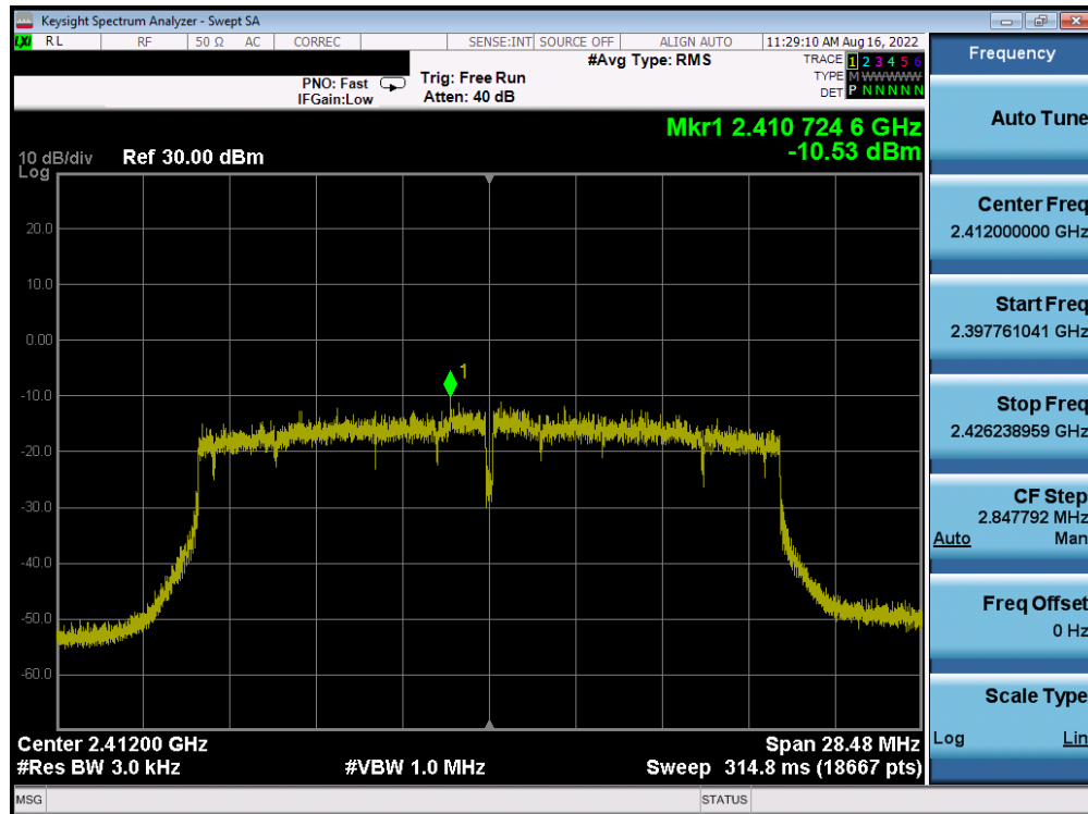
Plot 7-76. Power Spectral Density Plot Antenna WF8 (802.11ax (SU - 2.4GHz) – Ch. 1) – MCS4
