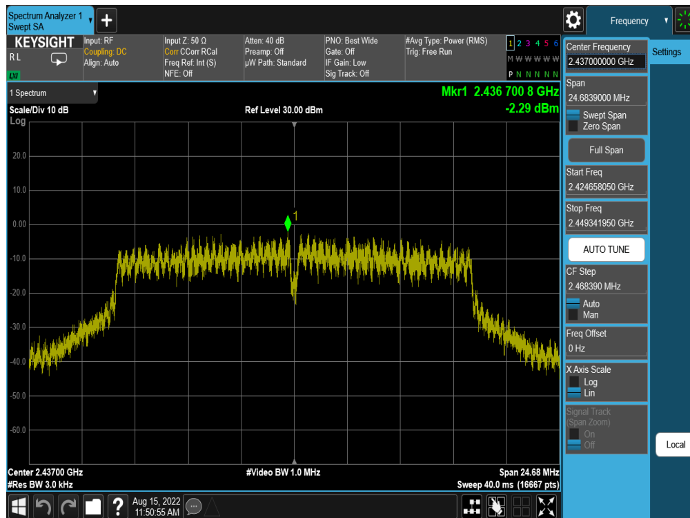
Plot 7-71. Power Spectral Density Plot Antenna WF8 (802.11g – Ch. 6) – 24Mbps
