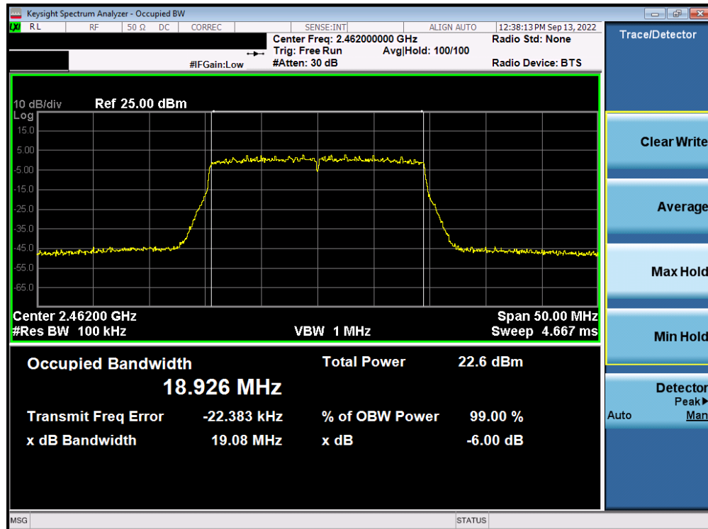
Plot 7-30. 6dB BW and 99% OBW Plot Antenna WF8 (802.11ax (SU - 2.4GHz) – Ch. 11) – MCS5
