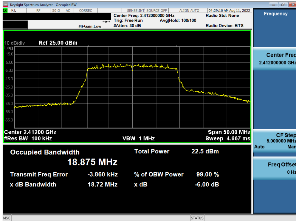
Plot 7-37. 6dB BW and 99% OBW Plot Antenna WF7b (802.11ax (SU - 2.4GHz) – Ch. 1) – MCS2
