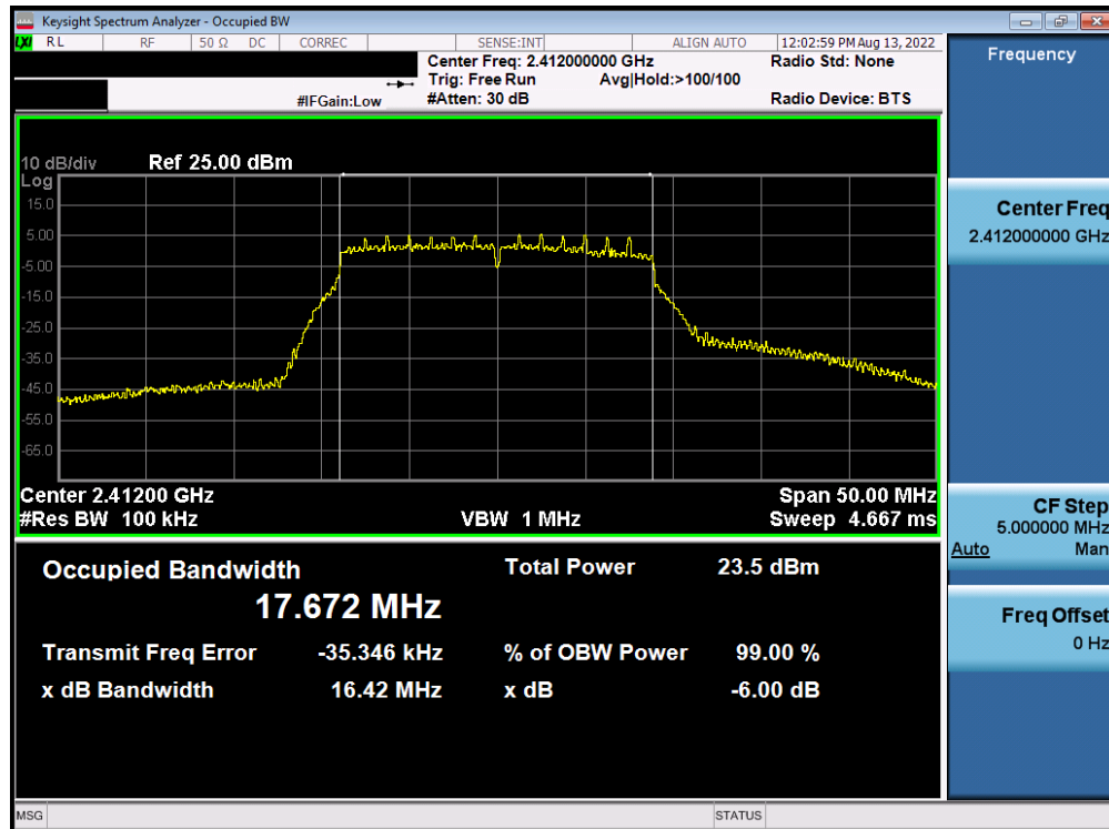
Plot 7-34. 6dB BW and 99% OBW Plot Antenna WF7b (802.11n (2.4GHz) – Ch. 1) – MCS2
