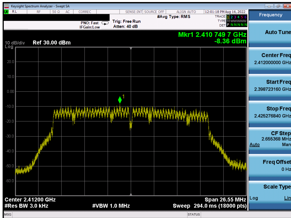
Plot 7-73. Power Spectral Density Plot Antenna WF8 (802.11n (2.4GHz) – Ch. 1) – MCS4
