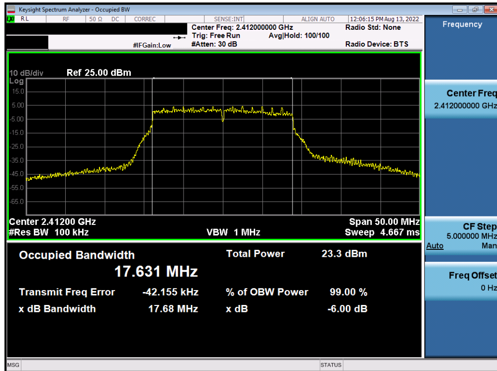
Plot 7-43. 6dB BW and 99% OBW Plot Antenna WF7b (802.11n (2.4GHz) – Ch. 1) – MCS4
