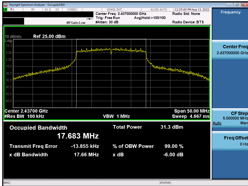
Plot 7-44. 6dB BW and 99% OBW Plot Antenna WF7b (802.11n (2.4GHz) – Ch. 6) – MCS4
