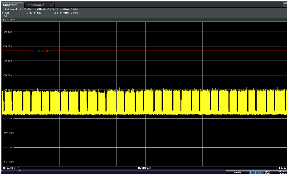
Figure 9-5. 5530MHz - Channel Loading - Mode 3 (80MHz)
