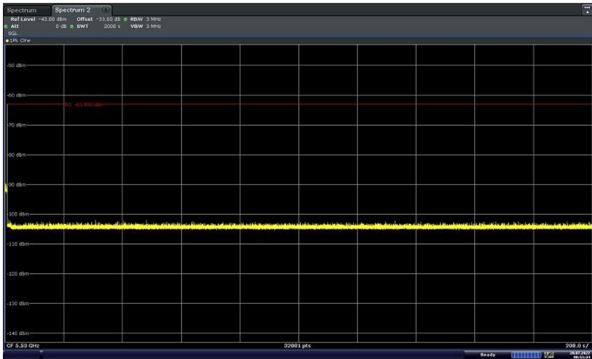
Figure 9-13. 5530MHz - Non-Occupancy Period (30 Minutes) - Mode 1 (80MHz)
