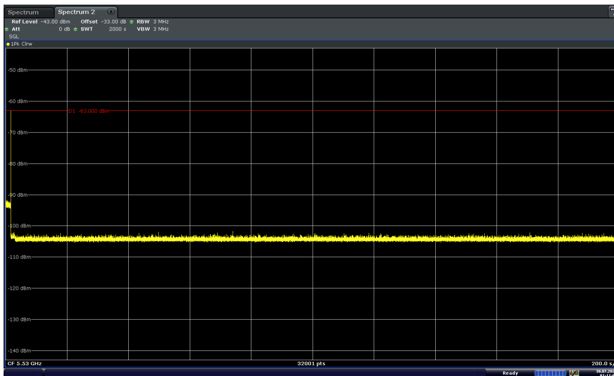
Figure 9-14. 5530MHz - Non-Occupancy Period (30 Minutes) - Mode 2 (80MHz)
