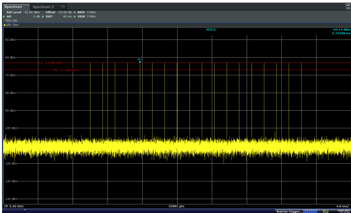
Figure 7-3. 5530MHz – Radar Pulse Type 0 (80MHz)
