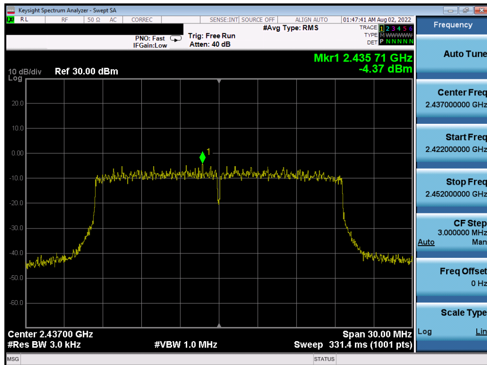
Plot 7-70. Power Spectral Density Plot CDD Antenna WF7b (802.11ax OFDMA – RU242 – Ch. 6)
