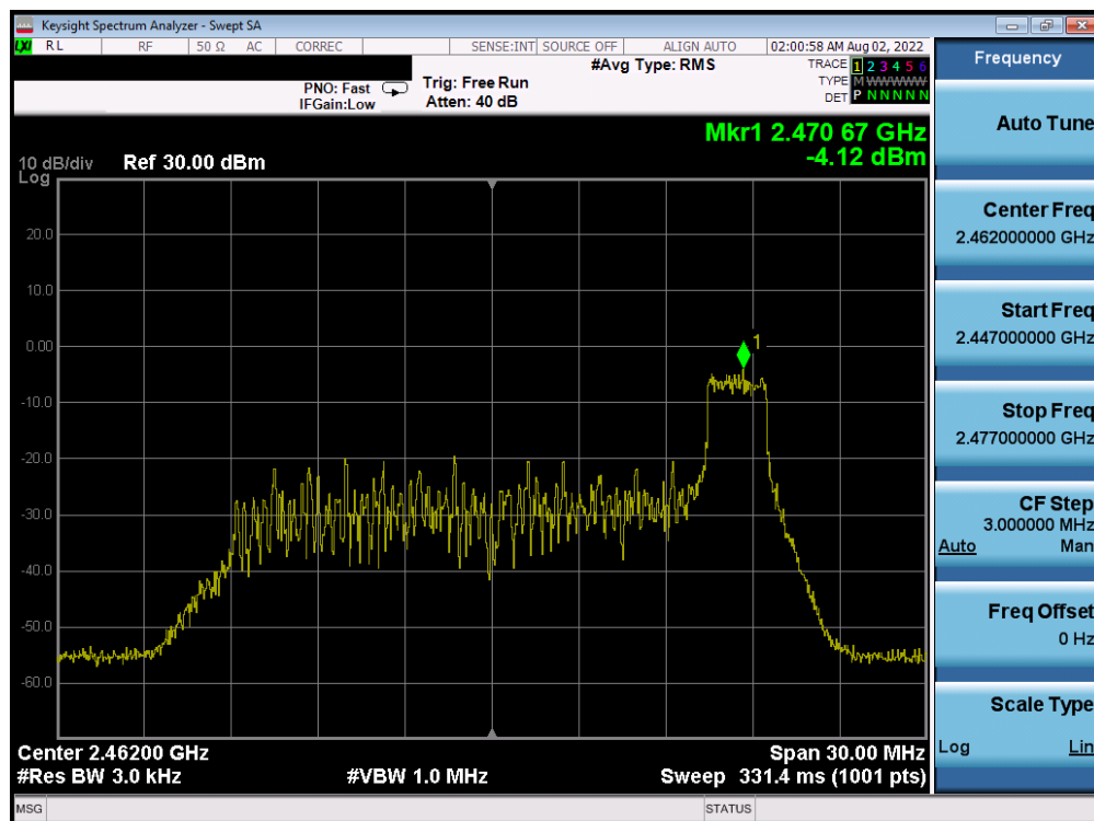
Plot 7-65. Power Spectral Density Plot CDD Antenna WF8 (802.11ax OFDMA – RU26 Index 8 – Ch. 11)
