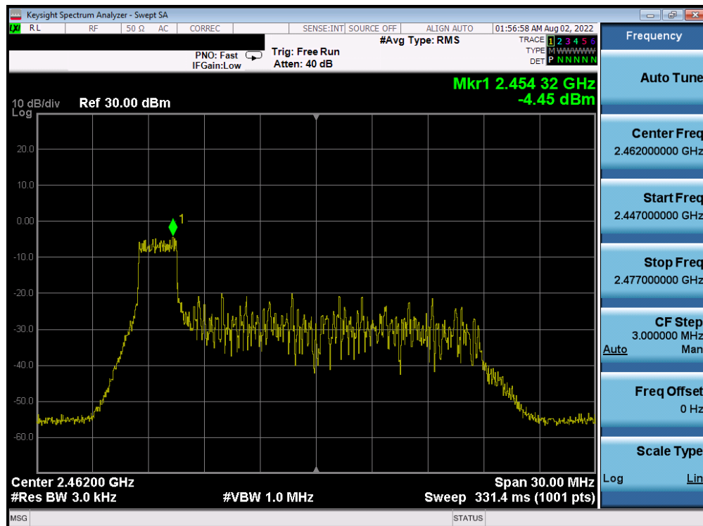
Plot 7-61. Power Spectral Density Plot CDD Antenna WF8 (802.11ax OFDMA – RU26 Index 0 – Ch. 11)
