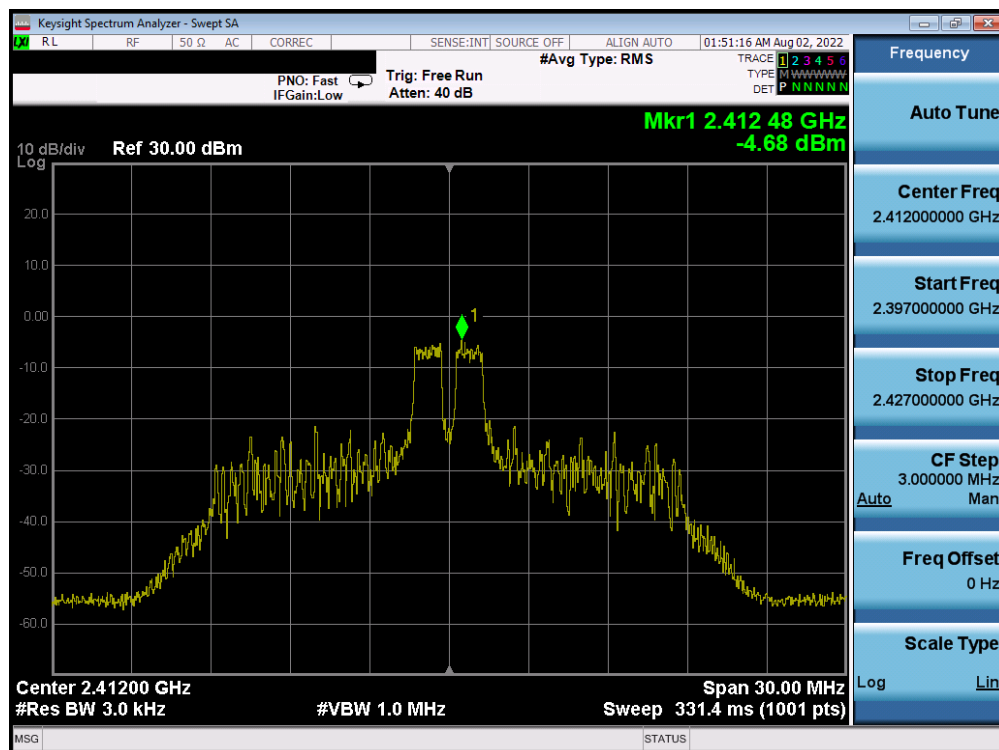
Plot 7-51. Power Spectral Density Plot CDD Antenna WF8 (802.11ax OFDMA – RU26 Index 4 – Ch. 1)
