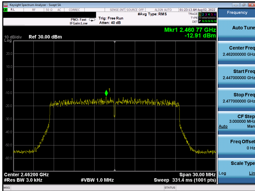
Plot 7-71. Power Spectral Density Plot CDD Antenna WF8 (802.11ax OFDMA – RU242 – Ch. 11)
