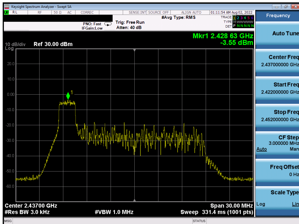
Plot 7-56. Power Spectral Density Plot CDD Antenna WF7b (802.11ax OFDMA – RU26 Index 0 – Ch. 6)
