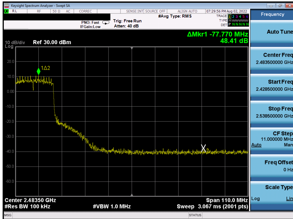
Plot 7-83. Band Edge Antenna WF8 (802.11ax OFDMA – RU242 – Ch. 6)
