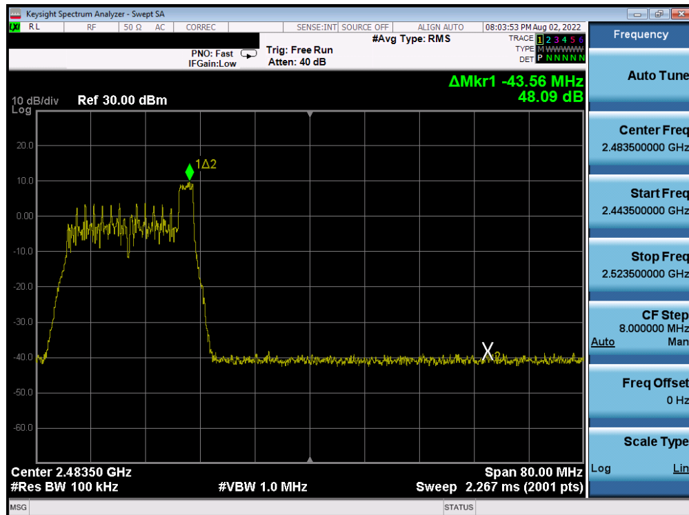
Plot 7-74. Band Edge Antenna WF8 (802.11ax OFDMA – RU26 Index 8 – Ch. 10)
