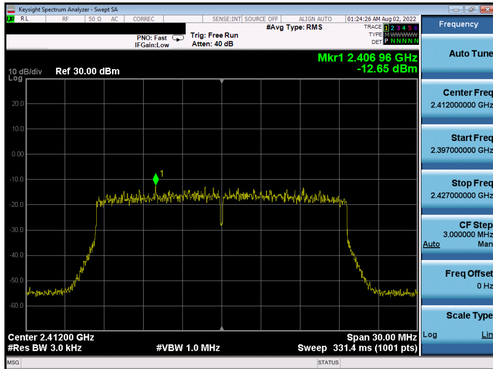
Plot 7-67. Power Spectral Density Plot CDD Antenna WF8 (802.11ax OFDMA – RU242 – Ch. 1)
