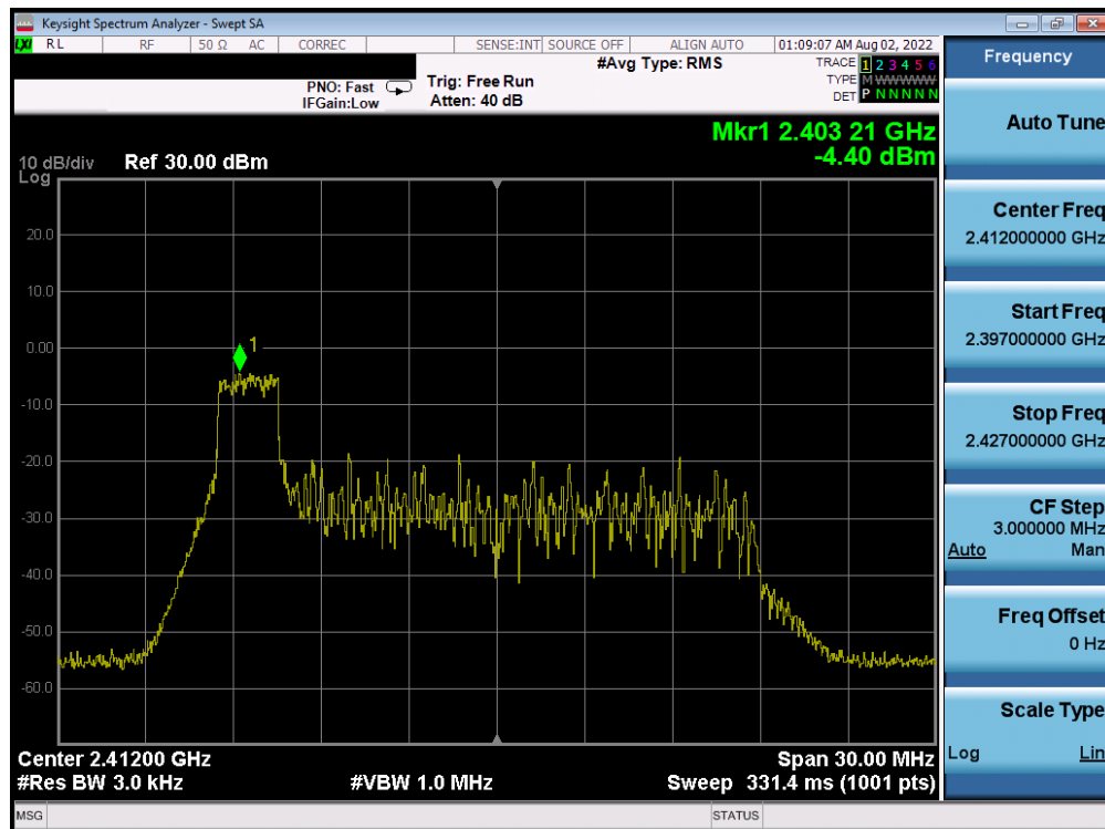
Plot 7-50. Power Spectral Density Plot CDD Antenna WF7b (802.11ax OFDMA – RU26 Index 0 – Ch. 1)
