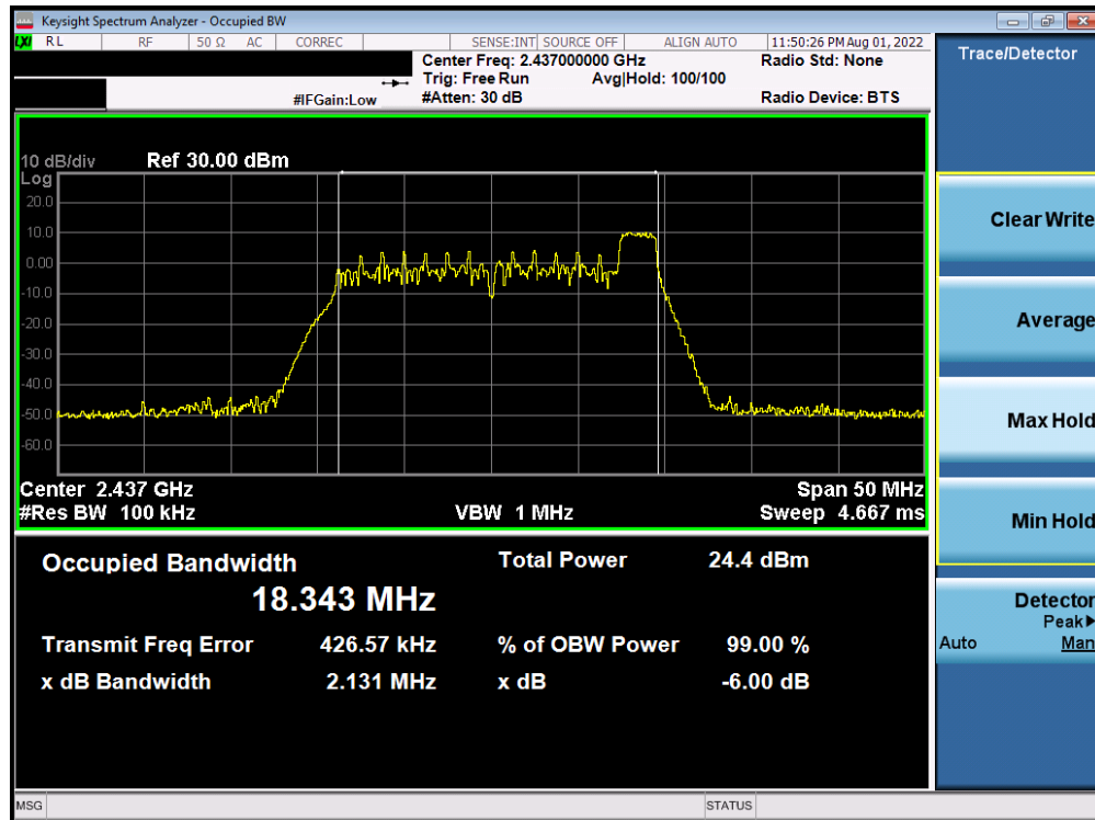
Plot 7-18. 6dB BW & 99% OBW Plot Antenna WF7b (802.11ax OFDMA – RU26 Index 8 – Ch. 6)
