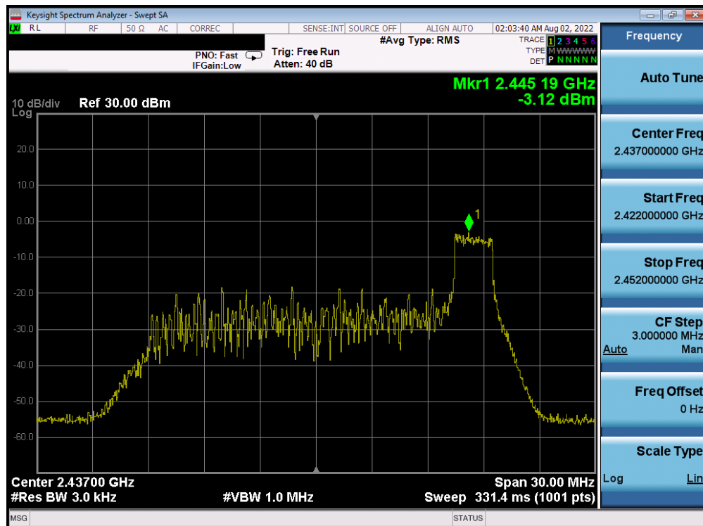
Plot 7-59. Power Spectral Density Plot CDD Antenna WF8 (802.11ax OFDMA – RU26 Index 8 – Ch. 6)
