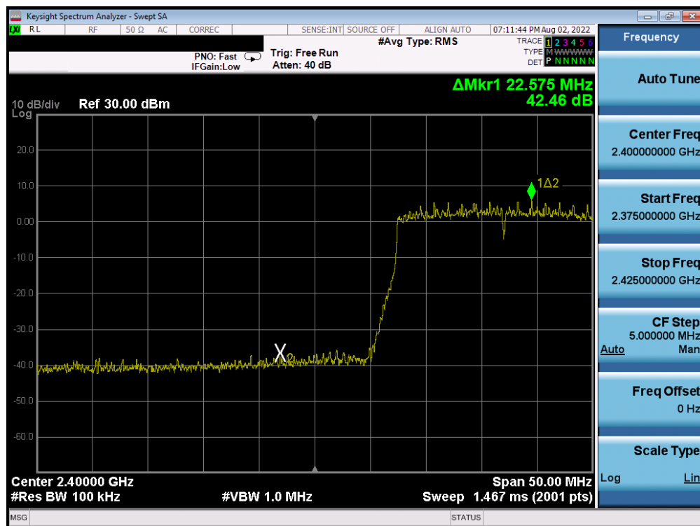
Plot 7-78. Band Edge Antenna WF8 (802.11ax OFDMA – RU242 – Ch. 2)
