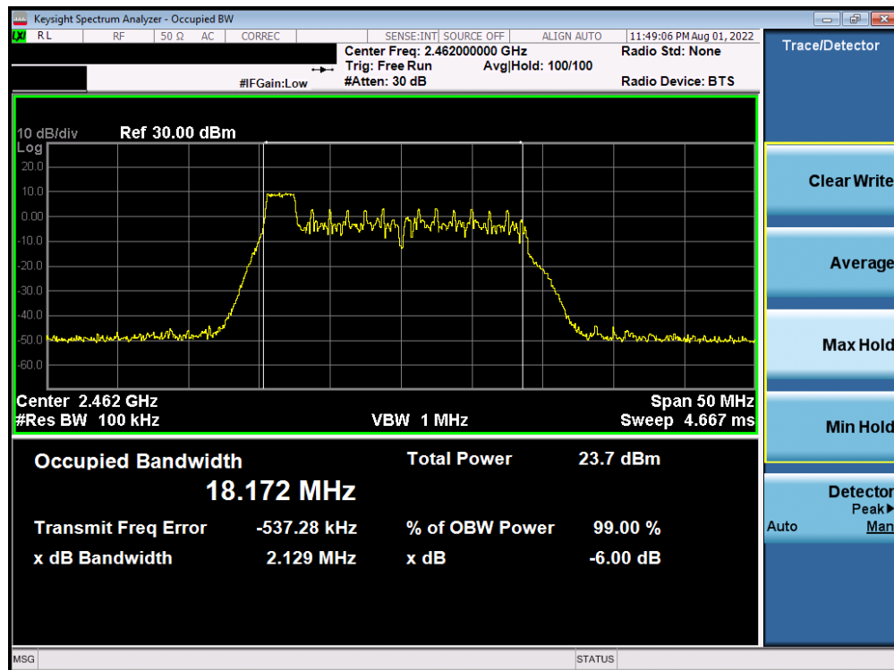
Plot 7-19. 6dB BW & 99% OBW Plot Antenna WF7b (802.11ax OFDMA – RU26 Index 0 – Ch. 11)
