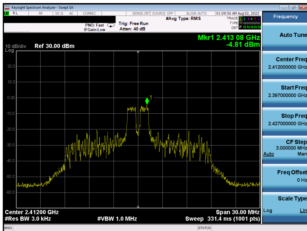
Plot 7-52. Power Spectral Density Plot CDD Antenna WF7b (802.11ax OFDMA – RU26 Index 4 – Ch. 1)
