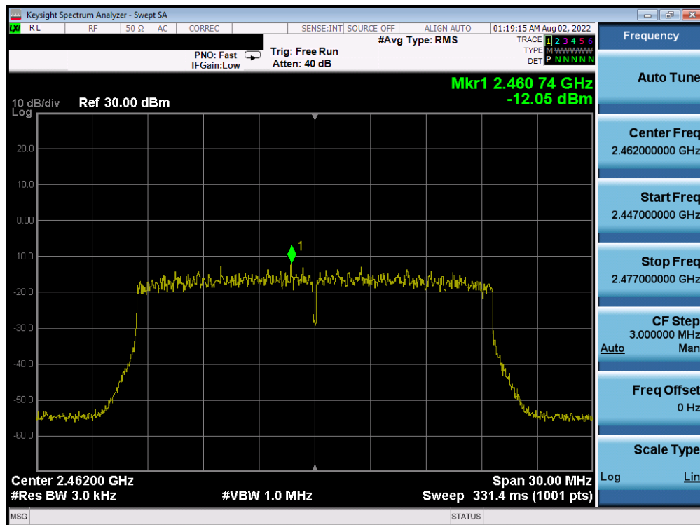
Plot 7-72. Power Spectral Density Plot CDD Antenna WF7b (802.11ax OFDMA – RU242 – Ch. 11)
