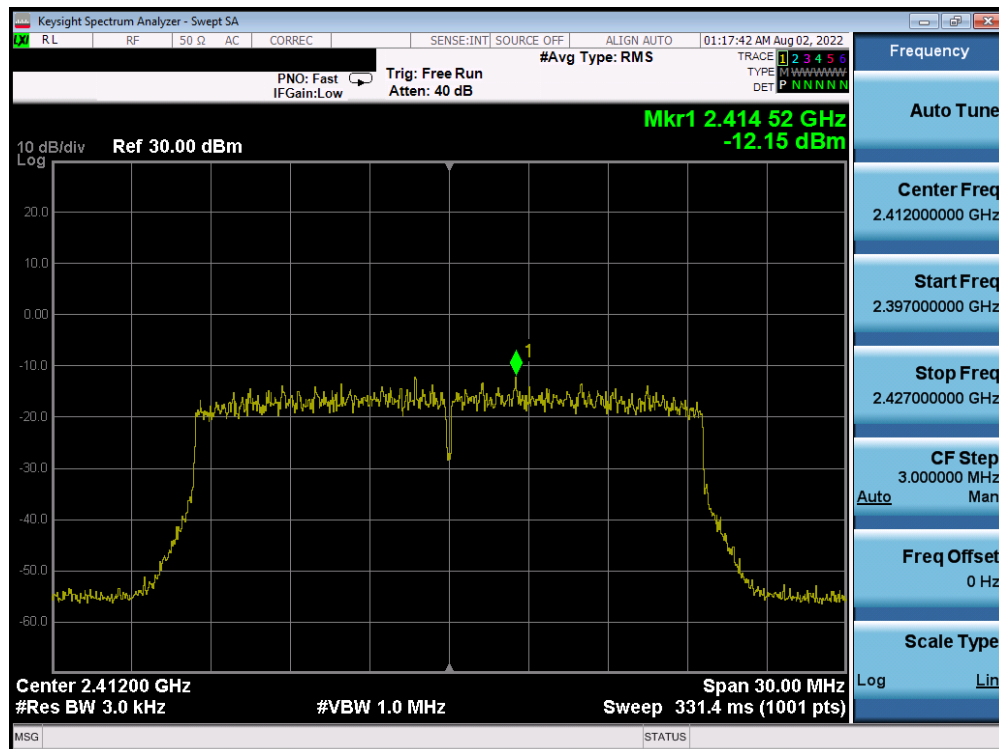
Plot 7-68. Power Spectral Density Plot CDD Antenna WF7b (802.11ax OFDMA – RU242 – Ch. 1)
