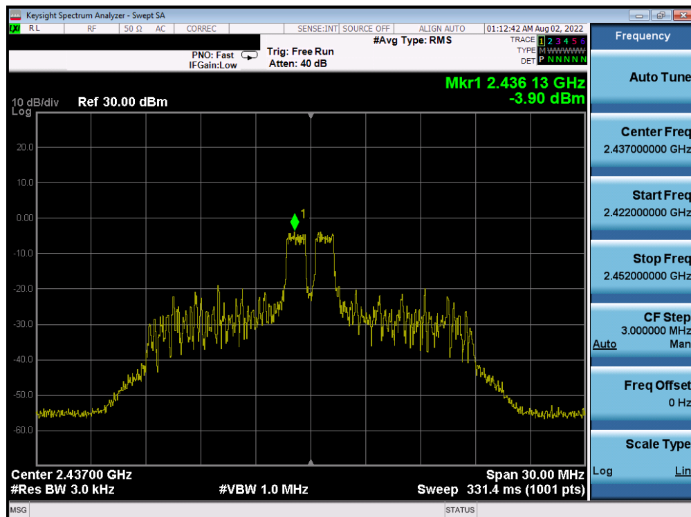
Plot 7-58. Power Spectral Density Plot CDD Antenna WF7b (802.11ax OFDMA – RU26 Index 4 – Ch. 6)
