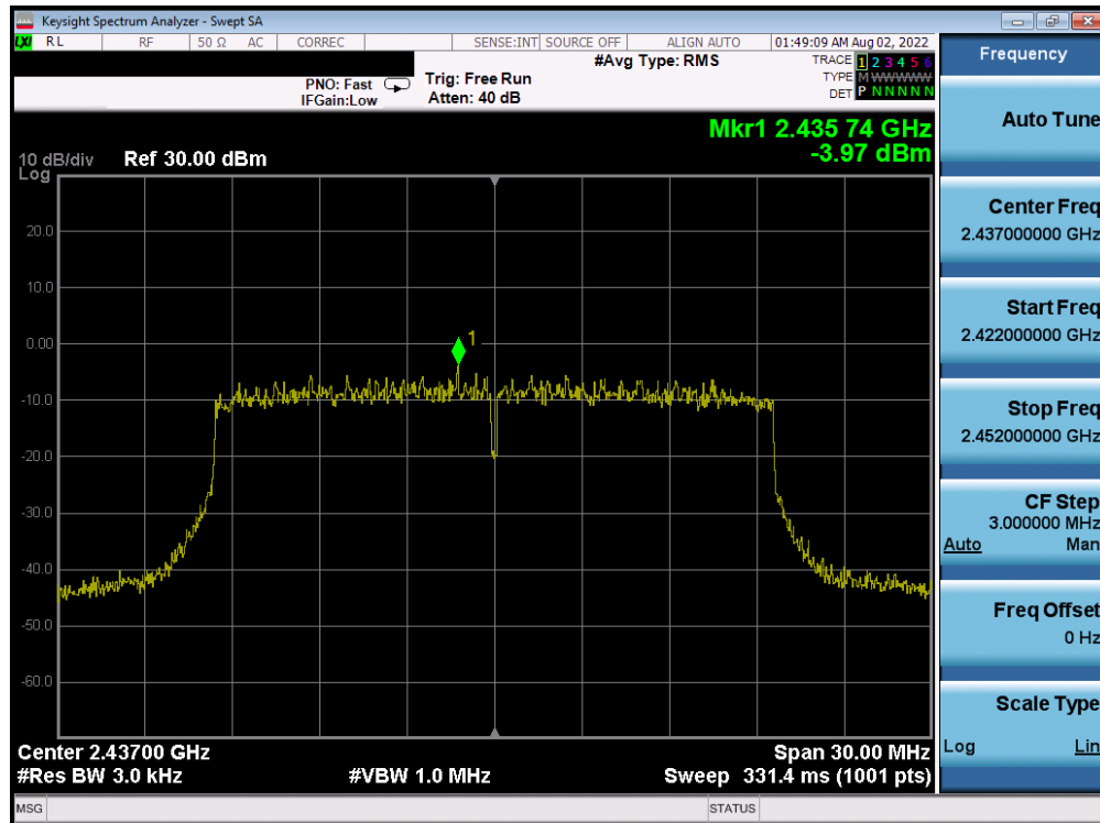
Plot 7-69. Power Spectral Density Plot CDD Antenna WF8 (802.11ax OFDMA – RU242 – Ch. 6)
