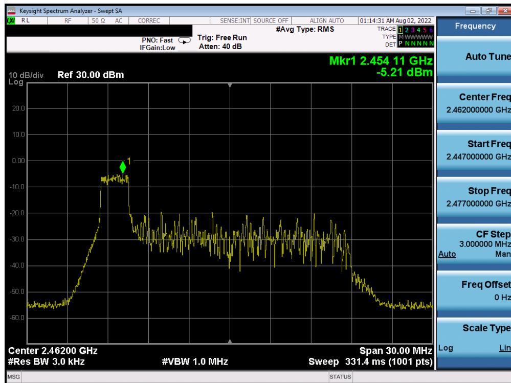
Plot 7-62. Power Spectral Density Plot CDD Antenna WF7b (802.11ax OFDMA – RU26 Index 0 – Ch. 11)
