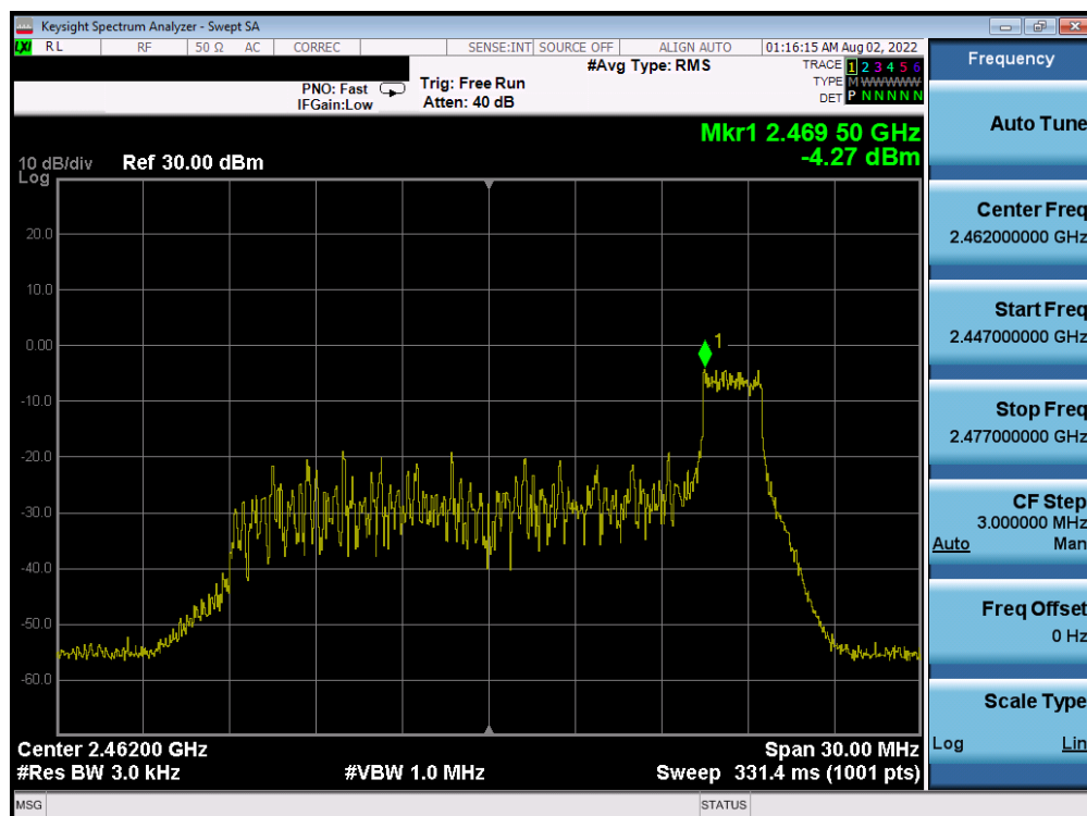
Plot 7-66. Power Spectral Density Plot CDD Antenna WF7b (802.11ax OFDMA – RU26 Index 8 – Ch. 11)
