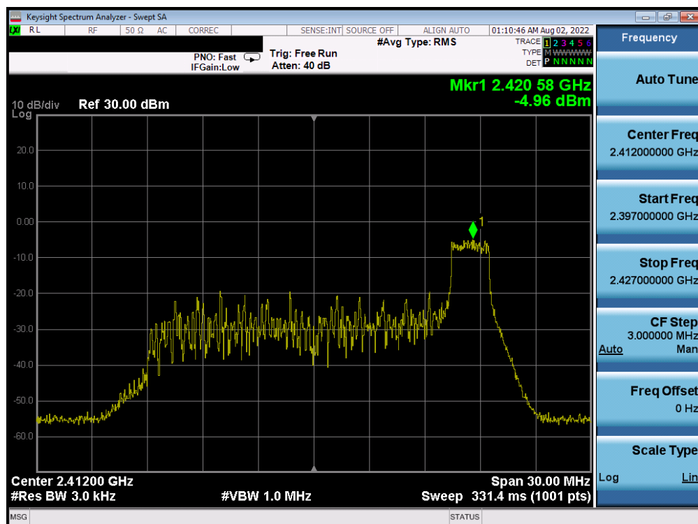
Plot 7-54. Power Spectral Density Plot CDD Antenna WF7b (802.11ax OFDMA – RU26 Index 8 – Ch. 1)
