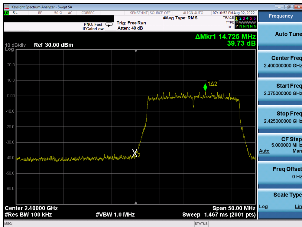
Plot 7-77. Band Edge Antenna WF8 (802.11ax OFDMA – RU242 – Ch. 1)
