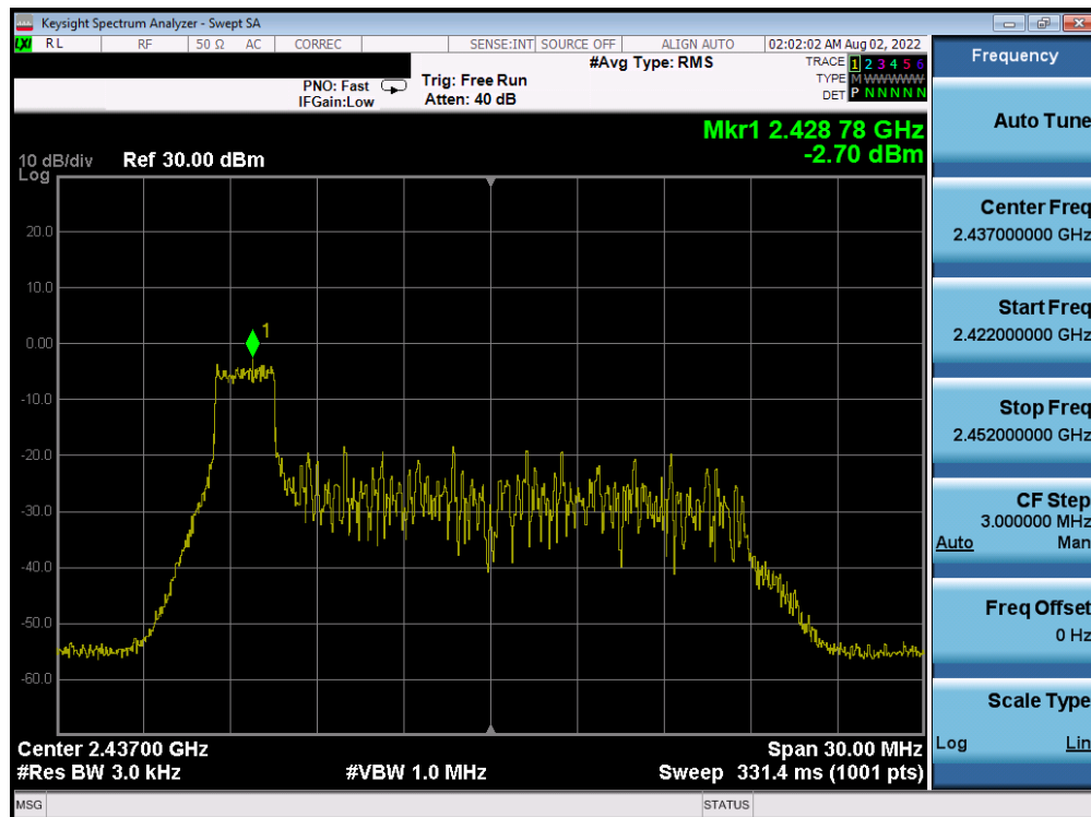
Plot 7-55. Power Spectral Density Plot CDD Antenna WF8 (802.11ax OFDMA – RU26 Index 0 – Ch. 6)
