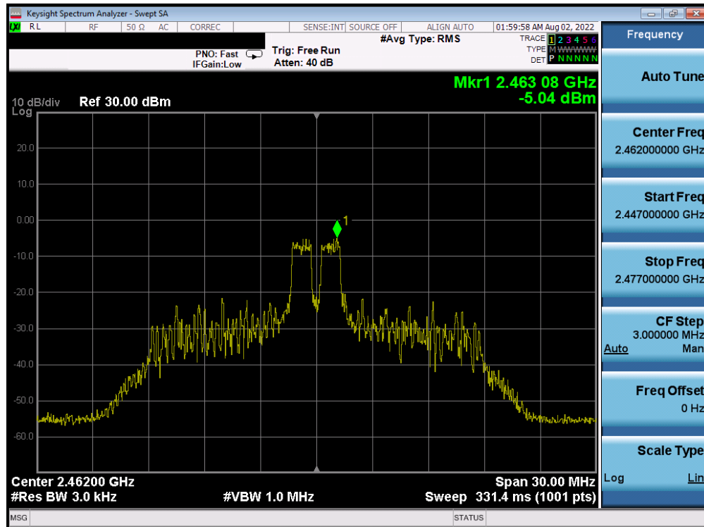
Plot 7-63. Power Spectral Density Plot CDD Antenna WF8 (802.11ax OFDMA – RU26 Index 4 – Ch. 11)
