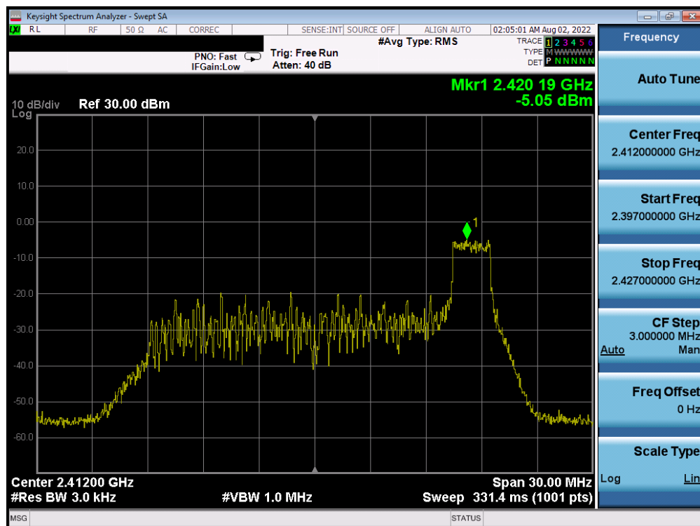
Plot 7-53. Power Spectral Density Plot CDD Antenna WF8 (802.11ax OFDMA – RU26 Index 8 – Ch. 1)
