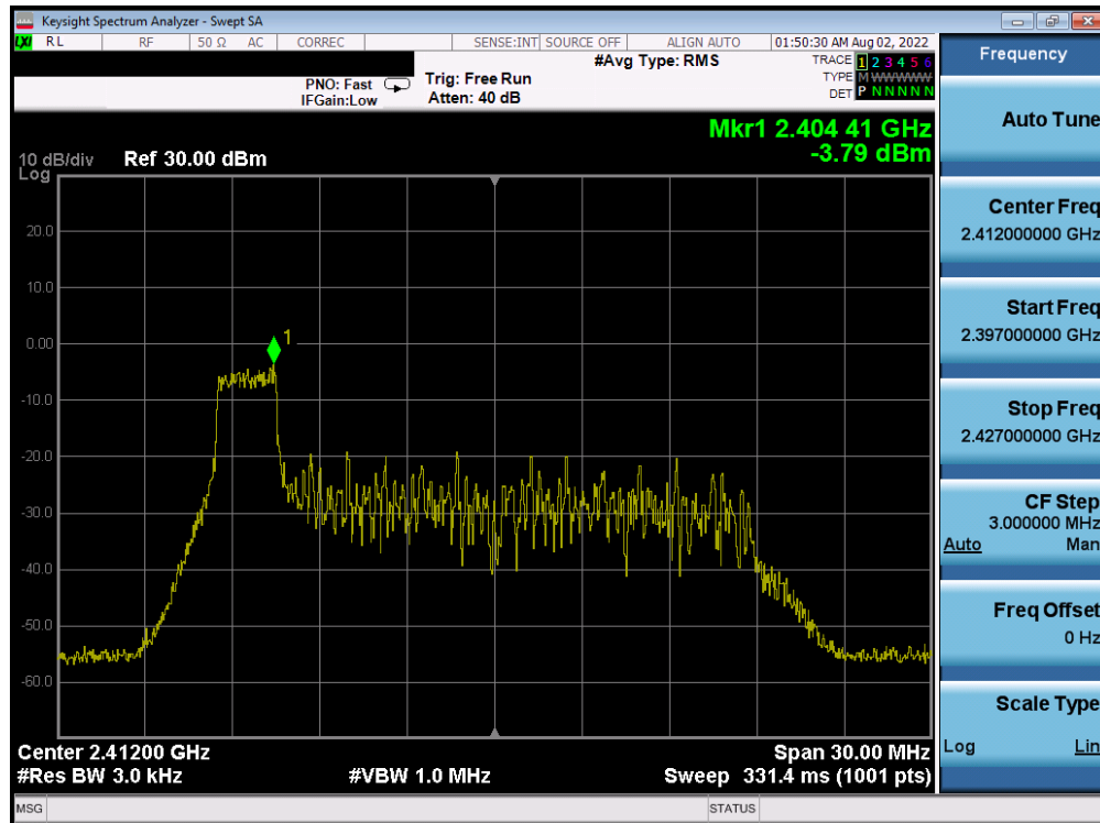
Plot 7-49. Power Spectral Density Plot CDD Antenna WF8 (802.11ax OFDMA – RU26 Index 0 – Ch. 1)
