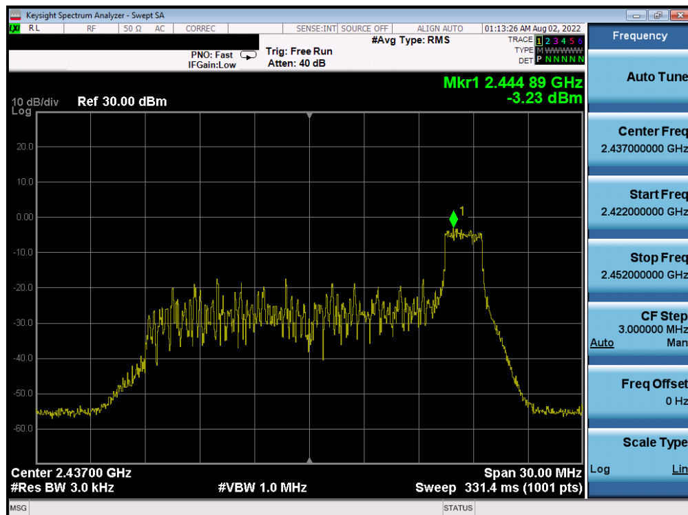
Plot 7-60. Power Spectral Density Plot CDD Antenna WF7b (802.11ax OFDMA – RU26 Index 8 – Ch. 6)
