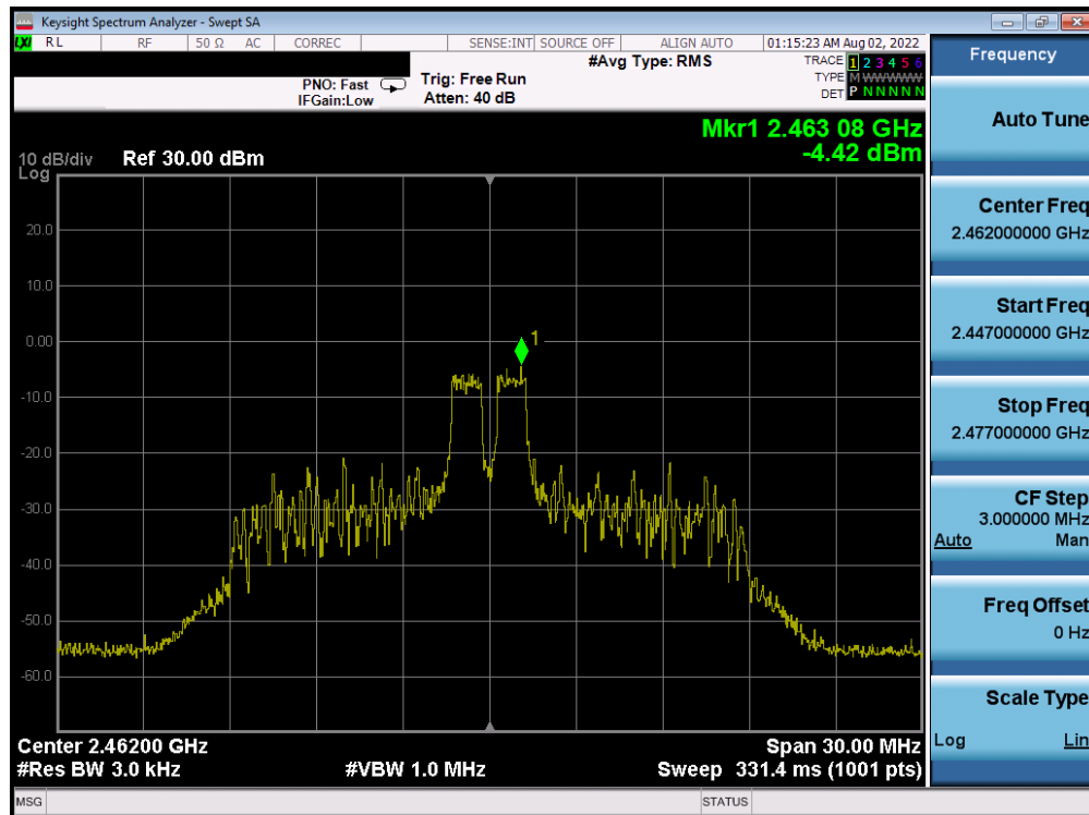
Plot 7-64. Power Spectral Density Plot CDD Antenna WF7b (802.11ax OFDMA – RU26 Index 4 – Ch. 11)
