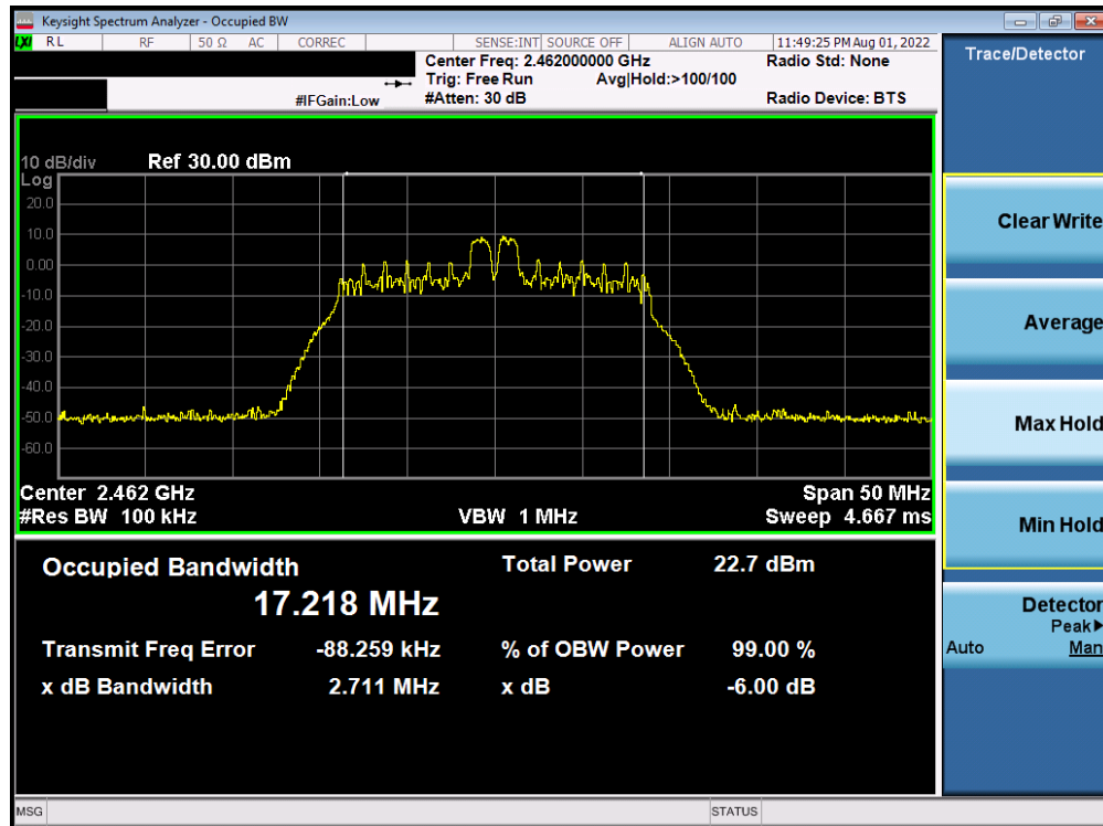
Plot 7-20. 6dB BW & 99% OBW Plot Antenna WF7b (802.11ax OFDMA – RU26 Index 4 – Ch. 11)
