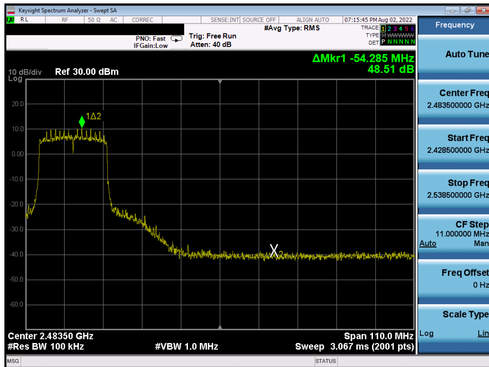
Plot 7-84. Band Edge Antenna WF8 (802.11ax OFDMA – RU242 – Ch. 7)
