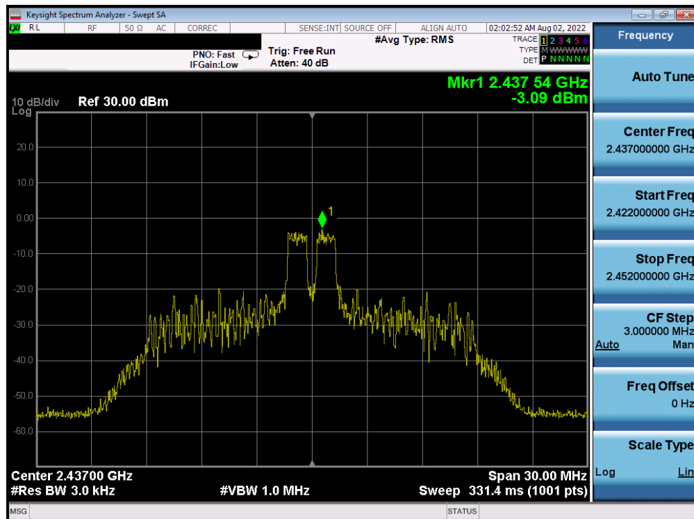
Plot 7-57. Power Spectral Density Plot CDD Antenna WF8 (802.11ax OFDMA – RU26 Index 4 – Ch. 6)
