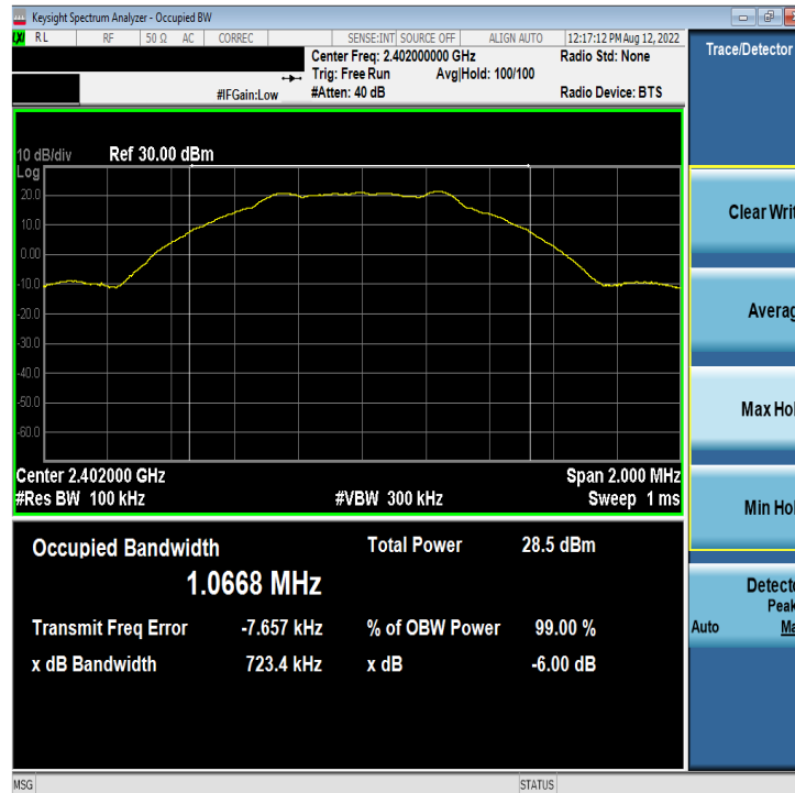
Plot 7-7. 6dB BW & 99% OBW Plot Antenna WF7b (Bluetooth (LE), 1Mbps, ePA – Ch. 0)
