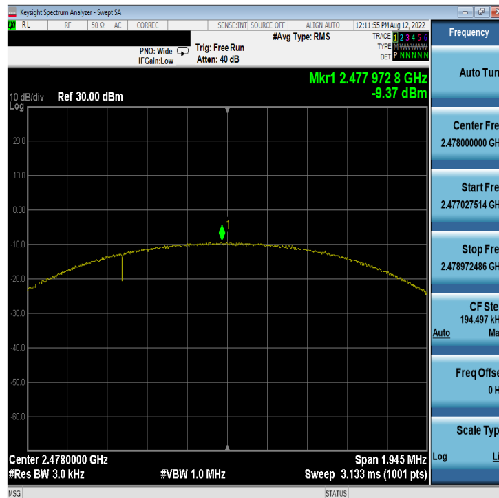
Plot 7-36. Power Spectral Density Plot Antenna WF7b (Bluetooth (LE), 2Mbps, iPA – Ch. 38)
