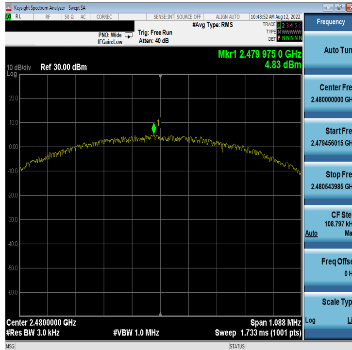
Plot 7-15. Power Spectral Density Plot Antenna WF8 (Bluetooth (LE), 1Mbps, ePA – Ch. 39)
