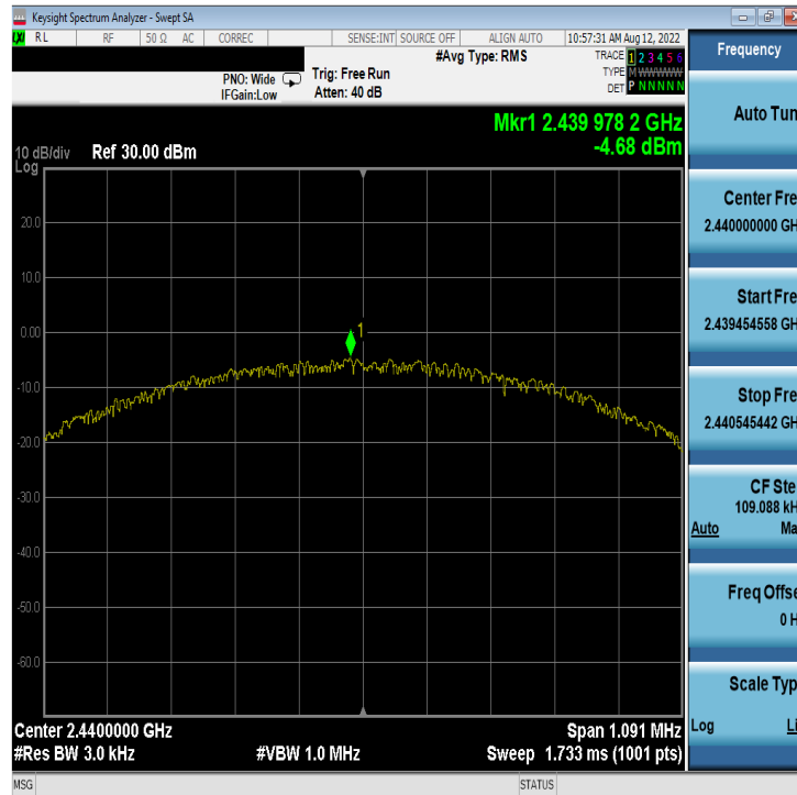
Plot 7-17. Power Spectral Density Plot Antenna WF8 (Bluetooth (LE), 1Mbps, iPA – Ch. 19)
