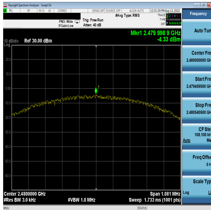
Plot 7-48. Power Spectral Density Plot Antenna WF7b (Bluetooth (LE), 1Mbps, iPA – Ch. 39)
