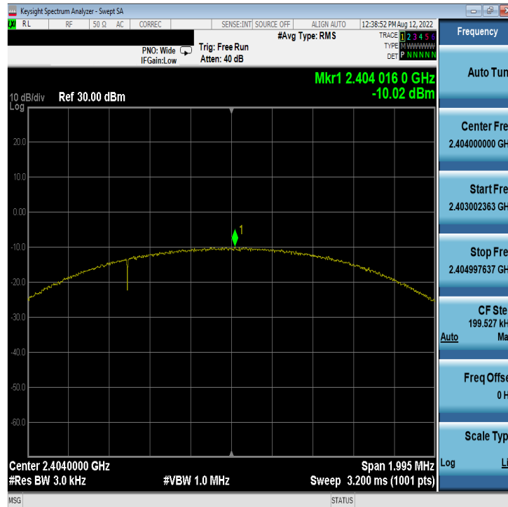
Plot 7-55. Power Spectral Density Plot Antenna WF8 (Bluetooth (LE), 2Mbps, iPA – Ch. 1)
