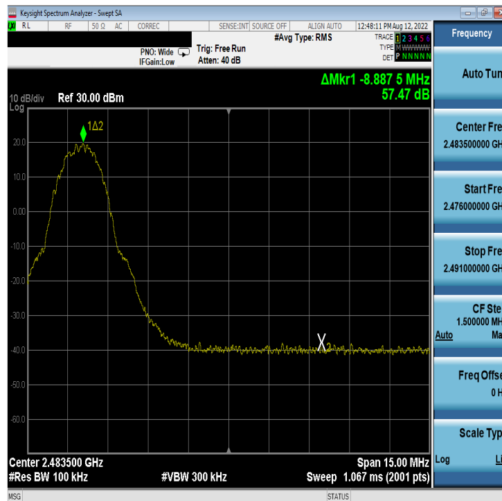
Plot 7-64. Band Edge Plot Antenna WF8 (Bluetooth (LE), 2Mbps, ePA – Ch. 38)
