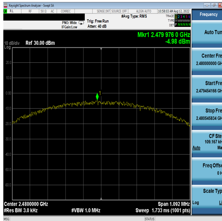
Plot 7-18. Power Spectral Density Plot Antenna WF8 (Bluetooth (LE), 1Mbps, iPA – Ch. 39)
