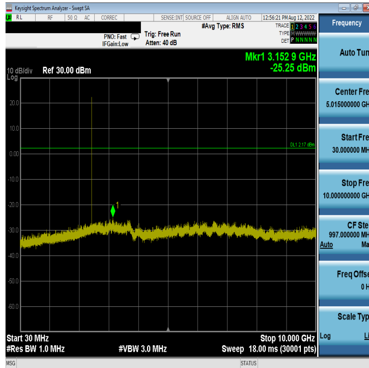
Plot 7-77. Conducted Spurious Plot Antenna WF7b (Bluetooth (LE), 1Mbps, ePA – Ch. 19)
