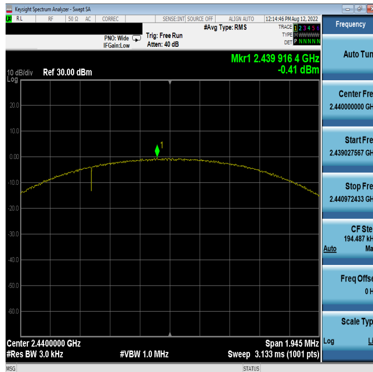
Plot 7-32. Power Spectral Density Plot Antenna WF7b (Bluetooth (LE), 2Mbps, ePA – Ch. 19)
