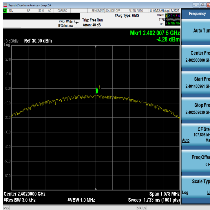
Plot 7-28. Power Spectral Density Plot Antenna WF7b (Bluetooth (LE), 1Mbps, iPA – Ch. 0)
