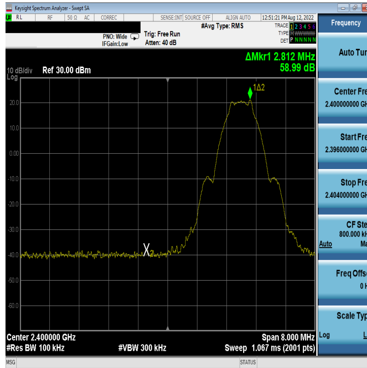
Plot 7-65. Band Edge Plot Antenna WF7b (Bluetooth (LE), 1Mbps, ePA – Ch. 0)
