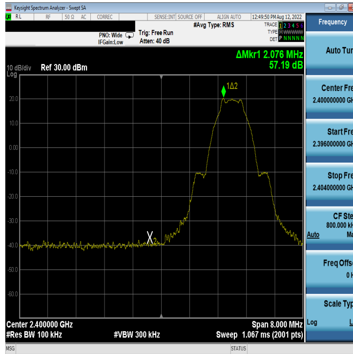
Plot 7-61. Band Edge Plot Antenna WF8 (Bluetooth (LE), 1Mbps, ePA – Ch. 0)
