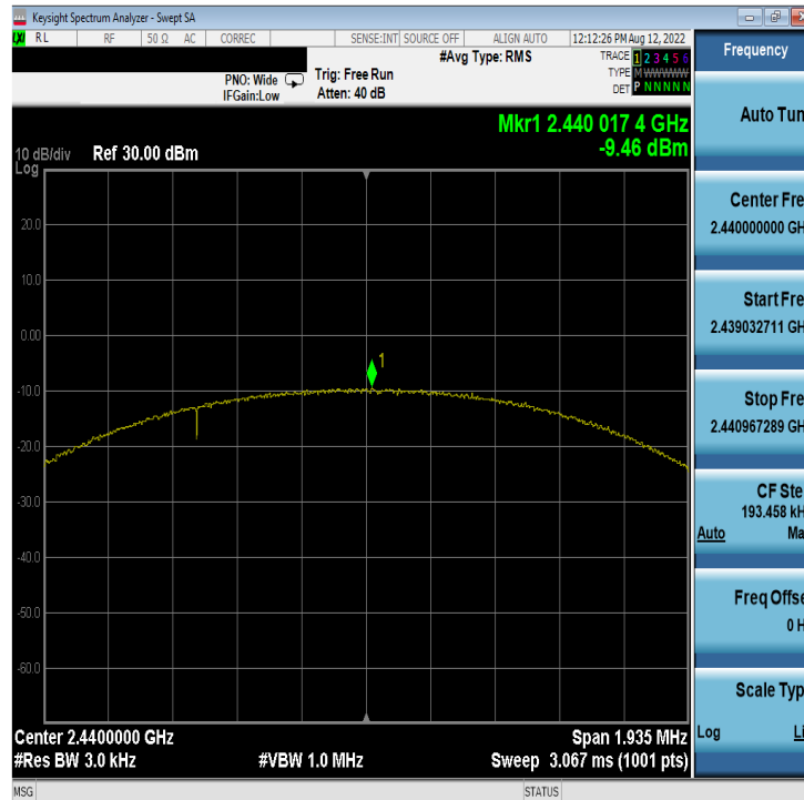
Plot 7-35. Power Spectral Density Plot Antenna WF7b (Bluetooth (LE), 2Mbps, iPA – Ch. 19)
