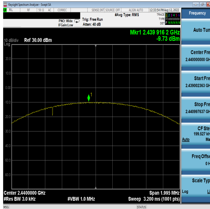
Plot 7-58. Power Spectral Density Plot Antenna WF7b (Bluetooth (LE), 2Mbps, iPA – Ch. 19)
