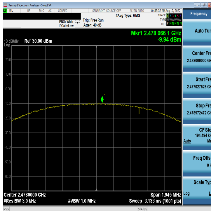
Plot 7-24. Power Spectral Density Plot Antenna WF8 (Bluetooth (LE), 2Mbps, iPA – Ch. 38)
