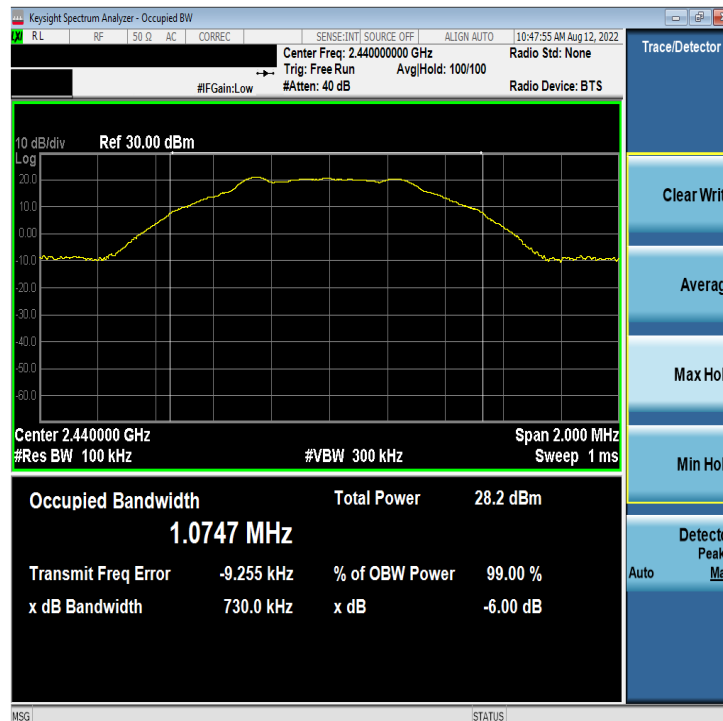
Plot 7-2. 6dB BW & 99% OBW Plot Antenna WF8 (Bluetooth (LE), 1Mbps, ePA – Ch. 19)
