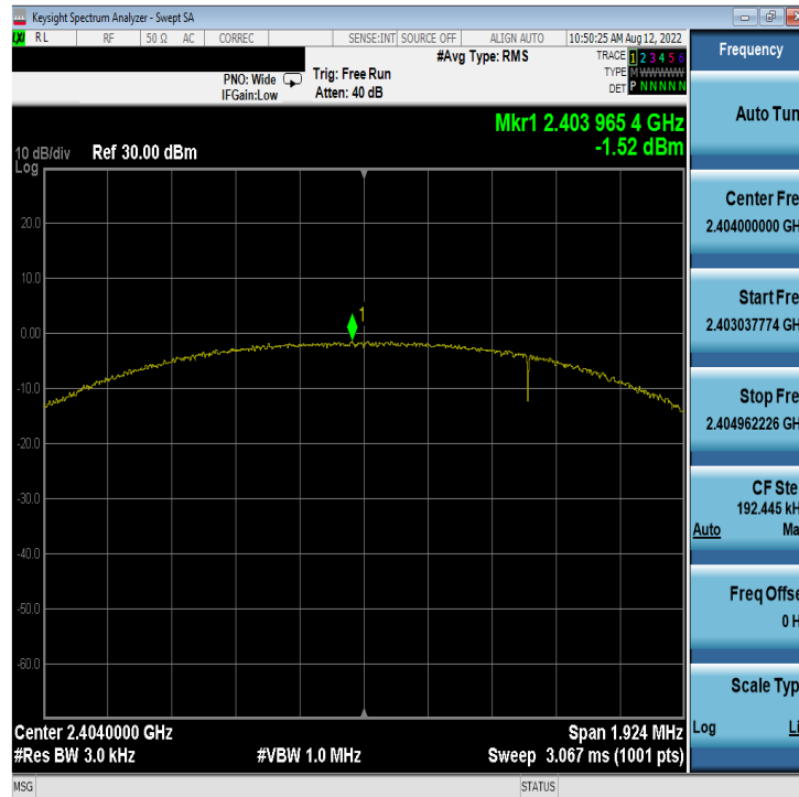
Plot 7-19. Power Spectral Density Plot Antenna WF8 (Bluetooth (LE), 2Mbps, ePA – Ch. 1)
