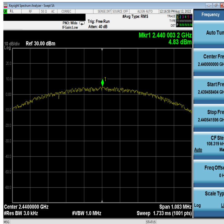
Plot 7-26. Power Spectral Density Plot Antenna WF7b (Bluetooth (LE), 1Mbps, ePA – Ch. 19)
