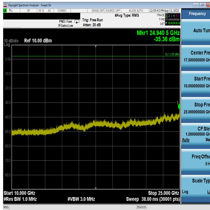
Plot 7-76. Conducted Spurious Plot Antenna WF7b (Bluetooth (LE), 1Mbps, ePA – Ch. 0)
