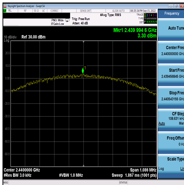
Plot 7-40. Power Spectral Density Plot Antenna WF7b (Bluetooth (LE), 1Mbps, ePA – Ch. 19)
