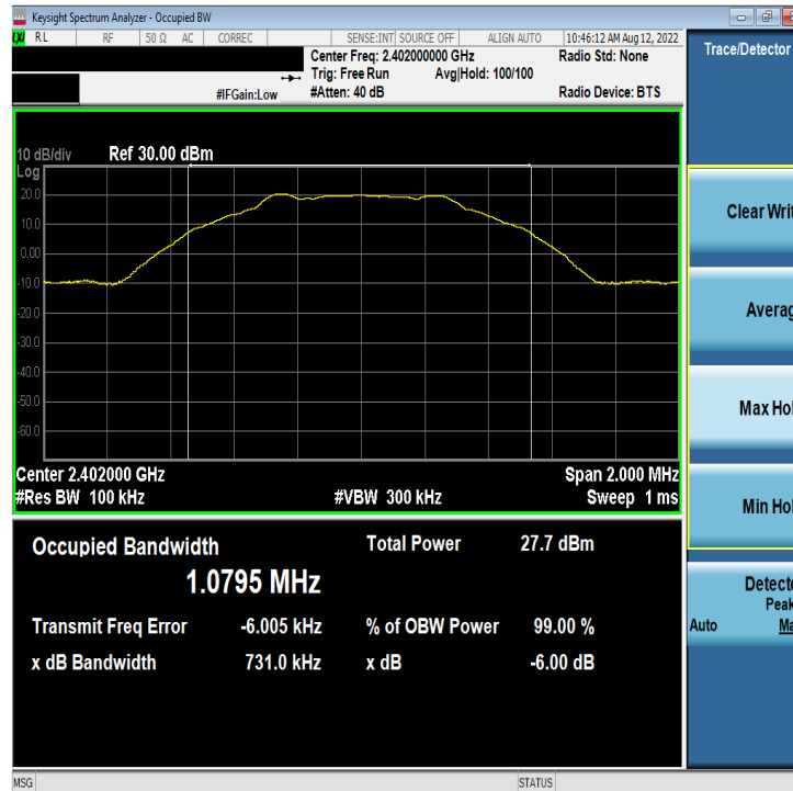
Plot 7-1. 6dB BW & 99% OBW Plot Antenna WF8 (Bluetooth (LE), 1Mbps, ePA – Ch. 0)
