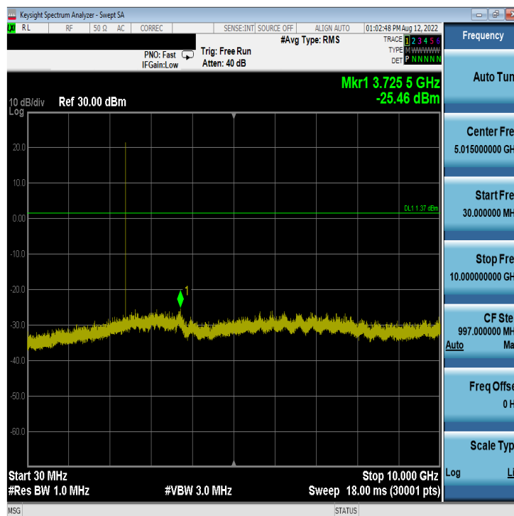
Plot 7-69. Conducted Spurious Plot Antenna WF8 (Bluetooth (LE), 1Mbps, ePA – Ch. 0)
