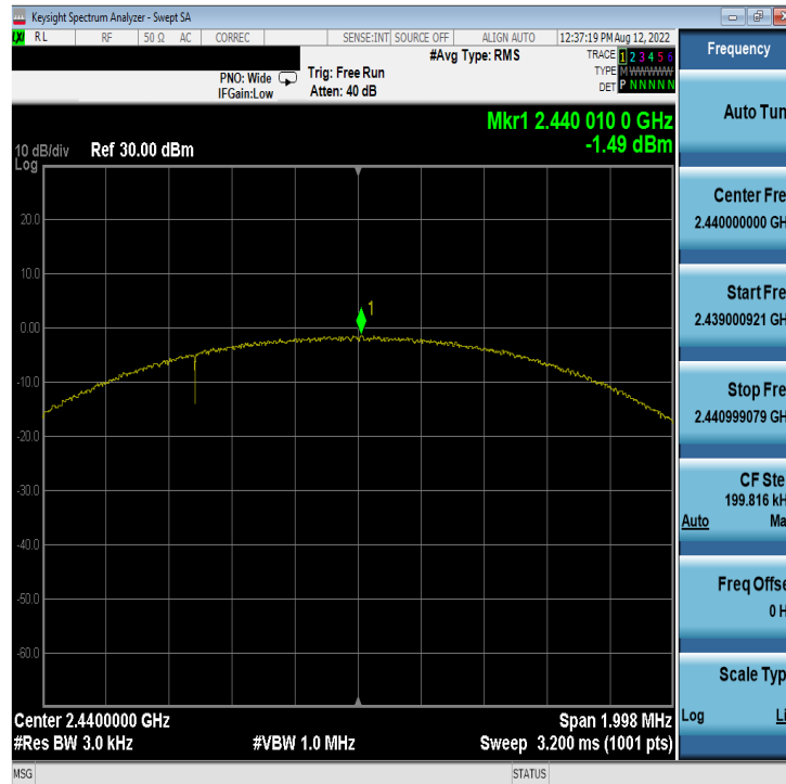
Plot 7-51. Power Spectral Density Plot Antenna WF8 (Bluetooth (LE), 2Mbps, ePA – Ch. 19)
