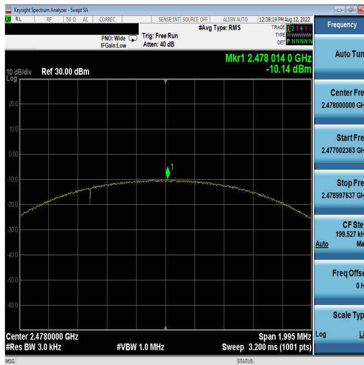
Plot 7-59. Power Spectral Density Plot Antenna WF8 (Bluetooth (LE), 2Mbps, iPA – Ch. 38)
