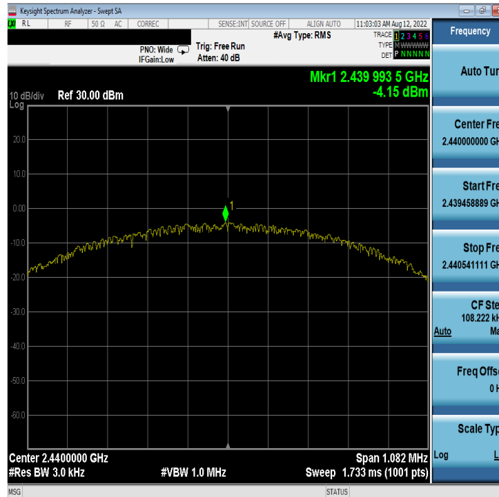
Plot 7-29. Power Spectral Density Plot Antenna WF7b (Bluetooth (LE), 1Mbps, iPA – Ch. 19)
