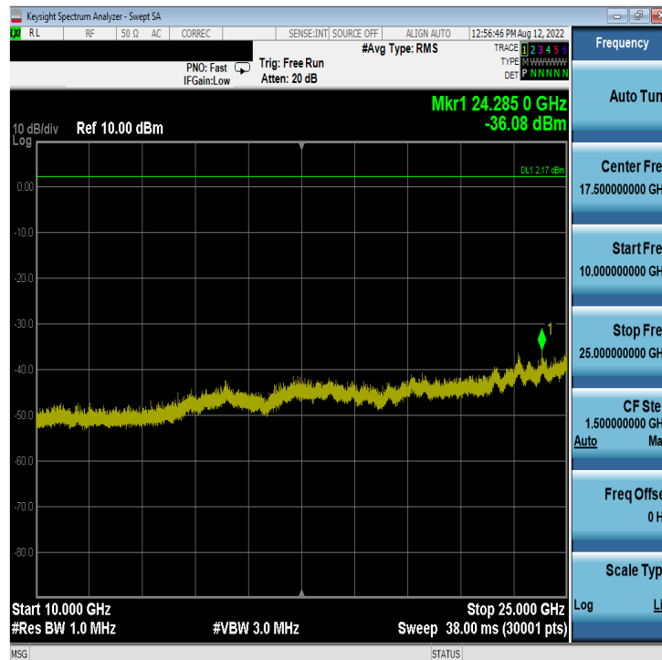
Plot 7-78. Conducted Spurious Plot Antenna WF7b (Bluetooth (LE), 1Mbps, ePA – Ch. 19)
