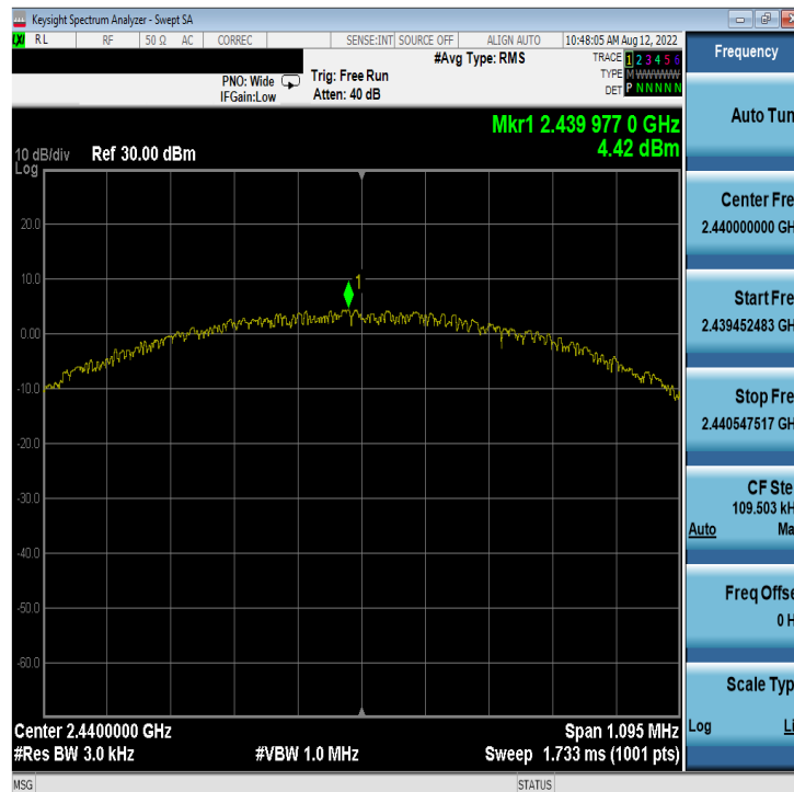
Plot 7-14. Power Spectral Density Plot Antenna WF8 (Bluetooth (LE), 1Mbps, ePA – Ch. 19)
