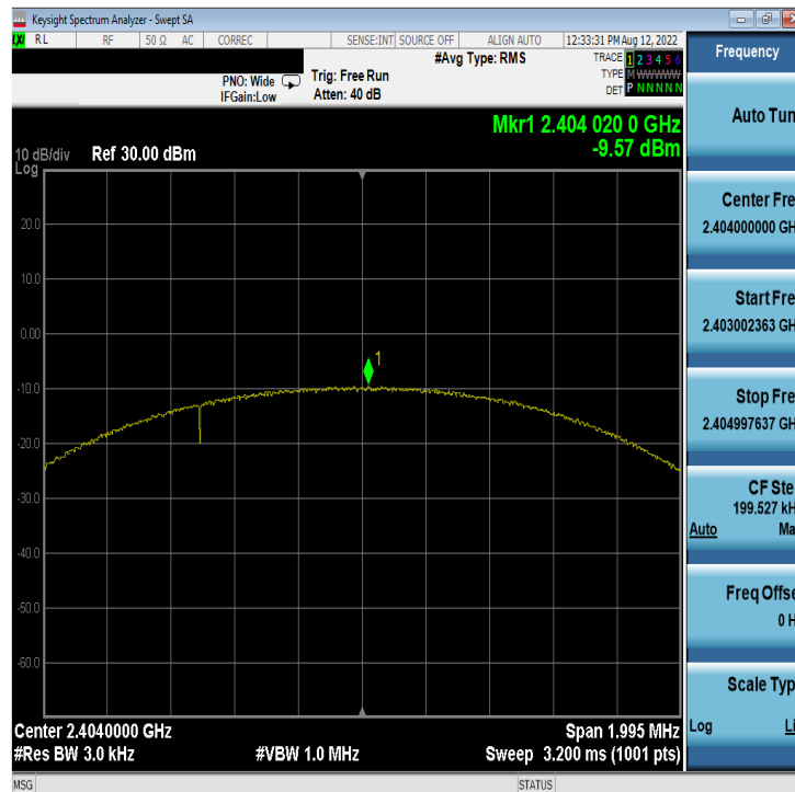
Plot 7-56. Power Spectral Density Plot Antenna WF7b (Bluetooth (LE), 2Mbps, iPA – Ch. 1)
