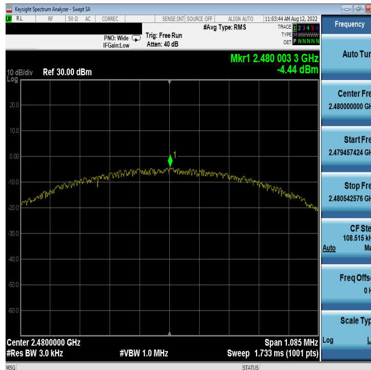
Plot 7-30. Power Spectral Density Plot Antenna WF7b (Bluetooth (LE), 1Mbps, iPA – Ch. 39)
