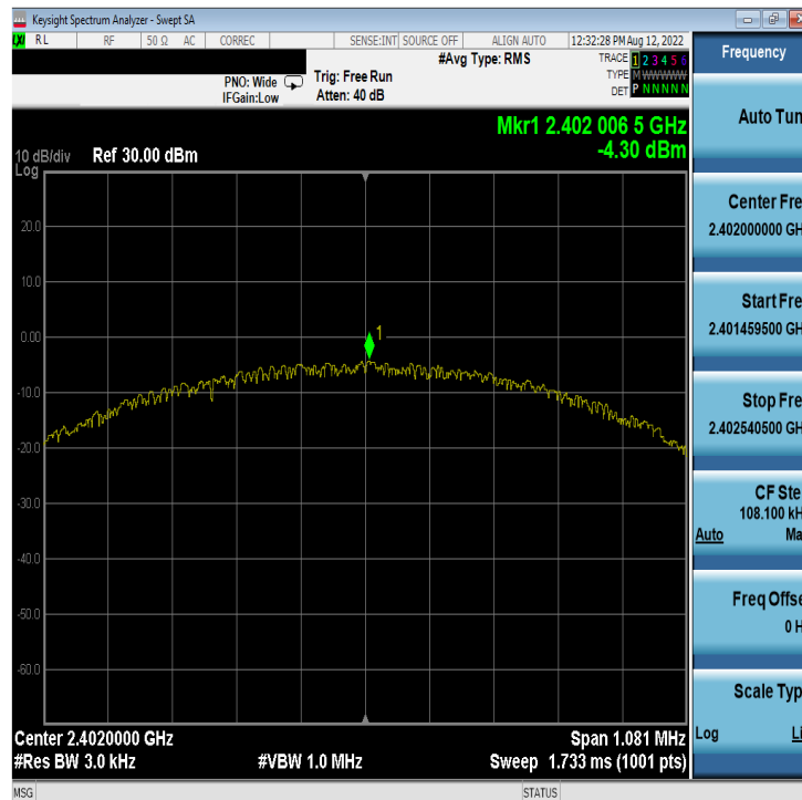
Plot 7-44. Power Spectral Density Plot Antenna WF7b (Bluetooth (LE), 1Mbps, iPA – Ch. 0)
