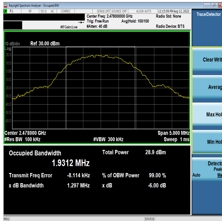
Plot 7-12. 6dB BW & 99% OBW Antenna WF7b (Bluetooth (LE), 2Mbps, ePA – Ch. 38)
