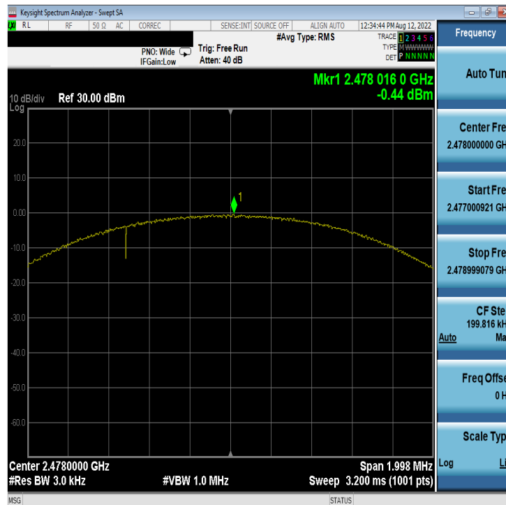
Plot 7-54. Power Spectral Density Plot Antenna WF7b (Bluetooth (LE), 2Mbps, ePA – Ch. 38)
