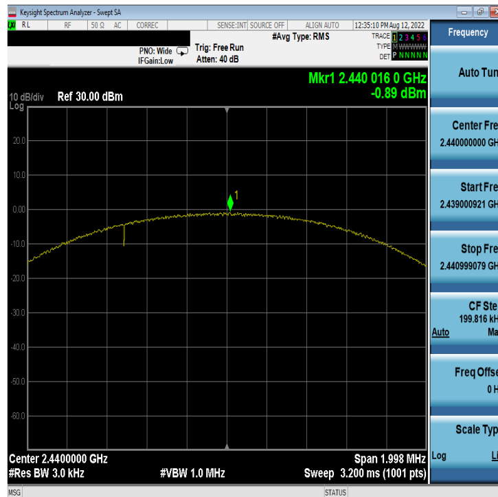
Plot 7-52. Power Spectral Density Plot Antenna WF7b (Bluetooth (LE), 2Mbps, ePA – Ch. 19)
