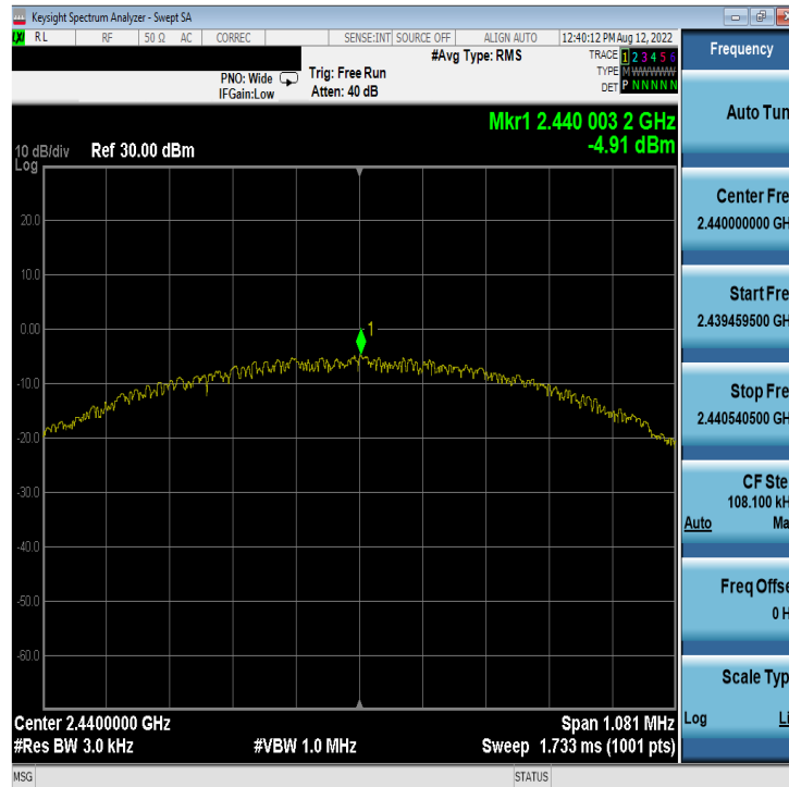
Plot 7-45. Power Spectral Density Plot Antenna WF8 (Bluetooth (LE), 1Mbps, iPA – Ch. 19)
