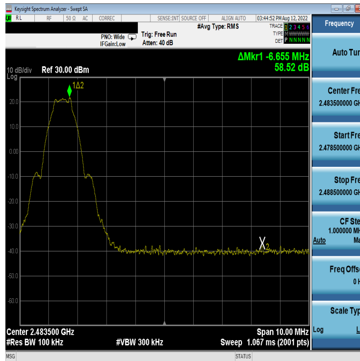
Plot 7-66. Band Edge Plot Antenna WF7b (Bluetooth (LE), 1Mbps, ePA – Ch. 39)
