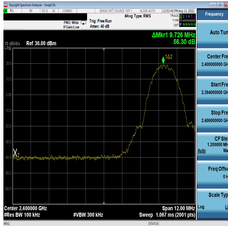
Plot 7-67. Band Edge Plot Antenna WF7b (Bluetooth (LE), 2Mbps, ePA – Ch. 1)
