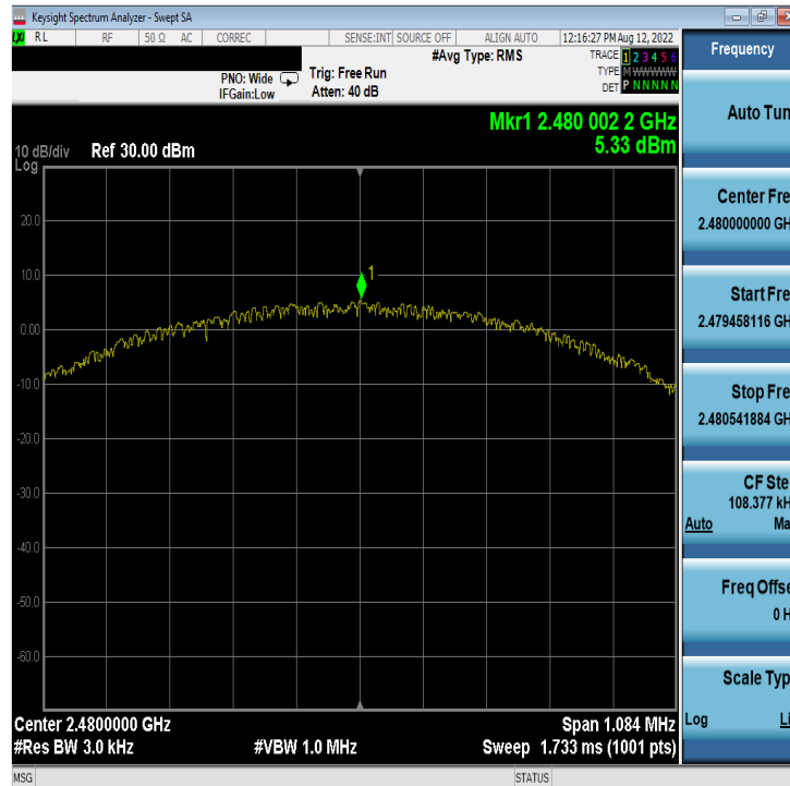
Plot 7-27. Power Spectral Density Plot Antenna WF7b (Bluetooth (LE), 1Mbps, ePA – Ch. 39)
