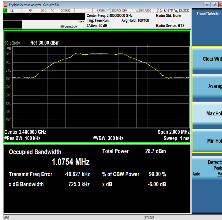
Plot 7-3. 6dB BW & 99% OBW Plot Antenna WF8 (Bluetooth (LE), 1Mbps, ePA – Ch. 39)
