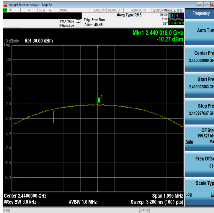
Plot 7-57. Power Spectral Density Plot Antenna WF8 (Bluetooth (LE), 2Mbps, iPA – Ch. 19)
