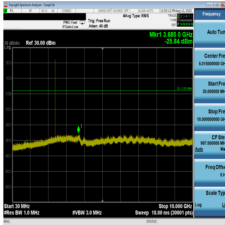
Plot 7-75. Conducted Spurious Plot Antenna WF7b (Bluetooth (LE), 1Mbps, ePA – Ch. 0)
