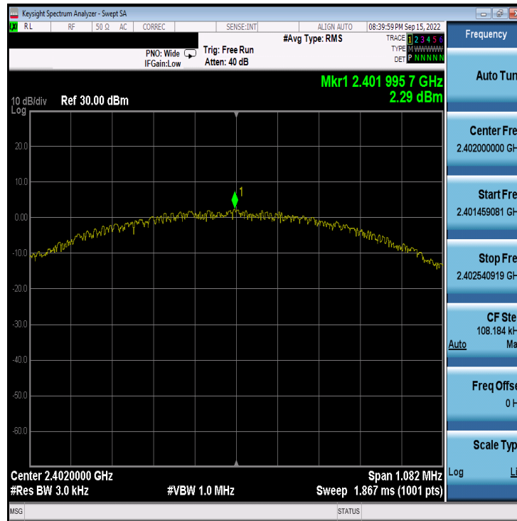
Plot 7-37. Power Spectral Density Plot Antenna WF8 (Bluetooth (LE), 1Mbps, ePA – Ch. 0)
