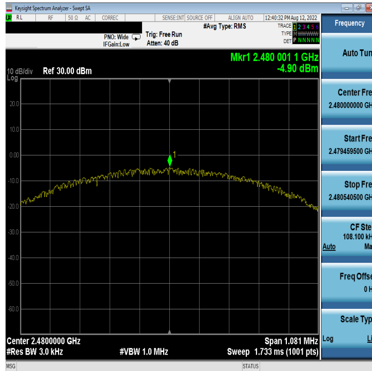
Plot 7-47. Power Spectral Density Plot Antenna WF8 (Bluetooth (LE), 1Mbps, iPA – Ch. 39)
