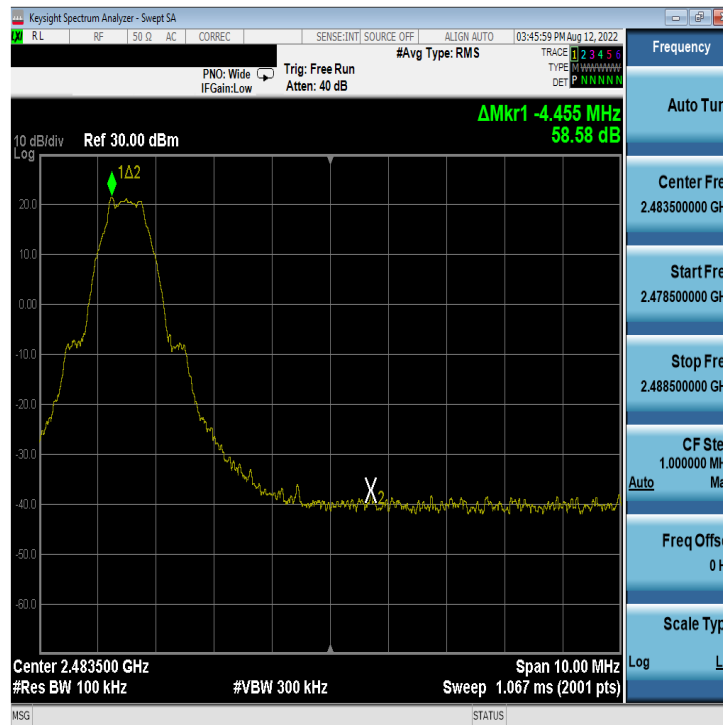
Plot 7-62. Band Edge Plot Antenna WF8 (Bluetooth (LE), 1Mbps, ePA – Ch. 39)
