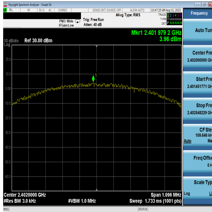
Plot 7-13. Power Spectral Density Plot Antenna WF8 (Bluetooth (LE), 1Mbps, ePA – Ch. 0)
