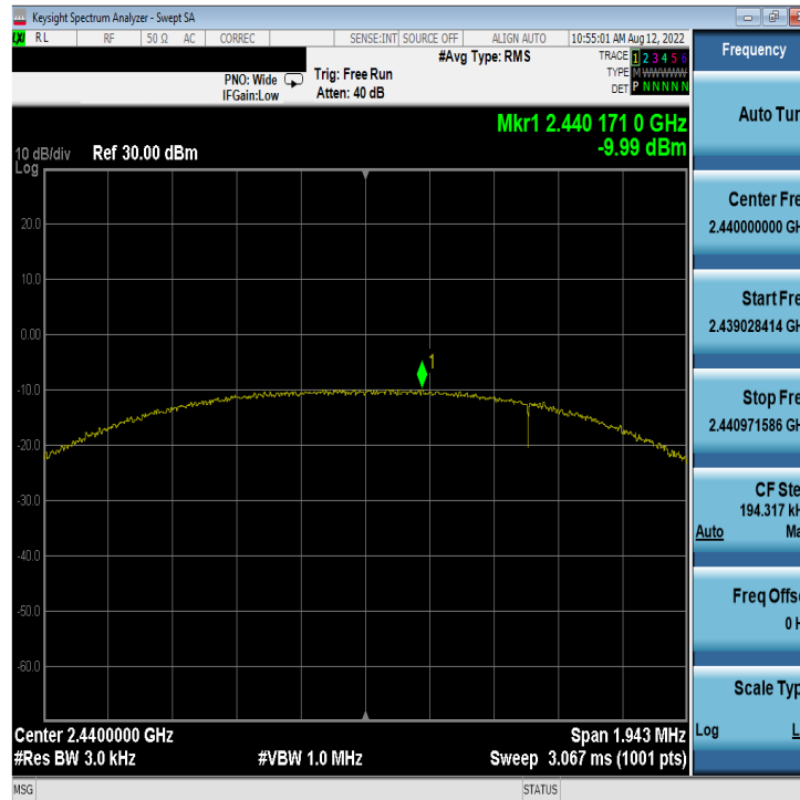
Plot 7-23. Power Spectral Density Plot Antenna WF8 (Bluetooth (LE), 2Mbps, iPA – Ch. 19)
