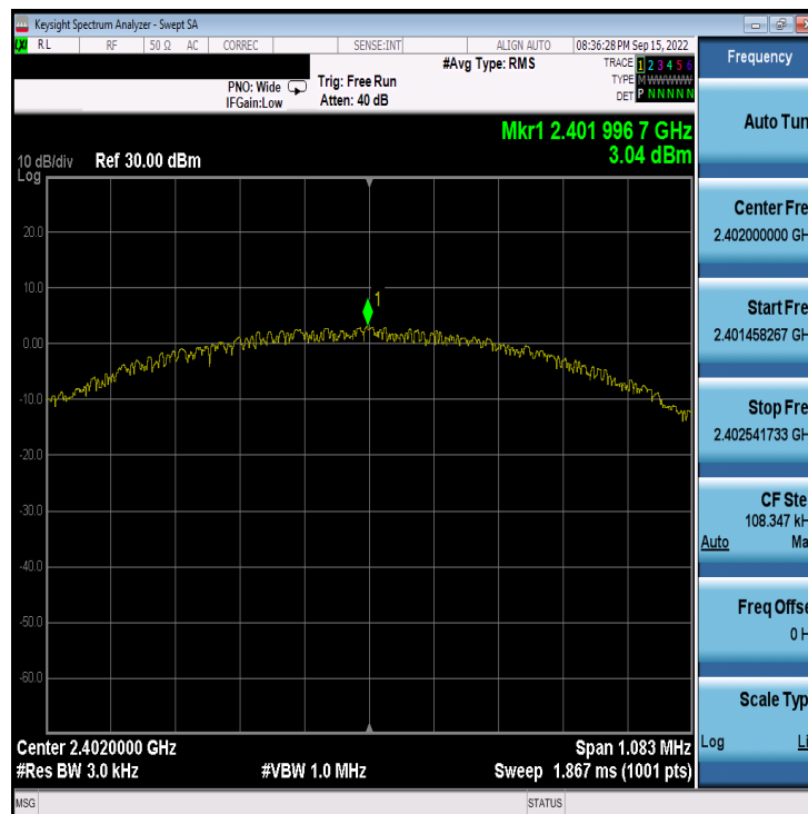
Plot 7-38. Power Spectral Density Plot Antenna WF7b (Bluetooth (LE), 1Mbps, ePA – Ch. 0)
