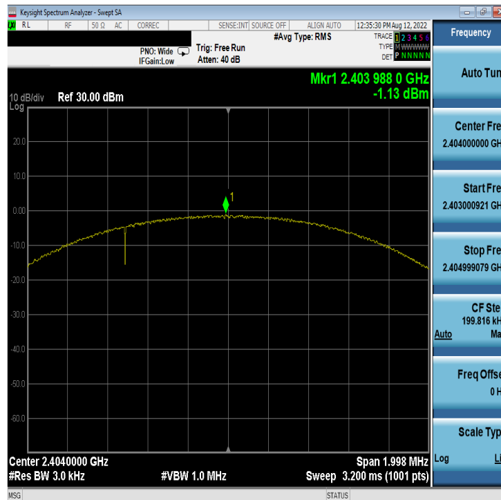
Plot 7-50. Power Spectral Density Plot Antenna WF7b (Bluetooth (LE), 2Mbps, ePA – Ch. 1)
