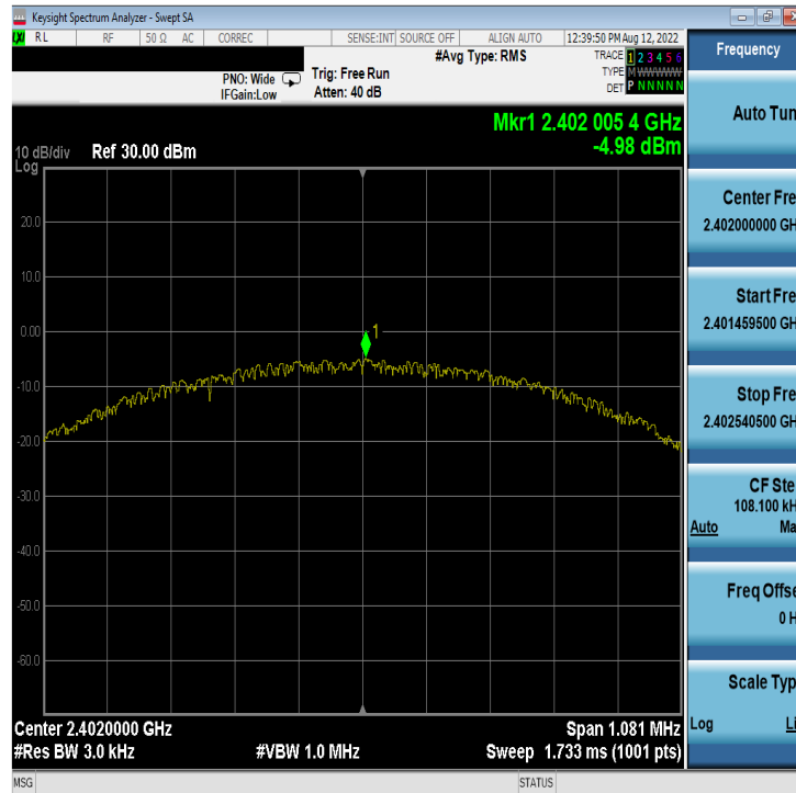
Plot 7-43. Power Spectral Density Plot Antenna WF8 (Bluetooth (LE), 1Mbps, iPA – Ch. 0)
