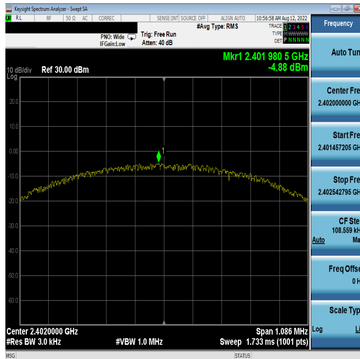
Plot 7-16. Power Spectral Density Plot Antenna WF8 (Bluetooth (LE), 1Mbps, iPA – Ch. 0)
