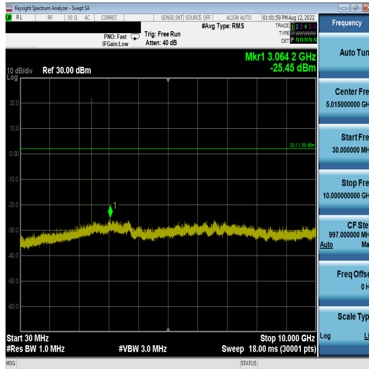
Plot 7-71. Conducted Spurious Plot Antenna WF8 (Bluetooth (LE), 1Mbps, ePA – Ch. 19)
