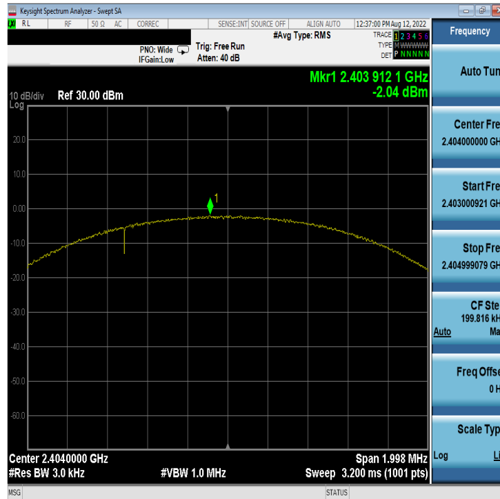
Plot 7-49. Power Spectral Density Plot Antenna WF8 (Bluetooth (LE), 2Mbps, ePA – Ch. 1)
