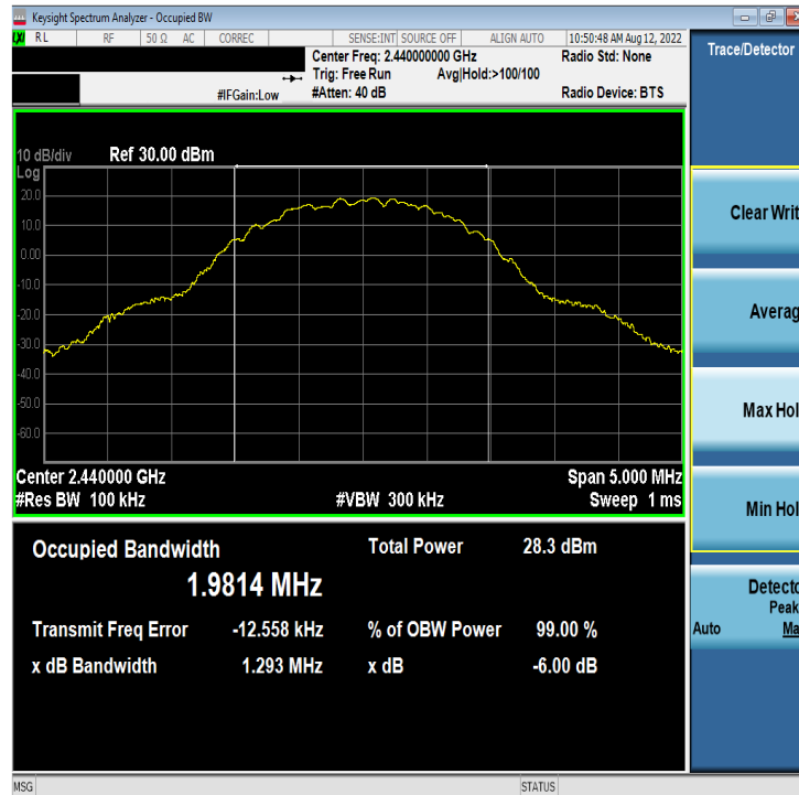
Plot 7-5. 6dB BW & 99% OBW Plot Antenna WF8 (Bluetooth (LE), 2Mbps, ePA – Ch. 19)
