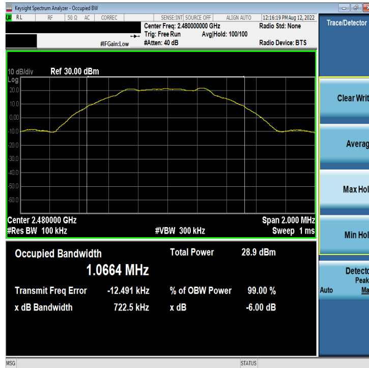
Plot 7-9. 6dB BW & 99% OBW Plot Antenna WF7b (Bluetooth (LE), 1Mbps, ePA – Ch. 39)
