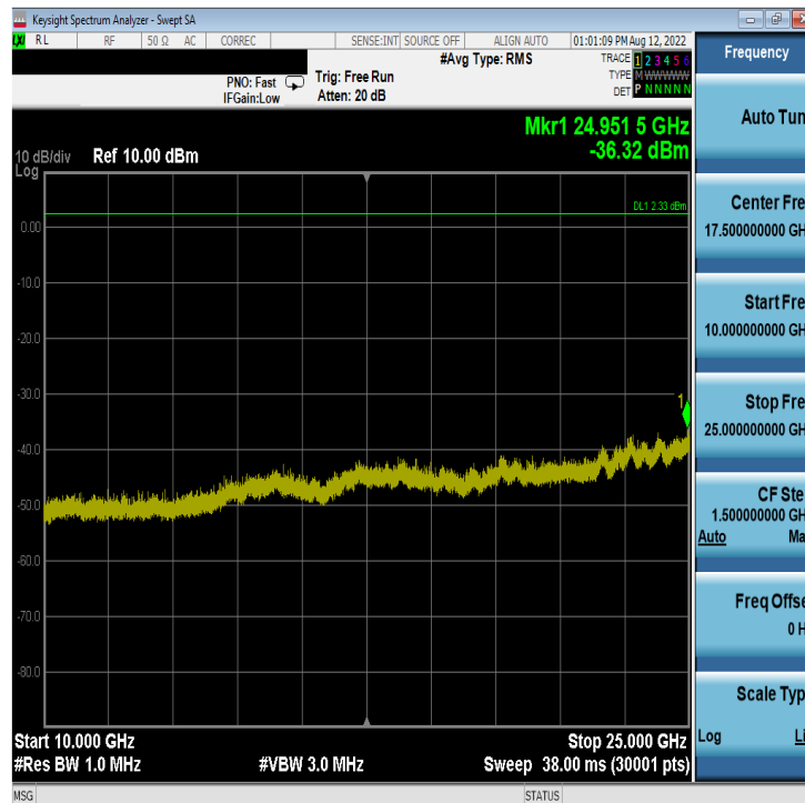
Plot 7-74. Conducted Spurious Plot Antenna WF8 (Bluetooth (LE), 1Mbps, ePA – Ch. 39)
