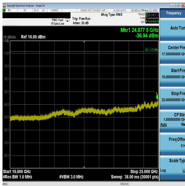
Plot 7-70. Conducted Spurious Plot Antenna WF8 (Bluetooth (LE), 1Mbps, ePA – Ch. 0)
