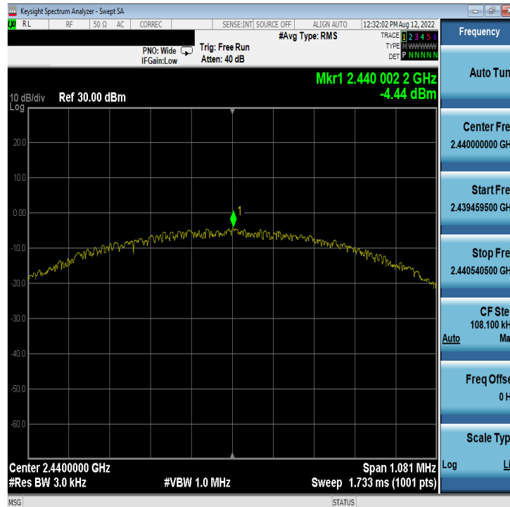
Plot 7-46. Power Spectral Density Plot Antenna WF7b (Bluetooth (LE), 1Mbps, iPA – Ch. 19)
