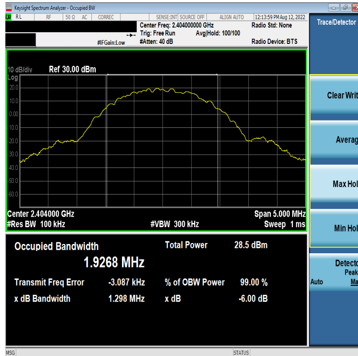
Plot 7-10. 6dB BW & 99% OBW Plot Antenna WF7b (Bluetooth (LE), 2Mbps, ePA – Ch. 1)
