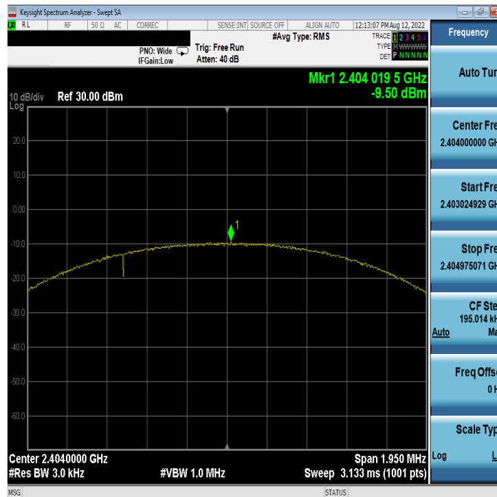
Plot 7-34. Power Spectral Density Plot Antenna WF7b (Bluetooth (LE), 2Mbps, iPA – Ch. 1)
