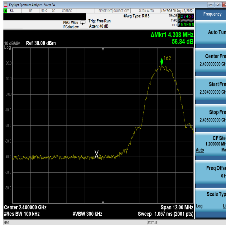
Plot 7-63. Band Edge Plot Antenna WF8 (Bluetooth (LE), 2Mbps, ePA – Ch. 1)
