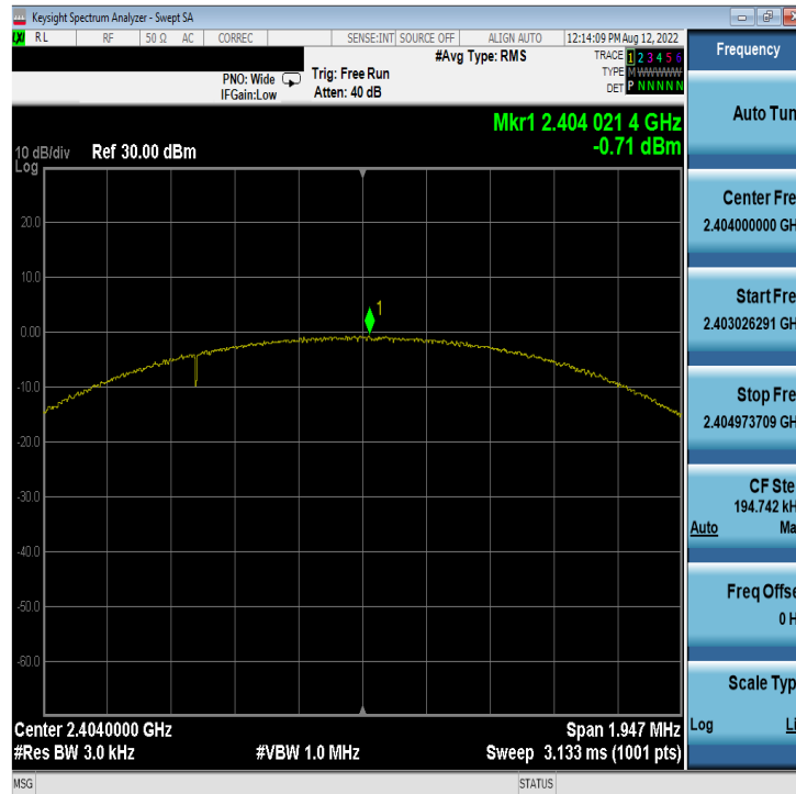
Plot 7-31. Power Spectral Density Plot Antenna WF7b (Bluetooth (LE), 2Mbps, ePA – Ch. 1)
