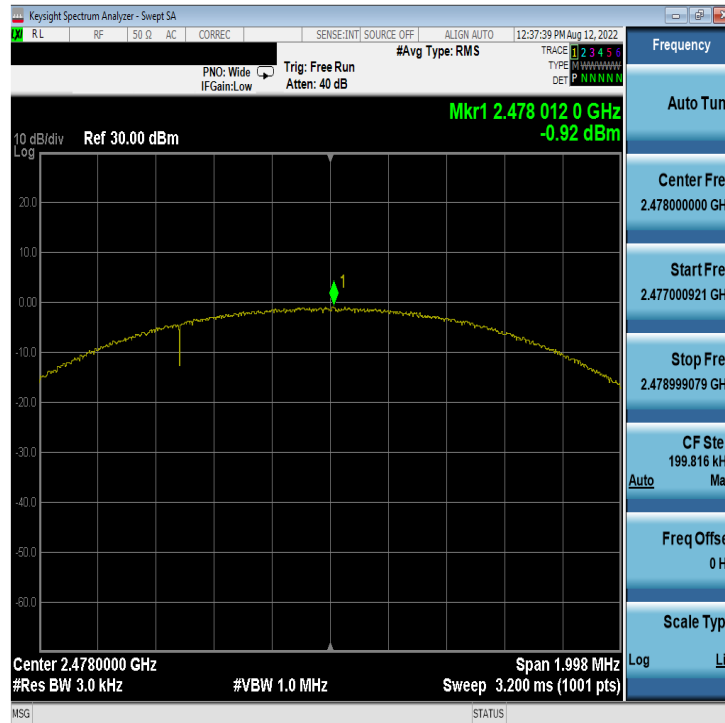
Plot 7-53. Power Spectral Density Plot Antenna WF8 (Bluetooth (LE), 2Mbps, ePA – Ch. 38)
