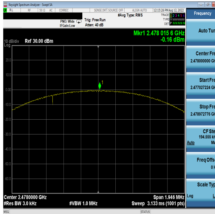
Plot 7-33. Power Spectral Density Plot Antenna WF7b (Bluetooth (LE), 2Mbps, ePA – Ch. 38)
