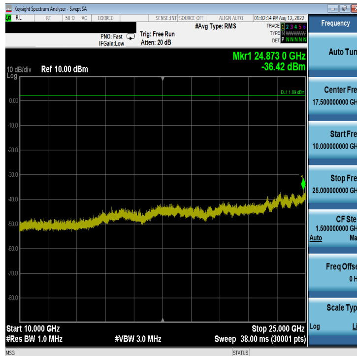
Plot 7-72. Conducted Spurious Plot Antenna WF8 (Bluetooth (LE), 1Mbps, ePA – Ch. 19)
