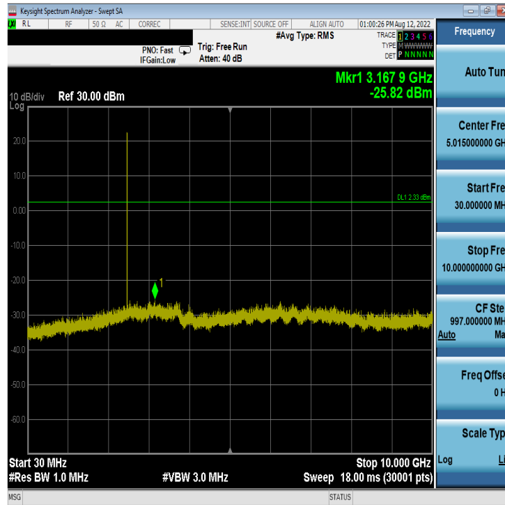
Plot 7-73. Conducted Spurious Plot Antenna WF8 (Bluetooth (LE), 1Mbps, ePA – Ch. 39)
