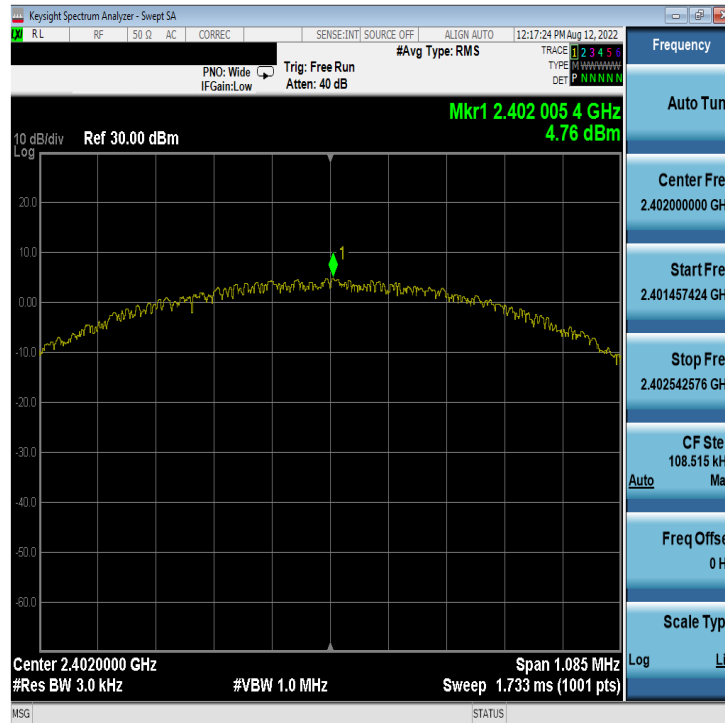
Plot 7-25. Power Spectral Density Plot Antenna WF7b (Bluetooth (LE), 1Mbps, ePA – Ch. 0)
