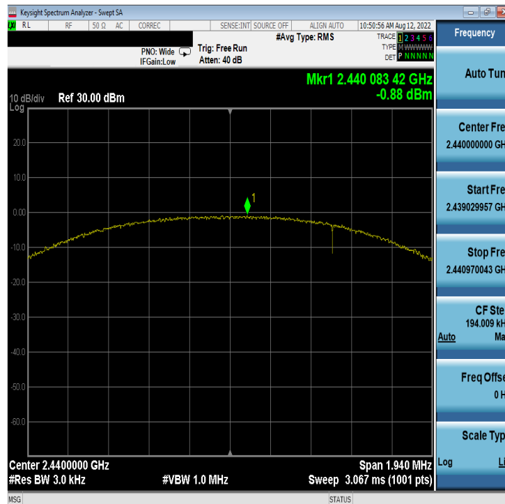
Plot 7-20. Power Spectral Density Plot Antenna WF8 (Bluetooth (LE), 2Mbps, ePA – Ch. 19)
