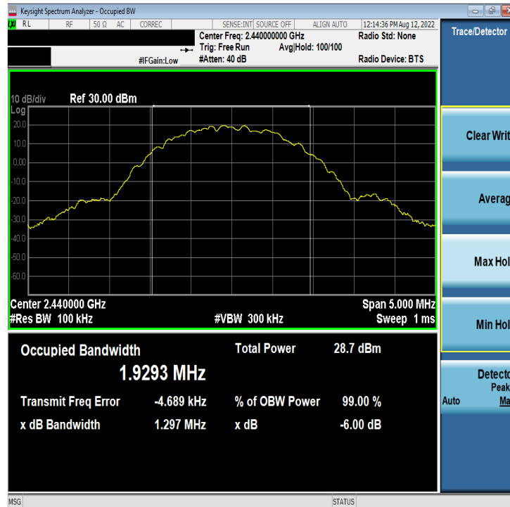
Plot 7-11. 6dB BW & 99% OBW Plot Antenna WF7b (Bluetooth (LE), 2Mbps, ePA – Ch. 19)
