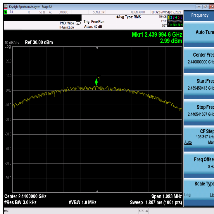
Plot 7-39. Power Spectral Density Plot Antenna WF8 (Bluetooth (LE), 1Mbps, ePA – Ch. 19)
