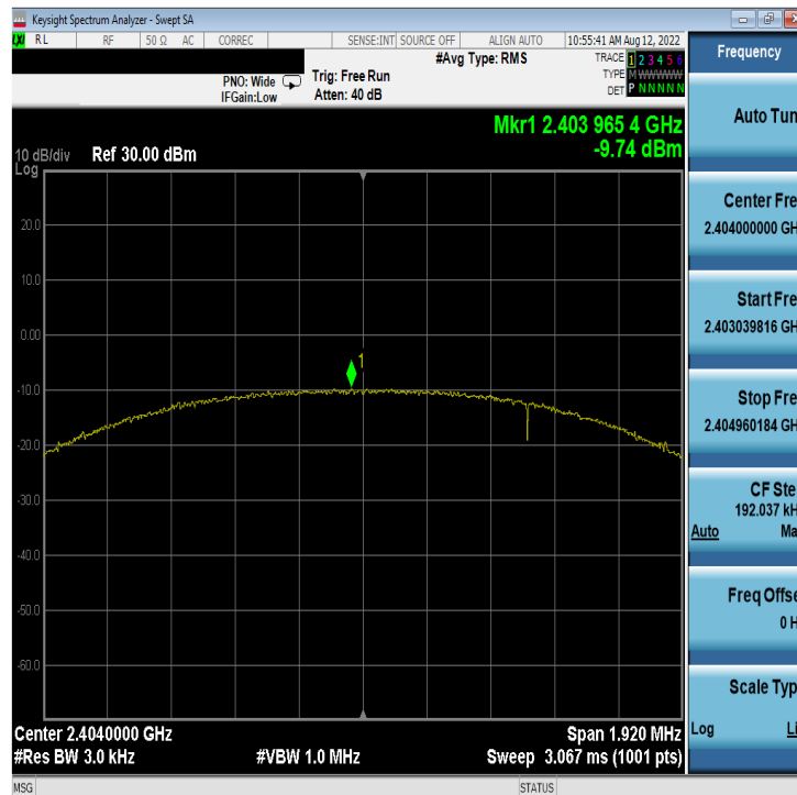
Plot 7-22. Power Spectral Density Plot Antenna WF8 (Bluetooth (LE), 2Mbps, iPA – Ch. 1)
