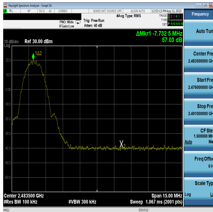
Plot 7-68. Band Edge Plot Antenna WF7b (Bluetooth (LE), 2Mbps, ePA – Ch. 38)
