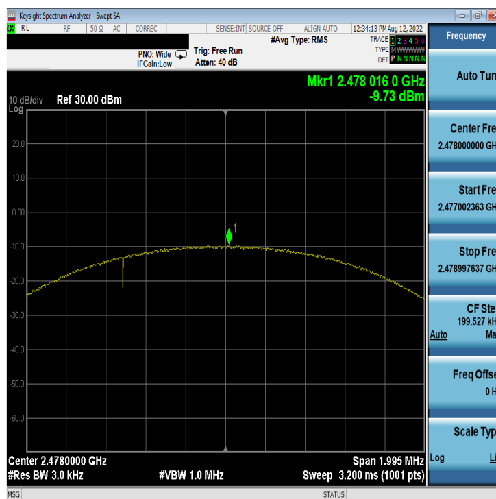
Plot 7-60. Power Spectral Density Plot Antenna WF7b (Bluetooth (LE), 2Mbps, iPA – Ch. 38)
