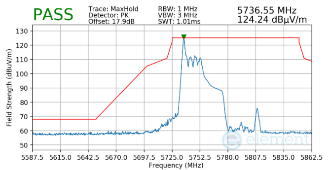
Plot 7-543. CDD (Pk, RU26, Index 0, Ch.151, MCS11)
