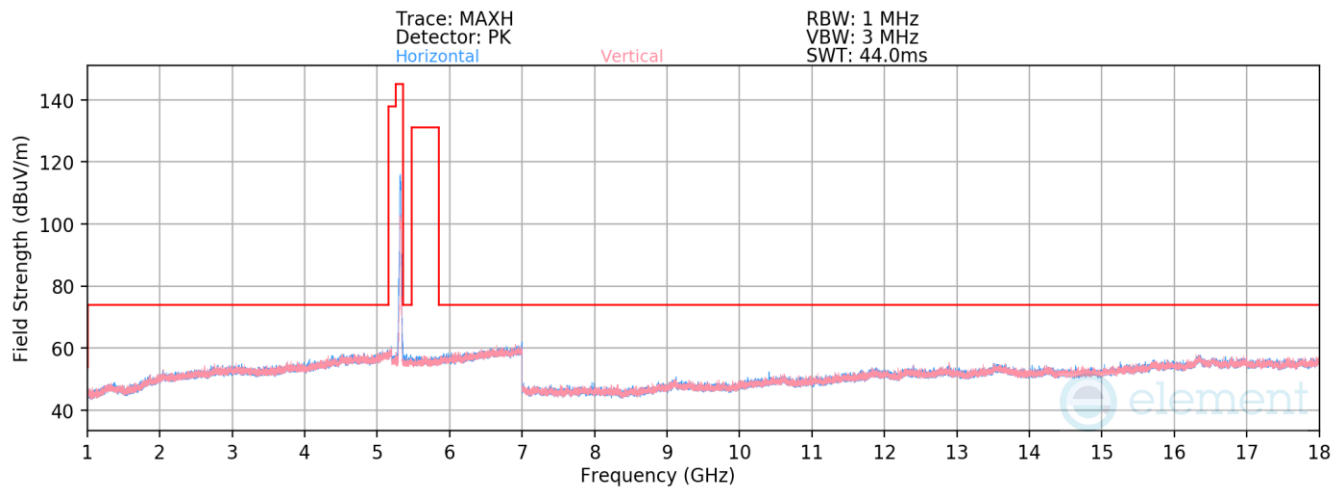
Plot 7-516. Radiated Spurious Emissions above 1GHz Antenna WF8 (802.11n – Ch. 64)
