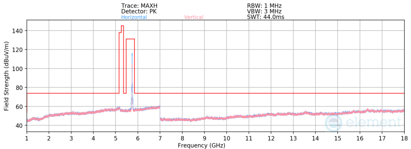
Plot 7-532. Radiated Spurious Emissions above 1GHz Antenna WF8 (802.11ax(SU) – Ch. 149)
