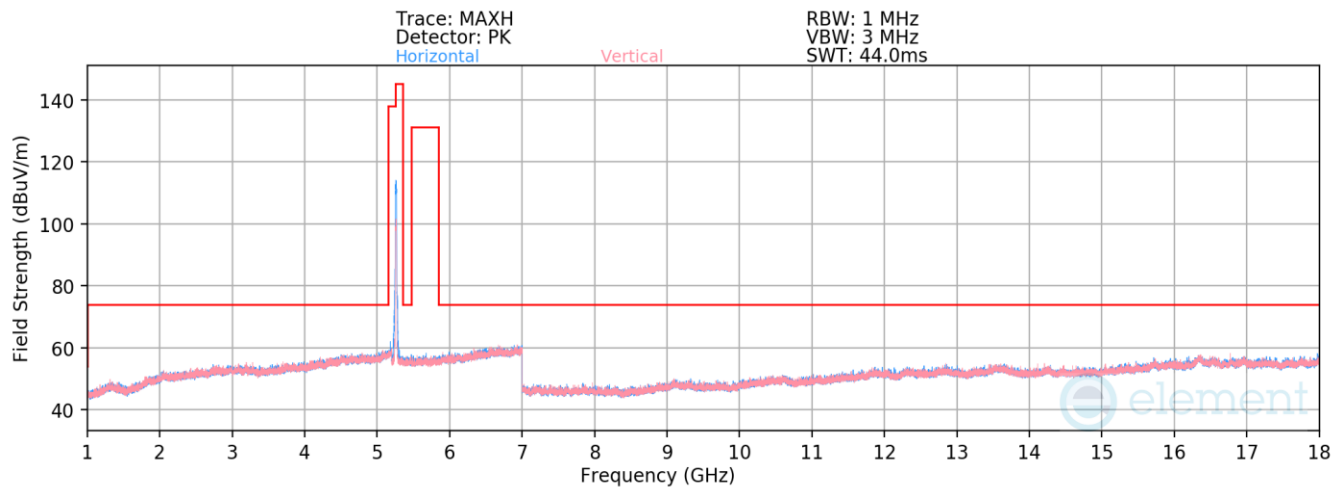
Plot 7-514. Radiated Spurious Emissions above 1GHz Antenna WF8 (802.11n – Ch. 52)
