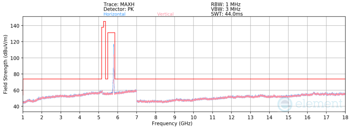
Plot 7-533. Radiated Spurious Emissions above 1GHz Antenna WF8 (802.11ax(SU) – Ch. 157)
