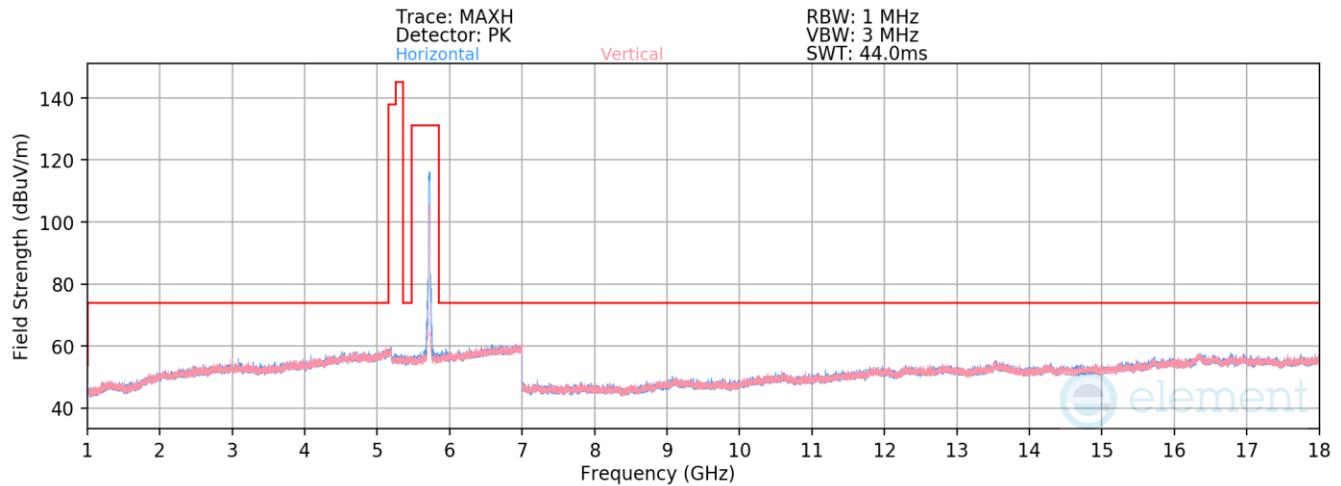
Plot 7-531. Radiated Spurious Emissions above 1GHz Antenna WF8 (802.11ax(SU) – Ch. 144)
