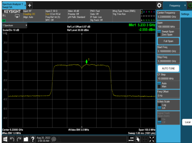
Plot 7-505. ISED PSD SDM Antenna WF8 (40MHz BW 11ax(SU) – Ch.46, MCS11)
