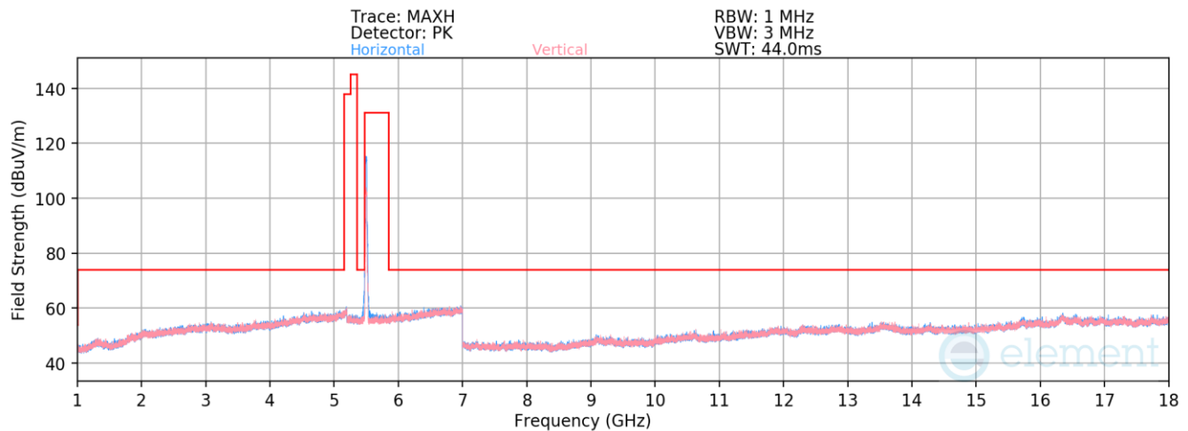
Plot 7-529. Radiated Spurious Emissions above 1GHz Antenna WF8 (802.11ax(SU) – Ch. 100)
