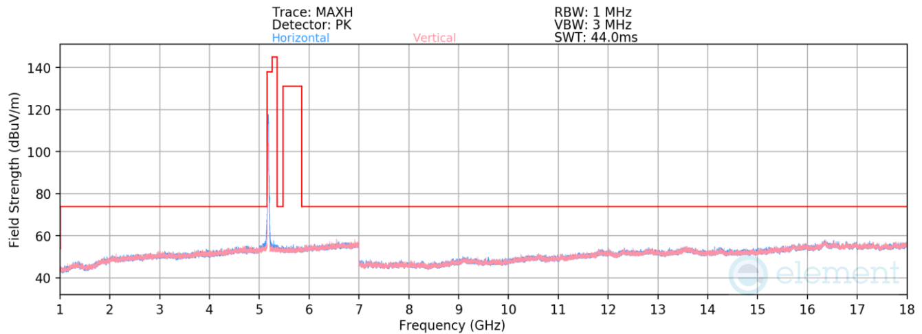
Plot 7-535. Radiated Spurious Emissions above 1GHz Antenna WF7a (802.11n – Ch. 36)
