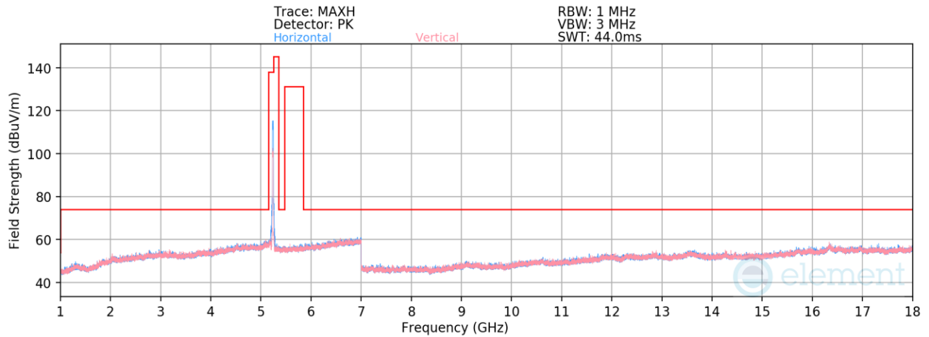
Plot 7-525. Radiated Spurious Emissions above 1GHz Antenna WF8 (802.11ax(SU) – Ch. 48)
