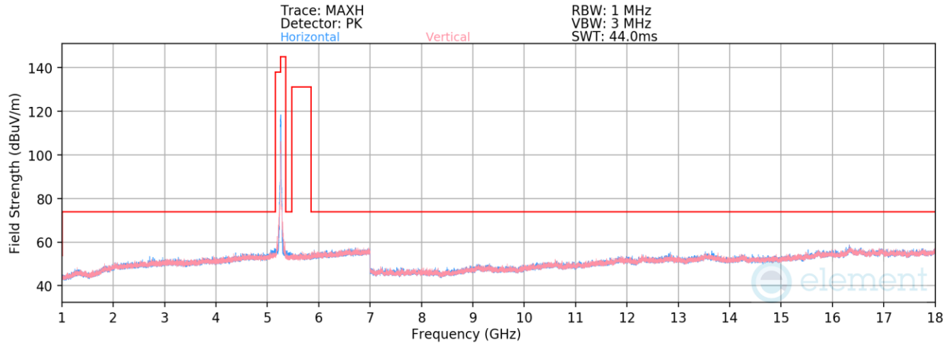
Plot 7-538. Radiated Spurious Emissions above 1GHz Antenna WF7a (802.11n – Ch. 52)
