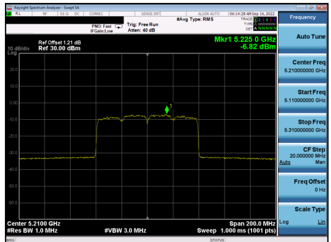
Plot 7-510. ISED PSD CDD Antenna WF7a (80MHz BW 11ax(SU) – Ch.42, MCS11)
