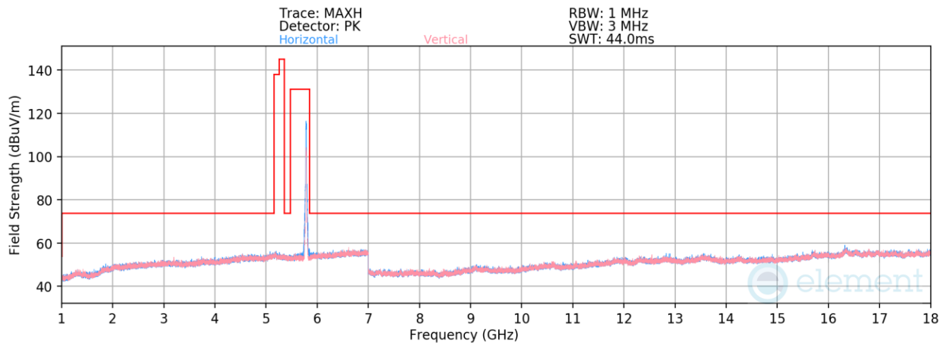
Plot 7-521. Radiated Spurious Emissions above 1GHz Antenna WF8 (802.11n – Ch. 157)
