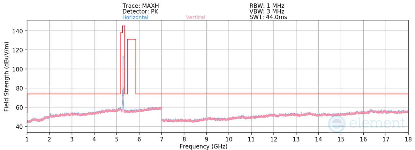
Plot 7-527. Radiated Spurious Emissions above 1GHz Antenna WF8 (802.11ax(SU) – Ch. 56)
