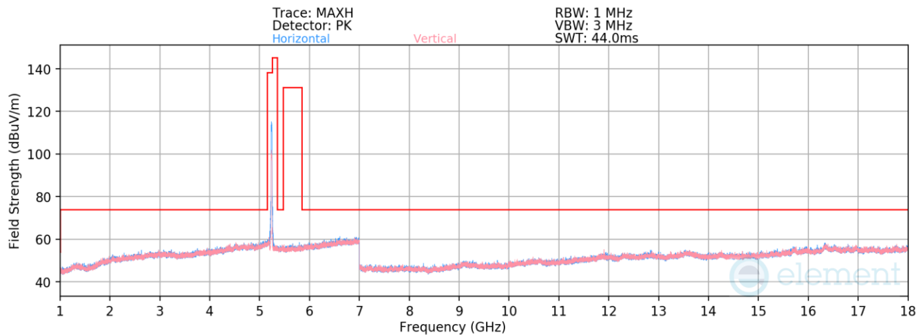
Plot 7-513. Radiated Spurious Emissions above 1GHz Antenna WF8 (802.11n – Ch. 48)
