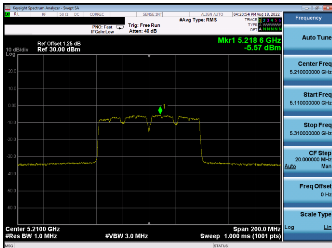
Plot 7-507. ISED PSD CDD Antenna WF8 (80MHz BW 11ac – Ch.42, MCS5)
