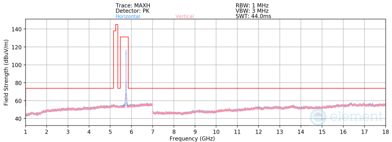
Plot 7-520. Radiated Spurious Emissions above 1GHz Antenna WF8 (802.11n – Ch. 149)
