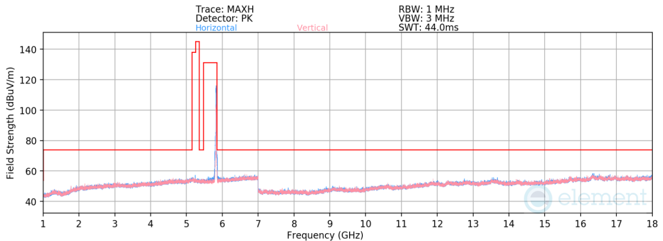
Plot 7-522. Radiated Spurious Emissions above 1GHz Antenna WF8 (802.11n – Ch. 165)
