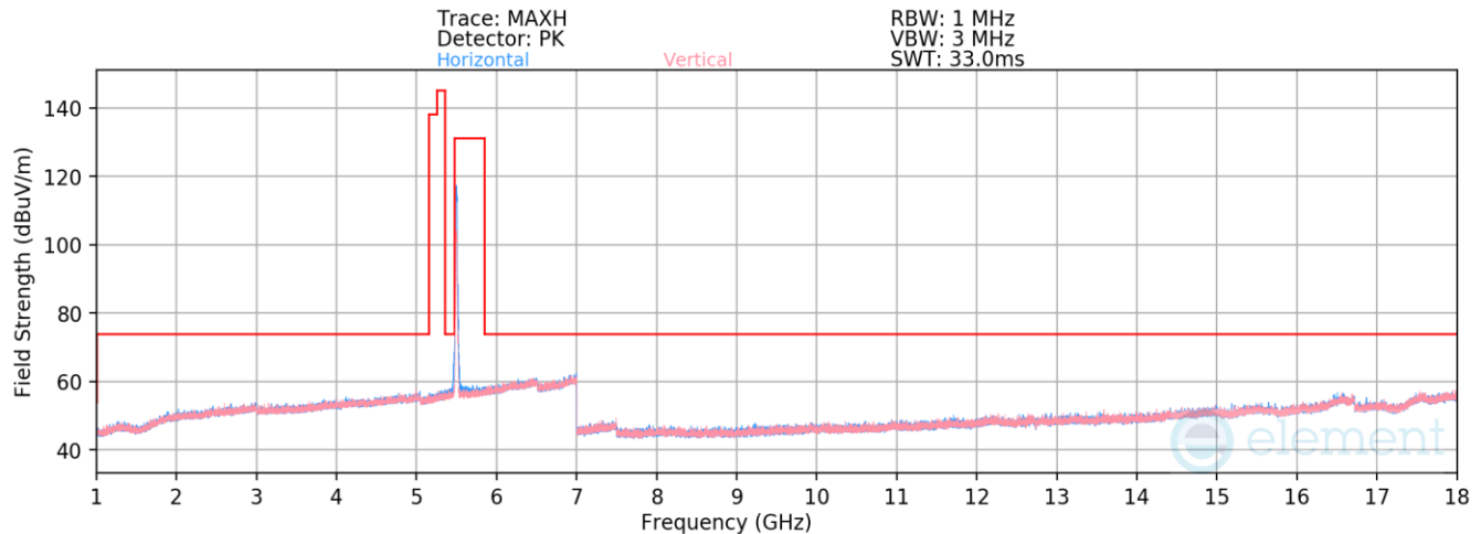
Plot 7-517. Radiated Spurious Emissions above 1GHz Antenna WF8 (802.11n – Ch. 100)
