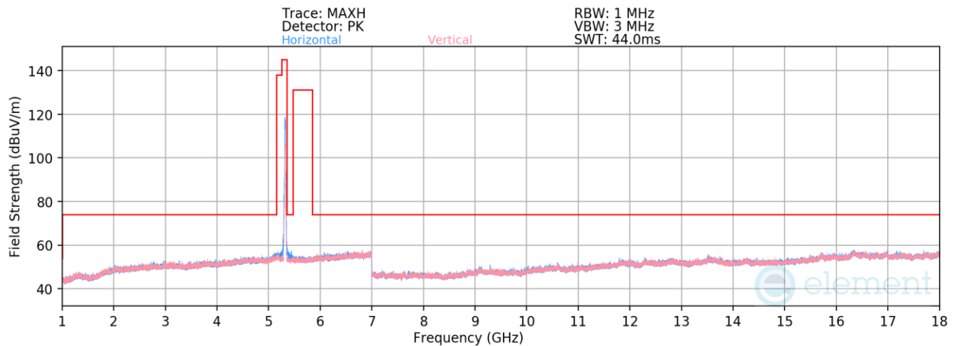
Plot 7-540. Radiated Spurious Emissions above 1GHz Antenna WF7a (802.11n – Ch. 64)
