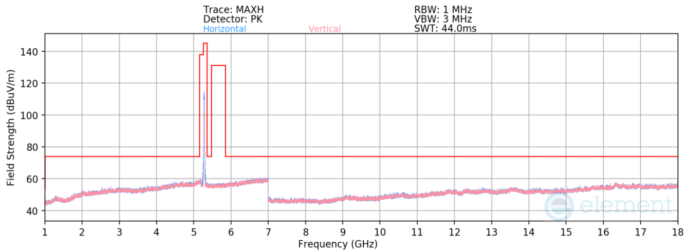
Plot 7-515. Radiated Spurious Emissions above 1GHz Antenna WF8 (802.11n – Ch. 56)
