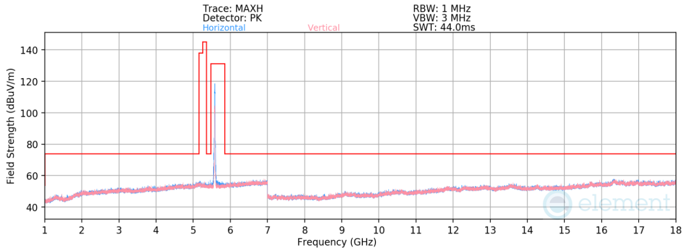
Plot 7-518. Radiated Spurious Emissions above 1GHz Antenna WF8 (802.11n – Ch. 116)
