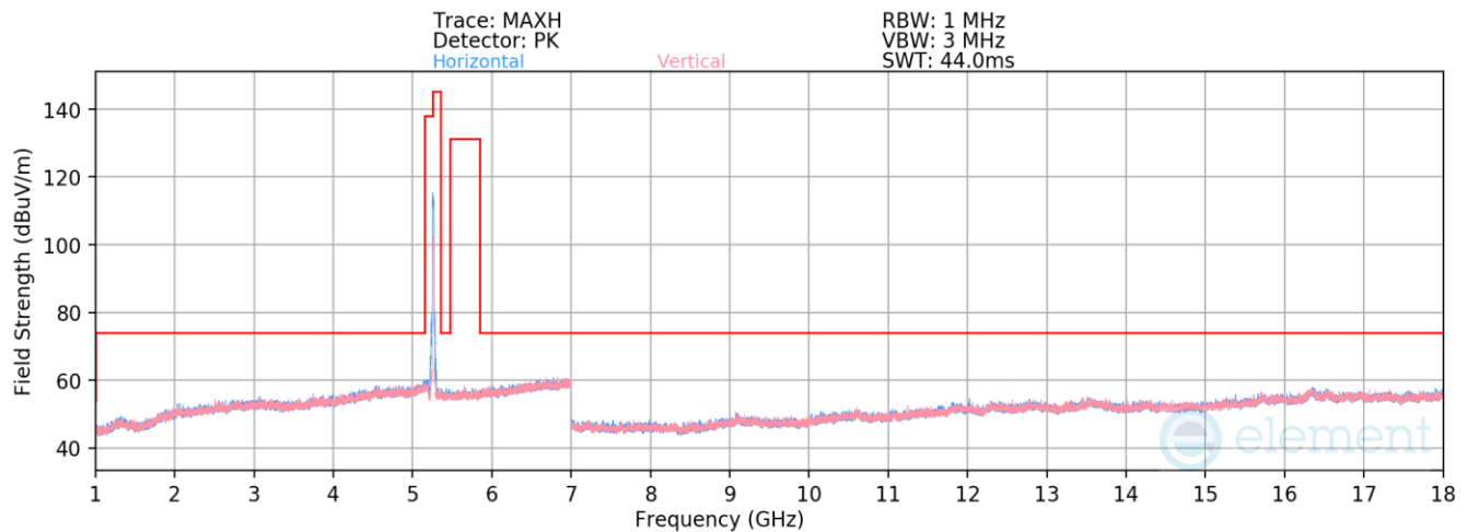
Plot 7-526. Radiated Spurious Emissions above 1GHz Antenna WF8 (802.11ax(SU) – Ch. 52)
