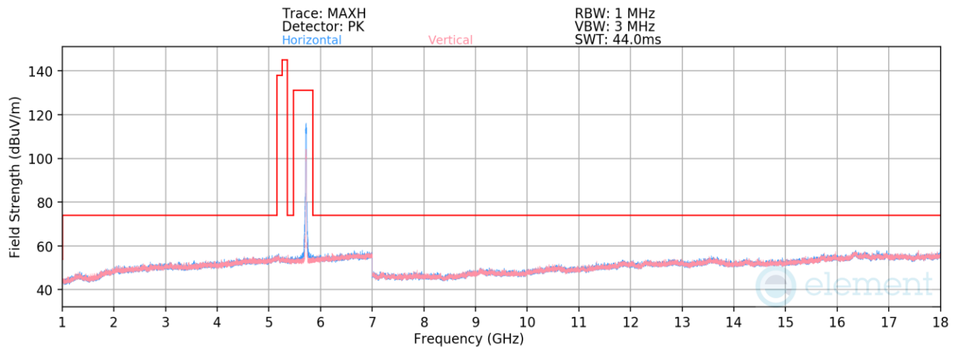
Plot 7-519. Radiated Spurious Emissions above 1GHz Antenna WF8 (802.11n – Ch. 144)
