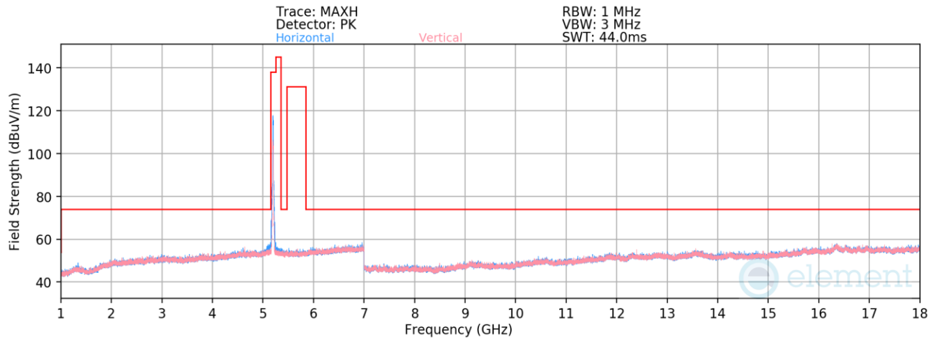
Plot 7-536. Radiated Spurious Emissions above 1GHz Antenna WF7a (802.11n – Ch. 40)
