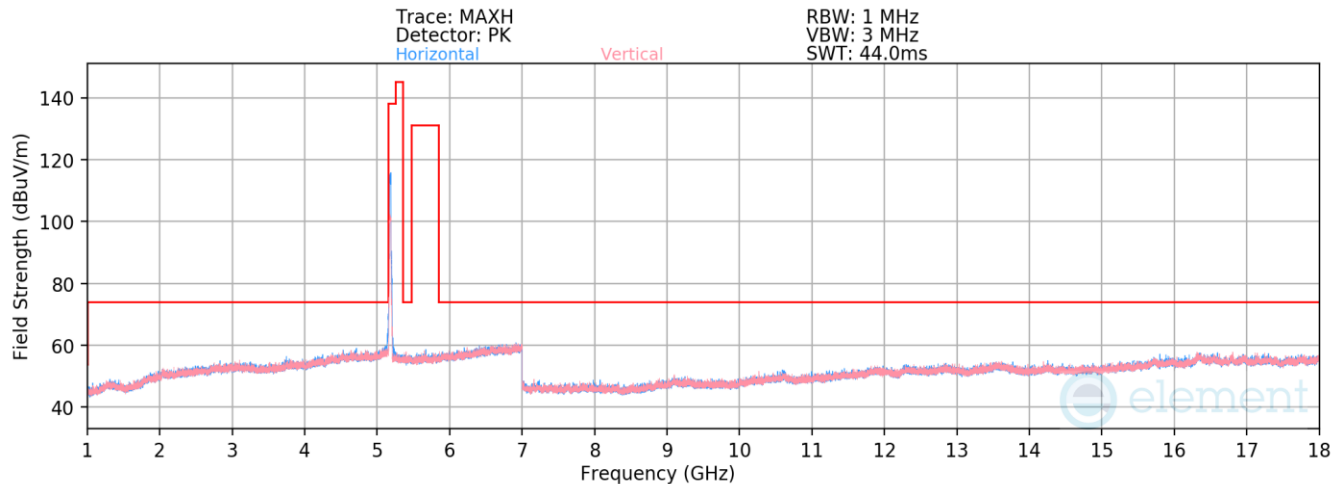
Plot 7-523. Radiated Spurious Emissions above 1GHz Antenna WF8 (802.11ax(SU) – Ch. 36)
