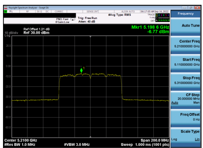
Plot 7-509. ISED PSD CDD Antenna WF8 (80MHz BW 11ax(SU) – Ch.42, MCS11)
