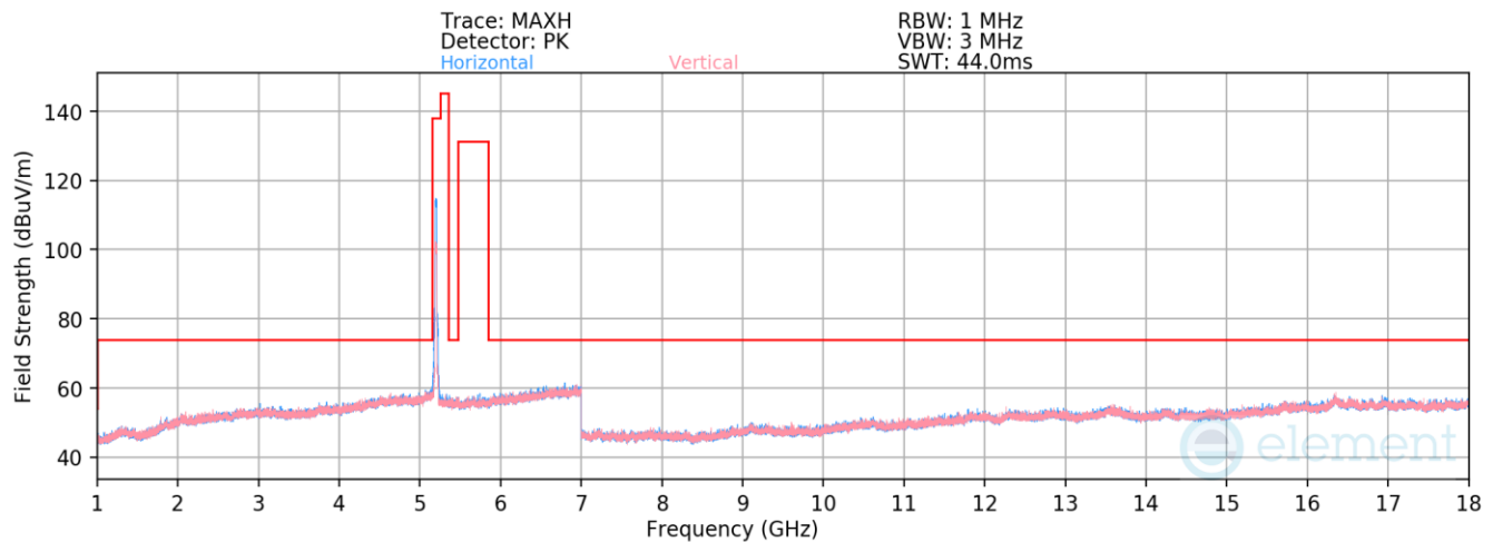
Plot 7-524. Radiated Spurious Emissions above 1GHz Antenna WF8 (802.11ax(SU) – Ch. 40)
