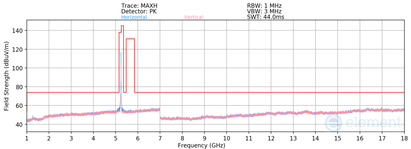
Plot 7-537. Radiated Spurious Emissions above 1GHz Antenna WF7a (802.11n – Ch. 48)
