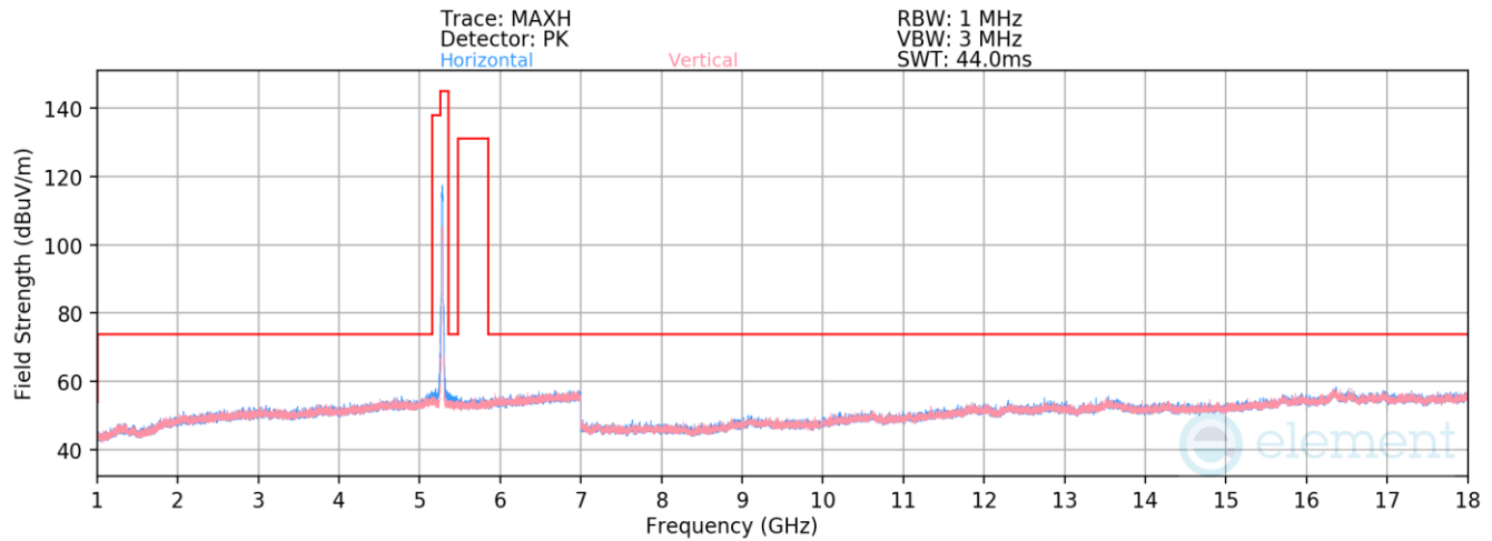
Plot 7-539. Radiated Spurious Emissions above 1GHz Antenna WF7a (802.11n – Ch. 56)
