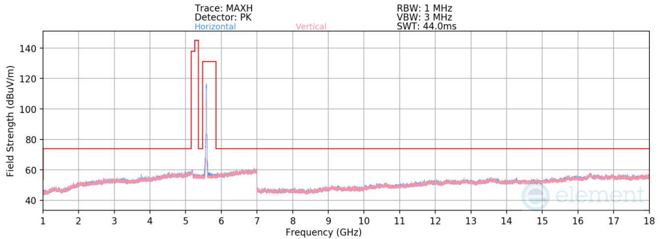
Plot 7-530. Radiated Spurious Emissions above 1GHz Antenna WF8 (802.11ax(SU) – Ch. 116)
