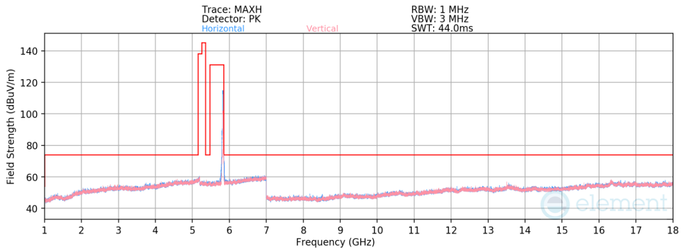
Plot 7-534. Radiated Spurious Emissions above 1GHz Antenna WF8 (802.11ax(SU) – Ch. 165)
