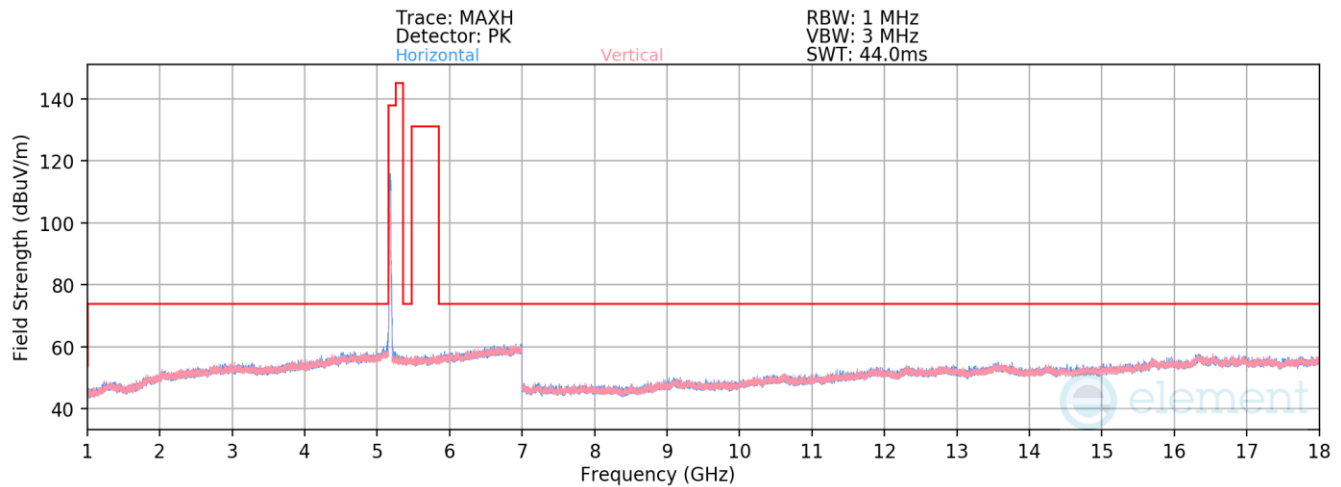
Plot 7-511. Radiated Spurious Emissions above 1GHz Antenna WF8 (802.11n – Ch. 36)
