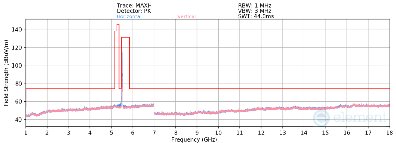
Plot 7-541. Radiated Spurious Emissions above 1GHz Antenna WF7a (802.11n – Ch. 100)
