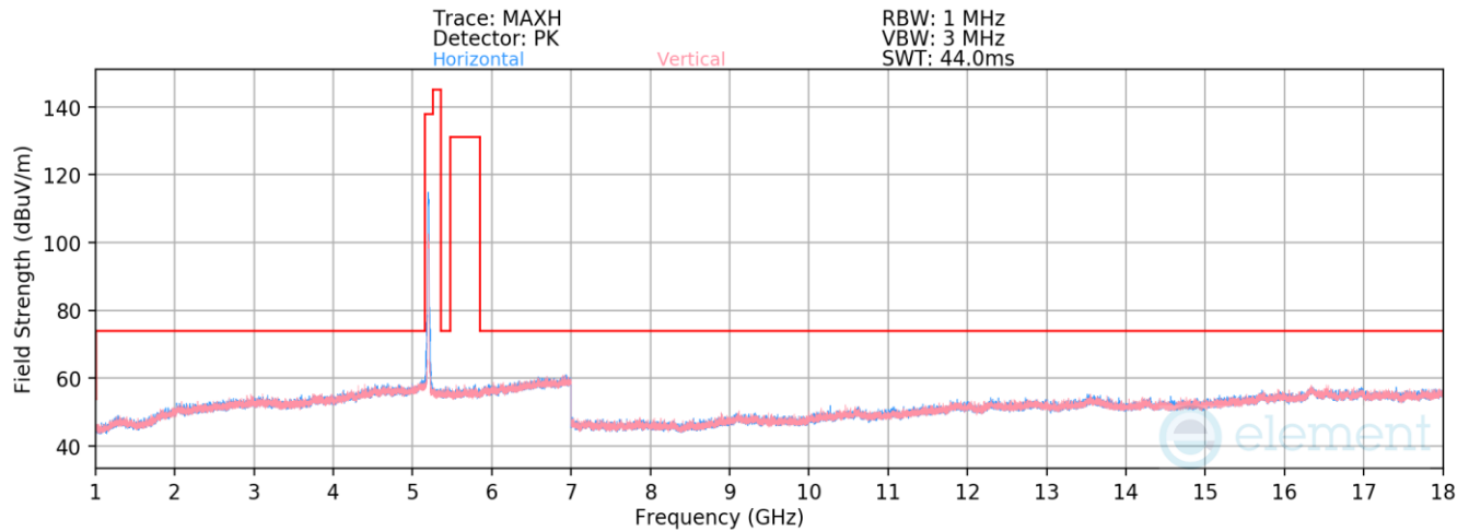
Plot 7-512. Radiated Spurious Emissions above 1GHz Antenna WF8 (802.11n – Ch. 40)
