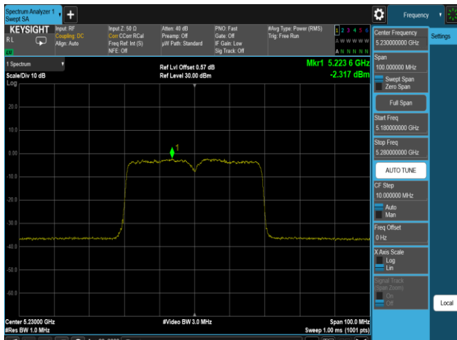
Plot 7-506. ISED PSD SDM Antenna WF7a (40MHz BW 11ax(SU) – Ch.46, MCS11)
