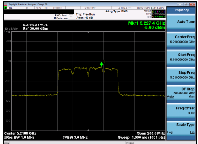
Plot 7-508. ISED PSD CDD Antenna WF7a (80MHz BW 11ac – Ch.42, MCS5)
