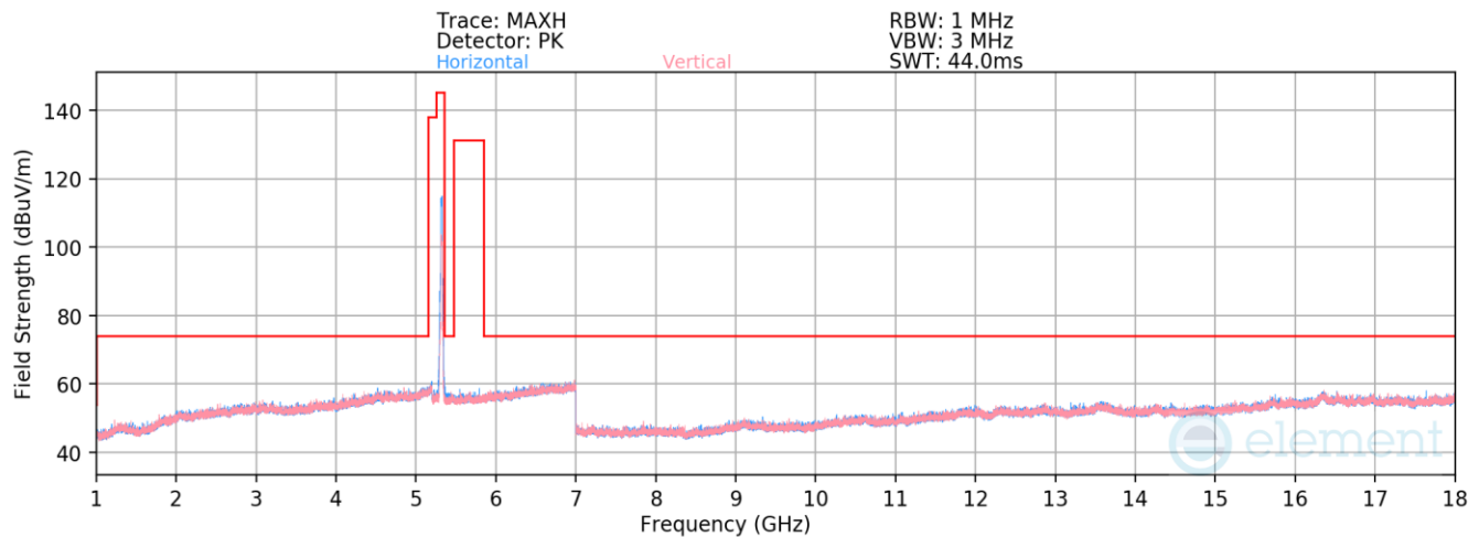
Plot 7-528. Radiated Spurious Emissions above 1GHz Antenna WF8 (802.11ax(SU) – Ch. 64)
