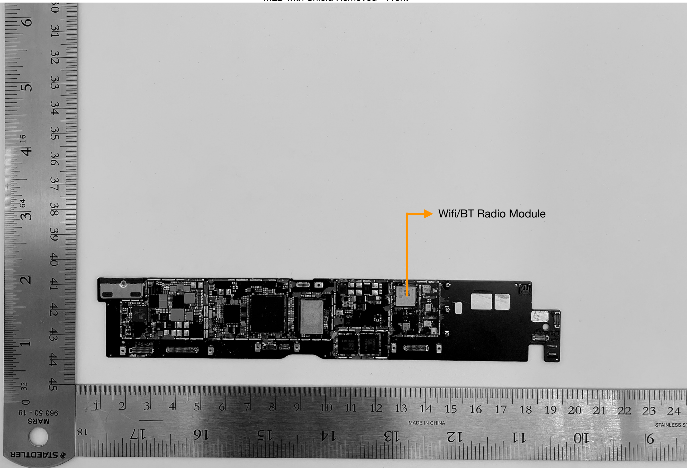
A2696 MLB with Shield Removed - Front
