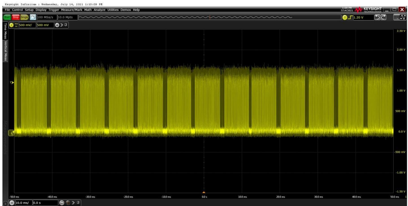
Plot 6-3. EUT RF Pulse Train (Mode 1)
