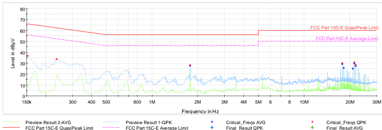
Plot 6-13. AC Line Conducted Plot (L1 - Mode 1, with Laptop)
