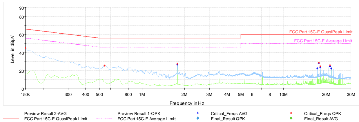
Plot 6-14. AC Line Conducted Plot (N - Mode 1, with Laptop)
