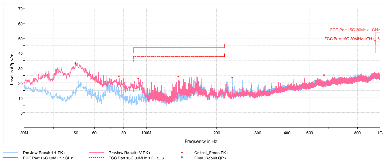
Plot 6-12. Radiated Spurious Emissions 30MHz – 1GHz (Mode 1, with Laptop)
