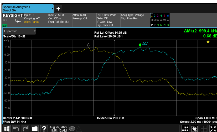
Figure 44 - 8-DPSK - 2441 MHz (CH39)
