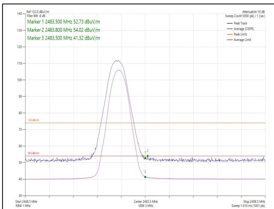
Figure 9 - Static - \pi/4 DQPSK/2DH5 - 2480 MHz - Band Edge Frequency 2483.5 MHz
