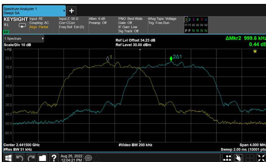
Figure 40 - \pi/4 DQPSK - 2441 MHz (CH39)
