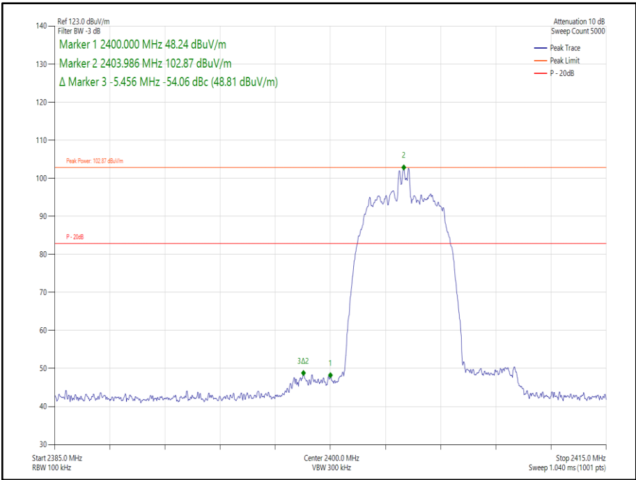
Figure 194 Core 1- \pi/4 DQPSK/HDR8 - 2404 MHz – Band Edge Frequency 2400.0 MHz
