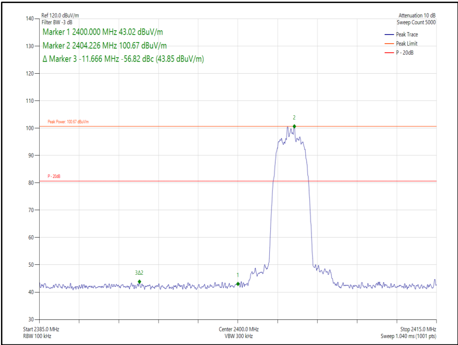
Figure 190 Core 2- \pi/4 DQPSK/HDR4 - 2404 MHz – Band Edge Frequency 2400.0 MHz
