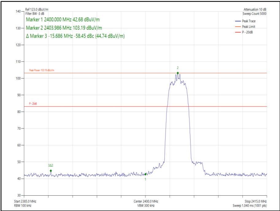
Figure 189 Core 1 - \pi/4 DQPSK/HDR4 - 2404 MHz – Band Edge Frequency 2400.0 MHz
