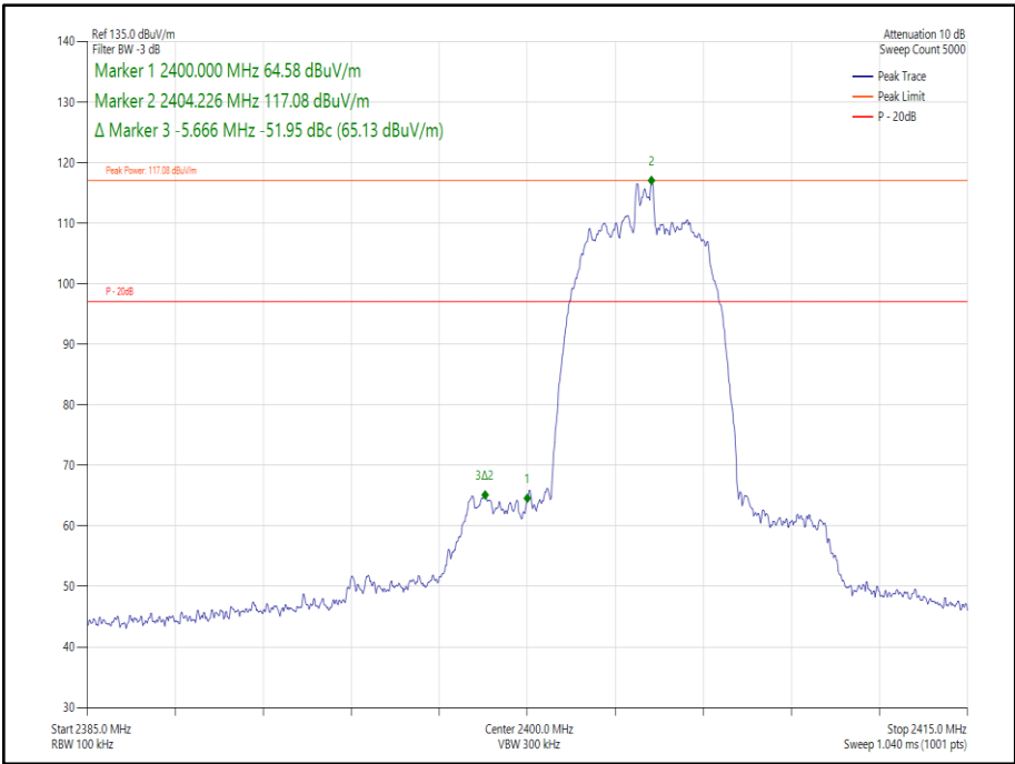
Figure 193 Core 1- \pi/4 DQPSK/HDR8 - 2404 MHz – Band Edge Frequency 2400.0 MHz
