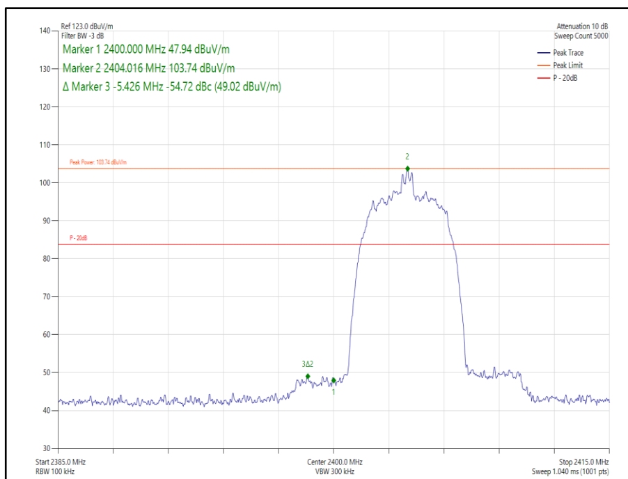
Figure 197 Core 0-1- \pi/4 DQPSK/HDR8 - 2404 MHz – Band Edge Frequency 2400.0 MHz
