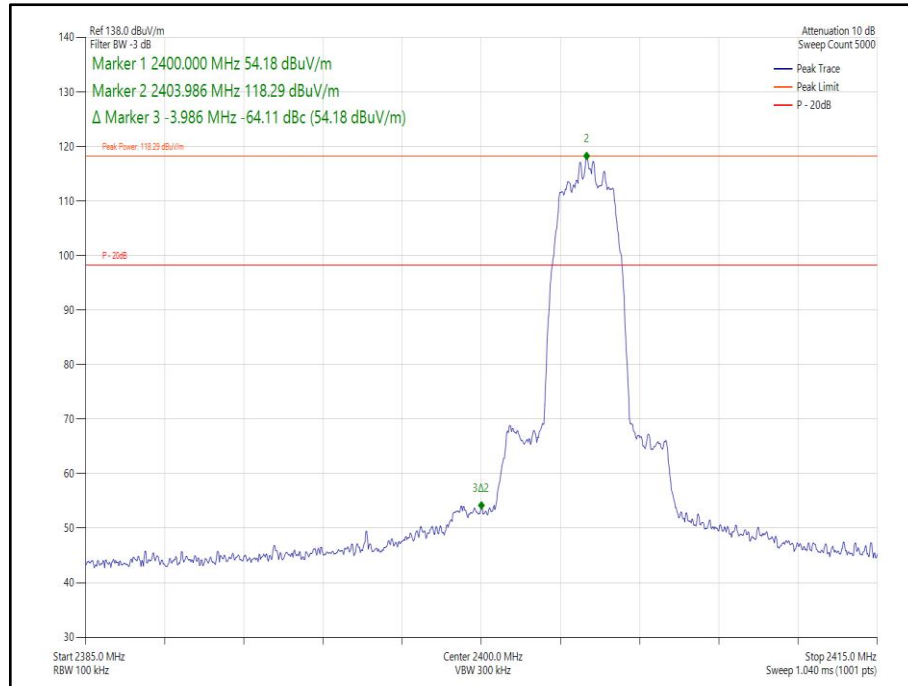
Figure 191 Core 0-1- \pi/4 DQPSK/HDR4 - 2404 MHz – Band Edge Frequency 2400.0 MHz
