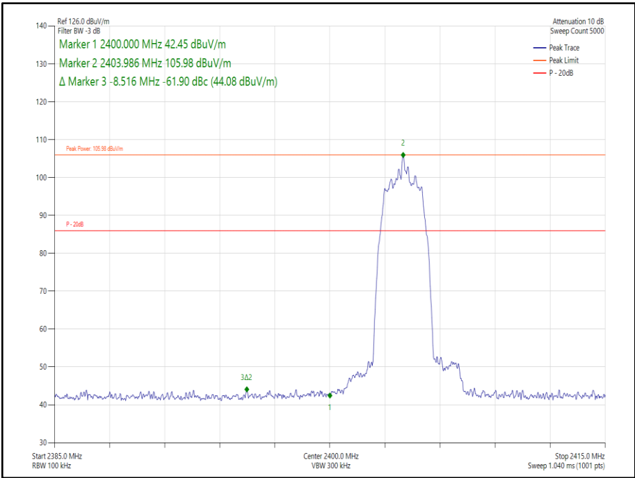
Figure 192 Core 0-1- \pi/4 DQPSK/HDR4 - 2404 MHz – Band Edge Frequency 2400.0 MHz
