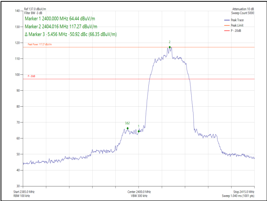
Figure 196 Core 0-1- \pi/4 DQPSK/HDR8 - 2404 MHz – Band Edge Frequency 2400.0 MHz
