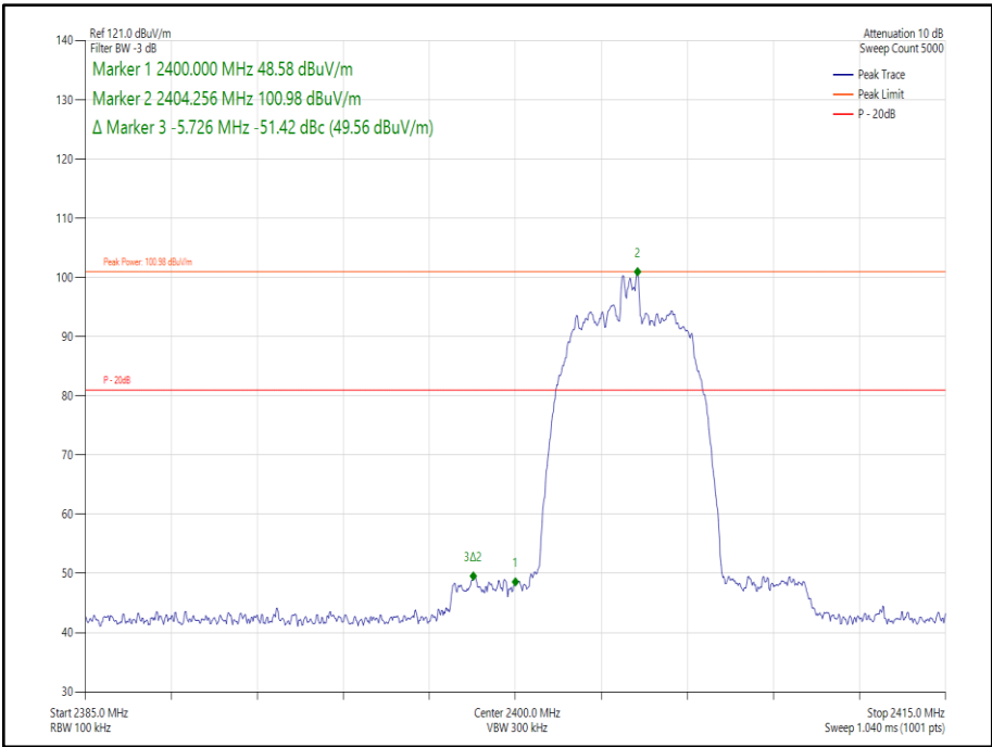
Figure 195 Core 2- \pi/4 DQPSK/HDR8 - 2404 MHz – Band Edge Frequency 2400.0 MHz
