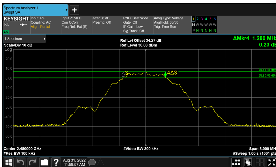
Figure 164 - Core 1 (B) 2480 MHz (CH39) 6 dB Bandwidth
