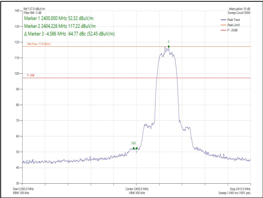
Figure 188 Core 1- \pi/4 DQPSK/HDR4 - 2404 MHz – Band Edge Frequency 2400.0 MHz
