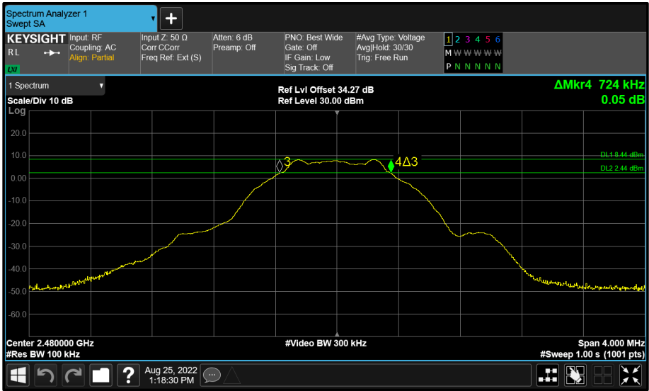
Figure 74 - Core 1 (B) 2480 MHz (CH39) 6 dB Bandwidth
