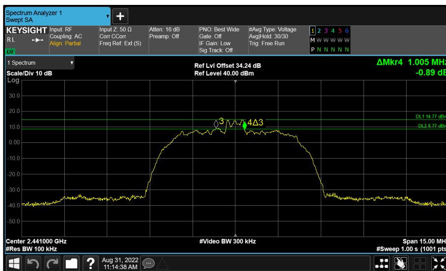
Figure 110 - Core 0 (A) 2441 MHz (CH39) 6 dB Bandwidth
