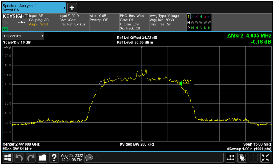
Figure 65 - Core 1 (B) 2441 MHz (CH39) 99% Bandwidth
