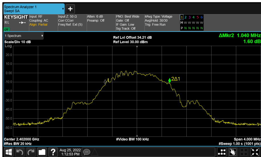
Figure 69 - Core 1 (B) 2402 MHz (CH37) 99% Bandwidth
