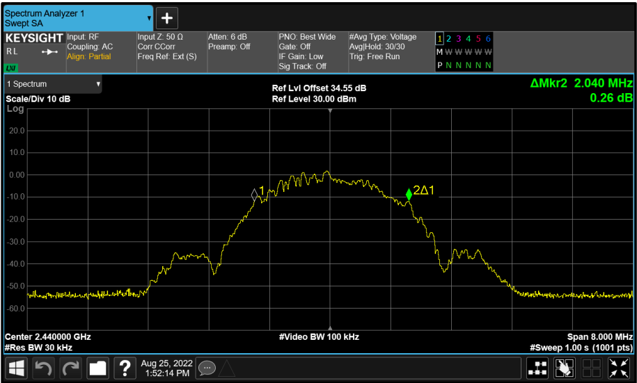
Figure 89 - BT Core 2 (C) 2440 MHz (CH17) 99% Bandwidth
