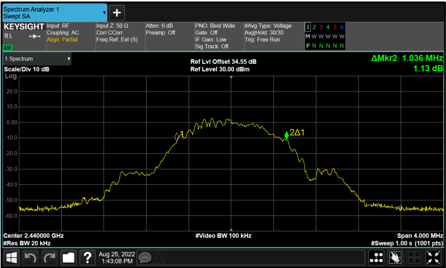
Figure 83 - BT Core 2 (C) 2440 MHz (CH17) 99% Bandwidth
