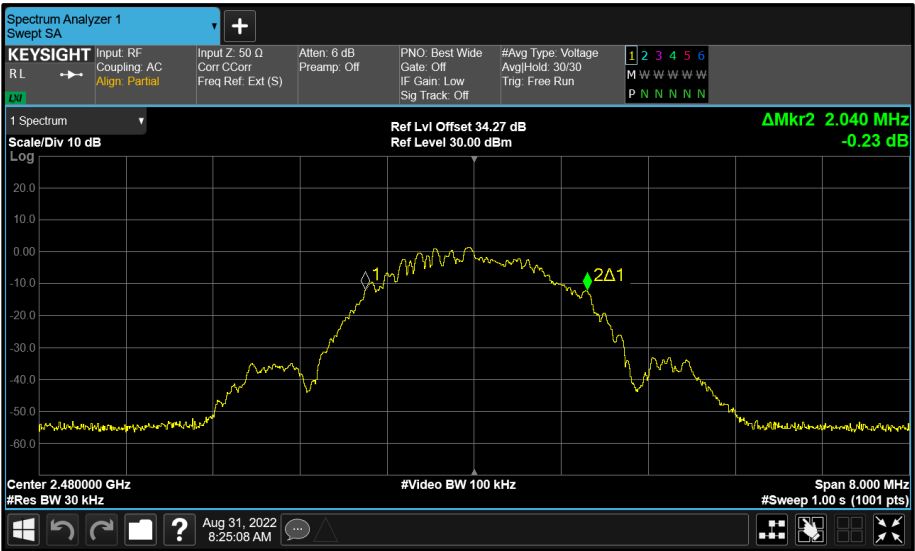
Figure 79 - Core 1 (B) 2480 MHz (CH39) 99% Bandwidth
