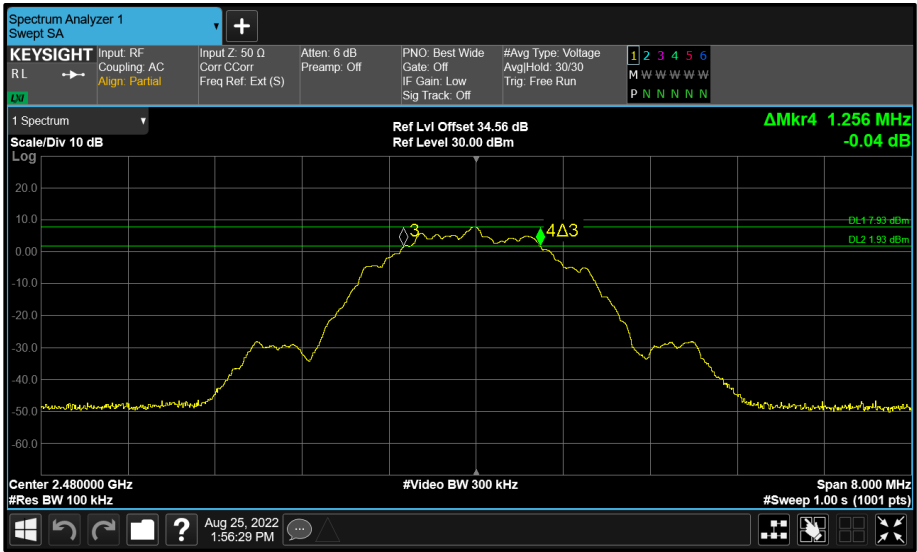
Figure 92 - BT Core 2 (C) 2480 MHz (CH39) 6 dB Bandwidth
