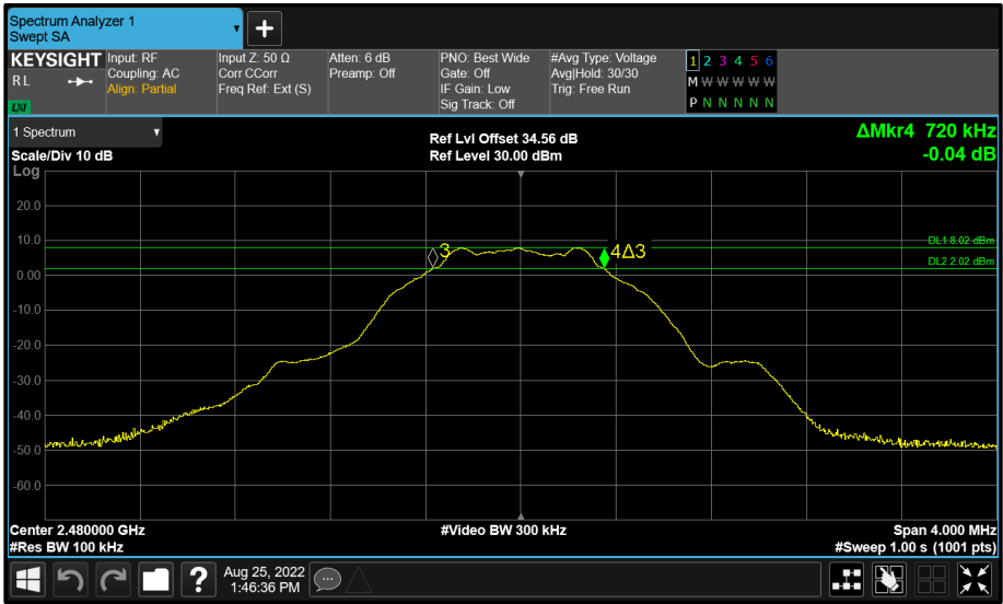
Figure 86 - BT Core 2 (C) 2480 MHz (CH39) 6 dB Bandwidth
