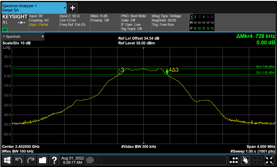
Figure 82 - BT Core 2 (C) 2402 MHz (CH37) 6 dB Bandwidth
