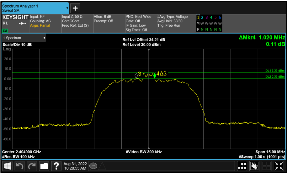
Figure 132 - Core 1 (B) 2404 MHz (CH2) 6 dB Bandwidth
