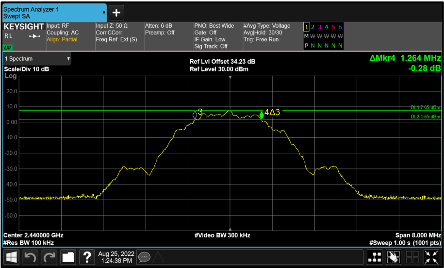
Figure 78 - Core 1 (B) 2440 MHz (CH17) 6 dB Bandwidth
