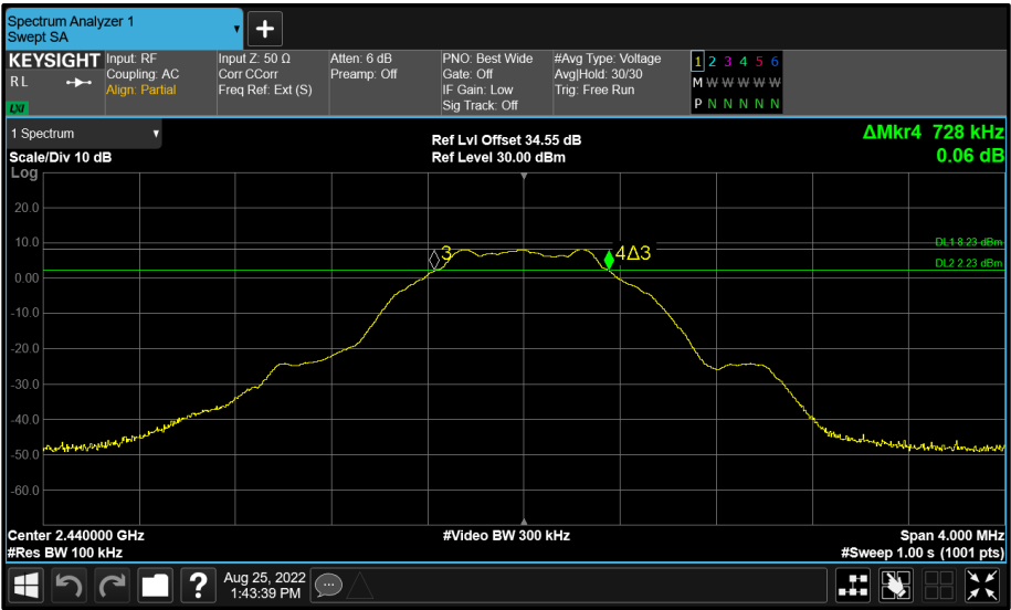
Figure 84 - BT Core 2 (C) 2440 MHz (CH17) 6 dB Bandwidth
