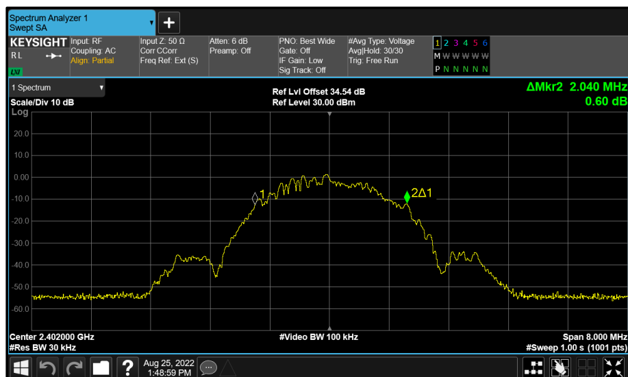
Figure 87 - BT Core 2 (C) 2402 MHz (CH37) 99% Bandwidth
