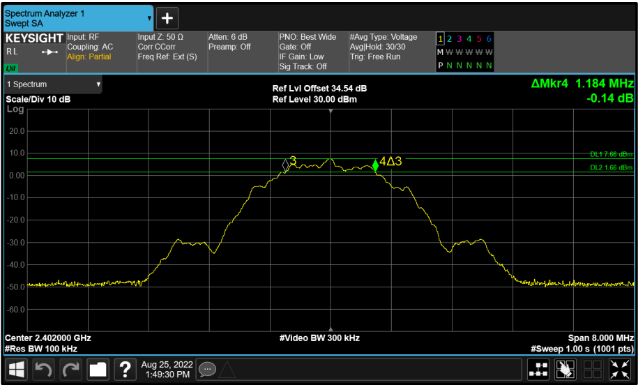
Figure 88 - BT Core 2 (C) 2402 MHz (CH37) 6 dB Bandwidth
