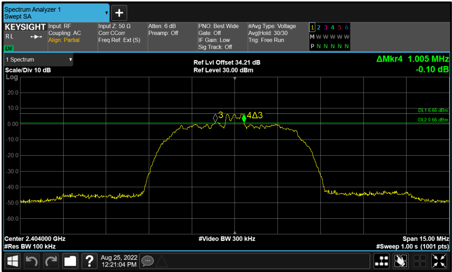
Figure 64 - Core 1 (B) 2404 MHz (CH2) 6 dB Bandwidth
