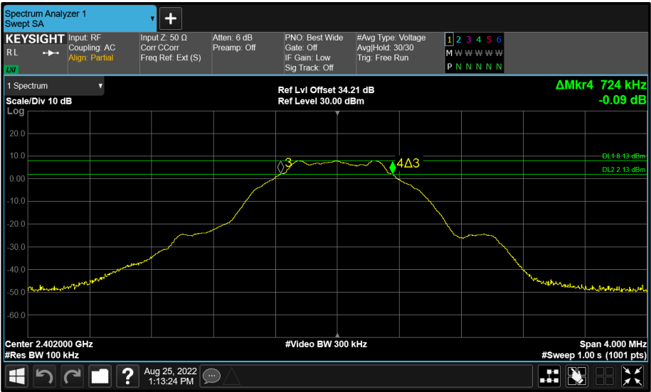
Figure 70 - Core 1 (B) 2402 MHz (CH37) 6 dB Bandwidth
