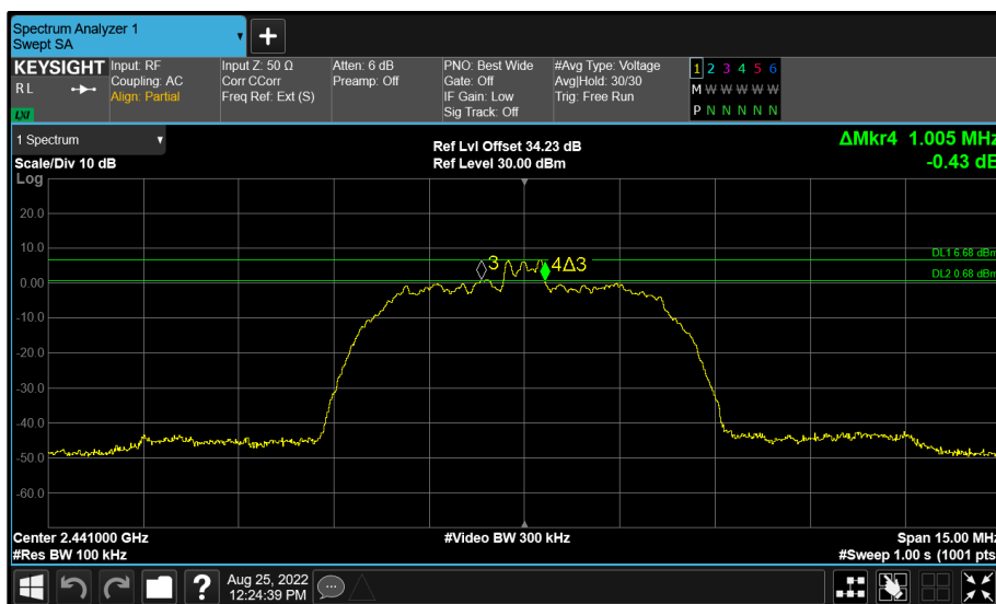
Figure 66 - Core 1 (B) 2441 MHz (CH39) 6 dB Bandwidth
