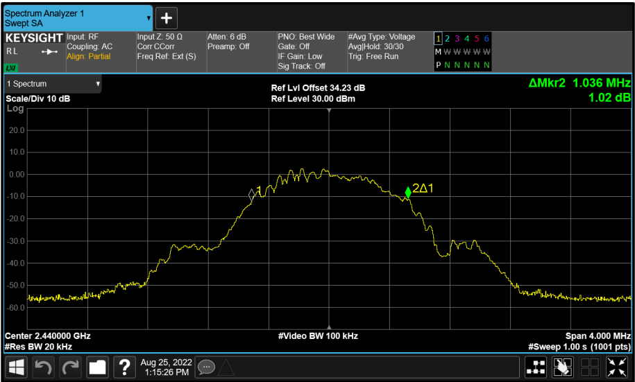
Figure 71 - Core 1 (B) 2440 MHz (CH17) 99% Bandwidth
