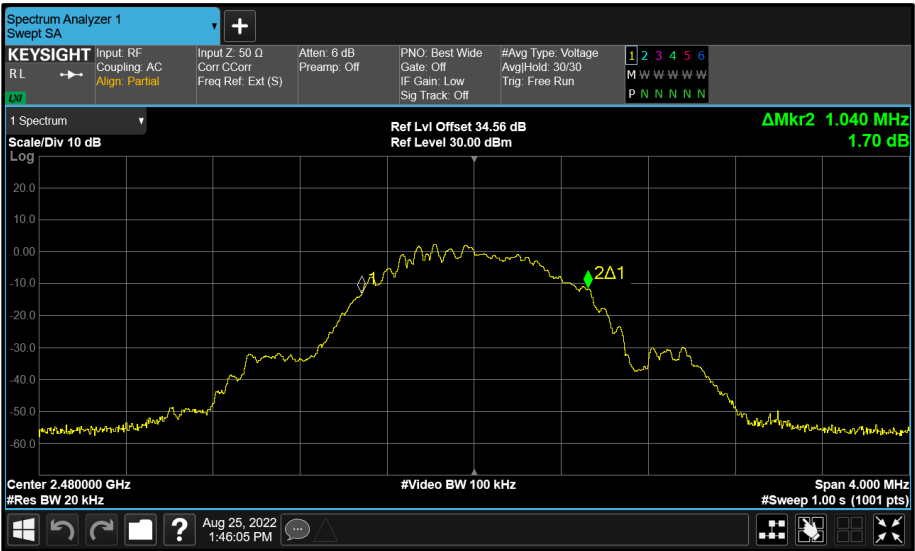
Figure 85 - BT Core 2 (C) 2480 MHz (CH39) 99% Bandwidth
