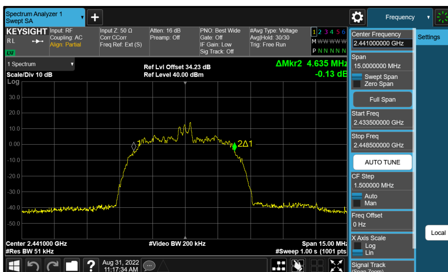
Figure 111 - Core 1 (B) 2441 MHz (CH39) 99% Bandwidth
