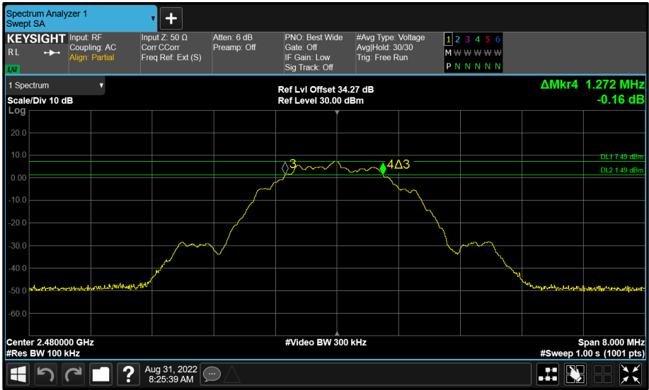
Figure 80 - Core 1 (B) 2480 MHz (CH39) 6 dB Bandwidth
