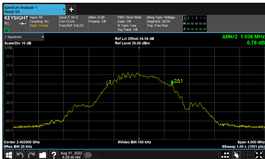
Figure 81 - BT Core 2 (C) 2402 MHz (CH37) 99% Bandwidth
