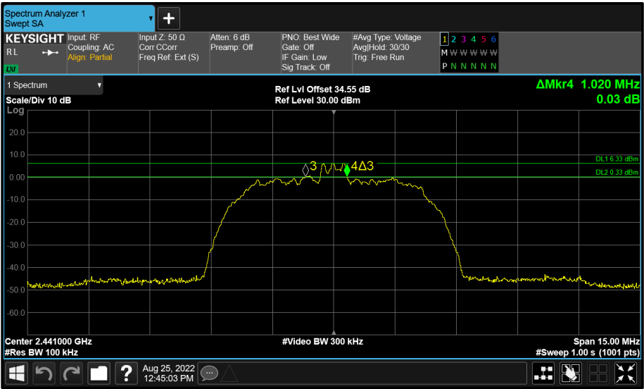
Figure 54 - BT Core 2 (C) 2441 MHz (CH39) 6 dB Bandwidth
