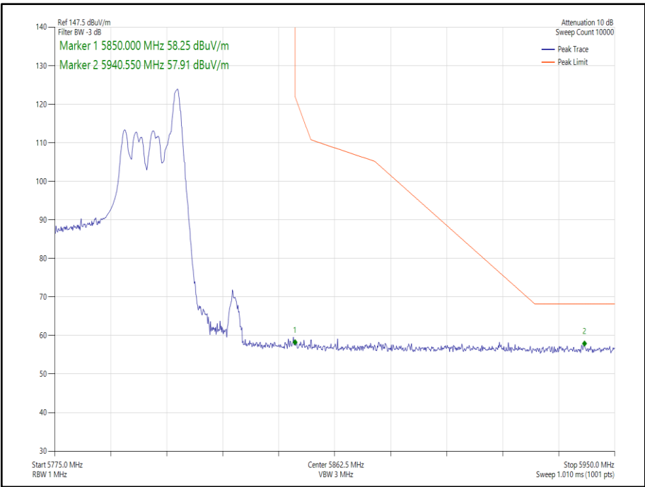
Figure 248 - 802.11ax HE40 SDM, Cores 0-1, RU26-17 - 5795 MHz Band Edge Frequency 5850 MHz
