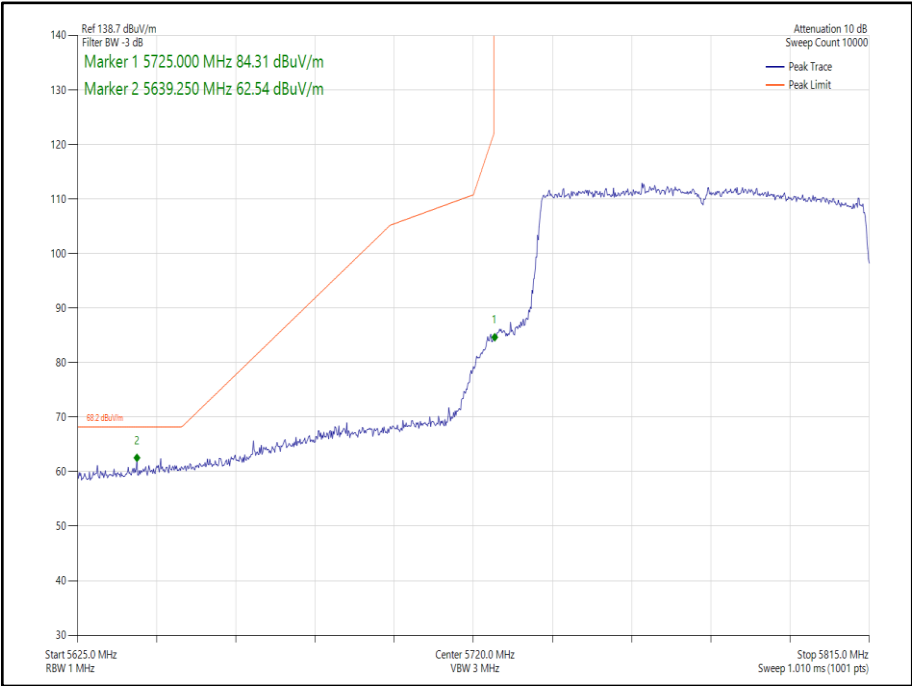
Figure 256 - 802.11ax HE80 Core 1 SU - 5775 MHz Band Edge Frequency 5725 MHz
