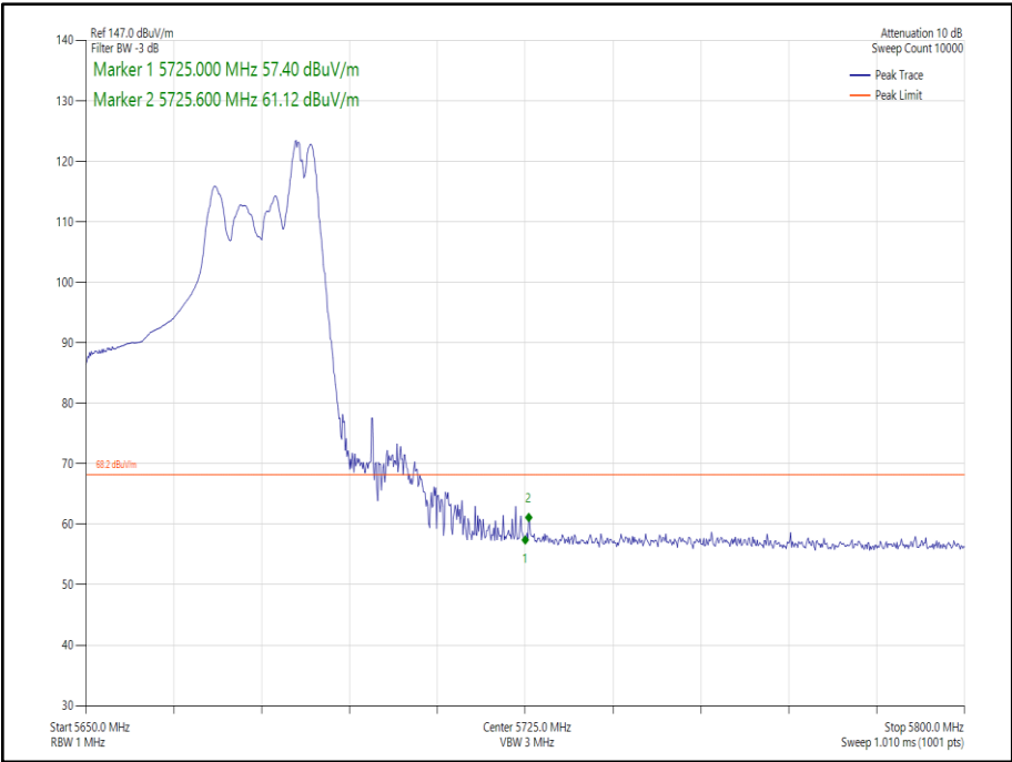
Figure 236 - 802.11ax HE40 SDM, Cores 0-1, RU52-44 - 5670 MHz Band Edge Frequency 5725 MHz
