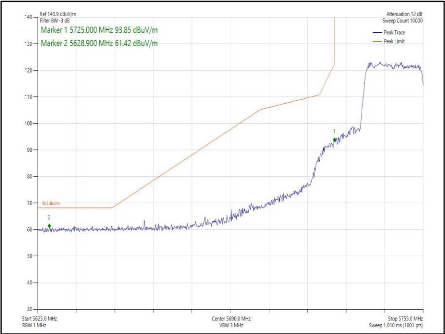
Figure 205 - 802.11ax HE20 SDM, Cores 0-1, SU - 5745 MHz Band Edge Frequency 5725 MHz
