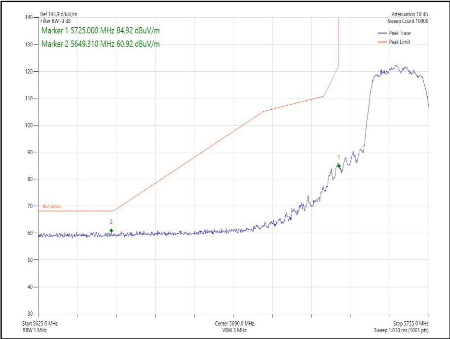
Figure 201 - 802.11n HT20 CDD, Cores 0-1 - 5745 MHz Band Edge Frequency 5725 MHz
