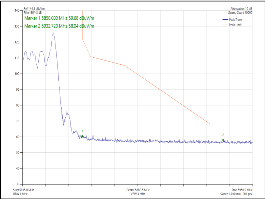
Figure 212 - 802.11ax HE20 SDM, Cores 0-1, RU26-8 - 5825 MHz Band Edge Frequency 5850 MHz
