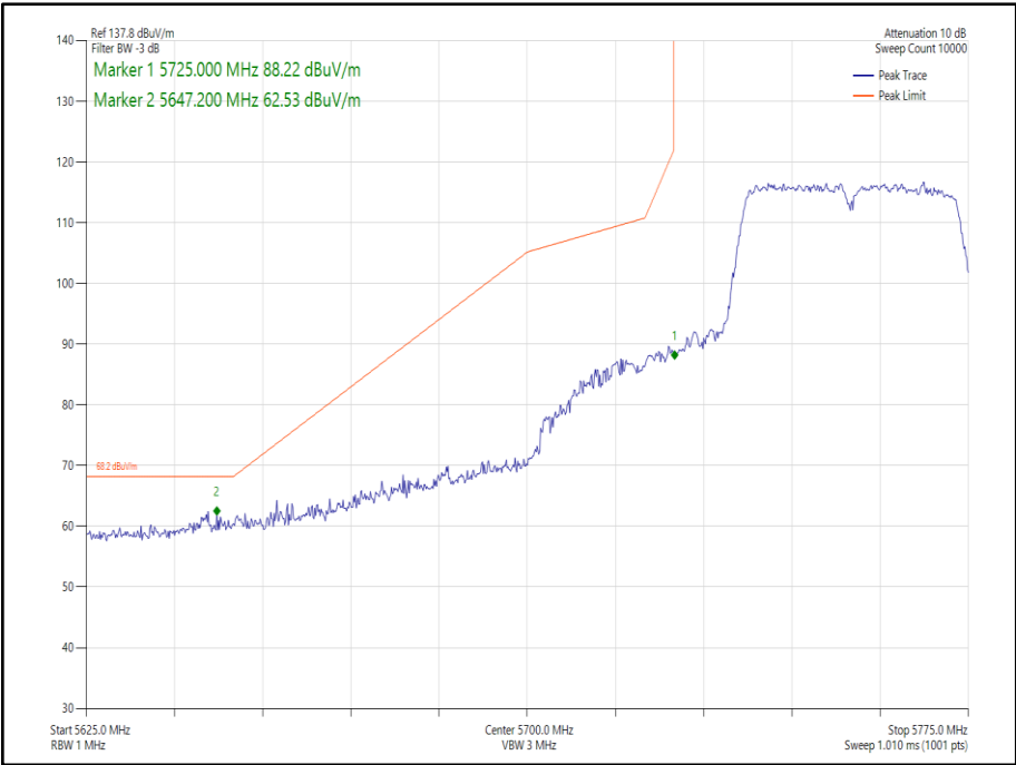
Figure 219 - 802.11n HT40, Core 1 - 5755 MHz Band Edge Frequency 5725 MHz
