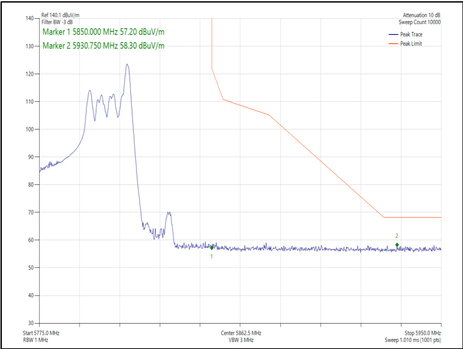
Figure 246 - 802.11ax HE40 CDD, Cores 0-1, RU26-17 - 5795 MHz Band Edge Frequency 5850 MHz
