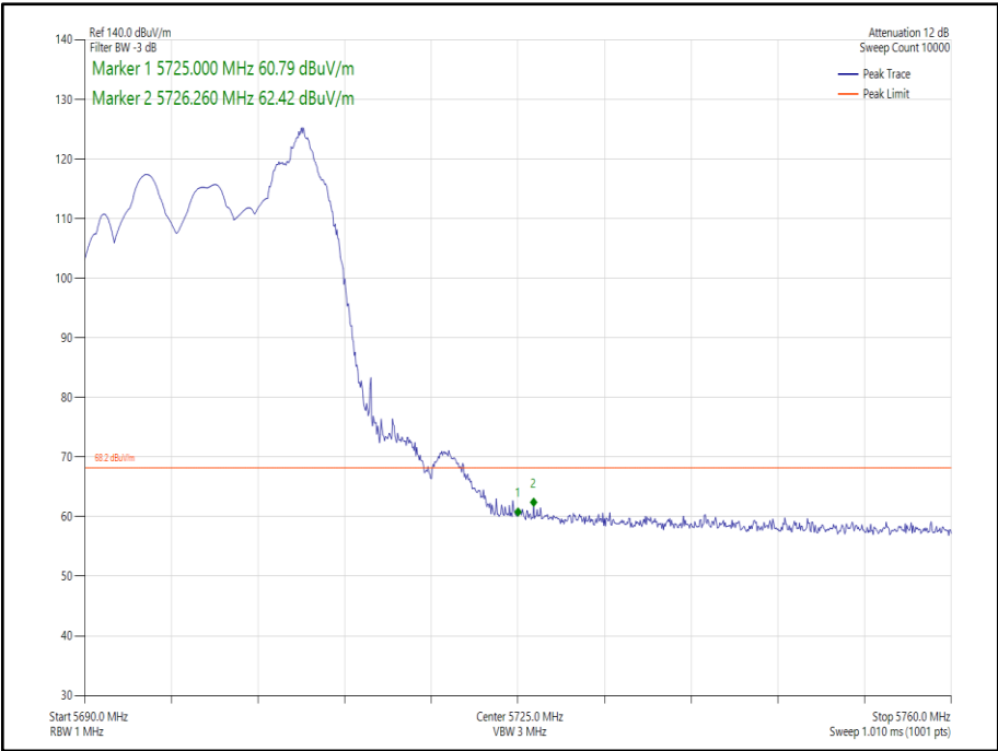
Figure 200 - 802.11ax HE20 SDM, Cores 0-1, RU52-40 - 5700 MHz Band Edge Frequency 5725 MHz
