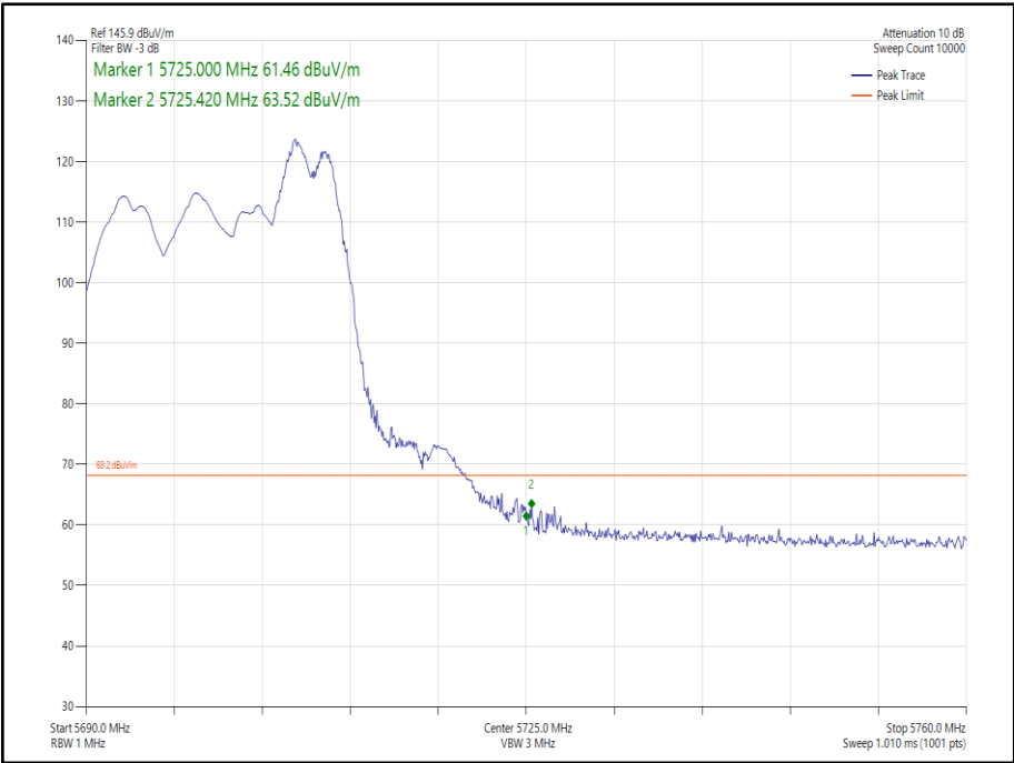
Figure 198 - 802.11ax HE20 CDD, Cores 0-1, RU52-40 - 5700 MHz Band Edge Frequency 5725 MHz
