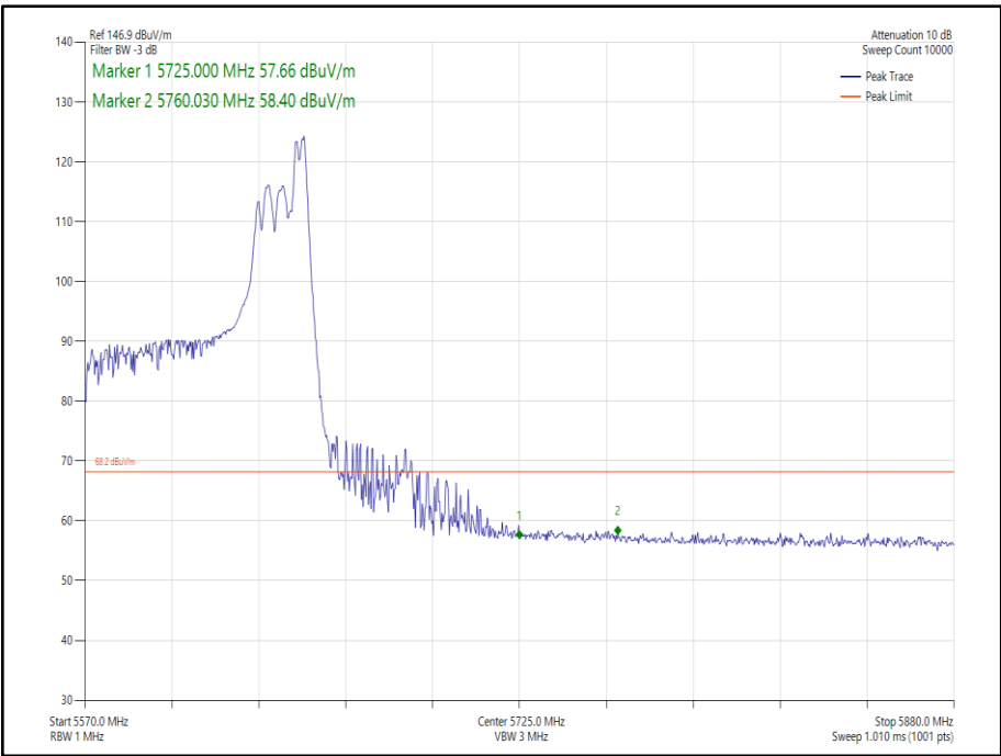
Figure 272 - 802.11ax HE80 SDM, Cores 0-1, RU26-36 - 5610 MHz Band Edge Frequency 5725 MHz
