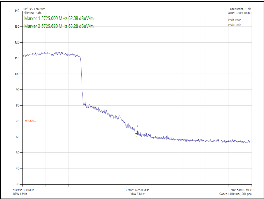
Figure 271 - 802.11ax HE80 SDM, Cores 0-1, SU - 5610 MHz Band Edge Frequency 5725 MHz
