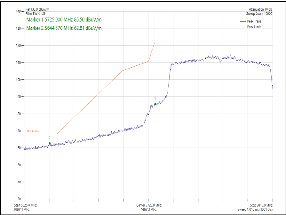
Figure 255 - 802.11ac VHT80 Core 1 - 5775 MHz Band Edge Frequency 5725 MHz
