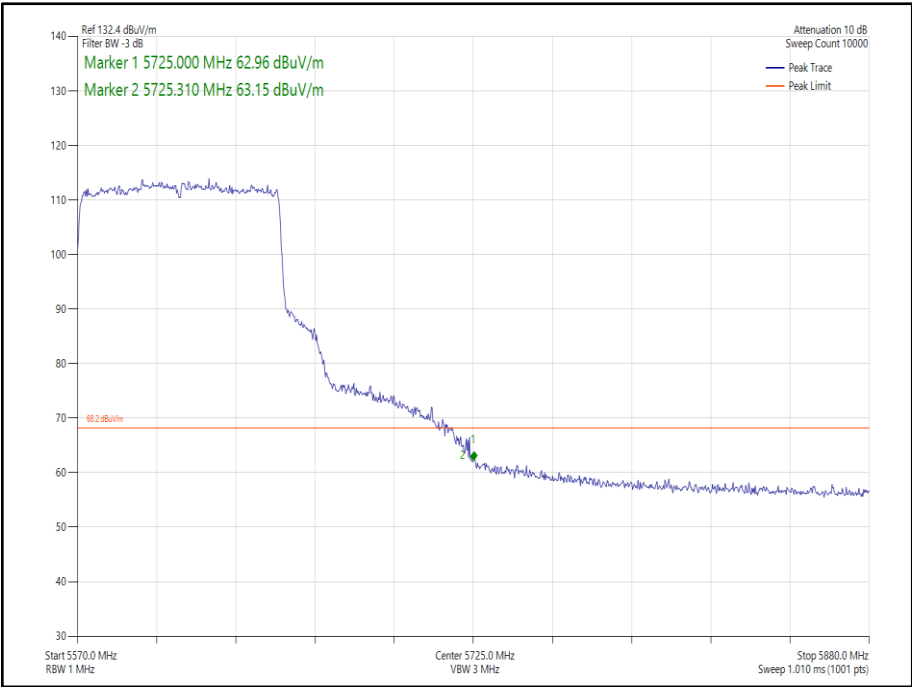
Figure 253 - 802.11ax HE80 Core 1 SU - 5610 MHz Band Edge Frequency 5725 MHz
