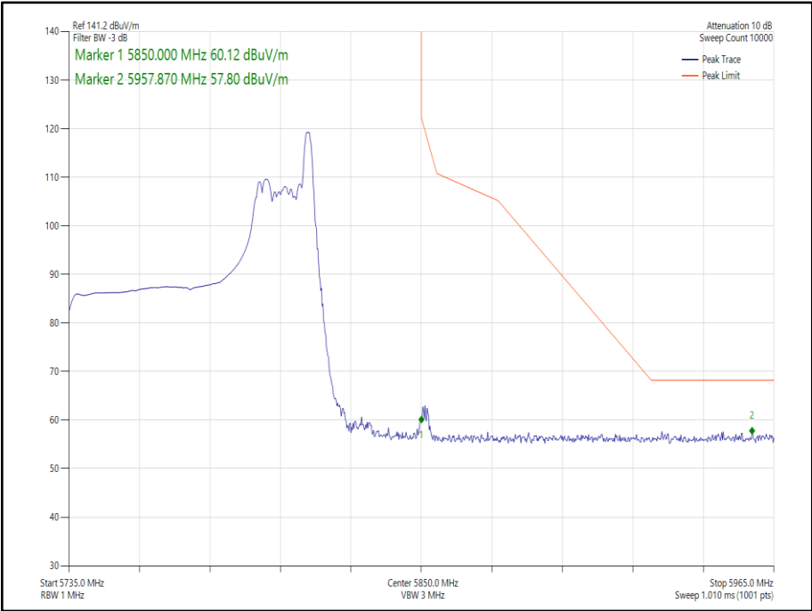
Figure 260 - 802.11ax HE80 Core 1 RU26-36 - 5775 MHz Band Edge Frequency 5850 MHz
