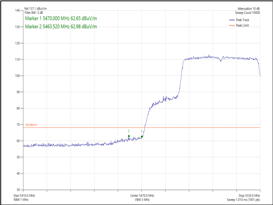
Figure 214 - 802.11ax HE40, Core 1, SU - 5510 MHz Band Edge Frequency 5470 MHz
