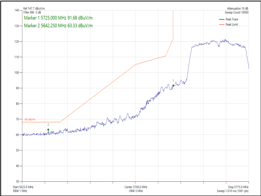
Figure 238 - 802.11n HT40 SDM, Cores 0-1 - 5755 MHz Band Edge Frequency 5725 MHz
