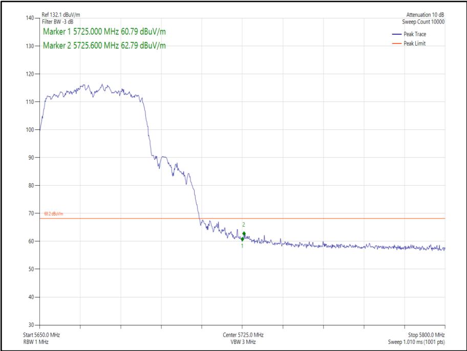
Figure 231 - 802.11n HT40 CDD, Cores 0-1 - 5670 MHz Band Edge Frequency 5725 MHz
