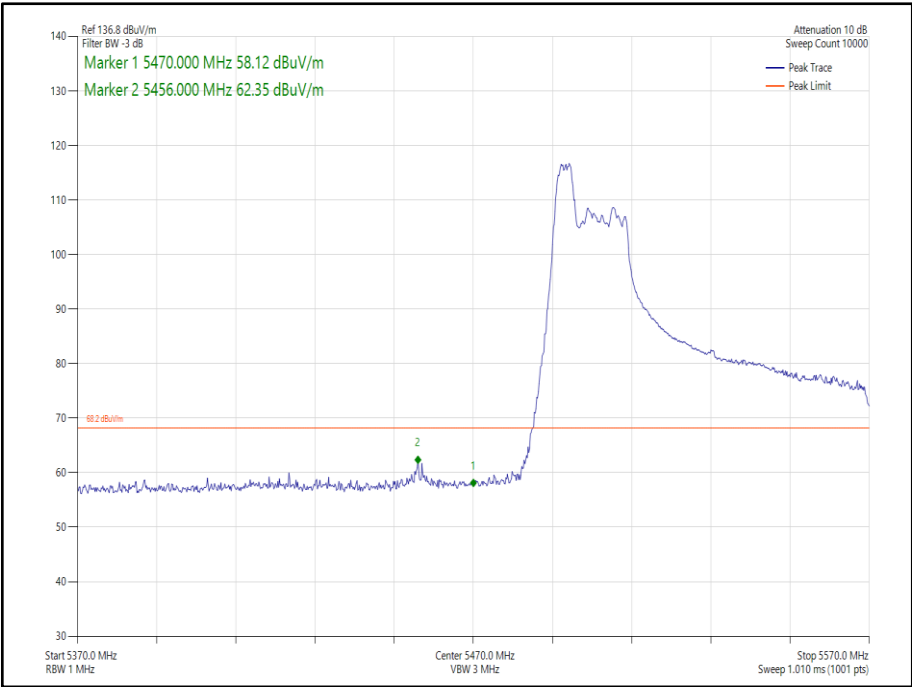
Figure 251 - 802.11ax HE80 Core 1 RU52-37- 5530 MHz Band Edge Frequency 5470 MHz
