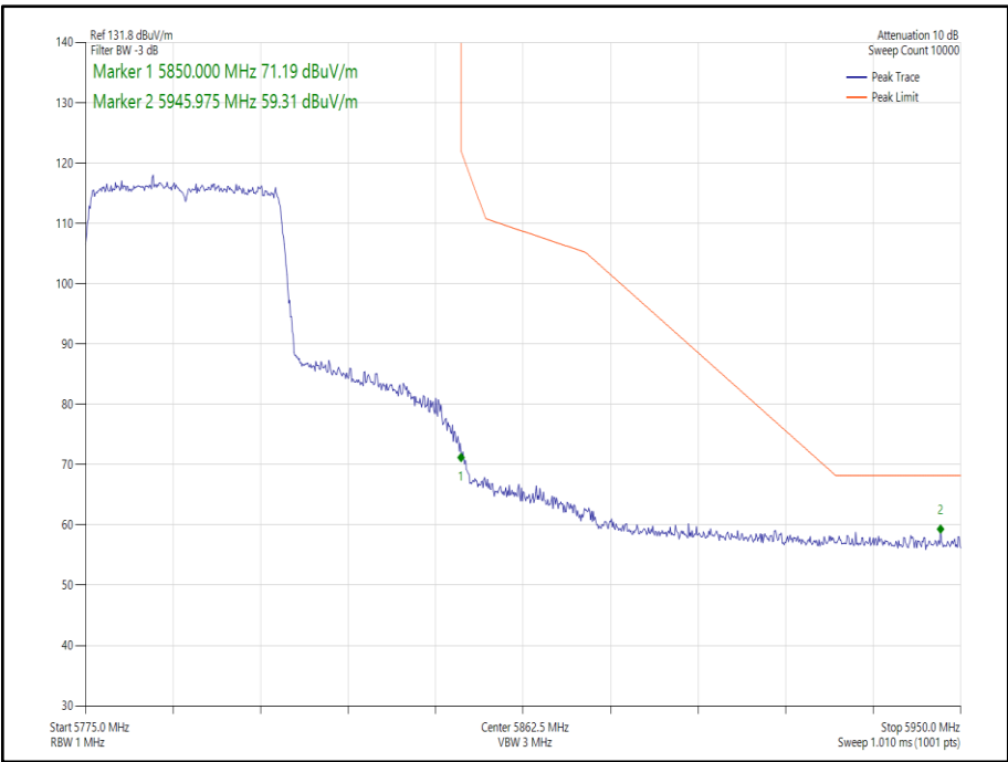
Figure 223 - 802.11ax HE40, Core 1, SU - 5795 MHz Band Edge Frequency 5850 MHz
