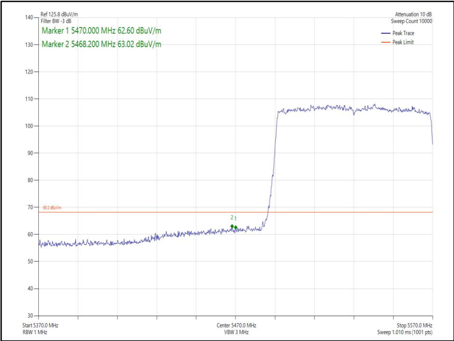
Figure 250 - 802.11ax HE80 Core 1 SU - 5530 MHz Band Edge Frequency 5470 MHz
