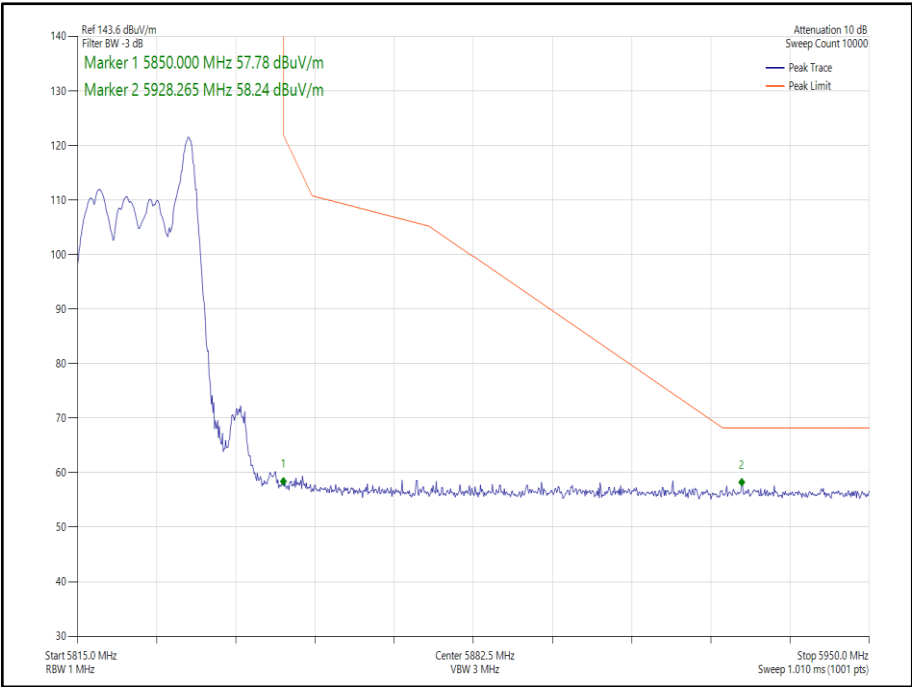
Figure 210 - 802.11ax HE20 CDD, Cores 0-1, RU26-8 - 5825 MHz Band Edge Frequency 5850 MHz
