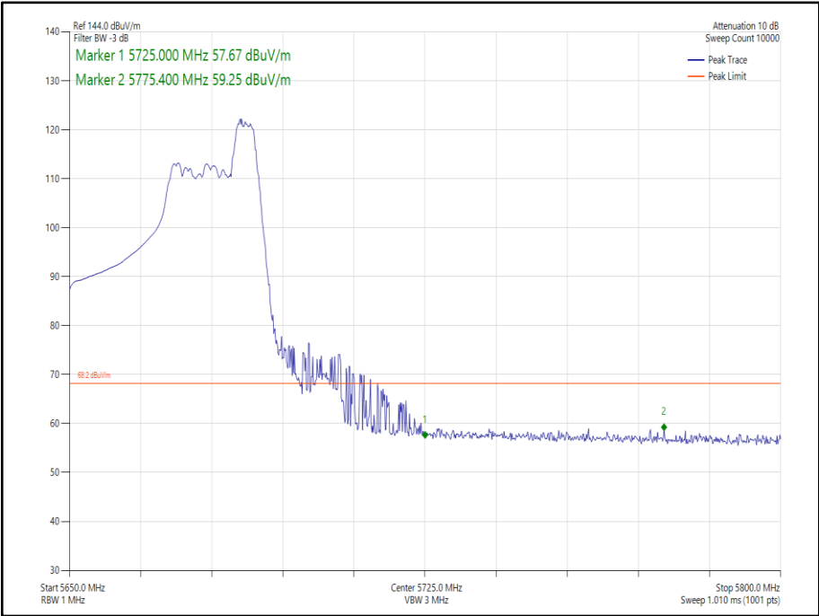
Figure 218 - 802.11ax HE40, Core 1, RU52-44 - 5670 MHz Band Edge Frequency 5725 MHz
