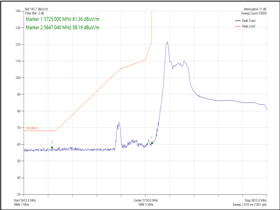
Figure 257 - 802.11ax HE80 Core 1 RU26-0 - 5775 MHz Band Edge Frequency 5725 MHz
