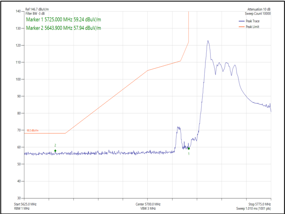
Figure 242 - 802.11ax HE40 SDM, Cores 0-1, RU26-0 - 5755 MHz Band Edge Frequency 5725 MHz
