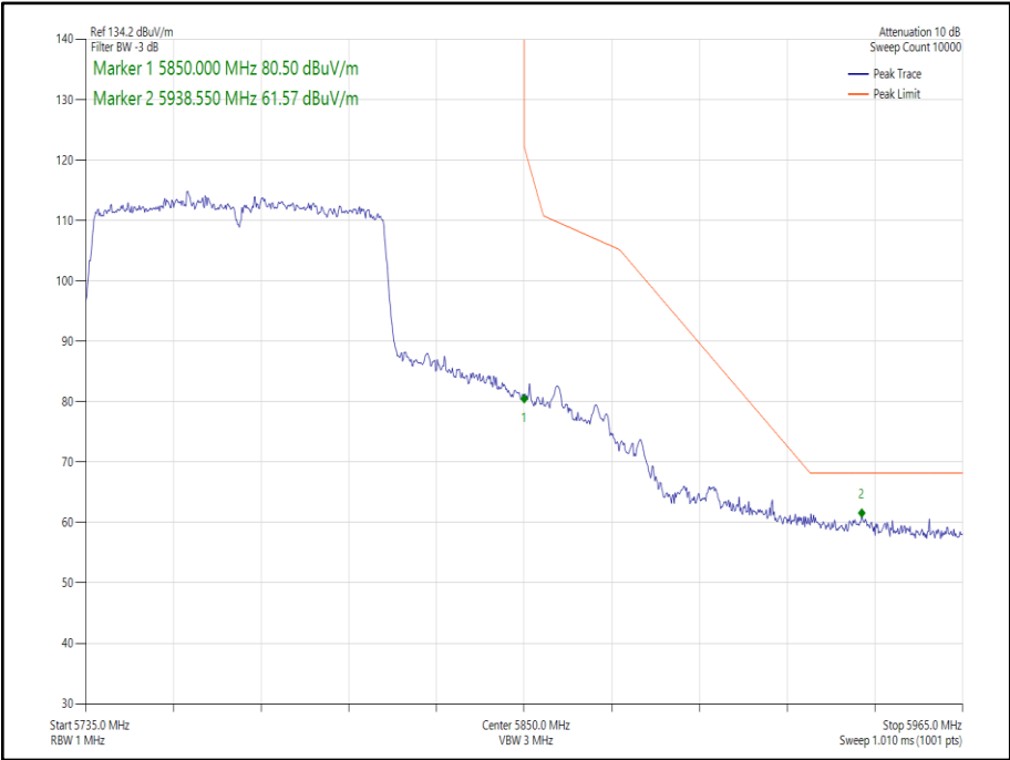
Figure 258 - 802.11ac VHT80 Core 1 - 5775 MHz Band Edge Frequency 5850 MHz
