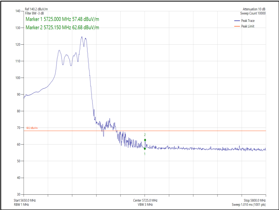
Figure 234 - 802.11ax HE40 CDD, Cores 0-1, RU52-44 - 5670 MHz Band Edge Frequency 5725 MHz
