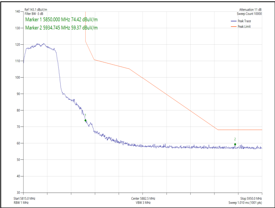
Figure 208 - 802.11n HT20 SDM, Cores 0-1 - 5825 MHz Band Edge Frequency 5850 MHz
