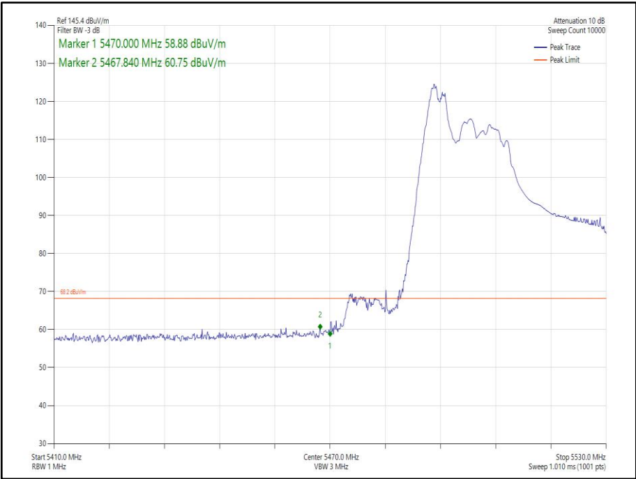
Figure 230 - 802. 11ax HE40 SDM, Cores 0-1, RU52-37 - 5510 MHz Band Edge Frequency 5470 MHz
