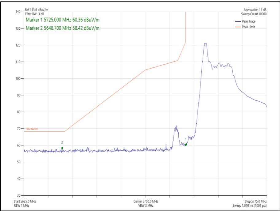
Figure 221 - 802.11ax HE40, Core 1, RU26-0 - 5755 MHz Band Edge Frequency 5725 MHz
