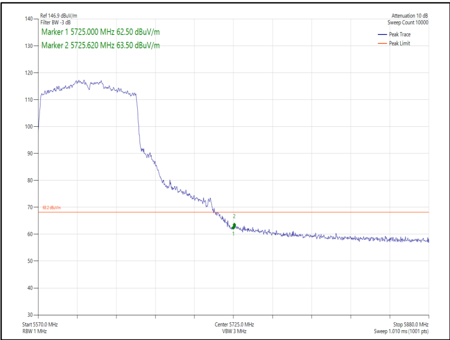
Figure 268 - 802.11ac VHT80 SDM, Cores 0-1 - 5610 MHz Band Edge Frequency 5725 MHz
