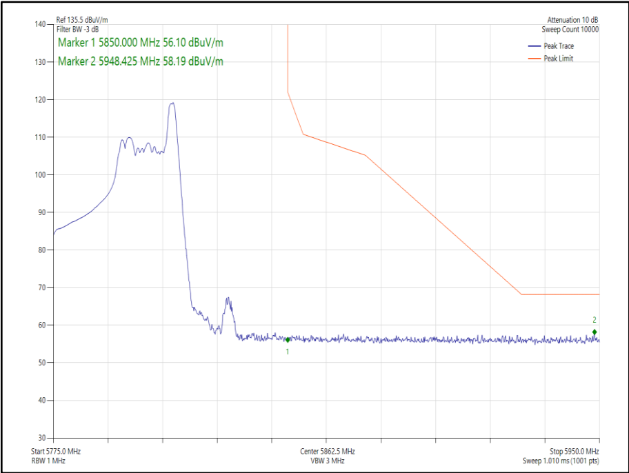
Figure 224 - 802.11ax HE40, Core 1, RU26-17 - 5795 MHz Band Edge Frequency 5850 MHz
