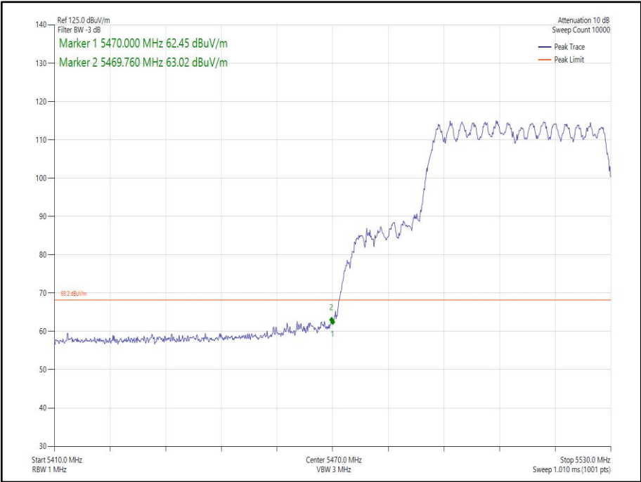
Figure 227 - 802.11ax HE40 CDD, Cores 0-1, SU - 5510 MHz Band Edge Frequency 5470 MHz
