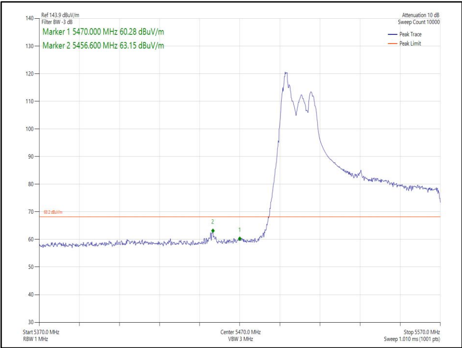
Figure 266 - 802.11ax HE80 SDM, Cores 0-1, RU52-37 - 5530 MHz Band Edge Frequency 5470 MHz
