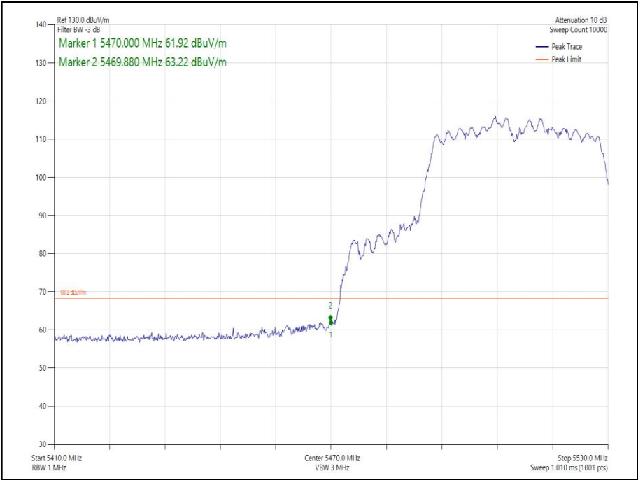
Figure 225 - 802.11n HT40 CDD, Cores 0-1 - 5510 MHz Band Edge Frequency 5470 MHz
