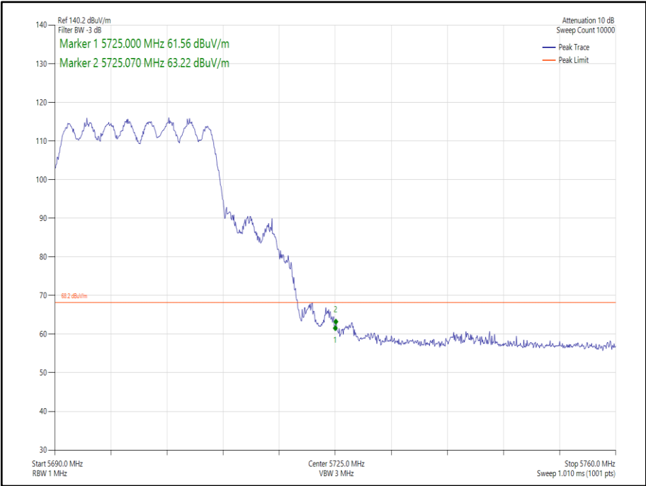
Figure 197 - 802.11ax HE20 CDD, Cores 0-1, SU - 5700 MHz Band Edge Frequency 5725 MHz
