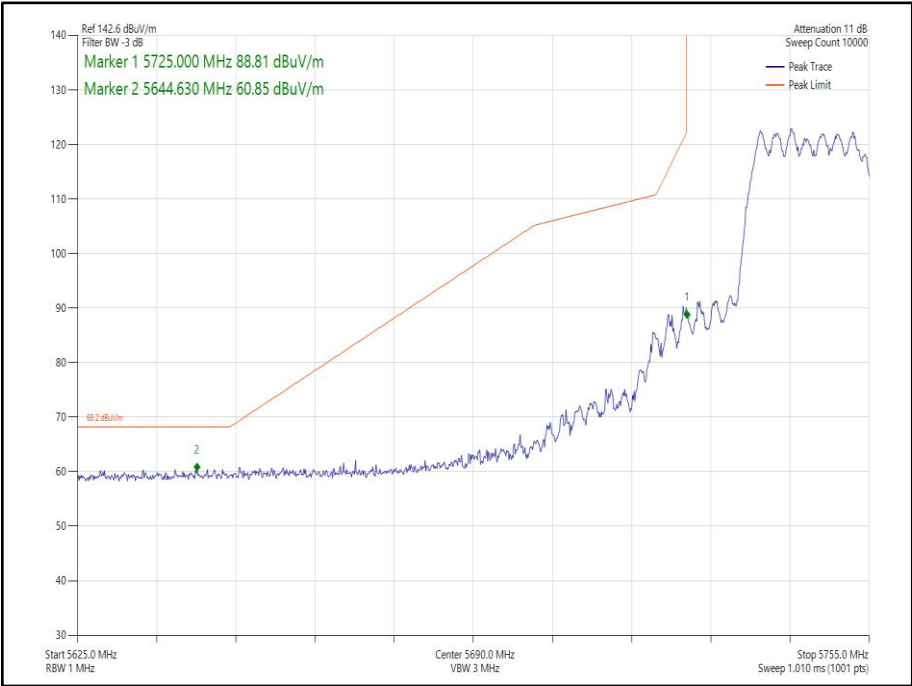
Figure 203 - 802.11ax HE20 CDD, Cores 0-1, SU - 5745 MHz Band Edge Frequency 5725 MHz
