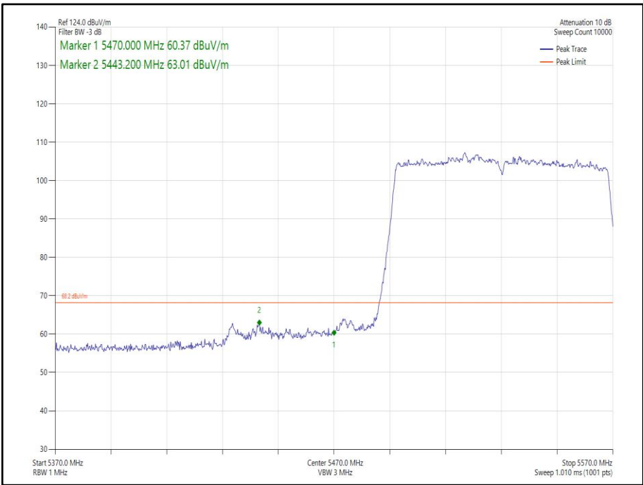
Figure 249 - 802.11ac VHT80 Core 1 - 5530 MHz Band Edge Frequency 5470 MHz
