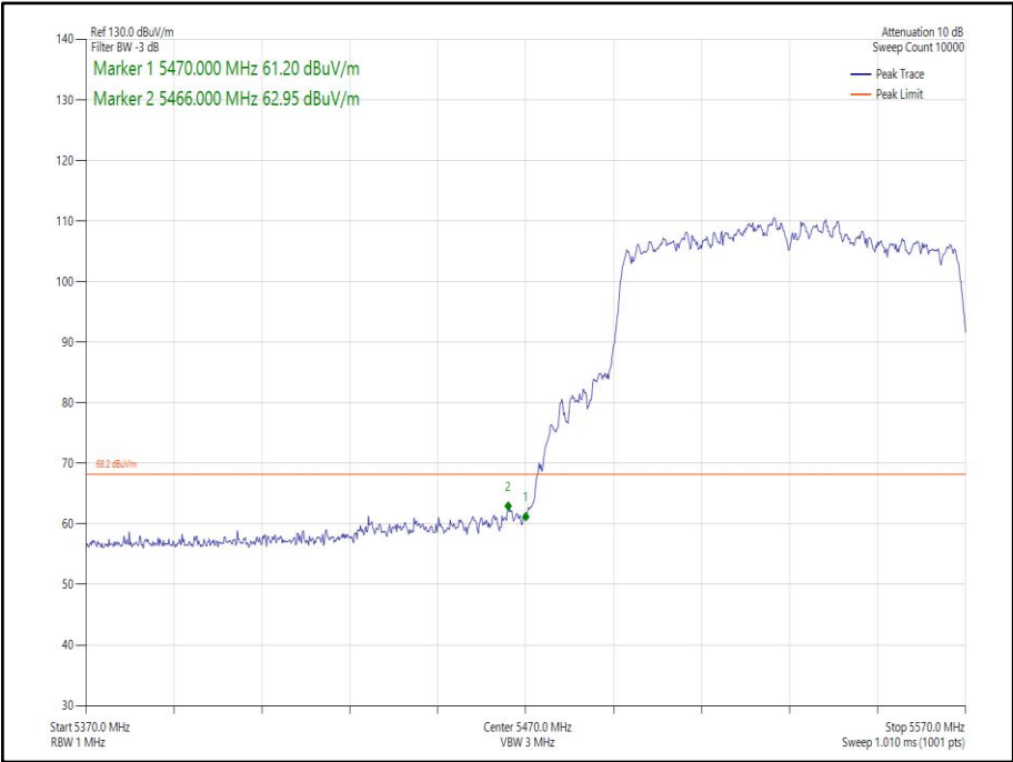
Figure 261 - 802.11ac VHT80 CDD, Cores 0-1 - 5530 MHz Band Edge Frequency 5470 MHz
