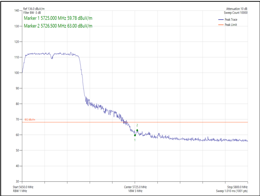
Figure 216 - 802.11n HT40, Core 1 - 5670 MHz Band Edge Frequency 5725 MHz
