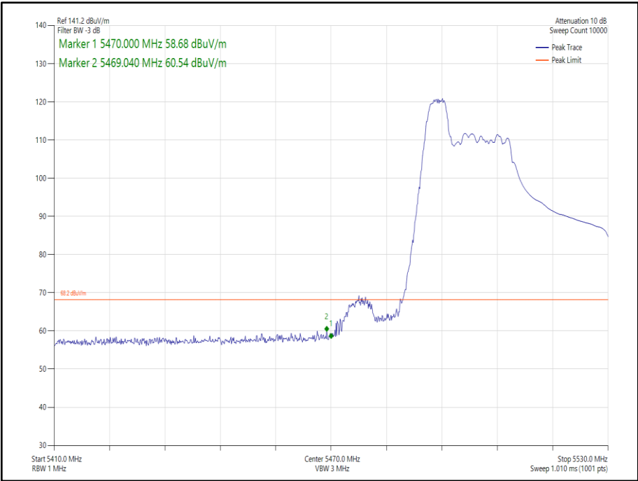
Figure 215 - 802.11ax HE40, Core 1, RU52-37 - 5510 MHz Band Edge Frequency 5470 MHz
