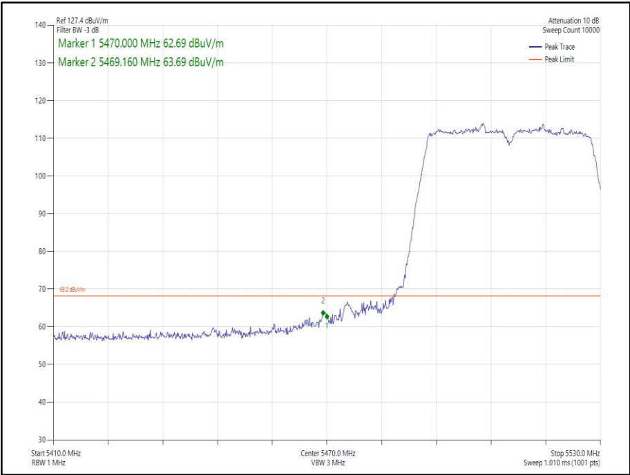
Figure 226 - 802.11n HT40 SDM, Cores 0-1 - 5510 MHz Band Edge Frequency 5470 MHz
