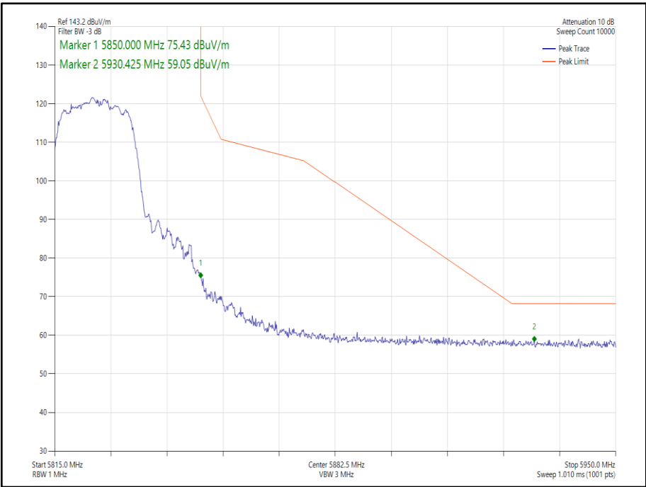
Figure 207 - 802.11n HT20 CDD, Cores 0-1 - 5825 MHz Band Edge Frequency 5850 MHz
