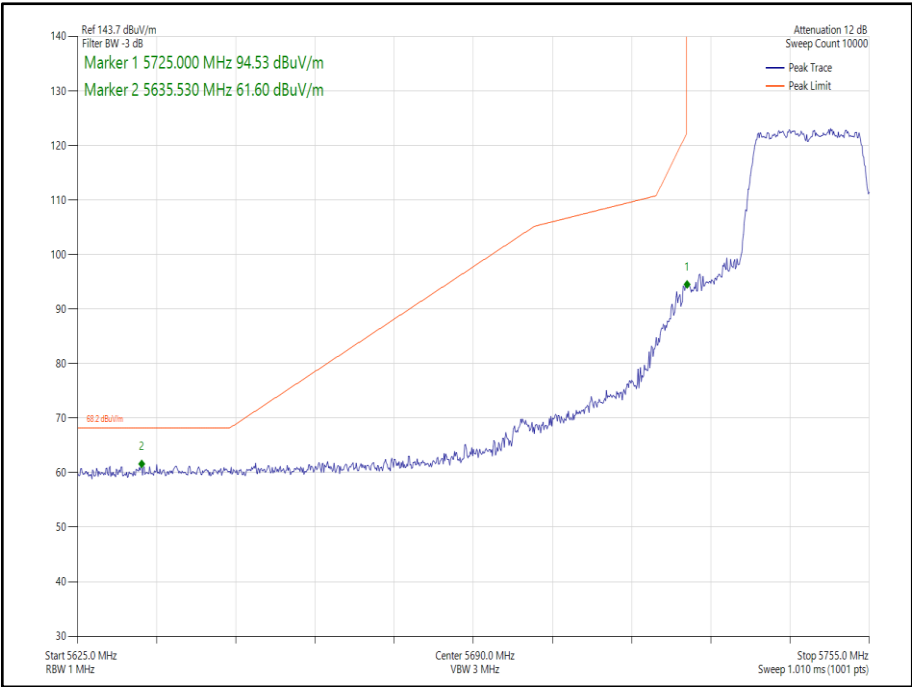
Figure 202 - 802.11n HT20 SDM, Cores 0-1 - 5745 MHz Band Edge Frequency 5725 MHz
