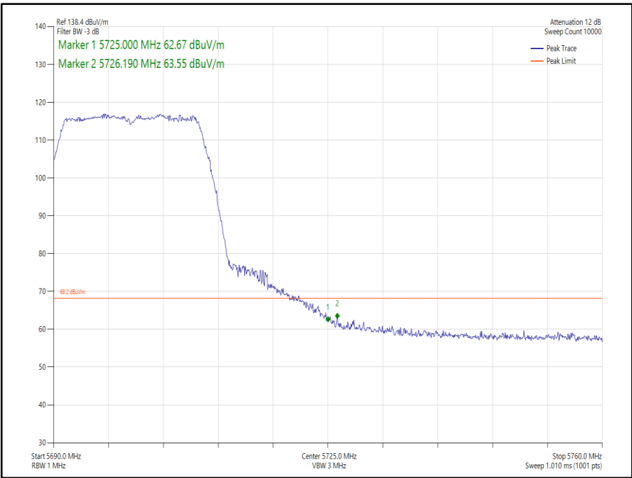
Figure 196 - 802.11n HT20 SDM, Cores 0-1 - 5700 MHz Band Edge Frequency 5725 MHz
