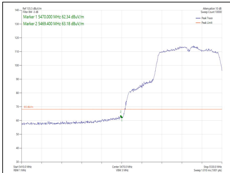
Figure 213 - 802.11n HT40, Core 1 - 5510 MHz Band Edge Frequency 5470 MHz
