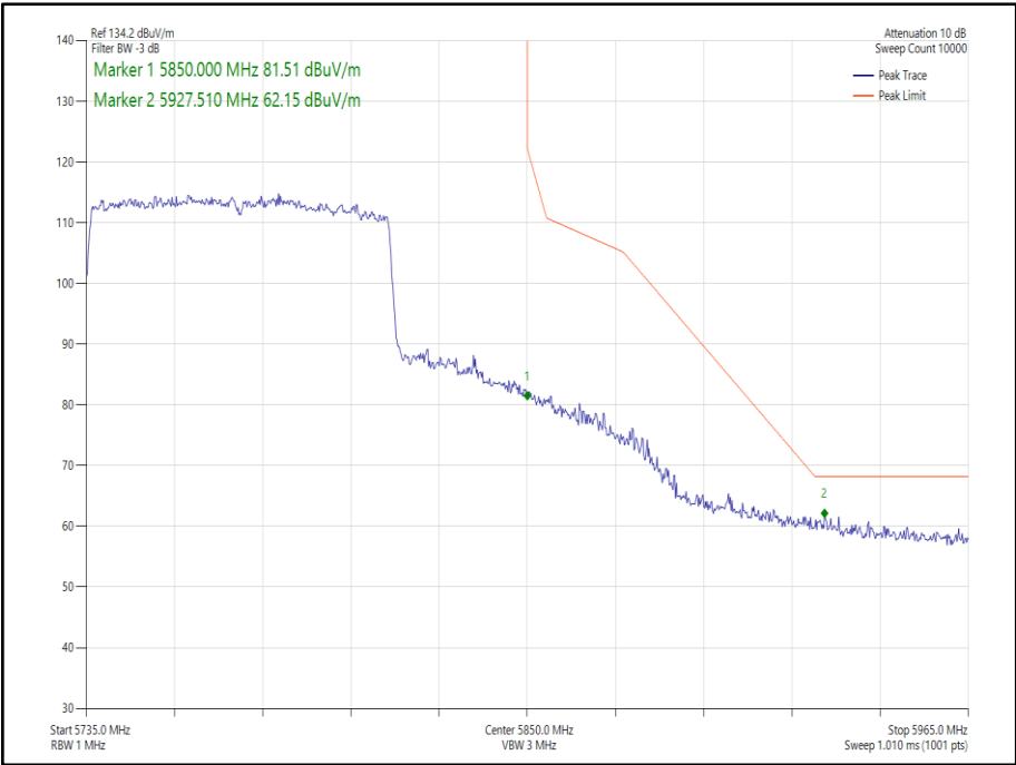
Figure 259 - 802.11ax HE80 Core 1 SU - 5775 MHz Band Edge Frequency 5850 MHz
