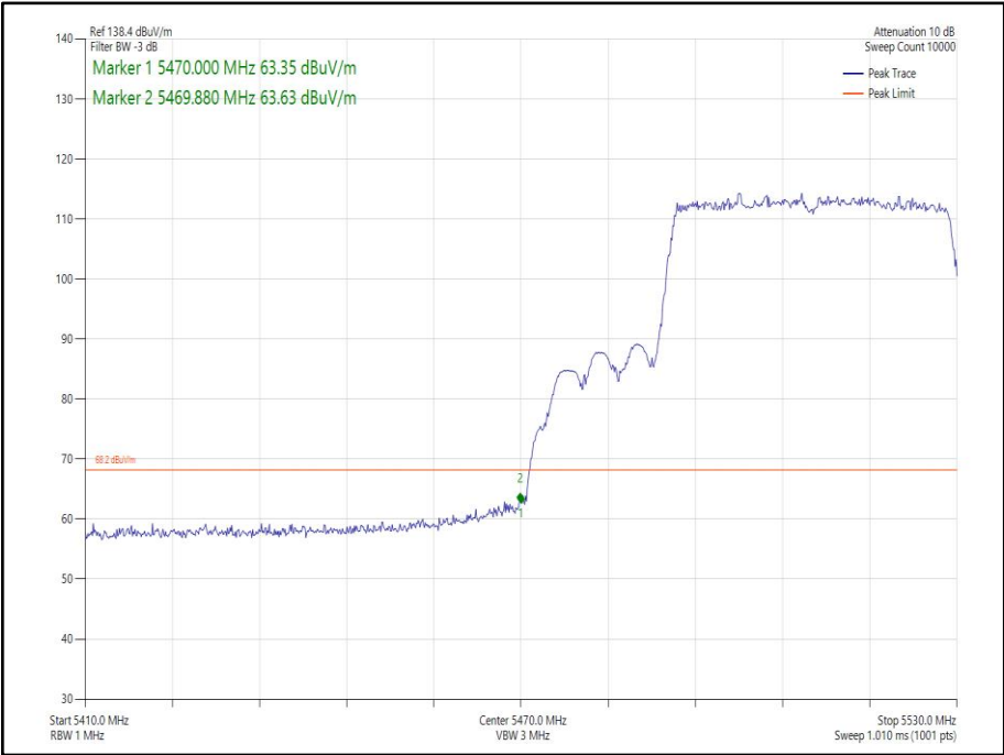
Figure 229 - 802.11ax HE40 SDM, Cores 0-1, SU - 5510 MHz Band Edge Frequency 5470 MHz
