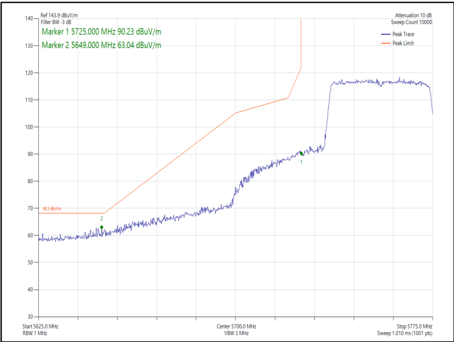
Figure 220 - 802.11ax HE40, Core 1, SU - 5755 MHz Band Edge Frequency 5725 MHz
