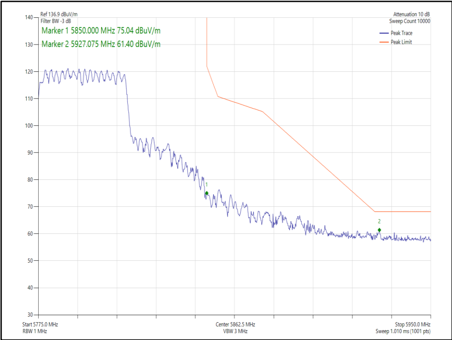
Figure 245 - 802.11ax HE40 CDD, Cores 0-1, SU - 5795 MHz Band Edge Frequency 5850 MHz
