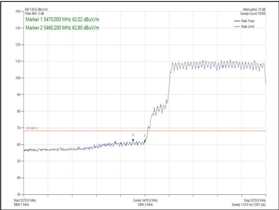
Figure 263 - 802.11ax HE80 CDD, Cores 0-1, SU - 5530 MHz Band Edge Frequency 5470 MHz
