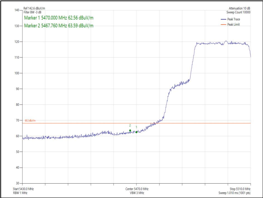
Figure 193 - 802.11ax HE20 SDM, Cores 0-1 SU - 5500 MHz Band Edge Frequency 5470 MHz
