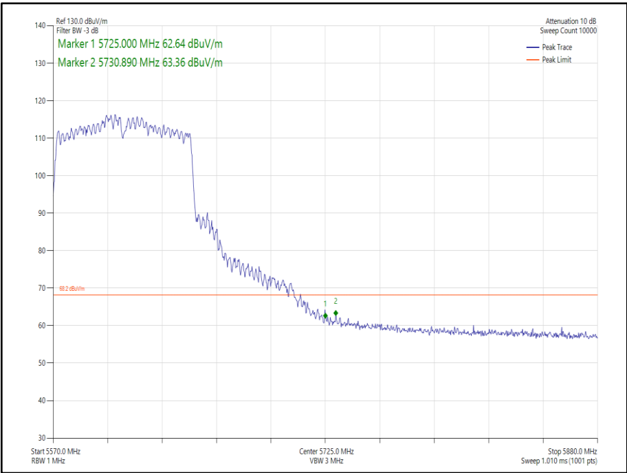
Figure 267 - 802.11ac VHT80 CDD, Cores 0-1 - 5610 MHz Band Edge Frequency 5725 MHz
