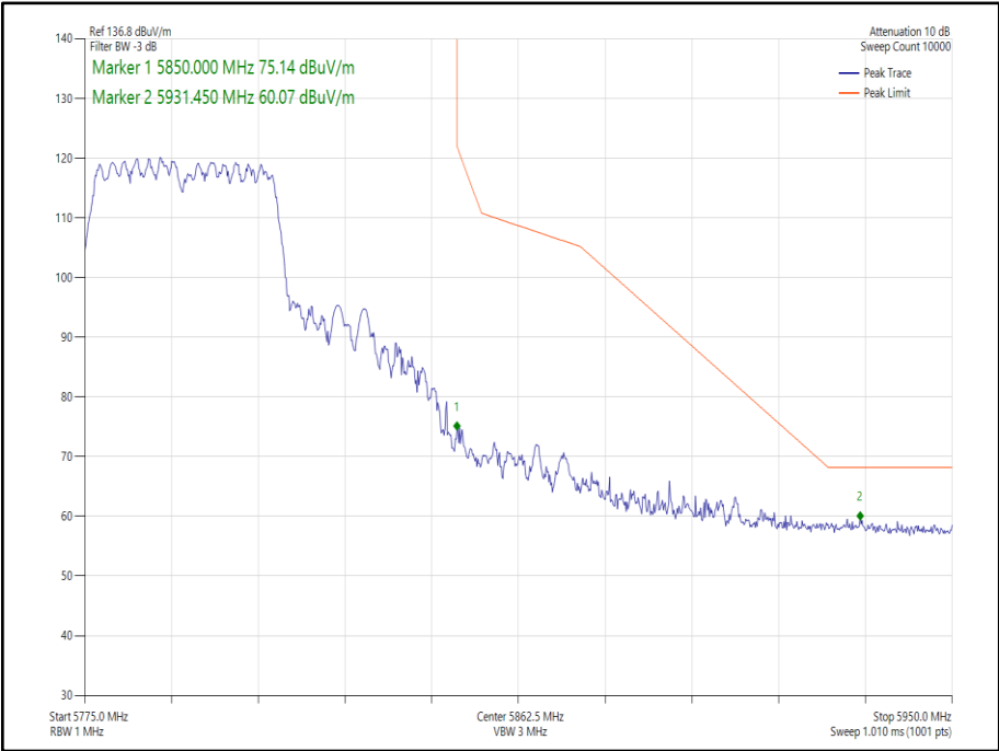
Figure 243 - 802.11n HT40 CDD, Cores 0-1 - 5795 MHz Band Edge Frequency 5850 MHz
