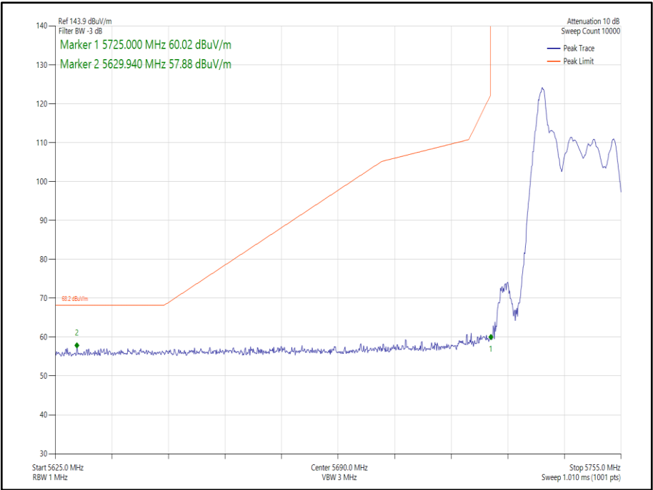
Figure 206 - 802.11ax HE20 SDM, Cores 0-1, RU26-0 - 5745 MHz Band Edge Frequency 5725 MHz
