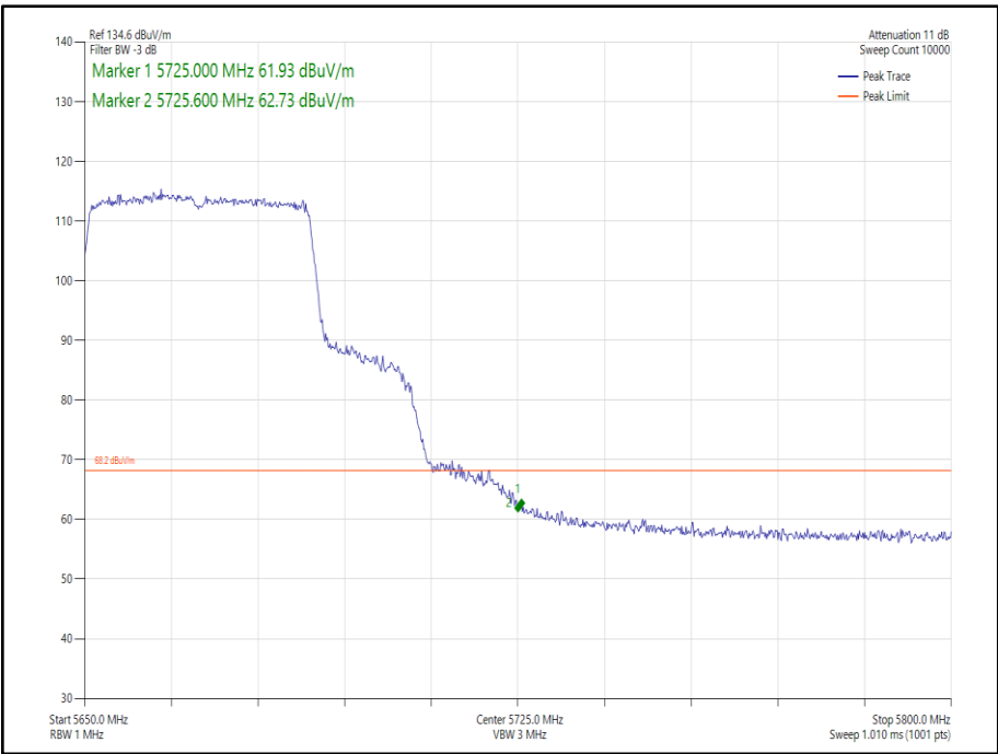
Figure 217 - 802.11ax HE40, Core 1, SU - 5670 MHz Band Edge Frequency 5725 MHz
