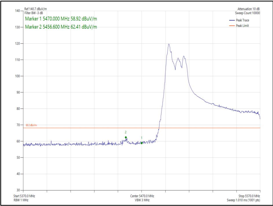
Figure 264 - 802.11ax HE80 CDD, Cores 0-1, RU52-37- 5530 MHz Band Edge Frequency 5470 MHz
