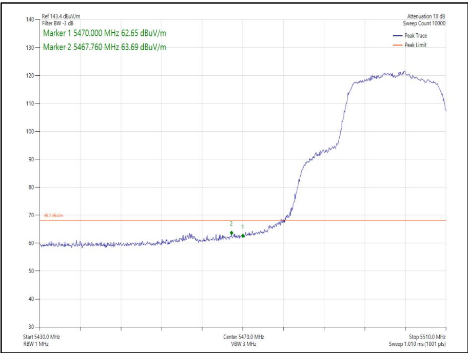
Figure 190 - 802.11n HT20 SDM, Cores 0-1 - 5500 MHz Band Edge Frequency 5470 MHz
