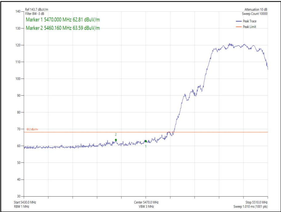
Figure 189 - 802.11n HT20 CDD, Cores 0-1 - 5500 MHz Band Edge Frequency 5470 MHz
