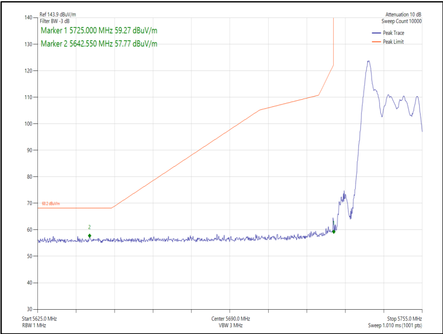
Figure 204 - 802.11ax HE20 CDD, Cores 0-1, RU26-0 - 5745 MHz Band Edge Frequency 5725 MHz
