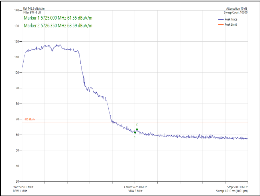
Figure 232 - 802.11n HT40 SDM, Cores 0-1 - 5670 MHz Band Edge Frequency 5725 MHz
