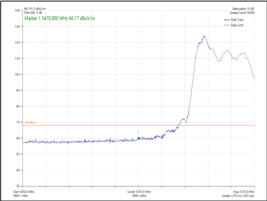
Figure 192 - 802.11ax HE20 CDD, Cores 0-1 RU52-37 - 5500 MHz Band Edge Frequency 5470 MHz
