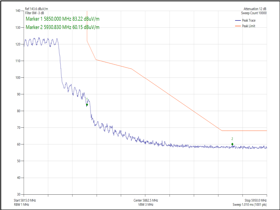
Figure 209 - 802.11ax HE20 CDD, Cores 0-1, SU - 5825 MHz Band Edge Frequency 5850 MHz
