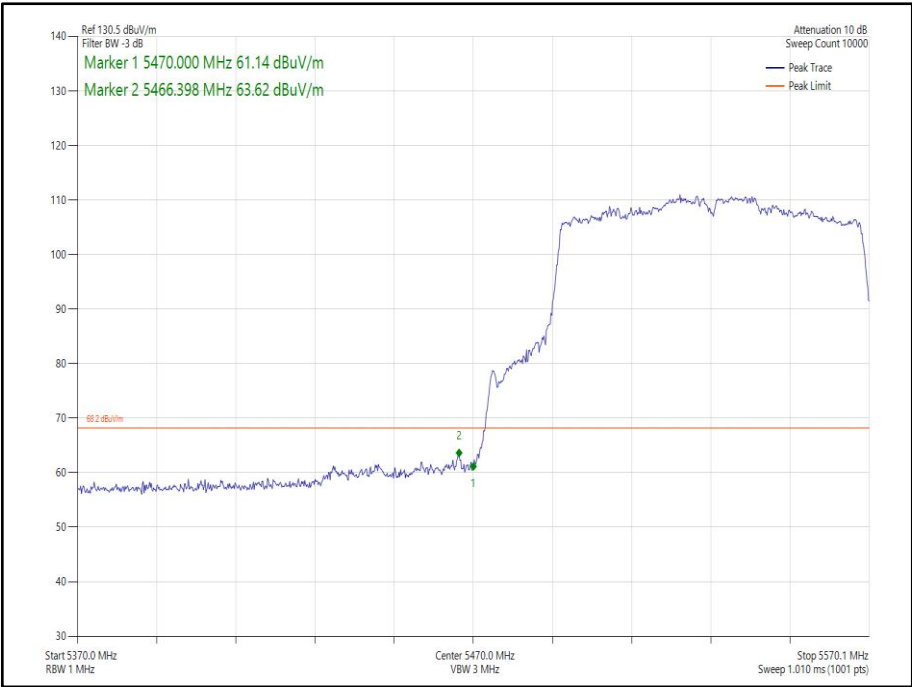
Figure 262 - 802.11ac VHT80 SDM, Cores 0-1 - 5530 MHz Band Edge Frequency 5470 MHz
