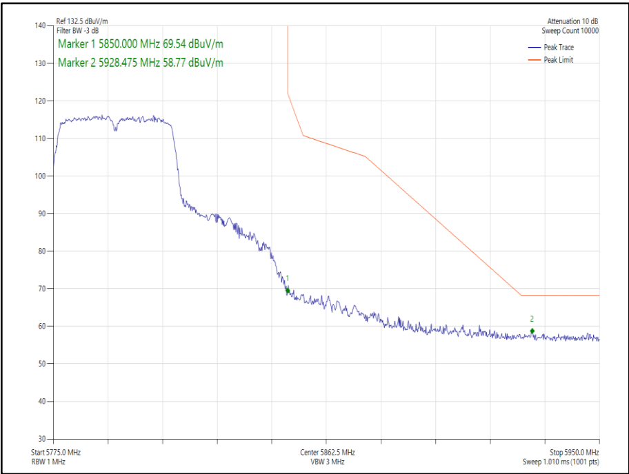
Figure 222 - 802.11n HT40, Core 1 - 5795 MHz Band Edge Frequency 5850 MHz
