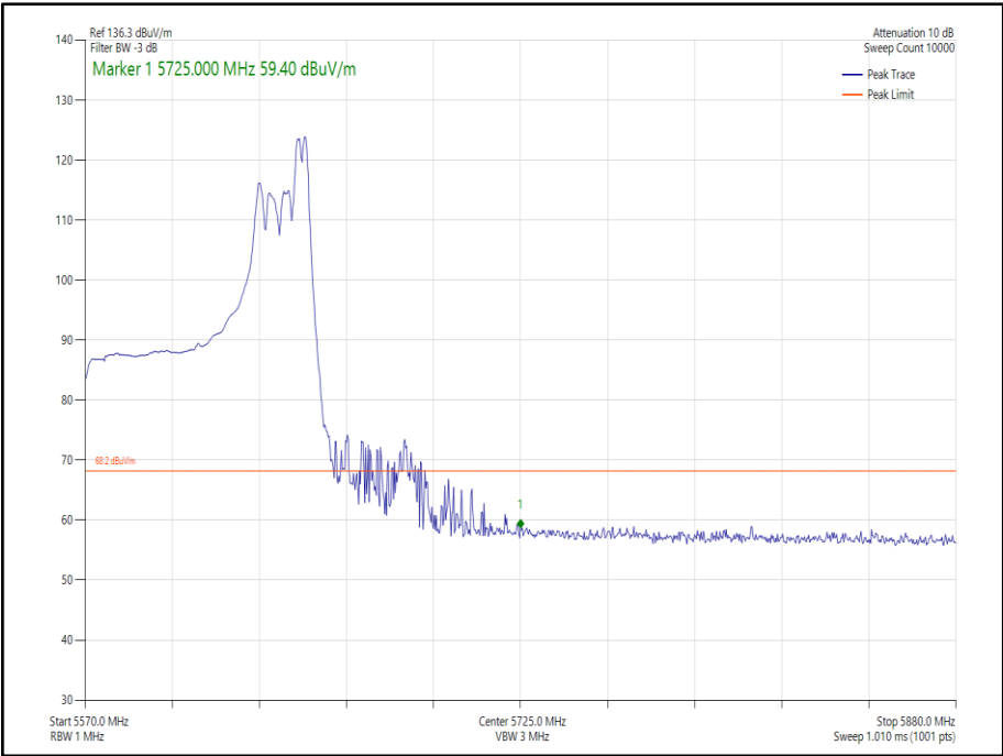
Figure 270 - 802.11ax HE80 CDD, Cores 0-1, RU52-52 - 5610 MHz Band Edge Frequency 5725 MHz
