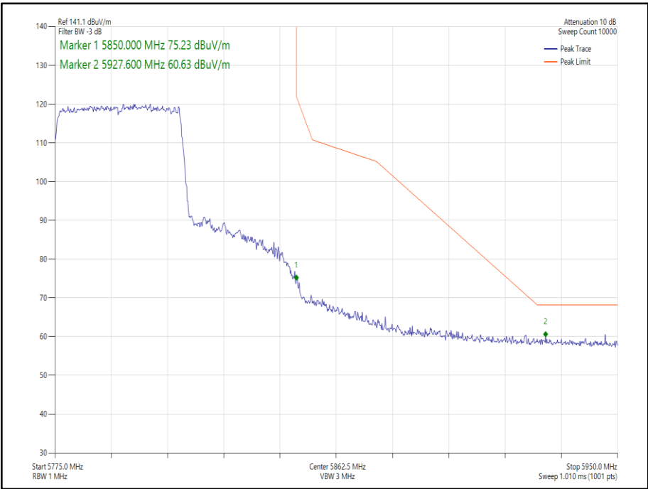
Figure 247 - 802.11ax HE40 SDM, Cores 0-1, SU - 5795 MHz Band Edge Frequency 5850 MHz
