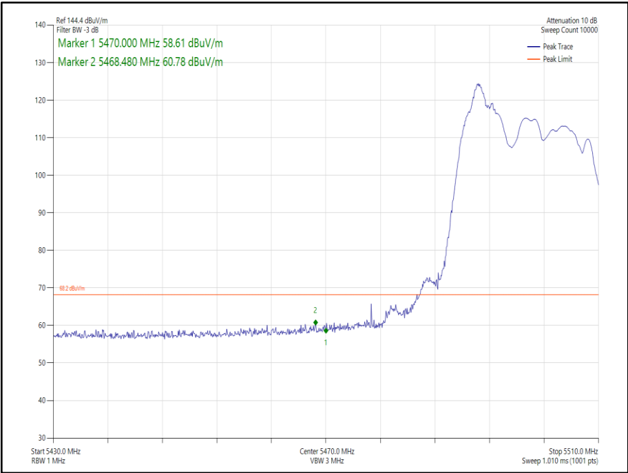
Figure 194 - 802.11ax HE20 SDM, Cores 0-1 RU52-37 - 5500 MHz Band Edge Frequency 5470 MHz
