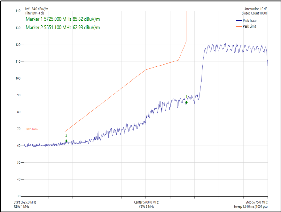
Figure 239 - 802.11ax HE40 CDD, Cores 0-1, SU - 5755 MHz Band Edge Frequency 5725 MHz
