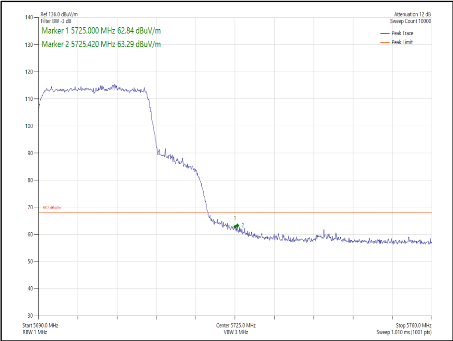
Figure 199 - 802.11ax HE20 SDM, Cores 0-1, SU - 5700 MHz Band Edge Frequency 5725 MHz
