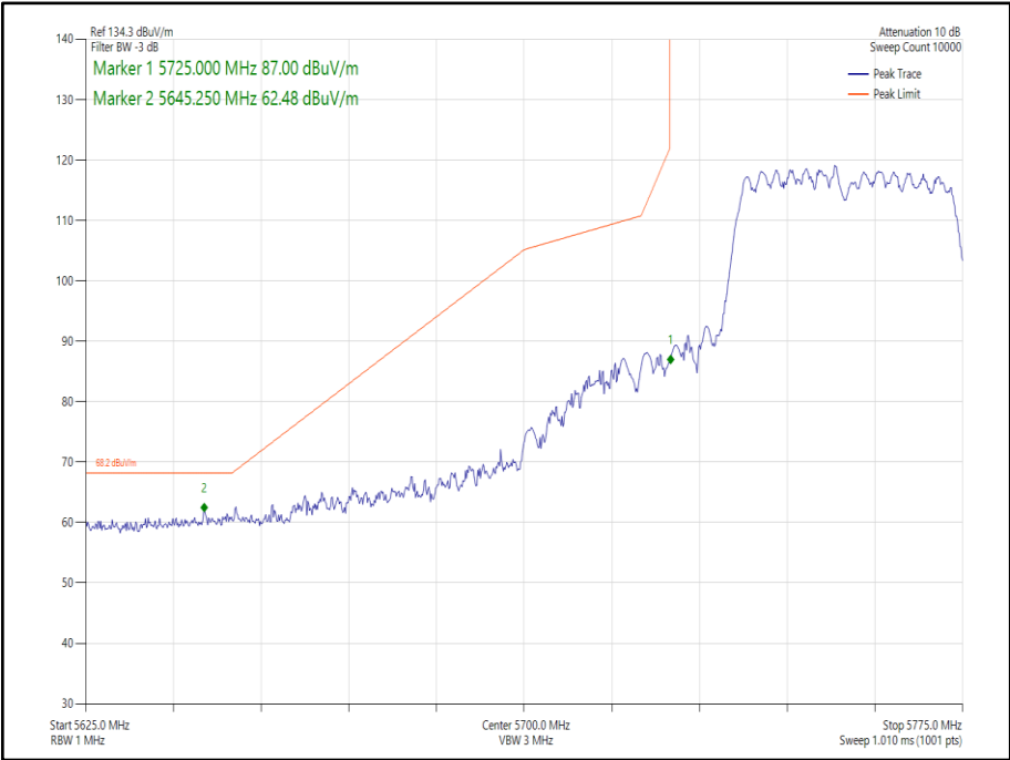
Figure 237 - 802.11n HT40 CDD, Cores 0-1 - 5755 MHz Band Edge Frequency 5725 MHz
