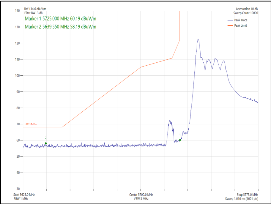
Figure 240 - 802.11ax HE40 CDD, Cores 0-1, RU26-0 - 5755 MHz Band Edge Frequency 5725 MHz
