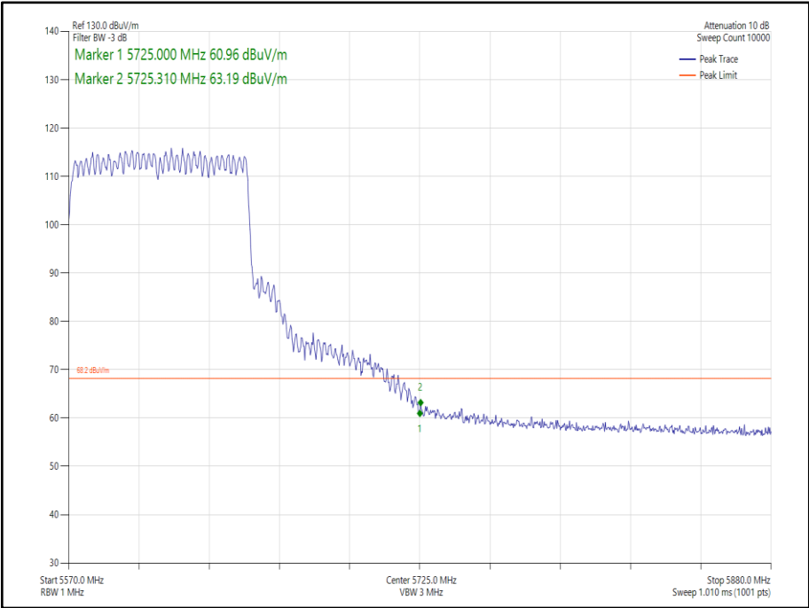
Figure 269 - 802.11ax HE80 CDD, Cores 0-1, SU - 5610 MHz Band Edge Frequency 5725 MHz
