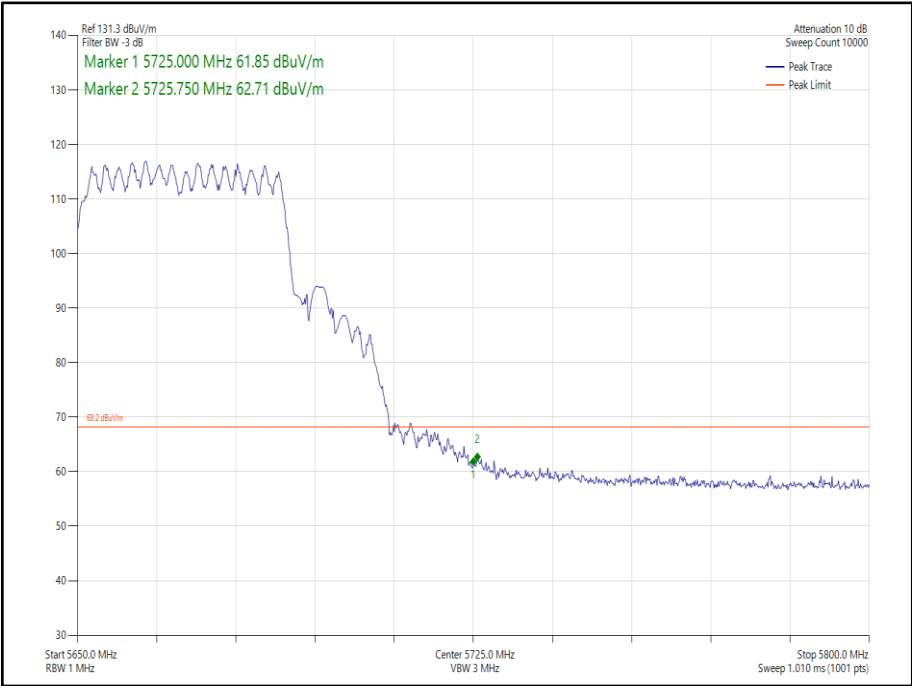
Figure 233 - 802.11ax HE40 CDD, Cores 0-1, SU - 5670 MHz Band Edge Frequency 5725 MHz
