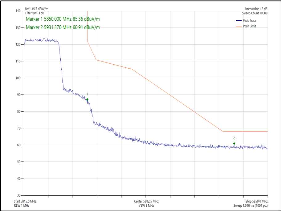
Figure 211 - 802.11ax HE20 SDM, Cores 0-1, SU - 5825 MHz Band Edge Frequency 5850 MHz
