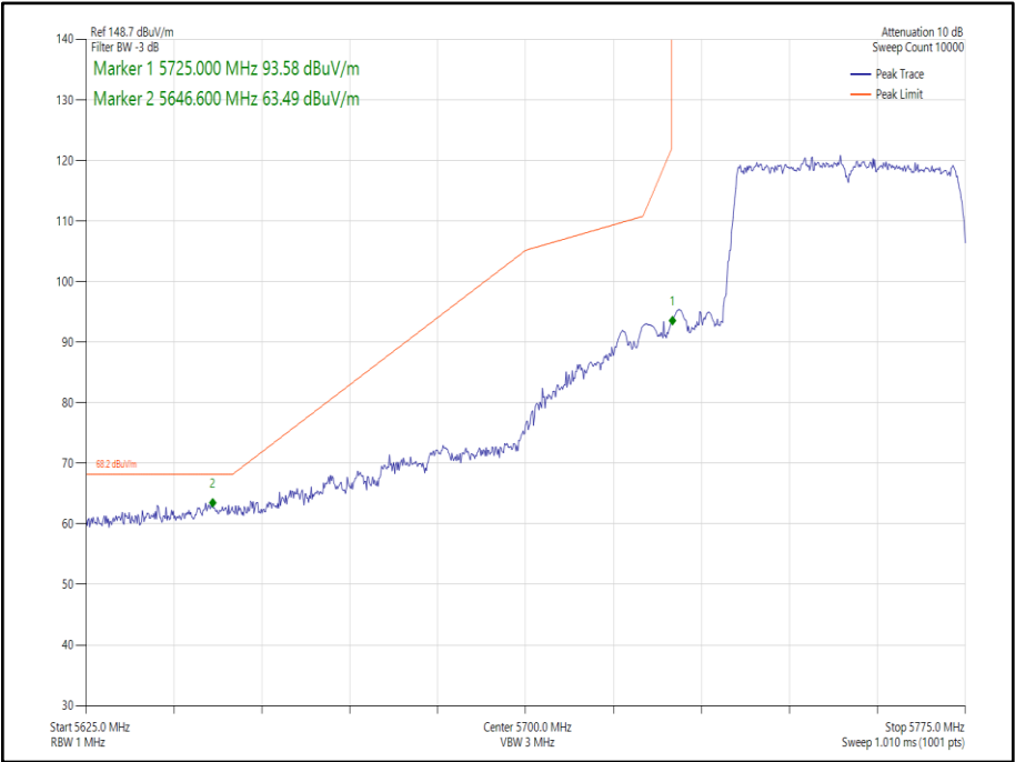
Figure 241 - 802.11ax HE40 SDM, Cores 0-1, SU - 5755 MHz Band Edge Frequency 5725 MHz
