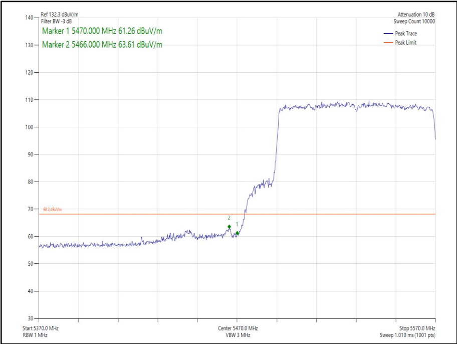
Figure 265 - 802.11ax HE80 SDM, Cores 0-1, SU - 5530 MHz Band Edge Frequency 5470 MHz
