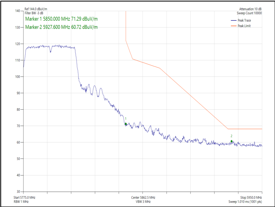
Figure 244 - 802.11n HT40 SDM, Cores 0-1 - 5795 MHz Band Edge Frequency 5850 MHz
