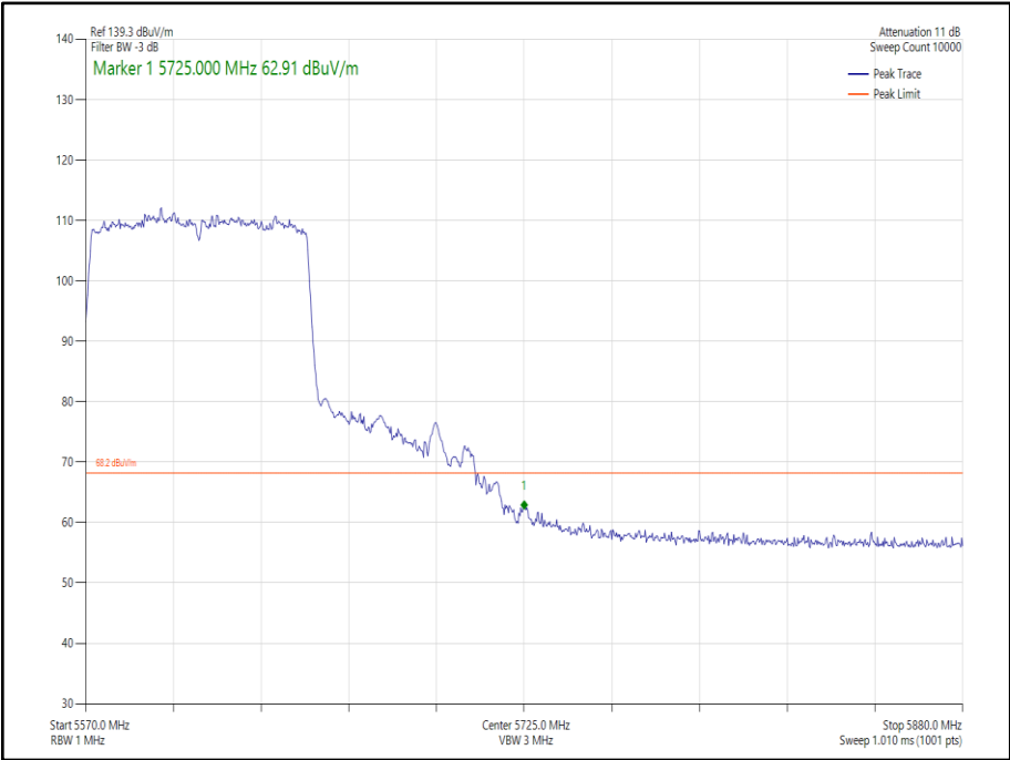
Figure 252 - 802.11ac VHT80 Core 1 - 5610 MHz Band Edge Frequency 5725 MHz
