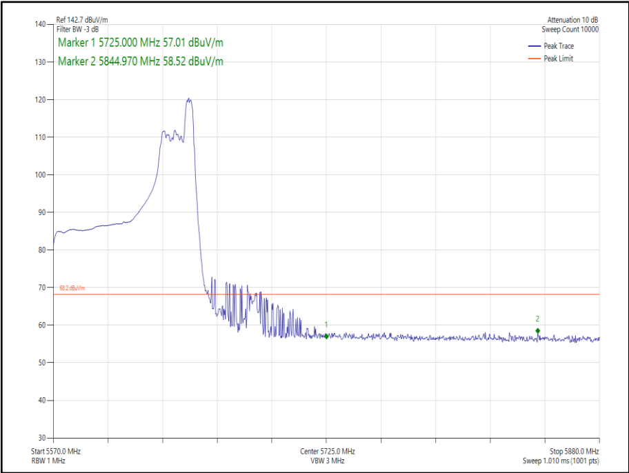
Figure 254 - 802.11ax HE80 Core 1 RU52-52 - 5610 MHz Band Edge Frequency 5725 MHz
