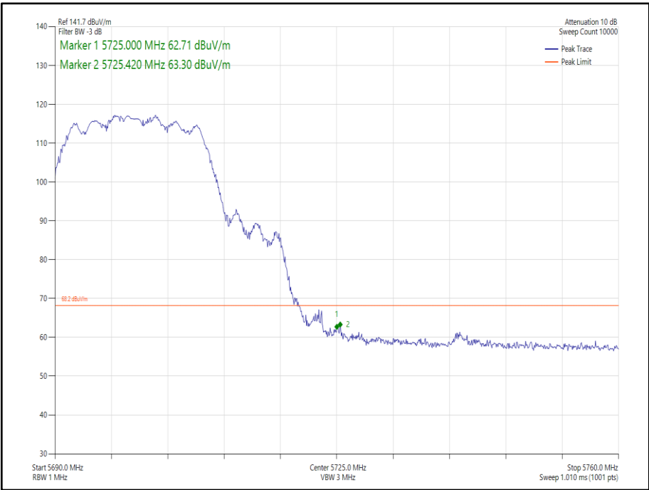
Figure 195 - 802.11n HT20 CDD, Cores 0-1 - 5700 MHz Band Edge Frequency 5725 MHz
