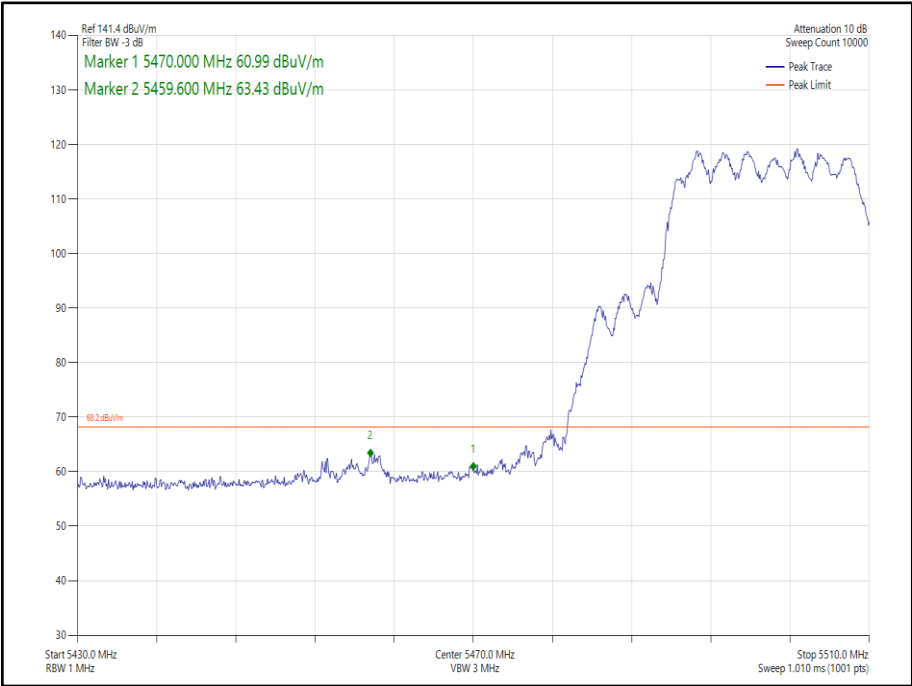
Figure 191 - 802.11ax HE20 CDD, Cores 0-1, SU - 5500 MHz Band Edge Frequency 5470 MHz
