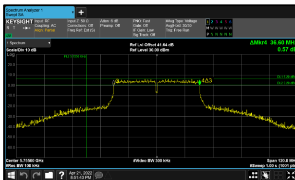
Figure 163 - 802.11n HT40 Minimum 6 dB EBW
