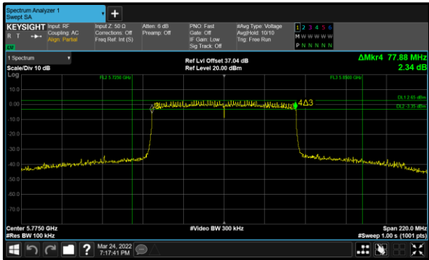
Figure 97 - 802.11ax HE80 SU Minimum 6 dB EBW
