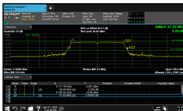
Figure 169 - 802.11n HT40 Minimum 99% OBW
