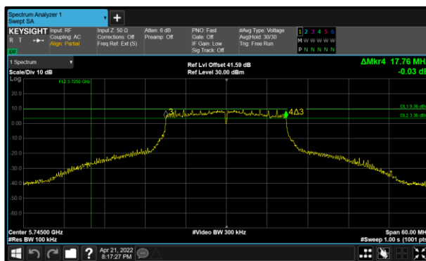
Figure 161 - 802.11n HT20 Minimum 6 dB EBW
