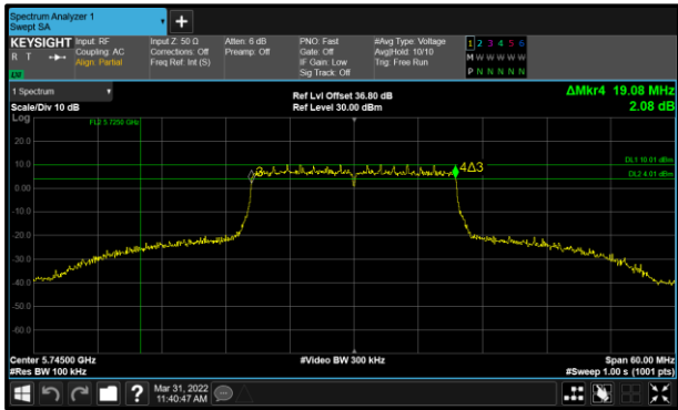
Figure 119 - 802.11ax HE20 SU Minimum 6 dB EBW
