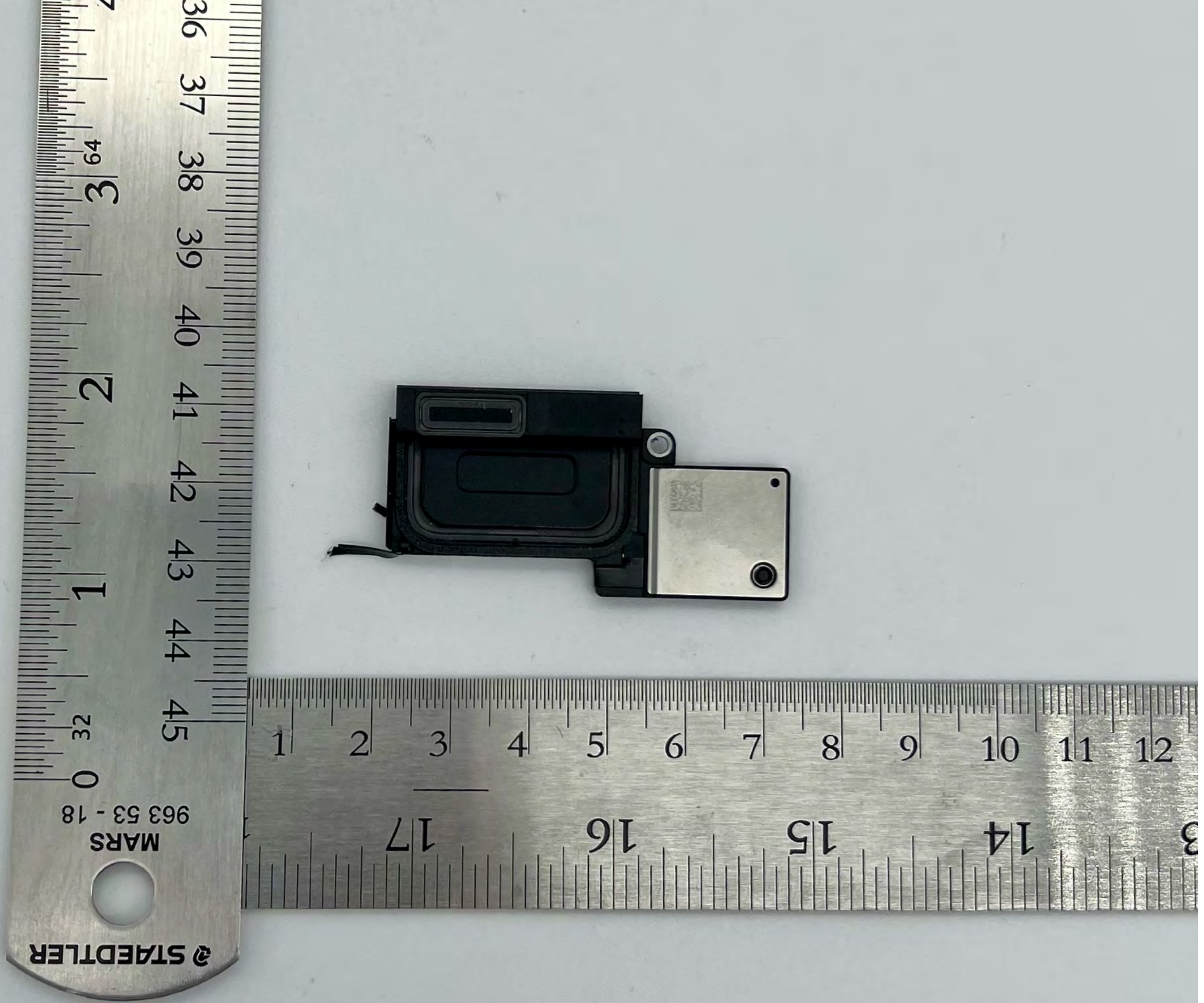
A2681 Right speaker structure- Back
