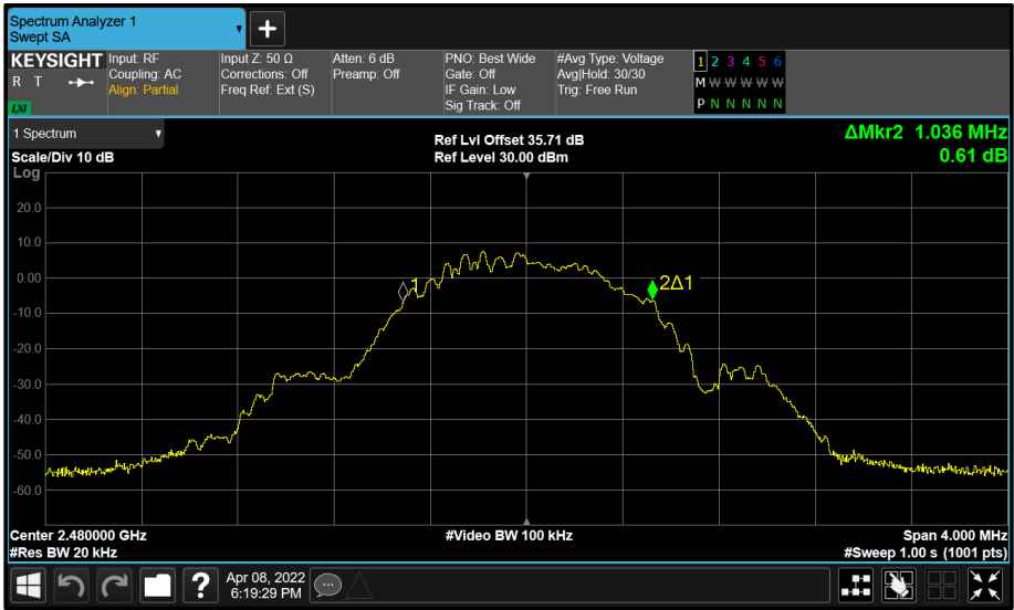
Figure 85 - Core 1 (B) 2480 MHz (CH39) 99% Bandwidth
