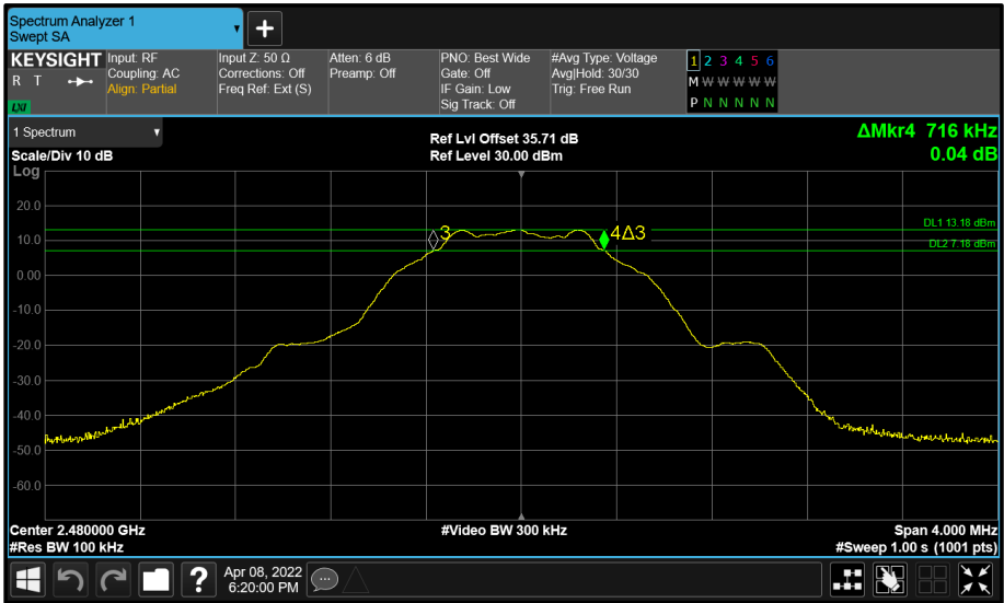
Figure 86 - Core 1 (B) 2480 MHz (CH39) 6 dB Bandwidth
