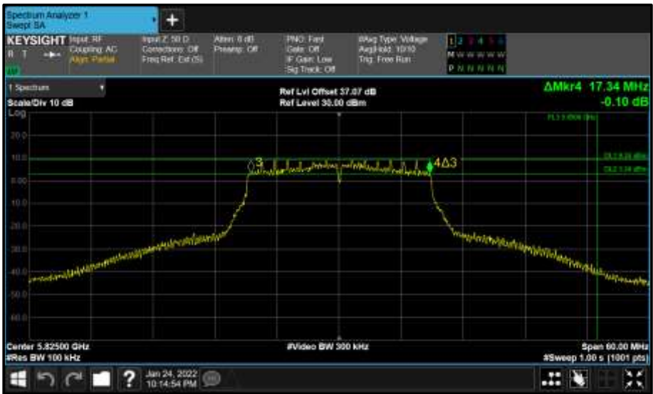
Figure 593 - Core 0 (A) 5825 MHz (CH165) 6 dB Bandwidth
