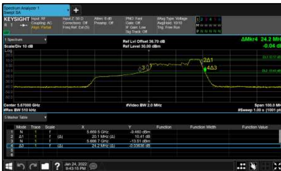
Figure 514 - Core 0 (A) 5670 MHz (CH134) 26 dB and 99% Bandwidth
