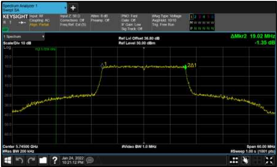
Figure 674 - Core 0 (A) 5745 MHz (CH149) 99% Bandwidth
