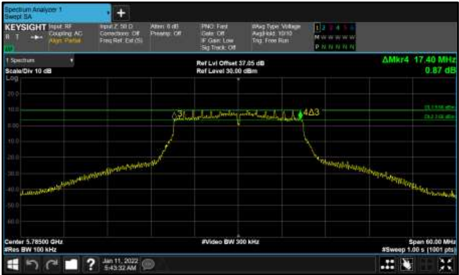
Figure 573 - Core 0 (A) 5785 MHz (CH157) 6 dB Bandwidth
