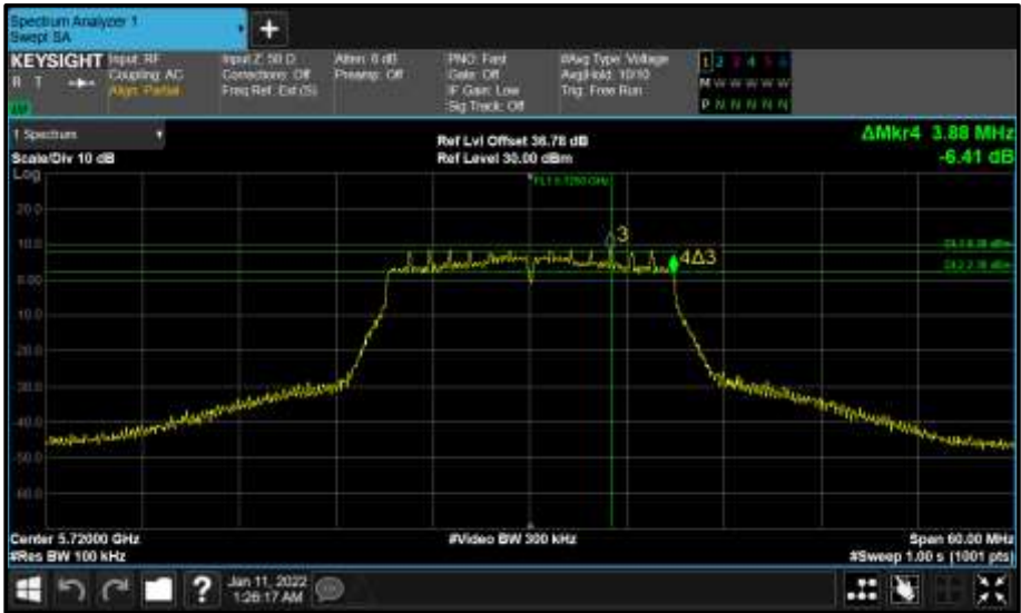
Figure 557 - Core 0 (A) 5720 MHz (CH144) 6 dB Bandwidth
