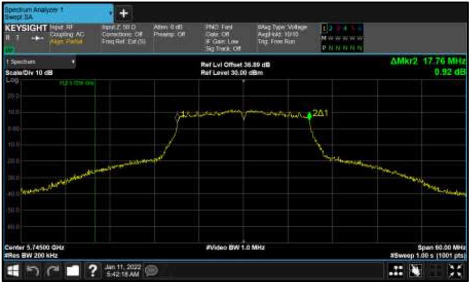
Figure 570 - Core 1 (B) 5745 MHz (CH149) 99% Bandwidth
