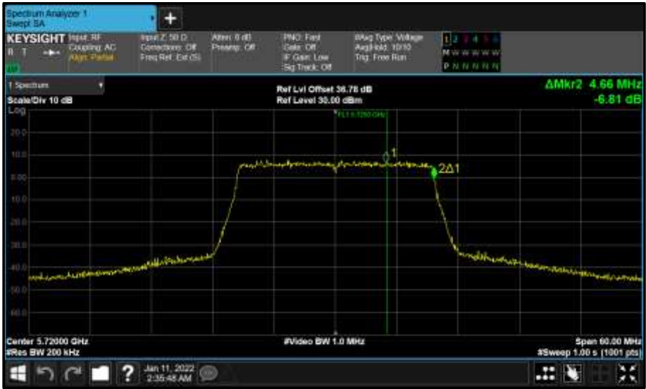
Figure 654 - Core 0 (A) 5720 MHz (CH144) 99% Bandwidth
