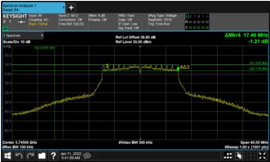
Figure 569 - Core 0 (A) 5745 MHz (CH149) 6 dB Bandwidth
