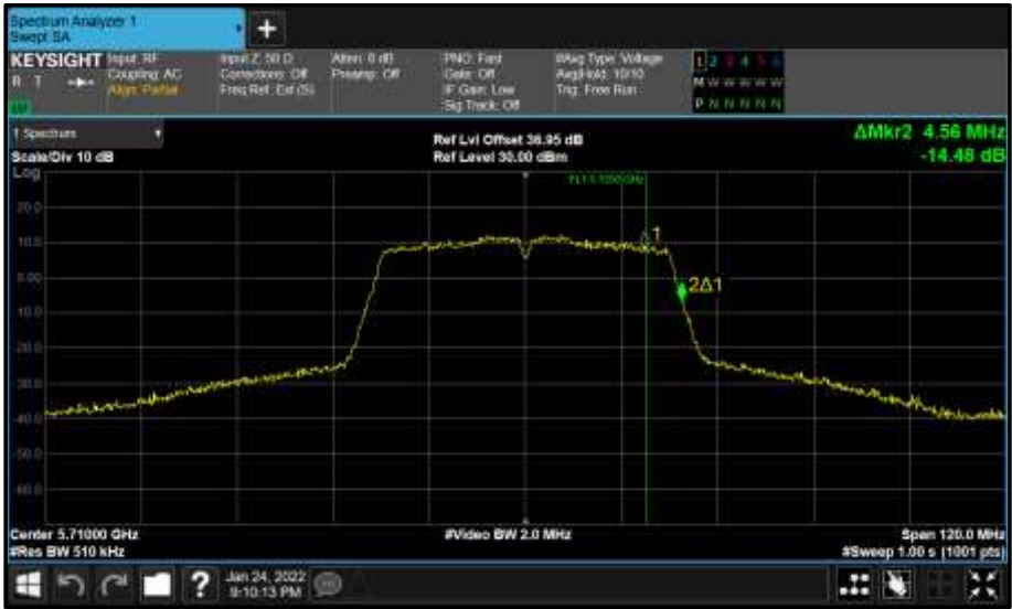
Figure 616 - Core 1 (B) 5710 MHz (CH142) 99% Bandwidth
