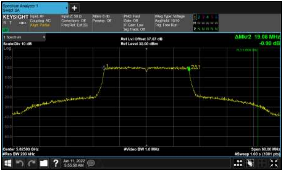
Figure 666 - Core 0 (A) 5825 MHz (CH165) 99% Bandwidth
