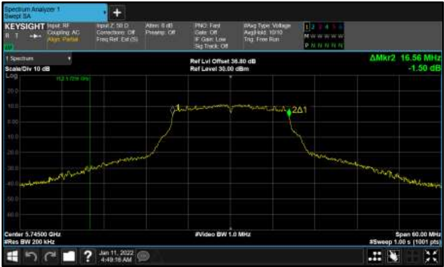
Figure 550 - Core 0 (A) 5745 MHz (CH149) 99% Bandwidth
