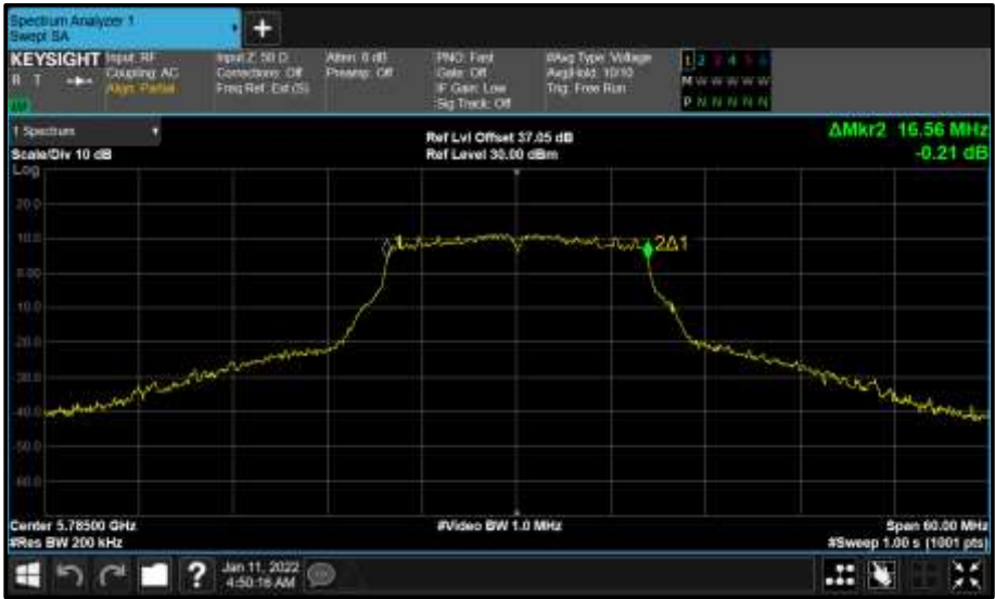
Figure 552 - Core 0 (A) 5785 MHz (CH157) 99% Bandwidth
