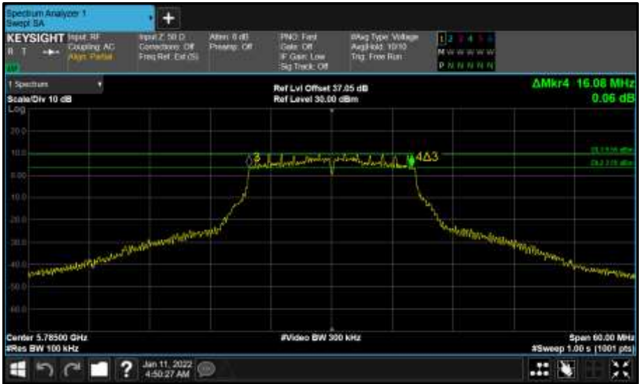
Figure 553 - Core 0 (A) 5785 MHz (CH157) 6 dB Bandwidth
