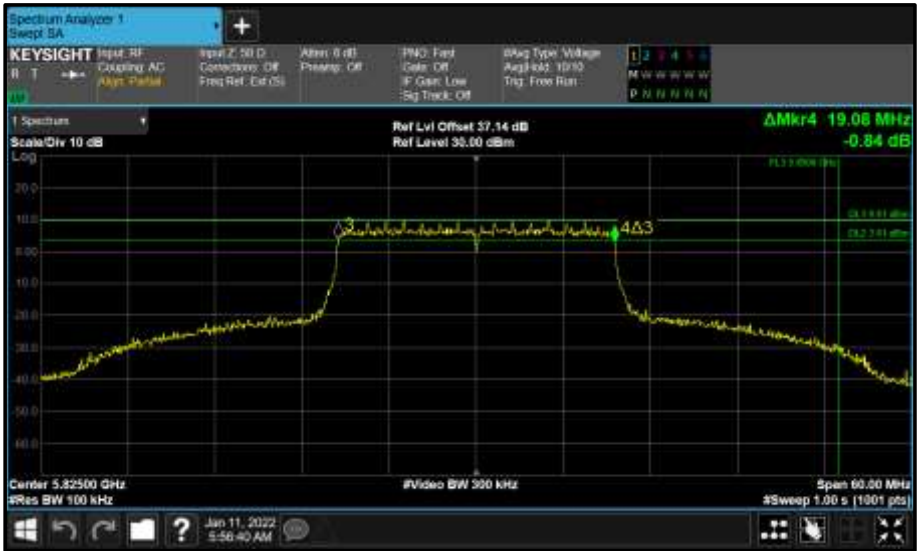
Figure 669 - Core 1 (B) 5825 MHz (CH165) 6 dB Bandwidth
