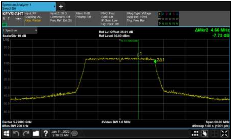
Figure 656 - Core 1 (B) 5720 MHz (CH144) 99% Bandwidth
