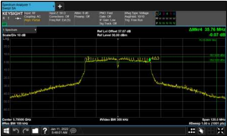
Figure 611 - Core 0 (A) 5795 MHz (CH159) 6 dB Bandwidth
