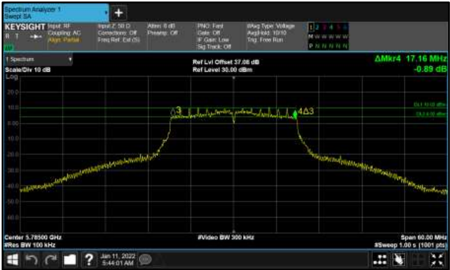
Figure 575 - Core 1 (B) 5785 MHz (CH157) 6 dB Bandwidth
