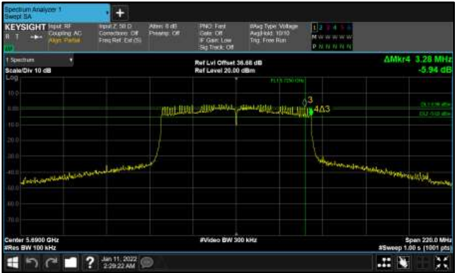
Figure 631 - Core 0 (A) 5690 MHz (CH138) 6 dB Bandwidth
