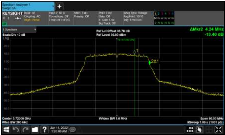
Figure 556 - Core 0 (A) 5720 MHz (CH144) 99% Bandwidth
