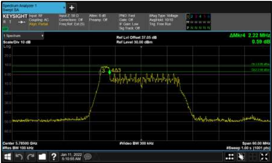
Figure 689 - Core 0 (A) 5785 MHz (CH157) 6 dB Bandwidth
