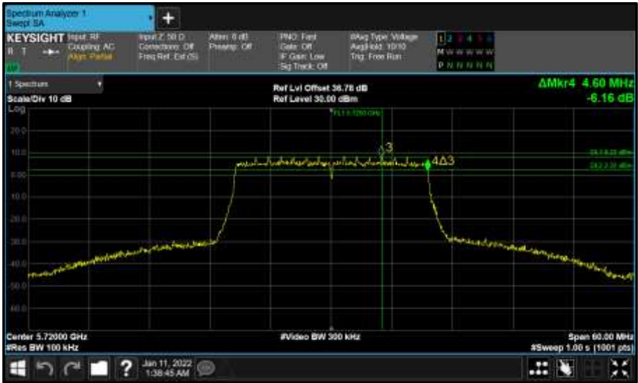
Figure 647 - Core 0 (A) 5720 MHz (CH144) 6 dB Bandwidth
