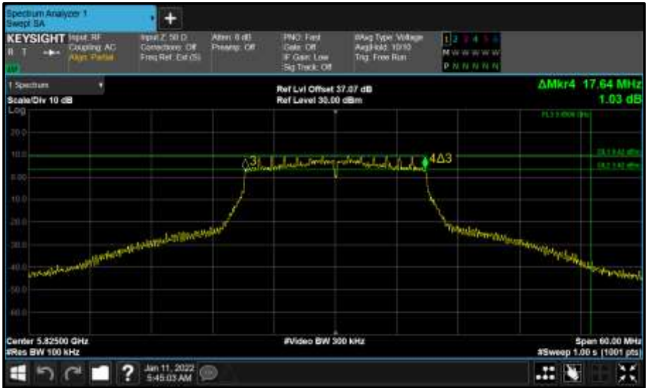
Figure 577 - Core 0 (A) 5825 MHz (CH165) 6 dB Bandwidth
