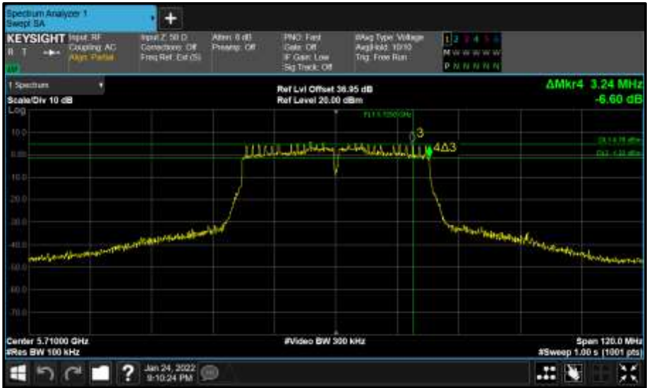
Figure 617 - Core 1 (B) 5710 MHz (CH142) 6 dB Bandwidth
