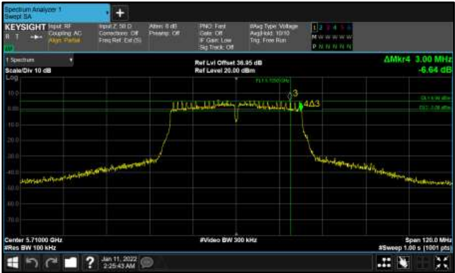
Figure 605 - Core 1 (B) 5710 MHz (CH142) 6 dB Bandwidth
