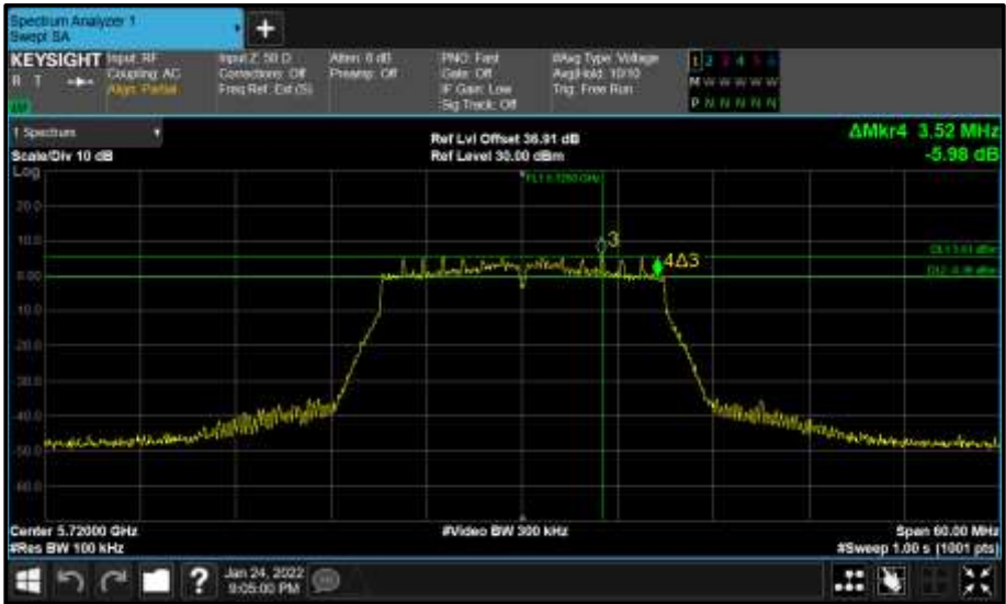
Figure 583 - Core 1 (B) 5720 MHz (CH144) 6 dB Bandwidth
