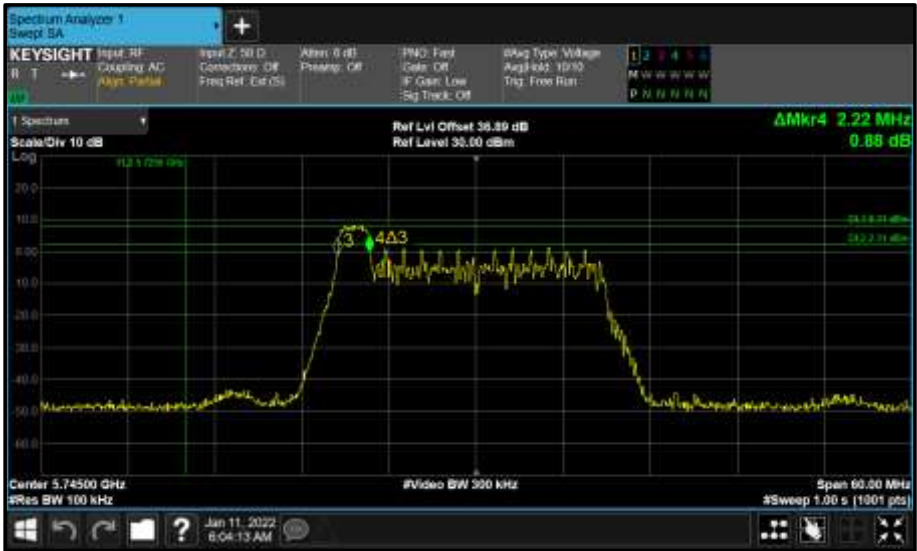
Figure 695 - Core 1 (B) 5745 MHz (CH149) 6 dB Bandwidth
