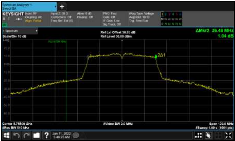
Figure 606 - Core 0 (A) 5755 MHz (CH151) 99% Bandwidth
