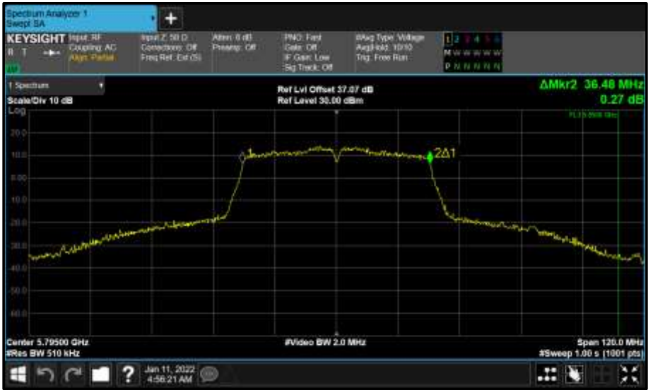
Figure 600 - Core 0 (A) 5795 MHz (CH159) 99% Bandwidth
