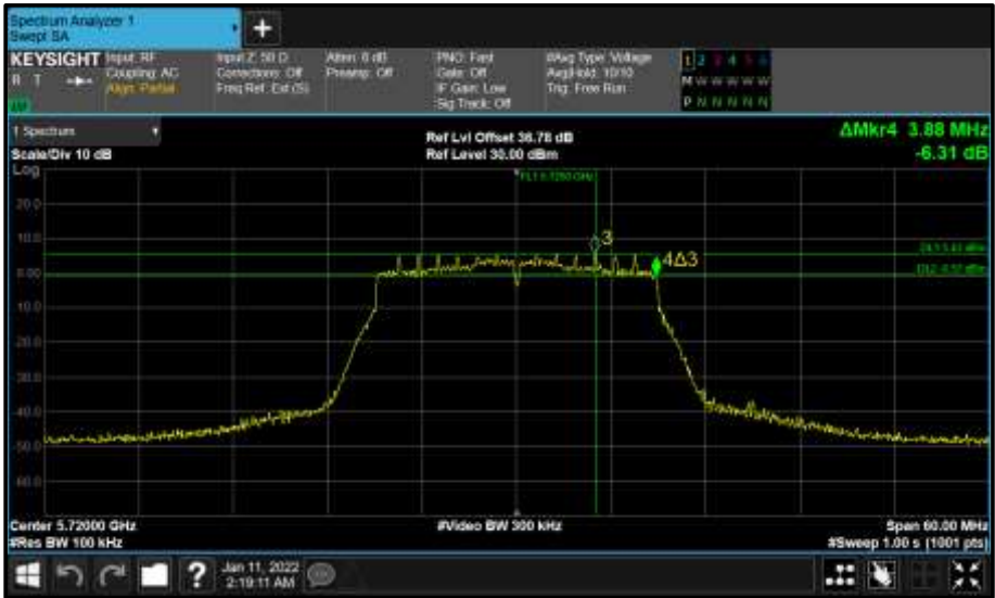
Figure 565 - Core 0 (A) 5720 MHz (CH144) 6 dB Bandwidth
