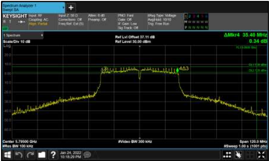
Figure 625 - Core 1 (B) 5795 MHz (CH159) 6 dB Bandwidth
