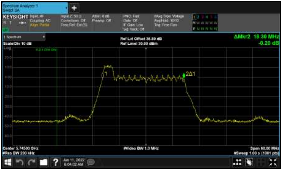
Figure 694 - Core 1 (B) 5745 MHz (CH149) 99% Bandwidth
