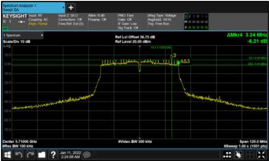
Figure 603 - Core 0 (A) 5710 MHz (CH142) 6 dB Bandwidth
