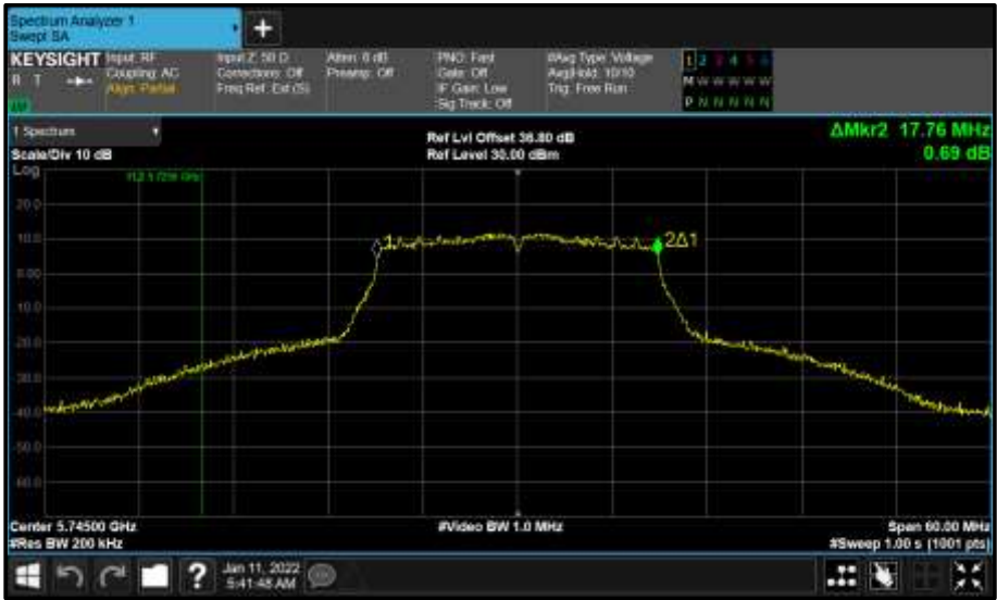
Figure 568 - Core 0 (A) 5745 MHz (CH149) 99% Bandwidth
