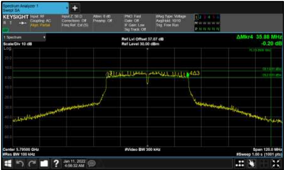
Figure 601 - Core 0 (A) 5795 MHz (CH159) 6 dB Bandwidth
