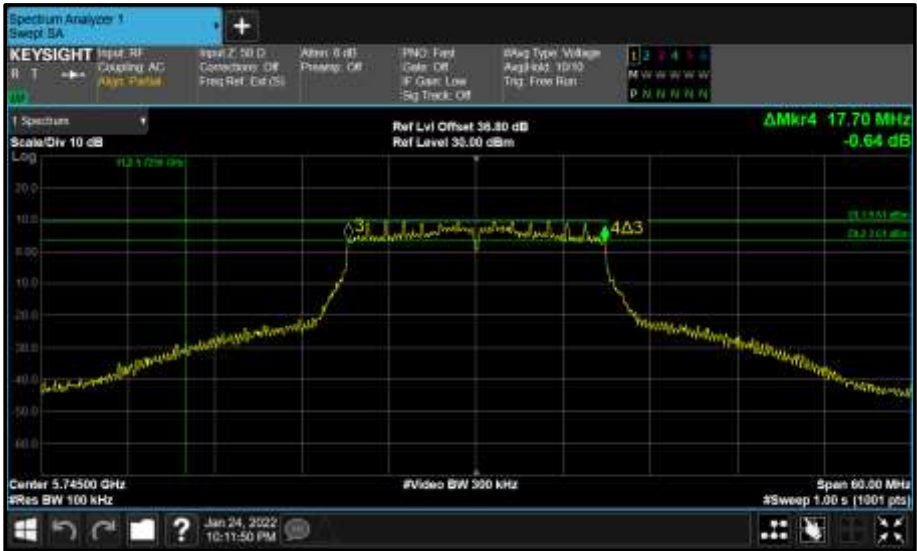
Figure 585 - Core 0 (A) 5745 MHz (CH149) 6 dB Bandwidth
