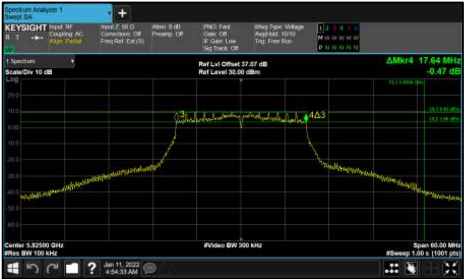
Figure 563 - Core 0 (A) 5825 MHz (CH165) 6 dB Bandwidth
