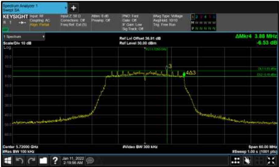
Figure 567 - Core 1 (B) 5720 MHz (CH144) 6 dB Bandwidth
