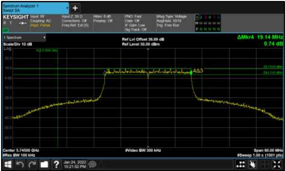
Figure 677 - Core 1 (B) 5745 MHz (CH149) 6 dB Bandwidth
