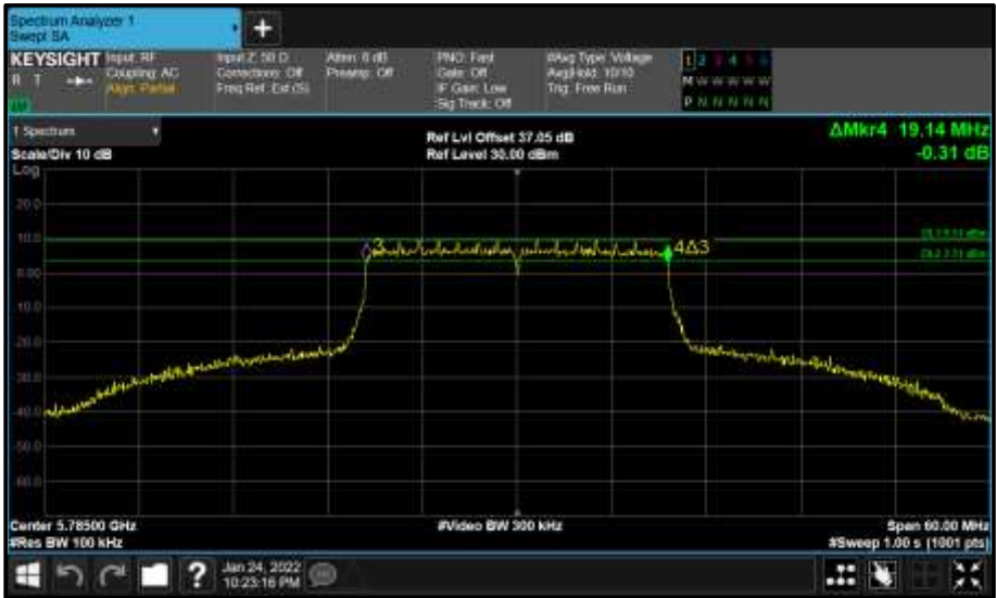
Figure 679 - Core 0 (A) 5785 MHz (CH157) 6 dB Bandwidth
