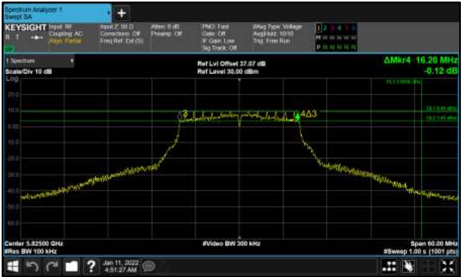
Figure 555 - Core 0 (A) 5825 MHz (CH165) 6 dB Bandwidth
