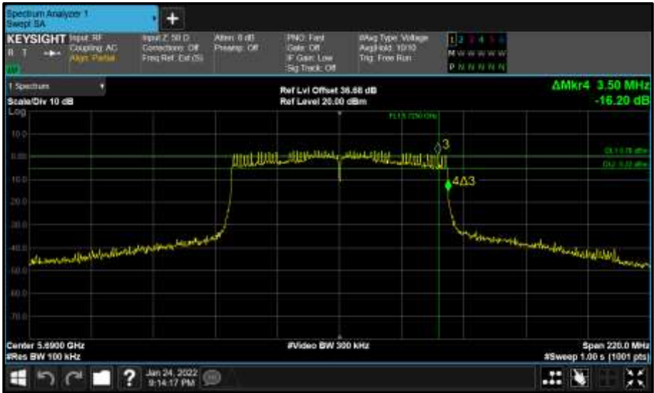
Figure 639 - Core 0 (A) 5690 MHz (CH138) 6 dB Bandwidth
