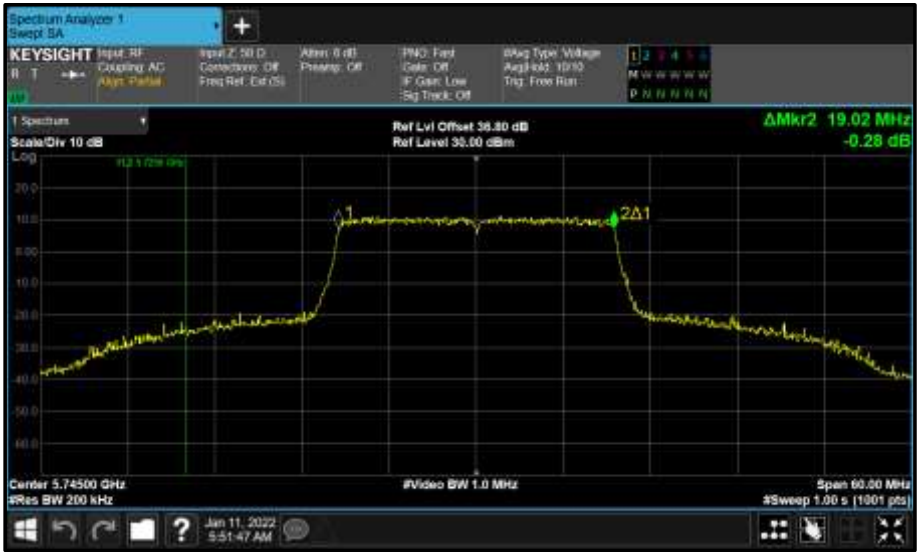
Figure 658 - Core 0 (A) 5745 MHz (CH149) 99% Bandwidth
