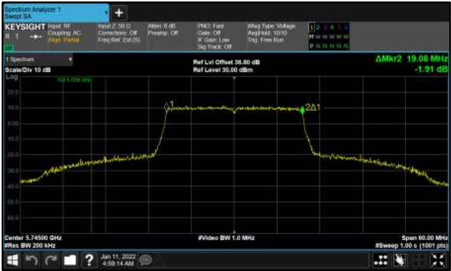
Figure 648 - Core 0 (A) 5745 MHz (CH149) 99% Bandwidth
