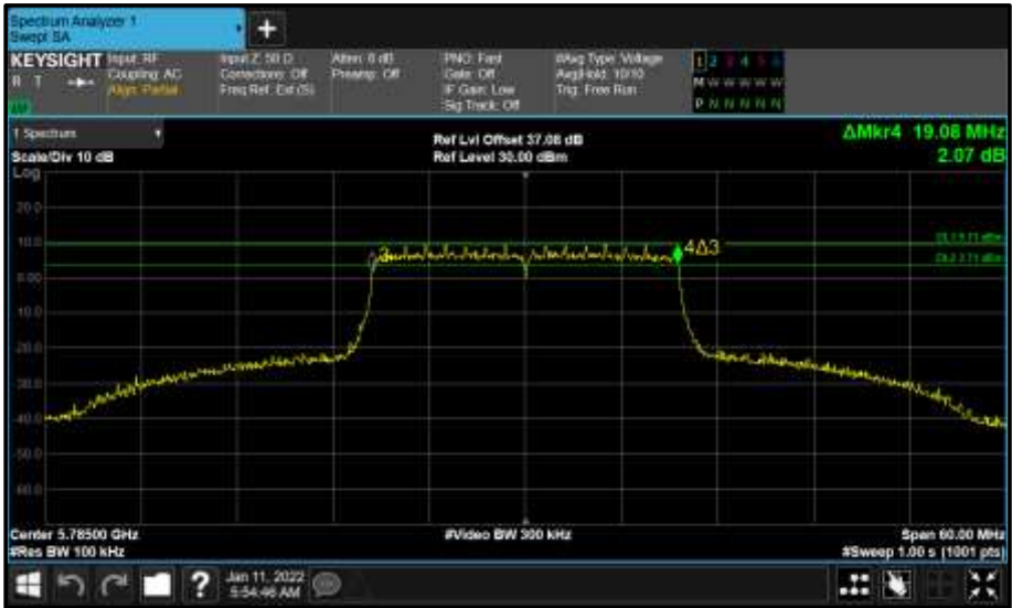
Figure 665 - Core 1 (B) 5785 MHz (CH157) 6 dB Bandwidth
