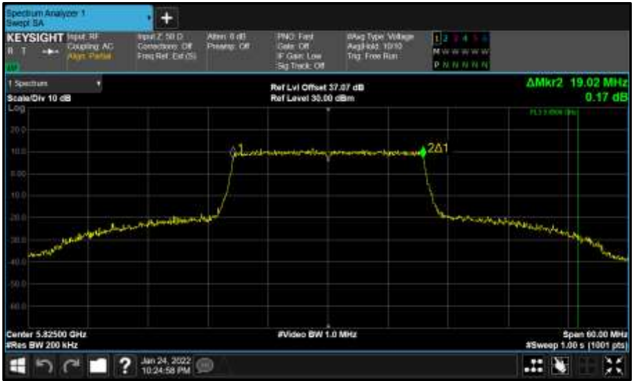
Figure 682 - Core 0 (A) 5825 MHz (CH165) 99% Bandwidth
