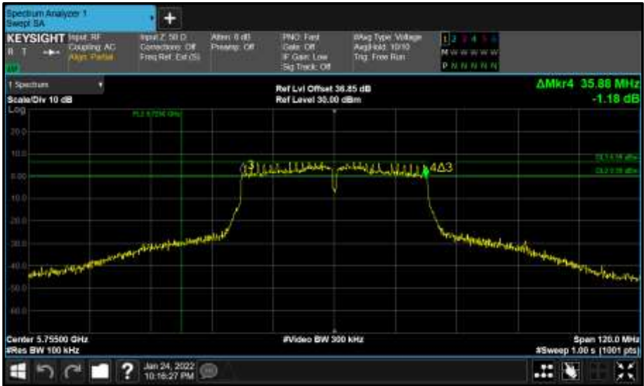
Figure 619 - Core 0 (A) 5755 MHz (CH151) 6 dB Bandwidth
