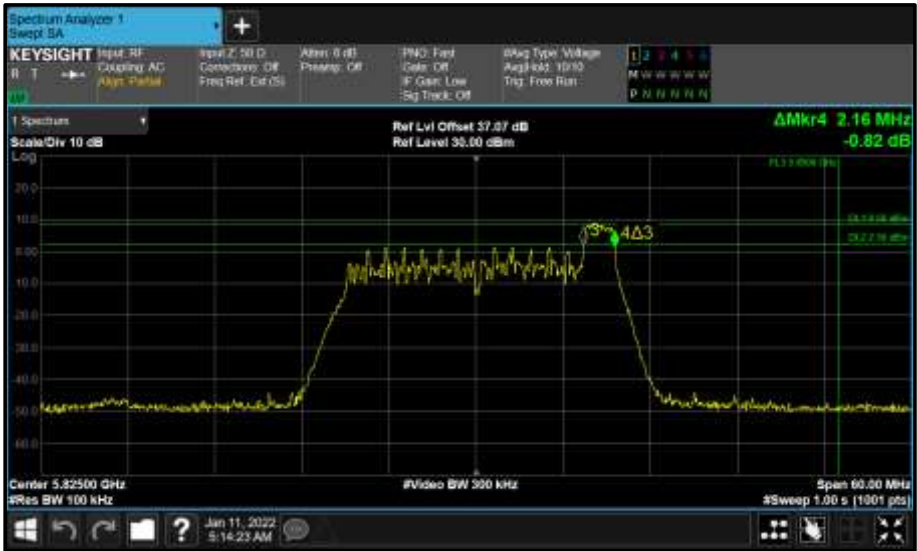
Figure 691 - Core 0 (A) 5825 MHz (CH165) 6 dB Bandwidth
