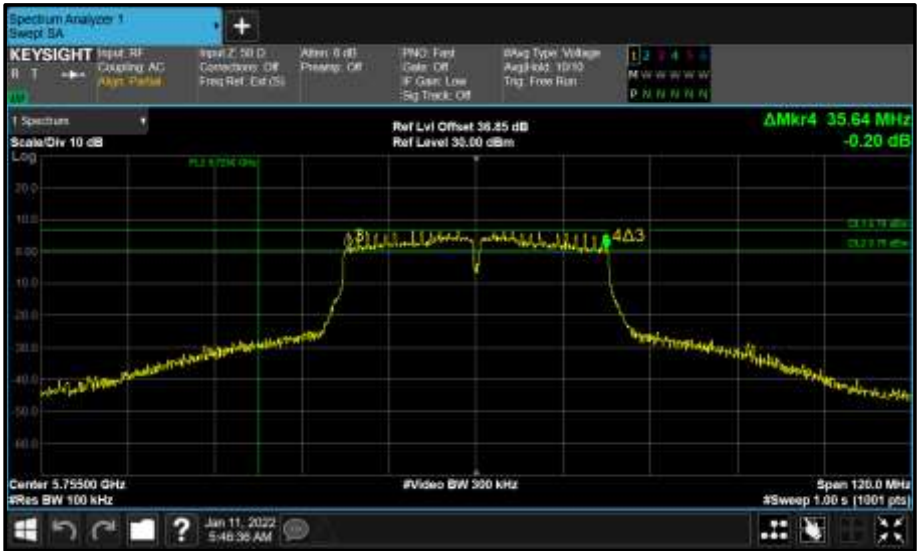
Figure 607 - Core 0 (A) 5755 MHz (CH151) 6 dB Bandwidth
