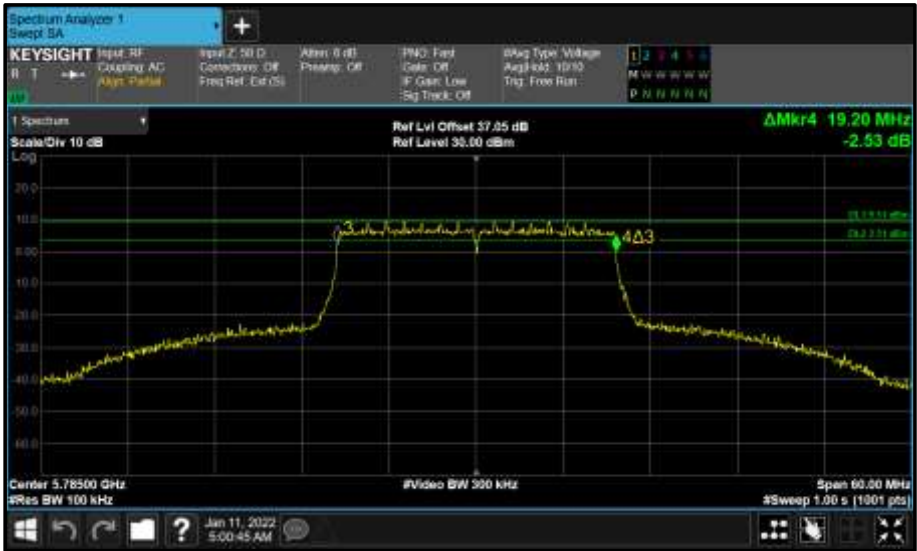
Figure 651 - Core 0 (A) 5785 MHz (CH157) 6 dB Bandwidth
