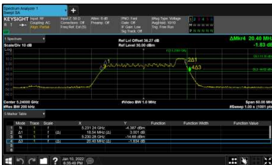
Figure 183 - Core 0 (A) 5240 MHz (CH48) 26 dB and 99% Bandwidth
