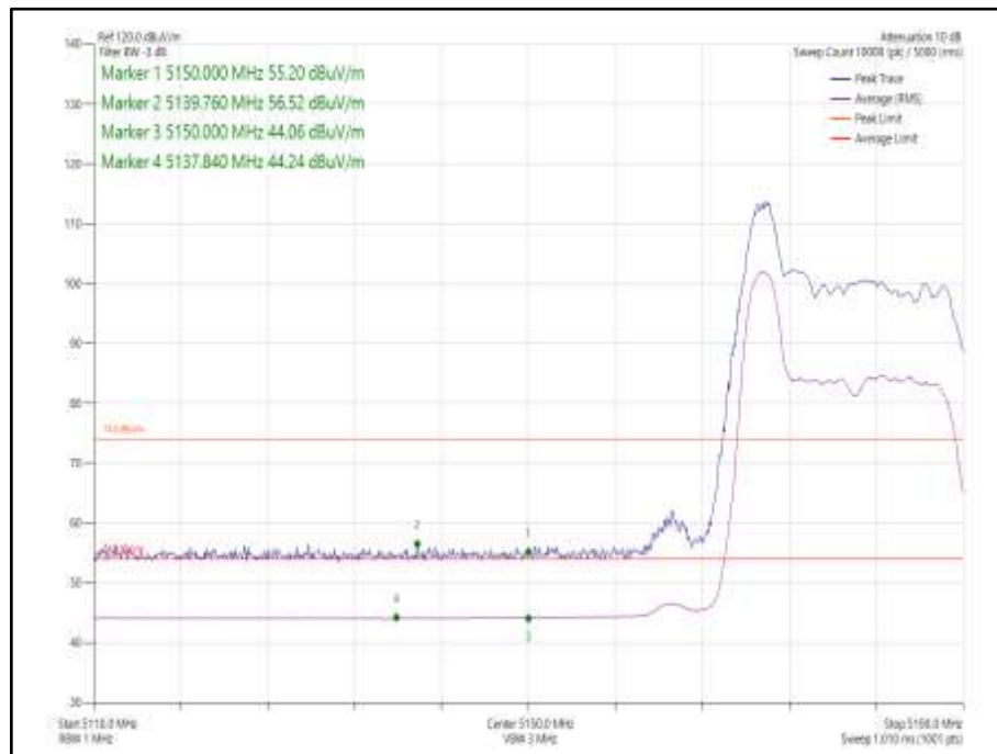
Figure 4 - 802.11ax HE20, Core 1, 26-0 - 5180 MHz, Band Edge Frequency 5150 MHz
