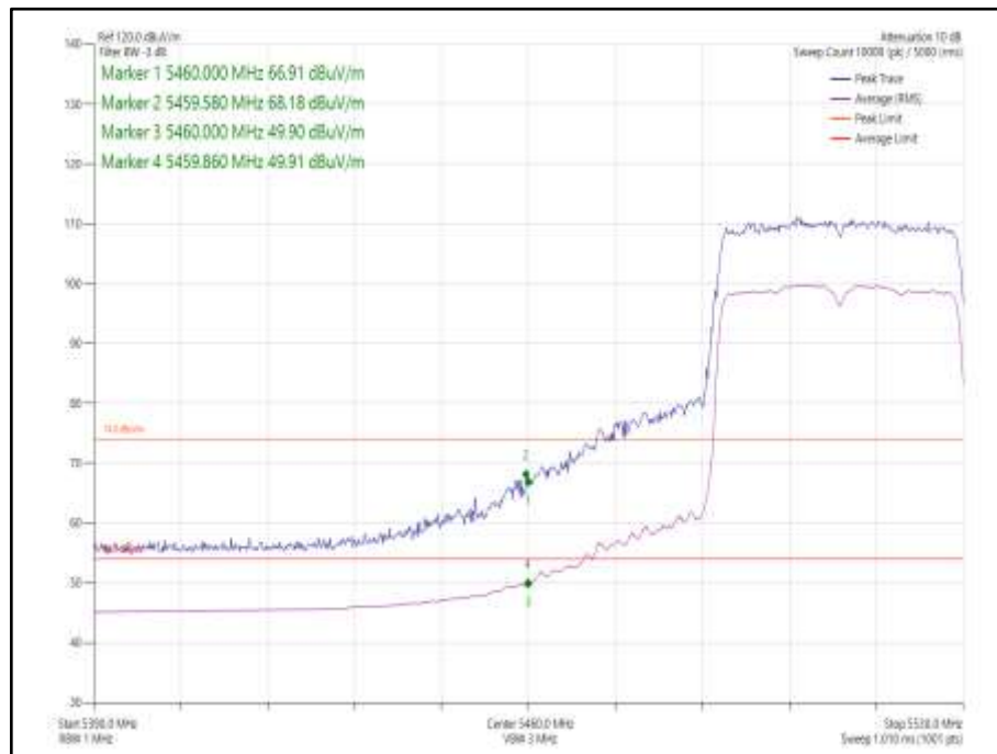
Figure 38 - 802.11ax HE40, Core 1, SU - 5510 MHz Band Edge Frequency 5460 MHz
