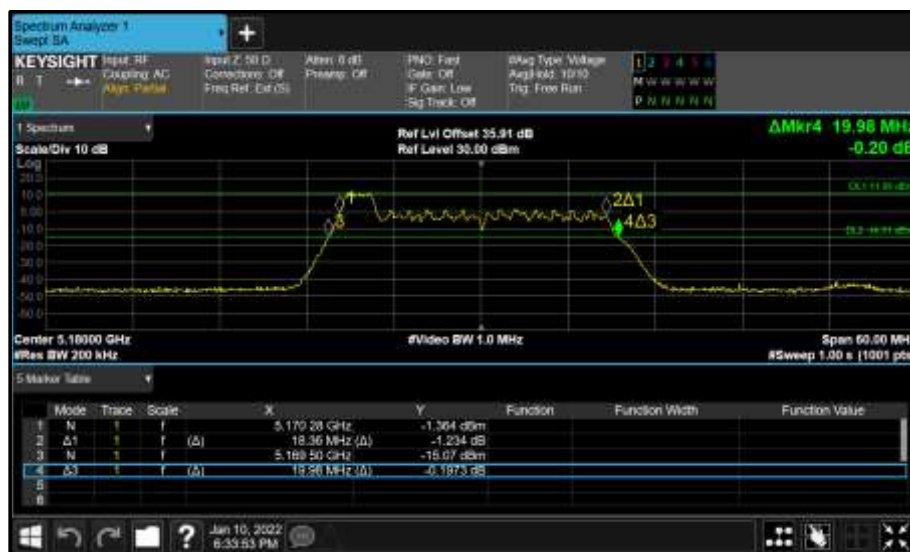
Figure 181 - Core 0 (A) 5180 MHz (CH36) 26 dB and 99% Bandwidth
