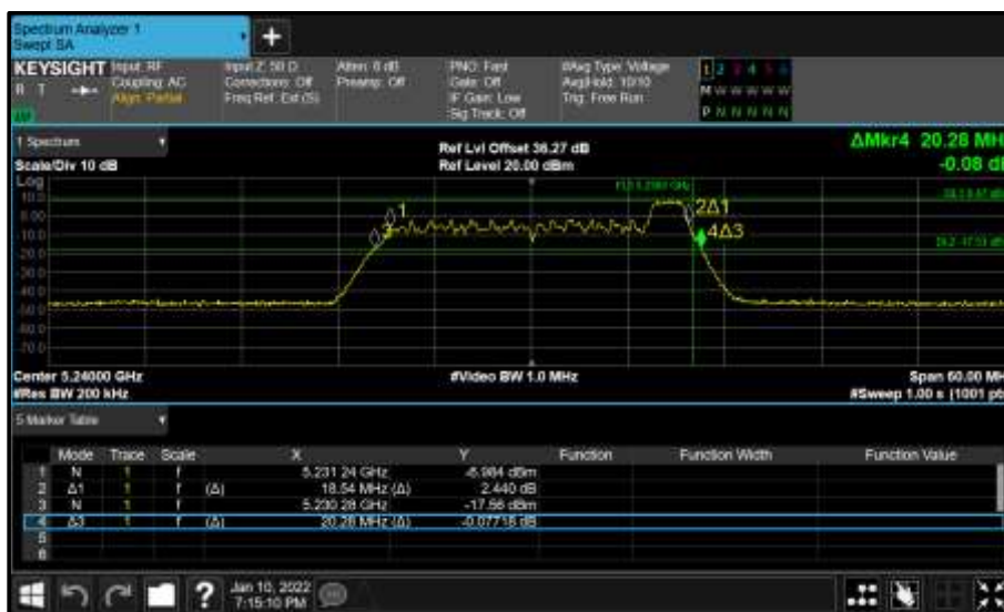
Figure 191 - Core 0 (A) 5240 MHz (CH48) 26 dB and 99% Bandwidth
