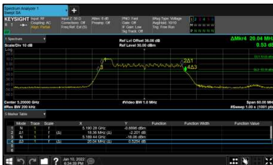
Figure 182 - Core 0 (A) 5200 MHz (CH40) 26 dB and 99% Bandwidth
